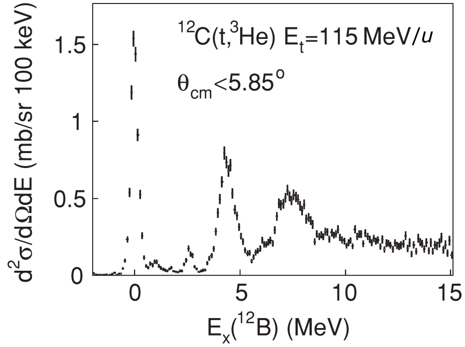
Figure 2.7 Excitation energy spectrum for the ^{12}\text{C}(t, ^3\text{He}) reaction at 115 MeV/ u . Of interest for this study is the strong peak at 0 MeV in the ^{12}\text{B} spectrum from the ^{12}\text{C}(0^+, \text{g.s.})(t, ^3\text{He})^{12}\text{B}(1^+, \text{g.s.}) . Graphic adapted from [29]
