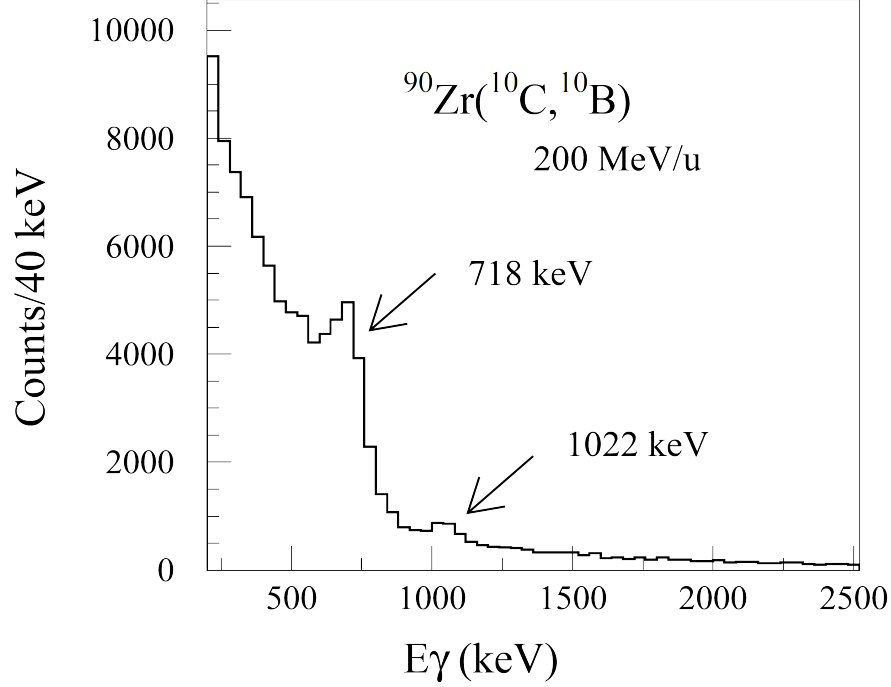
Figure 2.5 Gamma-ray spectrum with Doppler correction in the ^{90}\text{Zr}(^{10}\text{C}, ^{10}\text{B}) reaction [20].
