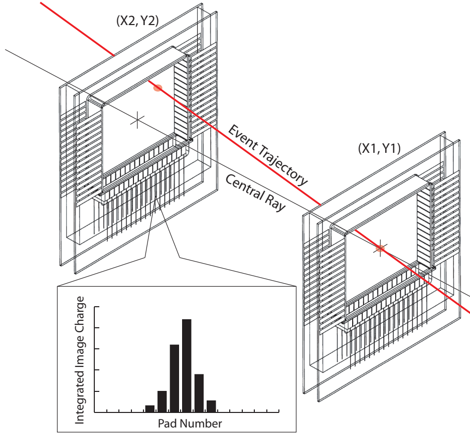
Figure 5.9 Layout of CRDC detectors and cartoon of cathode position determination. Figure taken originally from Reference [72], modified by Wes Hitt in Reference [81]
