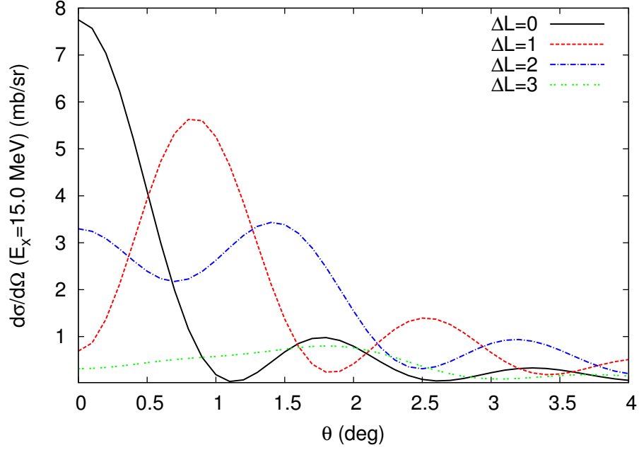
Figure 4.4 Angular distributions for ^{28}\text{Si}(^{10}\text{Be}, ^{10}\text{B})^{28}\text{Al} as calculated with FOLD, at E_X = 15.0\text{ MeV} .
