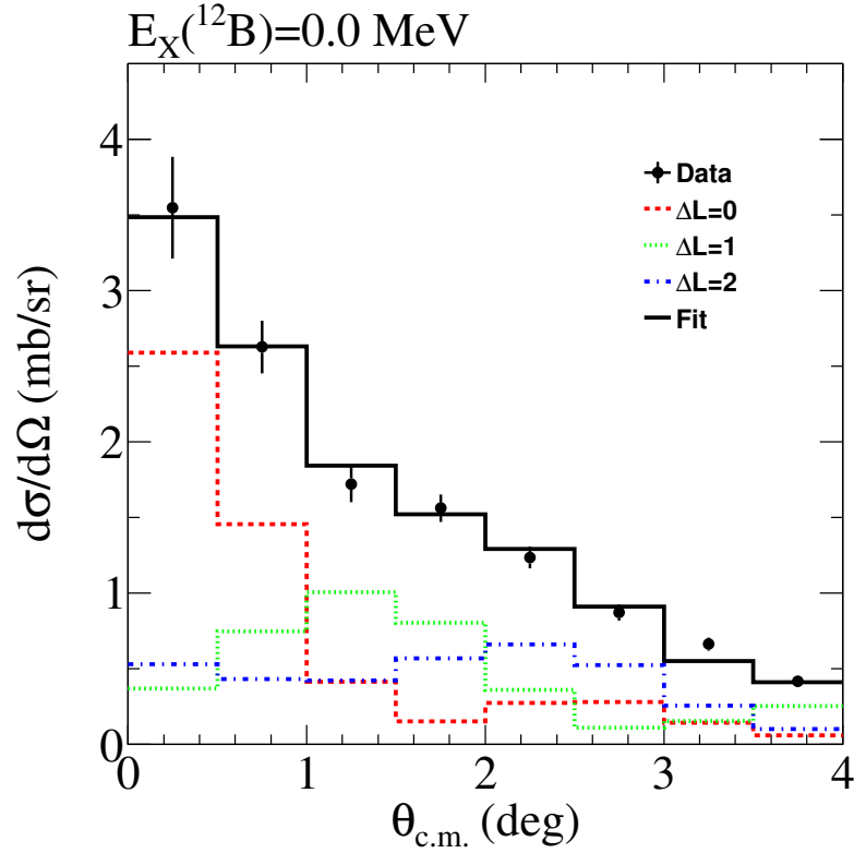
Figure 7.3 MDA of the GT ground state peak of ^{12}\text{B} in the ^{12}\text{C}(^{10}\text{Be}, ^{10}\text{B}+\gamma)^{12}\text{B} reaction. The measured angular distribution was fit with a linear combination of \Delta L = 0, 1 , and 2 theoretical angular distributions.
