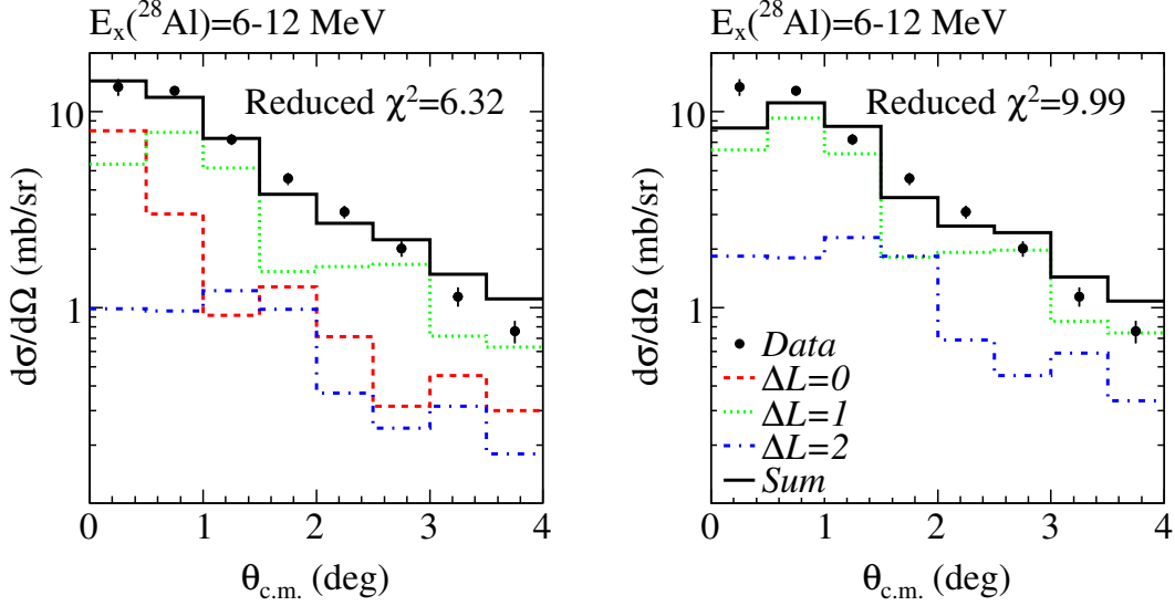
Figure 7.4 MDA of the peak region 6 < E_X(^{28}\text{Al}) \leq 12 MeV in the ^{28}\text{Si}(^{10}\text{Be}, ^{10}\text{B}+\gamma)^{28}\text{Al} reaction. (left) MDA result including the \Delta L = 0, 1 and 2 multipoles. (right) MDA fit excluding the \Delta L = 0 monopole, and only fitting with \Delta L = 1 and \Delta L = 2 , to observe the sensitivity of MDA to the monopole.
