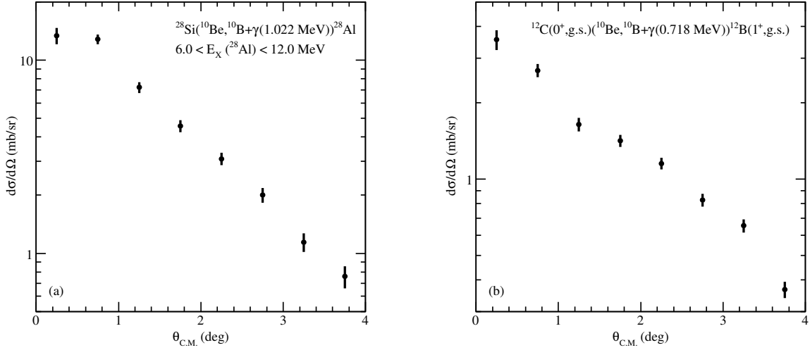
Figure 6.19 (a) Angular distribution for the ^{28}\text{Si}(^{10}\text{Be}, ^{10}\text{B} + \gamma(1.022 \text{ MeV}))^{28}\text{Al} \Delta T = 1, \Delta S = 0 reaction in the peak region of the excitation energy spectrum. (b) Angular distribution for the ^{12}\text{C}(0^+, \text{g.s.})(^{10}\text{Be}, ^{10}\text{B} + \gamma(0.718 \text{ MeV}))^{12}\text{B}(1^+, \text{g.s.}) \Delta T = 1, \Delta S = 1 reaction.
