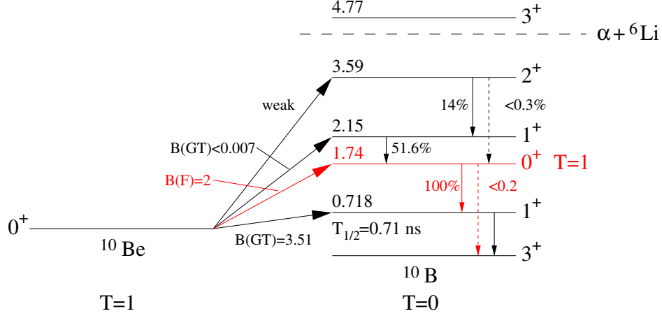
Figure 2.4 The level scheme of ^{10}\text{B} of relevance for the (^{10}\text{Be}, ^{10}\text{B} + \gamma) reaction to isolate \Delta S = 0 transitions. The ^{10}\text{Be}(0^+, T = 1, g.s.) \rightarrow ^{10}\text{B}(0^+, T = 1, 1.74 \text{ MeV}) transition is accompanied by a 1.022 MeV gamma-ray from deexcitation to the 0.718 MeV 1^+ state.
