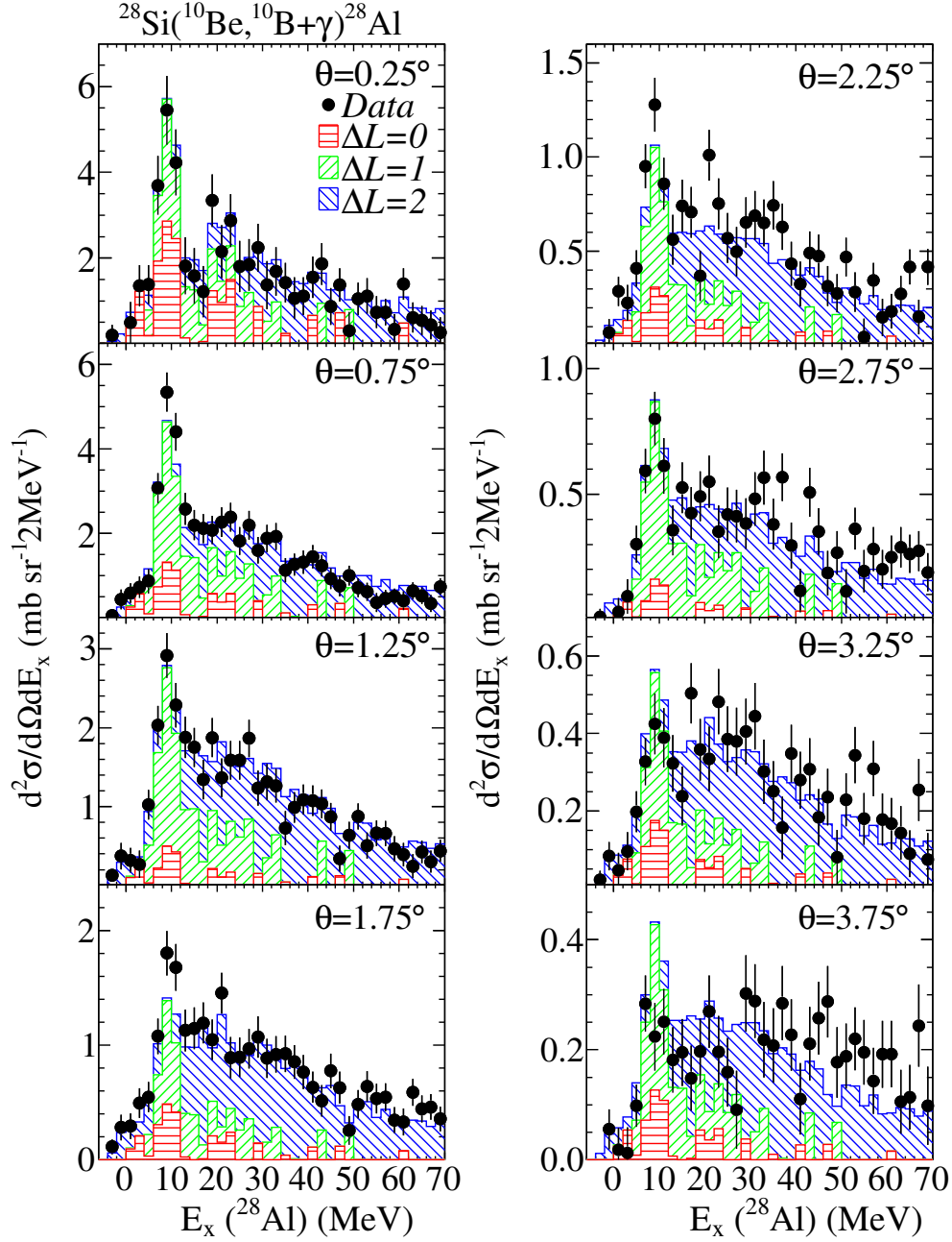
Figure 7.5 Result of the MDA presented as the double differential cross-section of the ^{28}\text{Si}(^{10}\text{Be}, ^{10}\text{B}+\gamma)^{28}\text{Al} reaction for each scattering angle bin of the angular distribution. Each 2 MeV energy bin's associated angular distribution was fit in the MDA with \Delta L = 0, 1 , and 2 theoretical angular distributions.
