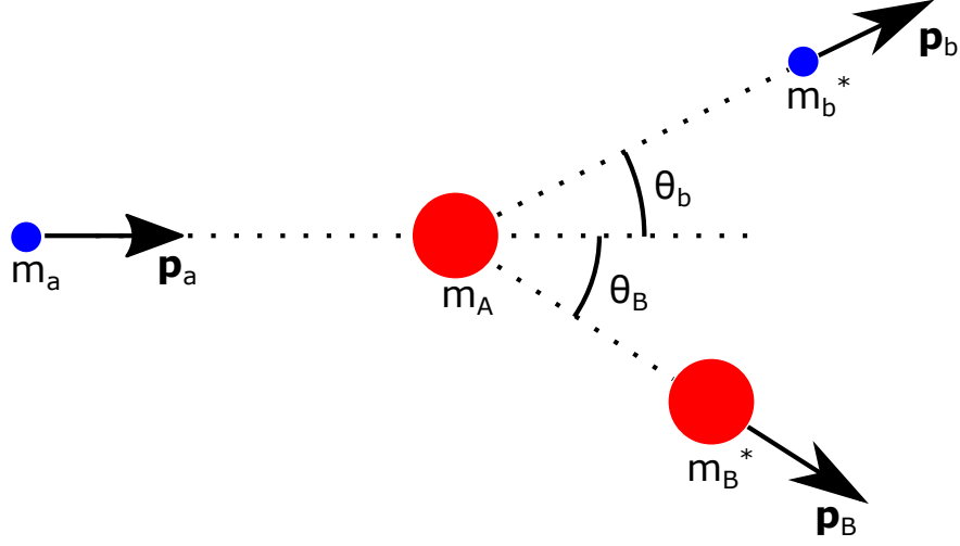
Figure 6.12 Definitions of the kinematic variables in the laboratory frame.
