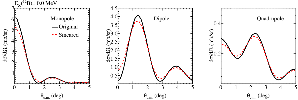
Figure 7.2 Effect of smearing the theoretically calculated angular distributions for the monopole, dipole, and quadrupole contributions to the ^{12}\text{C}(0^+, \text{g.s.})({}^{10}\text{Be}(0^+, \text{g.s.}), {}^{10}\text{B}(1^+, 0.718 \text{ MeV}))^{12}\text{B}(1^+, \text{g.s.}) reaction. Angular distributions shown are used in the MDA of the ground state peak in ^{12}\text{B} .
