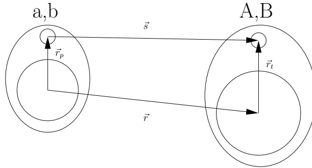
Figure 4.2 Coordinate definitions for the form factor calculation where the projectile/ejectile system is defined with a,b respectively and the target/residual system is defined with A,B respectively.
