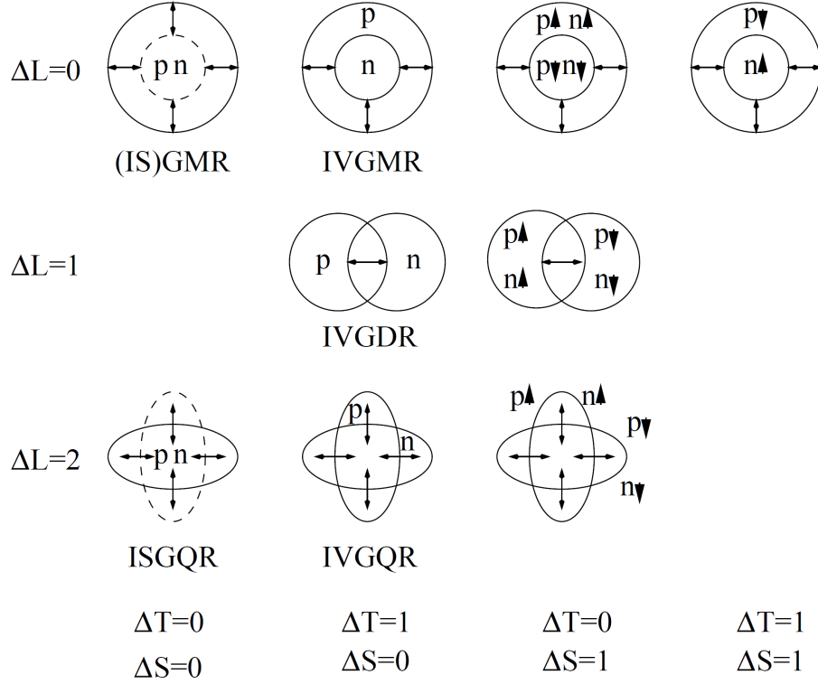
Figure 1.1 Schematic representation of various collective modes. Multipoles shown correspond to \Delta L = 0 (monopole), \Delta L = 1 (dipole), and \Delta L = 2 (quadrupole). Figure taken from [1].
