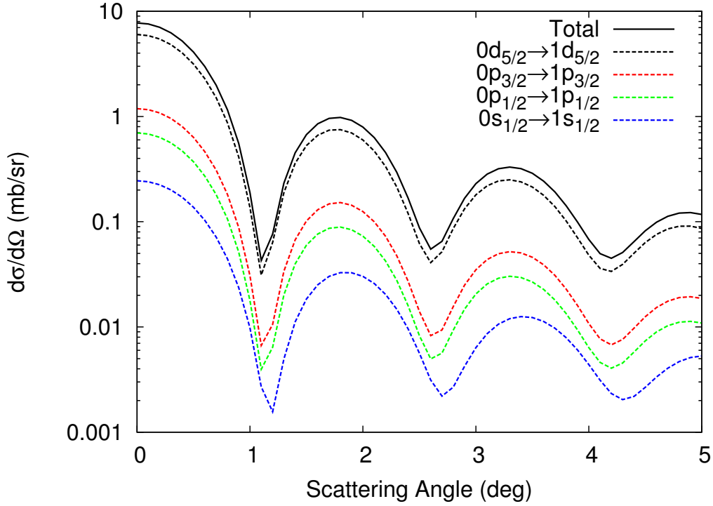
Figure 7.6 Calculated angular distributions for the IVGMR. The curve labeled total includes all single particle transitions in the excitation. Each dashed line represents only the indicated single particle transition for the IVGMR.
