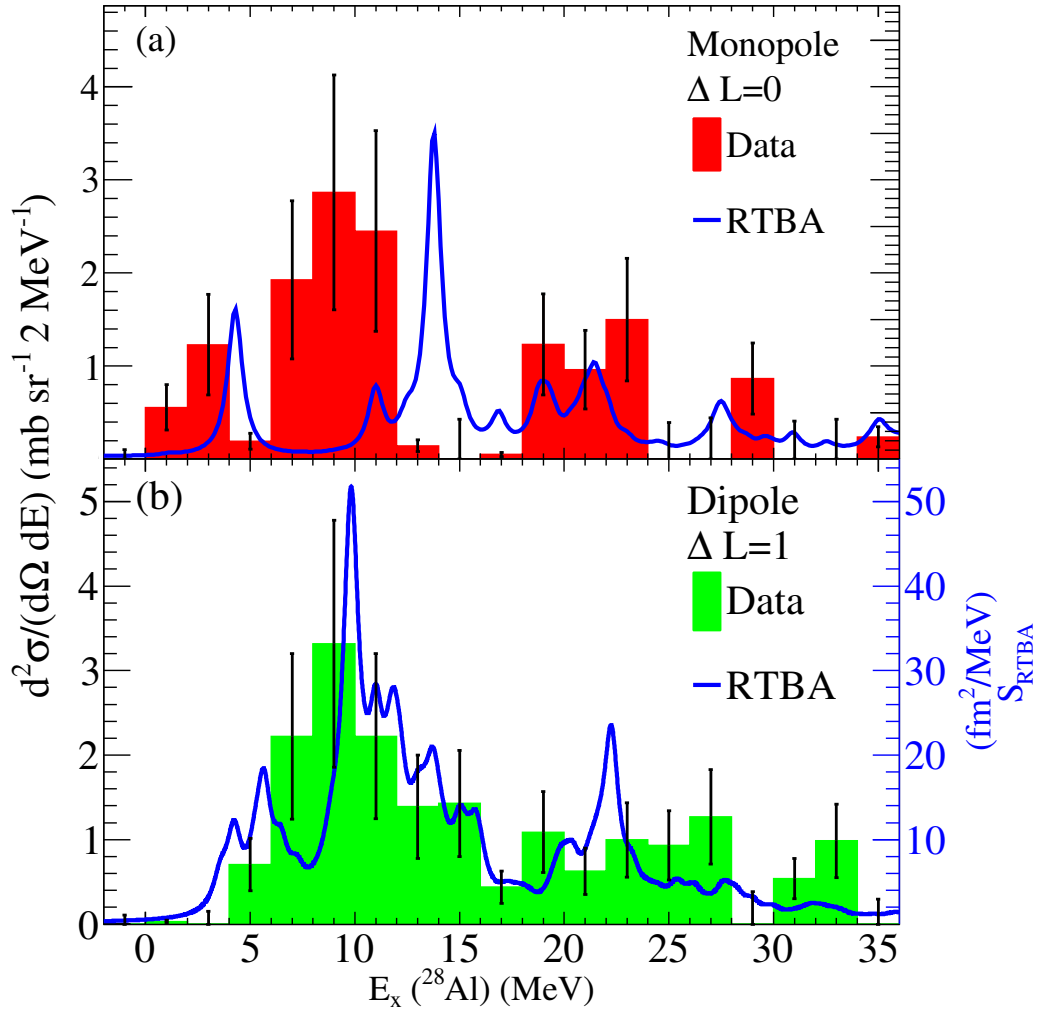
Figure 7.9 Comparison of measured \Delta L = 0 (monopole) and \Delta L = 1 (dipole) distributions with theoretical calculations from the RTBA. (a) The RTBA strength calculation has been converted into units of mb/sr/MeV. (b) The RTBA strength calculation is presented in units of \text{fm}^2/\text{MeV}
