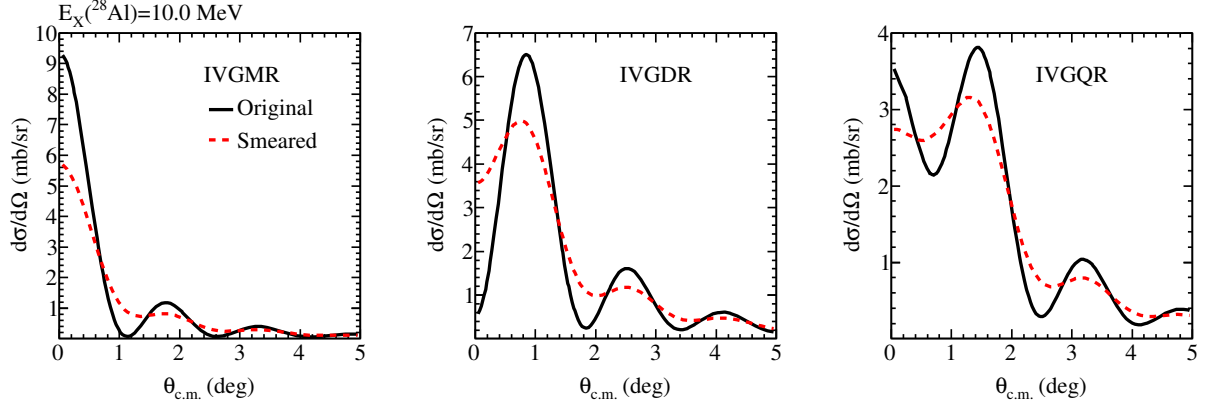
Figure 7.1 Effect of smearing the theoretically calculated angular distributions for the IVGMR, IVGDR, and IVGQR in the ^{28}\text{Si}(^{10}\text{Be}, ^{10}\text{B}(\text{IAS}))^{28}\text{Al} reaction at 10.0 MeV. Angular distributions shown are used in the MDA of the peak region of the ^{28}\text{Al} double differential cross section spectrum.
