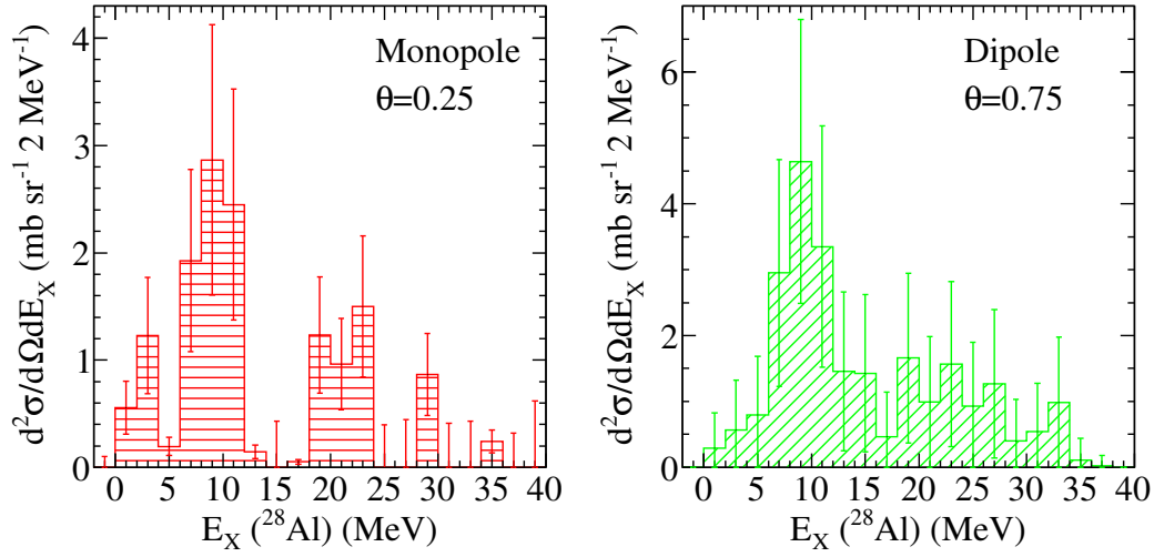
Figure 7.7 Extracted \Delta L = 0 (monopole) and \Delta L = 1 (dipole) double differential cross-sections for the ^{28}\text{Si}(^{10}\text{Be}, ^{10}\text{B} + \gamma)^{28}\text{Al} reaction. Distributions are shown for the experimental angular bin in which the angular distribution peaks.
