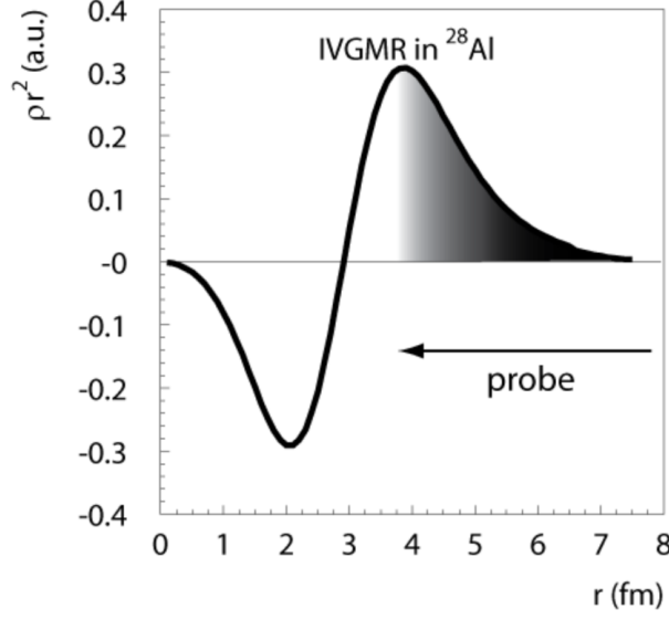
Figure 2.2 Transition density multiplied by r^2 for excitation of the IVGMR in ^{28}\text{Al} from ^{28}\text{Si} . Probing the IVGMR is preferably done using a probe that is strongly absorbed at the surface (as schematically indicated by the shaded area), to avoid the cancellation of the transition strengths due to the exterior and interior components of the transition density.
