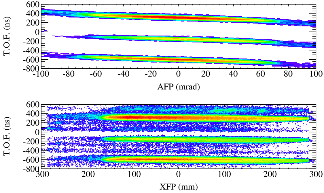
Figure 6.10 Correlation between ToF and the dispersive direction coordinates afp, xfp
