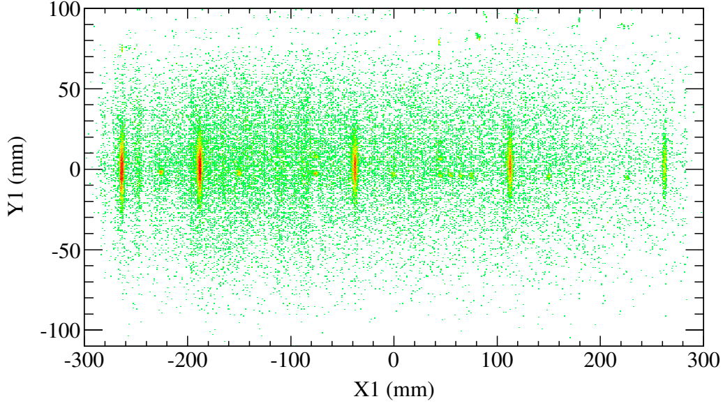
Figure 6.2 Sample spectrum of CRDC1. Calibration is complete in spectrum.
