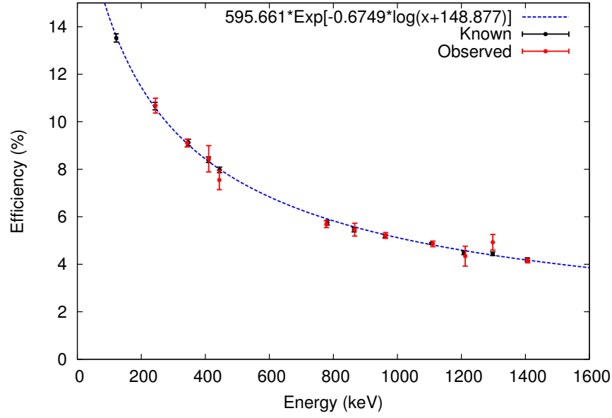
Figure 6.5 GRETINA efficiency as measured by ^{152}\text{Eu} . Observed values are from data taken during experimental run for comparison with reported efficiencies. The line is fit to the known data.
