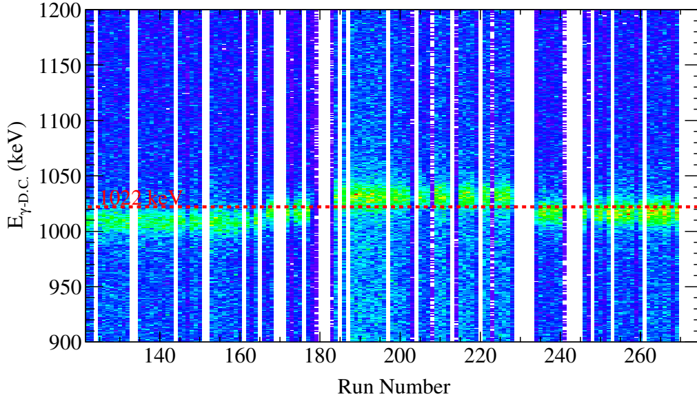
Figure 6.7 Observed energy shift of Doppler corrected 1022 keV gamma-ray due to target placement inaccuracies. Shifts above and below known energy are a result of the target placement upstream or downstream, respectively, of the assumed target location.
