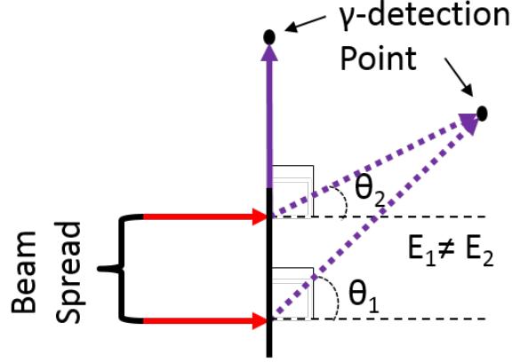
Figure 5.14 Cartoon depiction of angular uncertainty for forward angled detectors due to large beam spot as a result of dispersion matching. Image not drawn to scale.
