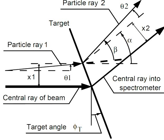
Figure 5.7 Schematic layout of the incident particle 1 and the outgoing particle 2 relative to the beam and spectrometer. Taken from Reference [77].
