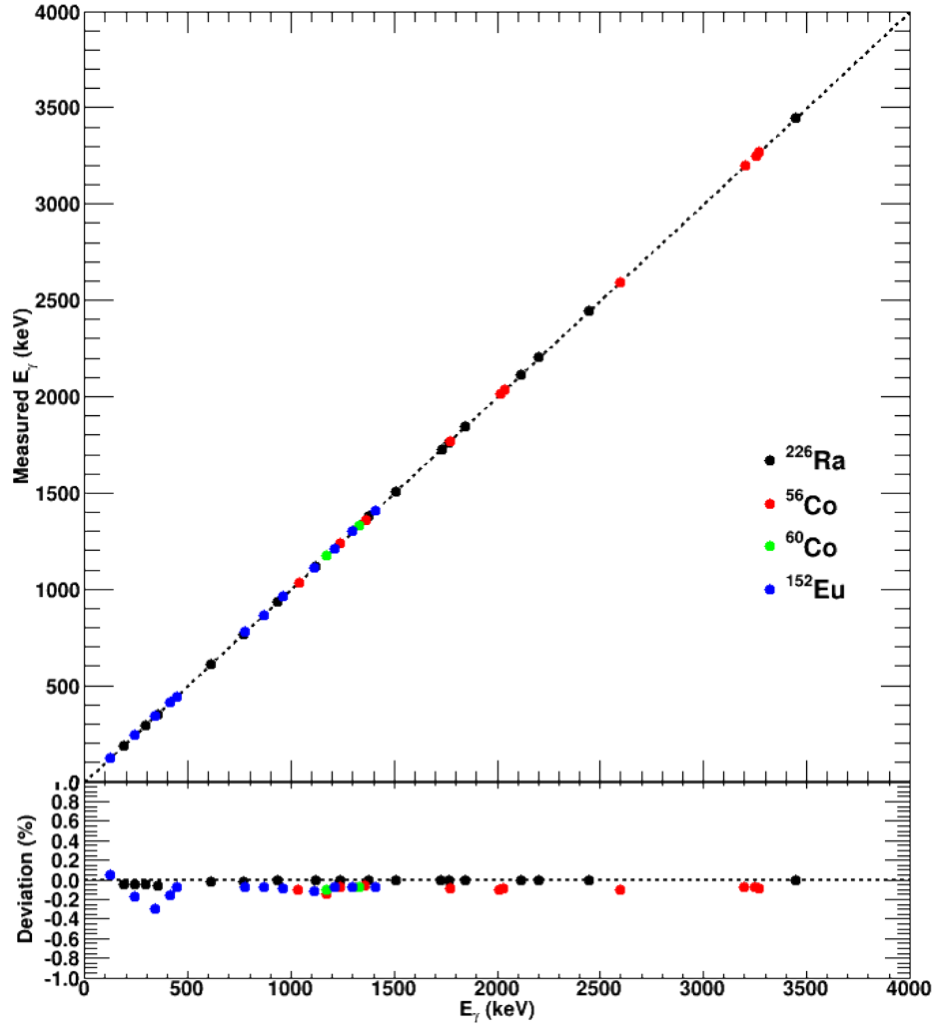
Figure 6.4 Comparison of known and measured peak energies for gamma sources ^{56}\text{Co} , ^{60}\text{Co} , ^{226}\text{Ra} , and ^{152}\text{Eu} .
