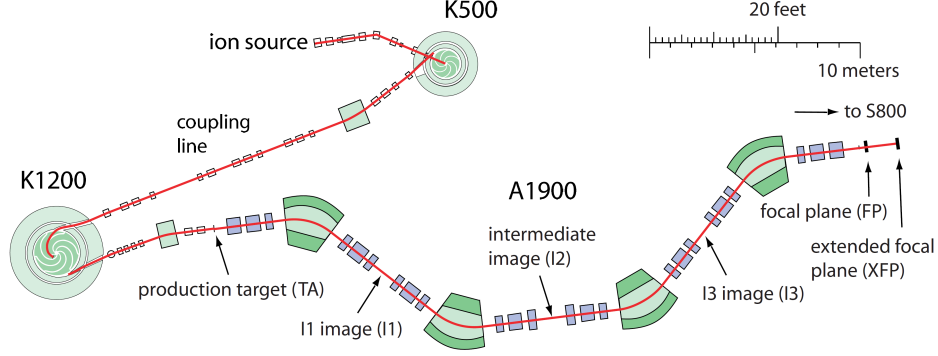
Figure 5.1 Schematic overview of the coupled K500 and K1200 cyclotrons and the A1900 Fragment Separator
