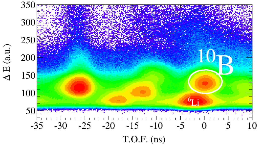
Figure 6.11 PID indicating ^{10}\text{B} particles. Figure includes corrections to the time-of-flight spectrum.
