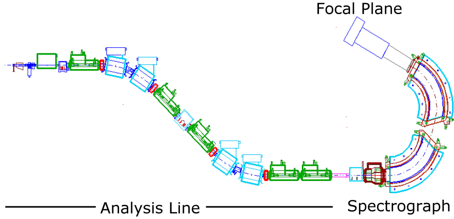
Figure 5.3 Schematic depicting analysis line and spectrograph components of the S800 Spectrograph
