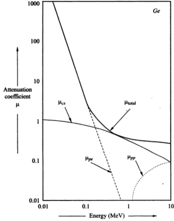
Figure 5.11 Linear attenuation coefficient as a function of photon energy in germanium. The components for the photoelectric absorption, Compton scattering, and pair production are shown as well as the total sum \mu_{total} . Figure taken from Reference [83]
