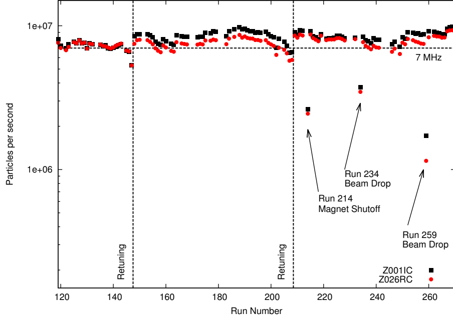
Figure 5.2 Incoming beam rate of ^{10}\text{Be} as measured by the non-intercepting probe Z001IC and the Faraday bar Z026RC. Cause for outliers from the trend are indicated with arrows. Also noted are when the beam was returned.
