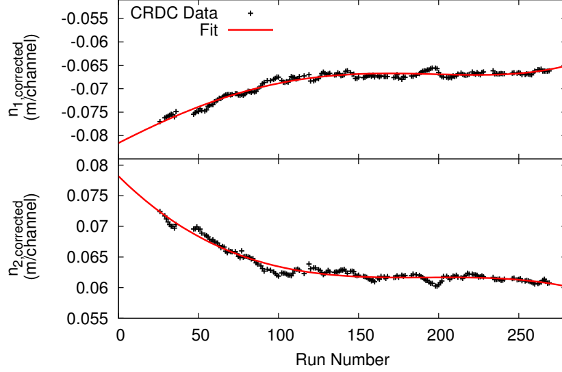
Figure 6.3 Polynomial fit of CRDC TAC data to track changes in electron drift velocity in the CRDC fill gas.
