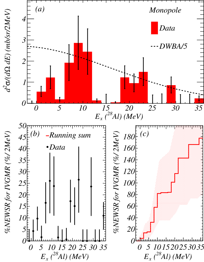
Figure 7.10 (a) Extracted monopole distribution at \theta_{com} = 0.25^\circ . The filled histogram represents the data. The dashed line is the calculated DWBA cross-section for the IVGMR as a function of excitation energy. The structural input to the theoretical angular distributions for the ^{28}\text{Si} \rightarrow ^{28}\text{Al} IVGMR came from the normal-modes calculation as described in Section 4.3.2.2. (b) Exhaustion of the NEWSR for the IVGMR for each energy bin of the extracted data. (c) Running total of the exhaustion of the NEWSR from (b).
