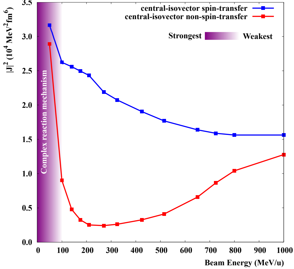
Figure 4.3 Energy dependence of the central components of the effective interaction. The square volume integrals |J|^2 are square amplitudes for the the t-matrix representing the transition between final and initial states, from [65]. Shading schematically representing the transition from complex reaction mechanisms to single-step reactions at 100 MeV/u is described in [18].
