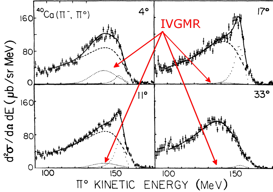
Figure 2.3 Previous experiment for ^{40}\text{Ca} using the pion charge exchange reaction [10]. The peak representing the IVGMR is indicated. To the right of the IVGMR is a peak representing the IVGDR. The IVGMR is covered by the background component, drawn with dashed lines. The three curves were fit to the data for extraction of the IVGMR.
