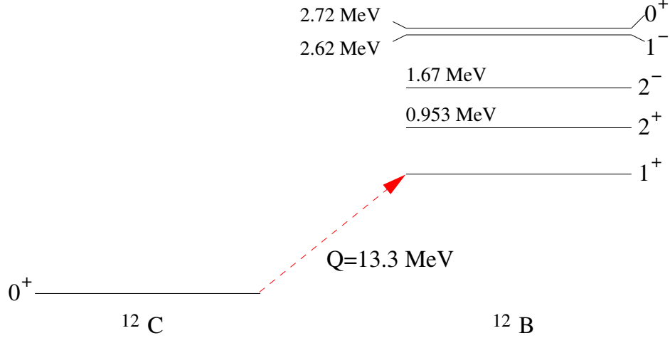
Figure 2.6 The level scheme of the ^{12}\text{B} of relevance to the (^{10}\text{Be}, ^{10}\text{B} + \gamma) reaction. Highlighted by the red, dashed arrow is the ^{12}\text{C}(0^+, \text{g.s.}) \rightarrow ^{12}\text{B}(1^+, \text{g.s.}) transition. States in ^{10}\text{B} up to 2.72 MeV are also listed.
