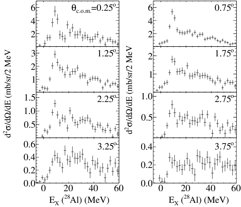
Figure 6.20 Double differential cross section for the ^{28}\text{Si}(^{10}\text{Be}, ^{10}\text{B})^{28}\text{Al} reaction, divided into angular bins. Uncertainties represented are statistical.
