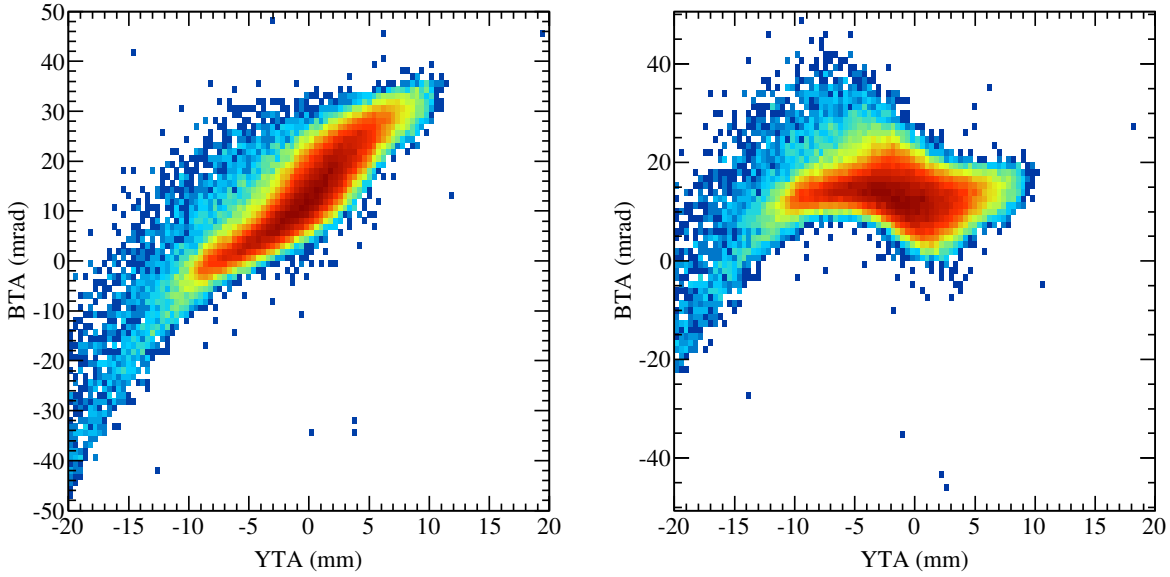
Figure 5.10 (Left) Effect of introduction of correlation in non-dispersive coordinates YTA and BTA through defocusing of the beam. (Right) Result of polynomial fit to correlation in YTA and BTA
