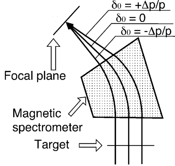
Figure 5.8 Cartoon depiction of lateral dispersion-matching, adapted from Reference [77]. Dispersion of rays with different momenta is compensated by the dispersion of the spectrometer.
