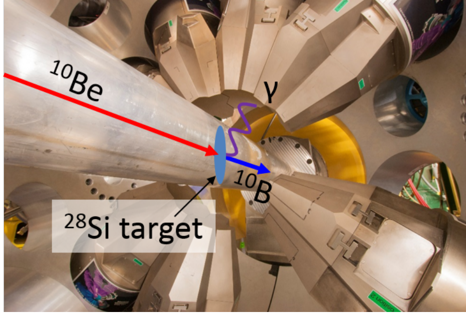
Figure 5.13 Experimental setup of the GRETINA detector array with all 7 detectors placed in their 90^\circ location surrounding the S800 spectrograph target position. Cartoon representations of the reaction of interest are drawn on the photograph. Photograph taken by Shumpei Noji.
