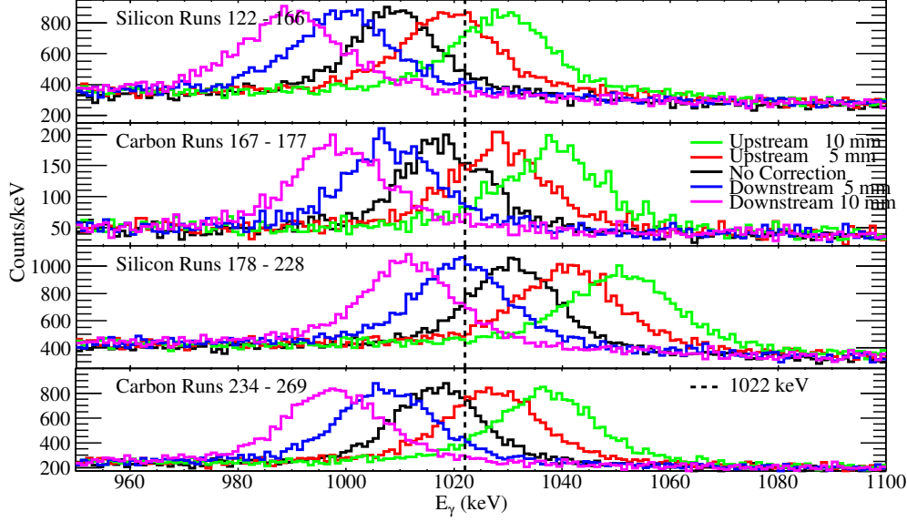
Figure 6.8 Effect of target placement on Doppler-correction of 1022 keV gamma-ray.
