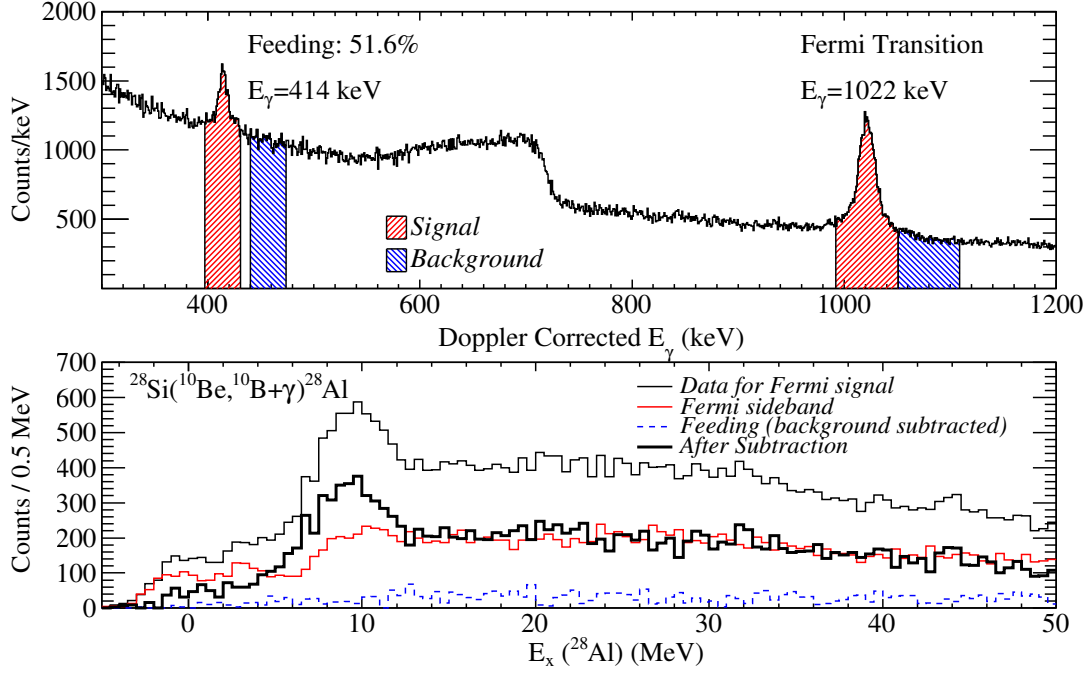
Figure 6.16 (Top) Doppler-corrected gamma-ray spectrum. Indicated are the 1022 keV Fermi transition of interest and the 414 keV GT transition that feeds into this state. Also shown is the signal, along with the side-band used for background subtraction. The gamma data in this figure is the same as in Figure 6.15, but now different regions are highlighted. (Bottom) Excitation energy spectrum of ^{28}\text{Al} for the ^{28}\text{Al}(^{10}\text{Be}, ^{10}\text{B} + \gamma)^{28}\text{Al} reaction. The thick black line is the result of subtraction of background and feeding in the coincidence data.
