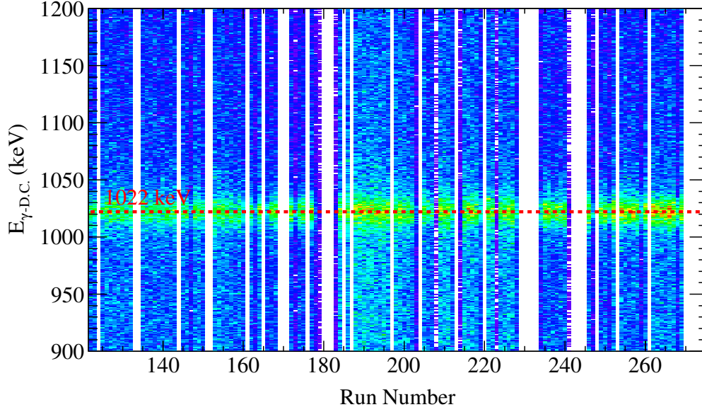
Figure 6.9 Target holder position corrected spectrum for the 1022 keV Doppler-corrected gamma-ray.
