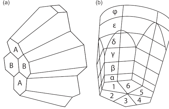
Figure 5.12 Schematic drawing of (a) four crystals packed into one module, two A-type crystals and two B-type crystals and (b) an individual crystal showing the electrical segmentation of its outer contact. Figure from Reference [73]
