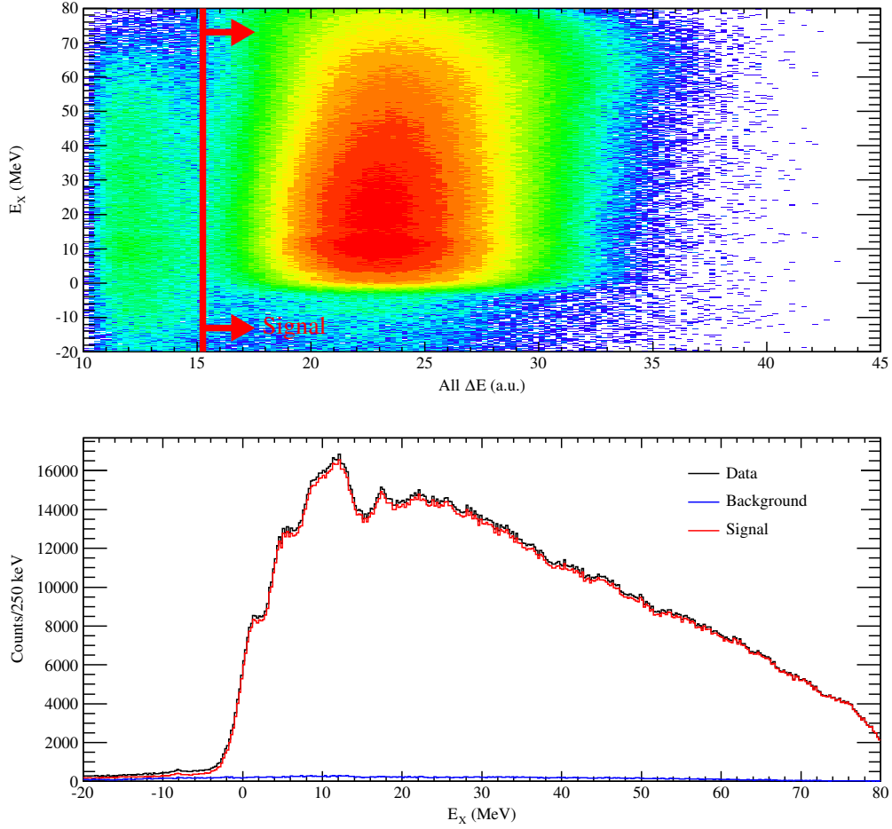
Figure 6.14 (Top) “All \Delta E ” as described in the text plotted as a function of ^{10}\text{B} excitation energy. A division between good events and background contamination is visible. The red line shows the “All \Delta E ” threshold of 15.25 in arbitrary units. (Below) Background subtracted excitation energy spectrum of ^{28}\text{Al} .
