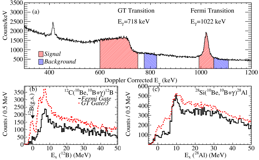
Figure 6.15 (a) Doppler-corrected gamma-ray spectrum. Indicated are the GT and F transitions, which indicate \Delta S = 1 and \Delta S = 0 reactions, respectively. Also shown is the signal, along with the side-band used for background subtraction. (b) Excitation energy spectrum of 12 B for the 12 C( 10 Be, 10 B+γ) 12 B reaction. Shown are background subtracted results for \Delta S = 0 reactions in black and \Delta S = 1 reactions in red. (c) Similar to (b), but for the 28 Al( 10 Be, 10 B+γ) 28 Al reaction.
