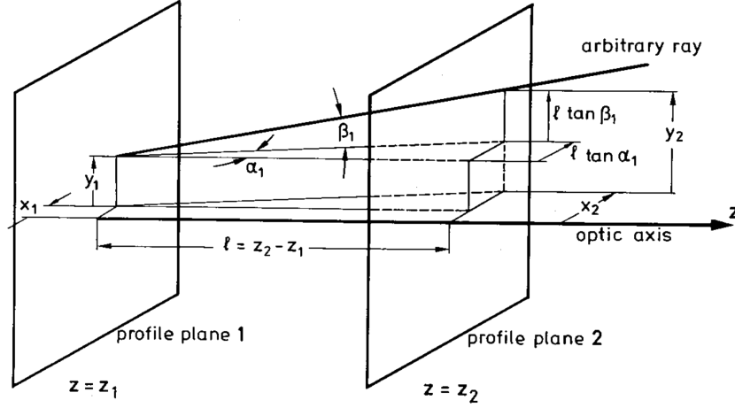
Figure 5.6 Deviations of a particle from the optic axis in a drift length l = z_2 - z_1 . Taken from Reference [75].
