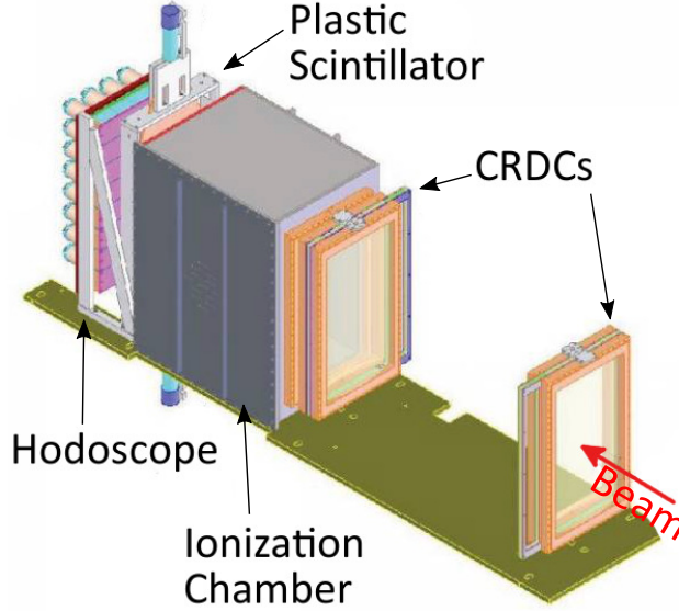
Figure 5.5 Schematic depicting the S800 focal plane detector suite. The Hodoscope was not utilized in this study [74].
