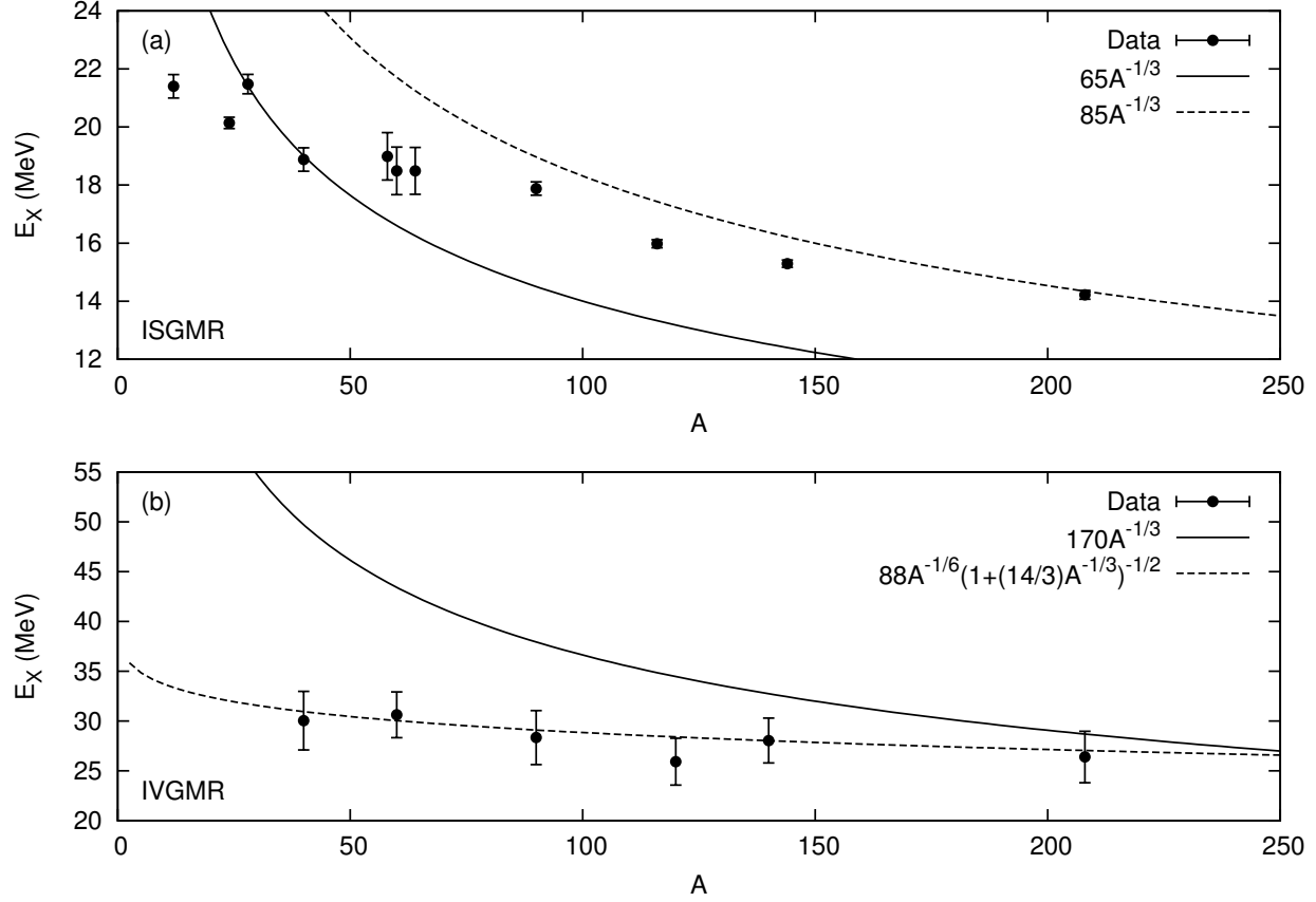
Figure 3.1 (a) Data obtained for the ISGMR via inelastic scattering of \alpha particles at small angles from Reference [32]. The solid line represents the location of the ISGMR as a function of mass ( A ) from Reference [30], and the dashed line represents an improvement from to the estimate with better knowledge of the nuclear incompressibility term from References [8, 9]. (b) Data obtained for the IVGMR from pion scattering from References [10, 11]. The solid line represents an initial estimate from the hydrodynamical model, and the dashed line represents the improvements to the model when including surface effects [33].
