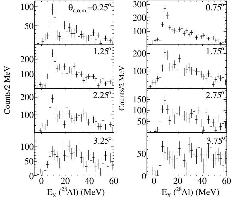
Figure 6.18 Excitation energy spectrum divided into angular bins used in cross-section calculation for the ^{28}\text{Si}(^{10}\text{Be}, ^{10}\text{B} + \gamma(1.022 \text{ MeV}))^{28}\text{Al} reaction for \Delta S = 0 reactions. Uncertainties represented are statistical.
