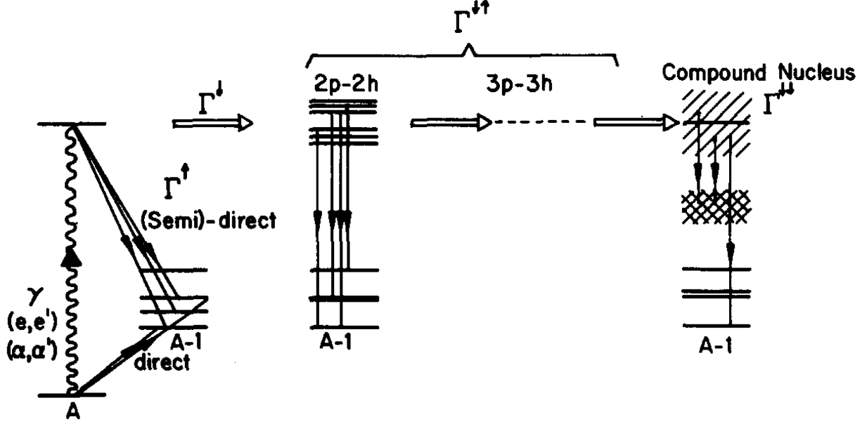
Figure 3.2 Schematic representation of the width of the collective 1p-1h state into a direct component \Gamma^\uparrow and a spreading component \Gamma^\downarrow . The spreading component can be further broken into terms describing statistical decay of the equilibrium compound nucleus \Gamma^\downarrow\downarrow and decay of the intermediate, pre-equilibrium states \Gamma^\uparrow\downarrow . Figure reproduced from [40].
