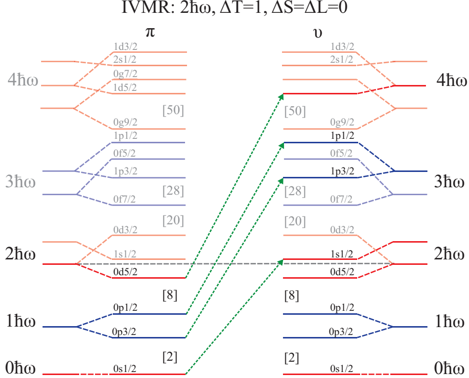
Figure 2.1 Illustrations of particle-hole contributions to the IVGMR in the ^{28}\text{Si} \rightarrow ^{28}\text{Al} system. The horizontal gray dashed line represents the Fermi level, up to which the particles fill the ground state. The IVGMR is a coherent superposition of the excitations highlighted with green arrows.
