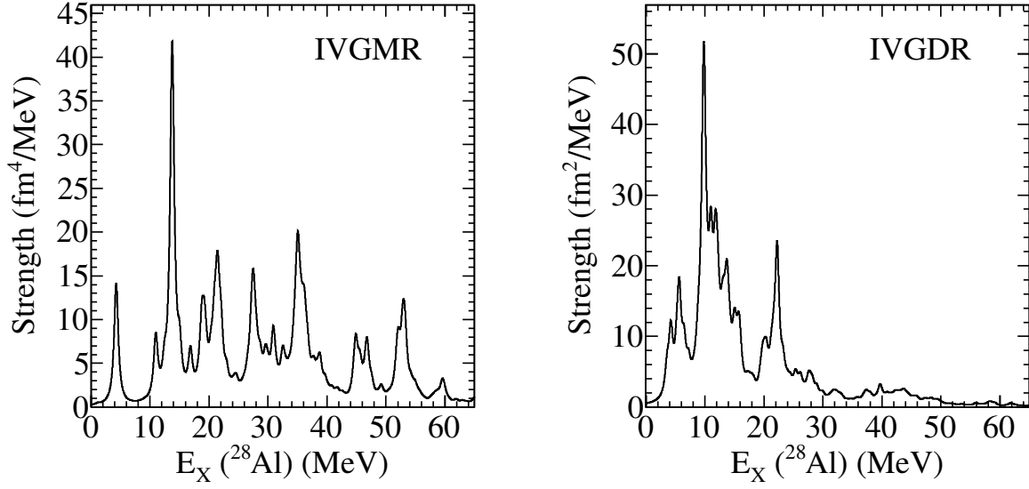
Figure 3.4 Results of the RTBA calculation for the IVGMR and the IVGDR by E. Litvinova [43, 42]. Strengths have been smeared with Lorentzians of 2 MeV in width.
