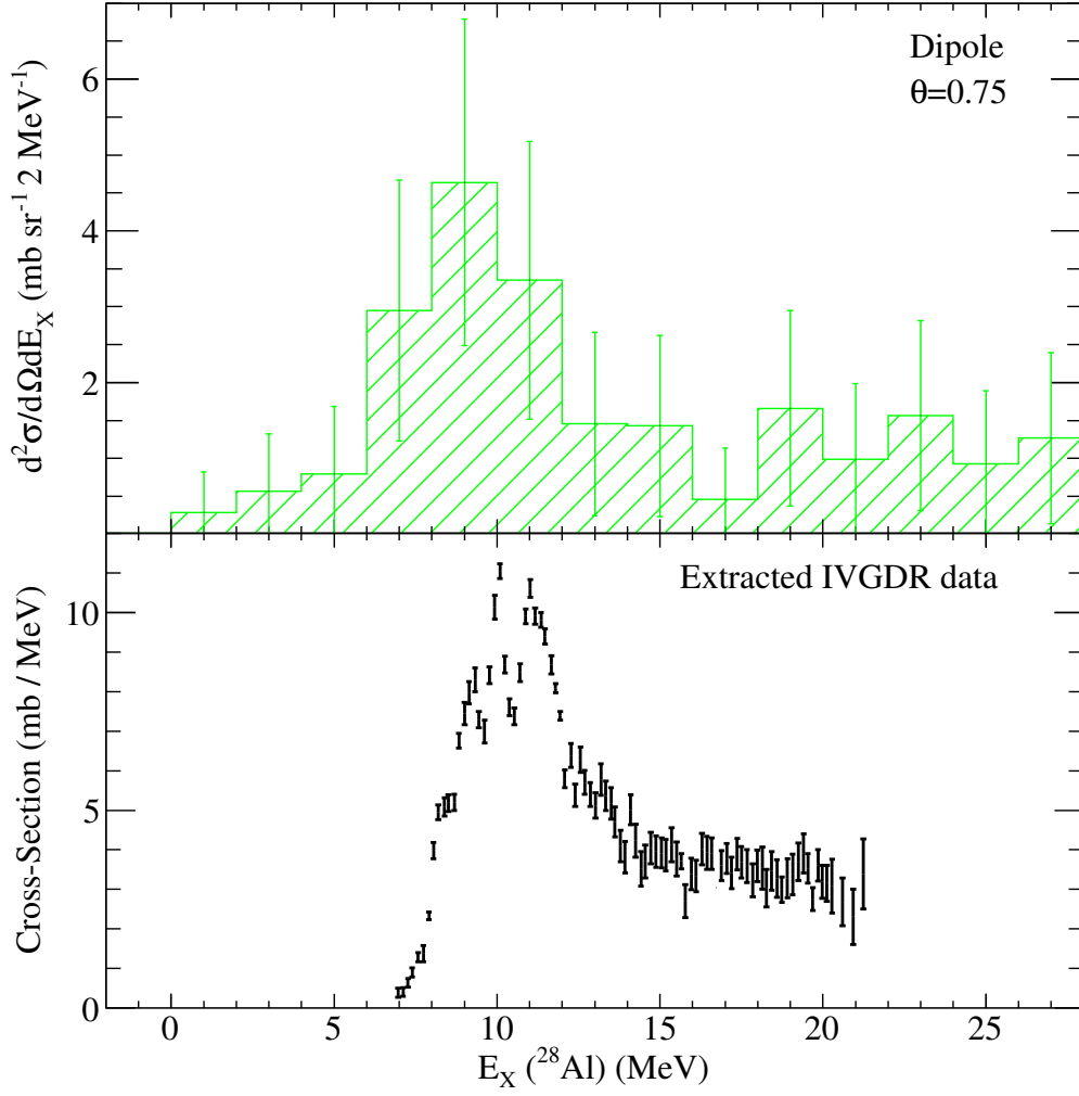
Figure 7.8 Comparison of the measured \Delta L = 1 (dipole) distribution for the ^{28}\text{Si}(^{10}\text{Be}, ^{10}\text{B} + \gamma)^{28}\text{Al} reaction with the IVGDR distribution measured previously in the ^{28}\text{Si}(\gamma, n) reaction [4].
