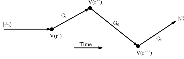
Figure 4.1 Illustration of the propagation of a projectile between scattering events.
