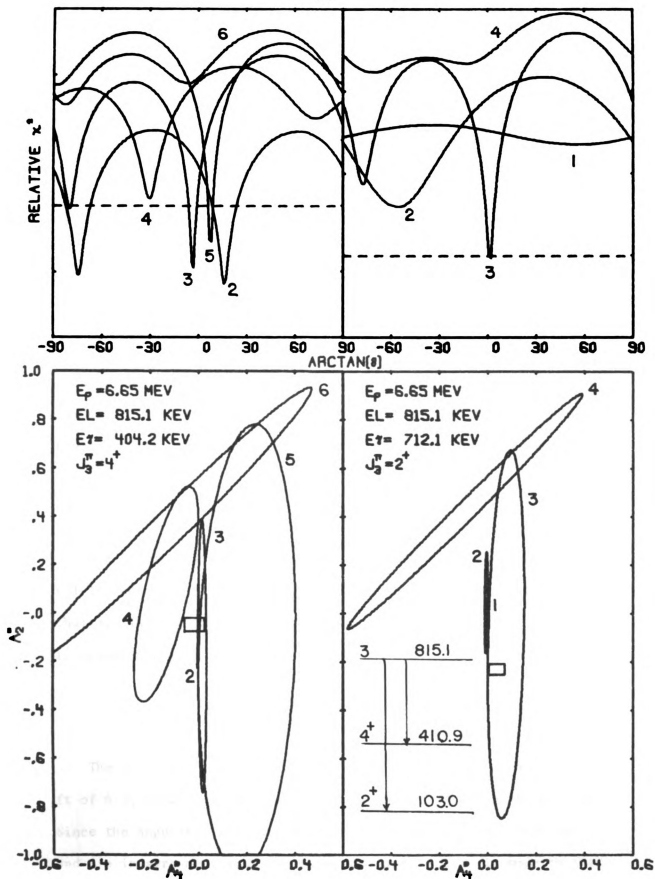
Chi square and delta ellipse plots for the 404.2 and 712.1 keV gamma rays.
