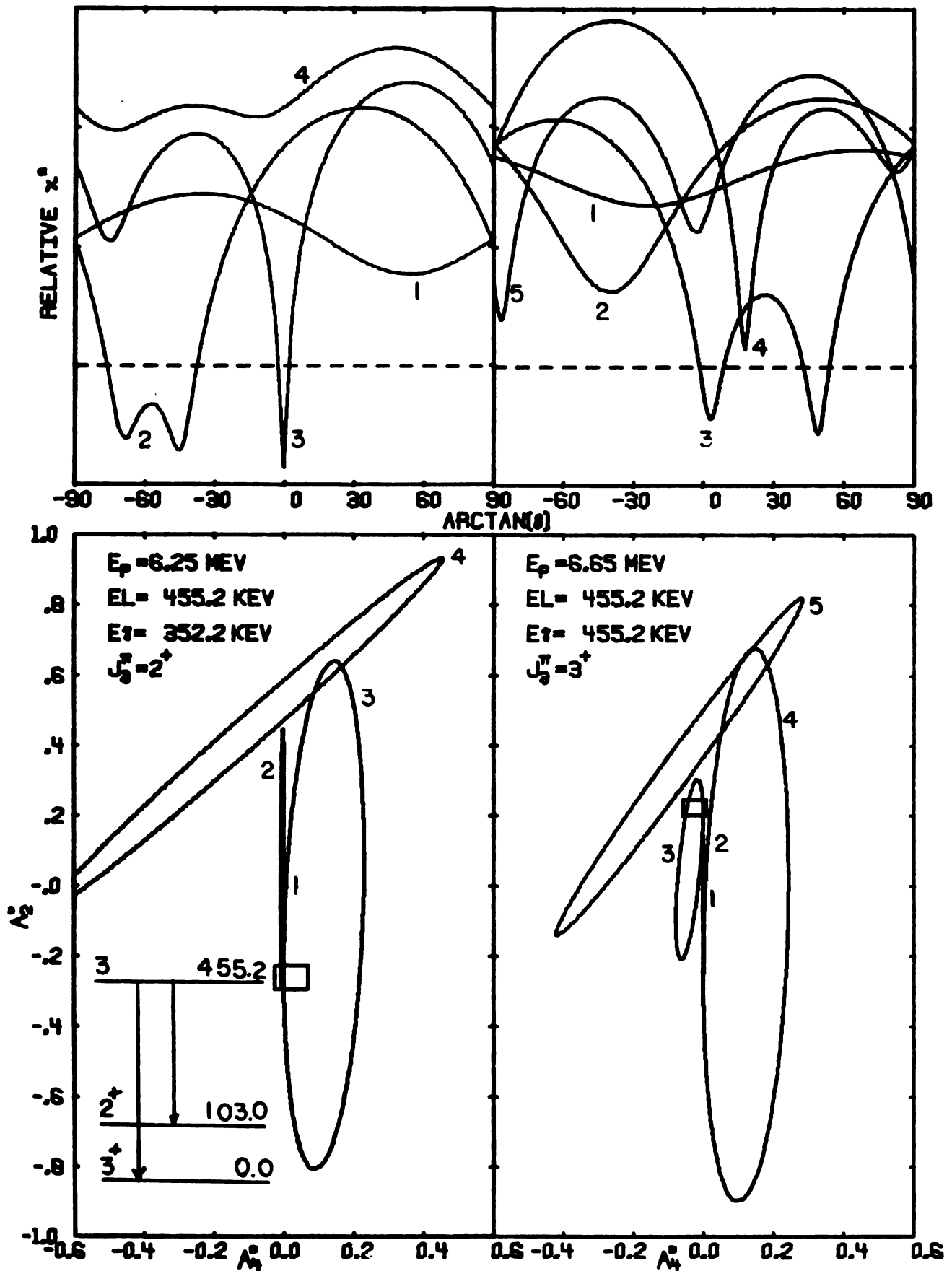
Chi square and delta ellipse plots for the 352.2 and 455.2 keV gamma rays.
