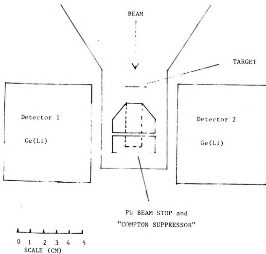
Arrangement for in-beam \gamma - \gamma coincidence.
