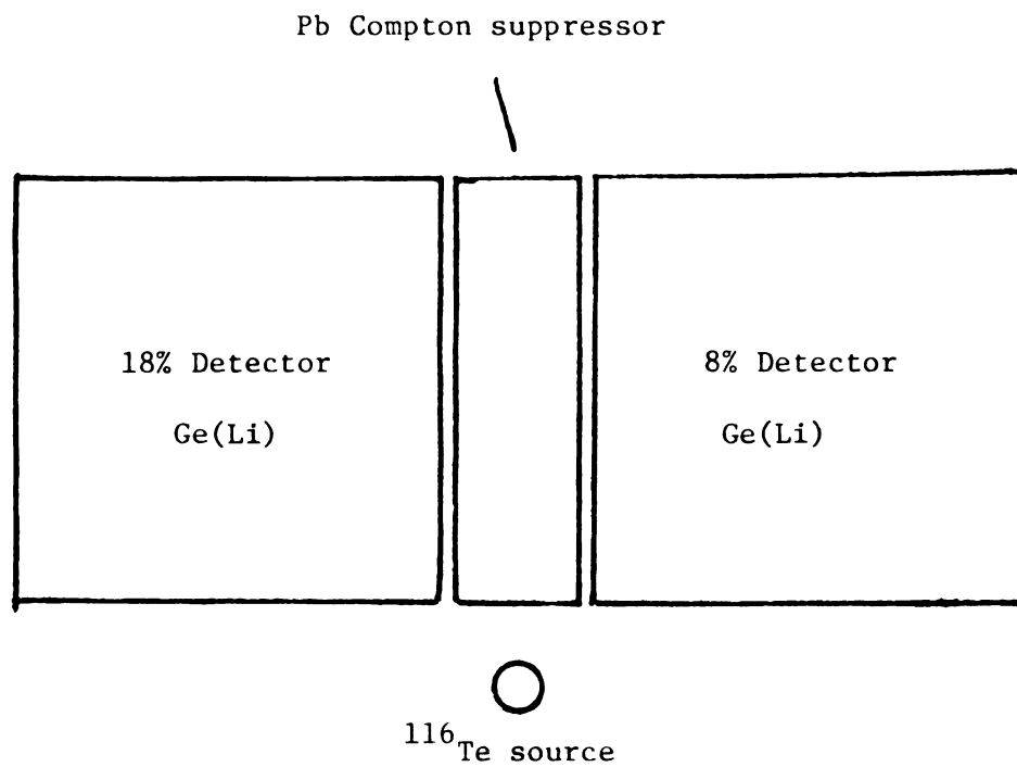
Detector arrangement for \gamma - \gamma coincidence.
