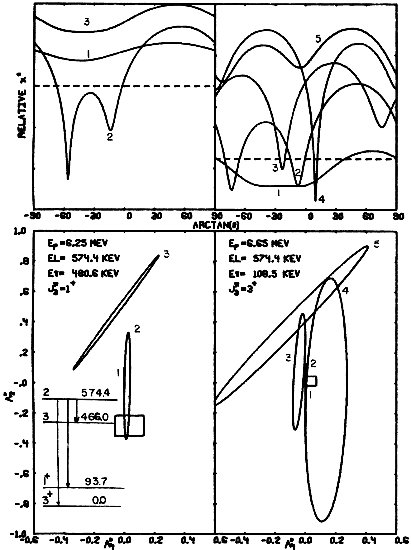
Chi square and delta ellipse plots for the 480.6 and 108.5 keV gamma rays.
