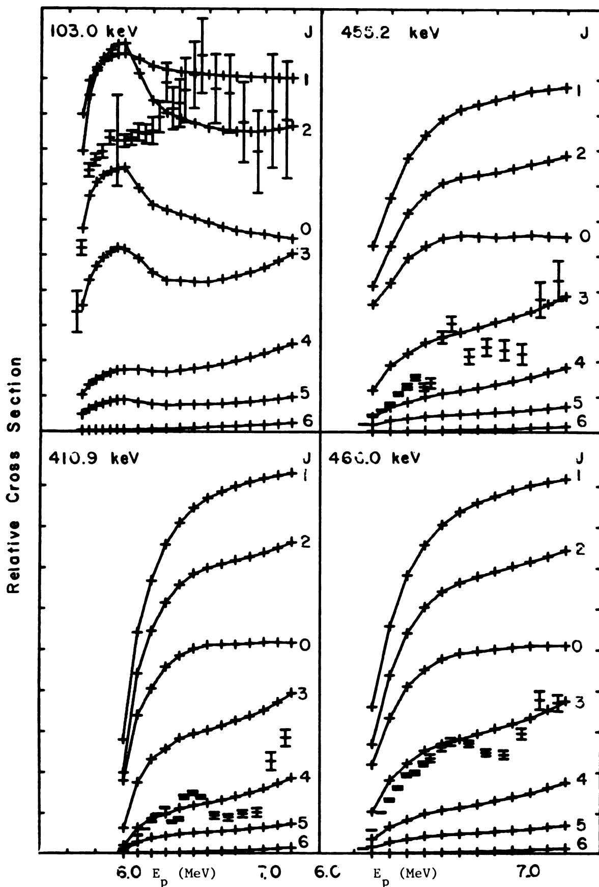
Excitation functions for 103.0, 410.9, 455.2, and 466.0 keV levels.
