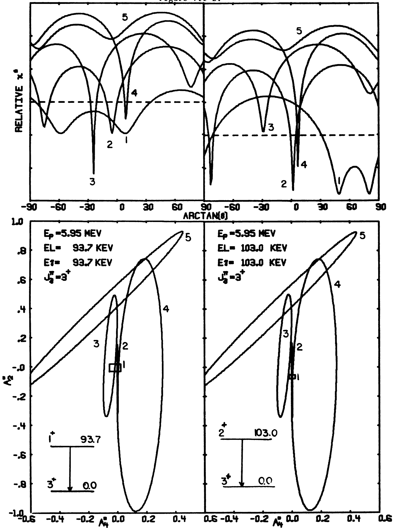
Chi square and delta ellipse plots for the 93.7 and 103.0 keV gamma rays.
