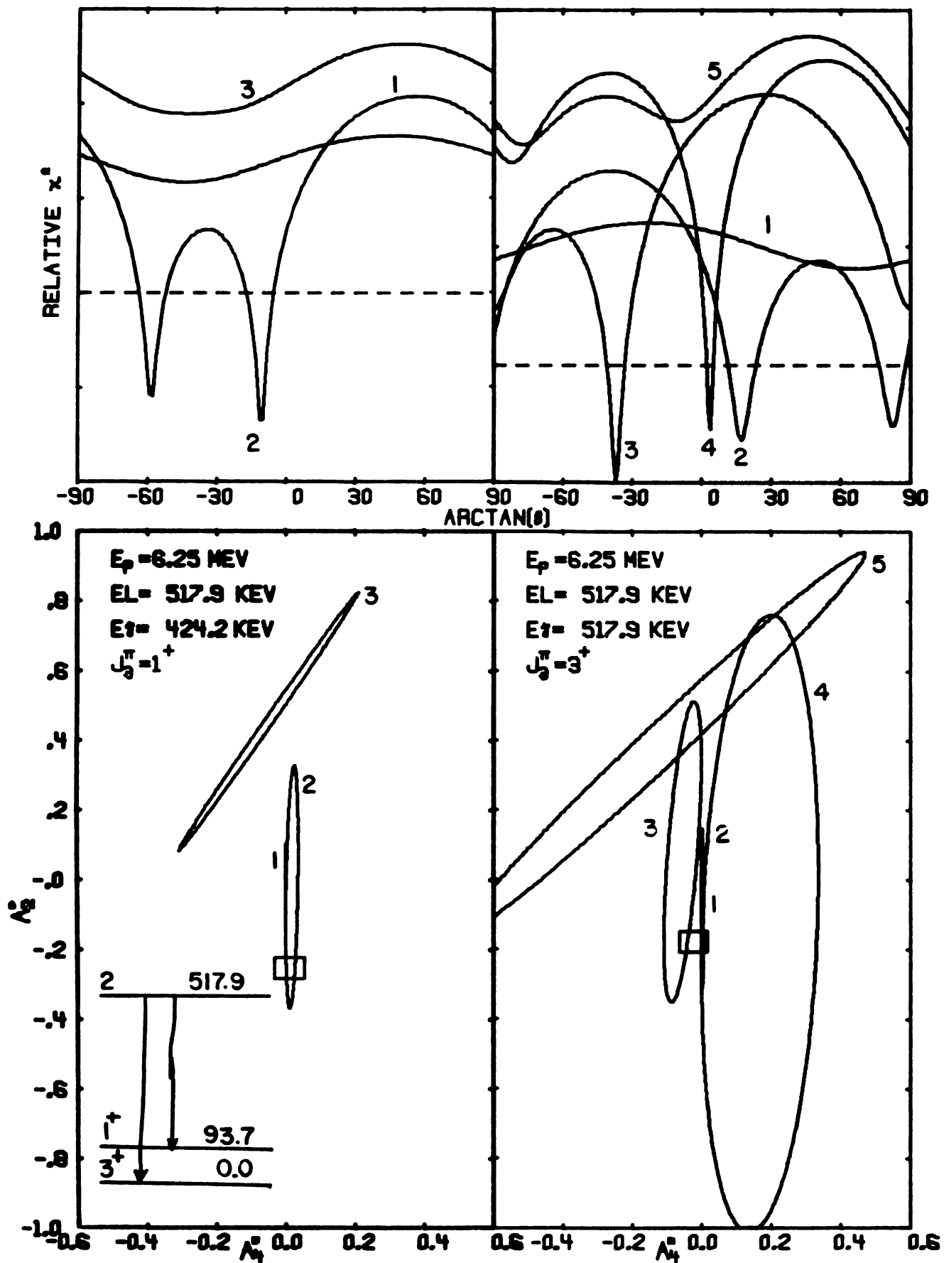
Chi square and delta ellipse plots for the 424.2 and 517.9 keV gamma rays.
