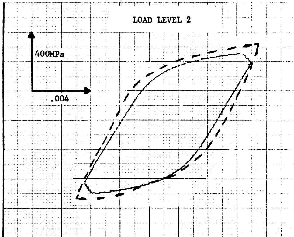
FIGURE 54 NEUBER PREDICTION AND STRESS SIMULATION AT 1,200°F
