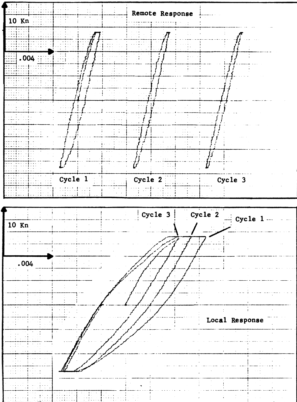
FIGURE 28 ROOM TEMPERATURE I.S.G. STRAIN VERSUS LOAD
