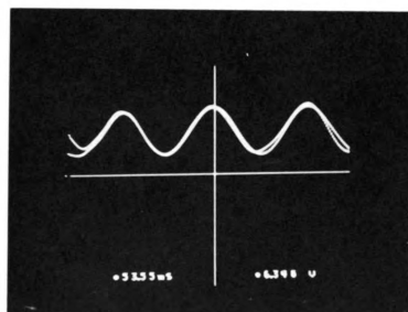
FIGURE 11 FRINGE PATTERN INTENSITY SIGNALS AT 70°F AND 1,200°F
