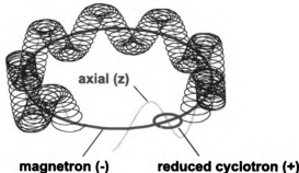
Figure 3.2. Cartoon illustrating the three independent eigenmotions executed by an ion in a Penning trap. The two radial eigenmotions are the cyclotron and magnetron motion, while the third motion is the axial oscillation.
