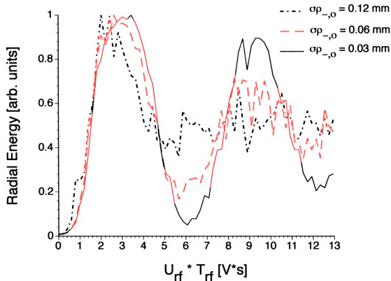
Figure 4.16. Simulated radial energy gain for three different values of \sigma_{\rho_{-,o}} as a function of U_{rf} for \nu_{rf} = 2\nu_c and \bar{\rho}_- = 0.55 mm.
