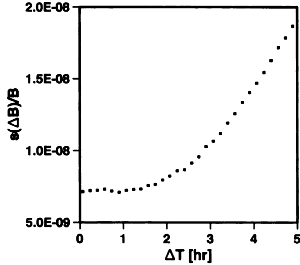
Figure 7.5. The magnetic field strength nonlinearity parameter, s(\Delta B)/B , as a function of \Delta t between reference measurements.
