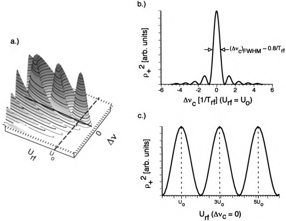
Figure 4.1. (a) surface plot of \rho_+^2 as a function of U_{rf} and \nu_{rf} for a given excitation time T_{rf} . (b) cut from plot (a) at U_{rf} = U_0 . Full conversion from magnetron to cyclotron motion is achieved at \Delta\nu_c = \nu_{rf} - \nu_c = 0 . (c) slice from plot (a) at \Delta\nu = 0 illustrating the beating of \rho_+^2 as a function of U_{rf} .
