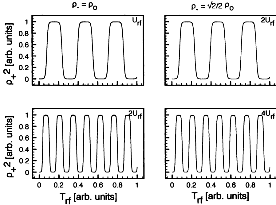
Figure 4.7. The left hand panels show \rho_+^2 as a function of T_{rf} for an ion with an initial \rho_{-,o} = \rho_o and \rho_{+,o} = 0 with applied RF amplitudes of U_{rf} and 2U_{rf} , respectively. The right hand panels \rho_+^2 for an ion with an initial \rho_{-,o} = \frac{\sqrt{2}}{2}\rho_o and applied RF amplitudes of 2U_{rf} and 4U_{rf} , respectively.
