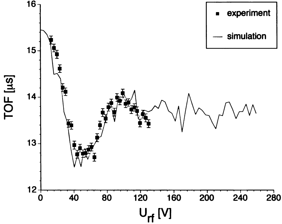
Figure 4.19. Time of flight as a function of U_{rf} for a octupolar excitation of ^{23}\text{Na}^+ with T_{rf} = 50 ms at \nu_{rf} = 2\nu_c . The solid line shows the results of a simulation.
