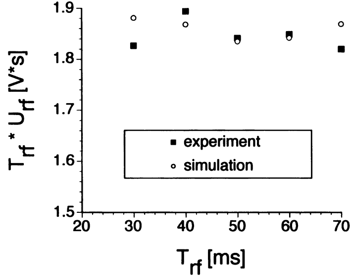
Figure 4.21. Product of U_o and T_{rf} , where T_{rf} is the duration of the octupolar excitation and U_o is the amplitude of applied octupolar RF field at which the TOF curve reaches its minimum.
