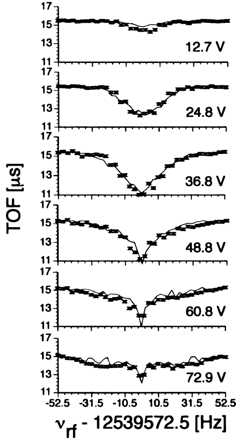
Figure 4.24. Several octupolar resonance profiles of ^{23}\text{Na}^+ with T_{rf} = 50 ms for various values of U_{rf} (data points) compared with simulated results (solid lines).
