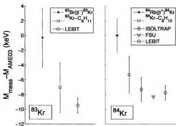
Figure 6.2. Deviation of individual mass measurements of ^{83,84}\text{Kr} from AME03. Values obtained from \beta decays use AME03 values for the masses of the parent nuclei.
