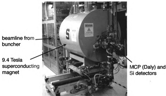
Figure 2.6. Photograph of the LEBIT Penning trap mass spectrometer.
