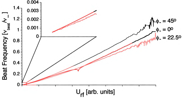
Figure 4.10. Beat frequency as a function of U_{rf} for three initial \phi_{-,o} 's. The insert zooms in to low beating frequencies and amplitudes.
