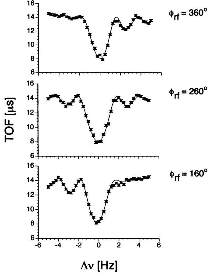
Figure 4.4. Three ^{39}\text{K}^+ quadrupolar resonances for T_{rf} = 500 ms measured for different values of \phi_{rf} . The solid line is the fit of the theoretical line shape.
