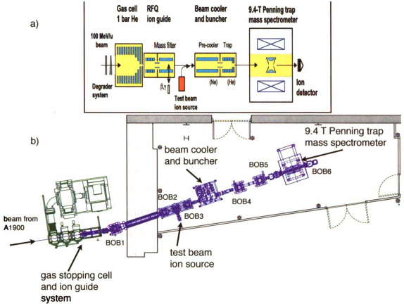
Figure 2.2. Layout of the LEBIT facility at the NSCL. BOB denotes beam observation boxes equipped with various detector systems. The two figures are (a) the schematic layout and (b) design drawing of the LEBIT system.
