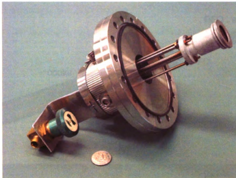
Figure 2.4. The test beam ion source.
