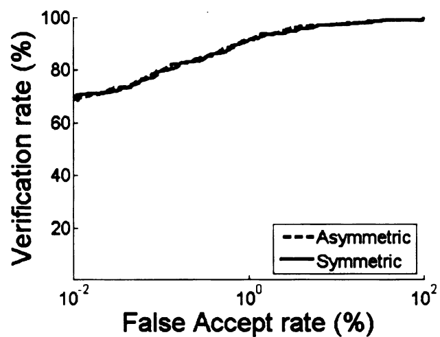
Figure 5.9: Symmetric matching performance on MSU dataset.
