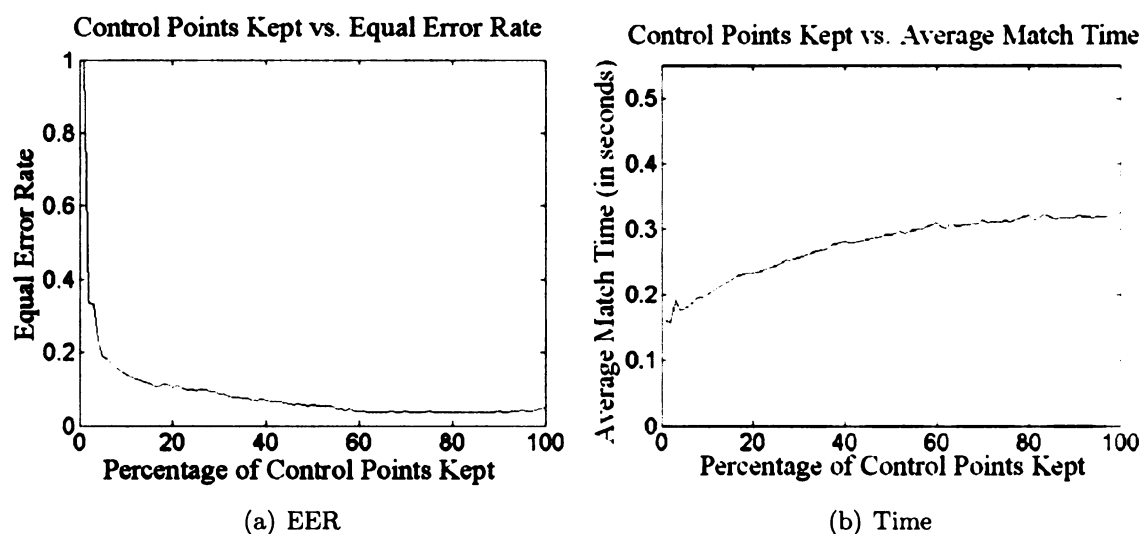
Figure 5.8: Results when varying the number of points trimmed.
