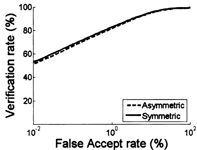
Figure 5.11: Symmetric matching performance on FRGC version 2.0 dataset.
