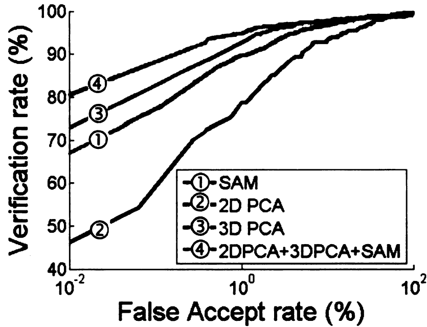
Figure 6.25: Comparing automatic PCA with manual PCA.
