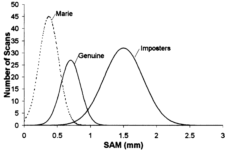
Figure 5.16: Gaussian approximation of SAM distributions.
