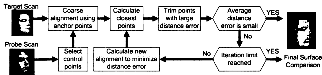
Figure 5.2: Alignment algorithm outline.
