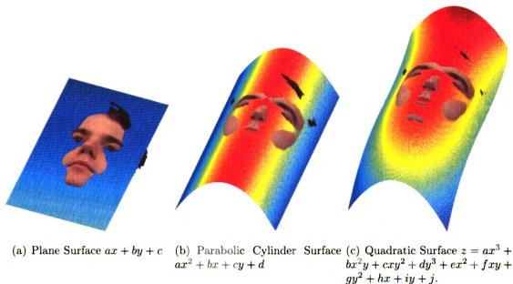
Figure 6.7: Parametric surface fitting using forced symmetrical surface fitting.
