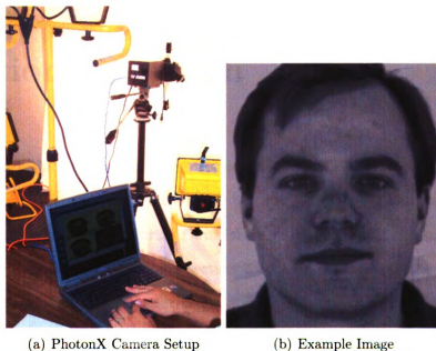
Figure 2.21: Example prototype setup for the PhotonX multi-image shape from shading camera.
