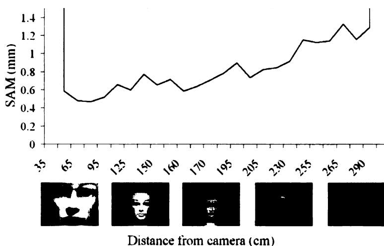
Figure 5.21: Change in stand off vs. SAM.
