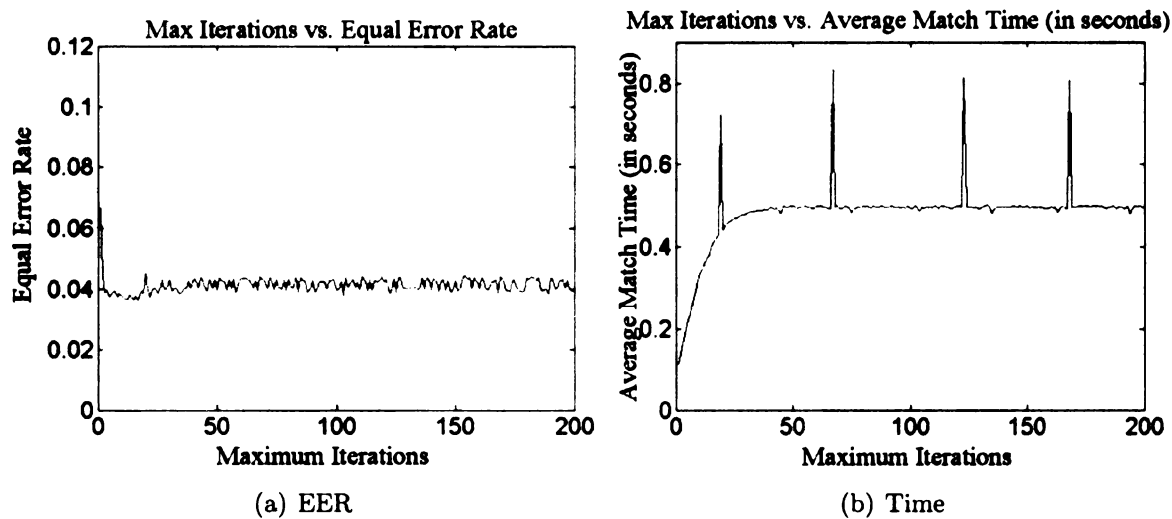
Figure 5.6: Results when varying the maximum number of iterations.
