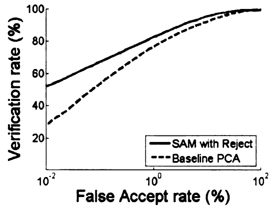
Figure 5.26: Performance on FRGC 2.0 dataset when the training data is from one semester and the testing data is from a later semester.
