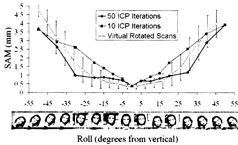
Figure 5.18: Change in roll vs. SAM.
