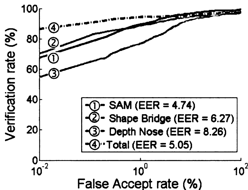
Figure 8.5: Fusion example. By fusing the nose correlation, bridge correlation and SAM score, significantly higher performance is achieved over any of the three matching scores by themselves.
