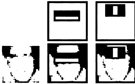
Figure 4.2: Simple and efficient 2D face detector using a cascade of dark-light-dark anchor point detectors [138].
