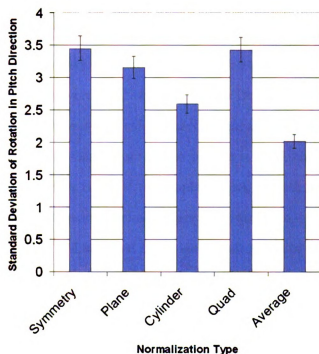
Figure 6.8: Comparison of pitch standard deviation over different fitting techniques.
