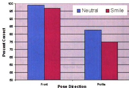
Figure 4.12: Percent of correctly selected anchor points versus the pose direction and facial expression. The success rate for frontal neutral faces is 99.0%.
