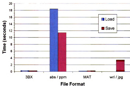
Figure A.1: Results of experiments to compare time taken to read and write common file types.
