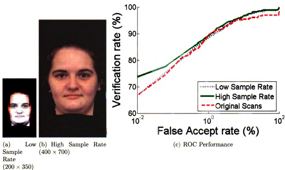
Figure 6.18: Depth maps sampled at two different resolutions using the MSU database. The higher resolution data improves ICP performance by allowing for small incremental changes during each iteration of the algorithm. The increased surface matching performs slightly better, as seen in (c).
