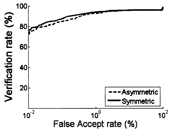
Figure 5.10: Symmetric matching performance on FRGC version 1.0 dataset.
