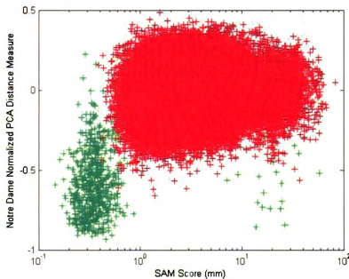
Figure 8.3: SAM score vs. PCA distance score on the MSU dataset. Red (dark) points represent impostors and green (light) points represent genuine.
