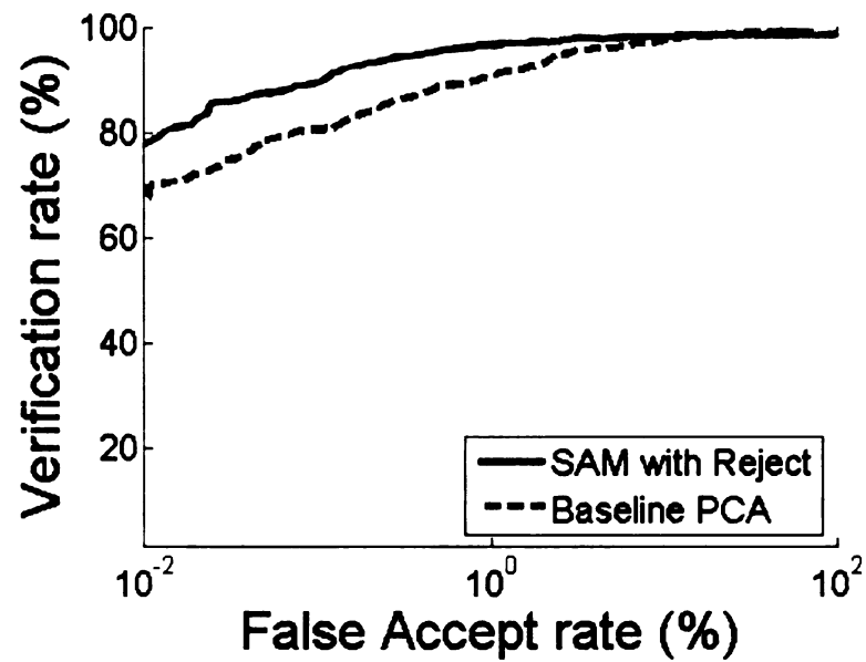
Figure 5.23: Resulting ROC curves for the FRGC 1.0 dataset.
