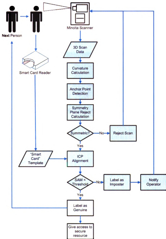
Figure 7.2: Flow chart representing the operation of the prototype 3D face verification system.
