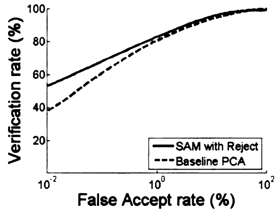
Figure 5.25: Performance on FRGC 2.0 dataset when the training and testing data are taken from two different semesters.
