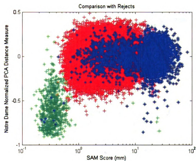
Figure 8.4: SAM score vs. PCA distance score on the MSU dataset. Red (dark) points represent impostors, green (light) points represent genuine and blue (darkest) points represent scores with either the model or the template scan rejected based on the symmetry criteria.
