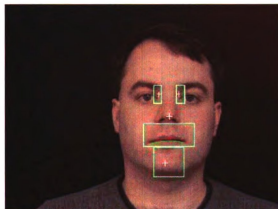
Figure 4.3: Example bounding boxes produced by the statistical face model and the location of the nose tip.
