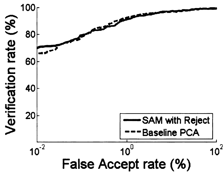
Figure 5.22: ROC curves for the MSU dataset.
