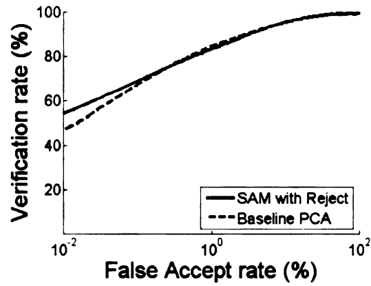
Figure 5.24: Performance on FRGC 2.0 dataset when the training and testing data are both from the same semester.
