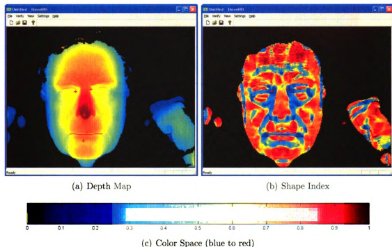
Figure 7.6: Matching algorithm demo visualization.
