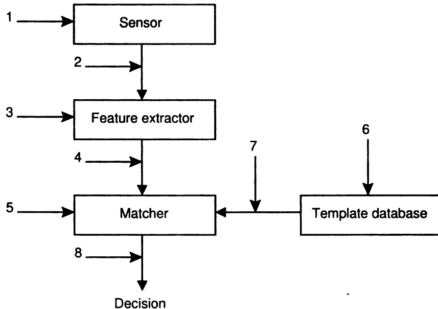
Figure 2.1: Locations of possible attacks in a biometric system.
