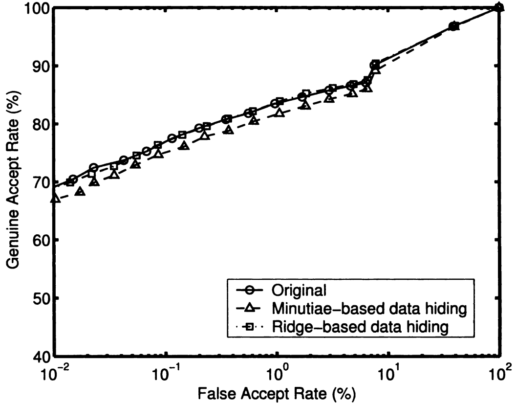
Figure 3.14: ROC curves corresponding to original and eigen-face carrying fingerprint images.
