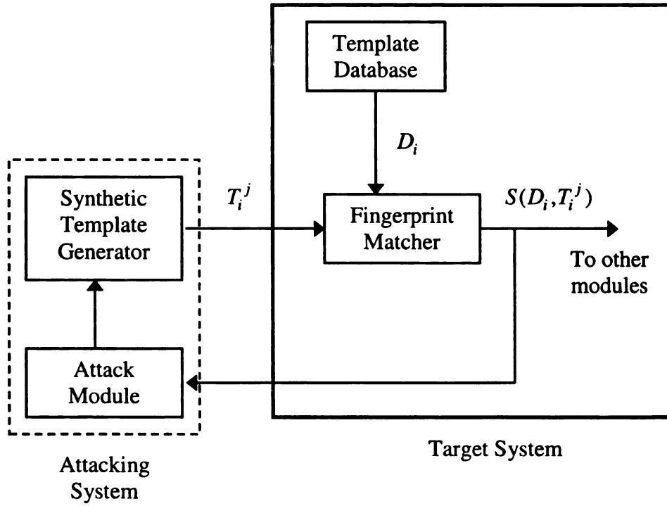
Figure 2.7: The block diagram of the minutiae template attack system.
