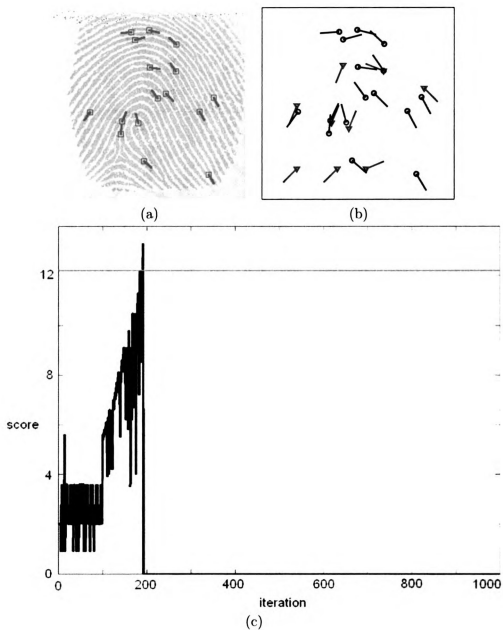
Figure 2.18: A sample account is broken: (a) target template with overlaid minutiae, (b) synthetic minutiae (red) and the original minutiae (blue) when the account is broken, (c) progression of matching scores (decision threshold is shown as the horizontal line).
