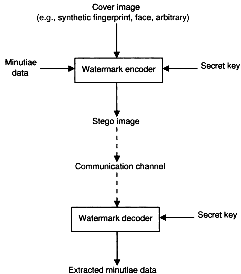
Figure 3.10: Block diagram of application scenario 1.
