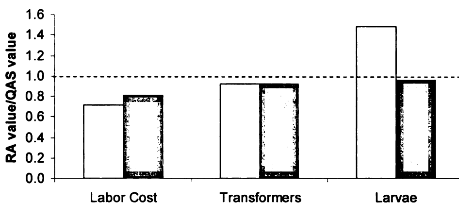
Figure 7. The ratio of RA values to QAS values for labor cost (assessment + control costs), total estimated number of transformers killed, and total estimated number of larvae killed when equal numbers of treatment staff days are allocated to treat streams ranked by RA and QAS. Light bars represent 2005 values, and dark bars represent 2006 values. Total transformer and larvae estimates were the sum of the population estimates generated by the ESTR model for the streams that would be treated based on the results of each assessment method. Dashed line indicates where the RA and QAS values are equal; above this line, RA values are higher, below this line QAS values are higher.
