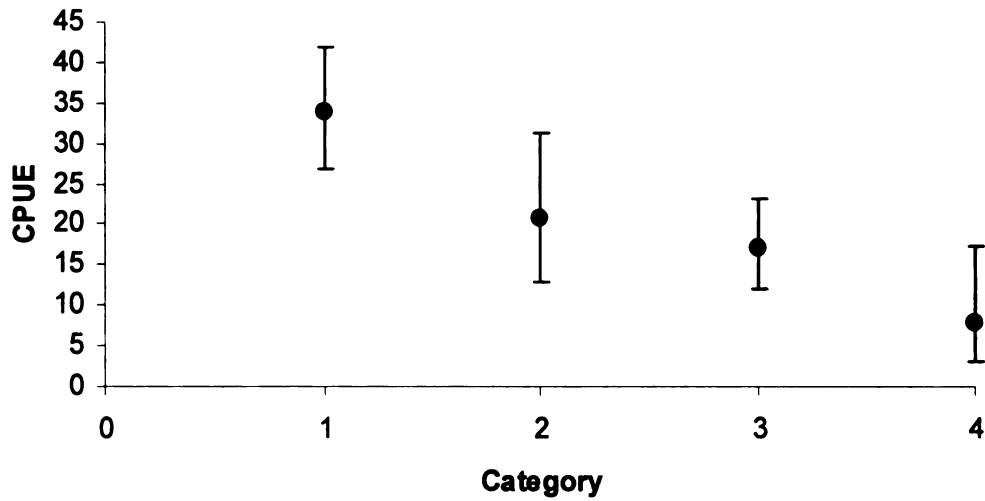
Figure 10. Mean CPUE (catch per hour) and 95% confidence intervals for each stream category as predicted by the linear model when holding lake constant (values shown are for Lake Superior streams).
