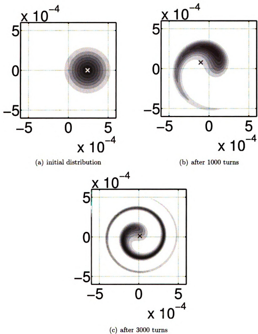
Figure 4.21. Particle distribution in the beam, the cross indicates the center of mass of the beam.
