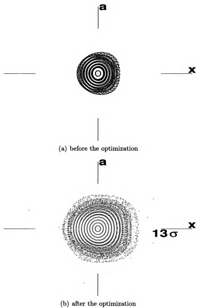
Figure 5.5. The comparison of the phase portraits in the (x, a) plane before and after the optimization. Particles are launched along the (x, y) diagonal with a step of one \sigma .
