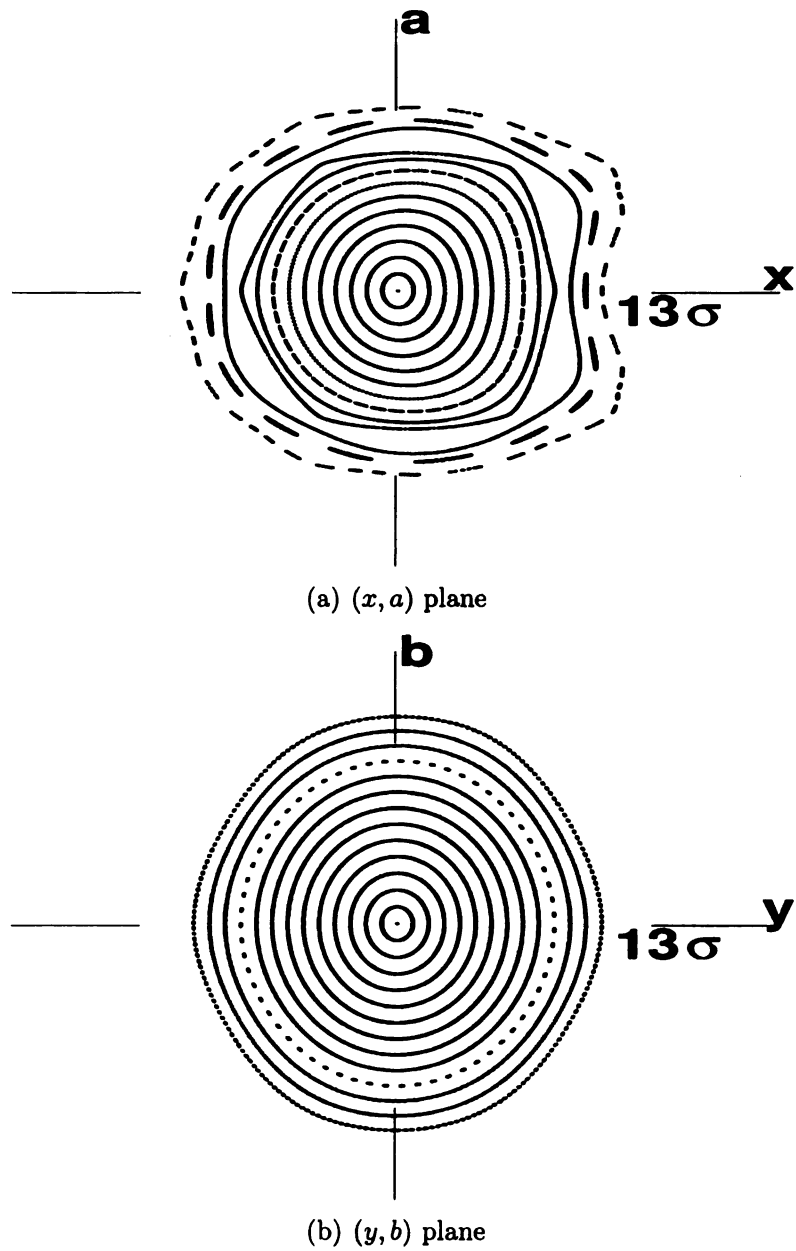
Figure 5.4. Phase portraits after the optimization in the (x, a) and (y, b) planes. Particles are launched along the x and y axes, respectively, with an increment of one \sigma , \sigma = 82 \cdot 10^{-6} m.
