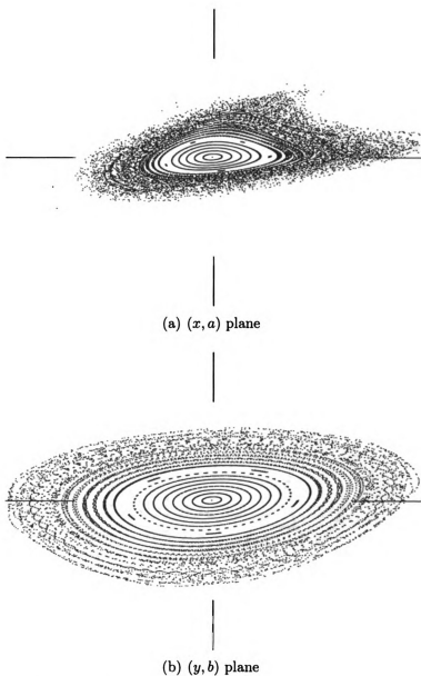
Figure 4.7. The (x, a) plane and (y, b) plane phase portraits after the optimization with 50% skew quadrupole errors in dipoles, errors are fixed according to Scheme I: around each defocusing quadrupole; particles are launched along the x axis and the y axis, respectively. The scales are 2.7 \cdot 10^{-3} m for the x and y axes and 4.0 \cdot 10^{-3} for the a and b axes.
