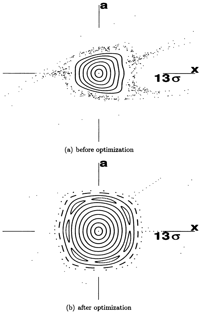
Figure 5.2. The comparison of the phase space portraits before and after the optimization using the first approach (minimization of individual high order coefficients) in the (x, a) plane. Particles are launched along the x axis with an increment of one \sigma , \sigma = 82 \cdot 10^{-6} m.
