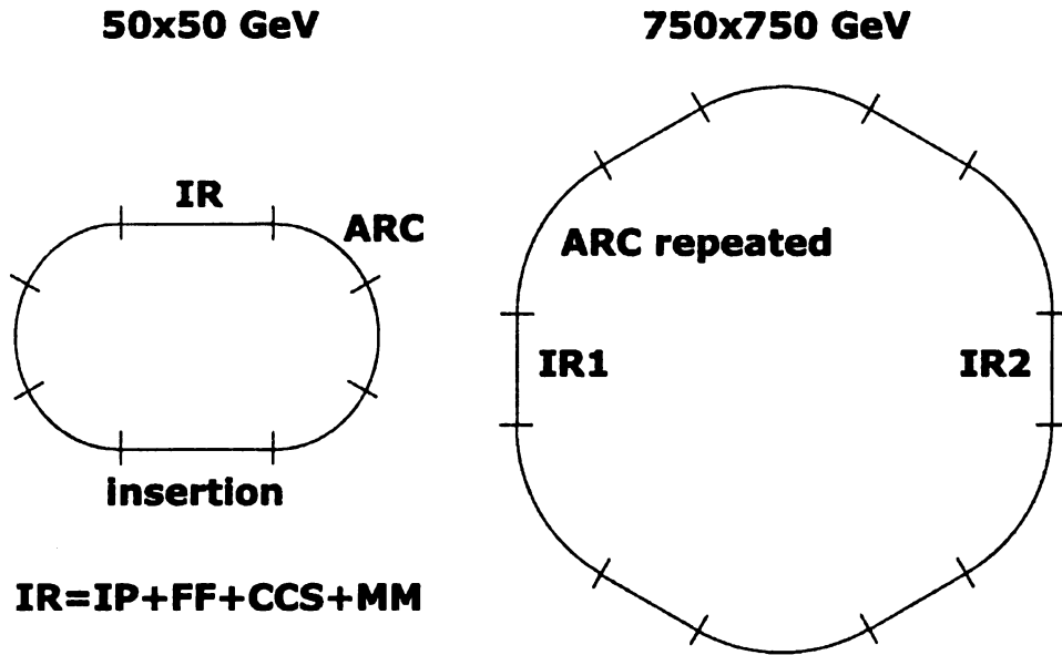
Figure 5.8. The baseline 50×50 GeV lattice scheme compared to the 750×750 GeV lattice scheme.
