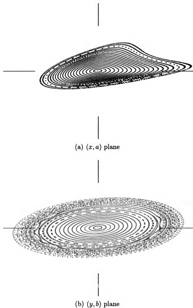
Figure 4.8. The (x, a) plane and (y, b) plane phase portraits after the optimization according to Scheme II: the skew quadrupole errors are removed in the two dipoles flanking each horizontally defocusing quadrupole, and particles are launched along the x axis and the y axis, respectively. The scales are 2.7 \cdot 10^{-3} m for the x and y axes and 4.0 \cdot 10^{-3} for the a and b axes.
