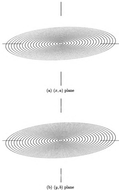
Figure 4.3. The (x, a) plane and (y, b) plane phase portraits, only dipoles and pure quadrupoles are active, and particles are launched along the x axis and the y axis, respectively. The scales are 2.7 \cdot 10^{-3} m for the x and y axes and 4.0 \cdot 10^{-3} for the a and b axes.
