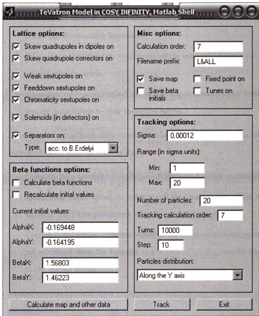
Figure B.1. Tevatron simulation GUI
