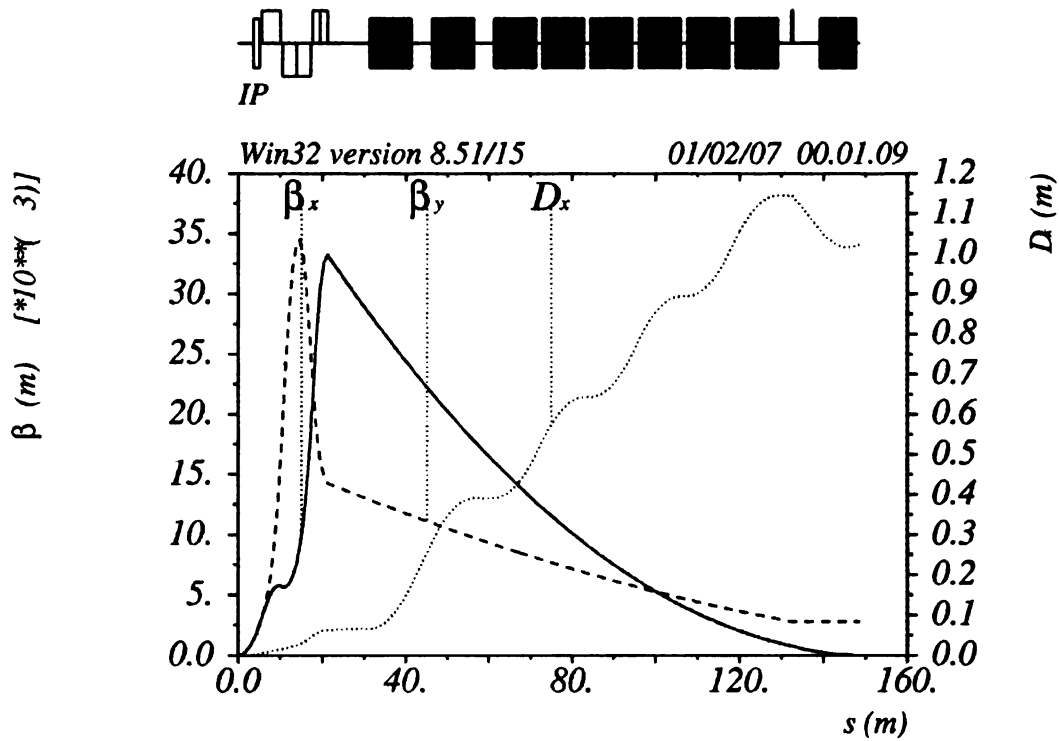
Figure 5.9. The final focus section beta functions and dispersion plots
