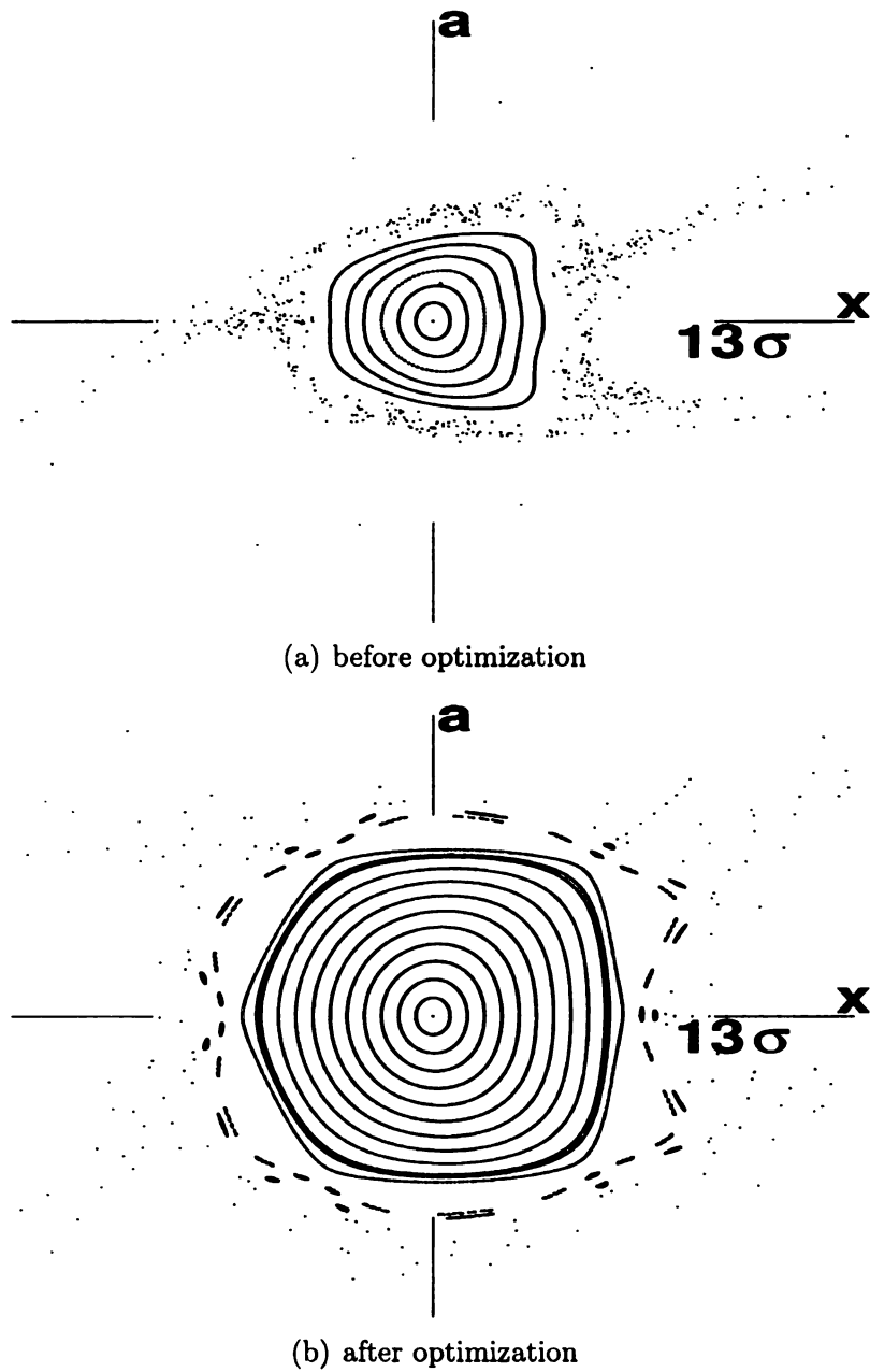
Figure 5.3. The comparison of the phase space portraits before and after the optimization using the second approach (minimization of the resonance strengths) in the (x, a) plane. Particles are launched along the x axis with an increment of one \sigma , \sigma = 82 \cdot 10^{-6} m.
