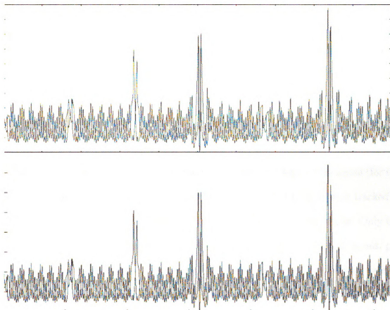
Figure 4.2. Beta functions comparison, top - OptiM32, bottom - COSY INFINITY
