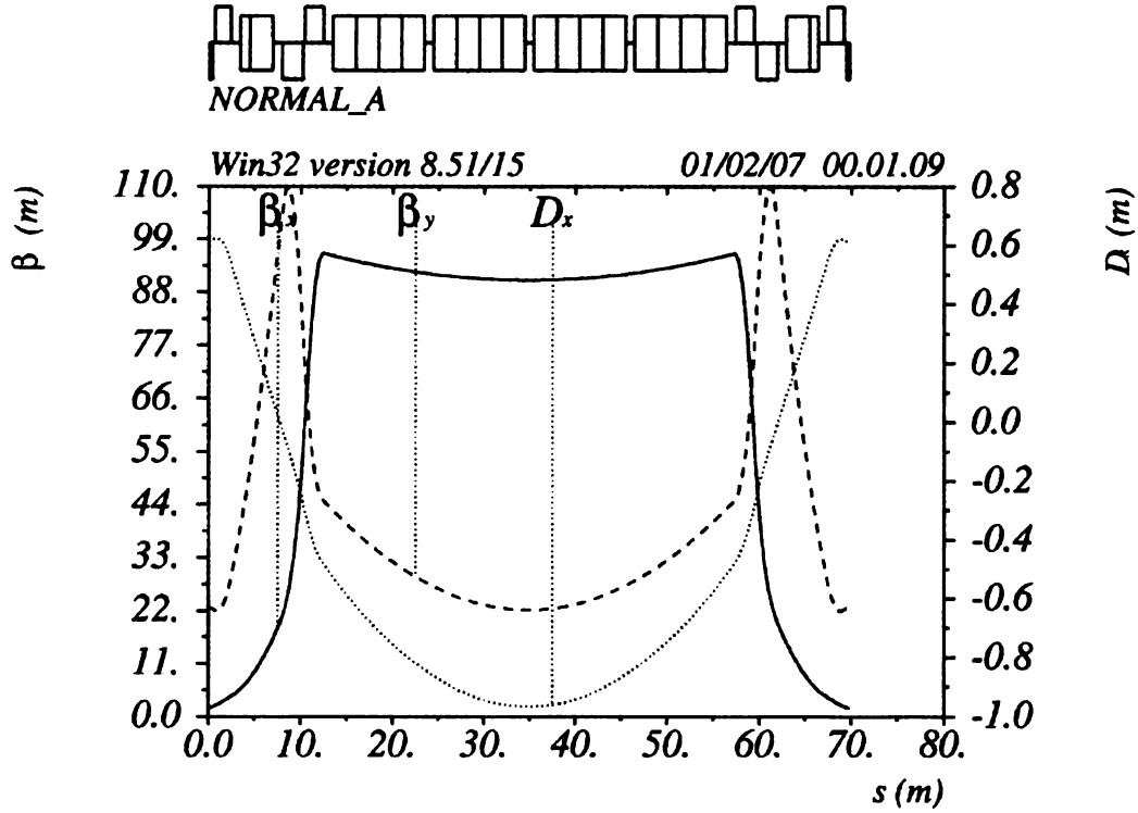
Figure 5.11. The arc module beta functions and dispersion plots
