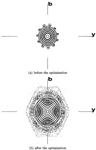
Figure 5.6. The comparison of the phase portraits in the (y, b) plane before and after the optimization. Particles are launched along the (x, y) diagonal with a step of one \sigma , \sigma = 82 \cdot 10^{-6} m.
