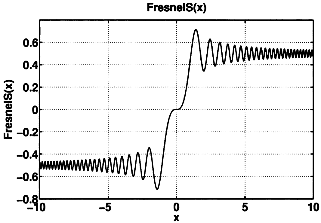
Figure 4.13. FresnelS function graph
