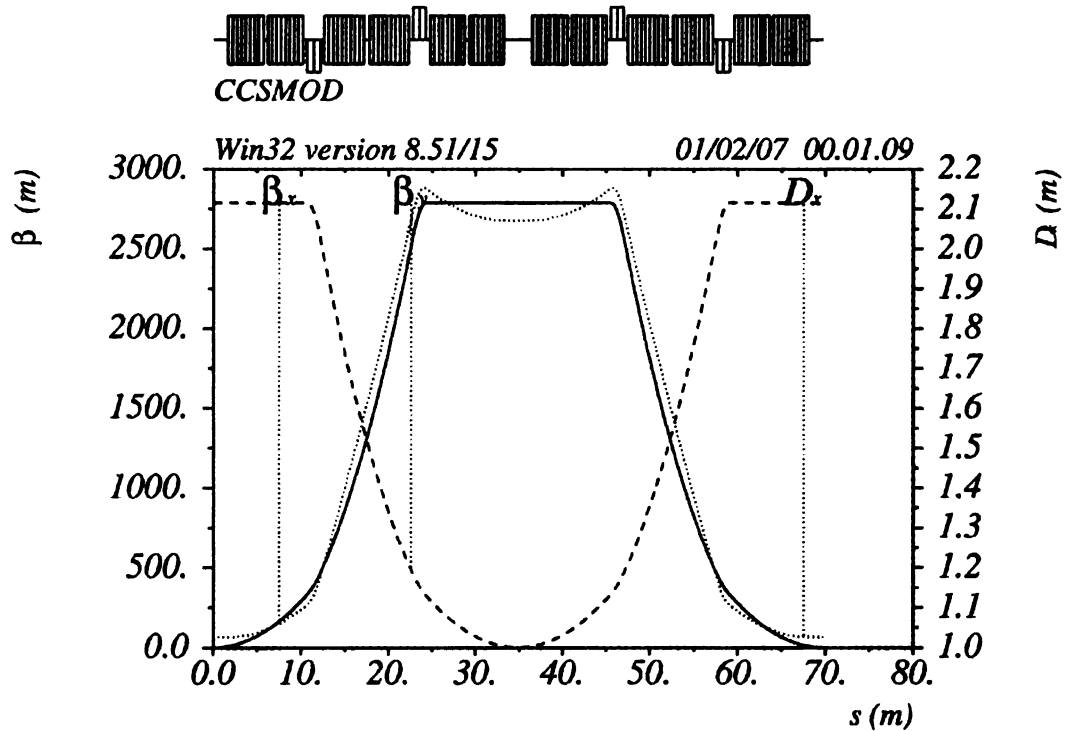
Figure 5.10. The chromaticity correction section beta functions and dispersion plots and the fact that the transfer map of the section is unity implies that the important aberration ( x|\delta\delta ) vanishes as well. The layout of the CCS is shown in Fig. 5.10.
