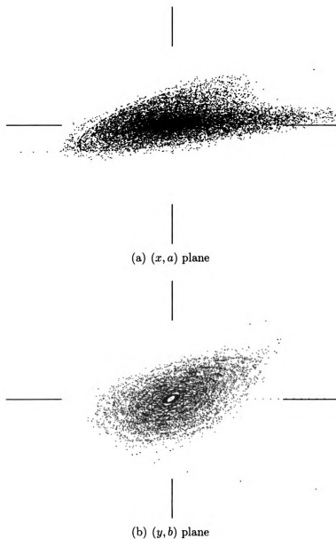
Figure 4.4. The (x, a) plane and (y, b) plane phase portraits before the optimization, particles are launched along the x axis and the y axis, respectively. The phase portraits include all sextupole and skew quadrupole fields (correctors plus errors) in addition to quadrupoles and dipoles, where 15% of the skew quadrupole errors have been removed in specific dipoles. the scales are 2.7 \cdot 10^{-3} m for the x and y axes and 4.0 \cdot 10^{-3} for the a and b axes.
