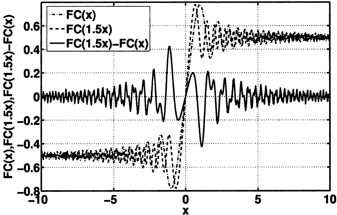
Figure 4.17. \text{FresnelC}(1.5x) - \text{FresnelC}(x) function graph
