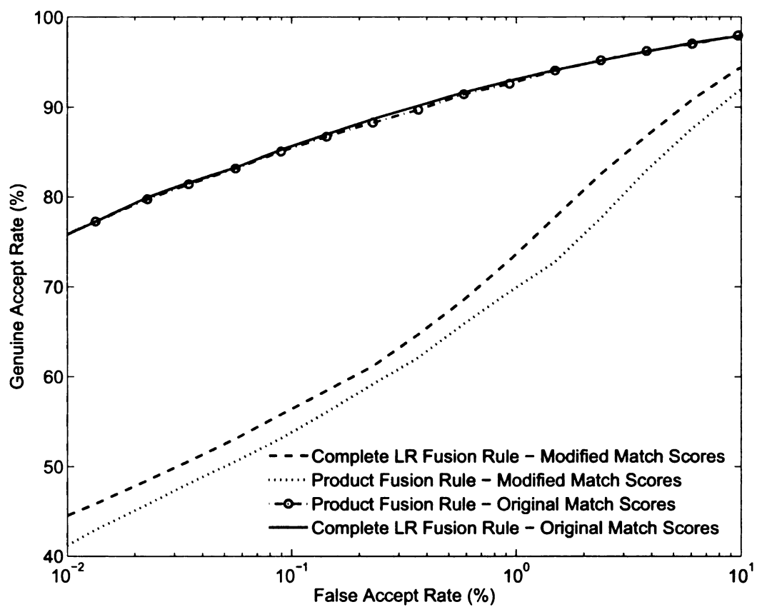
Figure 3.16: Performance of product and complete likelihood ratio based fusion rules for the two face matchers in the NIST-Face database.
