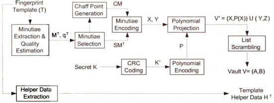
Figure 5.5: Proposed implementation of vault encoding.
