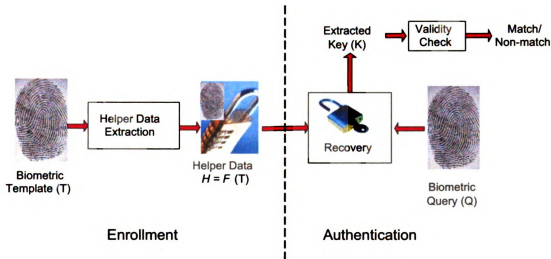
Figure 5.3: Authentication mechanism when the biometric template is secured using a key generation biometric cryptosystem. Authentication in a key-binding biometric cryptosystem is similar except that the helper data is a function of both the template and the key K , i.e., H = \mathcal{F}(T; K) .
