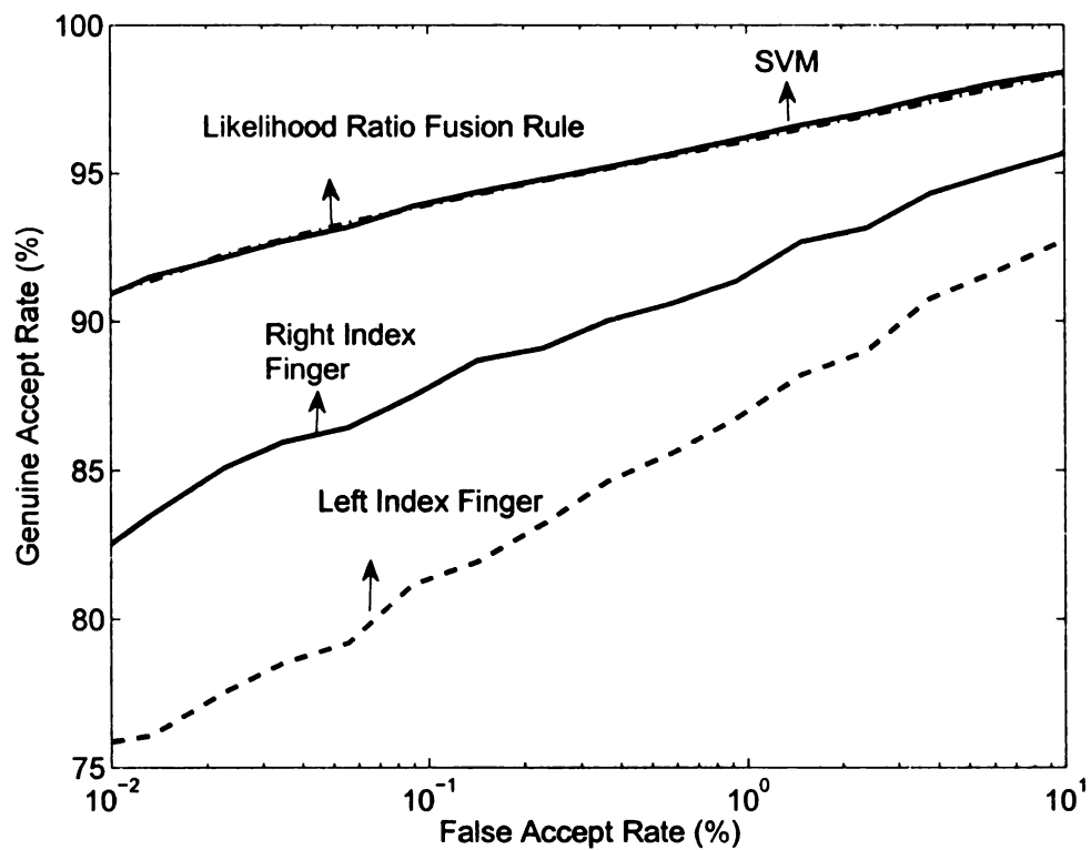
Figure 3.11: Performance of complete likelihood ratio based fusion rule and SVM-based fusion on the NIST-Fingerprint database. A radial basis function kernel with \gamma = 0.005 was used for SVM fusion.
