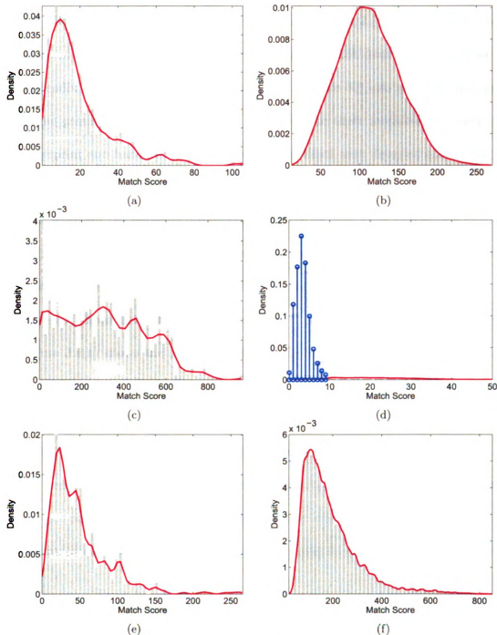
Figure 3.3: Histograms of match scores and the corresponding generalized density estimates for MSU-Multimodal database. (a) and (b) Genuine and impostor match scores for face modality. (c) and (d) Genuine and impostor match scores for fingerprint modality. (e) and (f) Genuine and impostor match scores for hand geometry modality. The solid line above the histogram bins is the density estimated using the kernel density estimator, and the spikes in (d) correspond to the discrete components.
