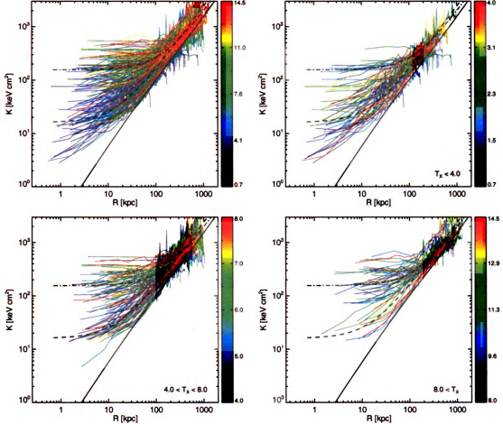
Figure 3.3 Composite plots of entropy profiles for varying cluster temperature ranges. Profiles are color-coded based on average cluster temperature. Units of the color bars are keV. The solid-line is the pure-cooling model of Voit et al. (2002), the dashed-line is the mean profile for clusters with K_0 \leq 50 \text{ keV cm}^2 , and the dashed-dotted line is the mean profile for clusters with K_0 > 50 \text{ keV cm}^2 . Top left: This panel contains all the entropy profiles in our study. Top right: Clusters with kT_X < 4 \text{ keV} . Bottom left: Clusters with 4 \text{ keV} < kT_X < 8 \text{ keV} . Bottom right: Clusters with kT_X > 8 \text{ keV} . Note that while the dispersion of core entropy for each temperature range is large, as the kT_X range increases so to does the mean core entropy.
