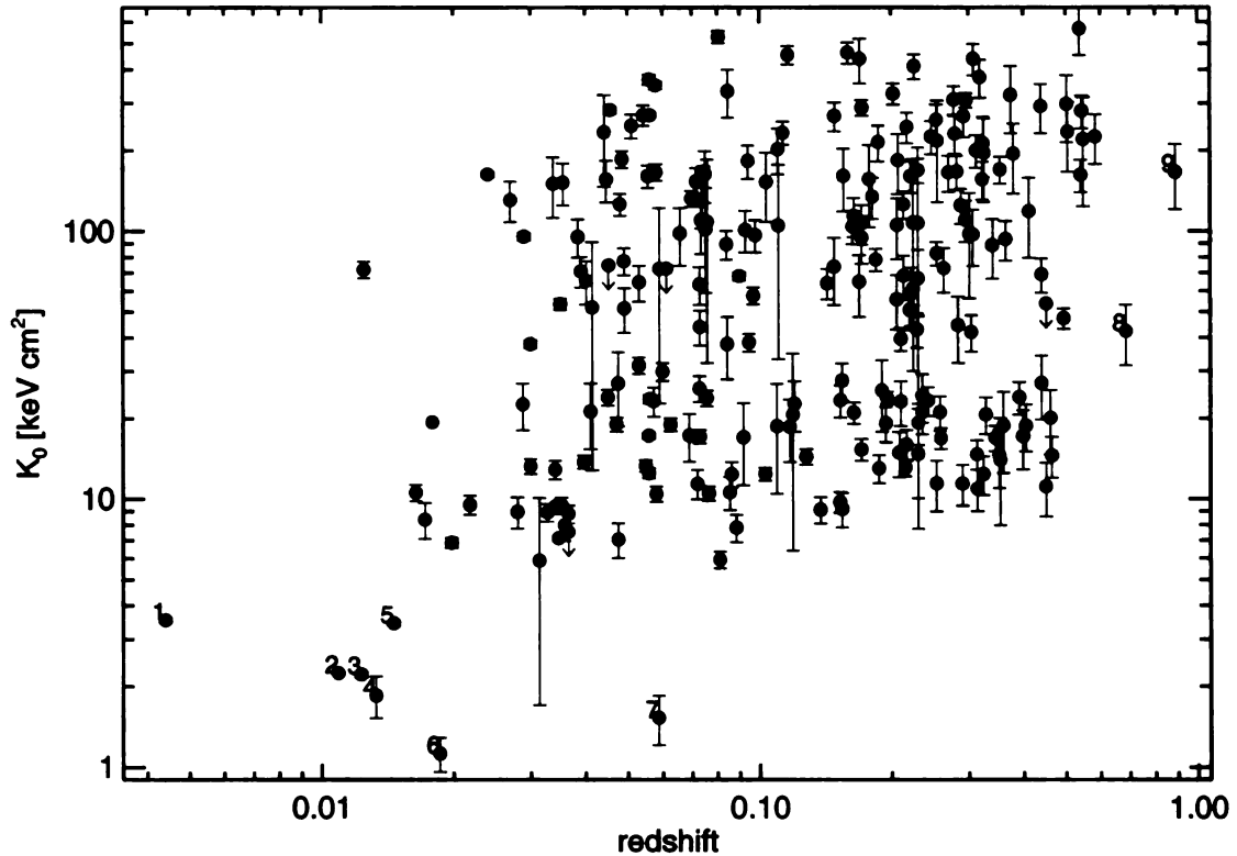
Figure 3.2 Best-fit K_0 versus redshift. Some clusters have K_0 error bars smaller than the point. The clusters with upper-limits ( black points with downward arrows ) are: A2151, AS0405, MS 0116.3-0115, and RX J1347.5-1145. The numerically labeled clusters are: (1) M87, (2) Centaurus Cluster, (3) RBS 533, (4) HCG 42, (5) HCG 62, (6) SS2B153, (7) A1991, (8) MACS0744.8+3927, and (9) CL J1226.9+3332. For CLJ1226, Maughan et al. (2007) found best-fit K_0 = 132 \pm 24 \text{ keV cm}^2 which is not significantly different from our value of K_0 = 166 \pm 45 \text{ keV cm}^2 . The lack of K_0 < 10 \text{ keV cm}^2 clusters at z > 0.1 is most likely the result of insufficient angular resolution (see §3.4.2).
