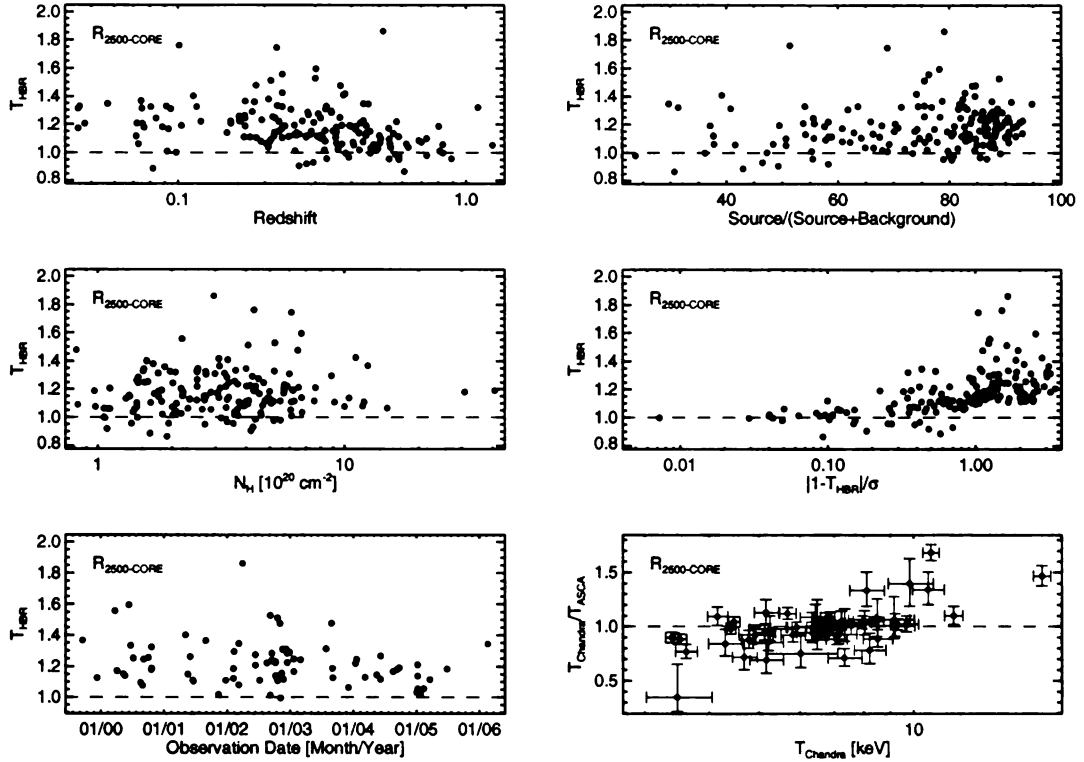
Figure 2.4 A few possible sources of systematic uncertainty vs. T_{HBR} calculated for the R_{2500} -CORE apertures (192 clusters). Error bars have been omitted in several plots for clarity. The line of equality is shown as a dashed line in all panels. ( Top left: ) T_{HBR} vs. redshift for the entire sample. The trend in T_{HBR} with redshift is expected as the T_{2.0-7.0} lower boundary nears convergence with the T_{0.7-7.0} lower boundary at z \approx 1.85 . Weighted values of T_{HBR} are consistent with unity starting at z \sim 0.6 . ( Top right: ) T_{HBR} vs. percentage of spectrum flux which is attributed to the source. We find no trend with signal-to-noise which suggests calibration uncertainty not is playing a major role in our results. ( Middle left: ) T_{HBR} vs. Galactic column density. We find no trend in absorption which would result if N_H values are inaccurate or if we had improperly accounted for local soft contamination. ( Middle right: ) T_{HBR} vs. the deviation from unity in units of measurement uncertainty. Recall that we have used 90% confidence ( 1.6\sigma ) for our analysis. ( Bottom left: ) T_{HBR} plotted vs. observation start date. The plotted points are culled from the full sample and represent only clusters which have a single observation and where the spectral flux is > 75\% from the source. We note no systematic trend with time. ( Bottom right: ) Ratio of Chandra temperatures derived in this work to ASCA temperatures taken from Horner (2001). We note a trend of comparatively hotter Chandra temperatures for clusters > 10 keV, otherwise our derived temperatures are in good agreement with those of ASCA .
