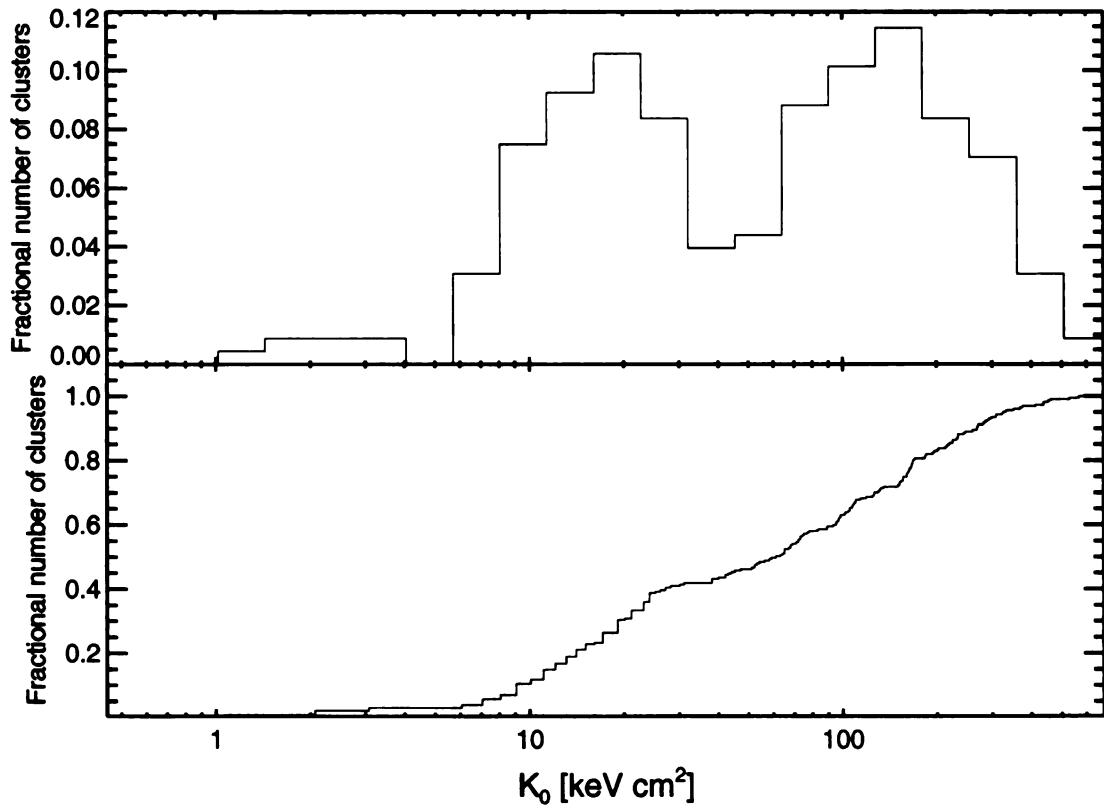
Figure 3.4 Top panel: Histogram of best-fit K_0 for all the clusters in ACCEPT . Bin widths are 0.15 in log space. Bottom panel: Cumulative distribution of K_0 values for the full sample. The distinct bimodality in K_0 is present in both distributions, which would not be seen if it were an artifact of the histogram binning. A KMM test finds the K_0 distribution cannot arise from a simple unimodal Gaussian.
