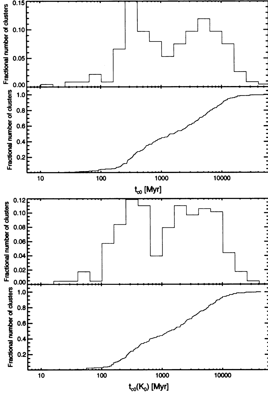
Figure 3.6 Top panel: Log-binned histogram and cumulative distribution of best-fit core cooling times, t_{c0} (eqn. 3.8), for all the clusters in ACCEPT . Histogram bin widths are 0.2 in log space. Bottom panel: Log-binned histogram and cumulative distribution of core cooling times calculated from best-fit K_0 values, t_{c0}(K_0) (eqn. 3.9), for all the clusters in ACCEPT . Histogram bin widths are 0.2 in log space. The bimodality we observe in the K_0 distribution is also present in best-fit t_{c0} . However, the gaps between the two populations of t_{c0} and t_{c0}(K_0) differ by \sim 0.3 Gyrs with scaled-entropy having the more pronounced gap with a shorter cooling time.
