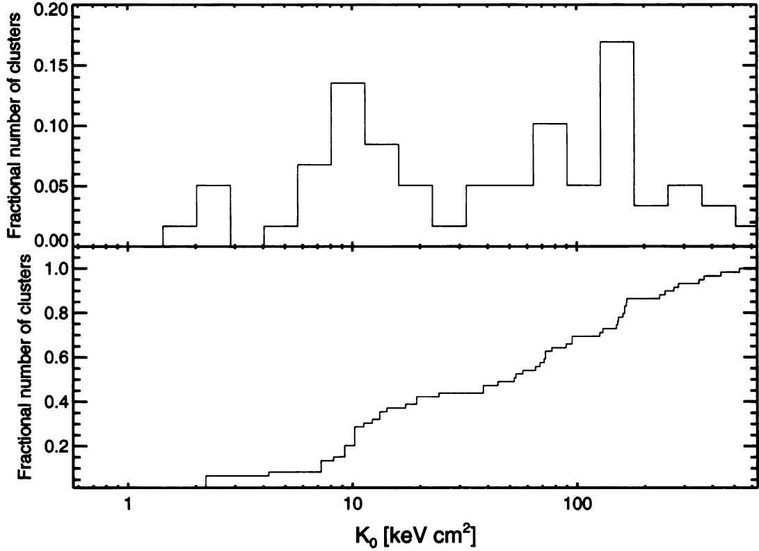
Figure 3.5 Top panel: Histogram of best-fit K_0 values for the primary HIFLUGCS sample. Bin widths are 0.15 in log space. Bottom panel: Cumulative distribution of best-fit K_0 values. The distinct bimodality seen in the full ACCEPT sample (Fig. 3.4) is also present in the HIFLUGCS subsample and shares the same gap starting at K_0 \approx 30 \text{ keV cm}^2 . That bimodality is present in both samples is strong evidence it is not a result of an unknown archival bias.
