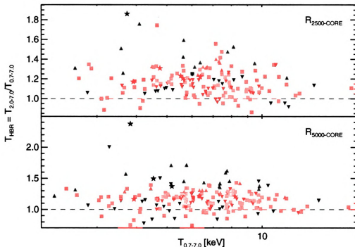
Figure 2.8 T_{HBR} plotted against T_{0.7-7.0} for the R_{2500} -CORE and R_{5000} -CORE apertures. Note that the vertical scales for both panels are not the same. The top and bottom panels contain 192 and 166 clusters, respectively. Only two clusters – Abell 697 and MACS J2049.9-3217 – do not have a T_{HBR} > 1.1 in one aperture and not the other. In both cases however, it was a result of narrowly missing the cut. The dashed lines are the lines of equivalence. Symbols and color coding are based on two criteria: (1) the presence of a CC and (2) the value of T_{HBR} . Black stars (6 in the top panel; 7 in the bottom) are clusters with a CC and T_{HBR} significantly greater than 1.1. Green upright-triangles (21 in the top; 27 in the bottom) are NCC clusters with T_{HBR} significantly greater than 1.1. Blue down-facing triangles (49 top; 60 bottom) are CC clusters and red squares (90 top; 98 bottom) are NCC clusters. We have found most, if not all, of the clusters with T_{HBR} \gtrsim 1.1 are merger systems. Note that the cut at T_{HBR} > 1.1 is arbitrary and there are more merger systems in our sample than just those highlighted in this figure. However it is rather suggestive that clusters with the highest values of T_{HBR} appear to be merging systems.
