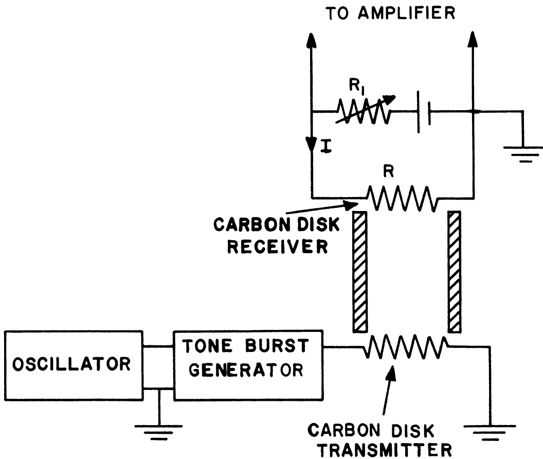
Figure 13 A schematic diagram of the apparatus used to measure the second sound amplitude T_2' produced by the carbon disk transmitter.
