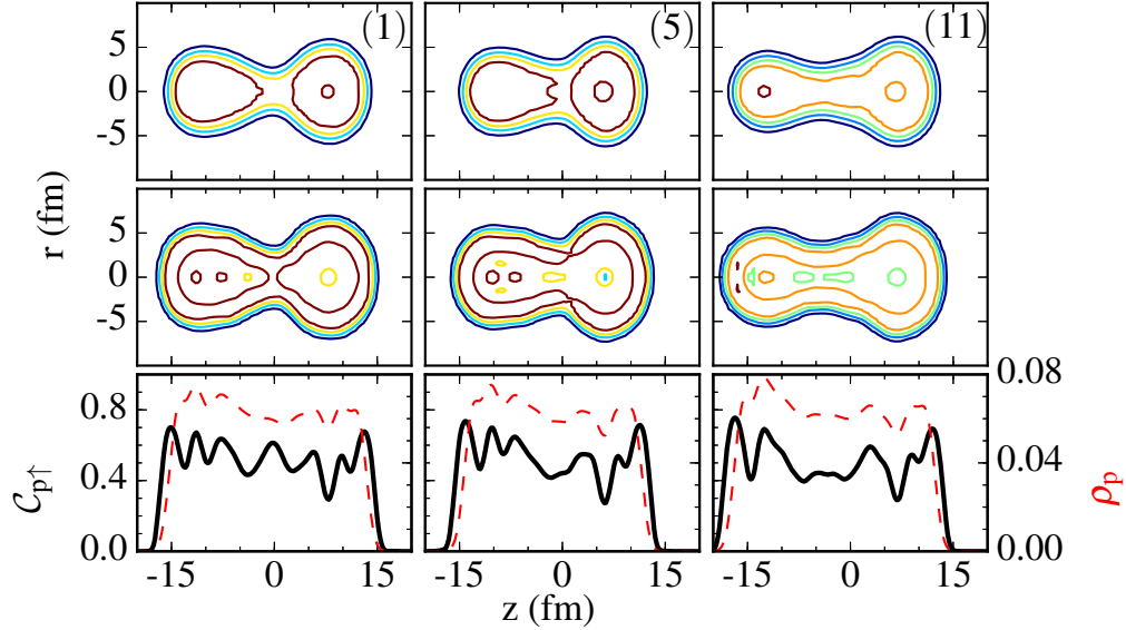
Figure 4.16: Same as Fig. 4.15, but for protons.
