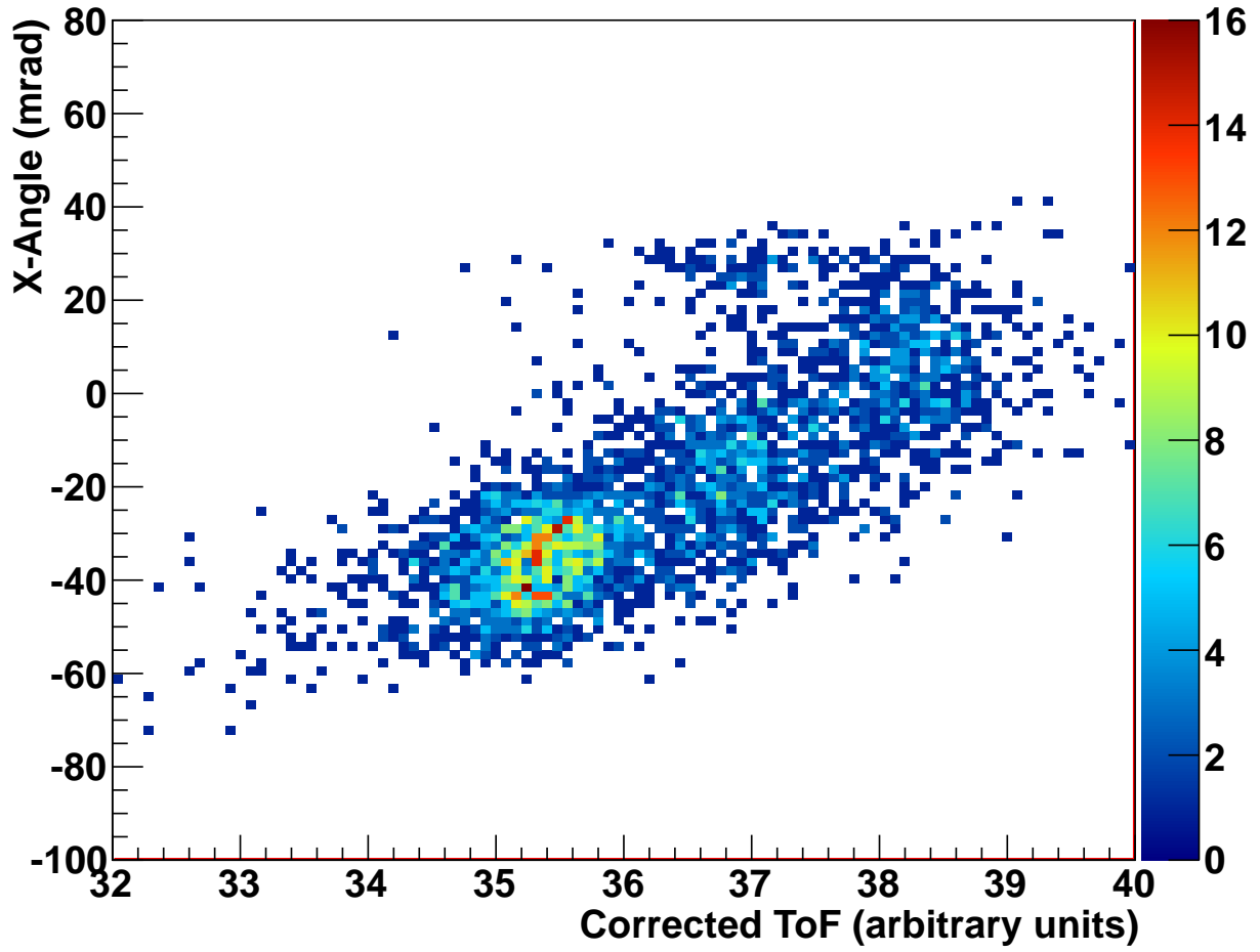
Figure 3.8: The angular correlation of oxygen isotopes to time-of-flight. The lighter isotopes are bent more by the sweeper magnet, so the isotopes of oxygen are identified (from left to right) as ^{22}\text{O} , ^{23}\text{O} , and ^{24}\text{O} .
