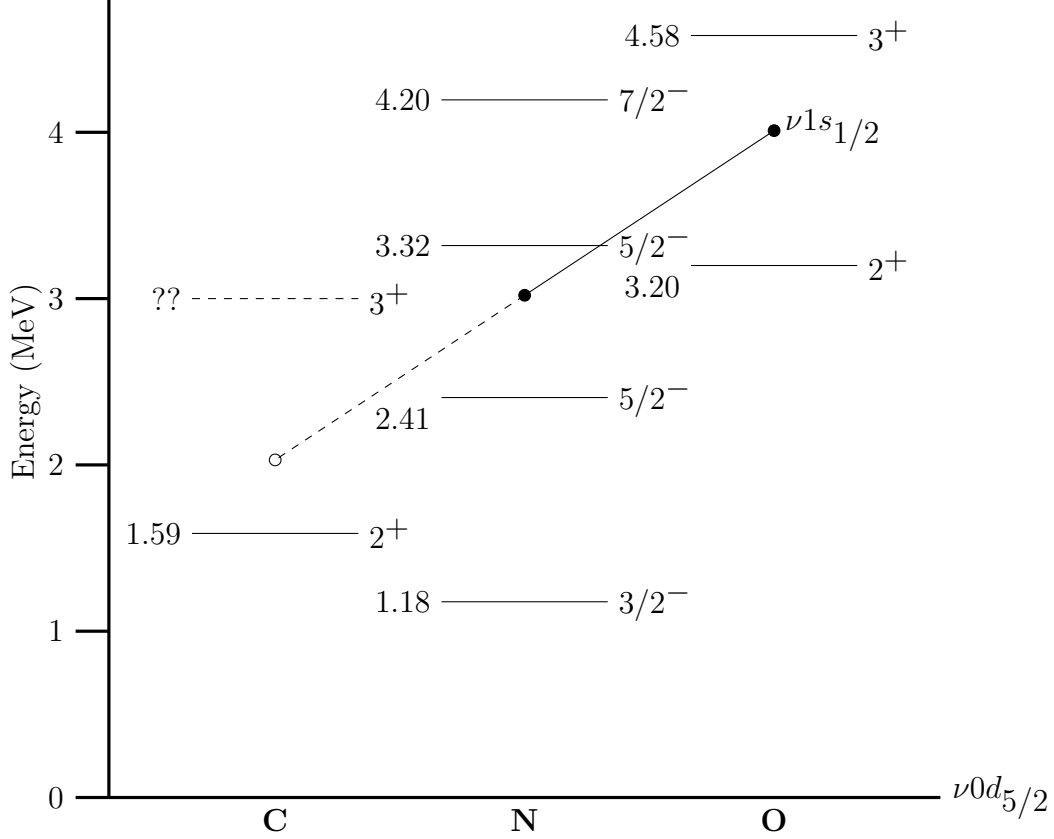
Figure 5.1: The “competition” between the \nu 0d_{5/2} and \nu 1s_{1/2} levels for the N = 14 isotones of carbon, nitrogen, and oxygen following the prescription of Ref. [31]. Experimental data for the levels of ^{22}\text{O} , ^{21}\text{N} , and ^{20}\text{C} are taken from Refs. [30],[29], and [27]. Higher excited states in ^{20}\text{C} , like the next expected \nu 1s_{1/2} -particle state with J^\pi = 3^+ , have not been observed.
