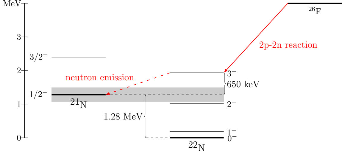
Figure 4.1: The proposed level scheme of ^{22}\text{N} \rightarrow ^{21}\text{N} + n decay created from a reaction of ^{26}\text{F} .
