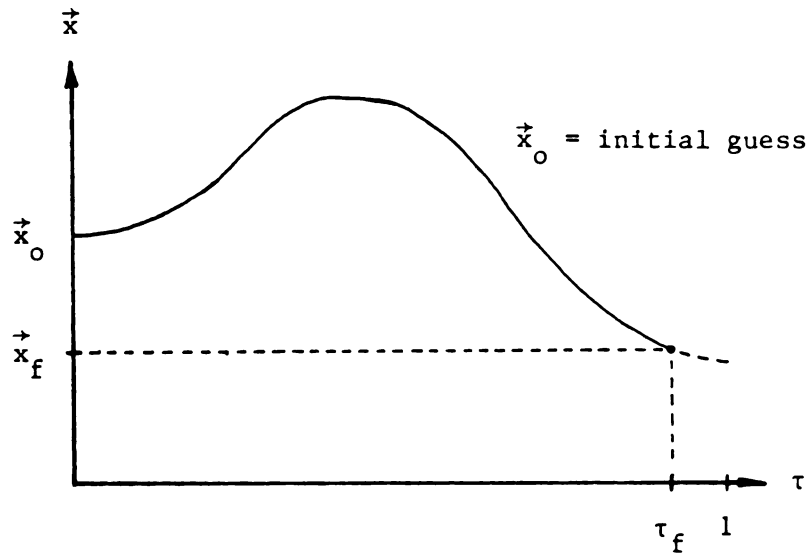
Figure 6.5.1. Typical path for continuation method in (\vec{x}, \tau) space.
