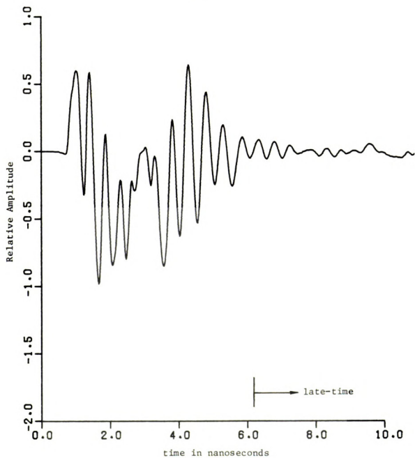
Figure 8.5.8. Convolution of 707 E-pulse with measured 707 response.
