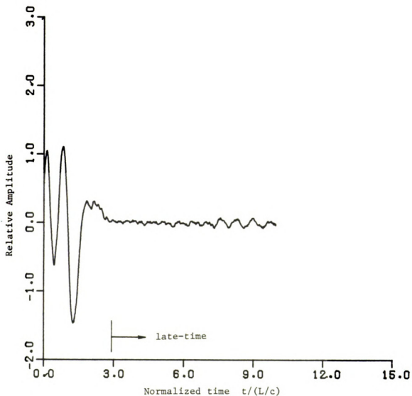
Figure 5.5.2.27. Best fit difference plot for sine third mode, noisy impulse response convolution.
