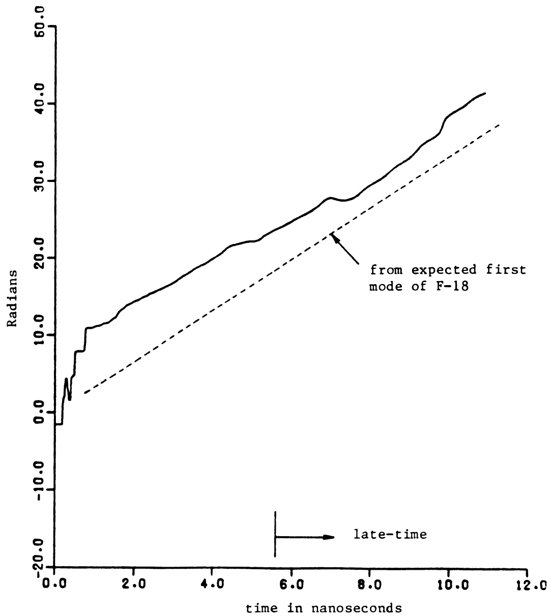
Figure 8.5.25. Radian frequency plot from convolution of first mode F-18 excitation signals with measured 707 response.
