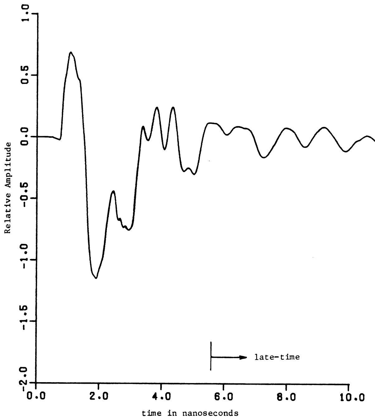
Figure 8.5.11. Convolution of F-18 E-pulse with measured 707 response.
