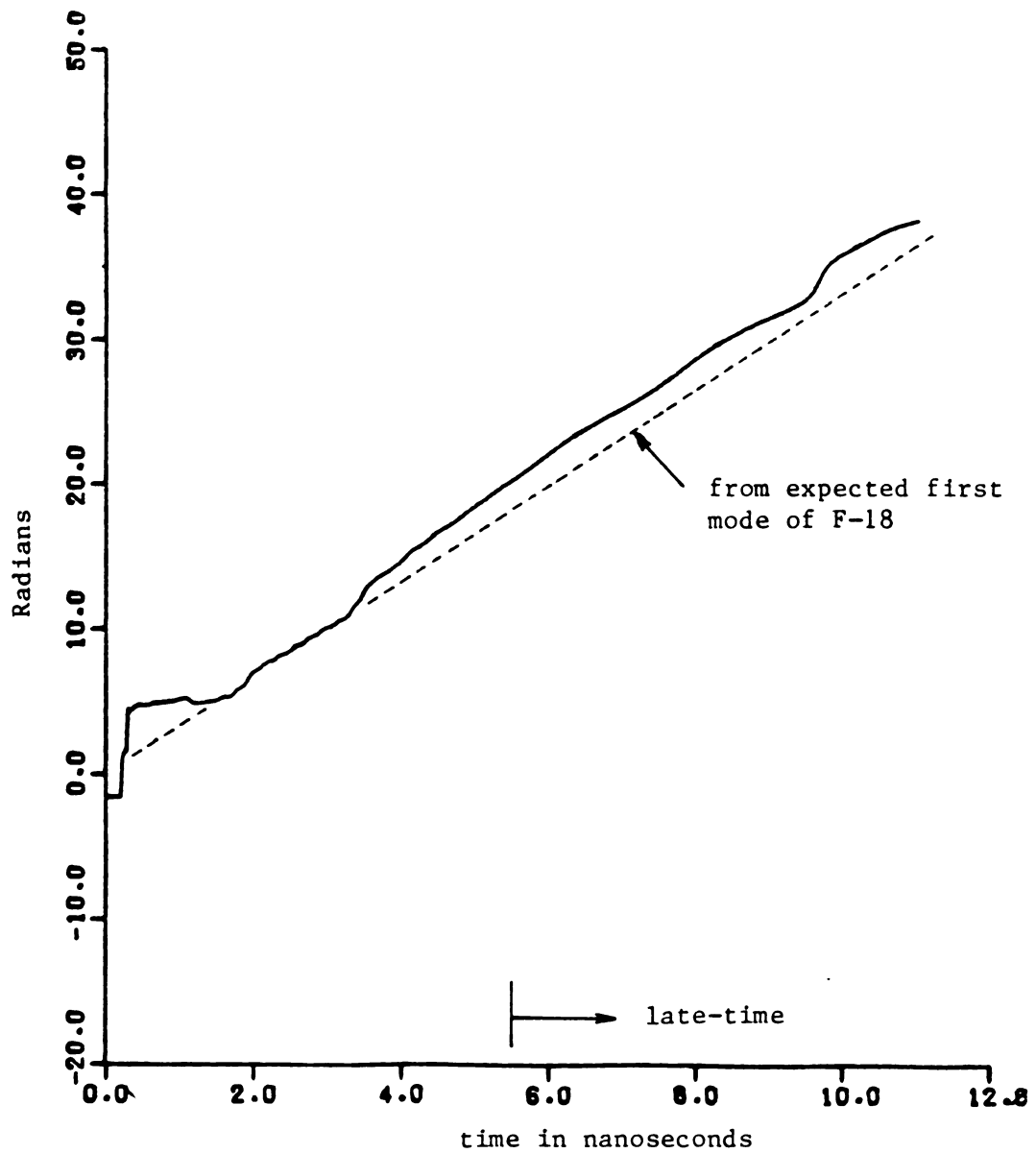
Figure 8.5.17. Radian frequency plot from convolution of first mode F-18 excitation signals with measured F-18 response.
