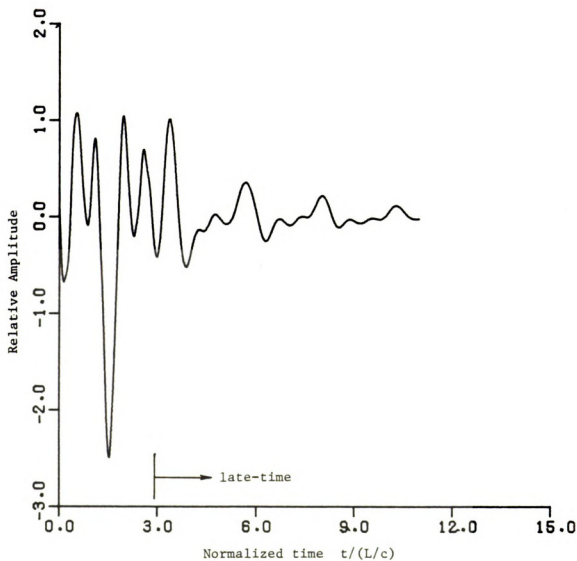
Figure 5.5.2.19. Best fit difference plot for sine third mode, 10% longer cylinder convolution.
