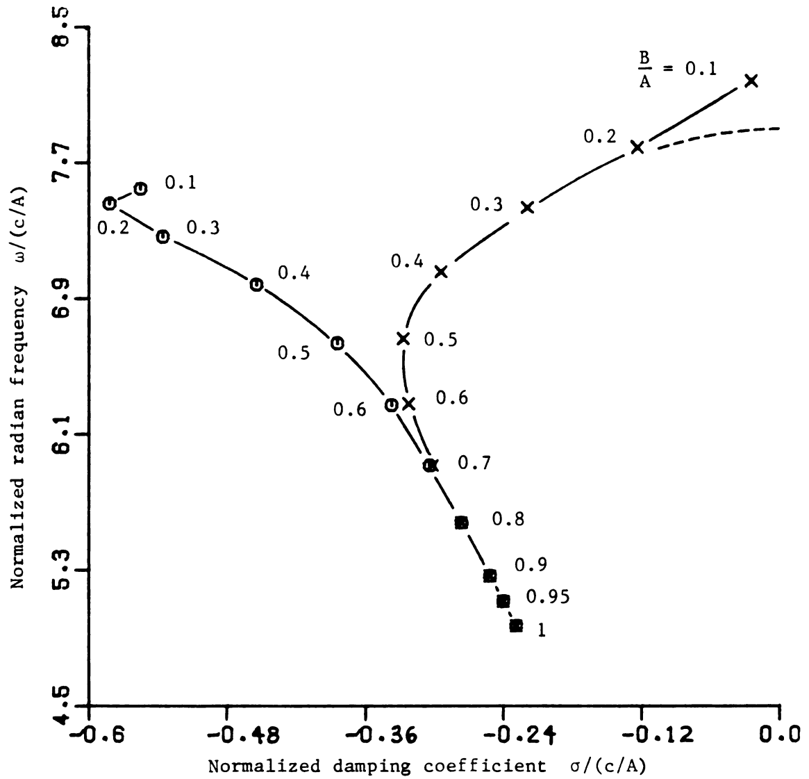
Figure 7.7.6. Case 1 (circles) and case 2 (crosses) natural frequencies of thin wire ellipse of wire radius a=0.01A arising from n=5 circular mode, for various values of B/A . Dotted line shows expected trajectory for transmission line limit.
