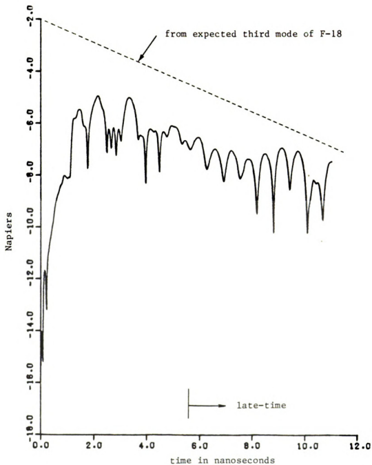
Figure 8.5.20. Damping coefficient plot from convolution of third mode F-18 excitation signals with measured F-18 response.
