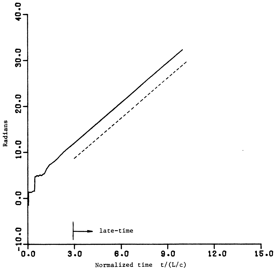
Figure 5.5.2.6. Radian frequency plot from first mode excitation signal convolutions. Dotted line is radian frequency plot of expected first mode.
