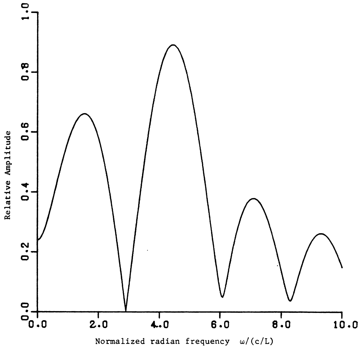
Figure 5.5.1.23. Spectrum of one mode damped sinusoid based E-pulse for \sigma = -0.2601 c/L.
