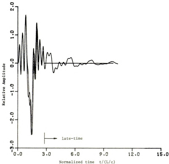
Figure 5.5.1.9. Convolution of forced E-pulse of duration T_e = 1.8 L/c with impulse response of thin cylinder of expected length, and with impulse response of a cylinder 5% longer.
