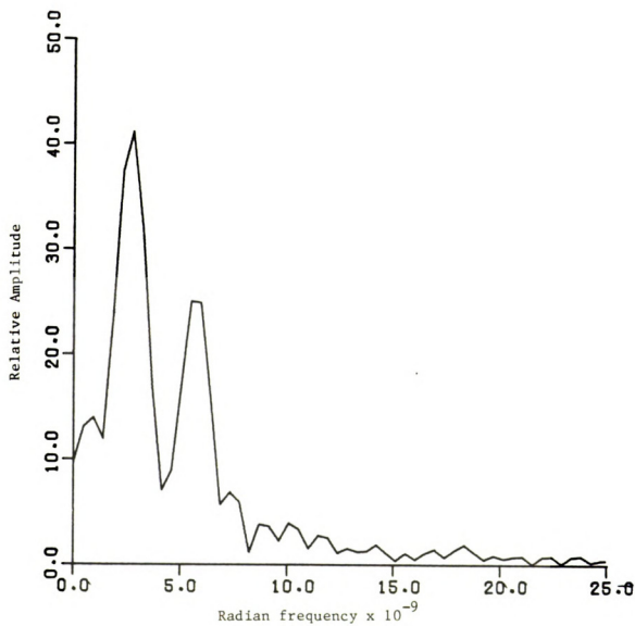
Figure 8.4.10. Fourier spectrum of measured 12 1/2" inclined thin cylinder scattered field response, obtained via FFT.
