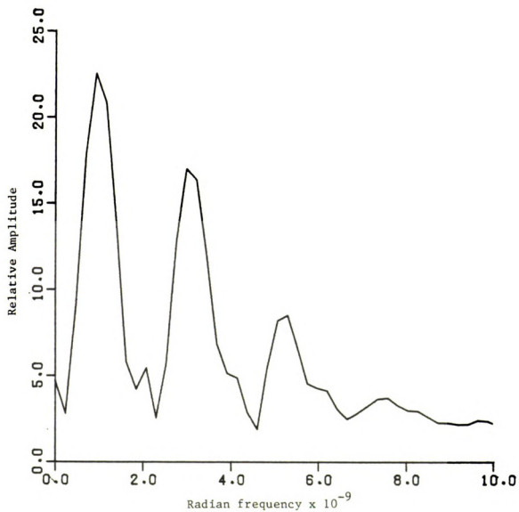
Figure 8.4.4. Fourier spectrum of 18½" thin cylinder measured surface current response, obtained via FFT.
