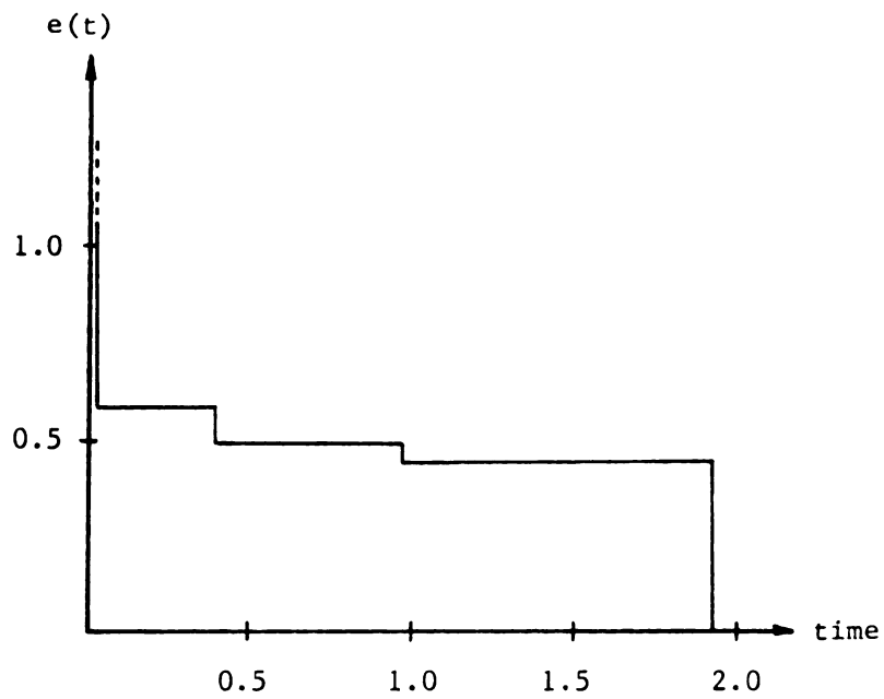
Figure 4.7.8. Two mode E-pulse synthesized via nonlinear E-pulse analysis.
