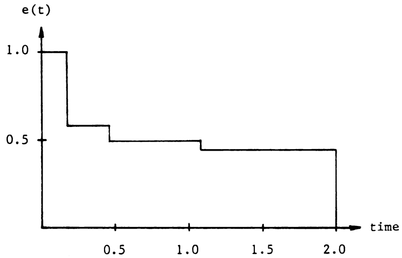
Figure 4.7.7. Two mode E-pulse synthesized via nonlinear E-pulse analysis.
