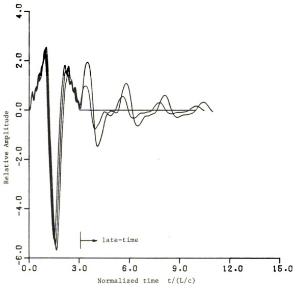
Figure 5.5.1.8. Convolution of natural E-pulse with impulse response of thin cylinder of expected length, and with impulse responses of cylinders 5% and 10% longer.
