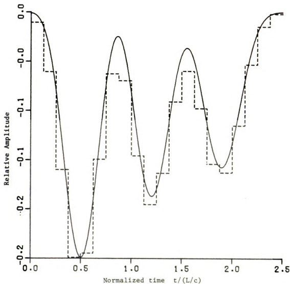
Figure 4.5.6.14. Forced sine single mode excitation waveforms of duration T_e = 2.5 L/c synthesized using pulse and Fourier cosine basis sets to excite the third mode of the thin cylinder, and eliminate modes one, two, and four through ten.
