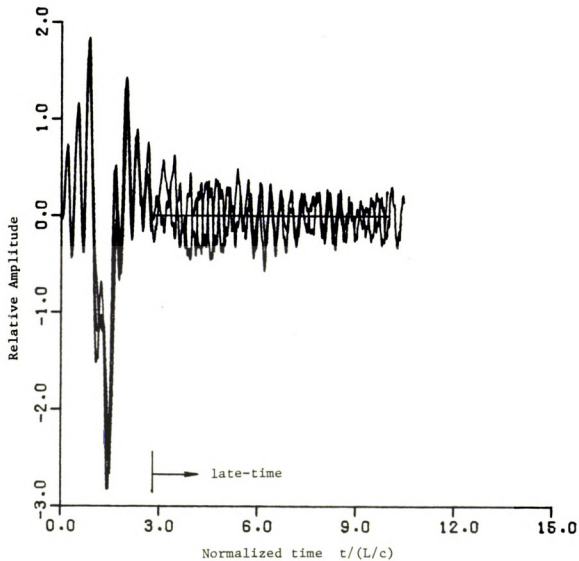
Figure 5.5.1.14. Convolution of forced E-pulse of duration T_e = 1.8 L/c with noisy impulse response of thin cylinder of expected length, and with noisy impulse response of a cylinder 5% longer.
