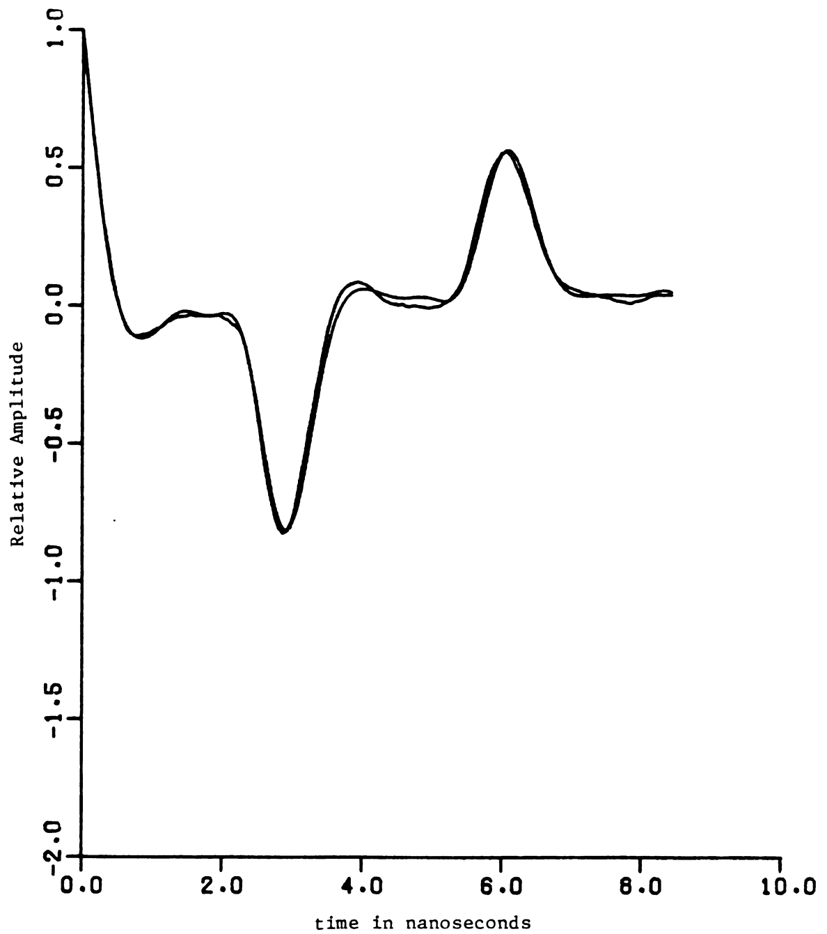
Figure 8.4.6. Four mode best fit to late-time, clutter free portion of measured 18\frac{1}{4} " thin cylinder surface current response.
