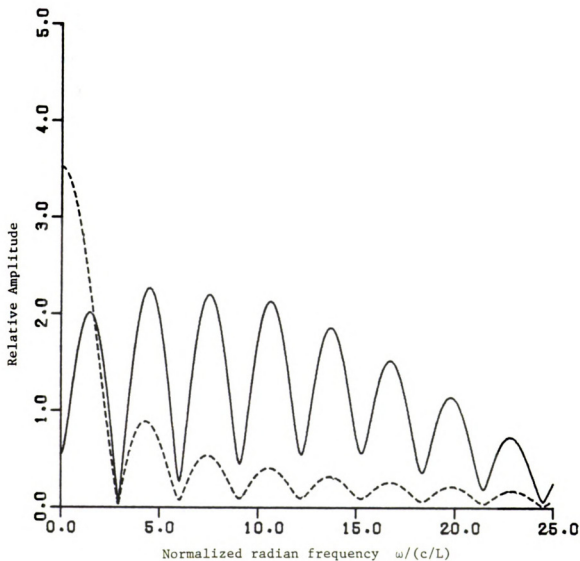
Figure 5.5.1.7. Spectra of natural E-pulse (dotted line) and natural DC E-pulse (solid line) for \sigma=-0.2601 c/L.
