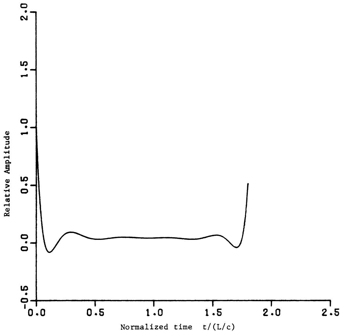
Figure 4.5.6.17. Forced E-pulse of duration T_e = 1.8 L/c synthesized using polynomial basis set to eliminate first ten modes of the thin cylinder.
