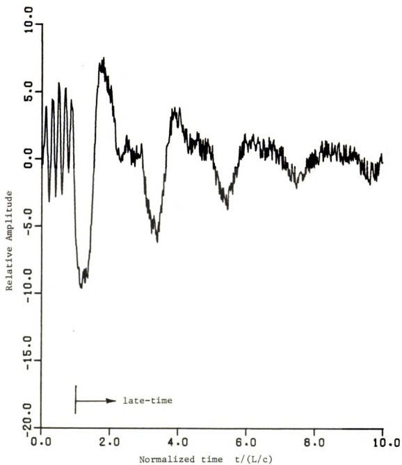
Figure 5.5.1.11. Five mode 60° thin cylinder impulse response with 10% random noise added.
