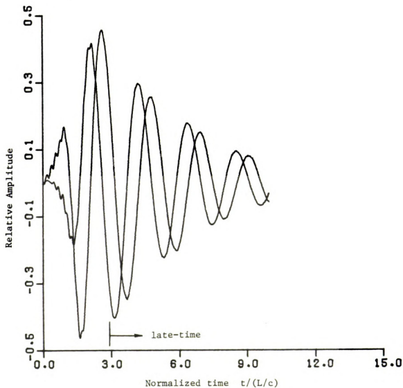
Figure 5.5.2.20. Convolution of first mode sine and cosine excitation signals with noisy five mode 60^\circ thin cylinder impulse response.
