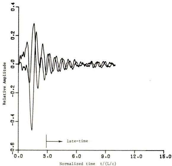
Figure 5.5.2.21. Convolution of third mode sine and cosine excitation signals with noisy five mode 60^\circ thin cylinder impulse response.
