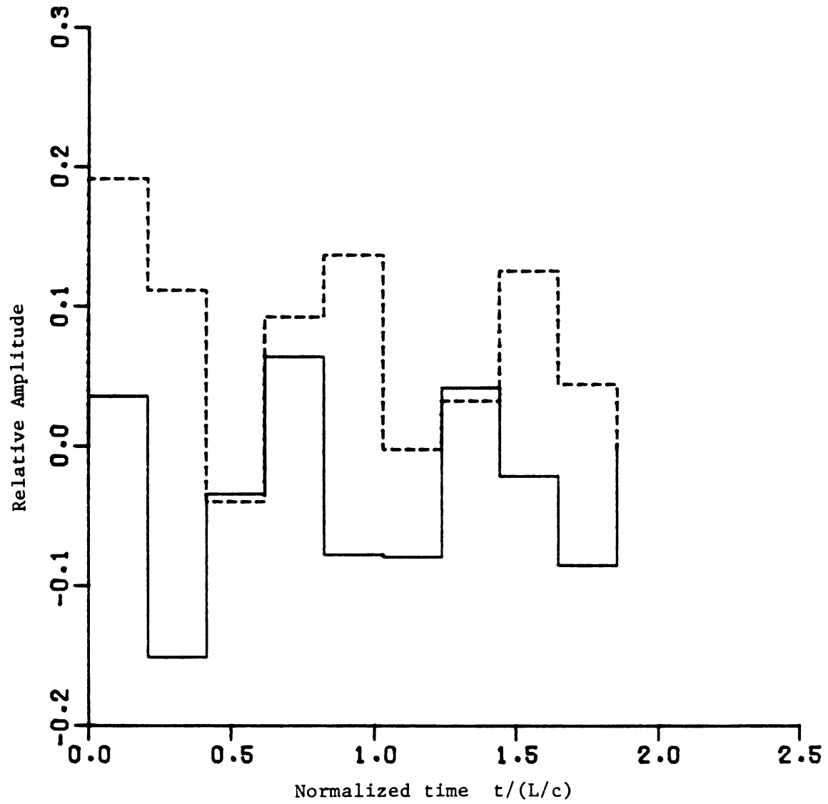
Figure 5.5.2.2. Natural sine (dotted line) and cosine (solid line) third mode excitation signals of minimum duration for five mode thin cylinder.
