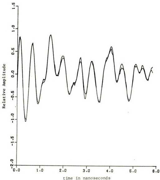
Figure 8.5.4. Seven mode best fit to late-time portion of measured 707 scattered field response.
