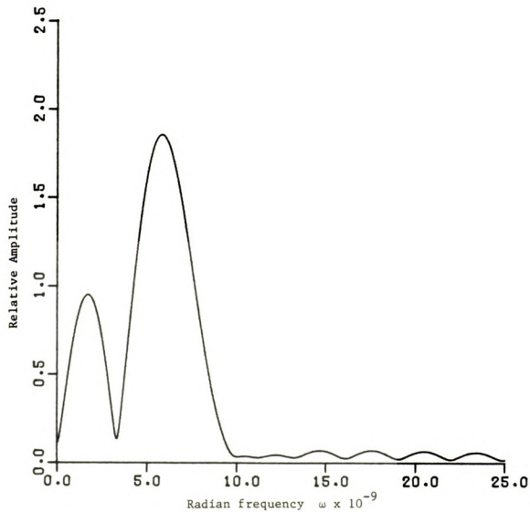
Figure 5.5.2.31. Spectrum of F-18 Fourier cosine second mode excitation signal at \sigma = -0.13 \times 10^9 .
