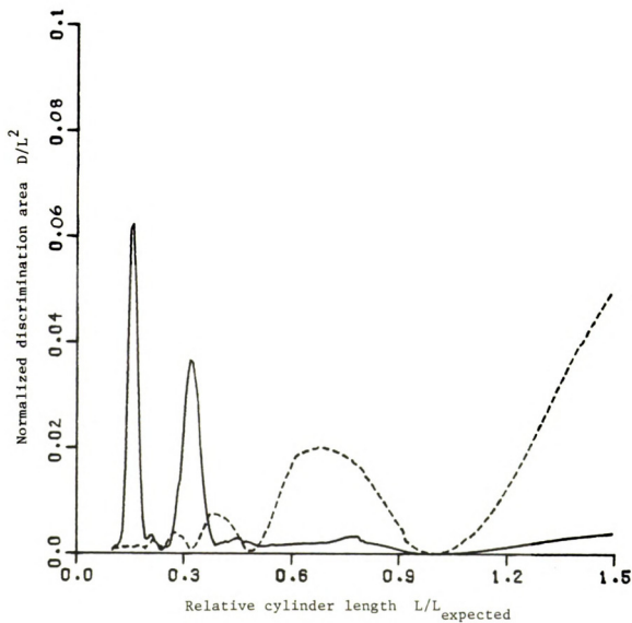
Figure 5.5.1.15. Discrimination area of 60^\circ five mode thin cylinder excited by natural E-pulse (dotted line) and forced E-pulse of duration T_0 = 1.8 L/c (solid line).
