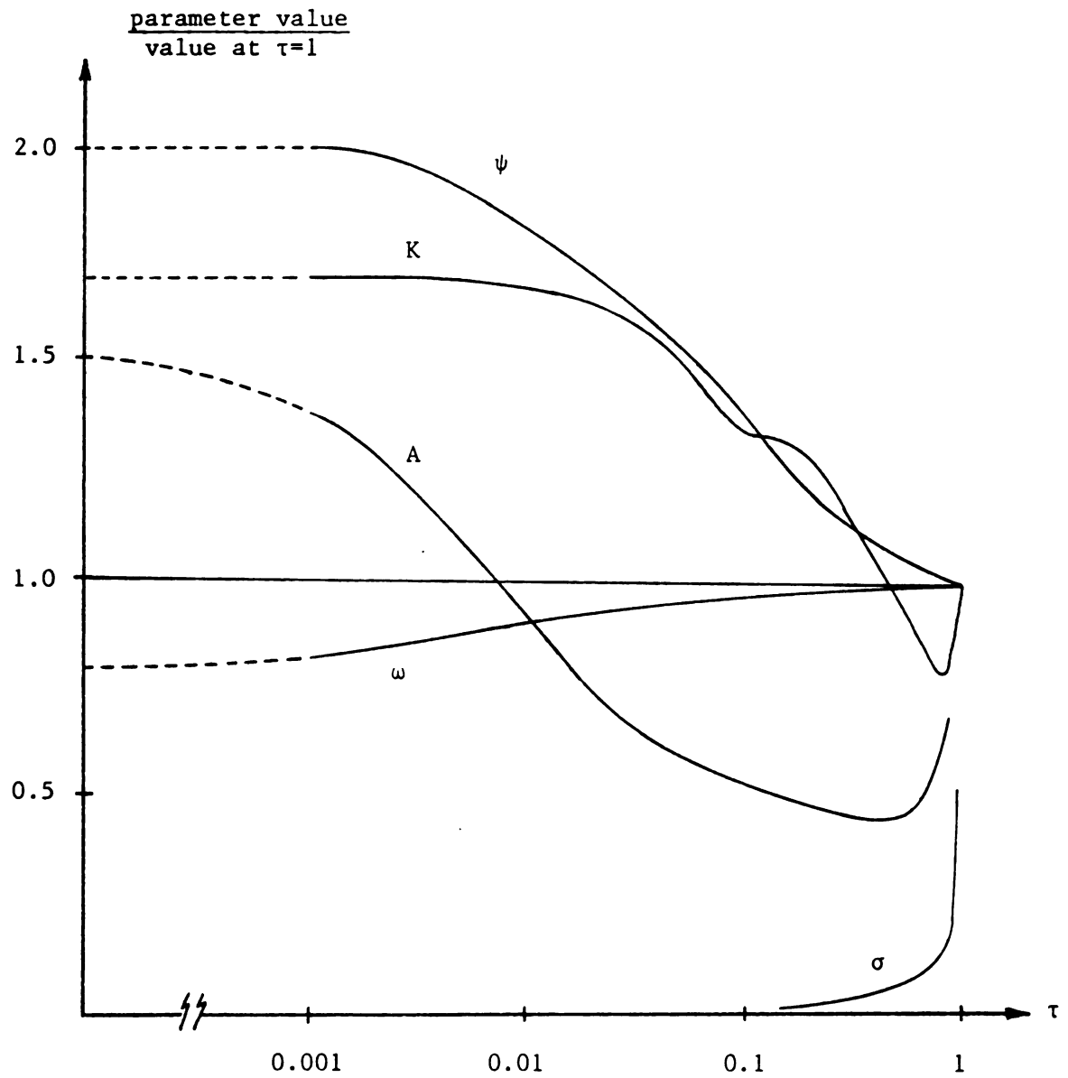
Figure 6.5.4. Example solution using the continuation method.
