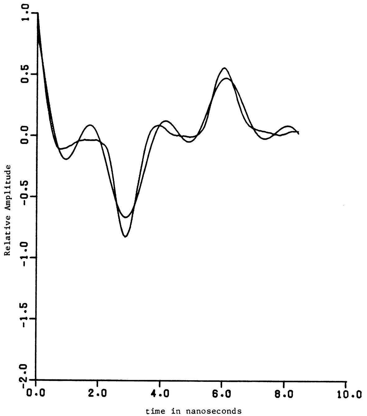
Figure 8.4.5. Two mode best fit to late-time, clutter free portion of measured 18 \frac{1}{4} " thin cylinder surface current response.
