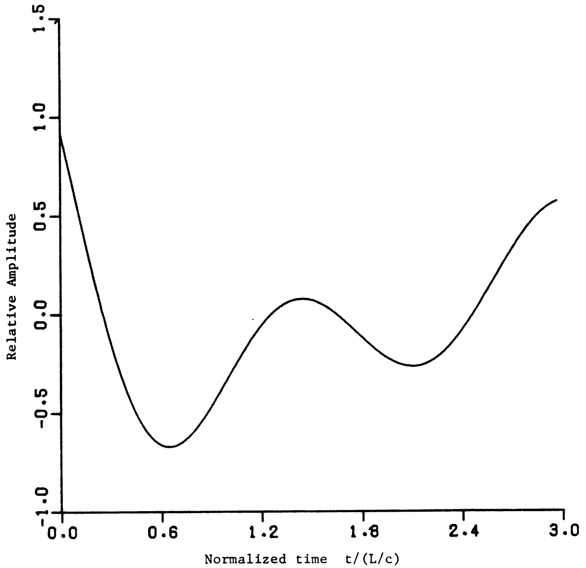
Figure 5.5.1.22. Natural E-pulse of minimum duration synthesized using damped sinusoid basis functions to eliminate the first mode of the thin cylinder.
