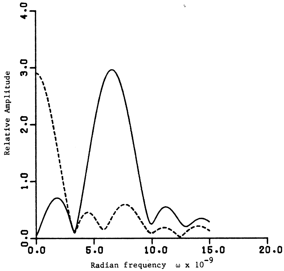
Figure 5.5.2.29. Spectra of pulse function (dotted line) and damped sinusoid (solid line) F-18 second mode excitation signals for \sigma = -0.13 \times 10^9 .
