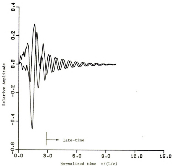
Figure 5.5.2.5. Convolution of third mode sine and cosine excitation signals with five mode 60^\circ thin cylinder impulse response.
