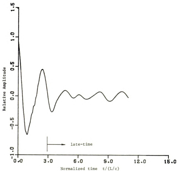
Figure 5.5.2.18. Best fit difference plot for sine first mode, 10% longer cylinder convolution.
