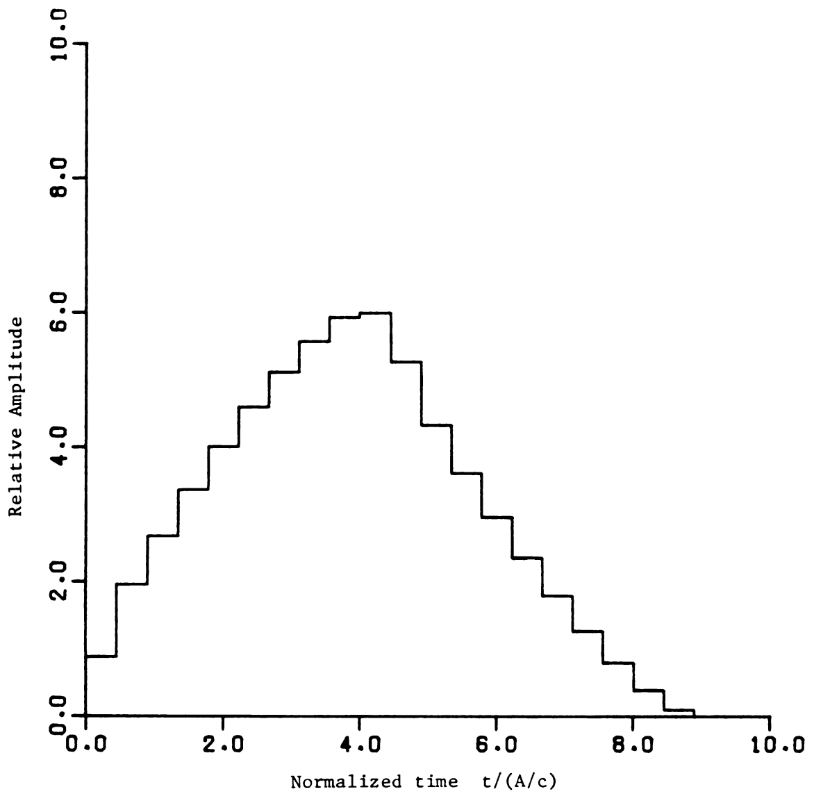
Figure 7.7.15. Natural E-pulse of minimum duration synthesized to eliminate the ten modes of the elliptical loop scatterer arising from the first five Type I circular modes, for B/A=0.4 .
