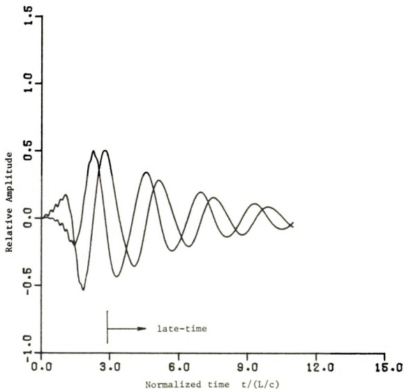
Figure 5.5.2.12. Convolution of first mode sine and cosine excitation signals with five mode impulse response of 60^\circ thin cylinder which is 10% longer than expected.
