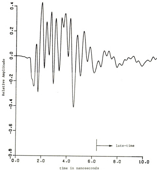
Figure 8.5.10. Convolution of 707 E-pulse with measured F-18 response.
