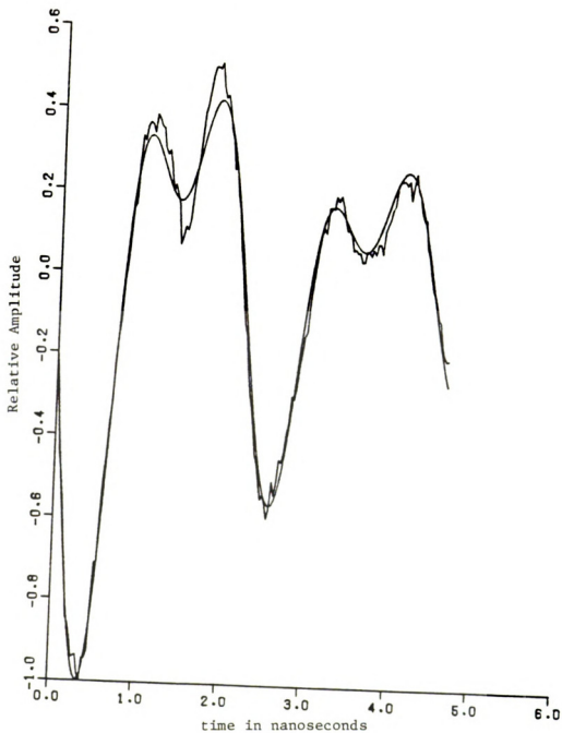
Figure 8.4.11. Three mode best fit to late-time portion of measured 12\frac{1}{2} " inclined thin cylinder scattered field response.
