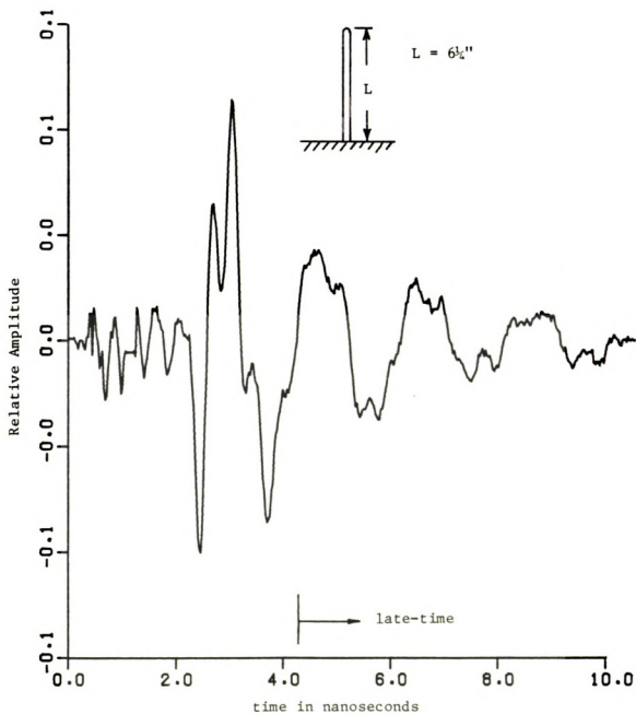
Figure 8.4.7. Measured scattered field response of a thin cylinder of length 6.25 inches placed perpendicular to the ground screen.
