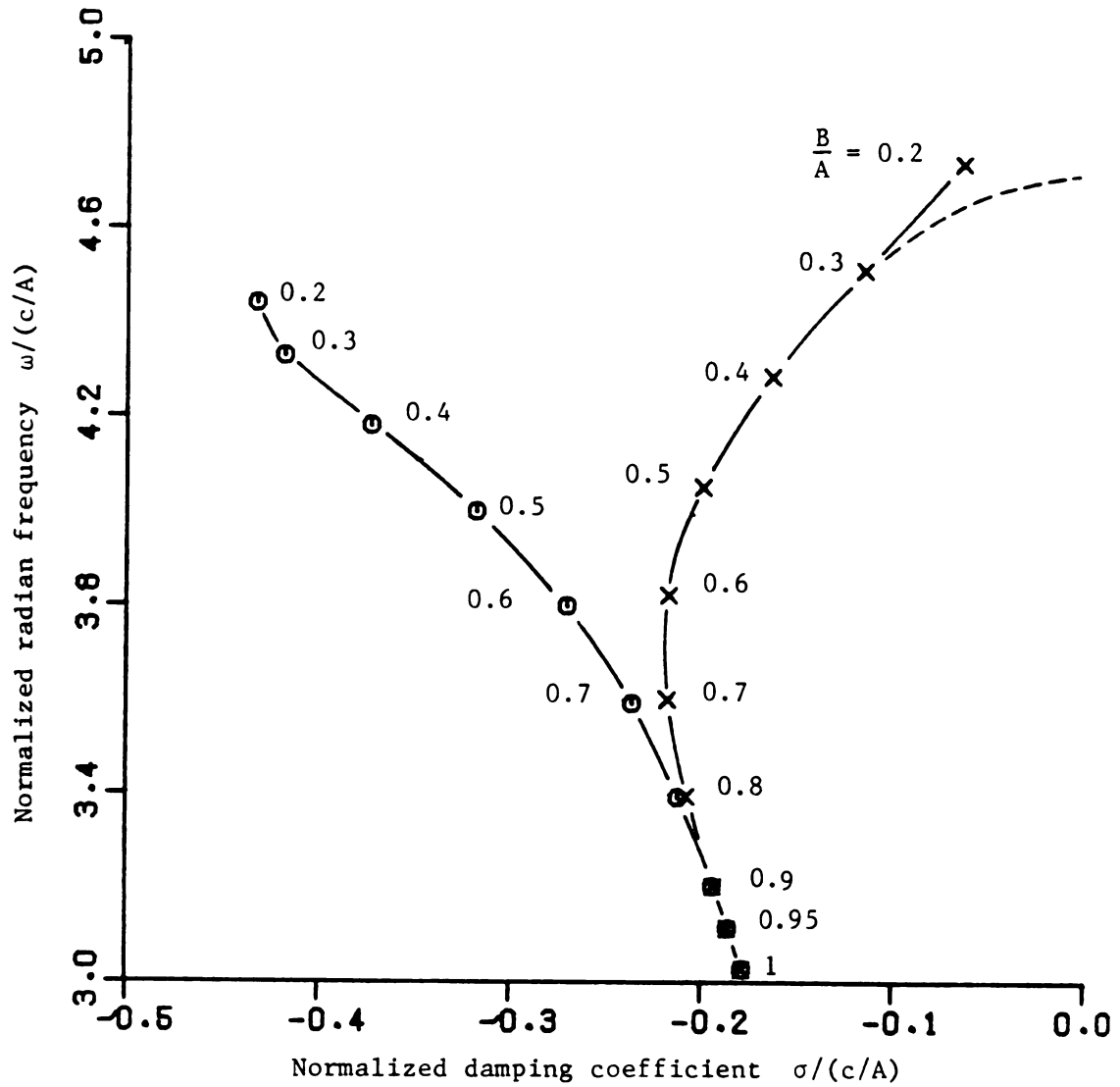
Figure 7.7.4. Case 1 (circles) and case 2 (crosses) natural frequencies of thin wire ellipse of wire radius a=0.01A arising from n=3 circular mode, for various values of B/A . Dotted line shows expected trajectory for transmission line limit.
