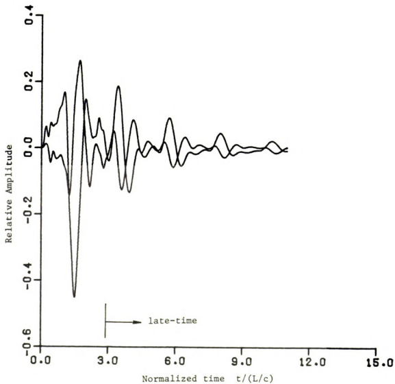
Figure 5.5.2.13. Convolution of third mode sine and cosine excitation signals with five mode impulse response of 60^\circ thin cylinder which is 10% longer than expected.
