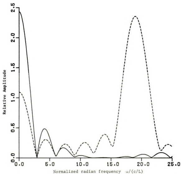
Figure 5.5.1.6. Spectra of forced E-pulses of duration T_e = 2.5 L/c (solid line) and T_e = 1.8 L/c (dotted line) for \sigma = -0.2601 c/L .
