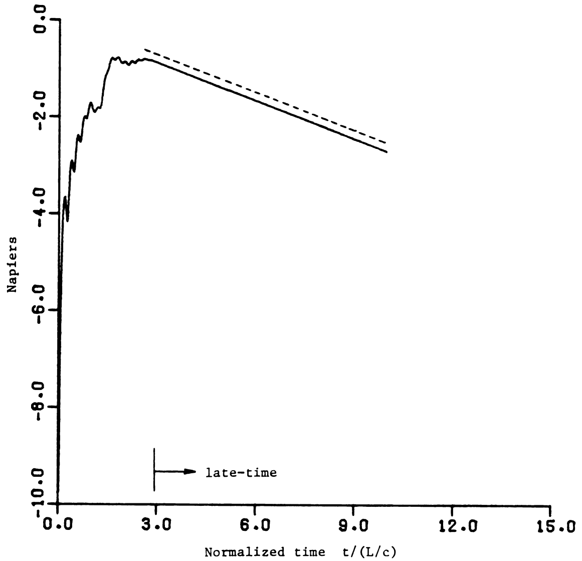
Figure 5.5.2.7. Damping coefficient plot from first mode excitation signal convolutions. Dotted line is damping coefficient plot of expected first mode.
