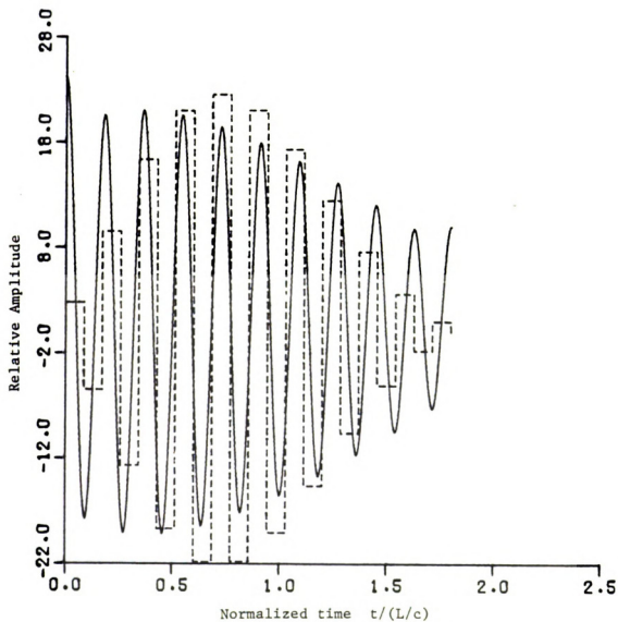
Figure 4.5.6.4. Forced E-pulses of duration T = 1.8 L/c synthesized using pulse and Fourier cosine basis sets to eliminate first ten modes of thin cylinder.
