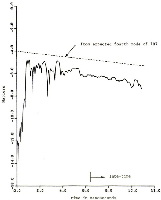
Figure 8.5.16. Damping coefficient plot from convolution of fourth mode 707 excitation signals with measured 707 response.
