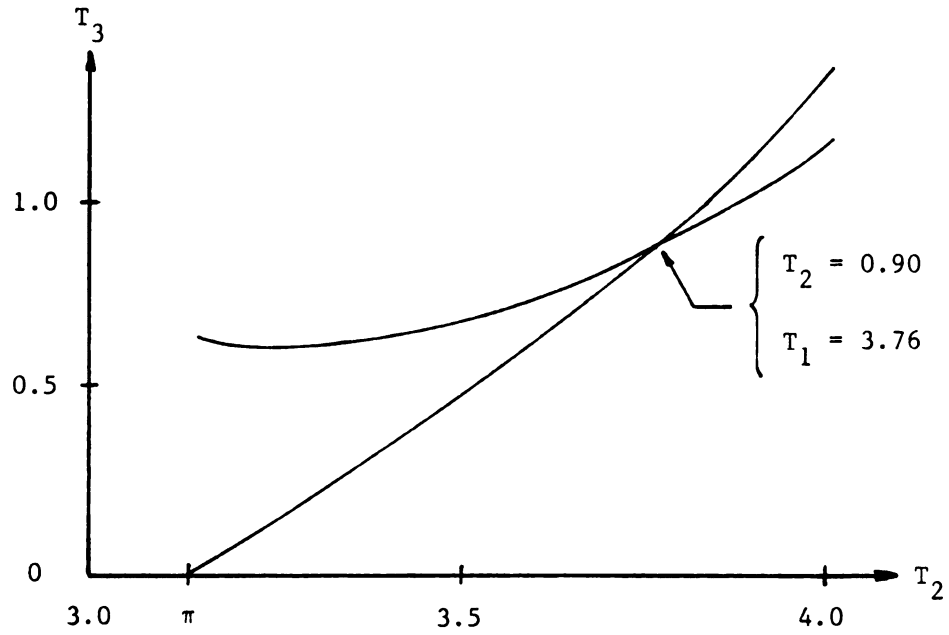
Figure 4.7.3. Graphical solution for impulse positions.
