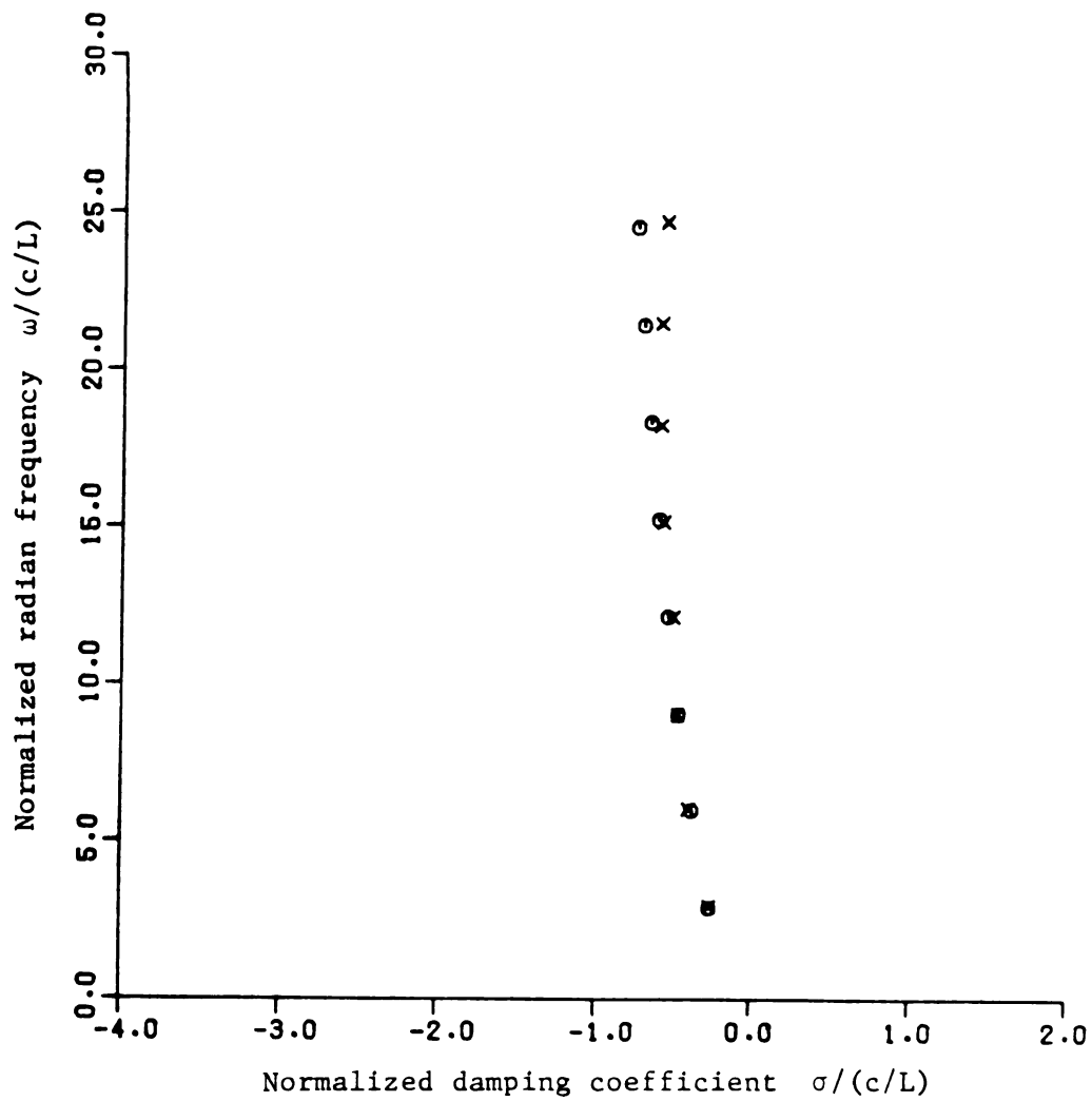
Figure 6.9.4. Natural frequencies extracted from noisy impulse response using continuation method with eight modes assumed ( \times ). Circles represent frequencies used to construct noise free impulse response.
