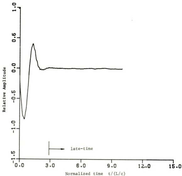
Figure 5.5.2.26. Best fit difference plot for sine first mode, noisy impulse response convolution.
