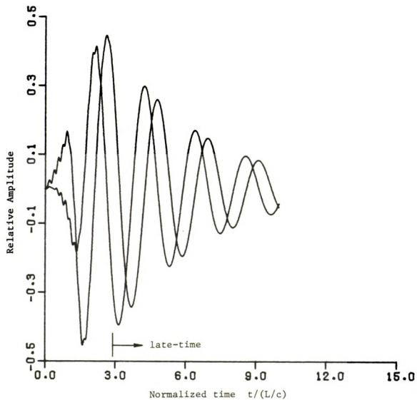
Figure 5.5.2.4. Convolution of first mode sine and cosine excitation signals with five mode 60^\circ thin cylinder impulse response.
