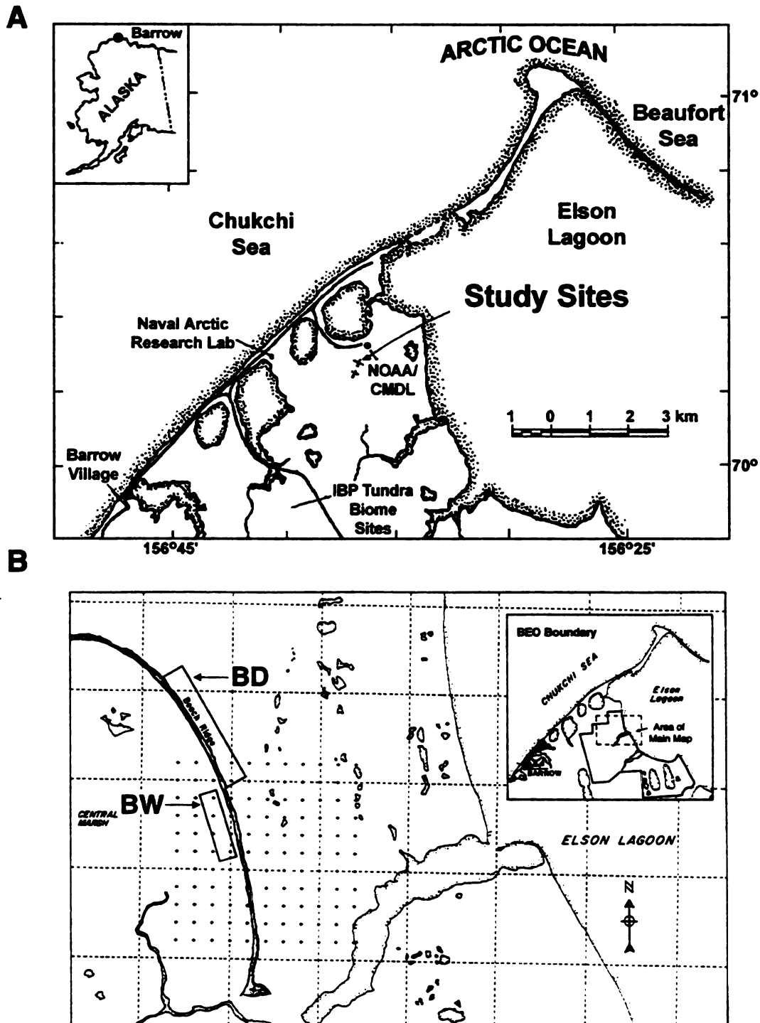
Figure I-20. A) Map of Barrow Peninsula and Alaska ( inset ) showing the study sites and other landmarks (Allessio and Tieszen 1975). B) Map of the research area and Barrow Peninsula ( inset ). The map displays the location of the sites (BD - Barrow Dry Heath; BW - Barrow Wet Meadow), ARCSS 1x1km grid ( crosses ), and other prominent features. The Boundary of the Barrow Environmental Observatory (BEO) is displayed on the inset (Hinkel et al. 1996).
