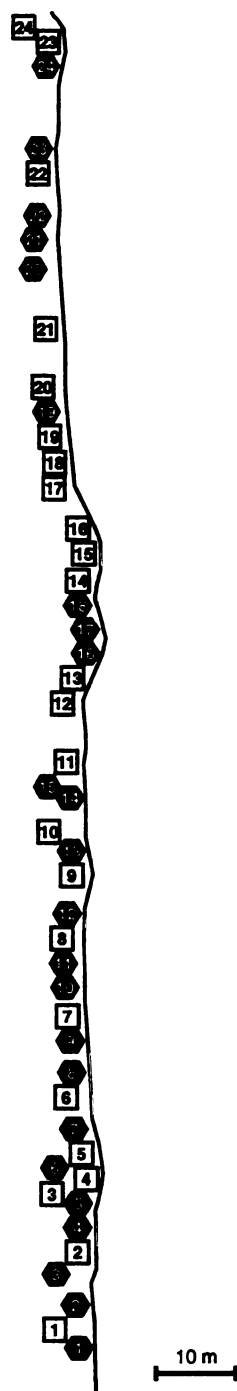
Figure A-4. Map of the plot locations within the Barrow Wet Meadow (BW) site. The closed hexagon symbol represents an open-top chamber (OTC), the open square symbol represents a control plot, and the line represents the boardwalk.
