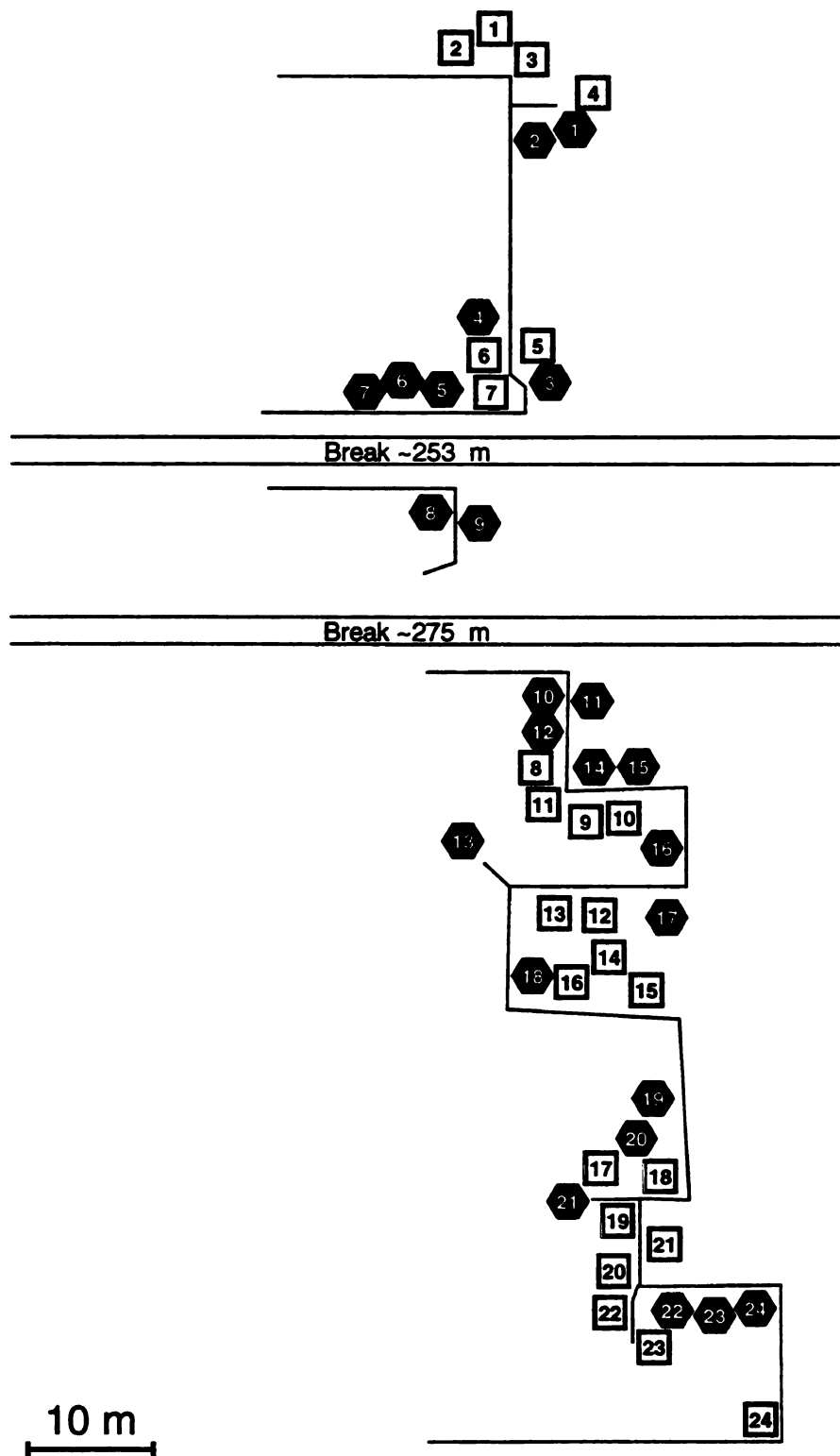
Figure A-3. Map of the plot locations within the Barrow Dry Heath (BD) site. The closed hexagon symbol represents an open-top chamber (OTC), the open square symbol represents a control plot, and the line represents the boardwalk.
