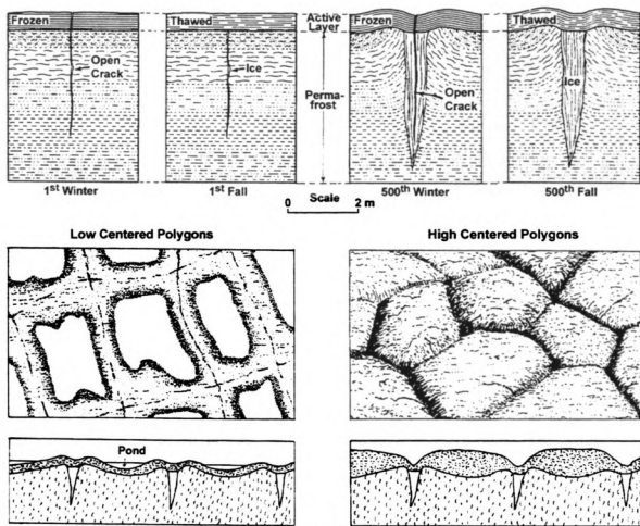
Figure I-12. Diagram of ice wedge formation ( top ) and polygons ( bottom ). The high and low centered polygons are not drawn to scale (redrawn from Tedrow 1977 and Pielou 1994).
