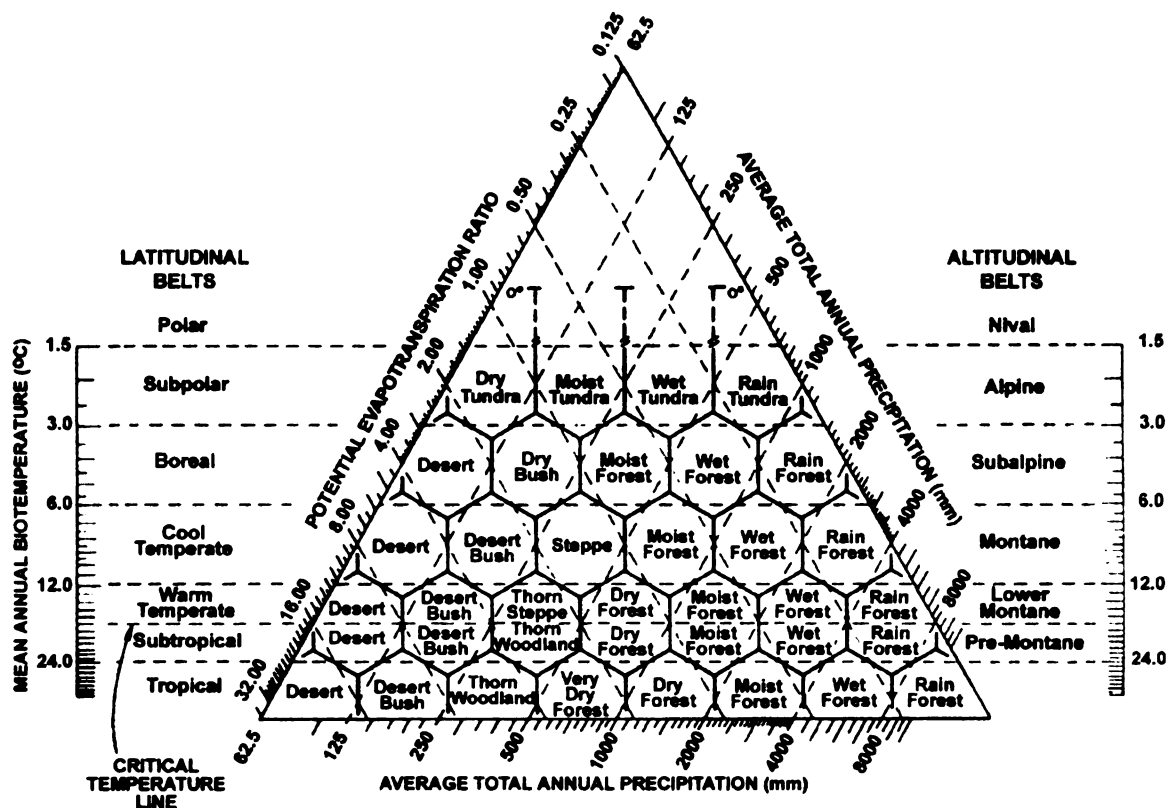
Figure I-10. The Holdridge scheme for the classification of the world's life zones (Holdridge 1947 as drawn in Shugart 1998).
