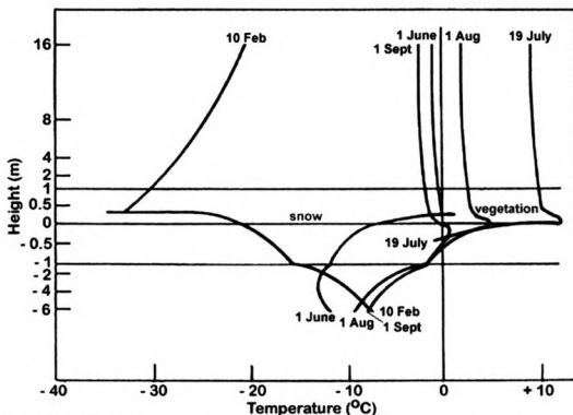
Figure I-3. Vertical temperature gradients in air, snow, vegetation, and soil on five typical days of the year over sedge-moss communities at Barrow, Alaska. Note the effects of snow (10 February and 1 June) and vegetation (1 August and 19 July) on the expanded \pm 1 m vertical profile (Weller and Holmgren 1974).
