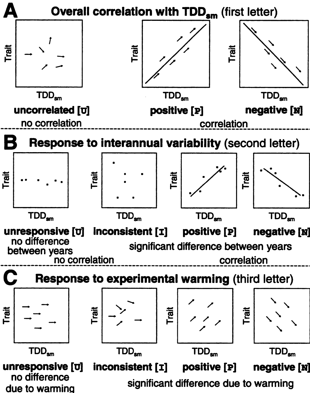
Figure IV-1. Conceptual response patterns of the trait of a species to thawing degree-day totals from snowmelt ( TDD_{sm} ). The relationship between the observed trait and TDD_{sm} is characterized by: A) the overall correlation with TDD_{sm} irrespective of year or treatment; B) the response to interannual variability; and C) the response to experimental warming. Lines represent significant correlations. Arrows represent the mean difference from the control to the warmed plots in a given year. Dots represent the mean value of the control plots in a given year. Each response was coded as unresponsive or uncorrelated [U], inconsistent [I], positive [P], or negative [N].
