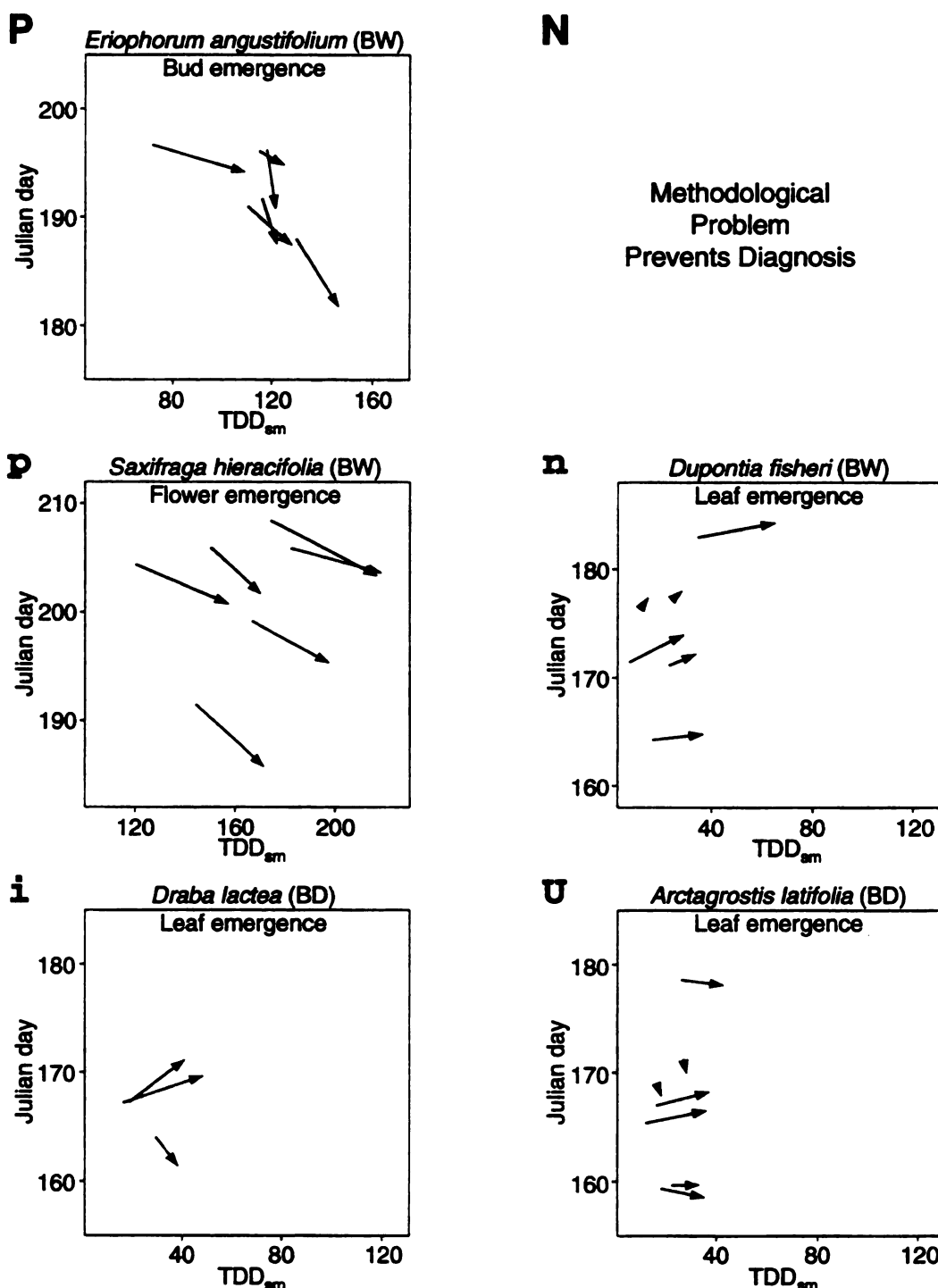
Figure IV-2. The Julian day that a phenological stage was reached versus the thawing degree-day totals from snowmelt (TDD sm ) of species representing the six temperature response types. Arrows represent the mean difference from the control to the warmed plots in a given year (arrow heads only represent small change). The site the species occurred in is presented in parentheses (AD - Atqasuk Dry Heath, BD - Barrow Dry Heath, BW - Barrow Wet Meadow). The temperature response types are: P - positive dominant response, p - positive subordinate response, N - negative dominant response, n - negative subordinate response, i - inconsistent response, and U - unresponsive.
