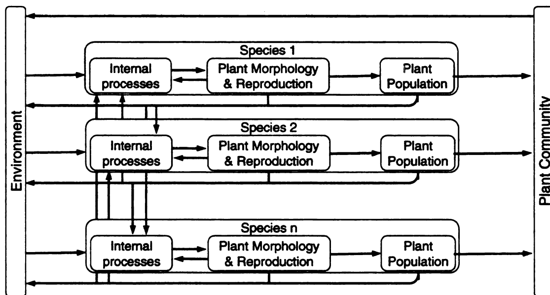
Figure VI-2. Conceptual model of the paths of influence of the environment on a plant community emphasizing the influence of species interactions. Arrows represent a pathway of influence. The long-term effects of a changing environment on the plant community may be difficult to predict due to the many interactions between species.
