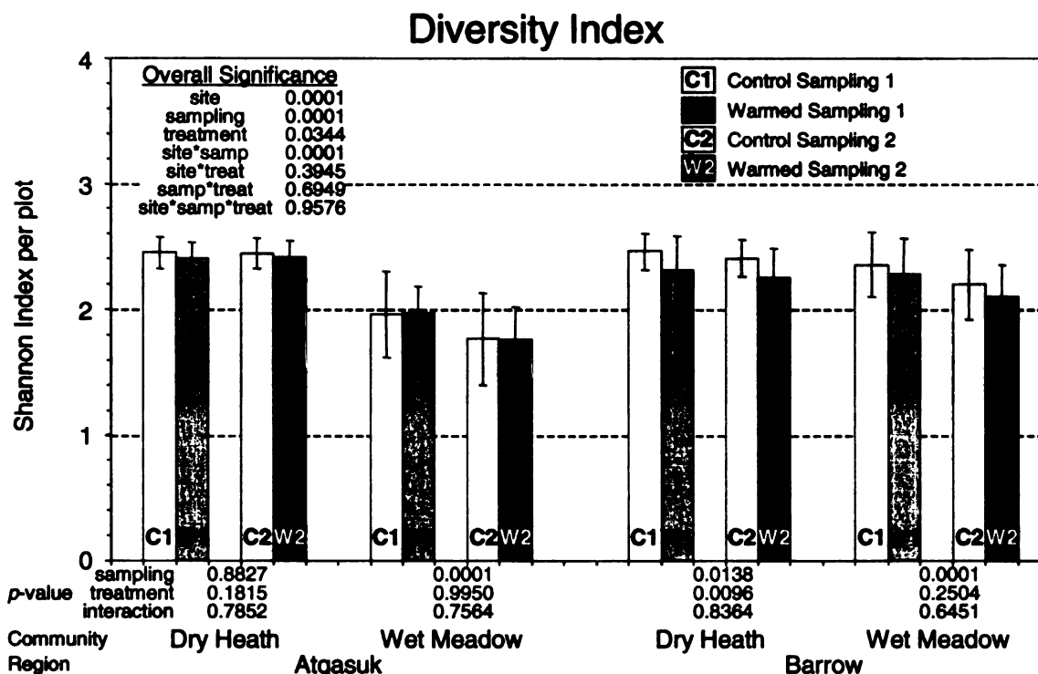
Figure V-5. Average Shannon index of diversity for each treatment at all sites (community and region) during both sampling times (error bars = \pm 1 SE, n = 24 ). Site and overall p -values were calculated from a two way and three way ANOVA respectively.
