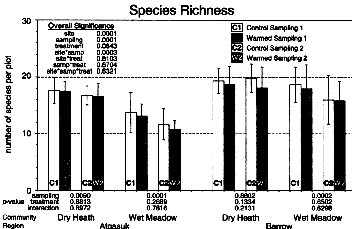
Figure V-4. Average species richness for each treatment at all sites (community and region) during both sampling times (error bars = \pm 1 SE, n = 24 ). Site and overall p -values were calculated from a two way and three way ANOVA respectively.
