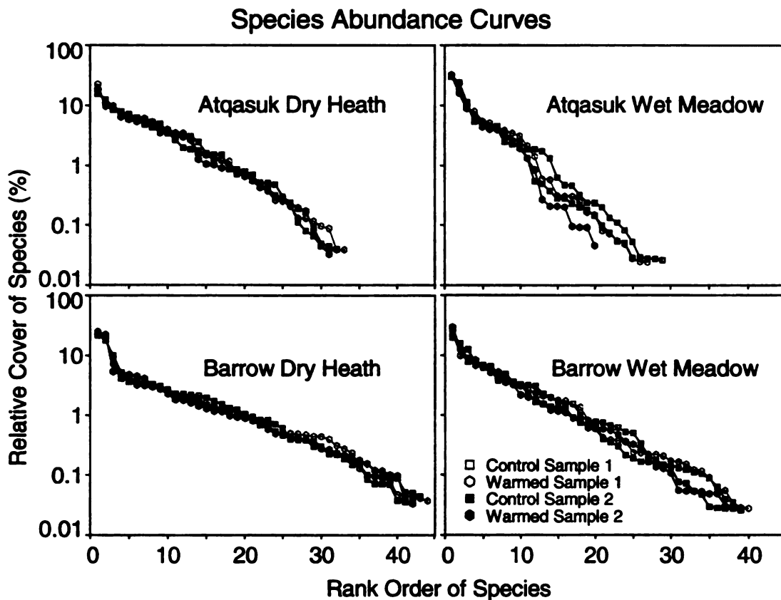
Figure V-6. Species abundance plots for each site. The relative cover of each species is graphed in sequence from highest cover to lowest cover for each treatment and sampling time.
