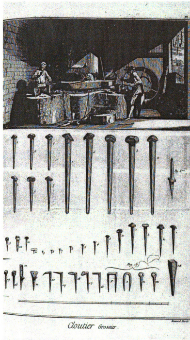
Figure A-51 - From Diderot's Encyclopédie, Recueil de Planches 1763 Part Two. Planche I, Nail Maker. Nail sizes are numbered 2, 4, 6, 10 and 14. Figure 10 (second row from bottom, fourth from left) is a shoe and Figure 12 nail (second row from the bottom, second from left) is a horse shoe nail. Diderot did not use the same terminology as the French Canadian military or the Montreal merchants.
