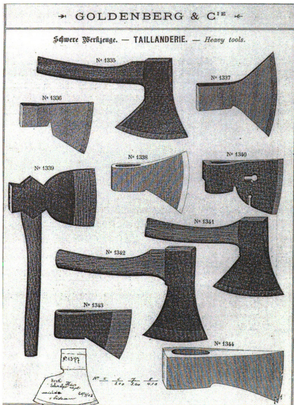
Figure A-55: Goldenberg tool catalogue 1895-1896. No. 1338 and 1343 both are Biscaye fashion axes.
