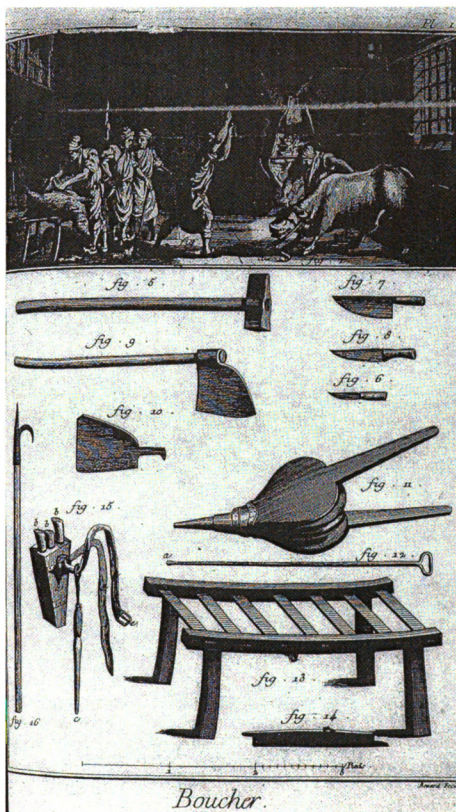
Figure A-47 – From Diderot's Encyclopédie, Recueil de Planches 1763 Part One. Planch 1 Butcher. Figures 6, 7, and 8 show three sizes of butcher knives.
