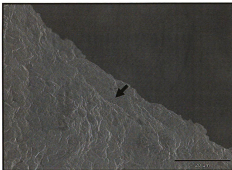
Figure 16: SEM Picture of Characteristic Traces from 15 minutes of Dry Hide Work (1500 X)
