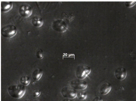
Figure 42.2: Elongate and Spherical Starches from Lablab purpureus (under polarize light)
