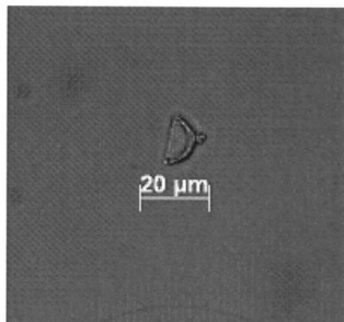
Figure 71.9: Damaged Starch from Pericarp of cf. Solanum
