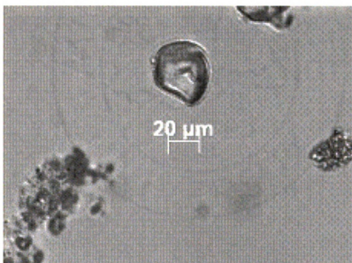
Figure 87.16: Starch from Seed of cf. Solanum
