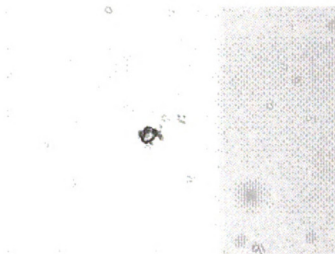
Figure 66.1: Compound Starch 1 (measurement)
