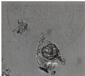
Figure 87.2: Unknown Damaged Starch 2
