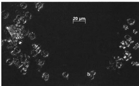
Figure 36.2: Starches from Sesame indicus (under polarize light)
