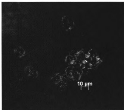
Figure 47.2: Starches from Pennisetum glaucum (under polarize light)
