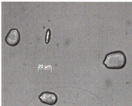
Figure 51.1: Starches from Zingiber officinale Rosc
