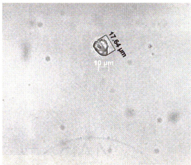
Figure 63.2: Unknown Damaged Starch 1 (measurements)
