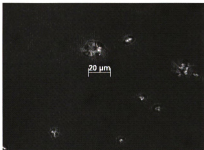
Figure 48.2: Compound Starches from Eleusine coracana L. (under polarize light)
