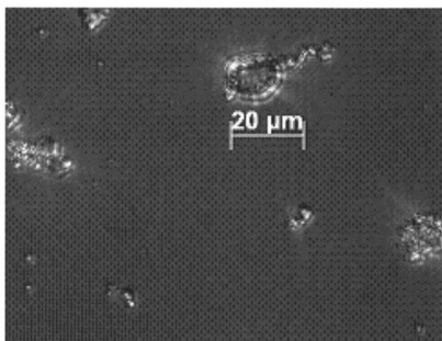
Figure 85.2: Damaged Seed Starch (under polarize light)
