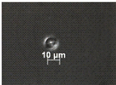
Figure 77.6: Starch from cf. Vigna sp. (measurement)
