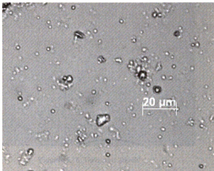
Figure 86.14: Starches from cf. Sesamum
