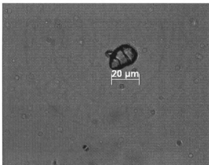
Figure 83.9: Starch from cf. Eleusine (under polarize light)
