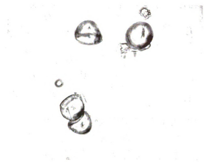
Figure 50.1: Bell Shaped Starch Grains from Ipomoea batatas
