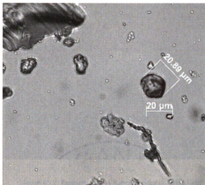
Figure 84.5: Starch from cf. Sorghum
