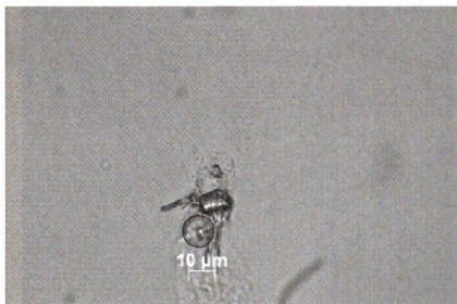
Figure 35.3: Spherical Starches from Phoenix dactylifera
