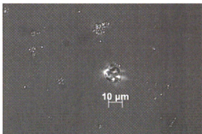
Figure 66.5: Unknown Starch (under polarize light)
