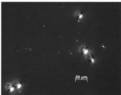
Figure 37.3: Characteristics of Vigna mungo (under polarize light)
