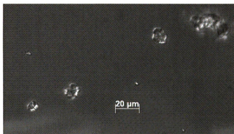
Figure 78.2: Starch Granules (measurement)
