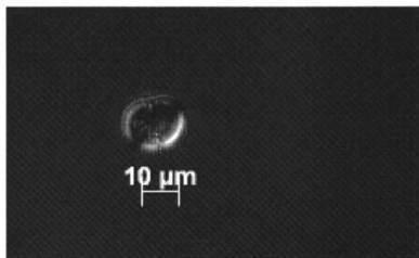
Figure 78.6: Unknown Bean Starch (under polarize light)
