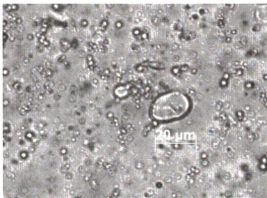
Figure 58.1: Elongate Starch from Pericarp of Solanum
