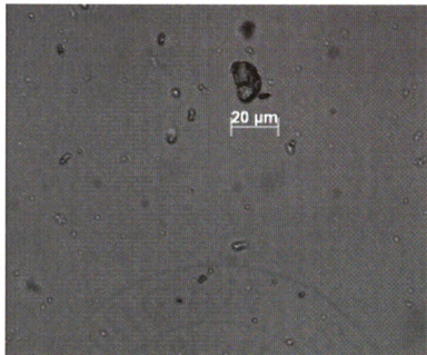
Figure 84.4: Damaged Unknown Bean Starch
