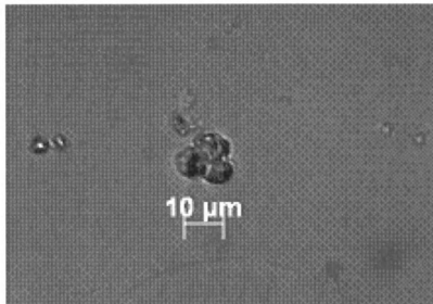
Figure 69.20: Starch Grains from cf. Sesamum
