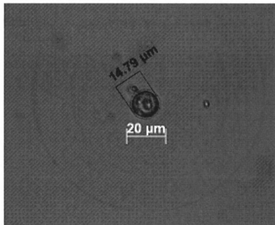
Figure 79.5: Starch from cf. Mangifera (measurement)
