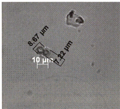
Figure 69.28: Starch Grain from cf. Sesamum (measurement)
