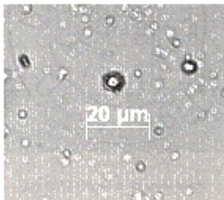
Figure 86.14: Starches from cf. Sesamum
