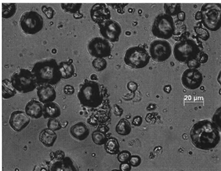
Figure 46.1: Starches from Sorghum bicolor
