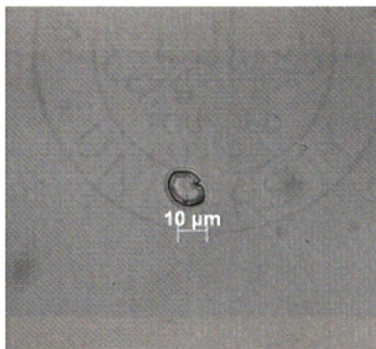
Figure 69.14: Starch Grain Consistent with cf. Mangifera (measurement)
