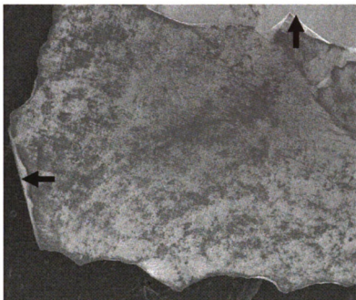
Figure 25: SEM picture of evidence of Fracture on a Point from being used as a Projectile (artifact no. 130)
