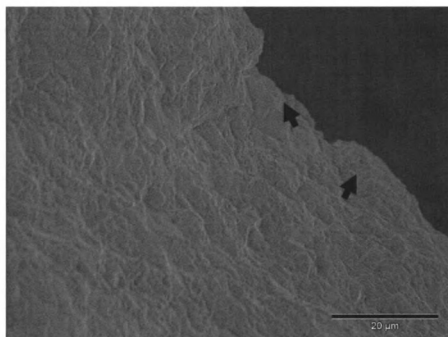
Figure 27: SEM picture of characteristic features from Scraping Dry Hide (artifact no. 150, 1500X)
