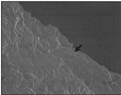
Figure 17: SEM Picture of Progression of Characteristic Traces from 1 hour of Dry Hide Work (1500 X)
