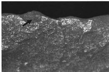
Figure 14 Characteristic Features from Wood Working or Soft Wood (300 X)
