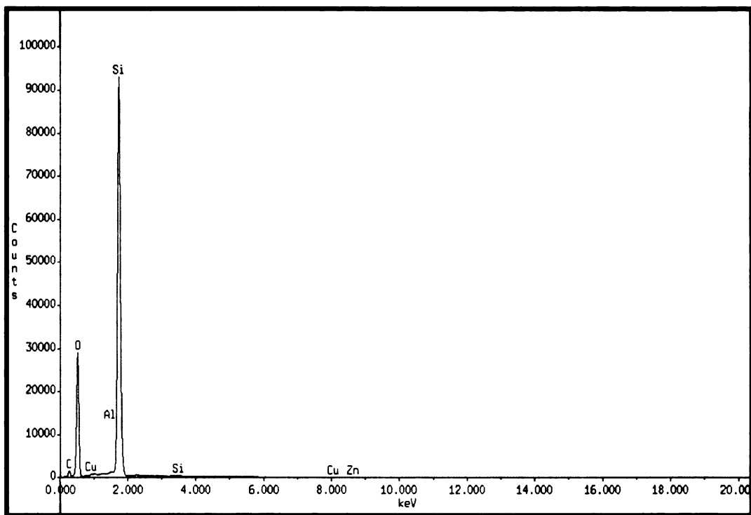
Figure 3.14: EDS Spectrum of Blade III
