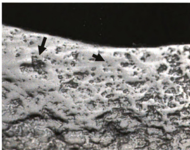
Figure 12: Polish from Cutting Reed (400 X)
