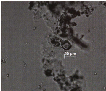
Figure 87.33: Starch from Seed of cf. Solanum
