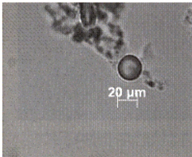
Figure 87.27: Unknown Starch 1 (on rotation)
