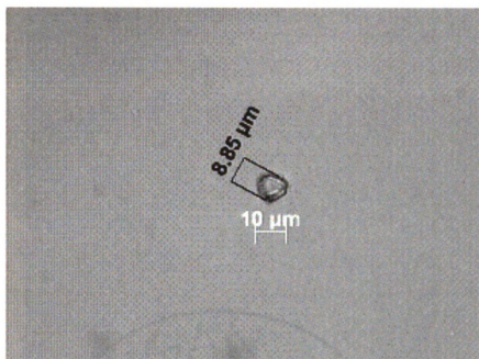
Figure 63.12: Compound Starch 2 (measurements)
