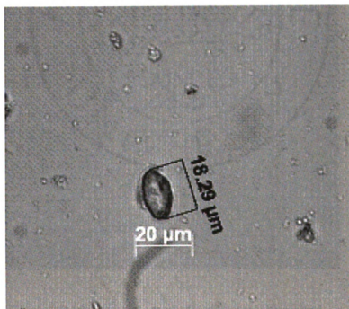
Figure 70.12: Elongate Starch from cf. Phoenix
