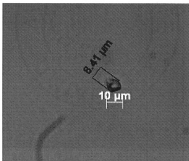
Figure 71.8: Compound Starch (measurement)
