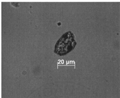
Figure 67.3: Damaged Bean Starch
