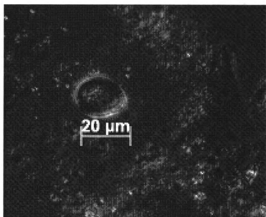
Figure 57.1: Spherical Starches from Mangifera
