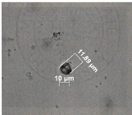
Figure 66.6: Unknown Starch (measurement)
