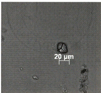
Figure 87.4: Starch from cf. Eleusine
