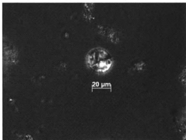
Figure 87.36: Starch from Seed of cf. Solanum (under polarize light)
