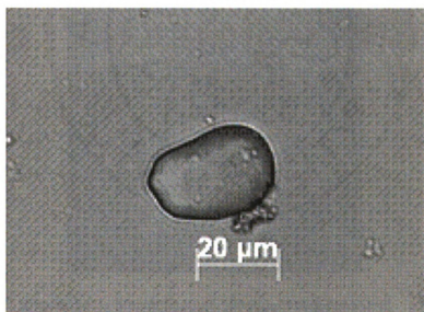
Figure 76.1: Starch from cf. Zingiber
