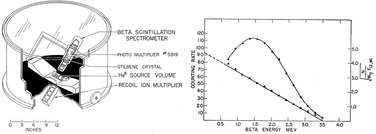
Figure 1-8: Left panel: a schematic sketch of the apparatus used to determine the electron-recoil ion correlation in the decay of ^6\text{He} . The beta-active source volume and the scintillation spectrometer are located in the common vacuum of the “bell-jar”. Right panel: the ^6\text{He} \beta -energy spectrum measured with the stilbene scintillation spectrometer. Figures taken from Ref. [10].
