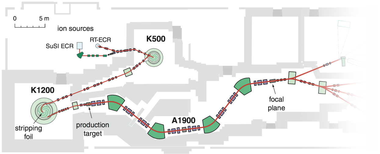
Figure 3-1: A schematic layout of the beam facility at National Superconducting Cyclotron Laboratory.
