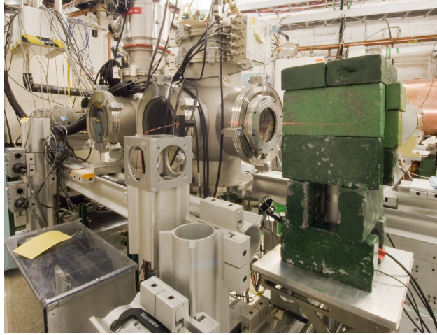
Figure 3-9: The setup of the CsI(Na) detector on the beamline. The {}^6\text{He} ions exiting from the beam pipe through the 75\text{ }\mu\text{m} thick Zr vacuum window (left) were implanted into the CsI(Na) detector (right) aligned perpendicular to the beamline. The CsI(Na) detector is surrounded by lead bricks (green).
