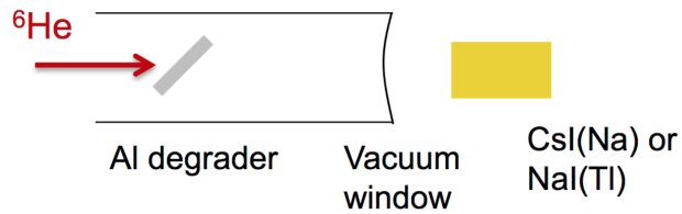
Figure 3-2: A cartoon of the top view of the setup. The secondary ^6\text{He} beam (red) of 76 MeV per nucleon passes through a degrader (gray). The beam was decelerated by the degrader down to 46 MeV per nucleon and was implanted into a CsI(Na) or NaI(Tl) detector (yellow).
