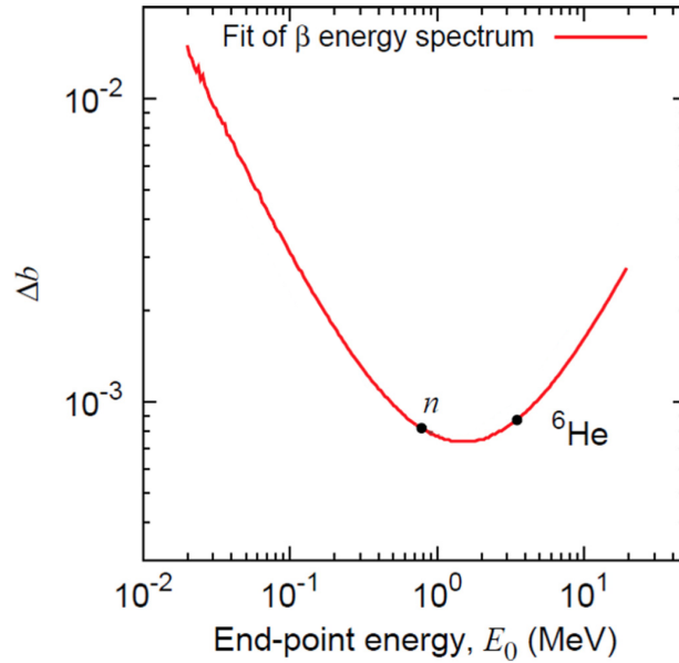
Figure 1-4: The 1\sigma statistical uncertainties of the Fierz interference term obtained by fitting the simulated \beta -energy spectra with different values of the endpoint energy. Figure taken from Ref. [6].
