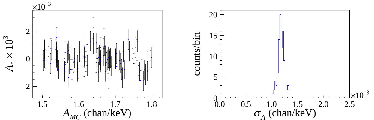
Figure 8-9: Left panel: values of A_r extracted from SM fits using Tspline3. Right panel: distribution of the statistical errors of A from the same fits.
