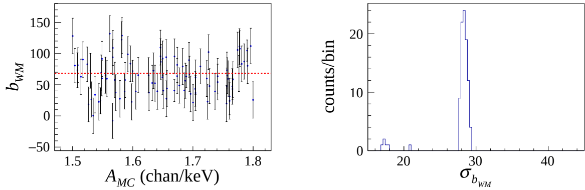
Figure 8-4: Left panel: values of b_{WM} extracted from SM fits using Interpolate . The dotted line indicates the input value used in the Monte Carlo. Right panel: distribution of the statistical errors of b_{WM} from the same fits.
