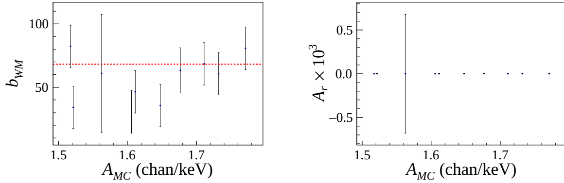
Figure 8-1: Left panel: values of b_{WM} extracted from SM fits using GetBinContent . The dotted line indicates the input value used in the Monte Carlo. Right panel: values of A_r calculated with A extracted from the same fits.
