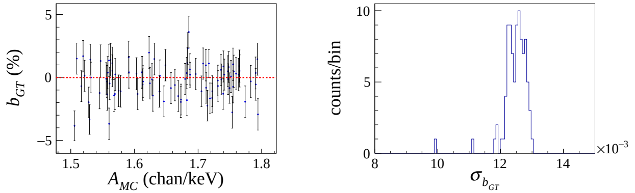
Figure 8-6: Left panel: values of b_{GT} extracted from BSM fits using Interpolate . The dotted line indicates the input value used in the Monte Carlo. Right panel: distribution of the statistical errors of b_{GT} from the same fits.
