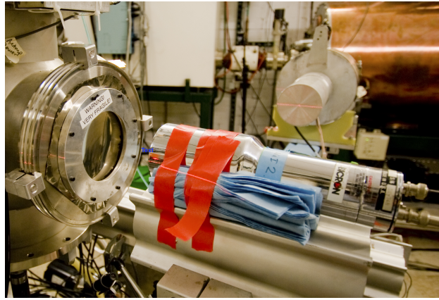
Figure 3-8: The setup of the NaI(Tl) detector on the beamline. The ^6\text{He} ions exiting from a beam pipe through the 75 \mu\text{m} thick Zr vacuum window (left) were implanted into the NaI(Tl) detector (right) aligned along the beamline.
