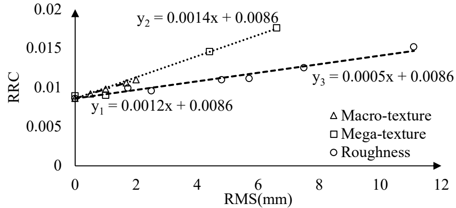
Figure 5-11. Comparison of the effect of macro-texture, mega-texture, and roughness on rolling resistance coefficient of the tire
