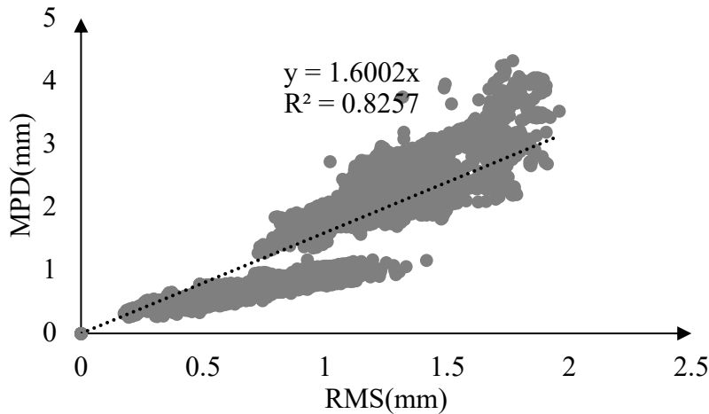
Figure 3-10. Relationship between RMS and MPD values for all databases
