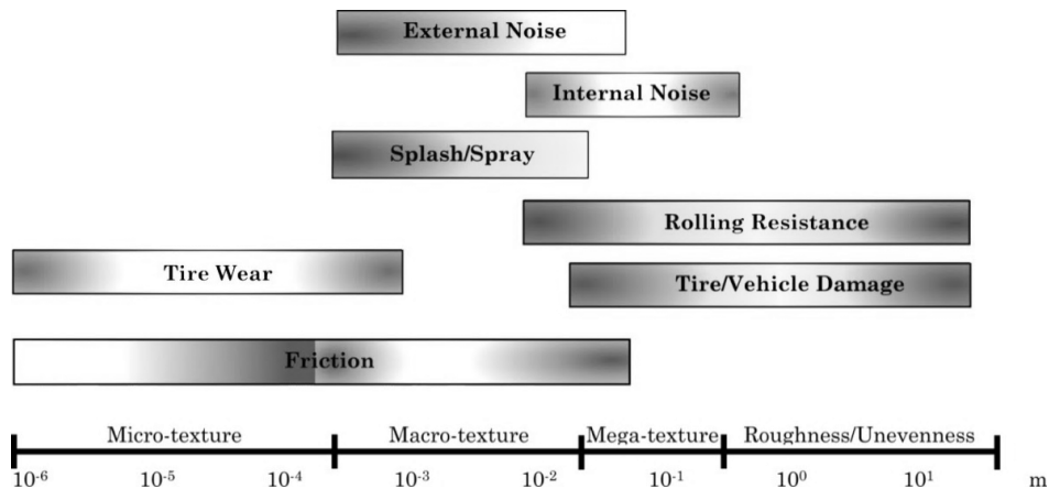
Figure 2-1. Influence of texture and roughness wavelength on vehicle/tire-pavement interactions (after Henry, 2000 and Sandburg and Ejmont, 2000)
