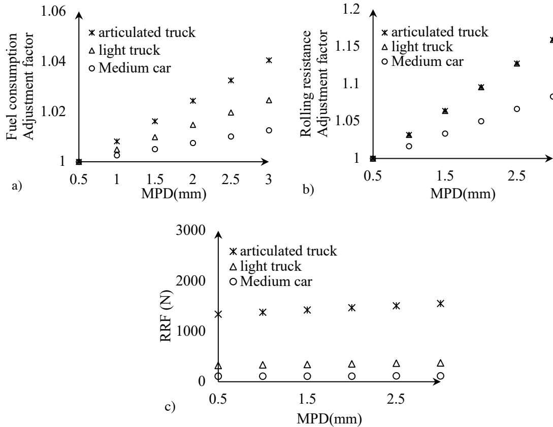
Figure 2-23. NCHRP 720 model- Relationships between pavement surface MPD and a) Adjustment factor for fuel consumption, b) Adjustment factor for rolling resistance, and c) Rolling resistance force at v=80\text{km/h} (Chatti and Zaabar, 2012)
