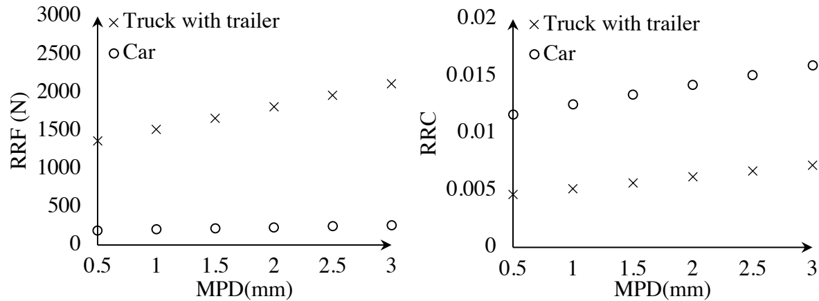
Figure 5-20. Rolling resistance force and coefficient for a full car, and equivalent articulated truck, from MIRIAM project
