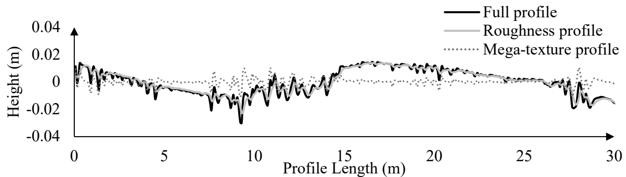
Figure 5-15. Profile 1, IRI= 5m/km
