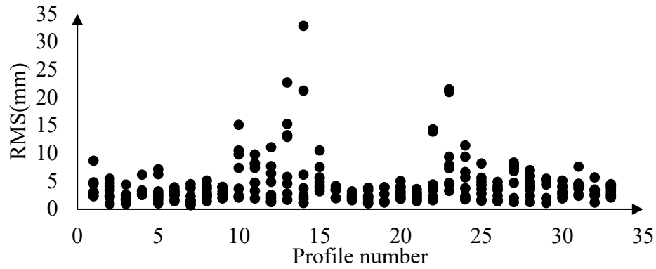
Figure 3-14. RMS variation for roughness profiles of 30 meters long
