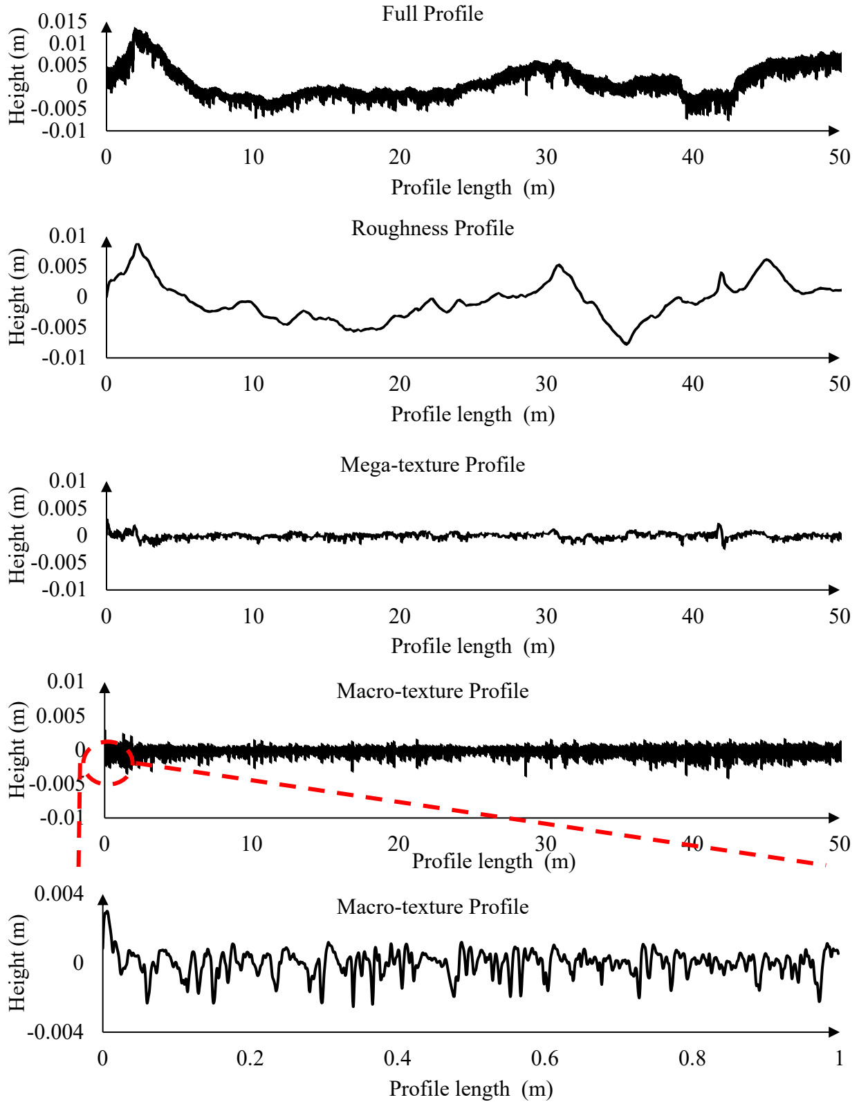
Figure 3-4. Division of the surface into different scales (Data from Danish road institute)
