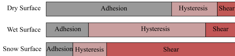
Figure A1-2. Compositions of Major influences on braking slip conditions (Hall, 2009)
