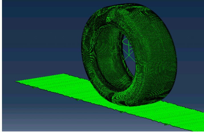
Figure 4-22. Tire model rolling on a textured surface
