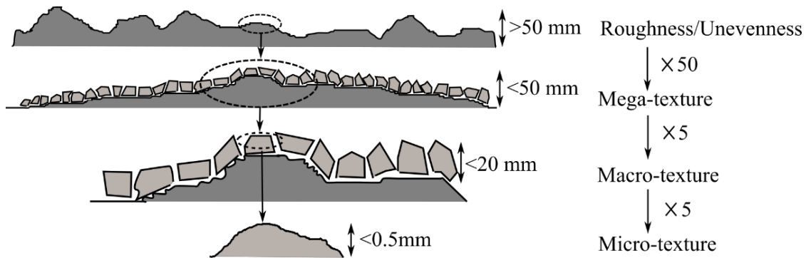
Figure 3-1. Simplified illustration of various pavement surface profile ranges (after Sandburg, 1990)
