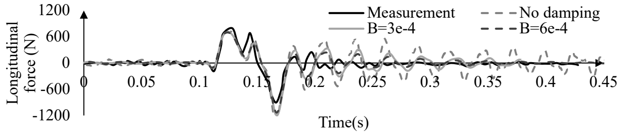
Figure 4-28. Variation of tire longitudinal force rolling over a 10mm *25mm step with 10km/h speed for different Rayleigh damping coefficients
