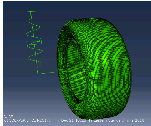
Figure 4-21. Schematic view of FE Quarter-car model
