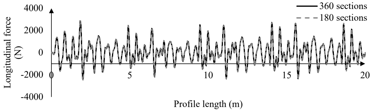
Figure 4-36. Variation of tire rolling resistance force rolling over a textured surface with mega-texture with RMS of 4 mm and speed of 80km/h for different numbers of radial sections
