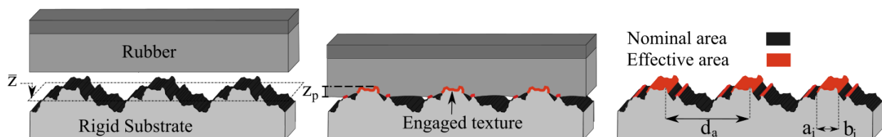
Figure 2-22. Contact of rubber with a rigid substrate as pavement
