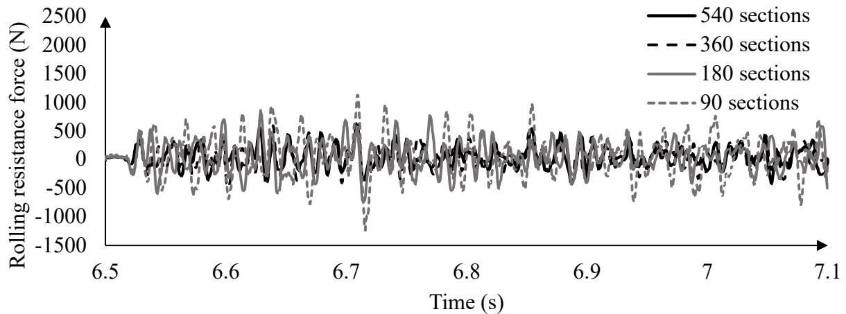
Figure 4-33. Variation of tire rolling resistance force rolling over a textured surface with macro-texture with RMS of 1.68 mm and speed of 80km/h for different numbers of radial sections
