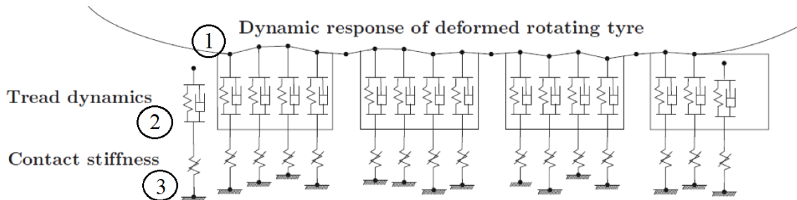
Figure 2-19. Schematic overview of the mechanistic tire-surface interaction model (Boere, 2009)
