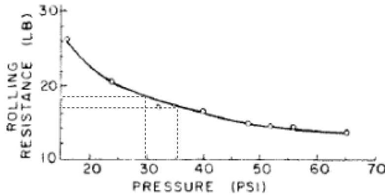
Figure 5-36. Relationship between tire inflation pressure and rolling resistance (Schuring, 1985)
