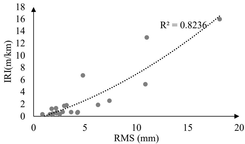
Figure 3-11. Relationship between RMS and IRI values
