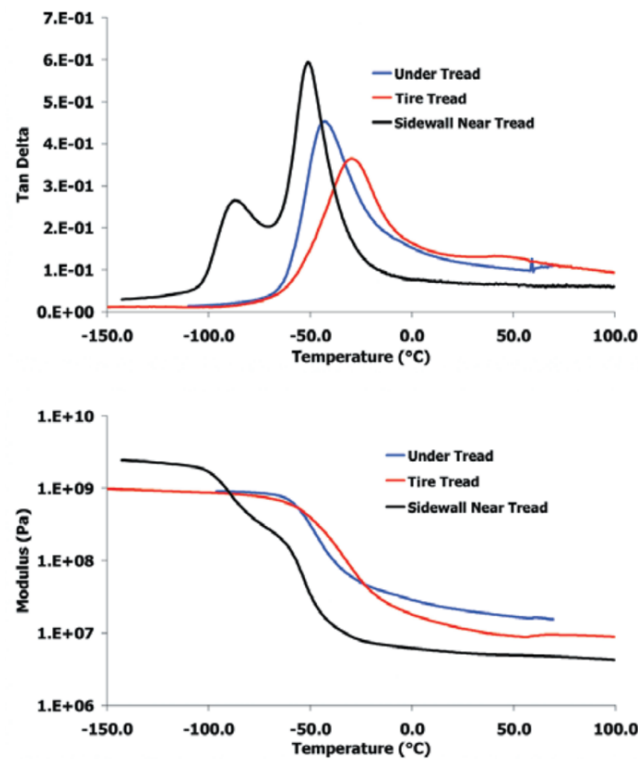
Figure 4-8. Glass transition of tire (by PerkinElmer, Inc)
