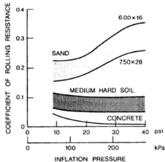
Figure 4-14. Effect of tire inflation pressure on rolling resistance on different surfaces (Wong, 2008)
