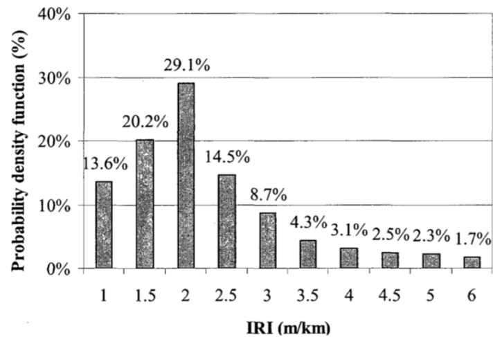
Figure 5-25. Histogram of the distribution of IRI in United states (Zaabar, 2010)
