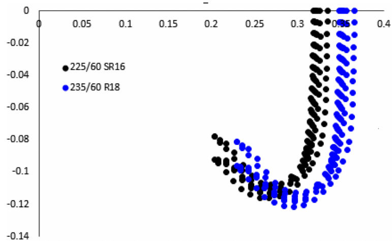
Figure 4-4. Conversion of the geometry of a 235/60 R18 tire to a 225/60 SR16 tire
