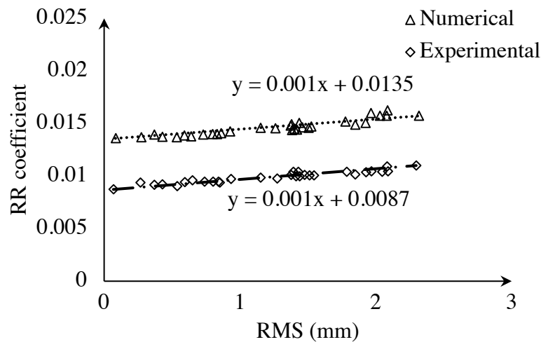
Figure 2-24. Boere model- Experimental and numerical relationships between rolling resistance and texture RMS at v=80\text{km/h} on 30 test tracks (Boere, 2009)
