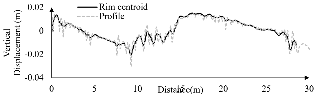
Figure 5-27. The vertical displacement of the rim centroid and the profile for IRI=5 m/km
