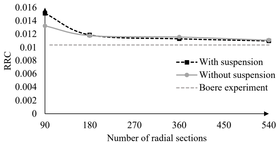
Figure 4-39. Mesh sensitivity analysis for the Quarter-car model on textured surface with RMS=1.68mm
