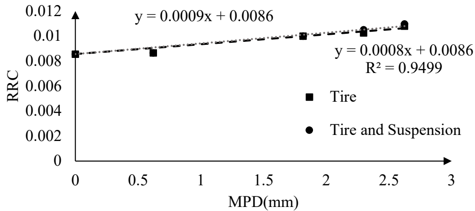
Figure 5-4. Effect of macro-texture profile's MPD on RRC of the tire and the quarter car model
