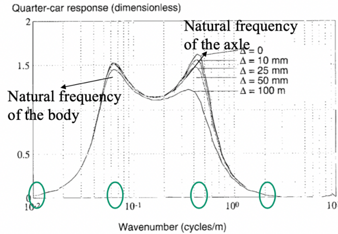
Figure 3-13. Effect of frequency on vehicle response (Mann et al. 1997)
