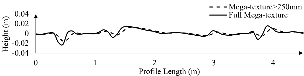
Figure 5-7. Filtered mega-texture profile (RMS=6.6mm)
