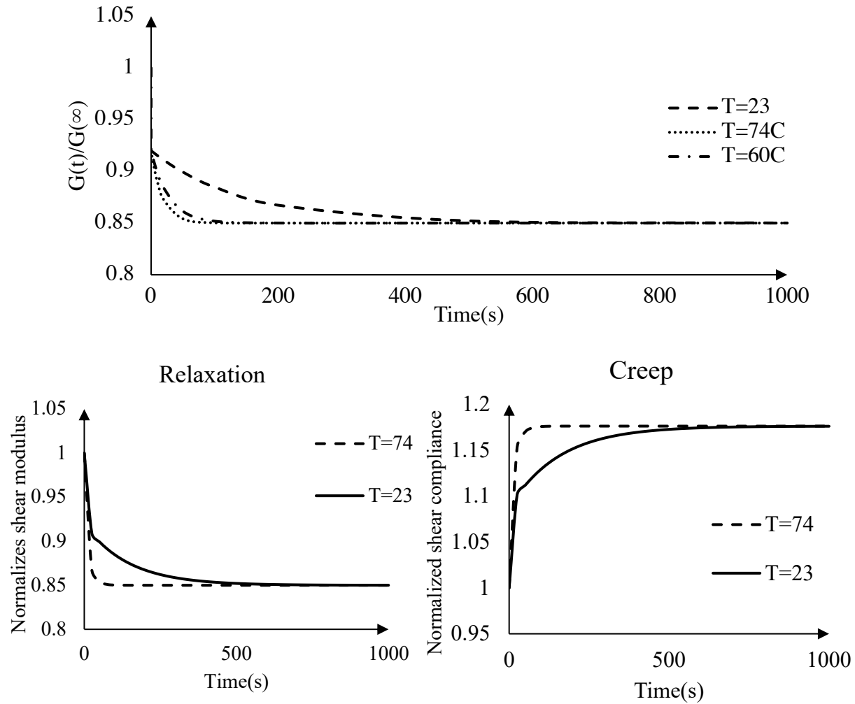
Figure 4-10. Effect of temperature on tire tread rubber material properties
