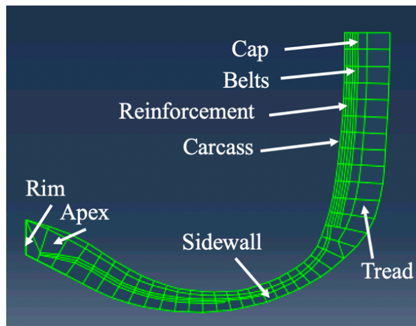
Figure 4-2. Tire cross section
