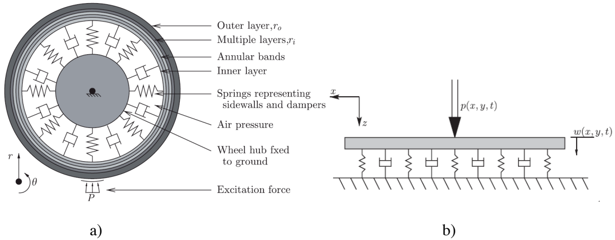
Figure 2-18. a) viscoelastic cylindrical model of the tire belt b) simple bending plate (O'boy and Dowling, 2009)
