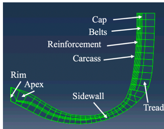
Figure 4-18. Generated 2D tire model
