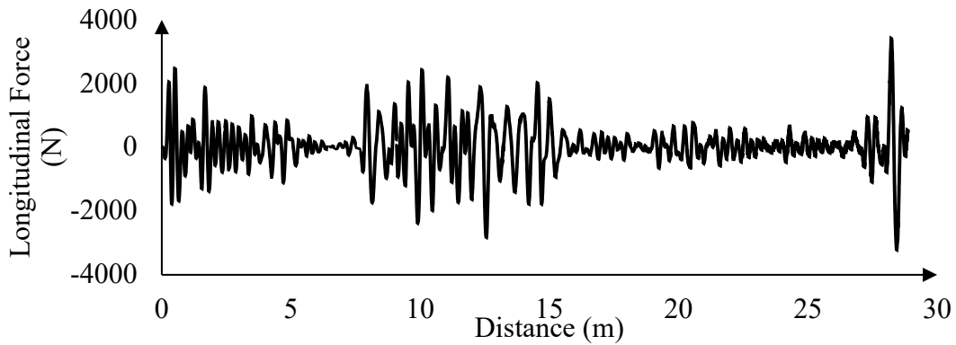
Figure 5-29. Longitudinal forces for IRI=5 m/km
