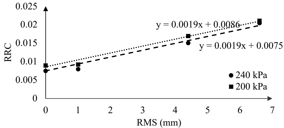
Figure 5-38. Effect of inflation pressure on variation of rolling resistance by surface mega-texture at 80km/h
