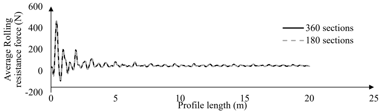
Figure 4-37. Variation of average rolling resistance force of the tire rolling over a textured surface with mega-texture with RMS of 4 mm and speed of 80km/h for different numbers of radial sections
