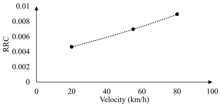
Figure 5-32. Variation of rolling resistance coefficient by velocity on a smooth surface
