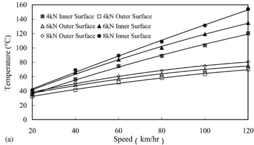
Figure 4-9. Variation of tire temperature with tire speed (Lin and Hwang, 2004)
