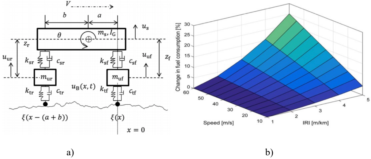
Figure 2-12. a) Half-car model, b) Relationship between energy dissipation, roughness, and speed (Kim et al. 2017)
