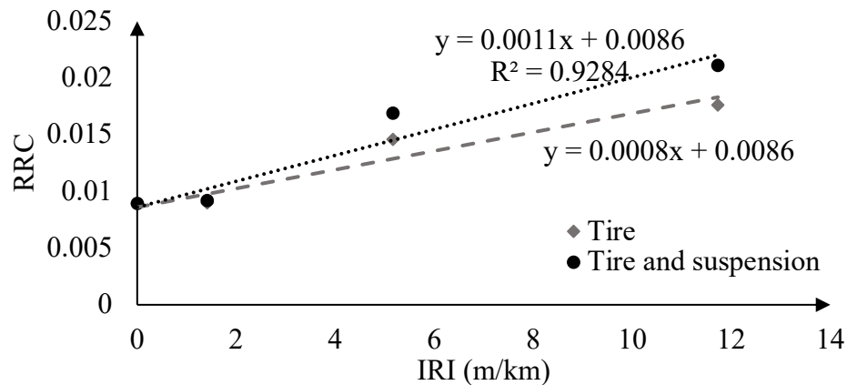
Figure 5-6. Effect of mega-texture profile's IRI on RRC of the tire and the quarter car models
