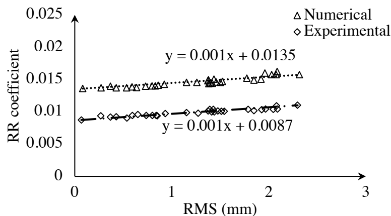
Figure 2-20. The effect of surface texture on rolling resistance of the tire (Boere, 2009)
