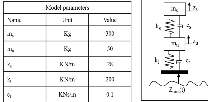
Figure 2-13. Schematic view of the Quarter-Car Vehicle Model (Zaabar et al. 2018)
