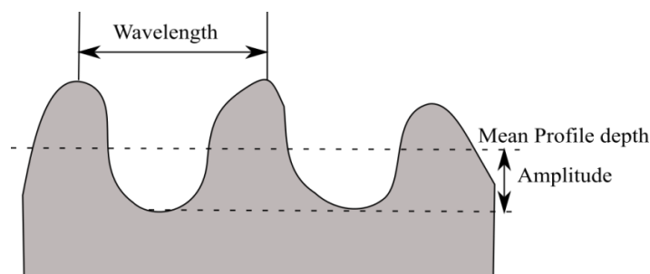
Figure 2-2. Simplified illustration of various pavement surface profile ranges (after Sandburg, 1990)
