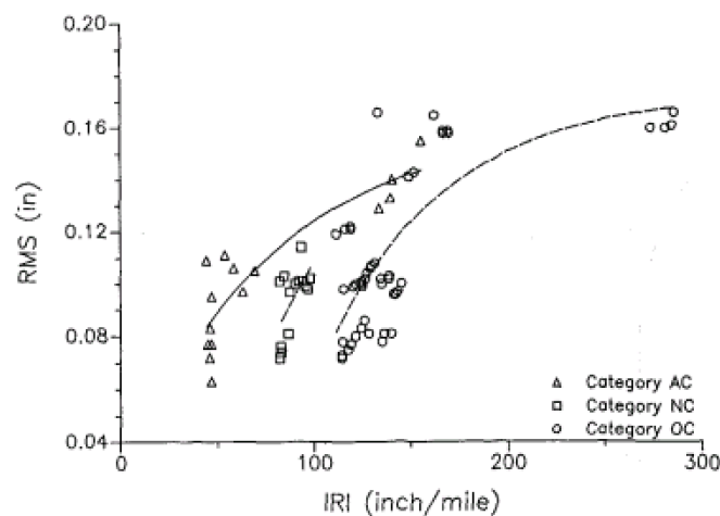
Figure 3-12. Relationship between RMS and IRI values for asphalt and new and old concrete surfaces (Marcondes et al, 1991)
