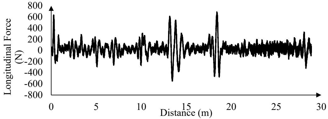
Figure 5-28. Longitudinal forces for IRI=3.3 m/km
