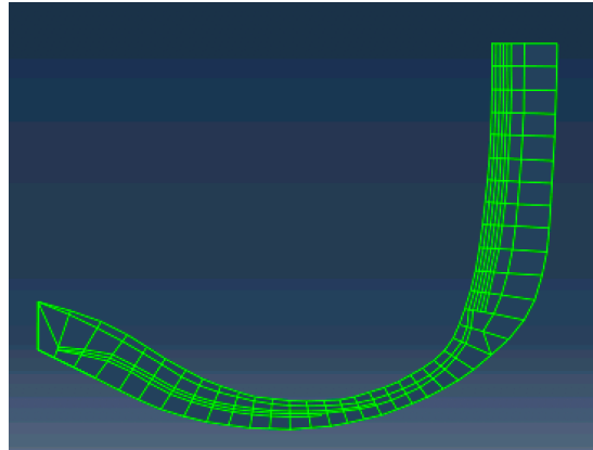
Figure 4-11. Final tire mesh
