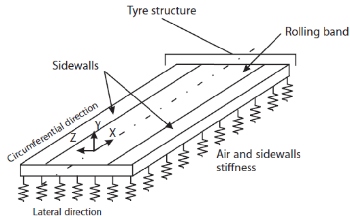
Figure 2-17. Pretensioned Kirchhoffs plate on a stiffness bedding (Wullens and Kropp, 2004)
