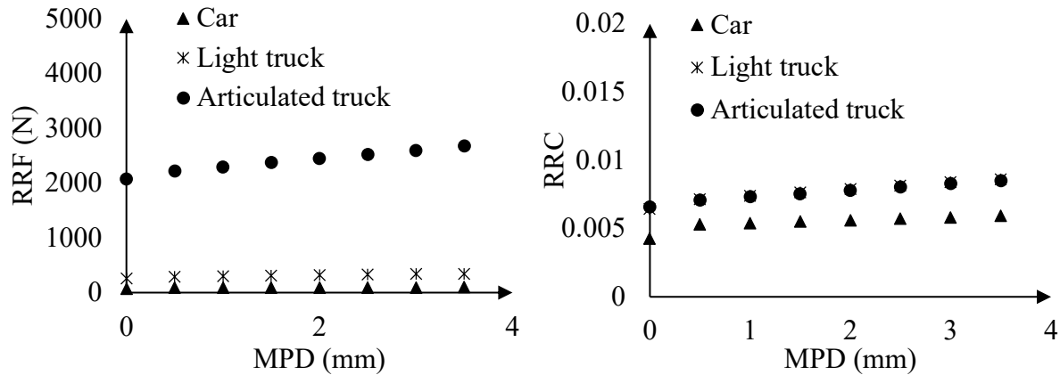
Figure 5-19. Rolling resistance force and coefficient for full car, light truck, articulated truck, from NCHRP 720 report
