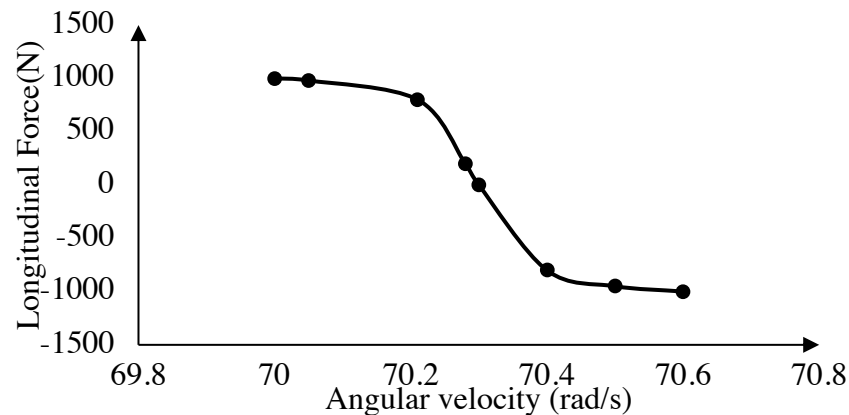
Figure 4-17. Variation of longitudinal force by angular velocity in steady state analysis
