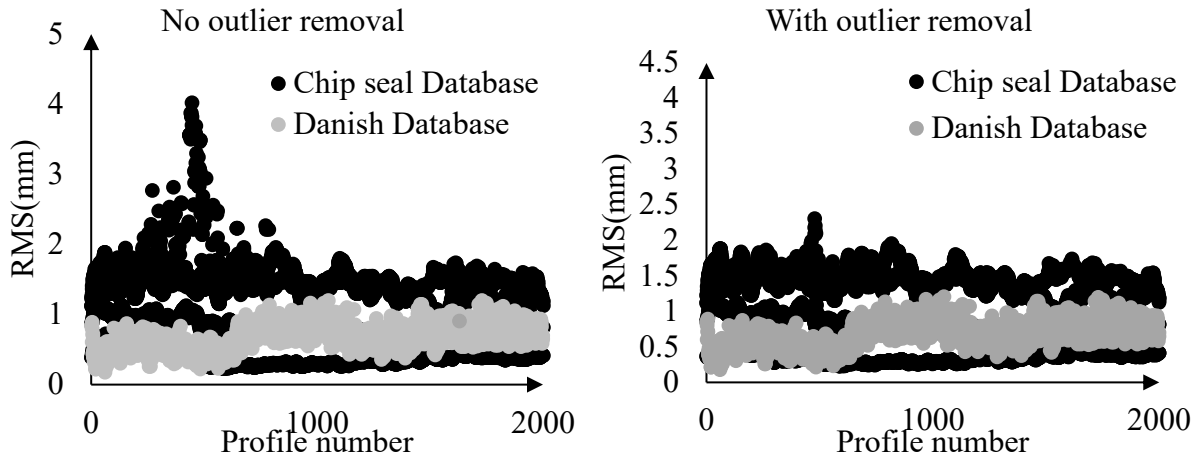
Figure 3-16. RMS variation for macro-texture profile of 0.45m long (data base maximum length)
