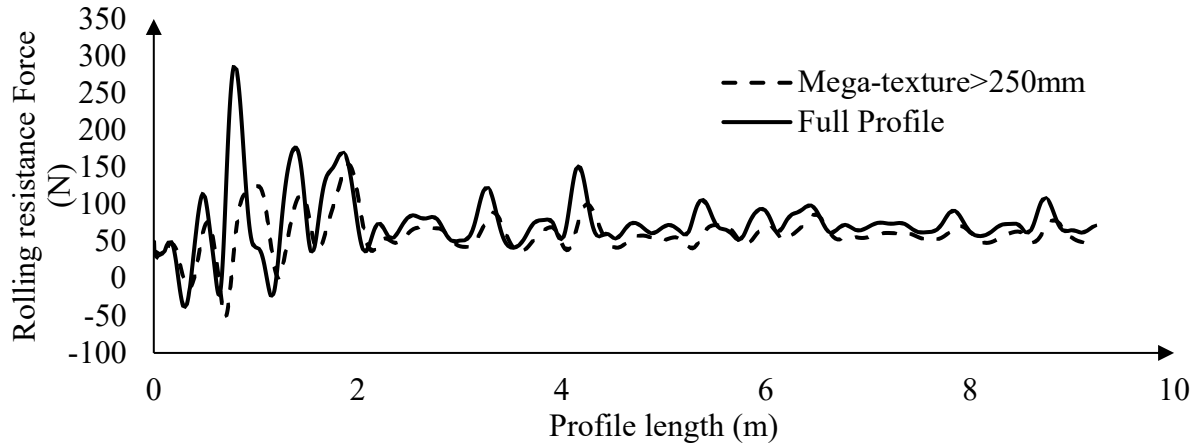
Figure 5-8. Effect of 250mm filtering of mega-texture on the rolling resistance force of the quarter-car FE model
