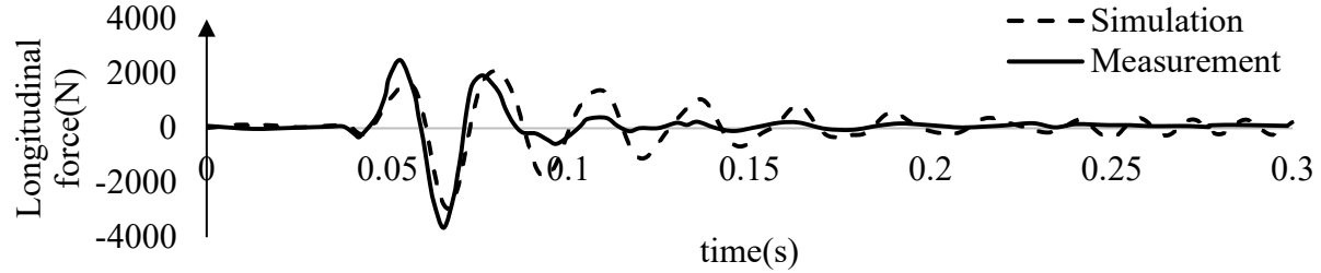
Figure 4-27. Comparison of the FE model with experimental measurements of Wei and Olatunbosun (2016), at velocity of 30km/h
