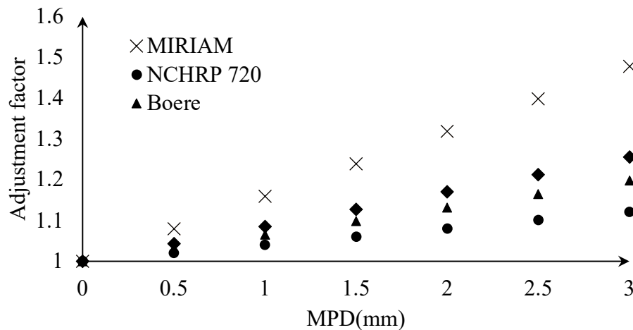
Figure 5-22. Comparison of rolling resistance adjustment factor of MIRIAM, NCHRP 720, Boere study and quarter-car FE model for a car at v=80 km/h
