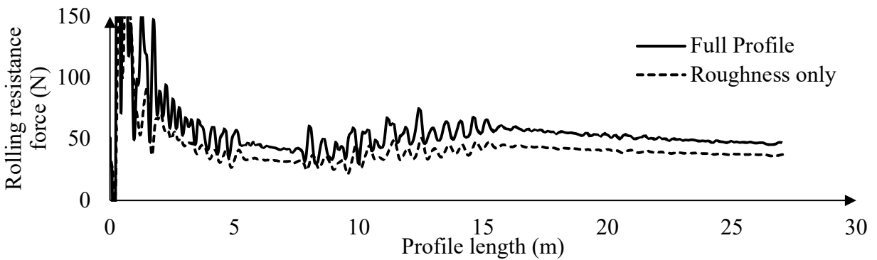
Figure 5-17. Rolling resistance forces for full profile and filtered roughness profile of profile 1 with IRI=5m/km
