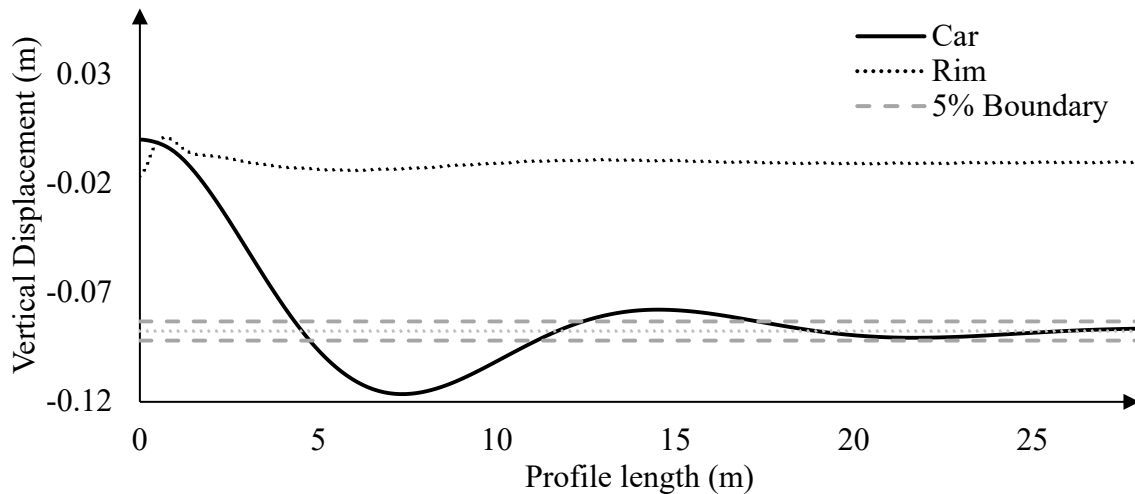
Figure 4-38. Vertical displacement of the spring mass under the vehicle load
