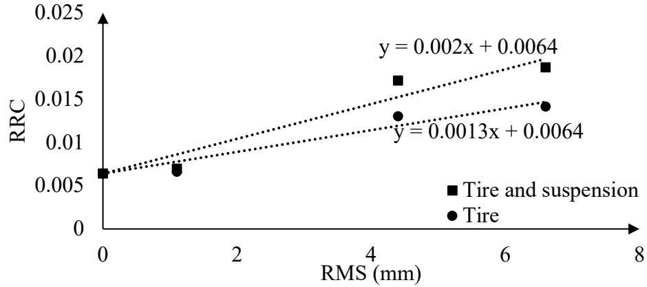
Figure 5-33. Effect of mega-texture on rolling resistance coefficient at V=55km/h
