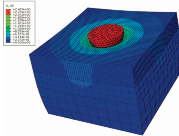
Figure 2-21. Finite element modeling of a single asperity contact
