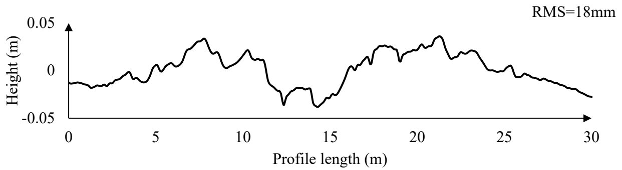
Figure 3-23. Selected profiles for roughness scale, with different RMS values
