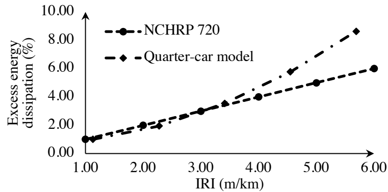
Figure 2-14. Effect of roughness on energy dissipation as a function of IRI at v=80 km/h (Zaabar et al., 2018)
