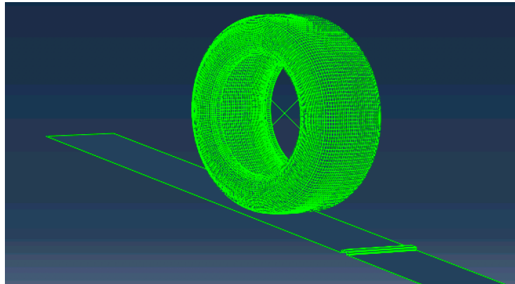
Figure 4-24. FE tire model rolling over a step
