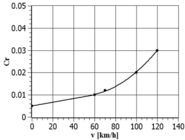
Figure 5-31. Effect of speed on rolling resistance coefficient (Mozharovskii et al. 2007)
