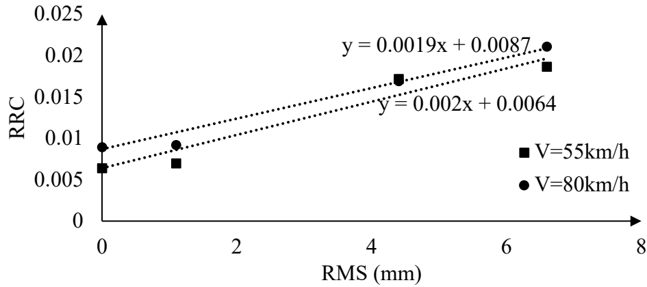
Figure 5-34. Effect of vehicle velocity on variation of rolling resistance with RMS of surface mega-texture
