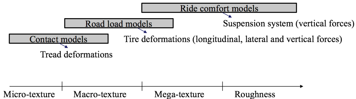
Figure 2-9. Influence of pavement profile on vehicle rolling resistance
