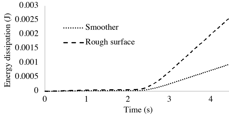
Figure A2-13. Energy dissipation in a rubber block with 4mm width for a rough and smooth surface
