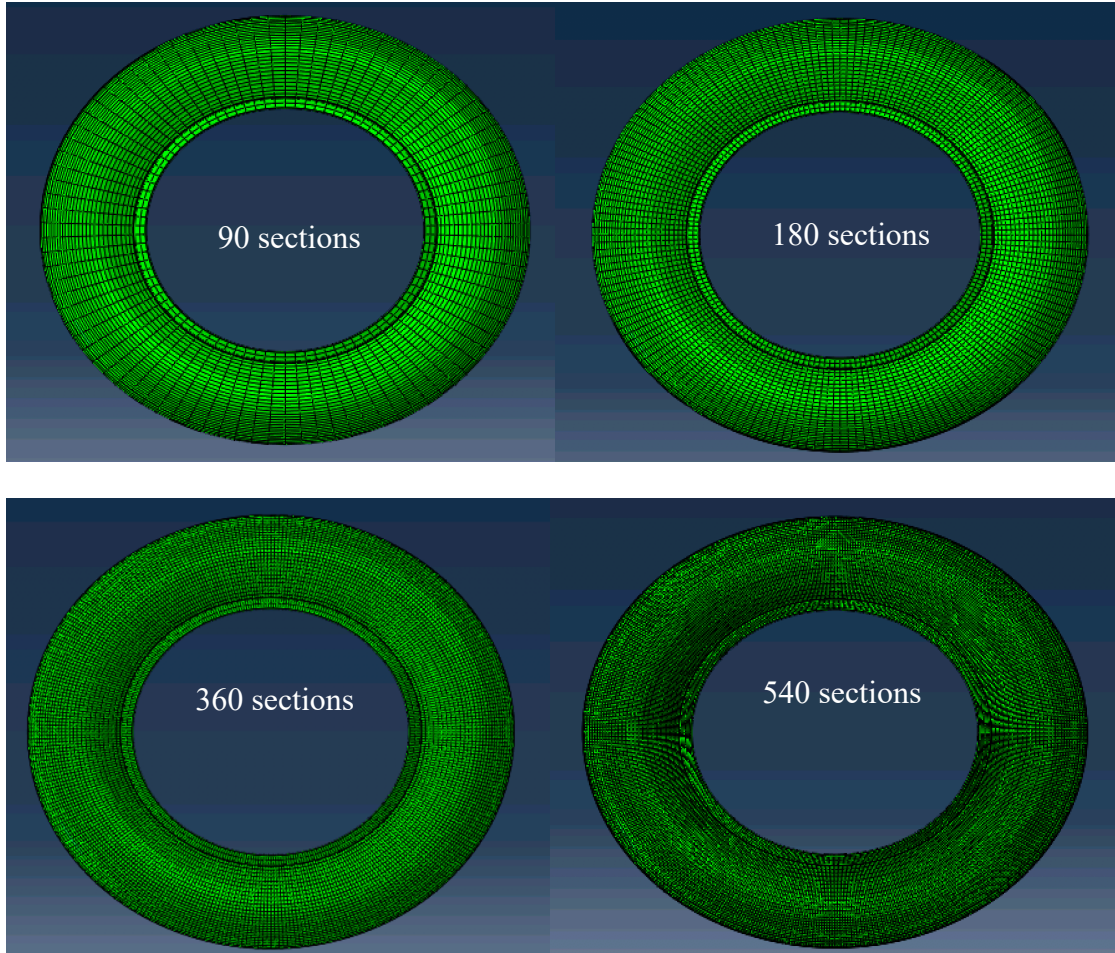
Figure 4-31. Different number of radial sections used in the mesh sensitivity analysis
