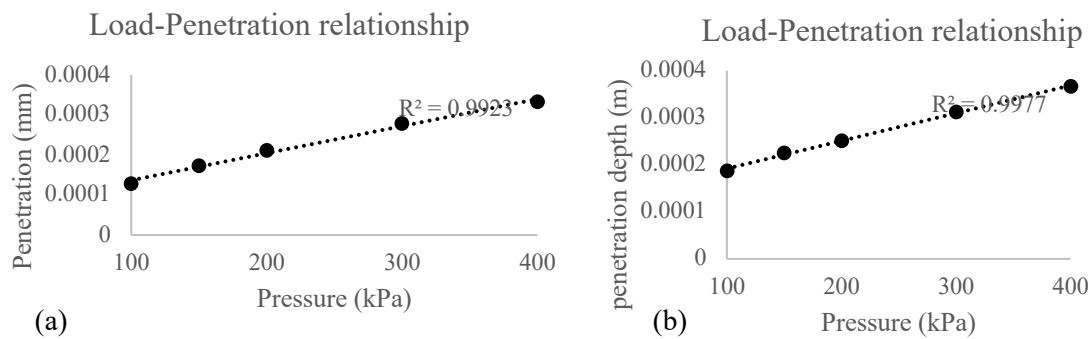
Figure A2-10. Load-Penetration relationship for (a) \lambda=4\text{mm} and (b) combination of \lambda=4\text{mm} , 1mm, and 0.25 mm
