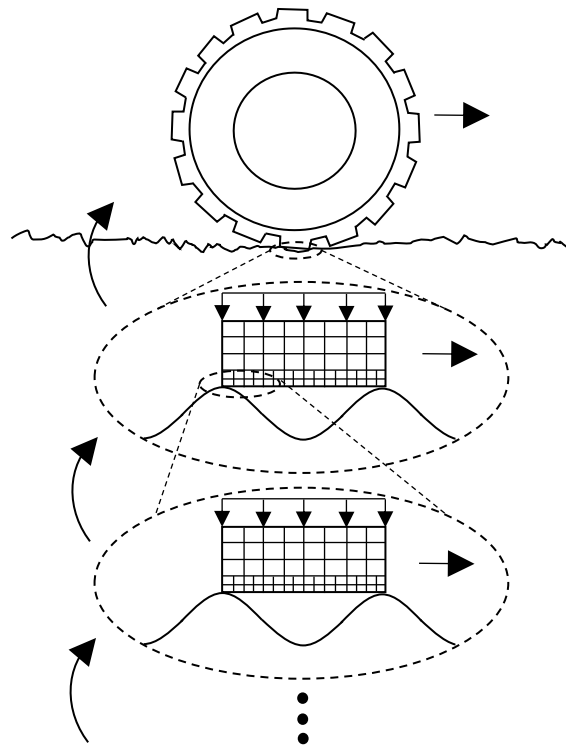
Figure A2-1. A sample of wavelength combination for pavement surface simulation in FE model Then, in each scale, the contact between the sinus wave and the rubber block with the same width as the wavelength of the sinus wave is modeled, see Figure A2-2.
