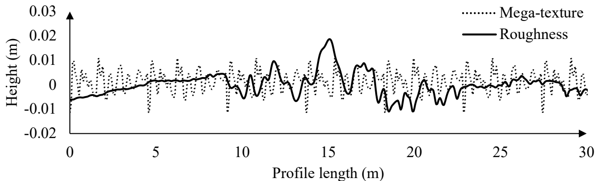
Figure 5-14. Comparison of mega-texture profile with RMS of 4.4 mm with roughness profile with RMS of 4.8 mm
