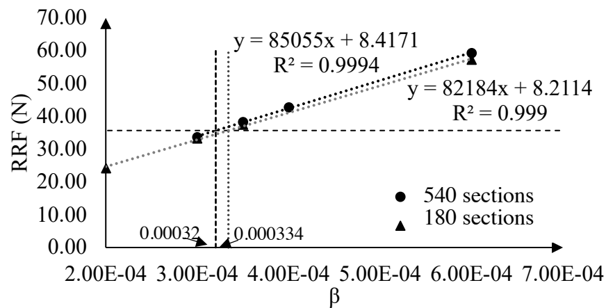
Figure 4-30. Relationship between the tire rolling resistance force and \beta rolling over a smooth surface with 80km/h speed
