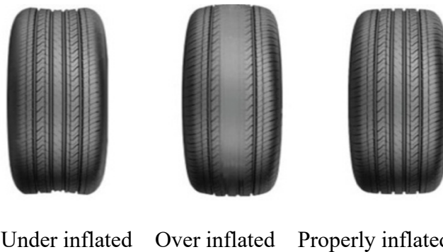
Figure 4-13. Effect of inflation pressure on tire deformation 2
