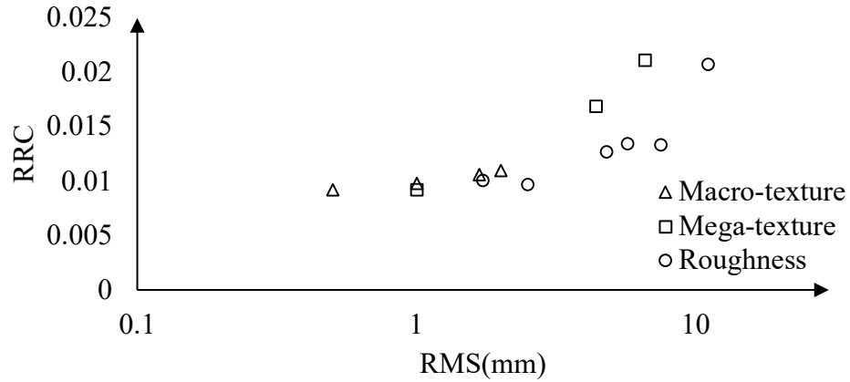
Figure 5-13. Comparison of the effect of macro-texture, mega-texture, and roughness on rolling resistance coefficient of quarter-car FE model in semi-log space
