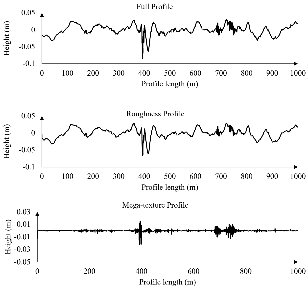
Figure 3-2. Division of the surface into different scales (data from NCHRP 720 report
