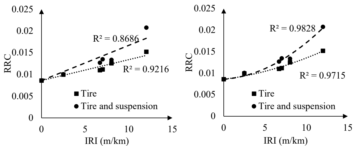
Figure 5-10. Effect of roughness profile IRI on RRC of the quarter car model with linear and non-linear relationships
