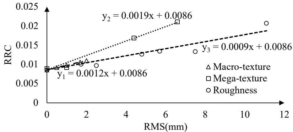
Figure 5-12. Comparison of the effect of macro-texture, mega-texture, and roughness on rolling resistance coefficient of quarter-car FE model
