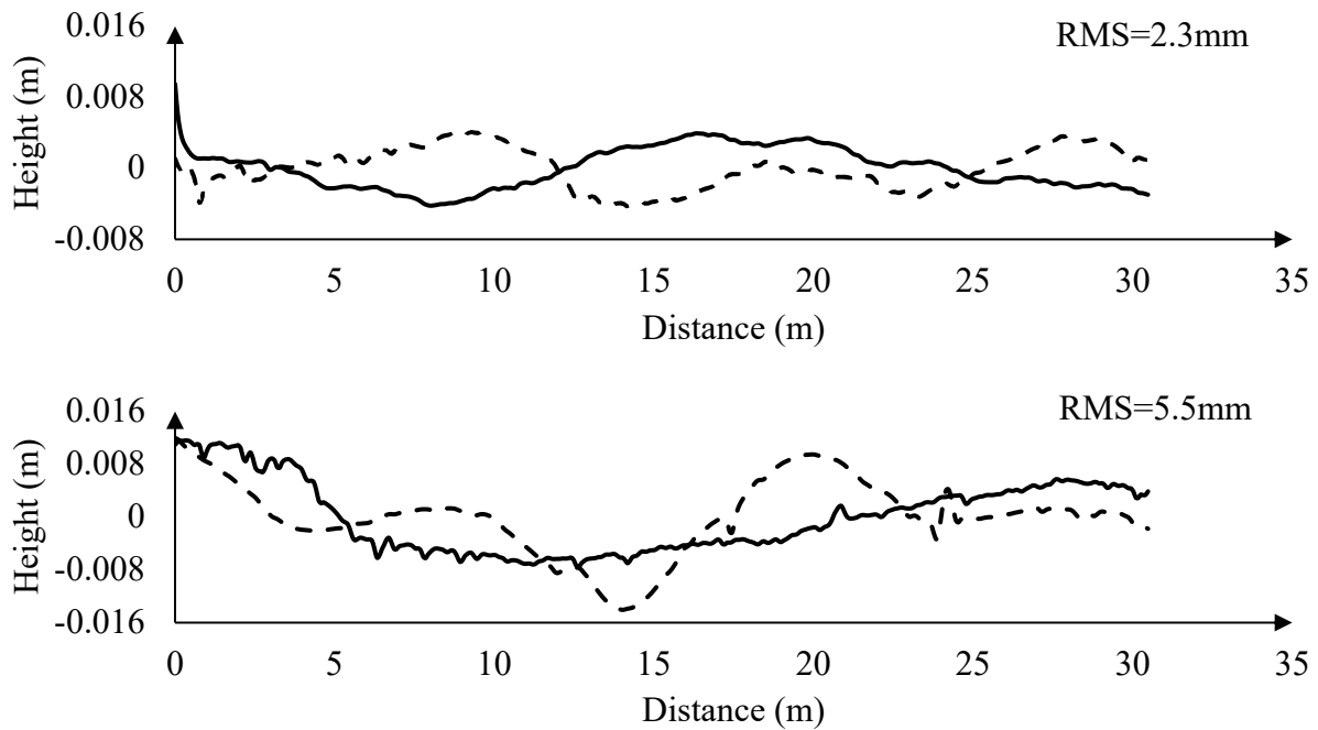
Figure 3-17. Comparison of different roughness profiles with the same RMS values
