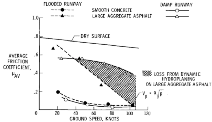
Figure 4-12. Friction coefficient on dry surfaces (Horne and Leland, 1962)
