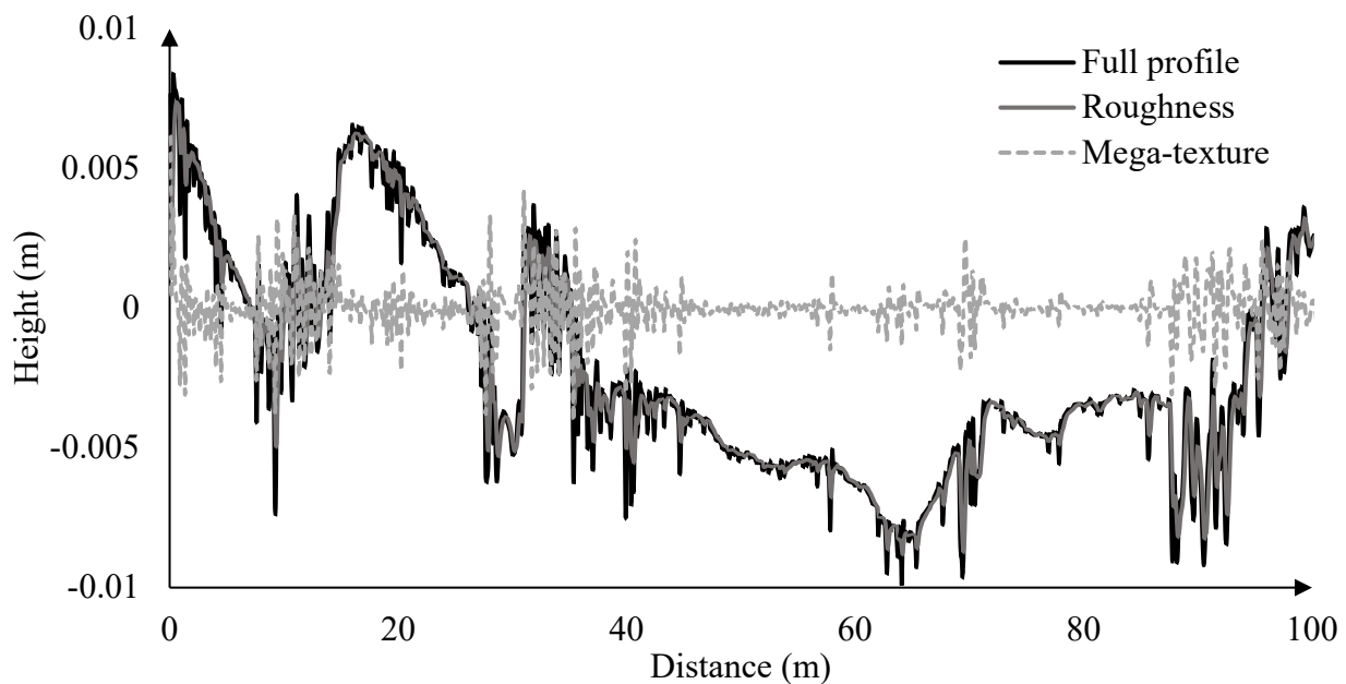
Figure 3-20. Frequency of the high mega-texture in the profile
