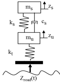
Figure 2-5. Schematic of Two DoF Quarter-Car Vehicle Model
