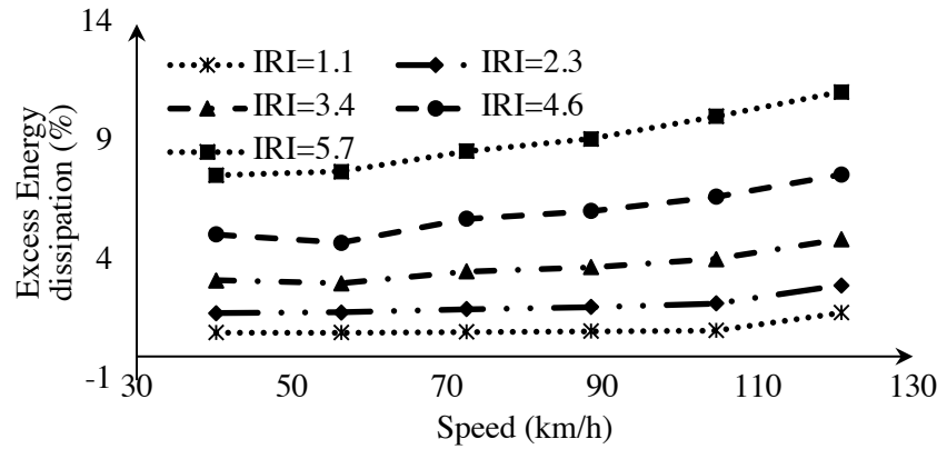
Figure 2-15. Effect of speed on energy dissipation at different roughness levels
