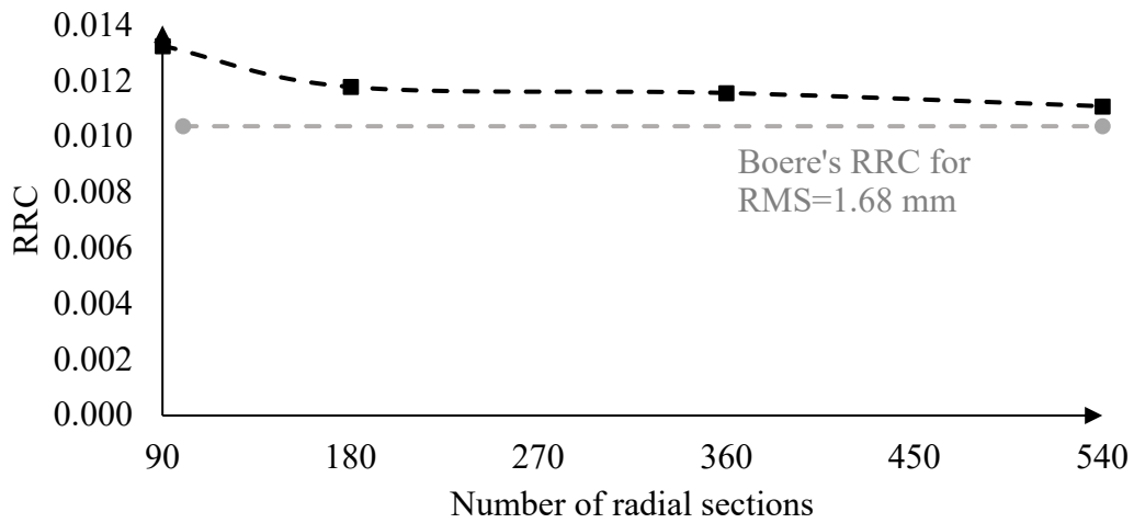
Figure 4-35. Variation of tire rolling resistance coefficient rolling over a textured surface with macro-texture RMS of 1.68 mm and speed of 80km/h for different numbers of radial sections
