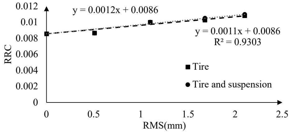
Figure 5-3. Effect of macro-texture profile's RMS on RRC of the tire and the quarter car model
