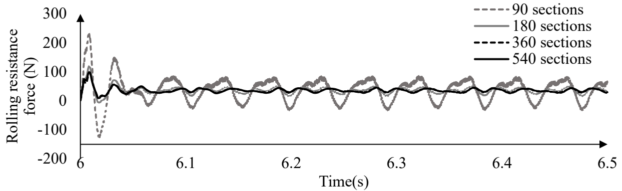
Figure 4-32. Variation of tire rolling resistance force rolling over a smooth surface with 80km/h speed for different number of radial sections
