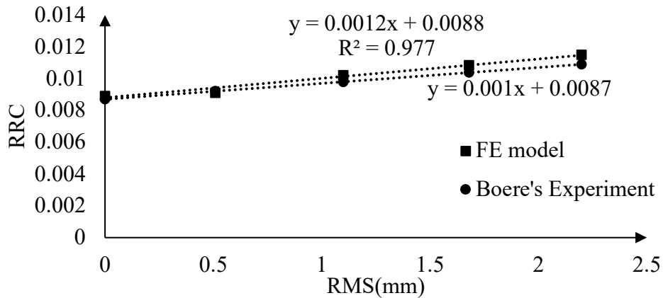
Figure 5-2. Effect of macro-texture profile's RMS on tire rolling resistance coefficient
