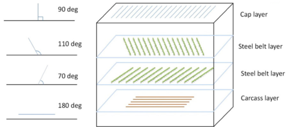
Figure 4-3. A schematic representation of reinforcement distribution in the tread layer (Wei and Olatunbosun, 2016)
