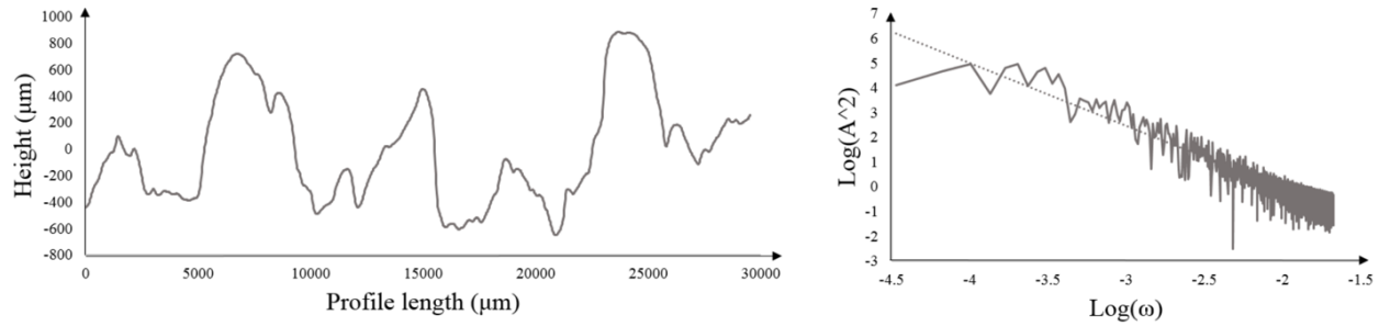
Figure 2-6. A surface profile and its corresponding PSD
