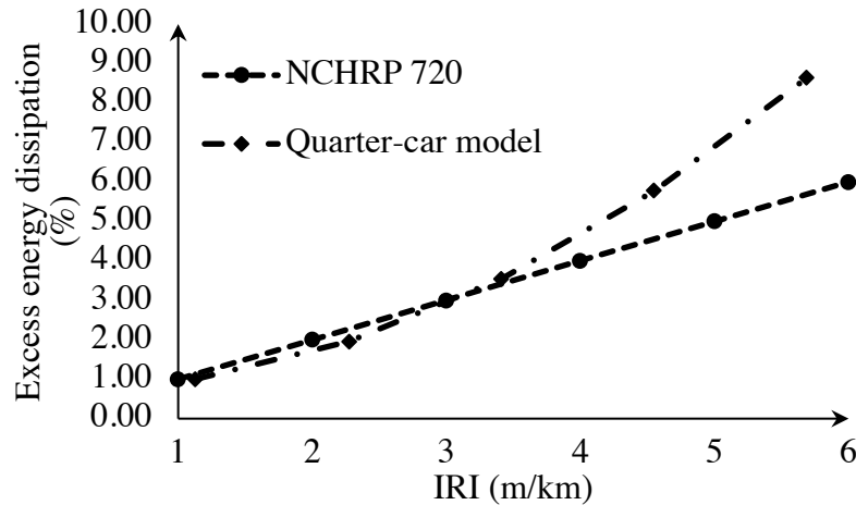
Figure 5-23. Comparison of the effect of IRI on energy dissipation of a car for NCHRP720 report and mechanistic quarter-car model at v=80 km/h (Zaabar et al. 2018)
