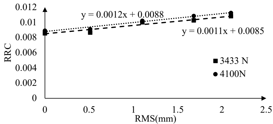
Figure 5-30. Effect of applied load on variation of rolling resistance with surface macro-texture Therefore, it can be concluded that although the normal load affects the absolute RRC value, it does not affect the variation of rolling resistance with texture (i.e., the effect of texture on rolling resistance).
