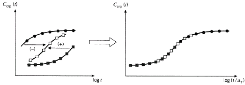
Figure 4-7. Master Curve (Roylance, 2001)
