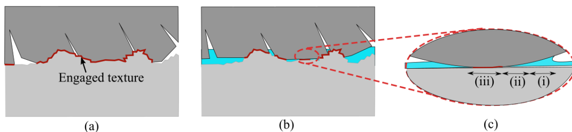
Figure A1-3. Effect of water presence on contact area (a) contact without water, (b) contact in presence of water, and (c) contact zone
