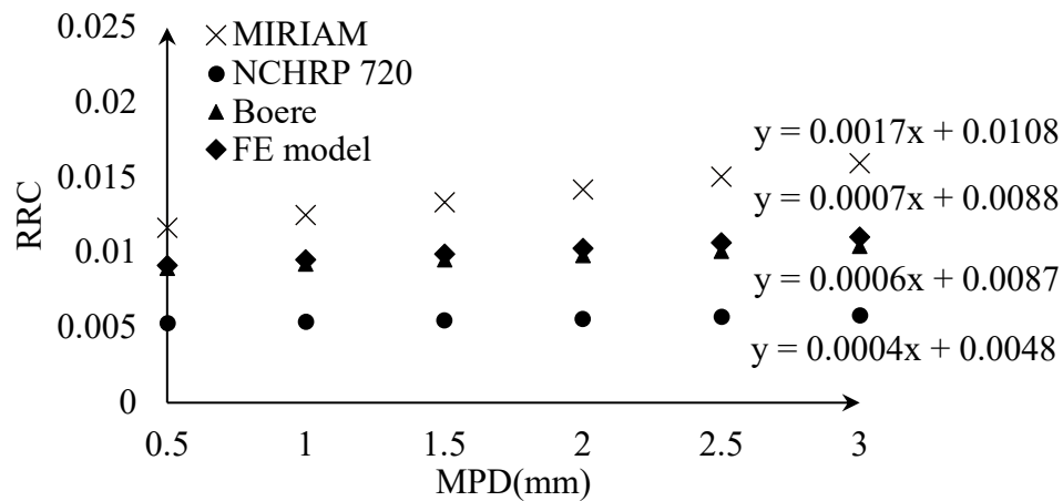
Figure 5-21. Comparison of rolling resistance coefficients of MIRIAM, NCHRP 720, Boere study and quarter-car FE model for a car at v=80 km/h
