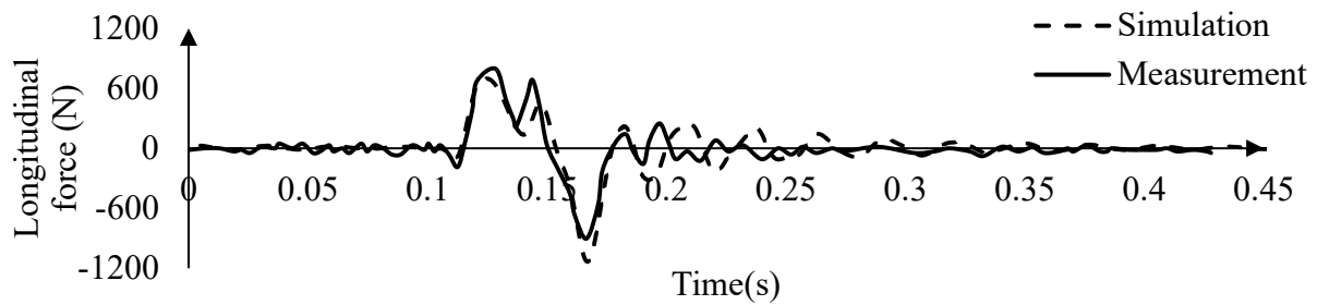
Figure 4-24. FE tire model rolling over a step
