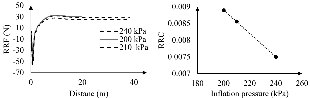
Figure 5-37. Effect of inflation pressure on rolling resistance force and coefficient on a smooth surface at 80km/h
