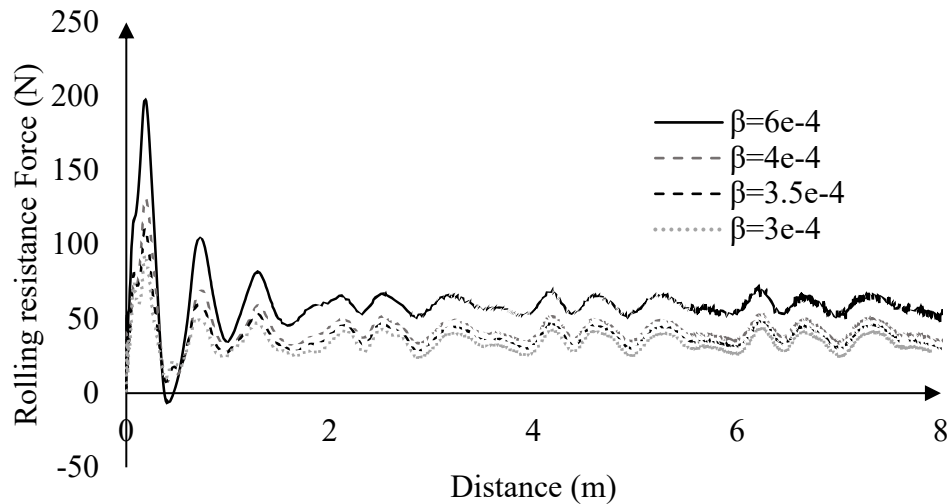
Figure 4-29. Variation of tire rolling resistance force rolling over a smooth surface with 80km/h speed for different Rayleigh damping coefficients
