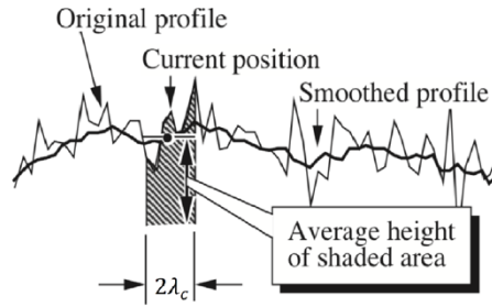
Figure 2-4. Moving average filter of a profile (Sayers and Karamihas, 1996)
