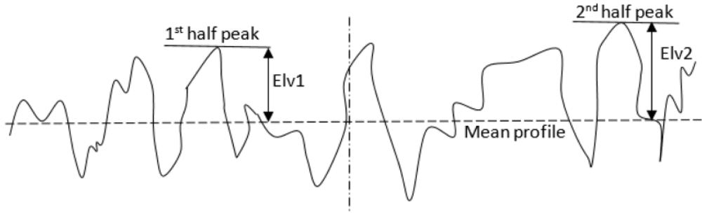
Figure 3-8. Surface texture MPD calculation
