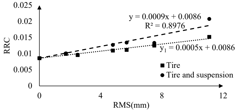
Figure 5-9. Effect of roughness profile RMS on RRC of the tire and the quarter car models
