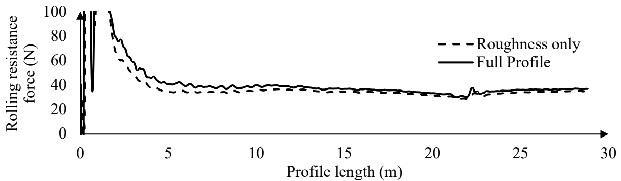
Figure 5-18. Rolling resistance forces for full profile and filtered roughness profile of profile 2 with IRI=3.85 m/km
