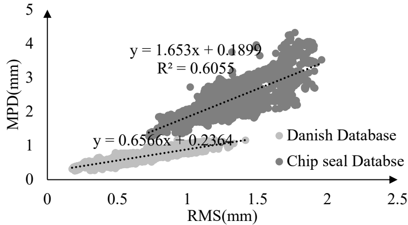
Figure 3-9 Relationship between RMS and MPD values for Danish and Chip seal databases
