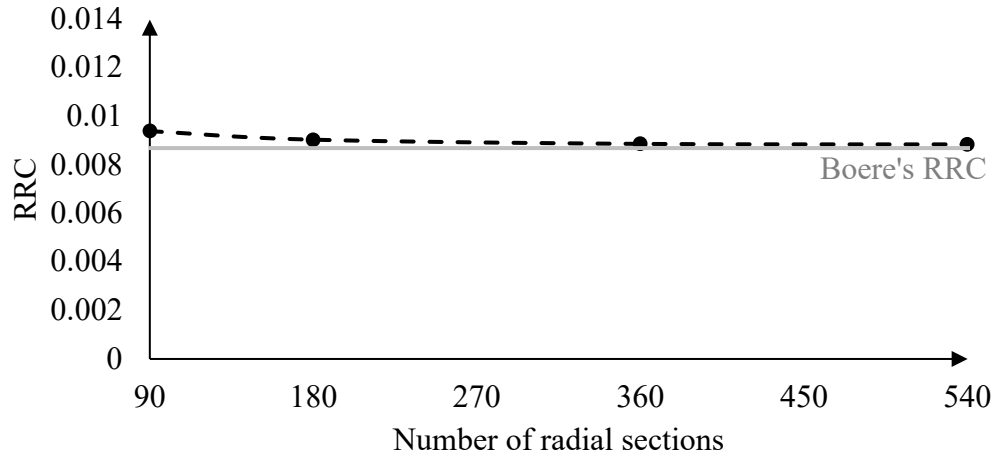
Figure 4-34. Variation of tire rolling resistance coefficient rolling over a smooth surface with 80km/h speed for different numbers of radial sections
