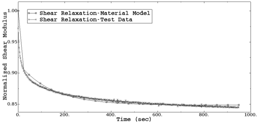
Figure 4-6. Prony series comparison to the test data (Wei et al, 2016)
