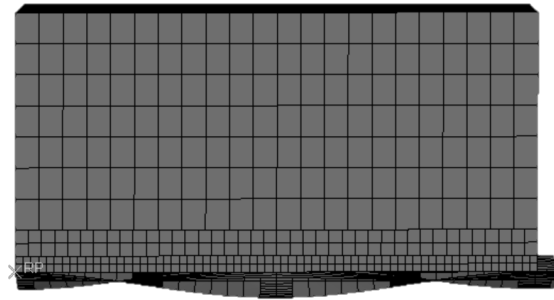
Figure A2-5. Rubber block mesh
