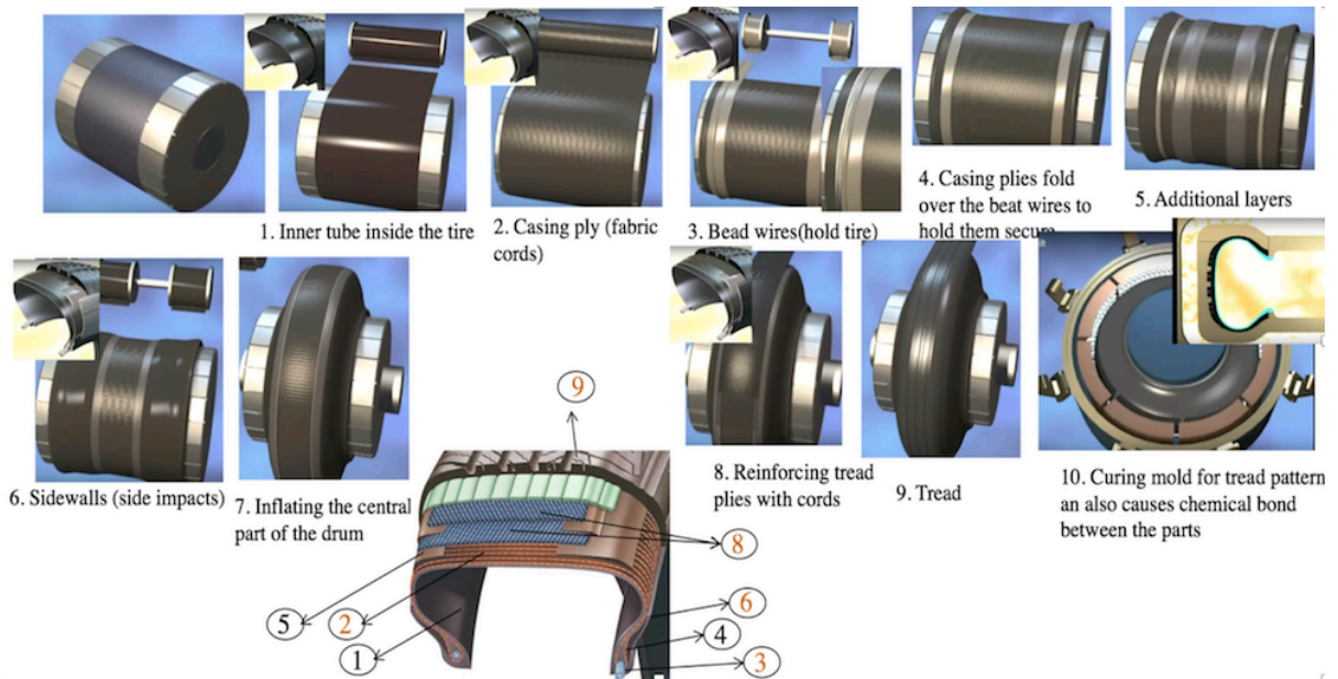
Figure 4-1. Tire manufacturing process and various parts (made from photos from Michelin's tire website)
