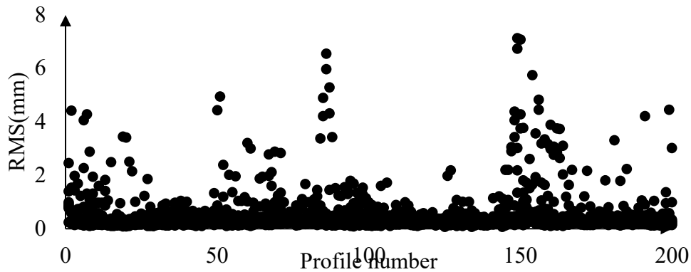
Figure 3-15. RMS variation for mega-texture profiles of 12 meters long
