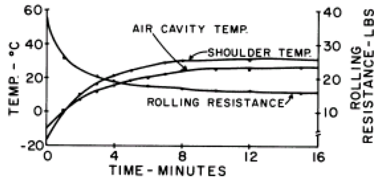
Figure 5-35. Inflated air temperature variation with tire shoulder temperature (Janssen and Hall, 1980)
