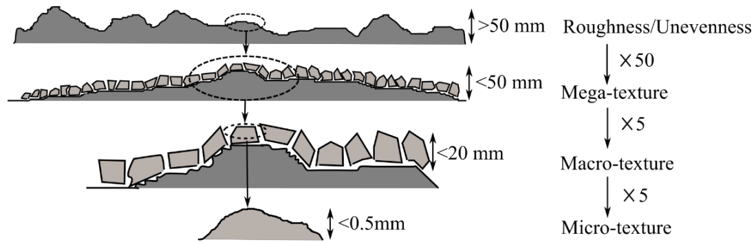
Figure 2-2. Simplified illustration of various pavement surface profile ranges (after Sandburg, 1990)
