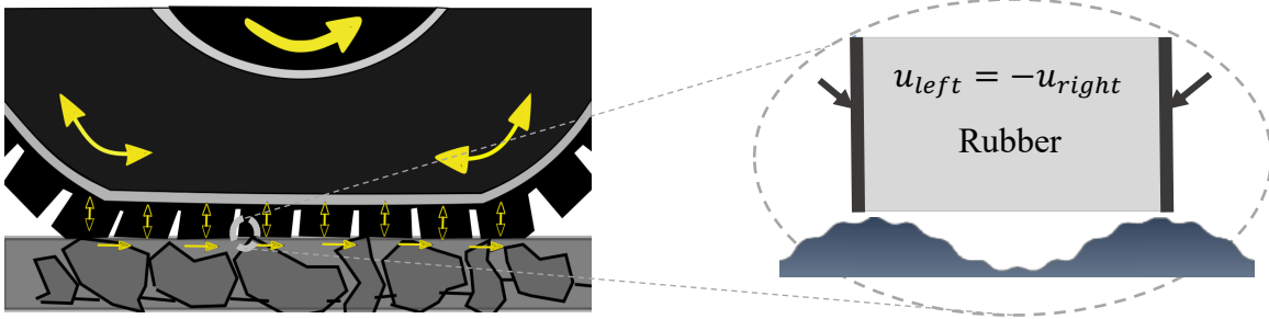
Figure A2-4. Periodic Boundary condition
