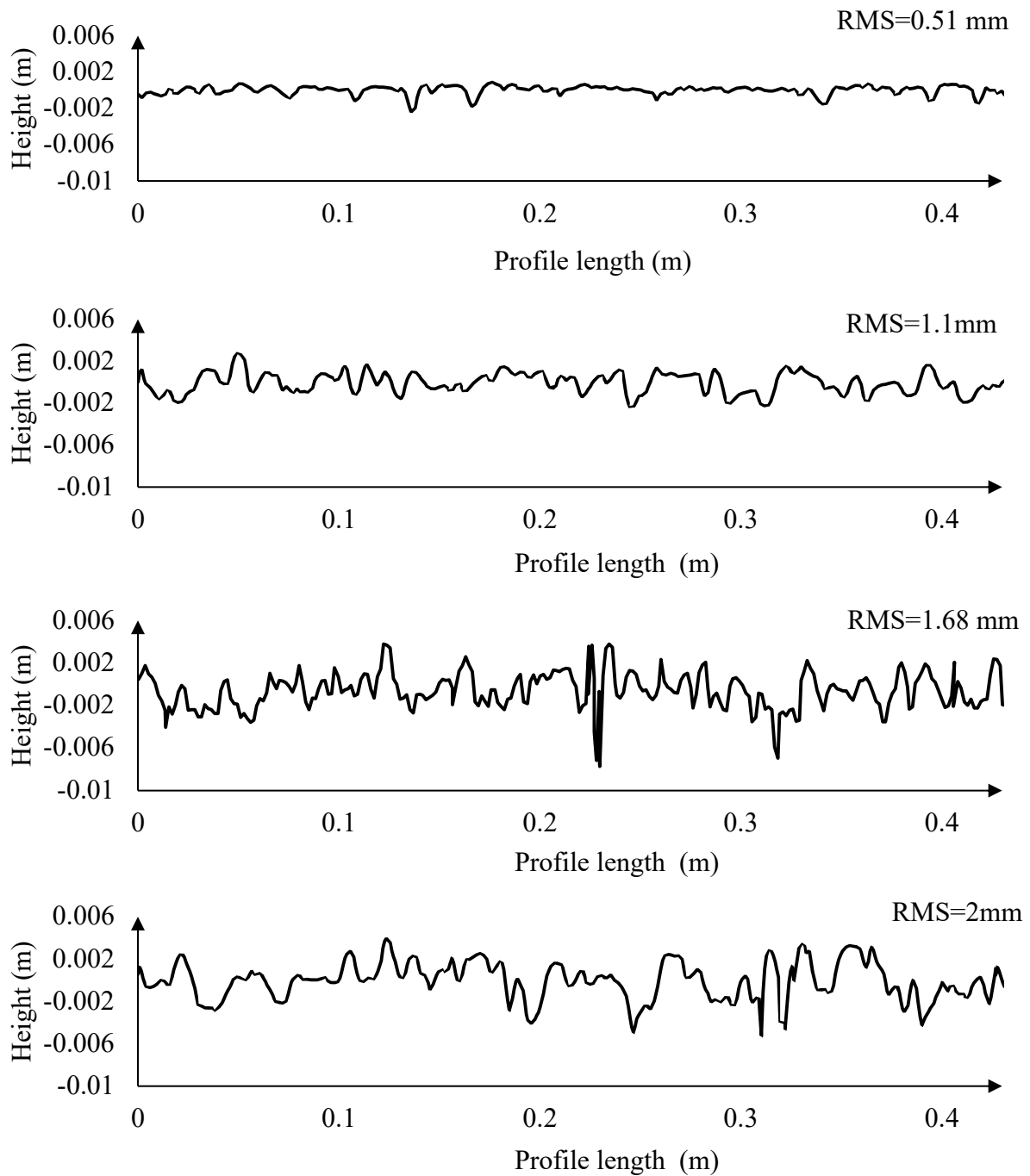
Figure 3-21. Selected profiles for macro-texture scale, with different RMS values
