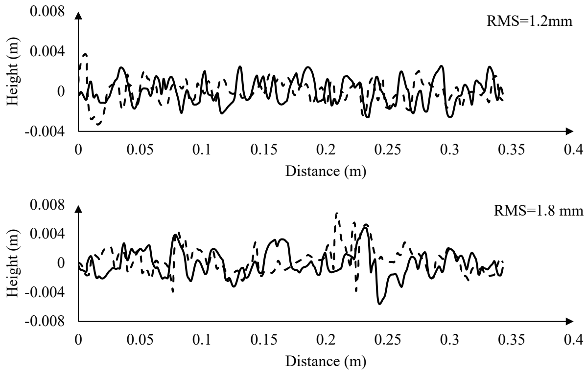
Figure 3-19. Comparison of different macro-texture profiles with the same RMS values
