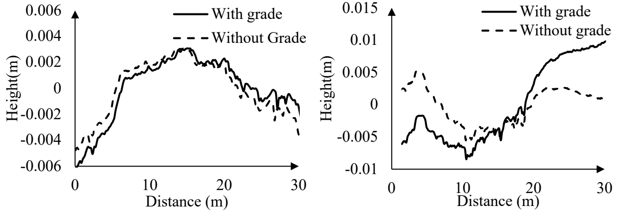
Figure 3-6. Grade removal from surface profiles
