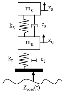
Figure 5-1. Schematic of Two DoF Quarter-Car Vehicle Model (Zaabar et al., 2018)
