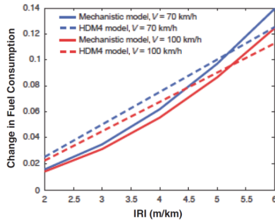
Figure 2-11. Fuel consumption variation with IRI at v = 70 and 100 km/h for a medium car (Louhghalam et al. 2015)
