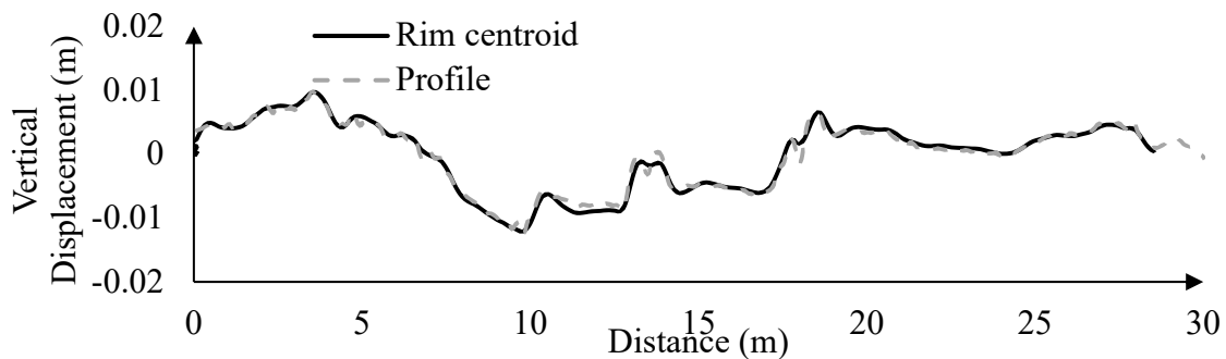
Figure 5-26. The vertical displacement of the rim centroid and the profile for IRI=3.3 m/km
