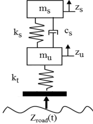
Figure 3-7. Standard Quarter-car model for IRI calculation (Zaabbar et al, 2018)
