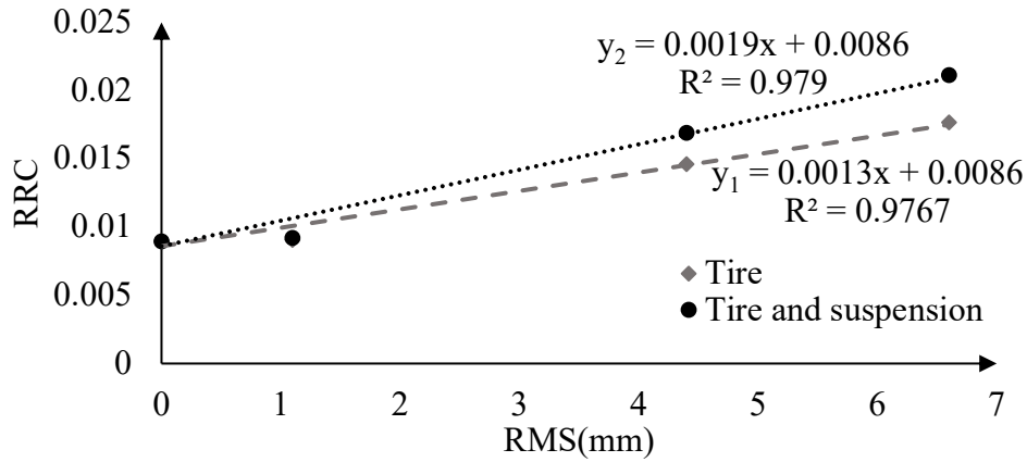
Figure 5-5. Effect of mega-texture profile's RMS on RRC of the tire and the quarter car models
