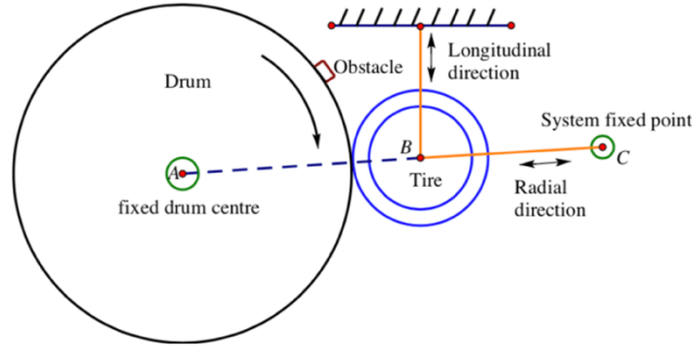
Figure 4-23. Schematic test setup for transient rolling of tire over an obstacle (Wei and Olatunbosun, 2016)
