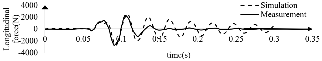
Figure 4-26. Comparison of the FE model with experimental measurements of Wei and Olatunbosun (2016), at velocity of 20km/h
