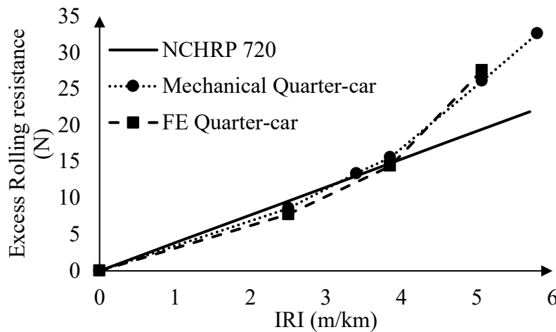
Figure 5-24. Comparison of the effect of IRI on rolling resistance of a car for quarter-car FE model and previous studies.
