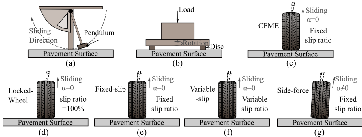
Figure A1-5. Friction measurement devices: (a) BPT (b) DFT (c) CFME (d) Locked-wheel (e) Fixed-slip (f) Variable-slip (g) Side-force
