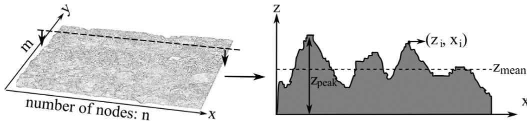
Figure 2-7. Surface texture parameters
