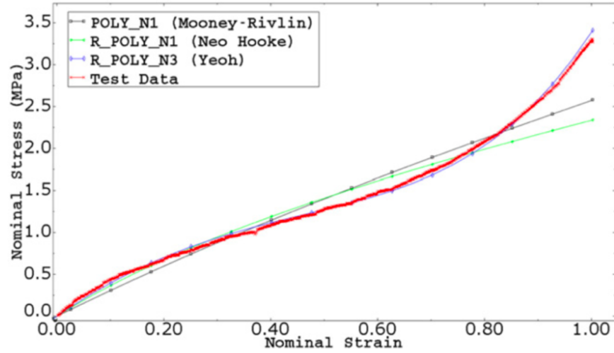
Figure 4-5. Yeoh model comparison to the test data (Wei and Olatunbosun, 2014)
