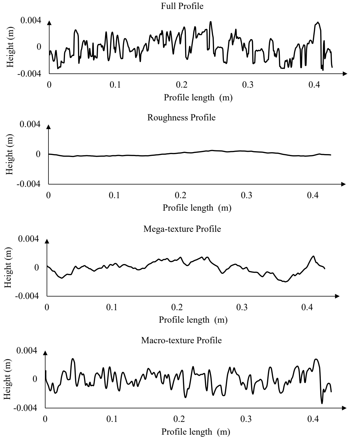
Figure 3-3. Division of the surface into different scales (Chip seal surfaces)
