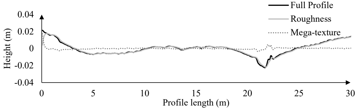
Figure 5-16. Profile 2, IRI= 3.85m/km
