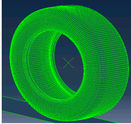
Figure 4-20. Full 3D tire model
