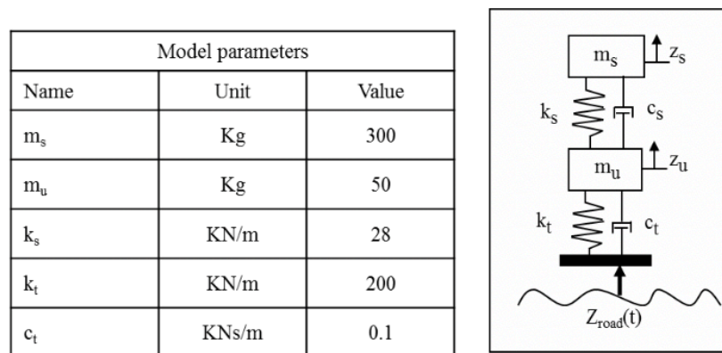
Figure 4-15. Quarter car model (Dixon, 2008)
