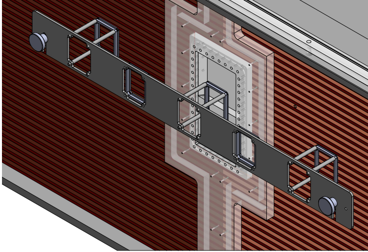
Figure 2.40: Target Ladder
