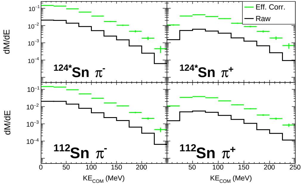
Figure 4.41: Pion kinetic energy spectra in COM frame. \pi^- are drawn on the left side, \pi^+ on the right. The top panels are for the ^{124}\text{Sn} system, while the bottom panels are for the ^{112}\text{Sn} system.
