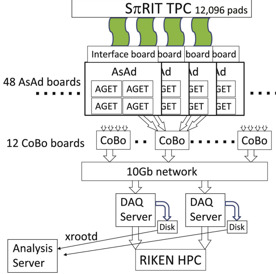
Figure 2.4: GET architecture employed for S \pi RIT TPC, from [5].
