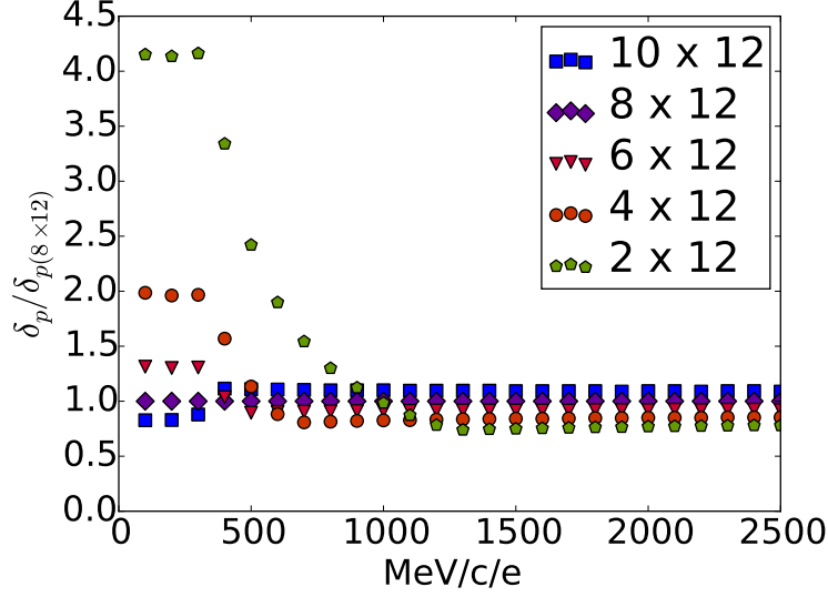
Figure 2.8: Relative error of momentum measurement for different pad sizes.
