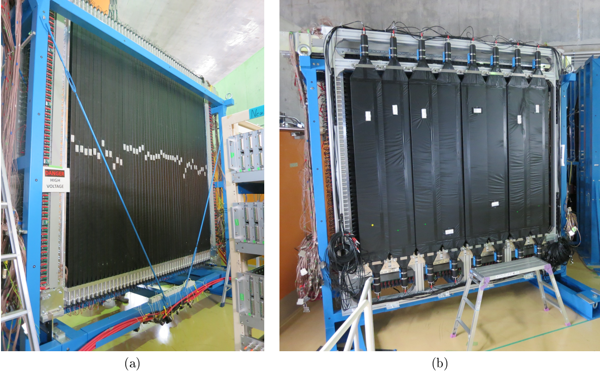
Figure 3.17: The partial NeuLAND array is shown in (a), and the charged particle veto array borrowed from NEBULA is shown in (b)
