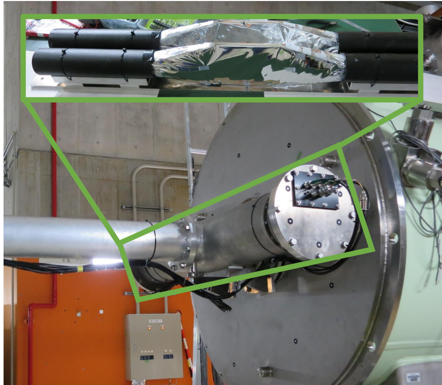
Figure 3.5: SBT array
