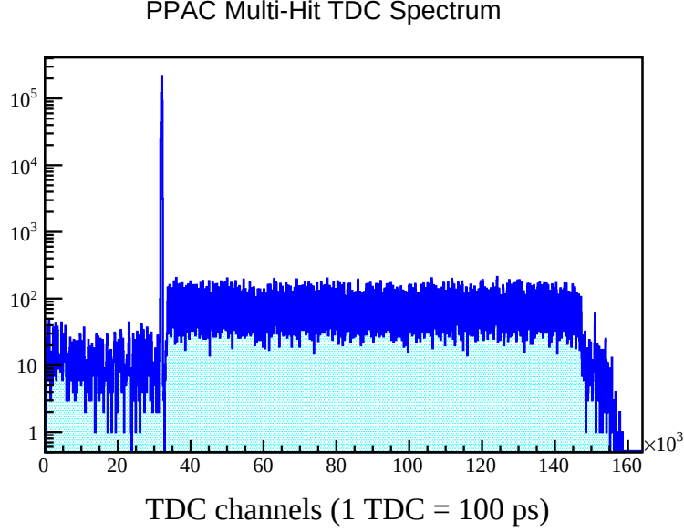
Figure 4.16: Multi-hit TDC spectra, from a PPAC at the F7 focal plane, for ^{132}\text{Sn} beam
