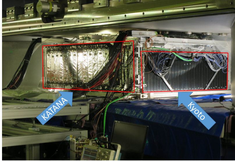
Figure 3.4: Photograph of the TPC and ancillary detectors installed in the SAMURAI spectrometer.
