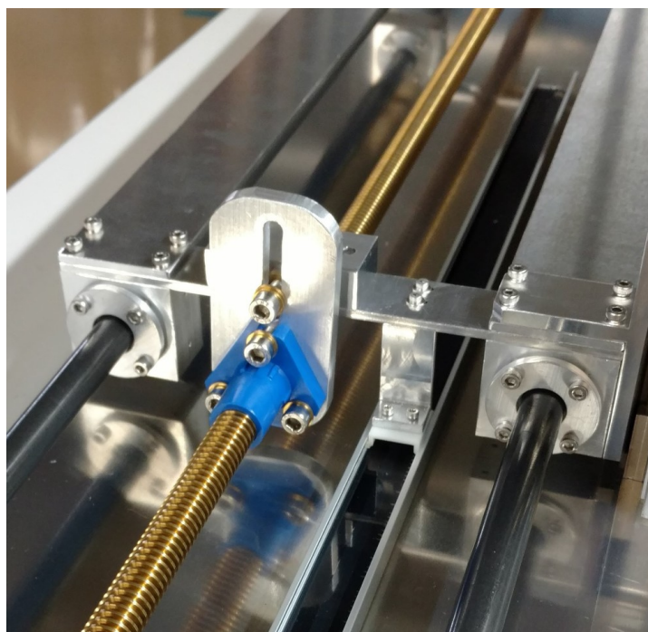
Figure 2.57: The installed target motion nut, which accommodates a warped lead screw (April 2018).
