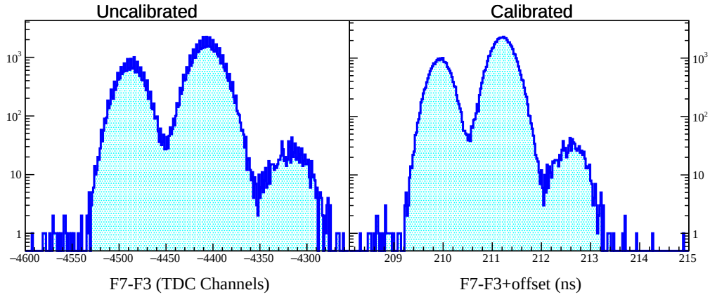
Figure 4.8: The uncalibrated (a) and calibrated (b) time-of-flight spectra from run 2894.
