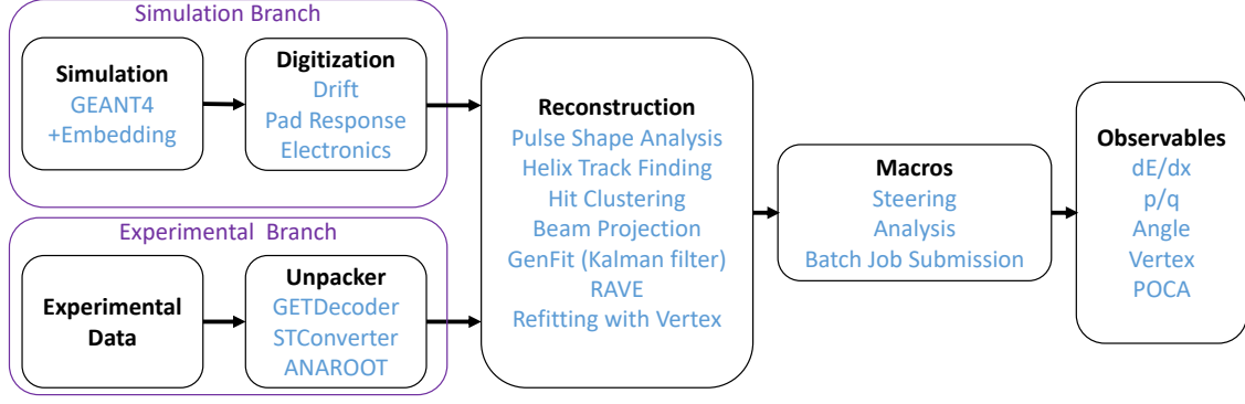
Figure 4.31: Analysis flow for the S \pi RITROOT software package, showing branches for experimental data as well as simulation
