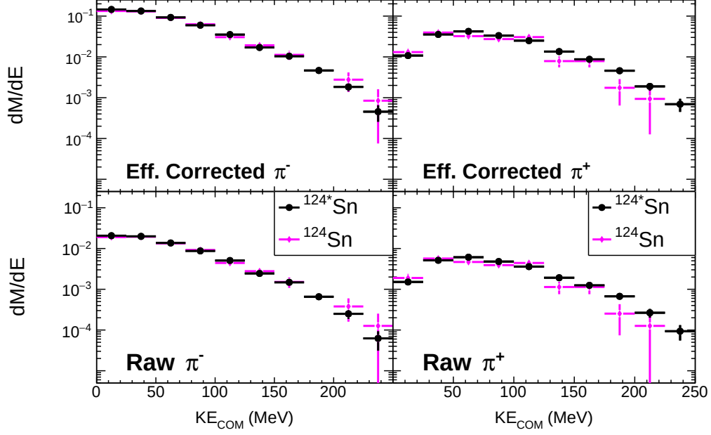
Figure 4.44: Pion KE_{COM} spectra for ^{124*}Sn and ^{124}Sn beams. The top panel is efficiency corrected, and the bottom is the raw spectra.
