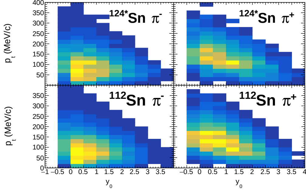
Figure 4.43: p_t - y_0 distributions, with rapidity normalized to beam rapidity. \pi^- are drawn on the left side, \pi^+ on the right. The top panels are for the ^{124*}\text{Sn} system, while the bottom panels are for the ^{112}\text{Sn} system.
