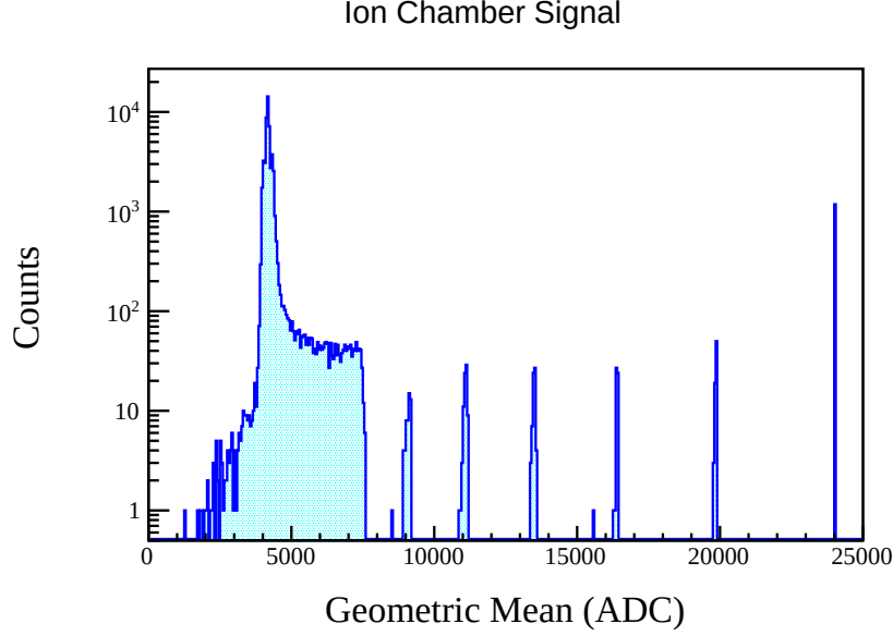
Figure 4.15: Ion chamber signal for ^{124}\text{Sn} beam
