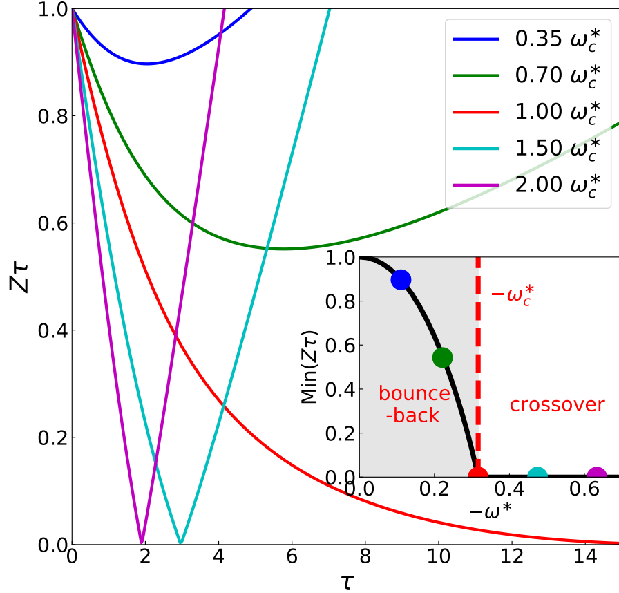
Figure 2.1: Longitudinal width evolution Z(\tau) of prolate spheroids with ( \alpha_0 = 10/75 ) driven by different initial chirps in numeric solutions of MFT ranging from below the critical chirp ( -0.35\omega_c^* ) to well above ( -2.0\omega_c^* ). The sub-graph shows the dependence of minimum width on initial reduced chirp. For this particular \alpha_0 , the critical value \omega_c^* (red dot), divides the focusing into bounce-back and crossover regimes.
