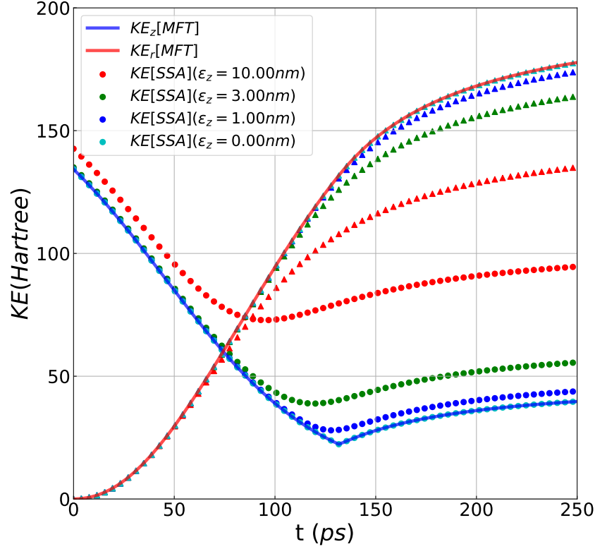
Figure 3.3: Kinetic energy evolution for cross-over case ( -1.5\omega_c^* in the longitudinal direction, corresponding to panel (c) in Fig. 3.2), with solid lines for MFT and dotted lines for SSA with different value of emittance (circle for KE_z and triangle for KE_r ). The sudden change of direction for MFT in longitudinal kinetic energy comes from the sign flip of the chirp as discussed in Sec. 2.
