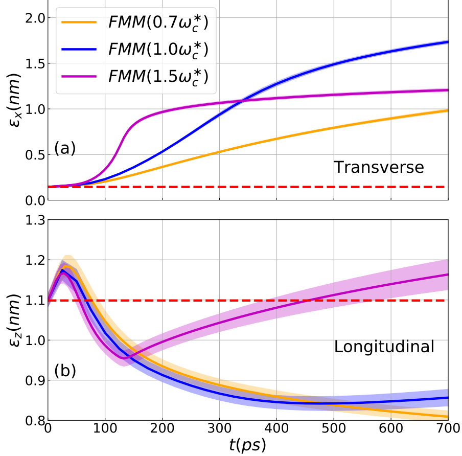
Figure 4.4: (rms) Emittance evolution in (a) transverse \varepsilon_x and (b) longitudinal \varepsilon_z direction for three different initial chirps.
