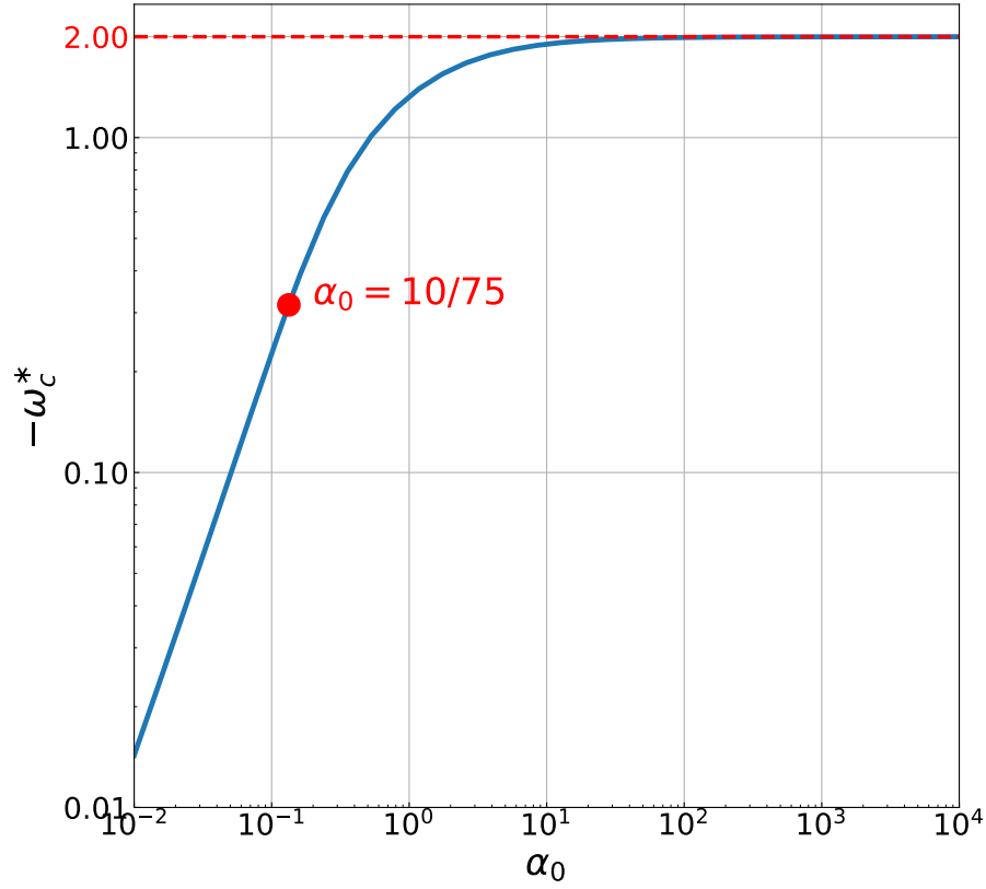
Figure 2.2: Dependence of critical reduced chirp \omega_c^* on initial aspect ratio \alpha_0 , with a horizontal asymptote of \omega_c^*(\alpha_0 \rightarrow \infty) = 2 .
