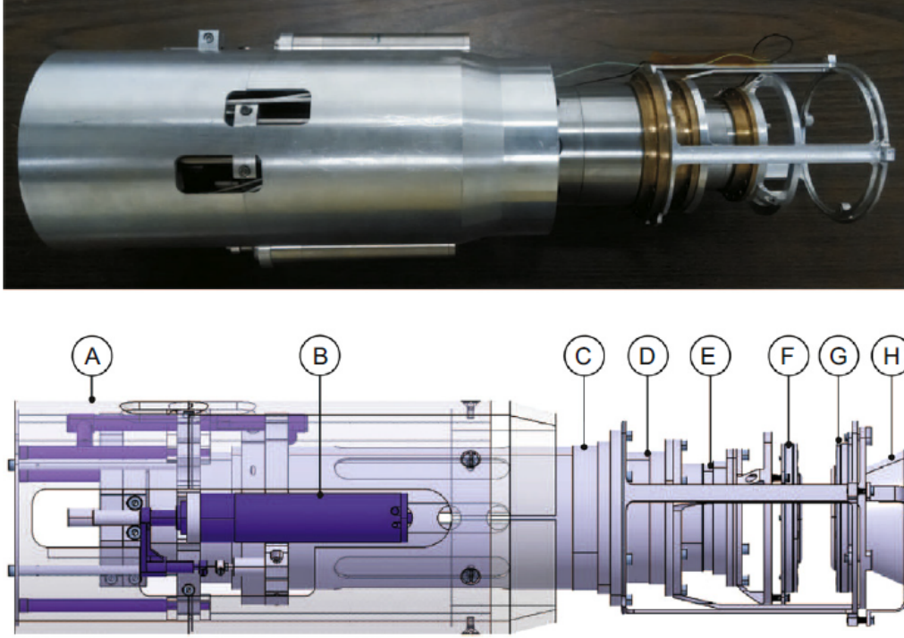
Figure 3.15: The TRIPLEX device used in this experiment. The schematic shows (A) the outer casing, (B) a piezoelectric motor, (C) the outermost tube, (D) the middle stationary tube, (E) the innermost tube, (F) the target positioned by the innermost tube E, (G) the first degrader held stationary by the middle tube, and (H) the second degrader positioned by the outermost tube. The figure is from Ref. [81].
