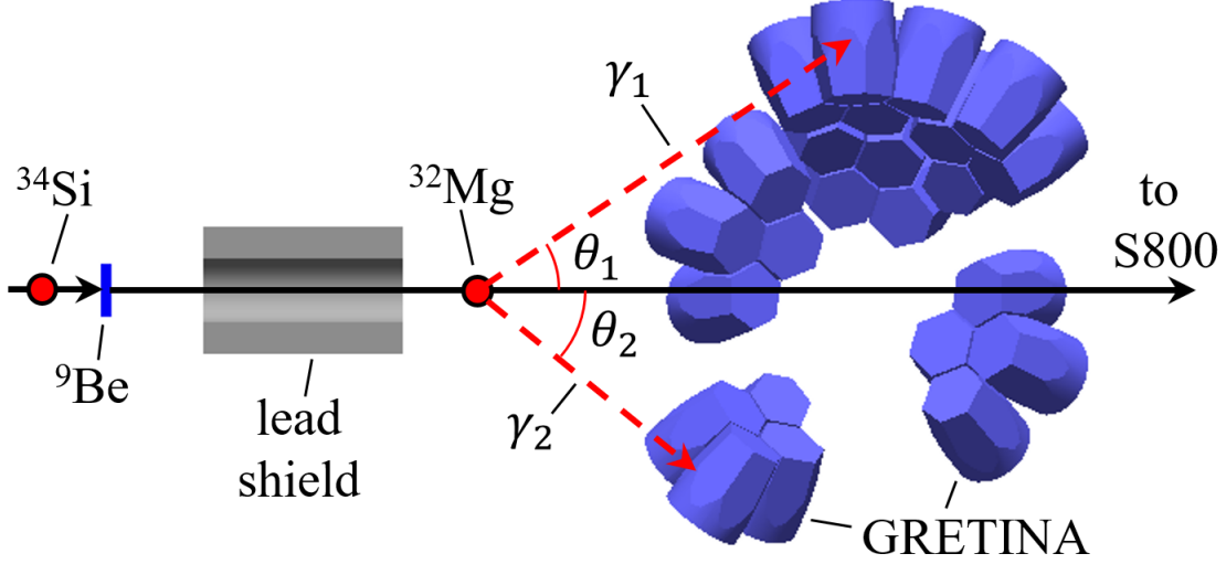
Figure 3.20: The setup for the part of the experiment with the upstream target, designed to measure the 0_2^+ isomer of ^{32}\text{Mg} . The ^9\text{Be}(^{34}\text{Si}, ^{32}\text{Mg})X reaction populates the 0_2^+ isomer which emits a cascade of gamma rays \gamma_1 and \gamma_2 at angles \theta_1 and \theta_2 relative to the ion trajectory.
