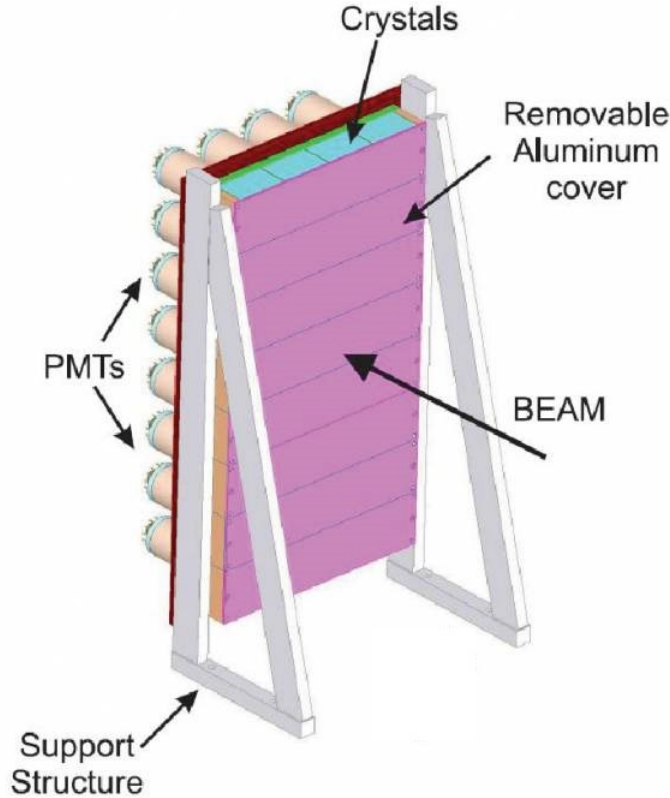
Figure 3.9: A diagram of the IsoTagger hodoscope. The 32 sodium-doped cesium iodide crystals are arranged into eight rows of four detectors each. The beam is stopped in an aluminum plate and gamma rays emitted from the decay of isomers are detected by the IsoTagger hodoscope.
