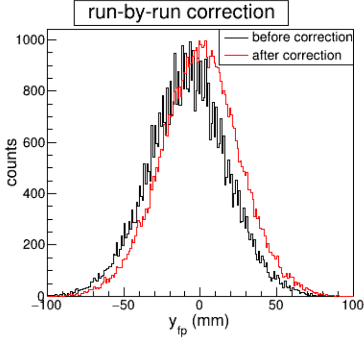
Figure 3.11: y_{fp} distributions, gated on ^{32}\text{Mg} reaction products. The distribution before run-by-run corrections is shown in black, while the distribution after run-by-run corrections is shown in red. The correction causes the distribution to be centered in the CRDC and slightly narrower.
