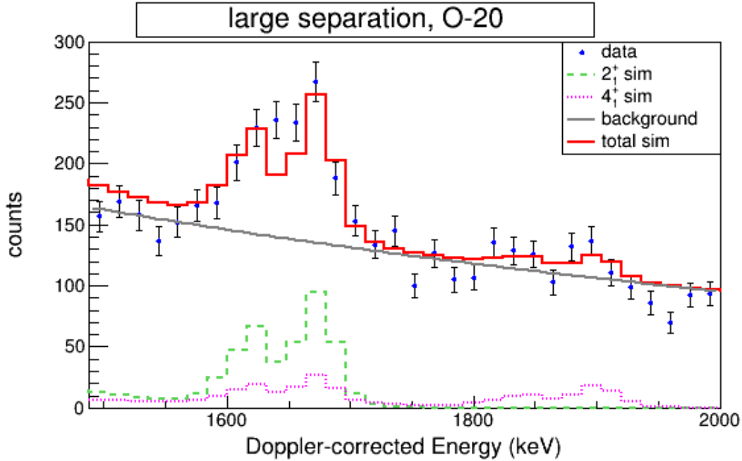
Figure 4.20: Doppler-corrected energy spectra of gamma rays from ^{20}\text{O} in the three-foil, large-separation setting. The data shows contributions at 1674-keV from the decay of the 2_1^+ state and at 1898-keV from the 4_1^+ state. The contributions of the populations of the 2_1^+ state and the 4_1^+ state are estimated with the simulated responses depicted with the dashed green and the dotted purple lines respectively. The solid gray line is an exponential background and the solid red line is the sum of the two simulation components and the background.
