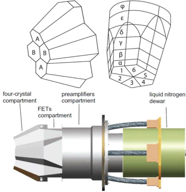
Figure 3.12: Diagram of a GRETINA module. The full module is shown in the bottom section. The four high-purity germanium crystals in a single module are depicted in the top-left. The segmentation of a single crystal is depicted in the top-right. The figure is adapted from Ref. [67].
