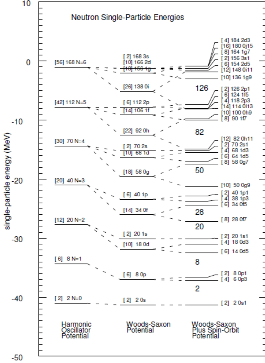
Figure 1.3: The single-particle orbits for neutrons in the ^{208}\text{Pb} nucleus, calculated for the harmonic oscillator potential, Woods-Saxon potential, and Woods-Saxon potential with spin-orbit term. The figure is adapted from Ref. [2]. The number in brackets is the occupancy of that orbit and is followed by the cumulative occupancy in that orbit and all lower-energy orbits. The orbits are labeled by the harmonic oscillator quantum number N , the orbital angular momentum quantum number l = s, p, d, f, g, h, i meaning l = 0, 1, 2, 3, 4, 5, 6 , and twice the total angular momentum quantum number 2j .
