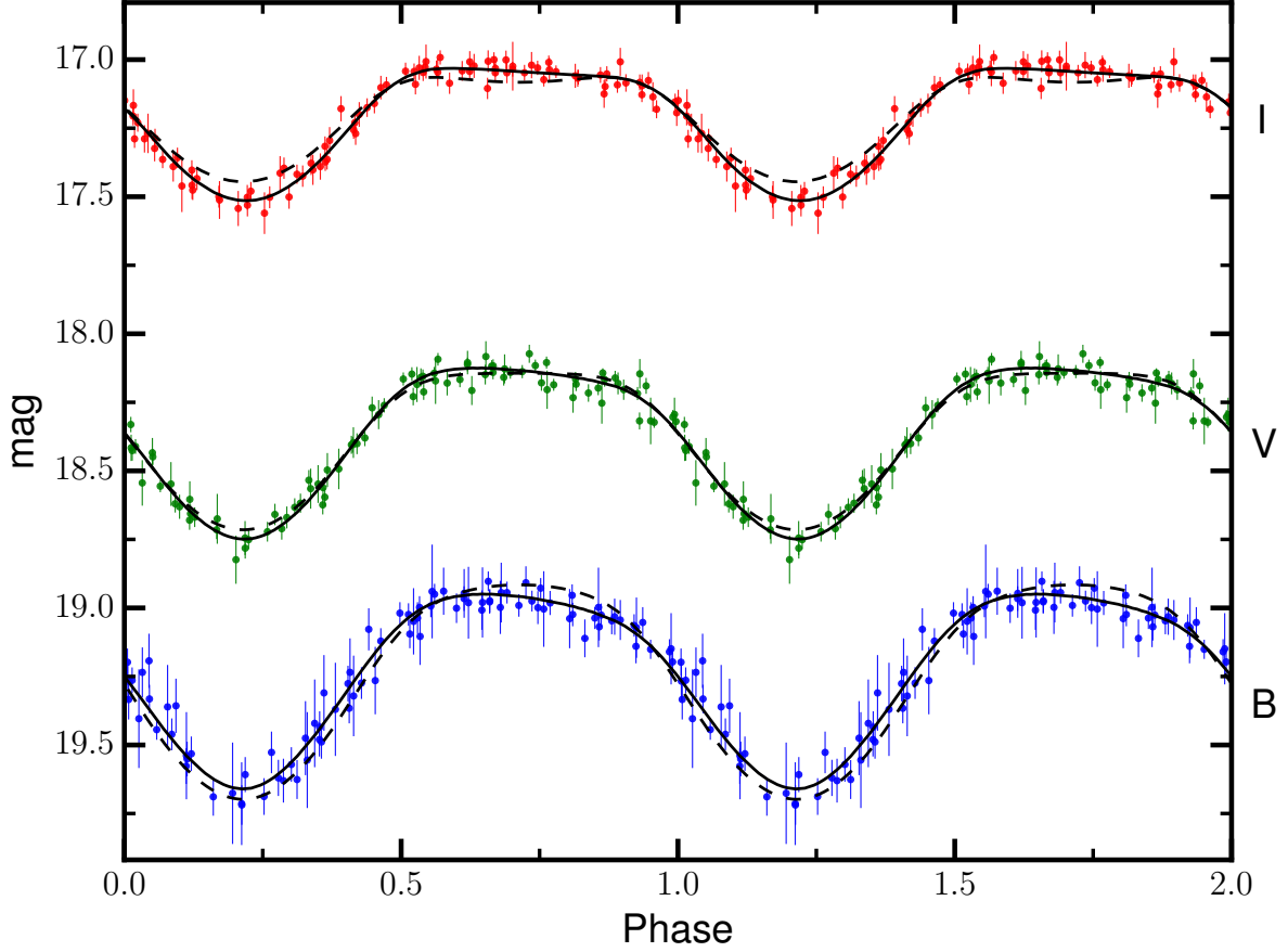
Figure 4.2: Optical light curve of PSR J1306–40. SMARTS optical photometry of PSR J1306–40. Black lines show the best fit “No Spot” (dashed) and “Hot Spot” (solid) ELC models from Table 4.3. Two full orbital phase cycles are shown for clarity.
