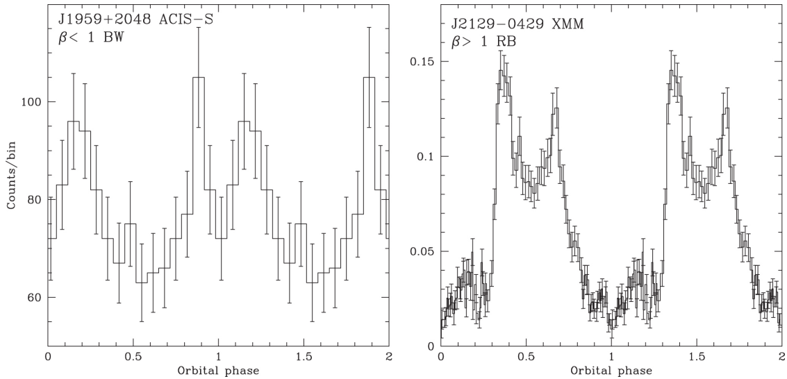
Figure 1.9: Example X-ray light curves due to strong intrabinary shocks. Example X-ray light curves showing the effects of the intrabinary shock for a black widow MSP binary with a weak companion wind (left), and a redback with a larger companion and a stronger wind (right). The data is repeated over two orbital cycles for visual clarity. The two peaks in the light curves are due to Doppler boosting of the shock when it is pointed towards the observer. In the black widow system, the shock wraps around the companion such that the peaks occur just before and just after the companion is in front of the MSP (pulsar superior conjunction). For the redback system, the companion wind is dominant so the shock wraps around the pulsar and the peaks are shifted by half an orbit (see text). Figure from Romani & Sanchez (2016).
