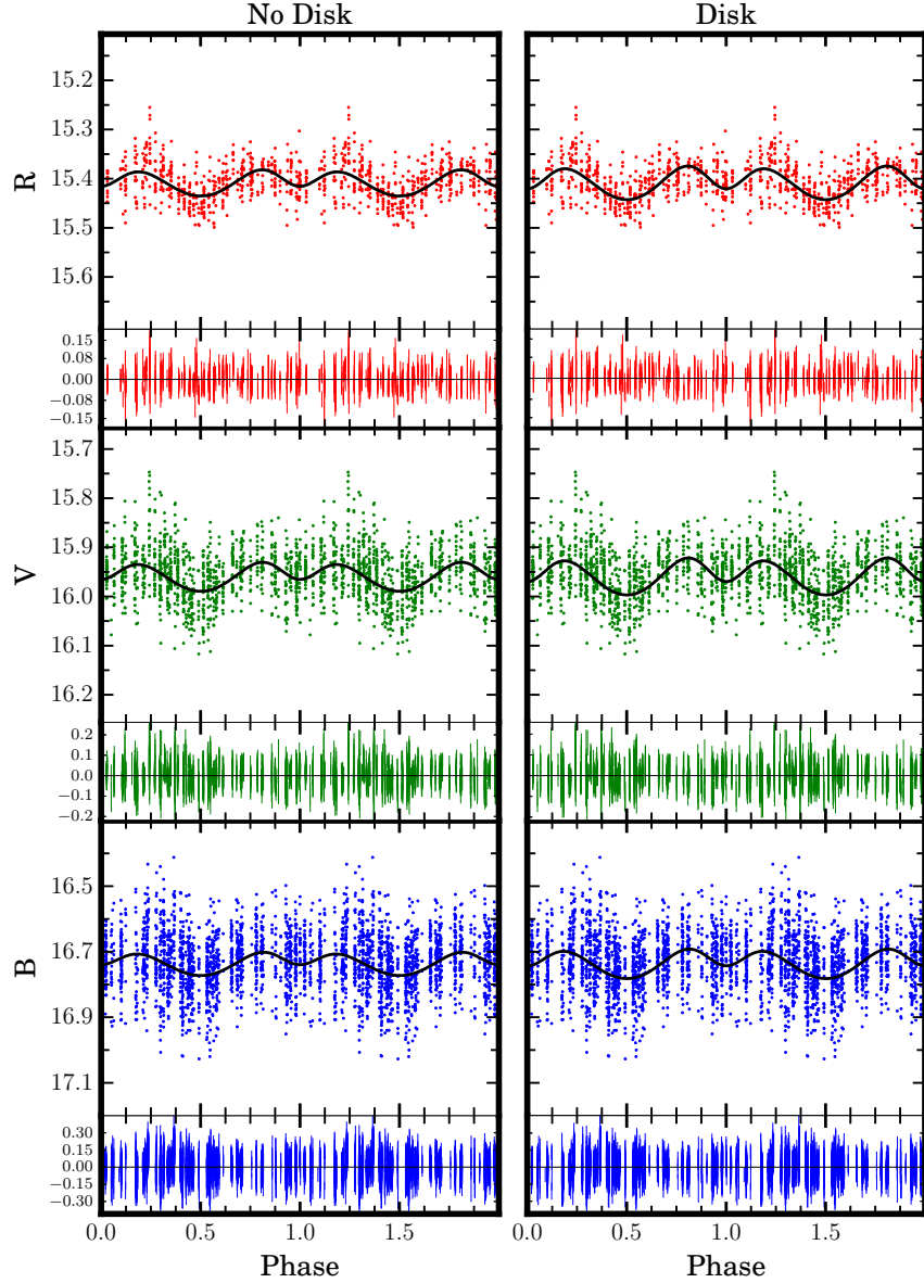
Figure 2.6: PROMPT optical light curve of 2FGL J0846.0+2820. PROMPT B , V , and R light curves folded on the spectroscopic period. The best fit ELC models that included (right) and excluded (left) a steady accretion disk component are shown with black lines. Uncertainties for each measurement are not shown in the upper panels, but are displayed in the fit residuals (lower panels). Two orbital phases are shown for clarity.
