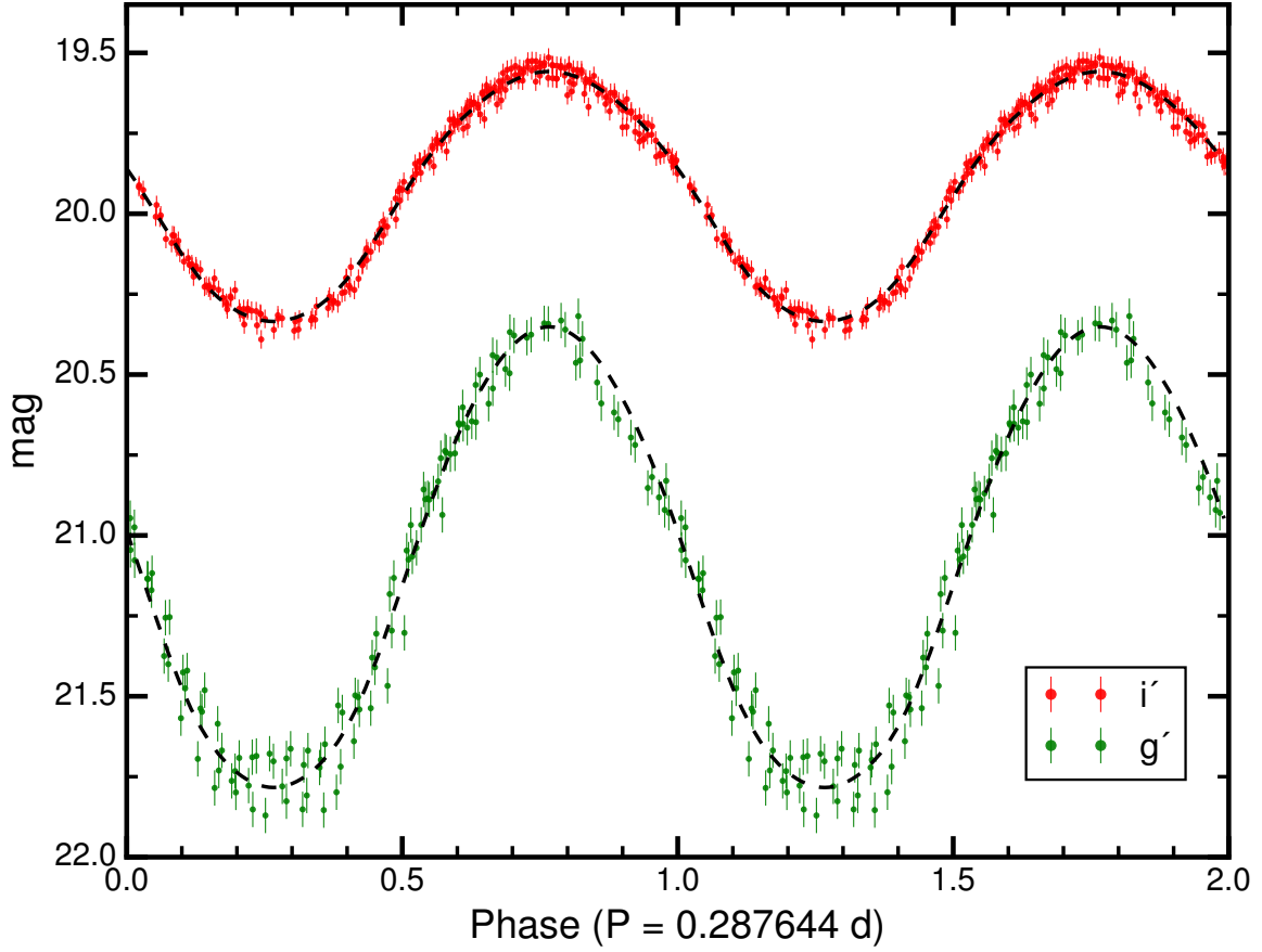
Figure 5.6: Optical light curve of 4FGL J2333.1–5527. SOAR g' (bottom) and i' (top) photometry of the companion to J2333 along with the best fit ELC model. The data described in § 5.2.3.1 have been folded on the best-fit period and ephemeris from § 5.3.1, and the uncertainties have been rescaled as described in the text (§ 5.3.4.1). Two orbital phases are shown for clarity.
