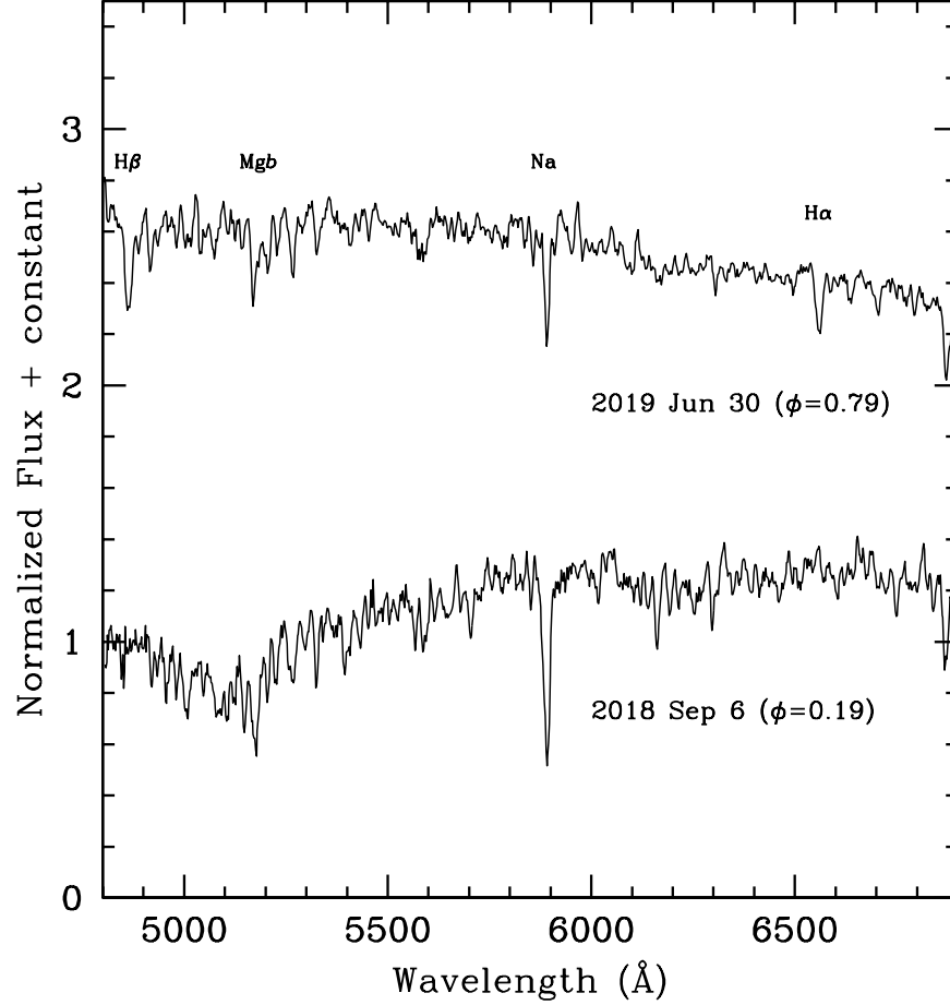
Figure 5.2: Optical spectra of 4FGL J2333.1–5527. Two of our SOAR spectra showing examples of the varying effective temperature of the companion. The dayside spectrum (top) is consistent with an early-G star, while the nightside spectrum (bottom) is markedly cooler, matching that of a mid-K dwarf. Our other low-resolution spectra typically lie somewhere between these extremes.
