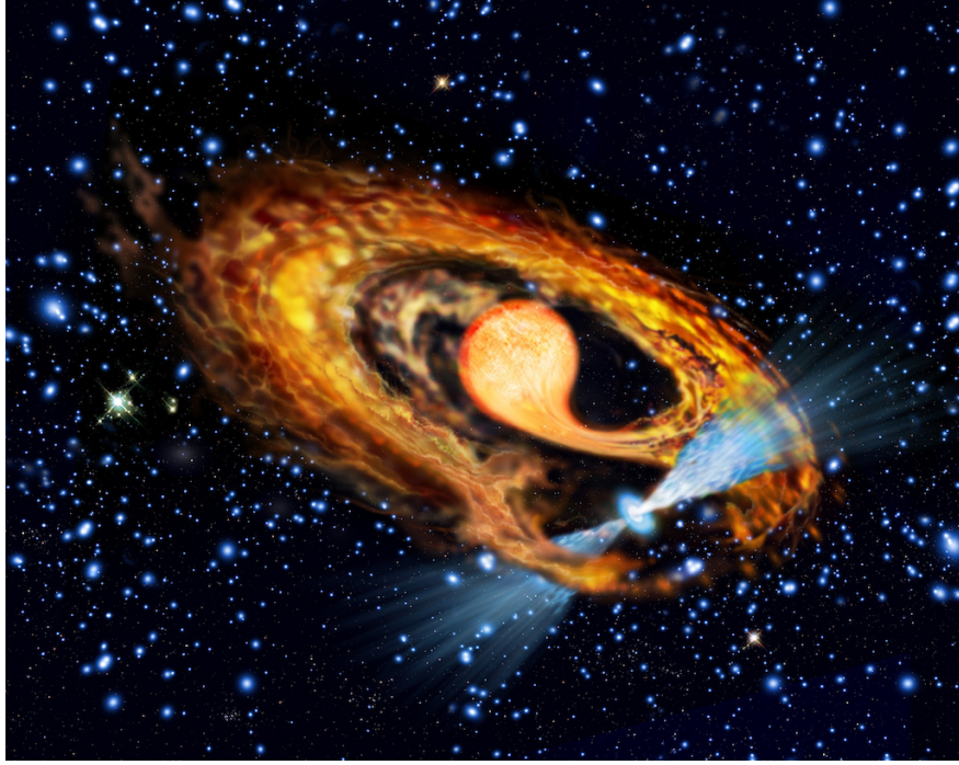
Figure 1.6: Artist rendition of an eclipsing spider MSP. The pulsar wind blows material off the non-degenerate companion star and prevents material from reaching the neutron star surface. This material may stay bound to the system, making it difficult to detect radio pulsations; Image credit: European Space Agency & Francesco Ferraro (Bologna Astronomical Observatory)
