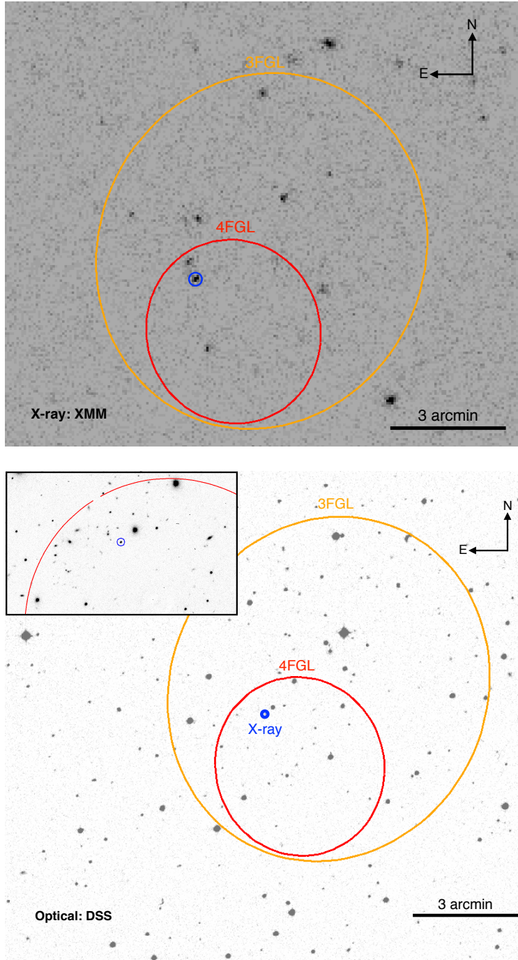
Figure 5.1: X-ray and optical finder images for 4FGL J2333.1–5527. Top: XMM-Newton /EPIC X-ray image of the field of 4FGL J2333.1–5527 with the 95% error regions from the 4FGL (red) and 3FGL (orange) catalogs overlaid. The subject of this work is marked with the blue circle. Bottom: Optical DSS image of the field with the location of the X-ray source marked in blue. The inset displays a zoomed-in view of one of our SOAR i' images showing the variable optical counterpart associated with the X-ray source.
