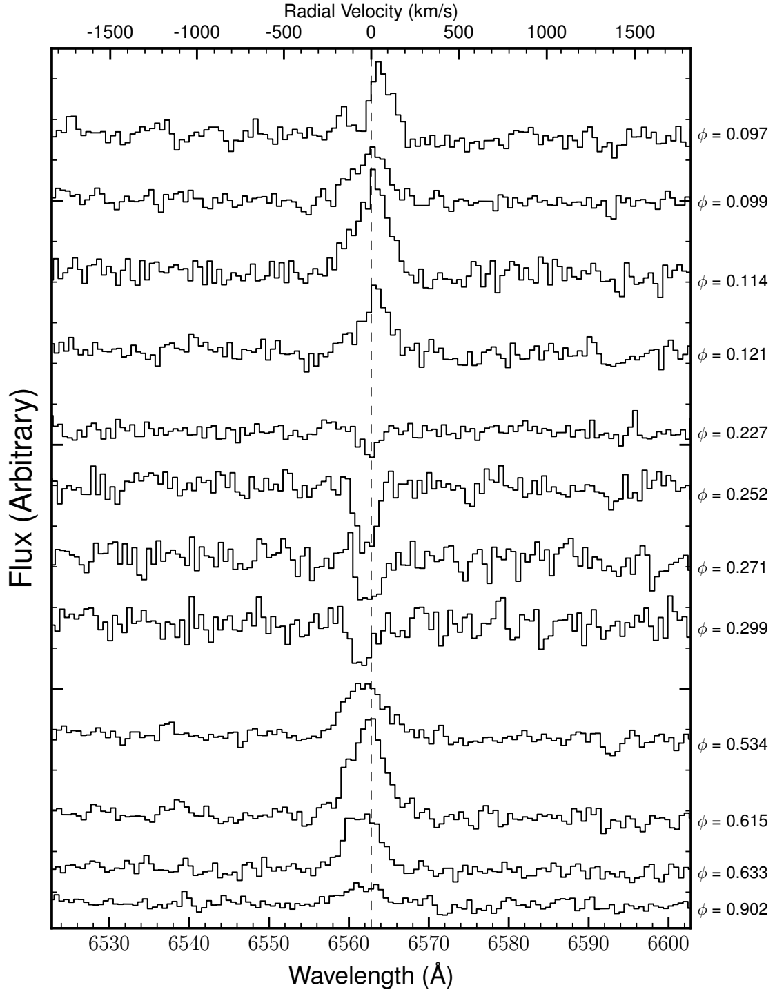
Figure 4.3: Phase-resolved optical spectra of PSR J1306-40 around the H \alpha region. Spectra have been corrected to the rest frame of the secondary (dashed line) and arbitrarily shifted in flux to display changes in the profile shape. The switch from emission to absorption near companion inferior conjunction ( \phi = 0.25 ) is apparent, likely due to an eclipse of the emission region.
