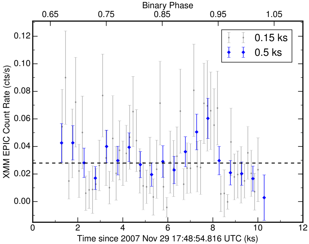
Figure 5.5: X-ray light curve of 4FGL J2333.1–5527. The XMM-Newton /EPIC light curve between 0.2–10 keV. The observation covers \sim 40\% of the binary orbit. Barycenter corrections have been applied to the photon arrival times and the data are grouped into 150s (black) and 500s (blue) bins. The weighted average of the 500s binned dataset is shown with a dashed line.
