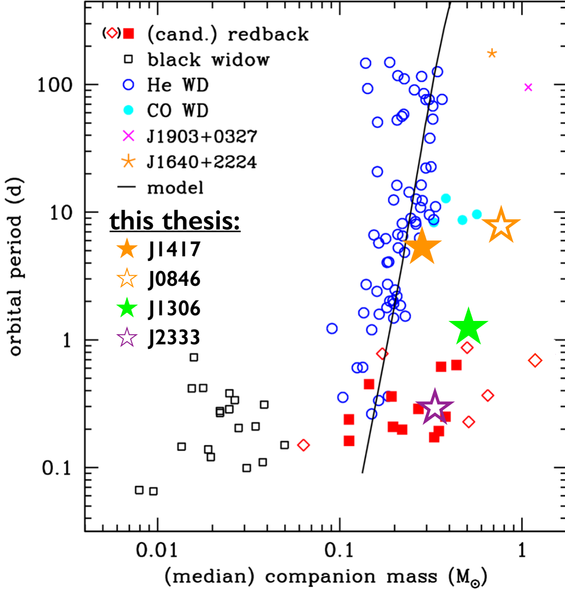
Figure 1.5: Orbital period versus companion mass for recycled field MSPs with known companion star types. Most MSPs have He white dwarfs (open blue circles) from the canonical binary evolution scenario, well-represented by models from Tauris & Savonije (1999). These models (black line) assume solar metallicity and an initial secondary mass of 1.0 M_{\odot} , and denote the endpoints of an ensemble of systems with varying initial period, not the evolution of a single binary. The few CO white dwarfs (filled cyan circles) likely had more massive secondaries and underwent close common-envelope evolution. The field redbacks (red squares) and black widows (open black squares) are visible at short orbital period, and it is clear that these systems will not have normal field MSPs as their progeny. Instead the likely progenitors to the canonical field MSPs are systems with red giant companions in relatively wide orbits, the aptly-named “huntmen” subclass (Section 1.4.4). The systems that are the subjects of this thesis (Chapters 2–5) are labeled with stars. Open red squares and stars refer to candidate systems for which radio pulsations have not yet been detected. Figure adapted from Strader et al. (2019).
