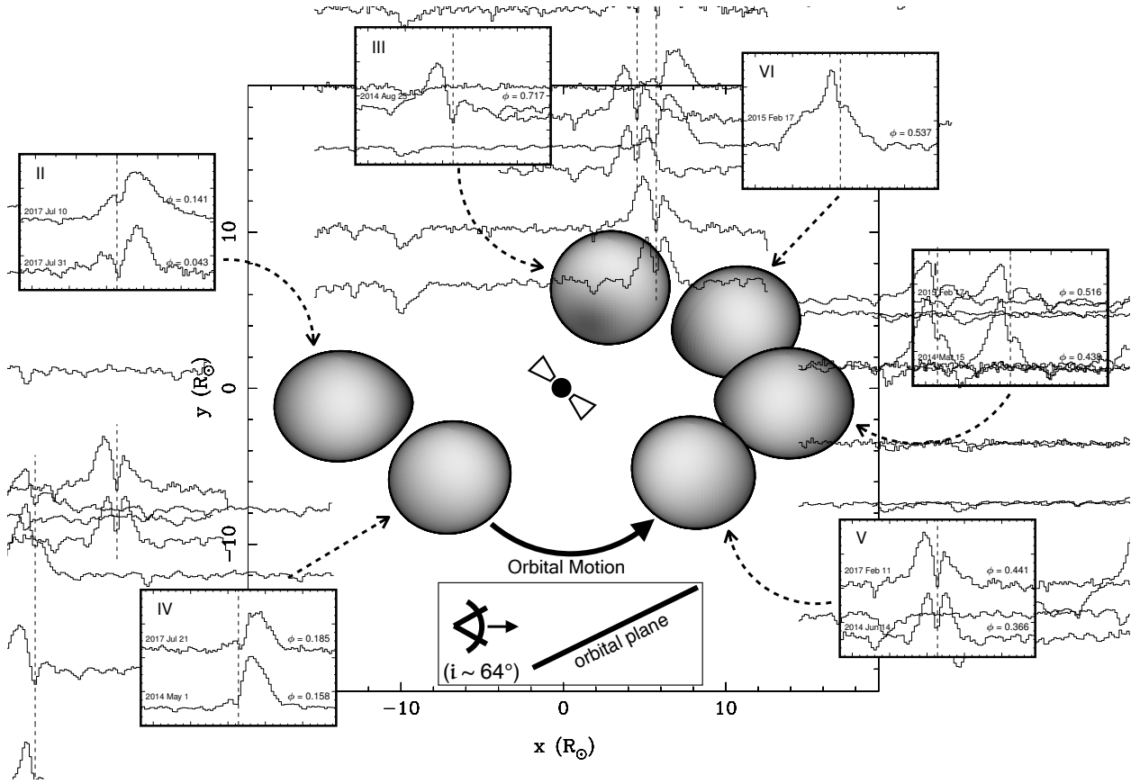
Figure 3.7: Orbital position of the secondary in 1FGL J1417.7–4407 corresponding to the varying H\alpha phenomenology. A schematic diagram of J1417 (as seen from Earth) showing the orbital position of the secondary corresponding to the range of H\alpha phenomenology we show in the panels of Figure 3.6.
