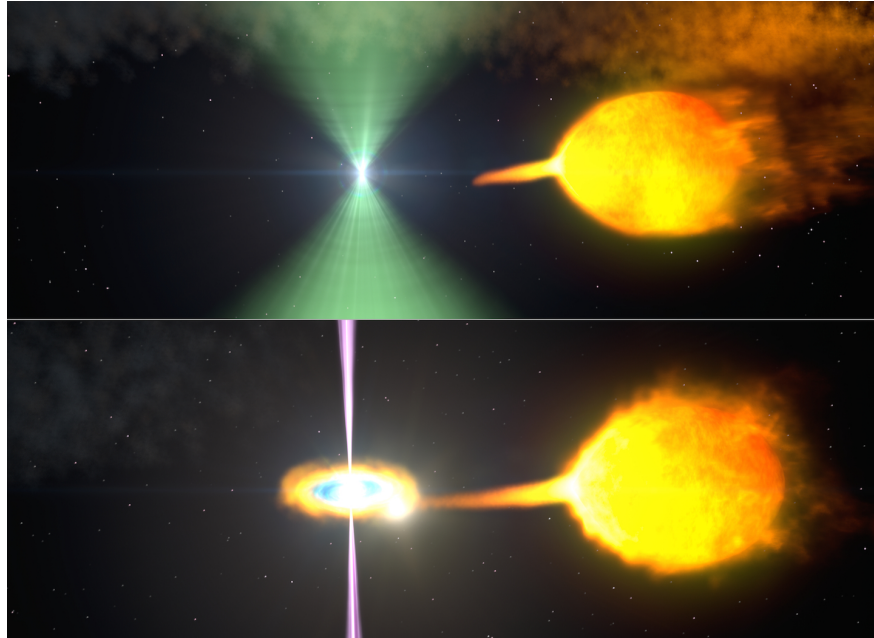
Figure 1.7: Artist’s renditions of the two main states of a transitional MSP , showing a model tMSP in the radio pulsar state (top) versus the accretion-powered disk state (bottom). In the pulsar state, the radio MSP (green) is observed, although it is typically eclipsed by ionized material blown off the companion. The optical emission is dominated by the tidally-distorted companion resulting in periodic variability (Section 1.5.3), and stellar absorption lines can be measured to track the secondary’s motion around the invisible MSP (Section 1.5.4.1). X-ray emission in this state is often modulated on the binary orbital period due to an intrabinary shock (Section 1.5.2). In the disk state, the pulsar wind can no longer hold off the mass inflow from the companion and an accretion disk forms around the MSP. The radio pulsar becomes undetectable, and the system becomes brighter in the optical/X-rays. The optical emission is dominated by contributions from the disk; the secondary’s absorption lines are often “filled-in” by disk emission and double-peaked Balmer emission lines, a hallmark of Doppler motion in the outer edges of an accretion disk, are observed in the optical spectra (Section 1.5.4.3). Occasionally, a flat-spectrum radio jet (purple) is observed in this state as material is ejected by the rotating pulsar magnetosphere. Figure credit: NASA’s Goddard Space Flight Center
