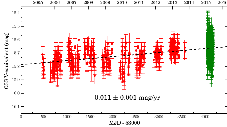
Figure 2.7: Long-term optical light curve of 2FGL J0846.0+2820. Long-term optical light curve showing a monotonic increase in the system brightness over the past decade. The Catalina data are shown in red and our recent PROMPT V -band data are in green (far-right on figure). The dashed line and rate of brightening are the result of a linear fit to the Catalina data only. A small zeropoint offset has been applied to the PROMPT data as described in § 2.4.5
