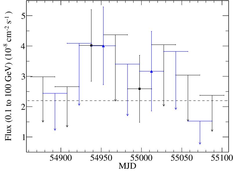
Figure 2.5: \gamma -ray light curve of 2FGL J0846.0+2820 near the time the flux dropped. The LAT light curve for the most significant 180-day interval ( \pm 60 days) in shorter 30-day time bins (black points). The data were shifted by 15 days (blue points) to find the last significant time bin. The upper limits are indicated when TS < 4 with fewer than four predicted photons. The dashed line marks the best fit average flux.
