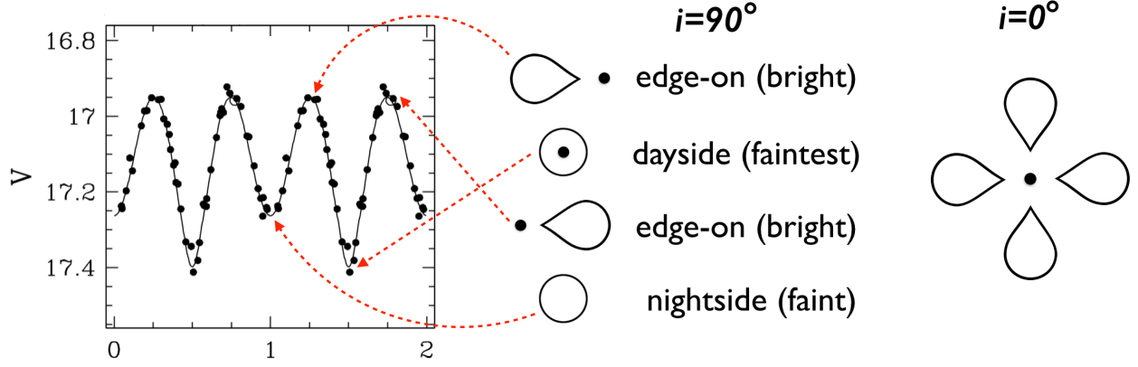
Figure 1.10: Diagram of ellipsoidal variations. Schematic demonstration of determining the binary inclination with ellipsoidal variations of a Roche lobe filling secondary (teardrop) and a compact object (small black circle). There are two equal maxima per orbit when the tidally distorted secondary has the largest projected surface area, and two unequal minima per orbit. The “dayside” of the secondary is nominally predicted to have the faintest optical flux due to gravity darkening (a lower effective temperature), but this effect can be reduced or even reversed if this side is also irradiated by the compact object (see text). The amplitude of the variations are largest when the system is edge-on ( i = 90^\circ ) but are undetectable if face-on ( i = 0^\circ ), with intermediate inclinations producing intermediate amplitude variations. Figure adapted from Greene et al. (2001).
