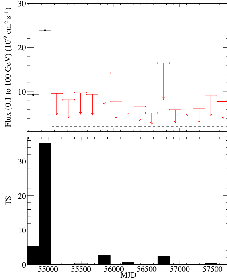
Figure 2.3: \gamma -ray light curve of 2FGL J0846.0+2820. Fermi -LAT 0.1–100 GeV \gamma -ray light curve (Top) and corresponding TS values (Bottom) in \sim 0.5 year bins. In the light curve, down arrows indicate 95% confidence upper limits on the fluxes, and the upper limit derived from the data after the first two bins is indicated with the horizontal dashed line.
