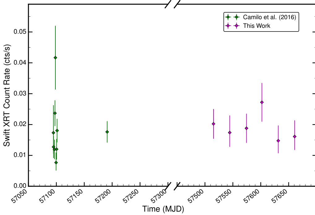
Figure 3.3: Long-term Swift X-ray light curve of 1FGL J1417.7–4407. The 0.3–10 keV Swift XRT count rates, extracted from 15 observations between 2015 Mar and 2016 Sept.
