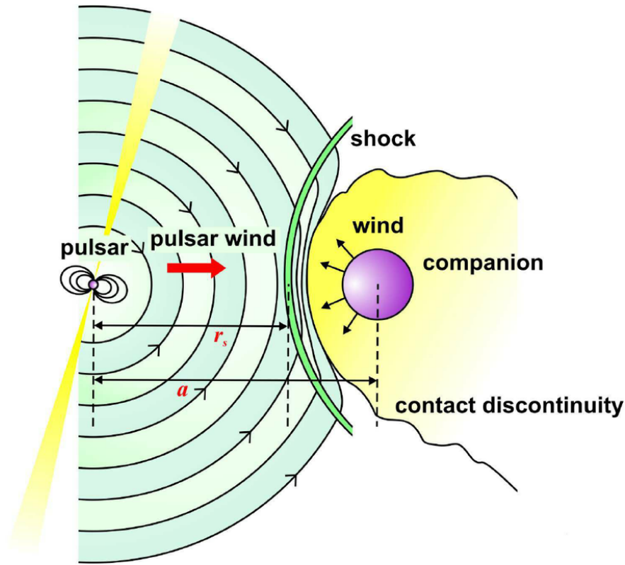
Figure 1.8: Diagram of an intrabinary shock. A cartoon showing the formation of an intrabinary shock, formed at the collision interface between the pulsar and companion winds. The relative strengths of the winds determine whether the shock wraps around the pulsar or the companion. Orbitally modulated X-ray emission is often observed due to the presence of the shock (see text and Figure 1.9). Figure from Venter et al. (2015).
