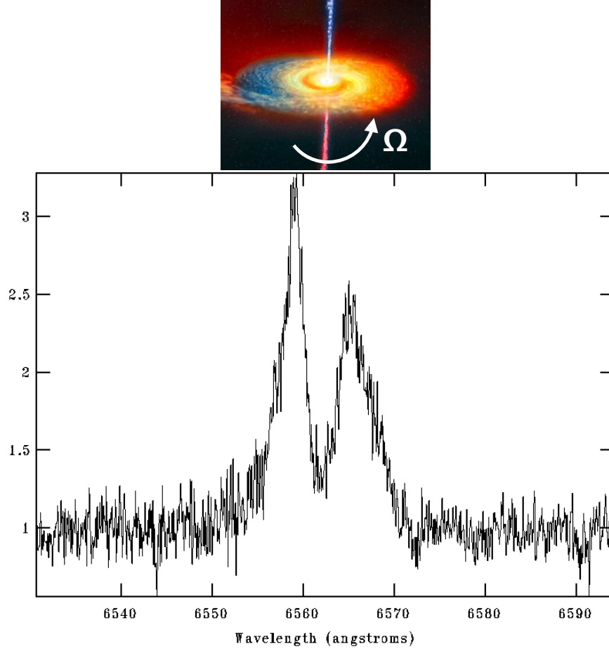
Figure 1.11: Example double-peaked H\alpha emission line due to an accretion disk. A high-resolution spectrum showing a double-peaked H\alpha emission line coming from an accretion disk. Due to the Doppler effect, the redward peak comes from the receding half of the disk, while the blue peak comes from the approaching side. This double-peaked Balmer emission is generally interpreted as arising from an accretion disk. However, an intrabinary shock, and material blown from a companion star and being heated by a pulsar wind, could provide an additional natural physical explanation for complex H\alpha profiles, as shown in Chapter 3 and Chapter 4. Cartoon credit: ESA; Spectrum taken with the PST1 telescope (Baranowski et al., 2009).
