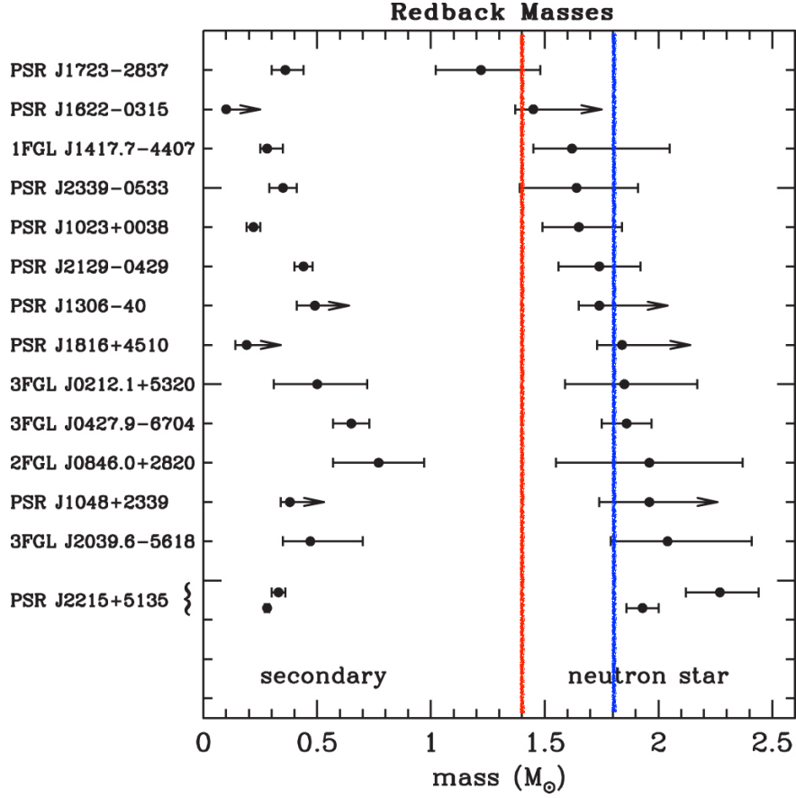
Figure 6.1: Component masses for the redback and huntsmen systems that have well-constrained mass estimates for the neutron star , sorted by neutron star mass. These systems have direct measurements (or meaningful lower limits) of the neutron star mass via a combination of optical spectroscopy, optical photometry, and in some cases the projected motion of the pulsar. Most non-recycled neutron stars with dynamically measured masses are near \sim 1.4 M_\odot (red line), however there is increasing evidence for a broad secondary peak in the neutron star mass distribution that peaks at \sim 1.8 M_\odot (blue line, Özel & Freire, 2016). Nearly all redbacks/huntsmen have neutron star masses consistent with this more massive peak, and therefore, discovering new systems will provide promising opportunities to find the most massive neutron stars. Figure adapted from Strader et al. (2019).
