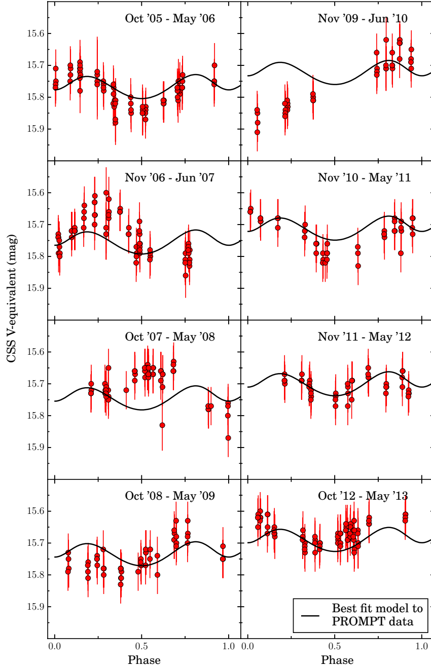
Figure 2.8: Long-term optical light curve of 2FGL J0846.0+2820 split into separate epochs. The long-term CSS data split into eight separate epochs (first 4 on left, last 4 on right) and phased on the spectroscopic period. The best fit ELC model (with a disk) from § 2.4.3 is shown in black, adjusted for the linear trend seen in Figure 2.7. The shape of the light curve does not appear consistent with typical ellipsoidal variations across all epochs.
