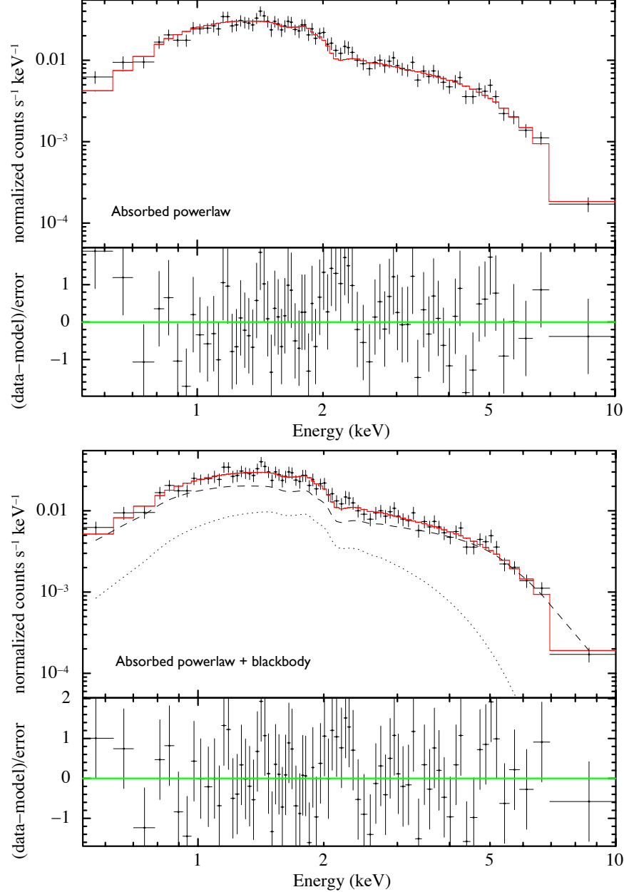
Figure 3.2: Chandra X-ray spectra of 1FGL J1417.7-4407 with best fit models in red. In the upper figure, the data is fit with a pure absorbed power-law model, while the lower figure shows an absorbed power-law (dashed) plus the addition of a blackbody component (dotted). Fit residuals are shown in the bottom panels.
