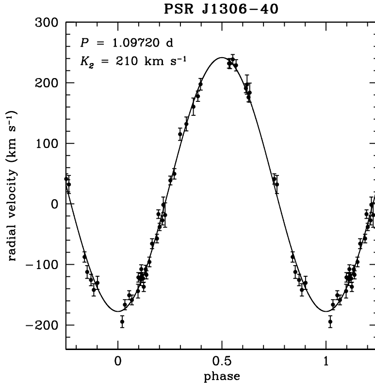
Figure 4.1: Radial velocity curve of PSR J1306-40. Circular Keplerian fit to the SOAR/Goodman barycentric radial velocities of PSR J1306-40 listed in Table 4.1.
