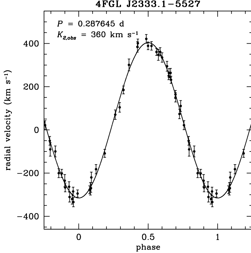
Figure 5.3: Radial velocity curve of 4FGL J2333.1–5527. Circular Keplerian fit to the observed radial velocities. As discussed in the text, the fit to the “corrected” velocities has a lower semi-amplitude but is otherwise extremely similar.
