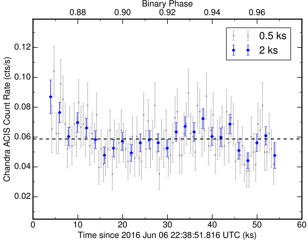
Figure 3.1: Chandra X-ray light curve of 1FGL J1417.7–4407. The Chandra ACIS light curve between 0.5–7 keV. The ~50 ks exposure covers ~11% of the binary orbit. Photon arrival times have been barycenter corrected and are grouped into 500s (black) and 2ks (blue) bins. The black dashed line marks the weighted average of the 2ks dataset.
