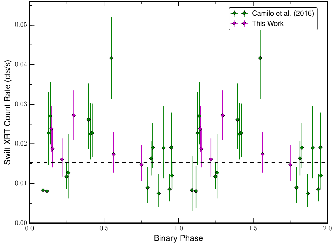
Figure 3.4: Swift X-ray light curve of 1FGL J1417.7–4407 folded on the binary period. Snapshots from the 15 Swift XRT observations in Figure 3.3 folded on the orbital period of the binary. The times spanned by each exposure are smaller than the symbol sizes. The dashed line shows the weighted average of all snapshots. Two orbital cycles are shown for clarity.
