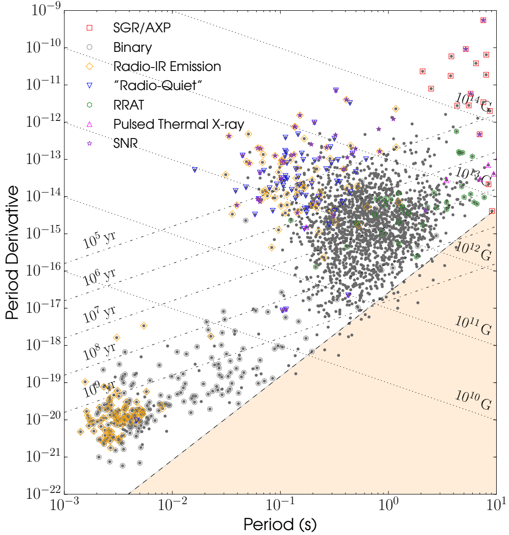
Figure 1.2: The P - \dot{P} diagram , showing the measured spin period and period derivative for all 2811 known pulsars from the ATNF pulsar catalogue 3 . Lines of constant surface magnetic field strength and characteristic pulsar age (see text for definitions) are shown. The “pulsar graveyard,” (see text) is represented by the shaded region in the lower right. This diagram is generally used as a convenient way to classify the different sub-populations of pulsars and track their basic evolution. The dark grey circles highlight the bulk of the pulsar population, with spin periods of \sim 0.5 s, ages from \sim 10^5 - 10^8 years, and moderate ( 10^{11} - 10^{13} G) magnetic fields. The top-right of the diagram hosts a population of young neutron stars with extremely strong magnetic fields, known as “magnetars,” or sometimes referred to as soft gamma-ray repeaters (SGRs) or anomalous X-ray pulsars (AXPs). The lower-left part of the diagram shows the objects that are the subject of this thesis. These are the rapidly-rotating millisecond pulsars, which attained their fast spin periods by being spun-up via accretion from a binary companion. Noteworthy features (e.g., presence of a binary companion) and associations (e.g., located in a supernova remnant (SNR)) for some of the pulsars are noted by the legend. Figure produced using the Python package psrqpy (Pitkin, 2018).
