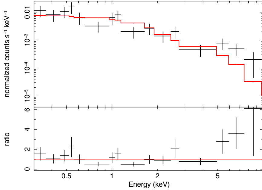
Figure 5.4: X-ray spectrum of 4FGL J2333.1–5527. XMM-Newton /EPIC MOS+pn spectrum of J2333, with model and model/data ratios. Due to the low number of source counts, the unbinned data were fitted with W-statistics and later rebinned to a minimum significance of 2.2\sigma for visualization purposes only. The model (red) shows our best-fit absorbed power-law model (TBabs*powerlaw) with photon index \Gamma = 1.6 \pm 0.3 .
