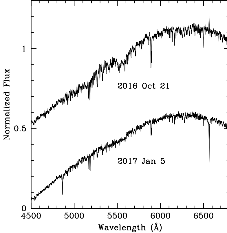
Figure 2.1: Optical spectra of 2FGL J0846.0+2820. Two of our OSMOS spectra showing the most extreme examples of varying effective temperature and H\alpha emission ( \lambda_{\text{rest}} = 6562.8 \text{ \AA} ). Our other low-resolution spectra lie somewhere between these extremes.
