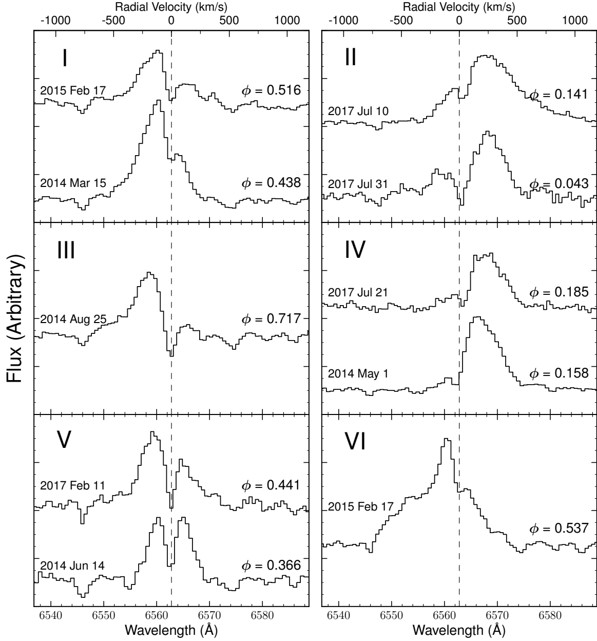
Figure 3.6: Phase-resolved optical spectra of 1FGL J1417.7–4407 near the H \alpha region. Example optical spectra of J1417 around the H \alpha region. All spectra have been shifted to the rest frame of the secondary (dashed line). Each panel shows spectra that are representative of nearly all the spectra obtained at that orbital phase.
