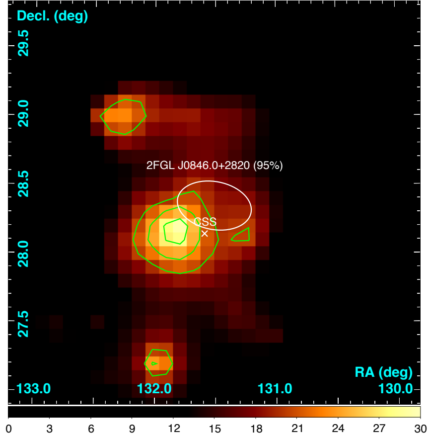
Figure 2.4: Map of \gamma -ray emission near the location of 2FGL J0846.0+2820. The LAT TS map centered on 2FGL J0846.0+2820 in J2000.0 coordinates (bottom bar indicates TS values). The green contours are, from inside out, 68, 95, 99% confidence on the localization, newly determined from the Pass 8 data analysis. The 2FGL 95% confidence ellipse (white ellipse) is shown as well as the optical CSS position (white cross).
