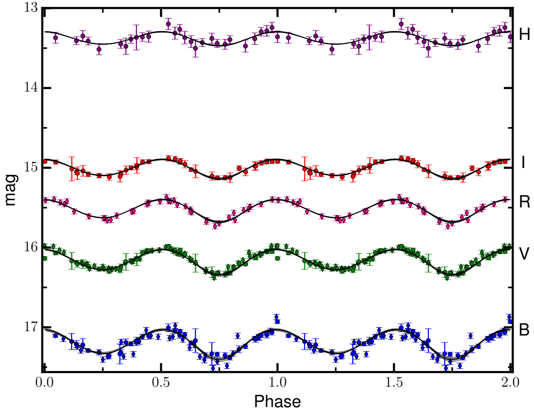
Figure 3.5: Optical/near-IR light curves of 1FGL J1417.7–4407. PROMPT (diamonds) and SMARTS (circles) optical/near-IR photometry with best fit ELC models. Two orbital phases are shown for clarity. The black lines show 8 random samples from the posterior marginalized over all the free parameters in the SMARTS+PROMPT “No Disk” MCMC run (Table 3.6, top panel, column 1).
