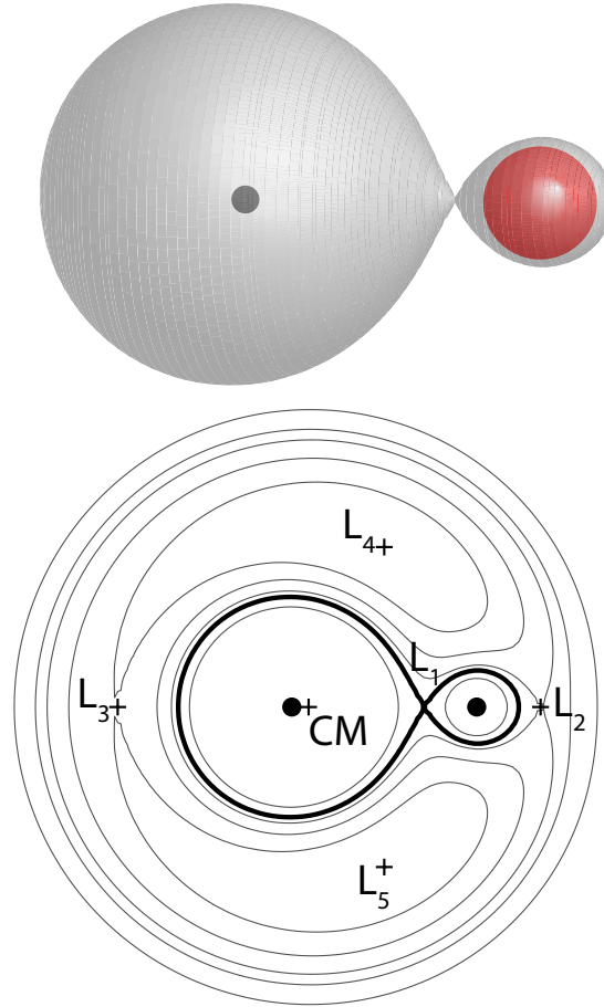
Figure 1.3: Schematic diagram demonstrating the concept of a Roche lobe in a binary system. Top: A neutron star (dark grey circle, size not to scale) and a companion star (red circle) are in a binary system. The light grey tear-drop-shaped regions denote the Roche lobes of the two stars, within which material is gravitational bound to each respective object. If the envelope of the companion expands to fill its Roche lobe, material can stream towards the neutron star. Bottom: Two stars orbit around a common center of mass (CM), which lies closer to the more massive object (left black dot). Thin grey lines denote surfaces of equal gravitational potential. Thick black lines are the Roche lobes of the two respective stars. If the companion (right black dot) fills its Roche lobe, material streams towards the massive object through inner Lagrange point L_1 . Figure credit: Ed Brown; License: Creative Commons Attribution–NonCommercial–ShareAlike 4.0 International (CC BY-NC-SA 4.0)
