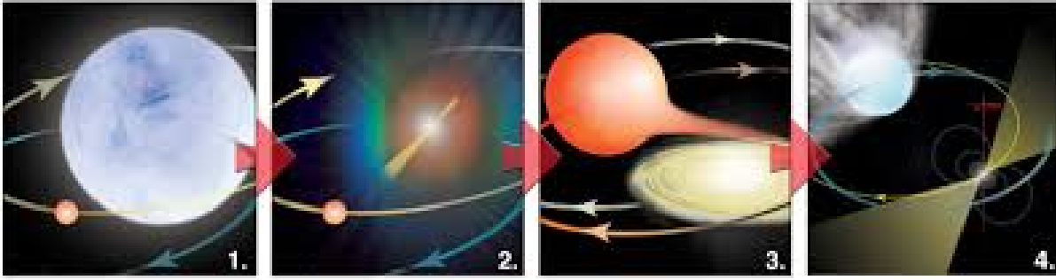
Figure 1.4: The key phases of the MSP recycling process. In the first panel, a massive star is being orbited by a Sun-like companion. Eventually the massive star will explode in a supernova, leaving behind a rotating neutron star visible as a radio pulsar (panel 2). The spin frequency of the pulsar will gradually slow down over time as it loses rotational kinetic energy. In the third panel, the lower-mass star has undergone normal stellar evolution and expands into its red giant phase. At this point material will fall down towards the pulsar forming an accretion disk, making the system visible as a low-mass X-ray binary, and transferring matter and angular momentum to the neutron star, spinning it up to rapid spin periods and likely increasing its mass. Finally, accretion eventually ends and the spun-up neutron star will become visible again, now as a millisecond radio pulsar (panel 4). The strong, relativistic pulsar wind impinges on the companion, ablating material from its surface, causing radio eclipses for substantial fractions of the orbit (see Section 1.4.2). Recent observations have shown that some systems can switch back and forth between the phases shown in panels 3 and 4 (see Section 1.4.3). Figure credit: Bill Saxton, NRAO
