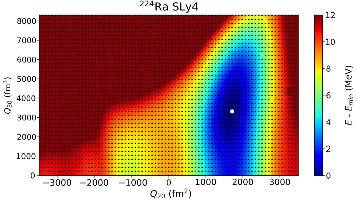
Figure 3.1: Potential energy surface of ^{224}\text{Ra} calculated using Skyrme energy density functional SLy4. The white circle marks the lowest binding energy, which serves as the baseline energy value.
