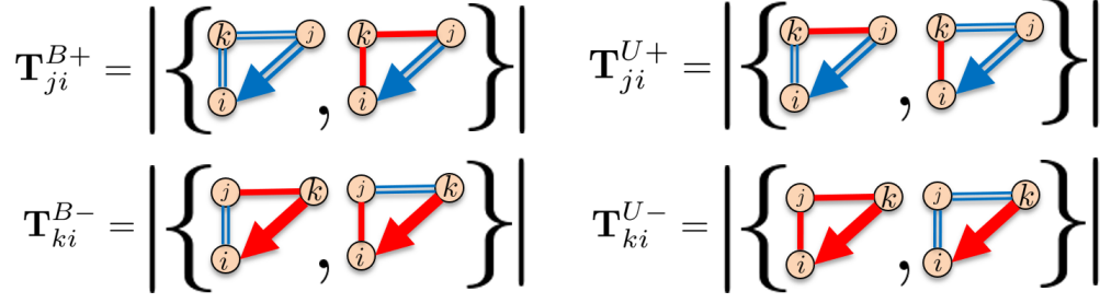
Figure 3.3: An illustration of how we calculate the matrices \mathbf{T}^{B+} , \mathbf{T}^{U+} , \mathbf{T}^{B-} , and \mathbf{T}^{U-} .
