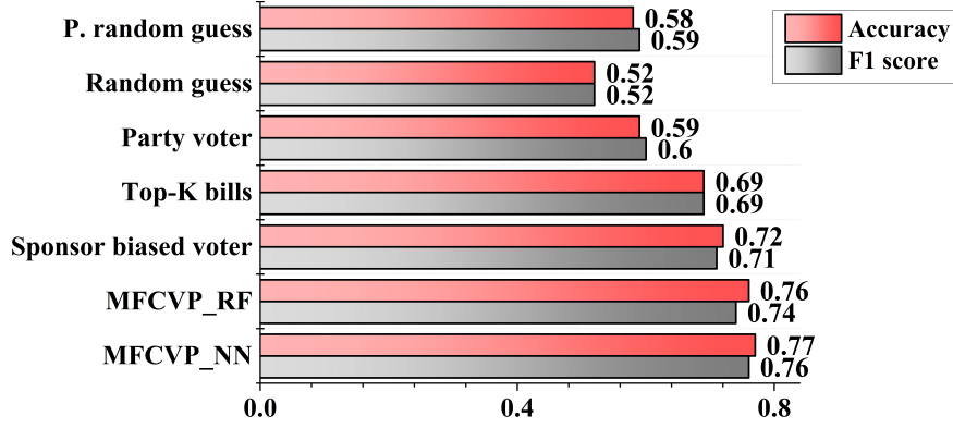
Figure 6.7: Performance evaluation of MFCVP predicting individual representative votes.
