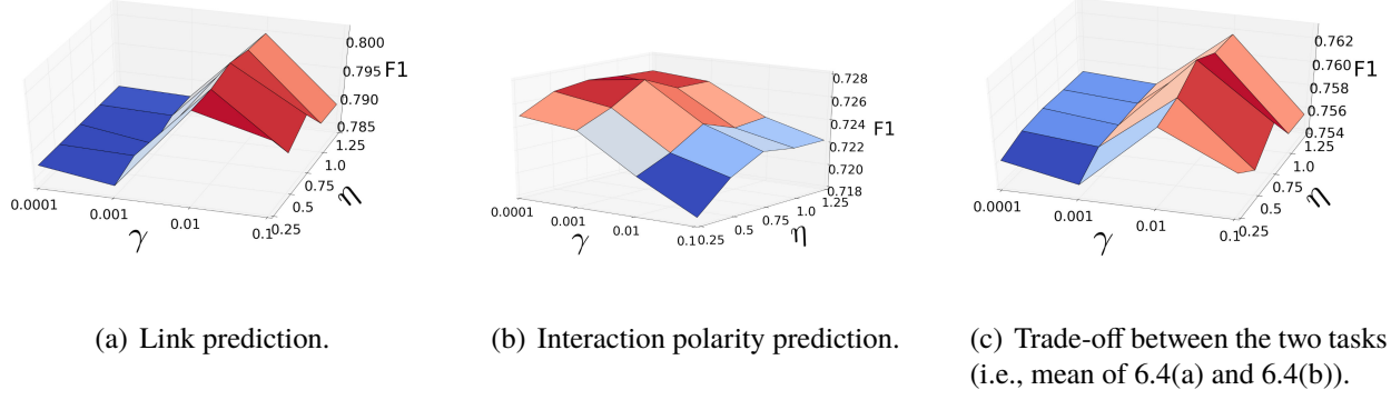
Figure 6.4: Performance variations of LIP on the 90% data sparsity experiment w.r.t. \eta and \gamma .
