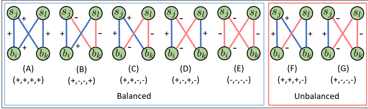
Figure 4.3: Undirected signed butterfly isomorphism classes.
