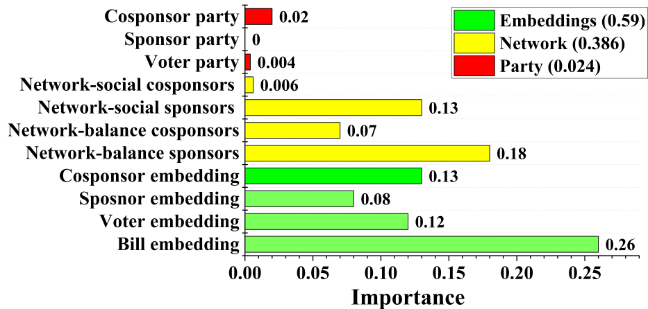
Figure 6.9: Feature analysis using the feature importance values from MFCVP_RF.
