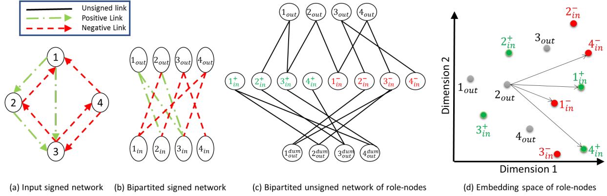
Figure 5.5: Transformation process of the input signed network to the network of role-node.
