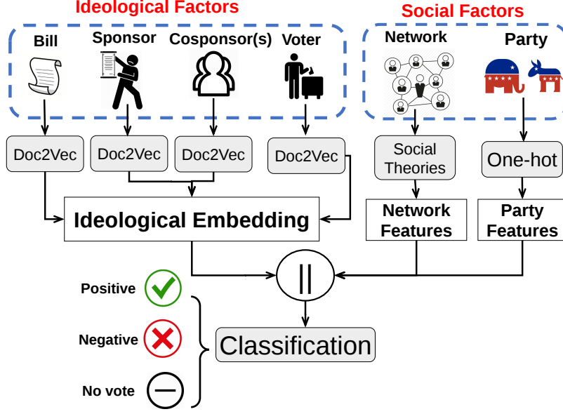
Figure 6.5: The proposed Multi-Factor Congressional Vote Prediction (MFCVP) framework.
