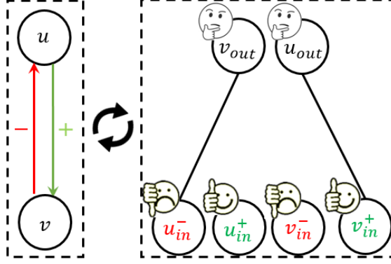
Figure 5.4: Transformation of a signed network with two nodes to an unsigned bipartite network of role-nodes.
