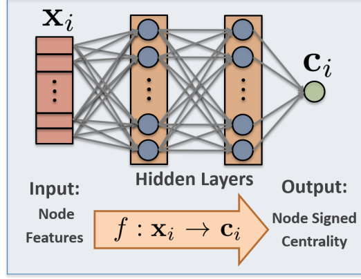
Figure 3.2: An illustration of our deep neural network for learning signed centrality scores.
