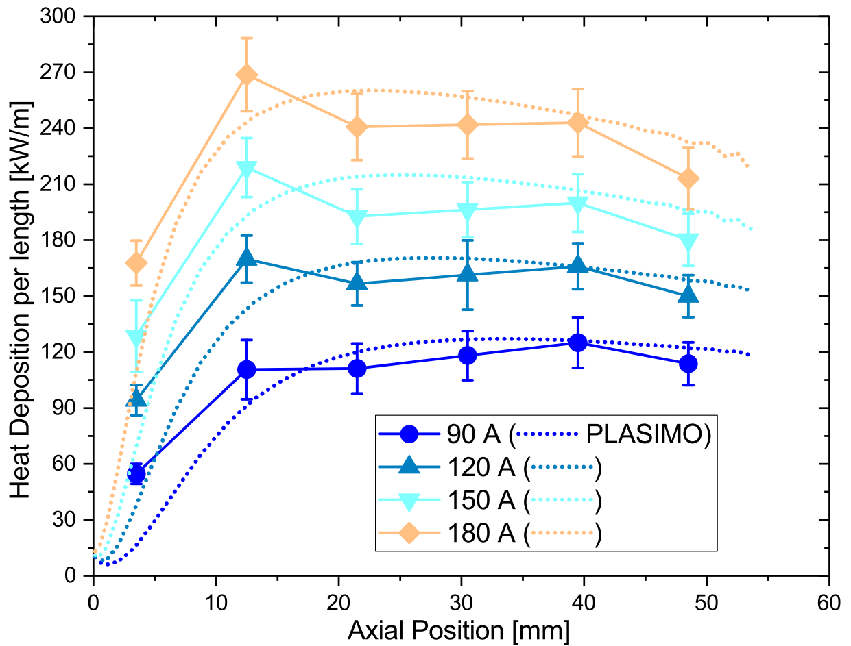
Figure 4.21: Similar to Fig. 4.20 but for helium. Power removed by water coolant for each PW plate in a 6x6mm configuration in helium arc. Each data set is taken at a GCS pressure of 200 torr.
