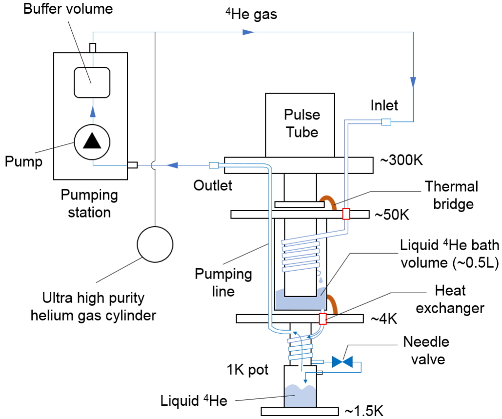
Figure 4.2: Schematic showing operation of the closed-cycle 1K cryostat. The 1K cryostat is precooled by a 4K pulse tube cryocooler (Cryomech PT410-RM) providing 1.0 W cooling power at T = 4.2 K. In the 1K circulation loop (blue color), the inlet ^4\text{He} gas at the pressure of \sim 1 atm is precooled by a heat exchanger on the 50K stage and then condenses at the 4K stage. The condensed helium flows through a counter-flow heat exchanger wrapped around the tube below the 4K stage to be cooled \sim 2 K. It then passes through a needle-valve into the 1K pot. To produce evaporation, the 1K pot is pumped by a dry vacuum pump through a pumping line. A buffer volume installed at the pump discharge stabilizes the pressure. If additional helium gas needs to be added, a standard helium gas cylinder is connected to the discharge side of the pump. The base temperature of the 1K system strongly depends on a flow through the needle valve and the pumping rate as well as any additional heat load from measurement wires and the helium fill line inside the fridge.
