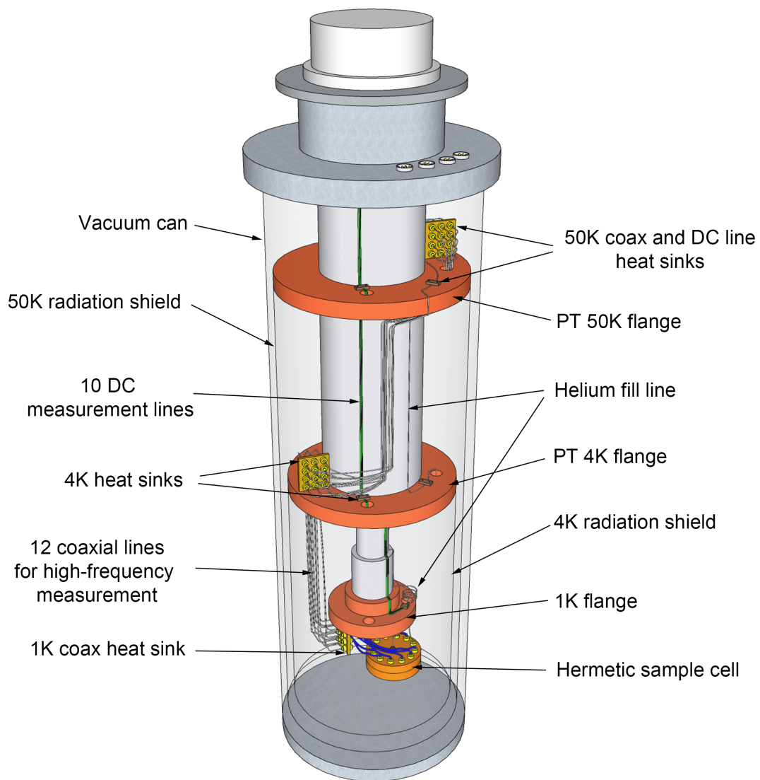
Figure 4.3: A simplified illustration of a closed cycle 1K refrigerator in which a helium fill line, wires, and a sample cell are shown in detail.
