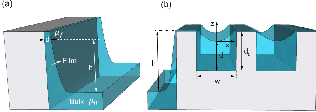
Figure 2.16: Helium film formation: (a) Van der Waals film on a vertical wall of the substrate. \mu_0 and \mu_f are the chemical potential of the bulk helium and the thin film of helium located at height h above the bulk level. (b) Helium film formation inside the channel of the micro-channel array by capillary force. Here w , d_0 , d , and h represent channel with, channel depth, helium film thickness in the channel, and the distance between the channel top and the bulk helium level in the reservoir.
