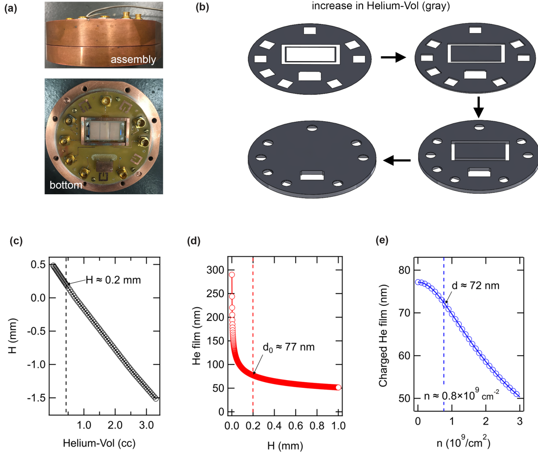
Figure B.1: The experimental sample cell and helium film thickness determination. (a) Photograph of the copper cell used for the SAW-based measurements of electrons on helium. The bottom portion of the cell contains a LiNbO 3 device (semi-transparent white) mounted on a printed circuit board (b) 3D CAD modeling of the liquid helium volume inside the experimental cell during filling with helium. (c) Calculation of H , the distance between the piezo-substrate top and the liquid helium level in the cell reservoir volume from the 3D CAD modeling of the open cell volume. The calculated value of H in the experiments is 0.2 mm for a helium vol. = 0.44 cc (vertical dashed black line). (d) Helium film thickness versus H before charging the film (see equation B.1). For an uncharged helium film d_0 \approx 77 nm (vertical dashed red line). (e) Charged helium film thickness versus electron density from equation B.2. The charged helium film thickness is calculated to be d \approx 72 nm for an electron density of n \approx 0.8 \times 10^9 \text{ cm}^{-2} (vertical dashed blue line).
