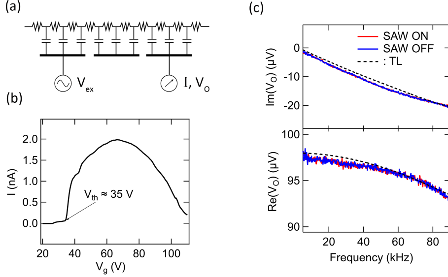
Figure A.2: (a) Transmission line (TL) circuit modeling of electrons on helium (b) Current of electrons on a helium film as a function of V_g in the low-frequency regime. The current was induced by applying a 0.1 mV, 60 kHz excitation V_{ex} and detected using standard lock-in techniques. The source and drain voltage were fixed at 60V. (c) Output voltage V_o as a function of the frequency of V_{ex} . The output voltage V_o corresponds to the voltage drop at the internal impedance of the signal detector (Lock-in amplifier) due to current flow in 2D electrons floating helium film. The blue and red solid traces represent experimental values with and without SAW excitation while the dashed trace is the theoretical curve. The frequency response is independent of SAW excitation, which implies that the low frequency transport is not affected by the SAW. For these measurements, all three electrodes were biased with 60 V.
