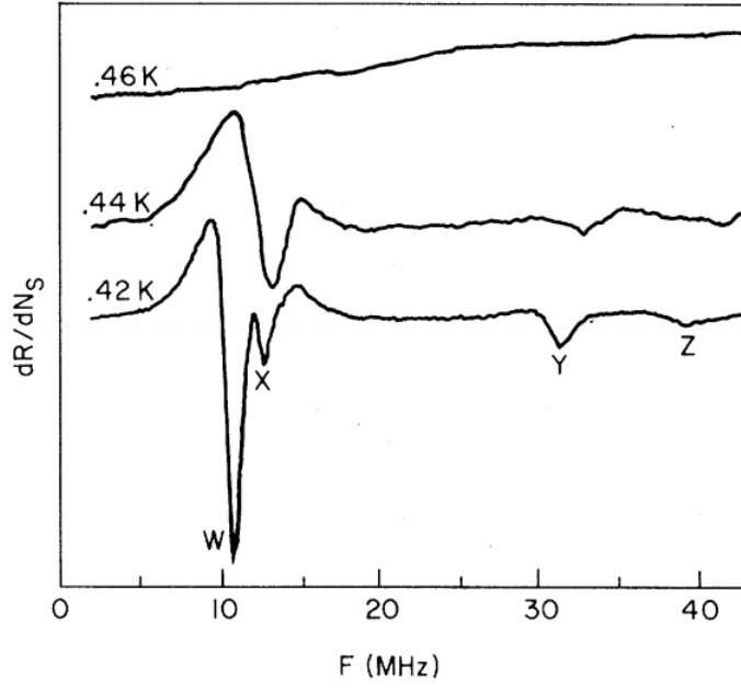
Figure 2.10: Coupled plasmon-ripplon resonances. The resonance only appear below 0.457 K where the sheet of electrons has crystallized into a triangular lattice (from Ref. [5]). dR/dN_s and F denote the derivative of the impedance of the electron layer with respect to the electron density and the frequency of the RF signal applied to the underlying electrode used to generate horizontal electron motion. A detailed description of a measurement setup is presented in the text.
