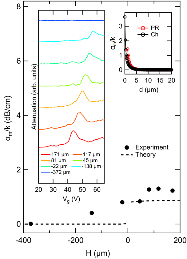
Figure 7.6: SAW attenuation versus helium level in the cell. Liquid helium was slowly and incrementally added to the charged helium film by supplying helium gas into the cell at T \cong 1.55 K. This film thickening raised the 2D electron layer away from the piezoelectric surface (GaAs) and reduced the piezoelectric coupling. The black closed circles and dashed line show the measured values and the calculation of the maximum attenuation \alpha_m at different H . Here H < 0 means the helium level is higher than the GaAs surface. The left inset shows the measurements of the attenuation versus V_g at various H while the right inset shows the calculation of maximum attenuation \alpha_m as a function of the distance d from the 2DES to the piezoelectric surface. Note that d is equivalent to |H| for bulk region ( H < 0 ).
