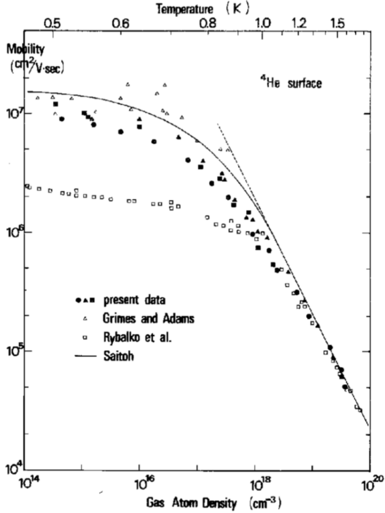
Figure 2.12: Mobility of electrons on helium versus the temperature and ^4\text{He} vapor density. Experimental data from Grimes and Adams [7], Rybalko et al. [8], and Iye [9] are shown together with a theoretical analysis from Saitoh [10]. The dashed line is the mobility considering vapor atom scattering alone. Figure taken from Ref. [9].
