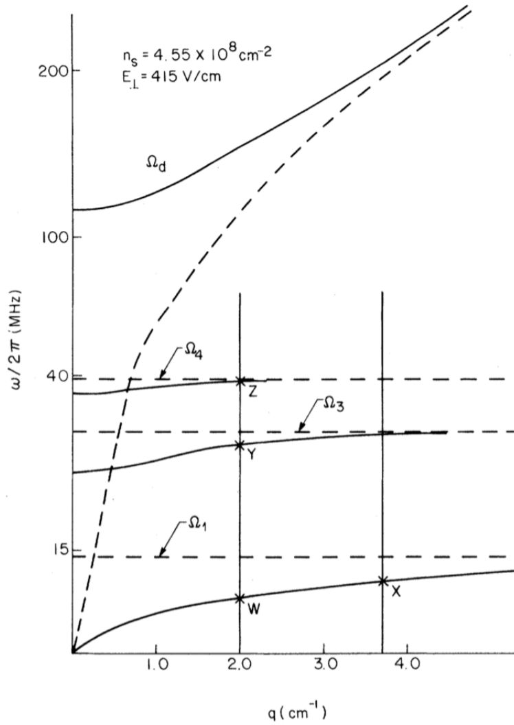
Figure 2.11: Dispersion relation of the longitudinal phonon-ripplon coupled modes (solid curves). The dashed curve is the bare longitudinal phonon spectrum of the electron crystal and the horizontal dashed lines represent the bare ripplon resonance frequencies when ignoring the phonon-ripplon coupling. The vertical lines are the wave vectors excited in the experiment. The resonances are labeled as in Ref. [5]. Figure taken from Ref. [6].
