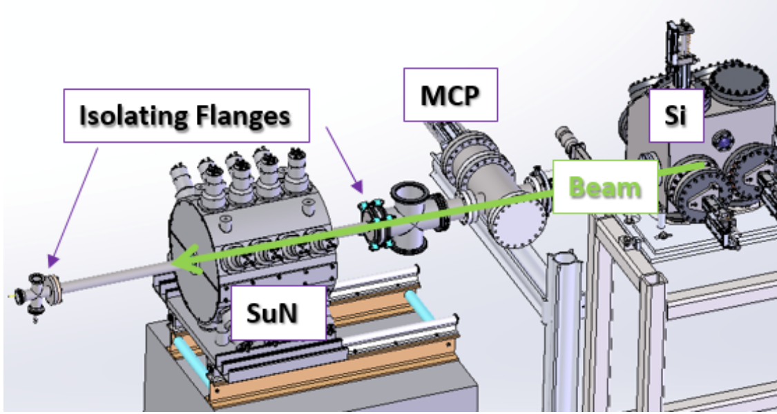
Figure 3.1: A close up of the experimental setup. The beam went from right to left following the green arrow. The positions of the Si and MCP detectors are shown. The SuNSCREEN detector is not pictured here but was sitting above SuN and the gas target was at the center of the SuN detector.
