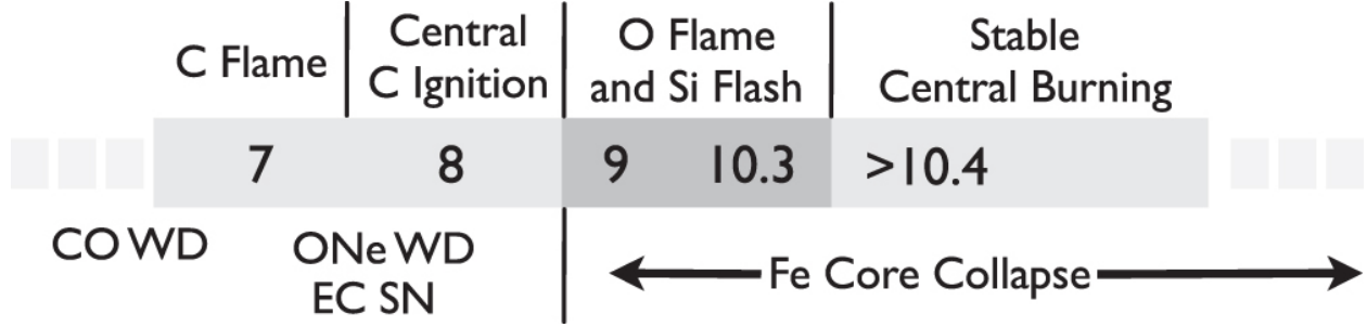
Figure 1.2: Evolutionary fates for a sample of stellar models in the mass range of 7-11 M_{\odot} . For this particular set of models, stars below 7 M_{\odot} form CO WDs, stars from 7-8 M_{\odot} ignite C off-center whereas from 8-9 M_{\odot} it ignites centrally. For models in the mass range 7-9 M_{\odot} a degenerate O-Ne-Mg core is produced that cools to a WD if the envelope is lost or results in a ECSNe if envelope remains. Stars above 9 M_{\odot} ignite Si either off-center (up to \approx 10.3 M_{\odot} ) or centrally (above 10.3 M_{\odot} ) to end in iron core-collapse. Figure from Woosley & Heger (2015).
