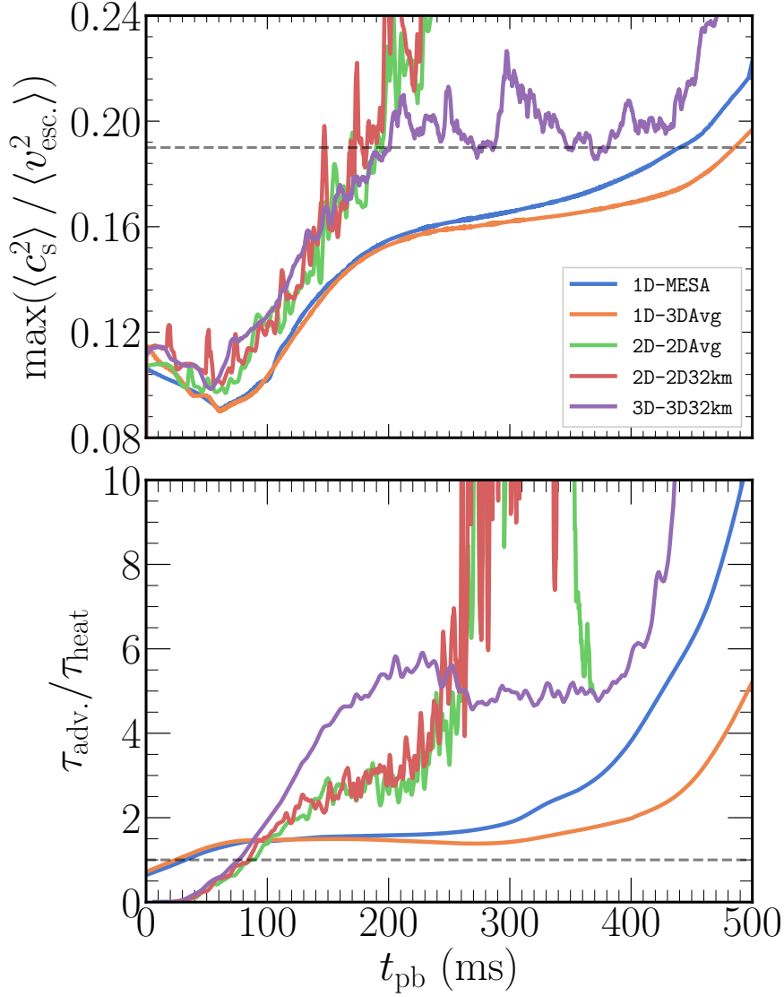
Figure 5.4: The antesononic condition, ratio of \langle c_s^2 \rangle / \langle v_{esc.}^2 \rangle (top) and the ratio of the advective and heating timescales for all five CCSN explosion simulations. In the top panel the explosion threshold for an isothermal accretion flow ( \approx 0.19 ) is denoted by a dashed horizontal line. In the bottom panel, a value of unit is denoted by a dashed horizontal line.
