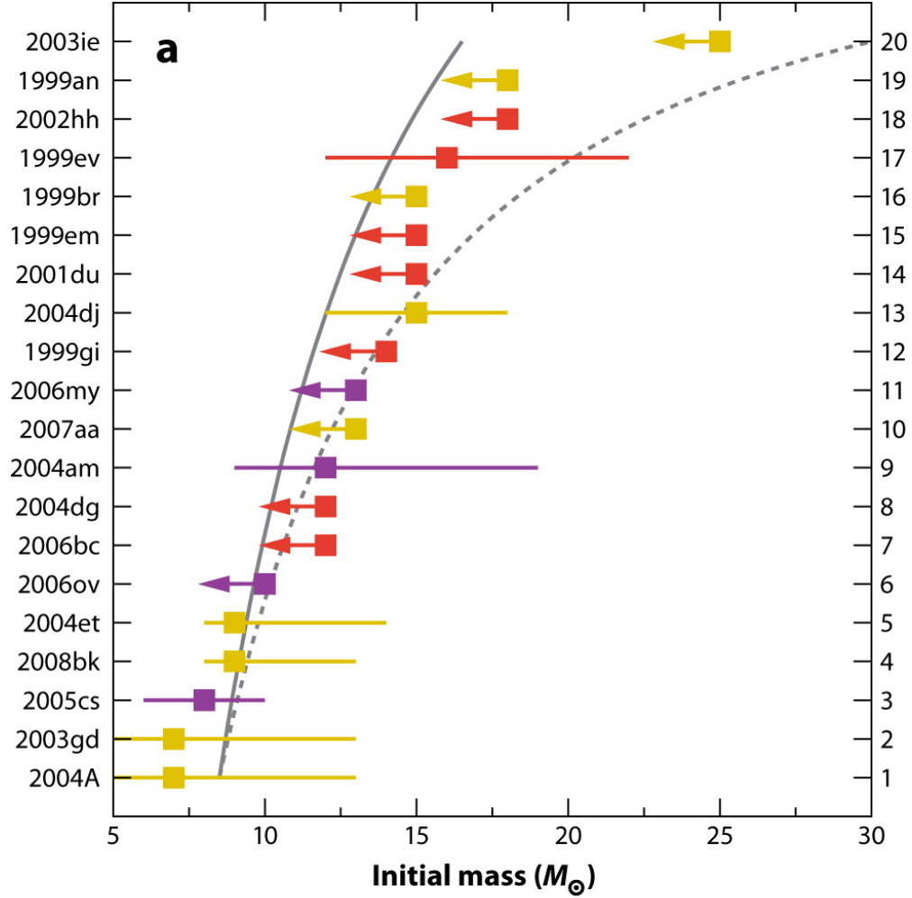
Figure 1.3: A cumulative frequency plot of the masses of II-P progenitors of observed supernovae. The solid line represents a Salpeter IMF best fit to the observed data with a minimum mass of 8.5 M_{\odot} and maximum mass of 16.5 M_{\odot} while the dashed line has a maximum mass of 30 M_{\odot} . The right axis is a cumulative count of events within these two limits. The events are colored according to the metallicity used in model ranging from the composition of the Large Magellanic Cloud to Solar. The supernovae are grouped in metallicity bins \log O/H + 12 = 8.3-8.4 (gold), 8.5-8.6 (red), 8.7-8.9 (purple). Figure from Smartt (2009).
