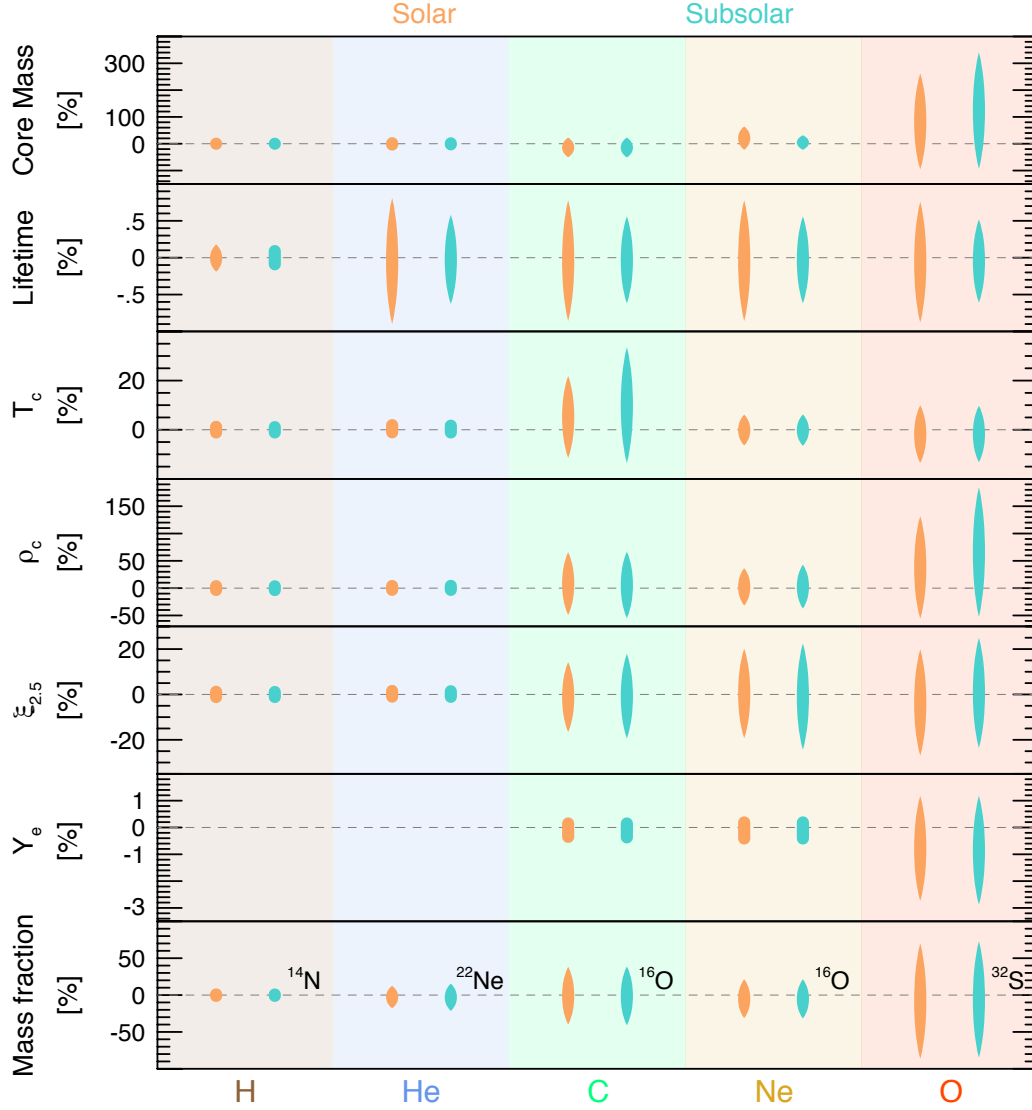
Figure 2.21: Percent variations of the core mass, lifetime, central temperature, central density, compactness parameter, electron fraction, and a chosen “interesting” mass fraction (top to bottom) at H-, He-, C-, Ne-, and O-depletion (left to right). The vertical length of each tapered uncertainty band is the 95% CI for variations about the mean arithmetic value and the horizontal width of each tapered uncertainty band schematically represents the underlying PDF. Solar metallicity models are shown by the orange bands and subsolar metallicity models by the green bands. The first occurrence of significant variation in the compactness parameter \xi_{2.5} occurs at C-depletion. For the mass fractions, we choose to show X_c(^{14}\text{N}) at H-depletion as it holds the star’s initial CNO abundances, X_c(^{22}\text{Ne}) at He-depletion as it holds the neutronization of the core, X_c(^{16}\text{O}) at C- and Ne-depletion as it is dominant nucleosynthesis product of massive stars, and X_c(^{32}\text{S}) at O-depletion as it is a key component of the ashes of O-burning.
