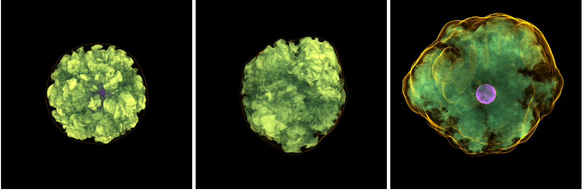
Figure 5.2: Volume rendering of the specific entropy of the 3D-3D32km explosion model at three different times: t_{\text{pb}} \approx 75, 232, and 491 ms from left to right, respectively. The edge of the shock is outlined in orange and the PNS is shown in pink.
