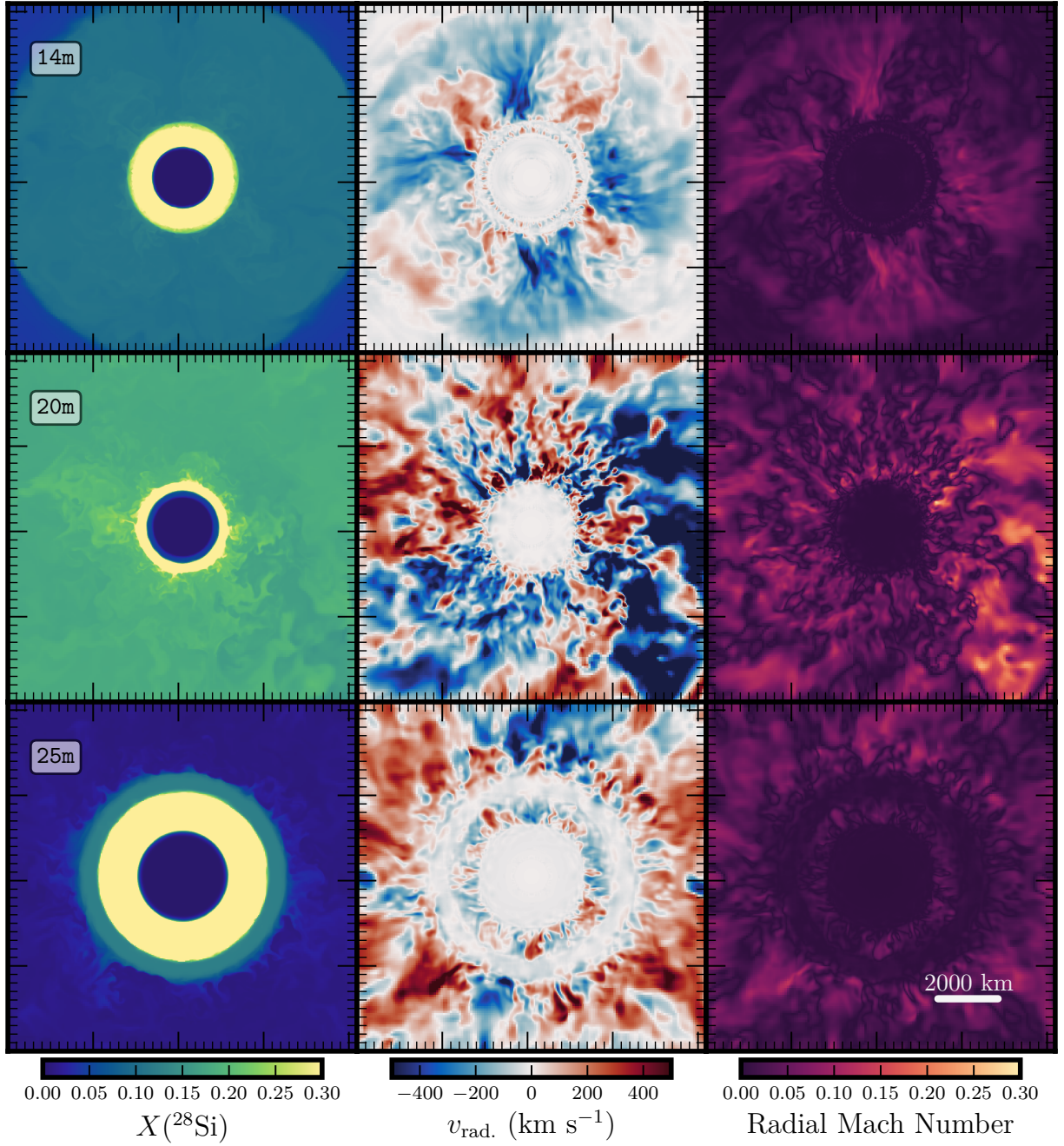
Figure 4.5: Slice plot for the specific ^{28}\text{Si} mass fraction (left column), the radial velocity (middle column), and the radial mach number (right column) in the x - y plane at a time approximately 5 seconds before iron core-collapse for all three 3D models.
