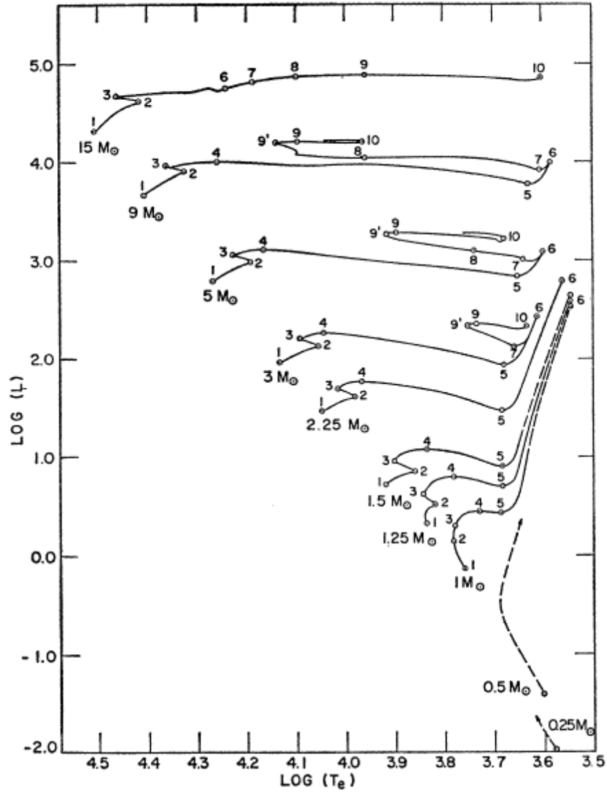
Figure 1.1: Evolutionary paths in the HR diagram of stars with initial mass M_{\text{ZAMS}}=0.25 to 15 M_{\odot} . Dashed lines denote estimated evolutionary tracks. Figure from Iben (1967).
