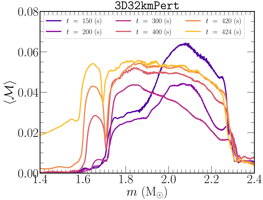
Figure 3.15: The profile of the angle averaged Mach number as a function of mass coordinate at six different times for the 3D32kmPert stellar model. At t = 424 s the average Mach number reaches \langle \mathcal{M} \rangle \approx 0.06 in the Si-shell and at the base of the O-shell.
