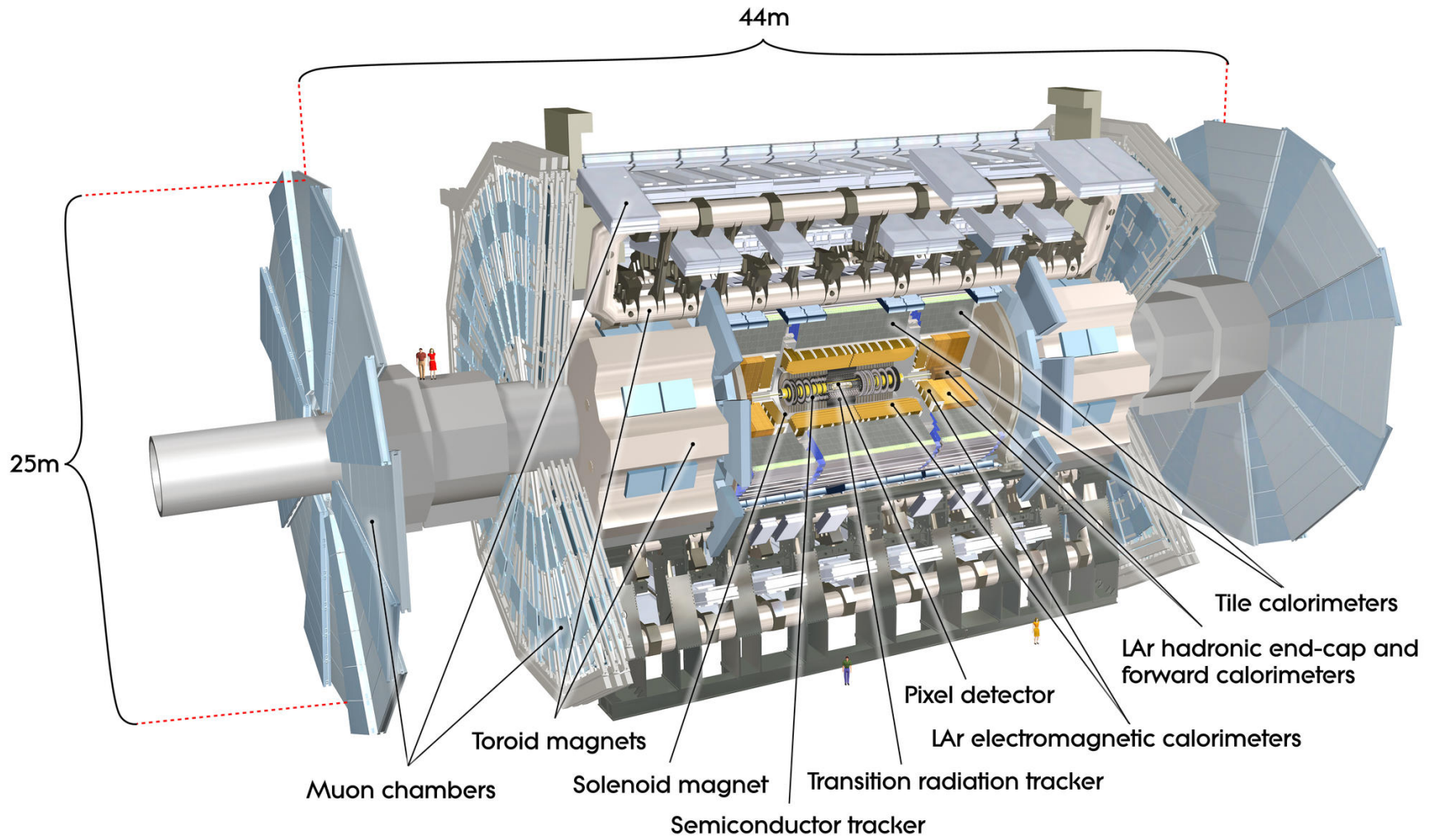
Figure 4.9: Computer generated image of the ATLAS detector indicating all of its major systems [153].
