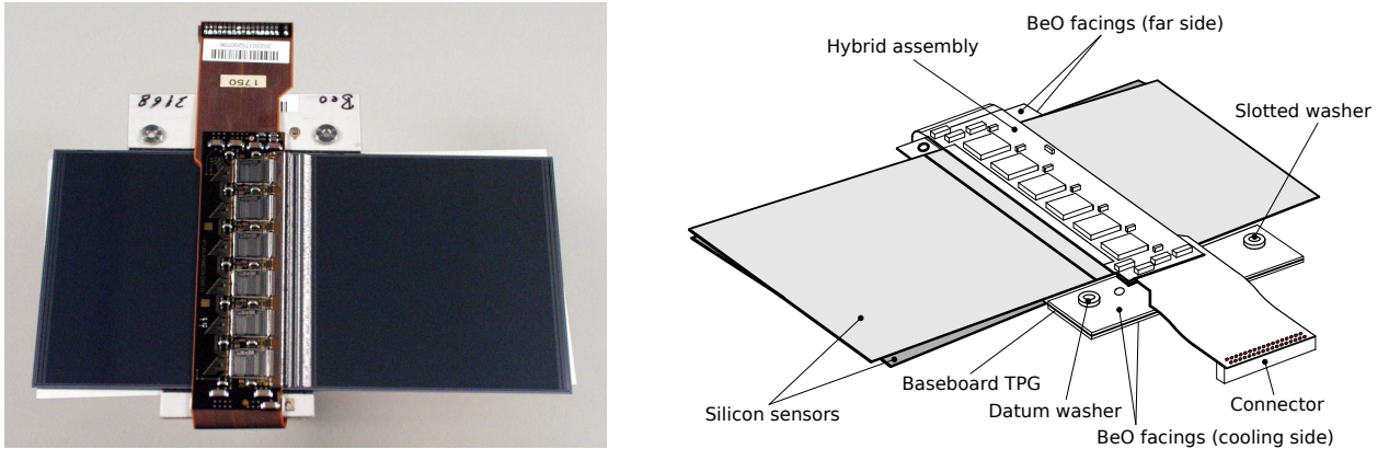
Figure 4.12: Photograph (left) and drawing (right) showing the main components of a SCT barrel module [127].
