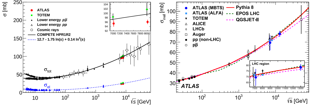
Figure 4.7: Left: Comparison of the total and elastic pp cross section measurements, including measurements from ATLAS and TOTEM at 7 and 8 TeV [151]. Right: The inelastic pp cross section as a function of \sqrt{s} , including measurements at \sqrt{s} = 13 TeV [152].
