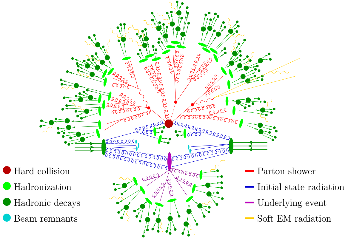
Figure 3.2: Sketch of a hadron-hadron collision as simulated by a Monte Carlo event generator [32].
