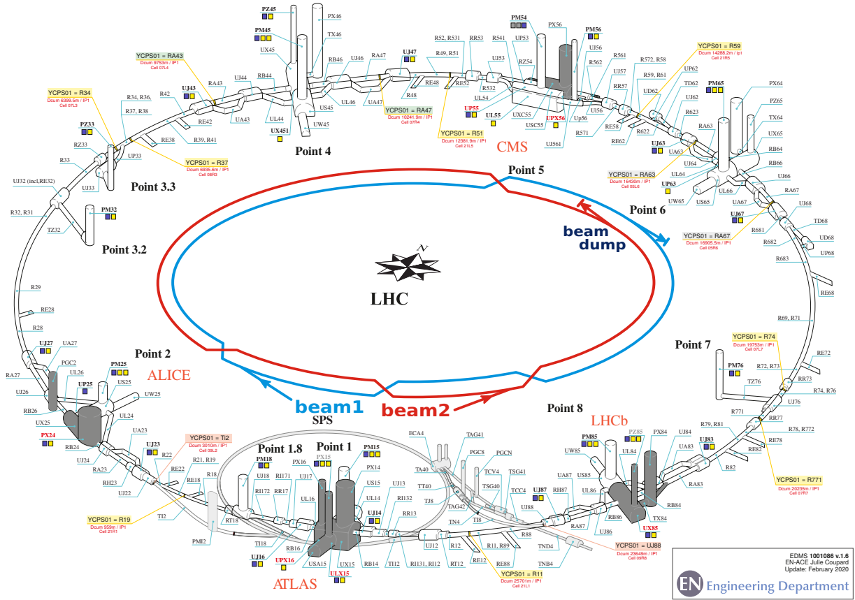
Figure 4.2: Detailed view of the underground LHC facilities, showing the locations of the experiments and beam intersection points [135, 136]. The locations of the four major LHC experiments: ATLAS, CMS, LHCb, and ALICE are highlighted in gray.
