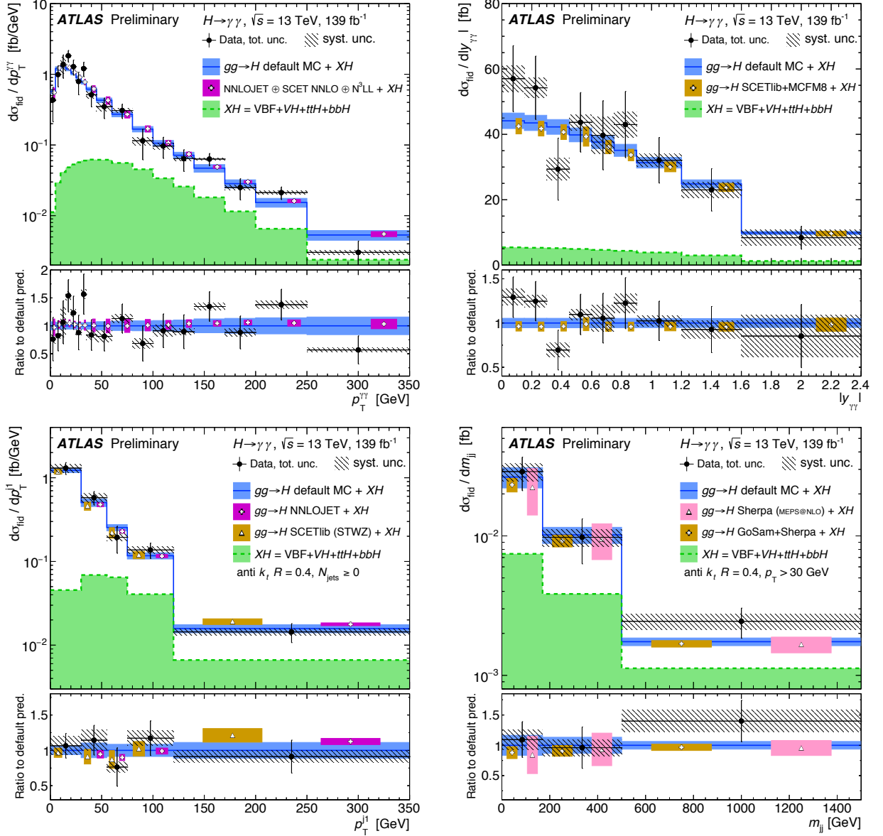
Figure 6.24: Fiducial differential cross section measurements for p_T^{\gamma\gamma} , |y_{\gamma\gamma}| , p_T^{j_1} , and m_{jj} done with \int L = 139.0 \text{ fb}^{-1} in 2019 [277, 278].
