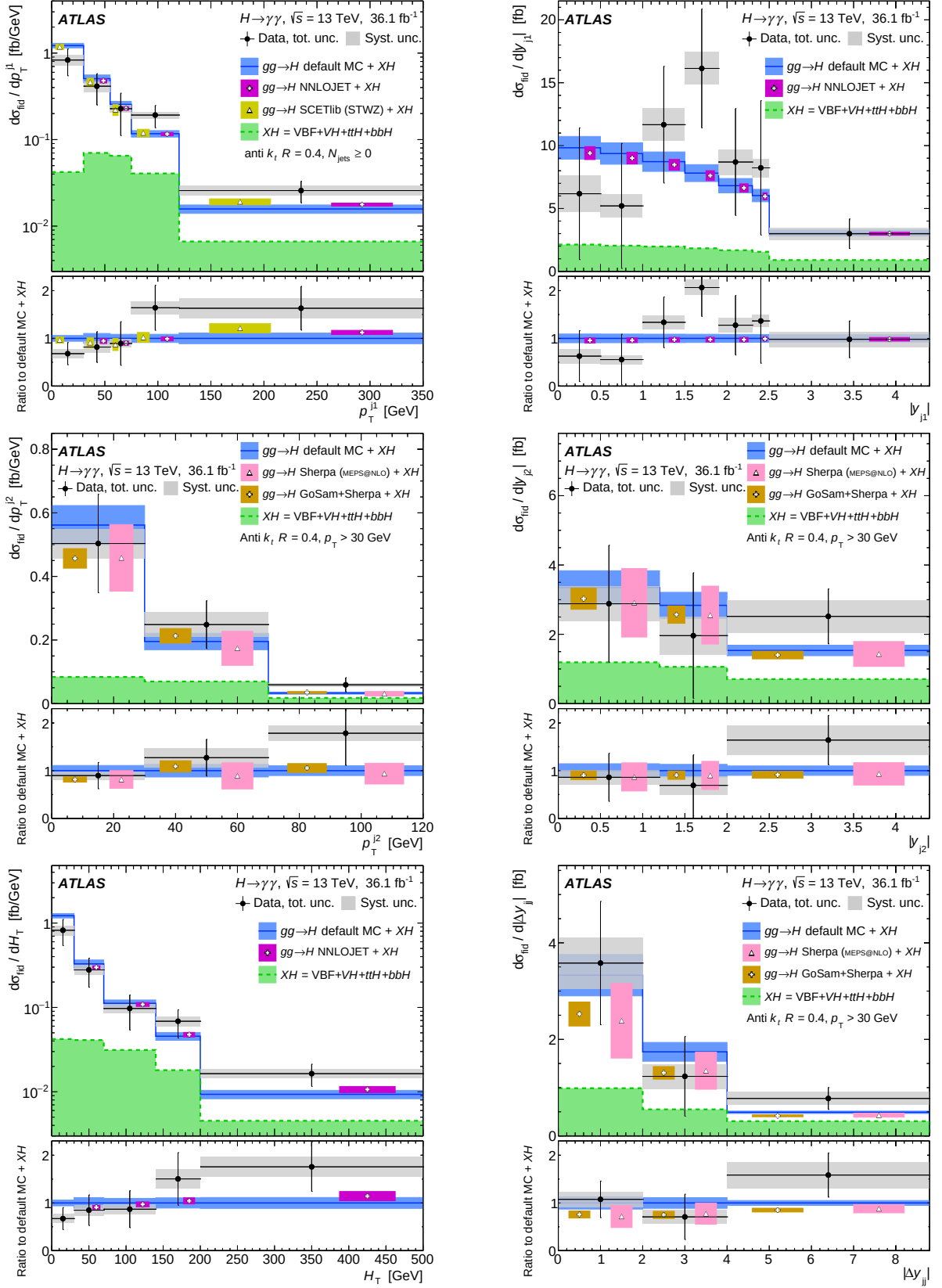
Figure 6.31: Fiducial differential cross section measurements for p_T^{j1} , |y_{j1}| , p_T^{j2} , |y_{j2}| , H_T , and |\Delta y_{jj}| done with \int L = 36.1 \text{ fb}^{-1} in 2017 [272–274].
