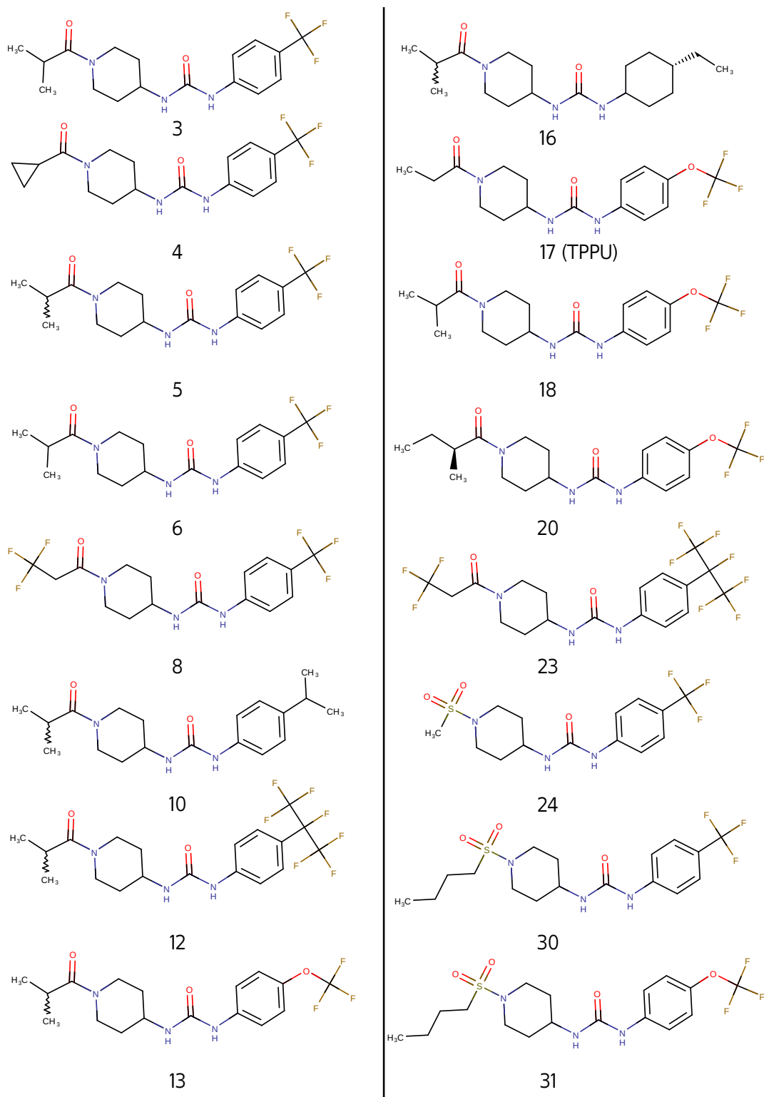
Figure 6.2: Chemical structures of all of the inhibitors from [2] that had both unbinding rates and affinities experimentally measured as in Table 6.1. The R_2 groups are oriented to the left and the R_1 groups are oriented to the right. Bonds shown as a zig-zag were measured as a racemic mixture of stereo-isomers.
