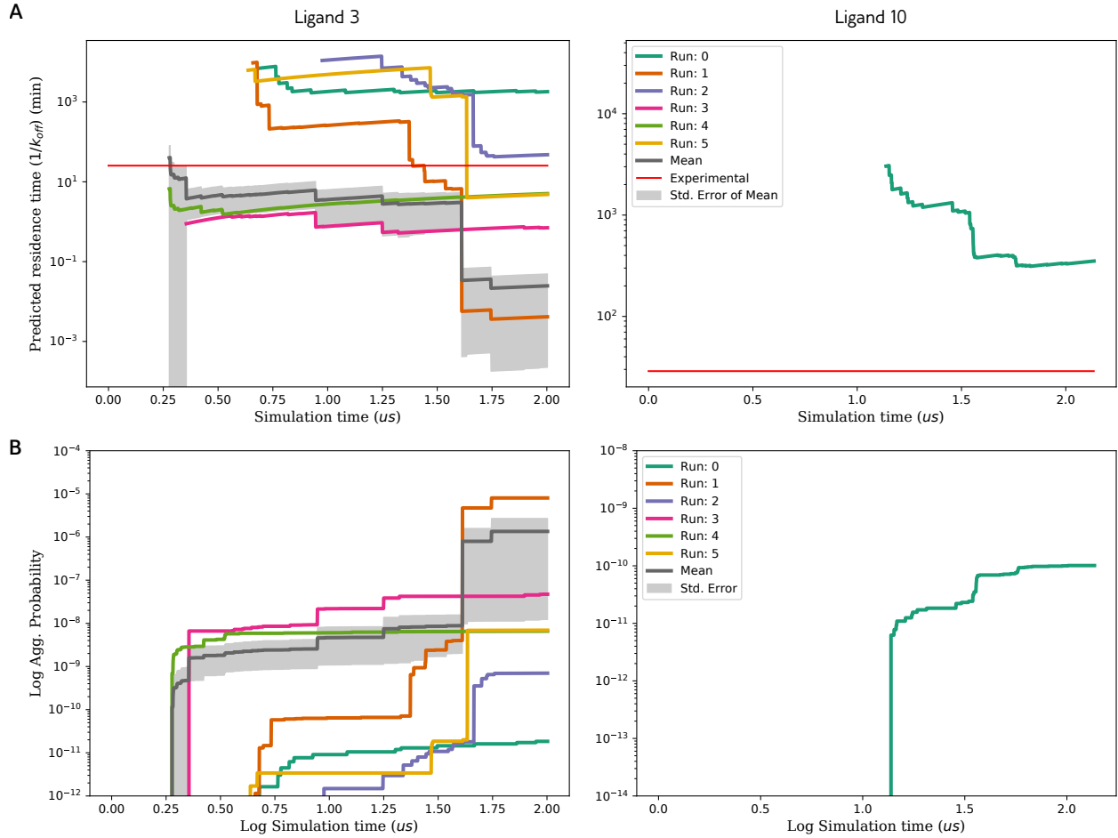
Figure 6.7: Plots of the rate estimates (Panel A) and aggregate probability flux through the unbinding boundary condition Panel B. The total aggregate simulation time across all walkers is given on all of the horizontal axes for each plot in microseconds. For all plots the individual replicate runs for which there were unbinding events observed are plotted in color lines (see the legend in plots) and the average of these is plotted in the dark grey line with the standard error of the mean shown as the light grey envelope. Plots in Panel A show the predicted residence time RT = 1/k_{\text{off}} over time starting with the first unbinding event observed for a simulation. The horizontal red line is the experimentally determined rate as determined by Lee et al. (2014) [2]. Plots in Panel B show the cumulative probability over time that had crossed the boundary. Ligand 10 only had a single replicate observe unbinding.
