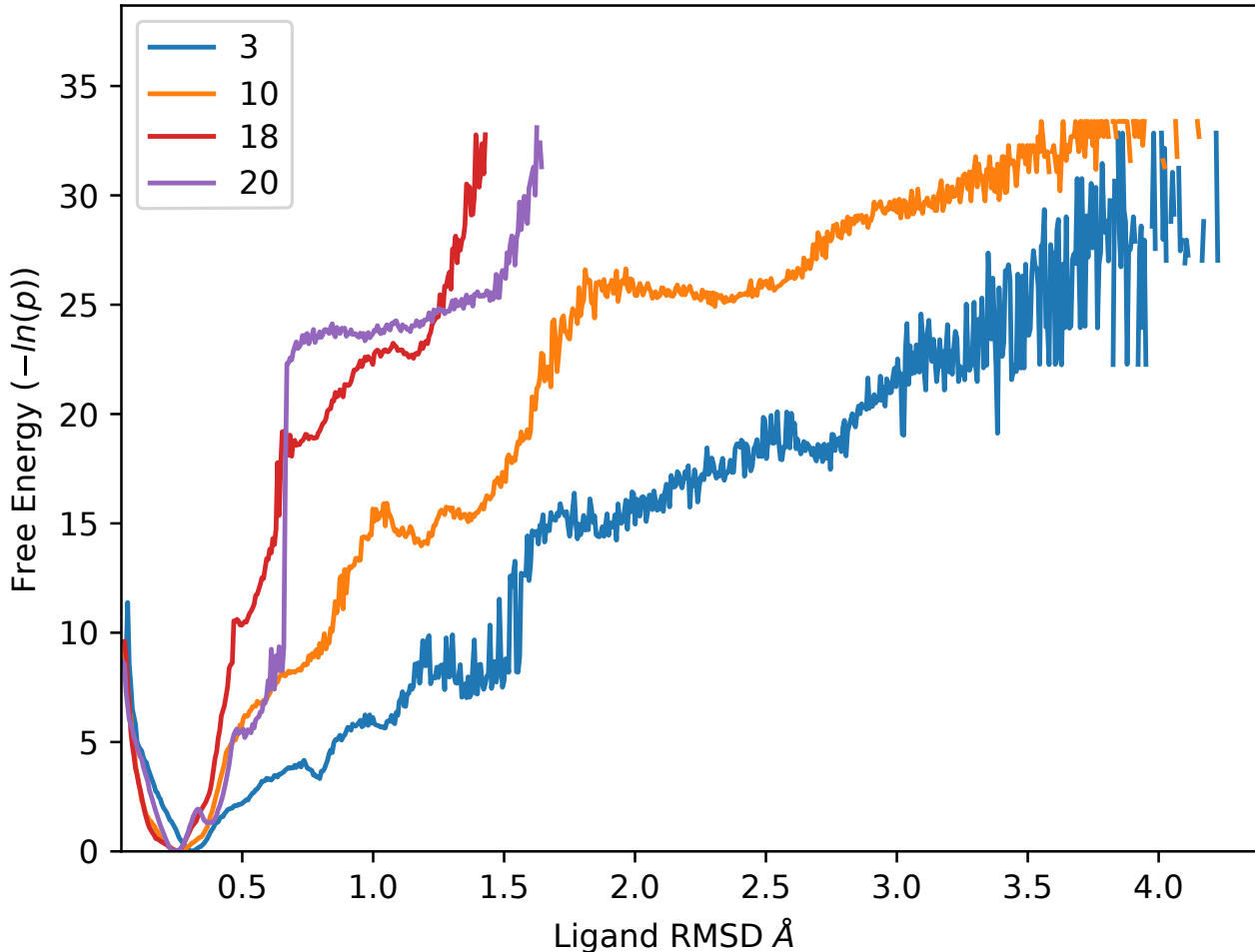
Figure 6.10: Average between each replicate final free energies ( -\ln p ) for each ligand over the ligand RMSD ( \text{\AA} ).
