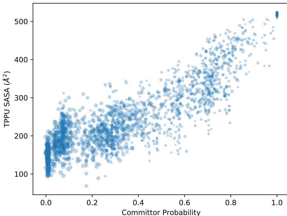
Figure 5.20: Plot of the ligand TPPU solvent accessible surface area (SASA) ( \text{\AA}^2 ) [4] for every cluster representative in the network over their committor probabilities. The size of the points is equal to the negative of the free energy ( -\ln(p) ) of the cluster translated to the positive domain. Clusters which were not assigned a committor probability are not included.
