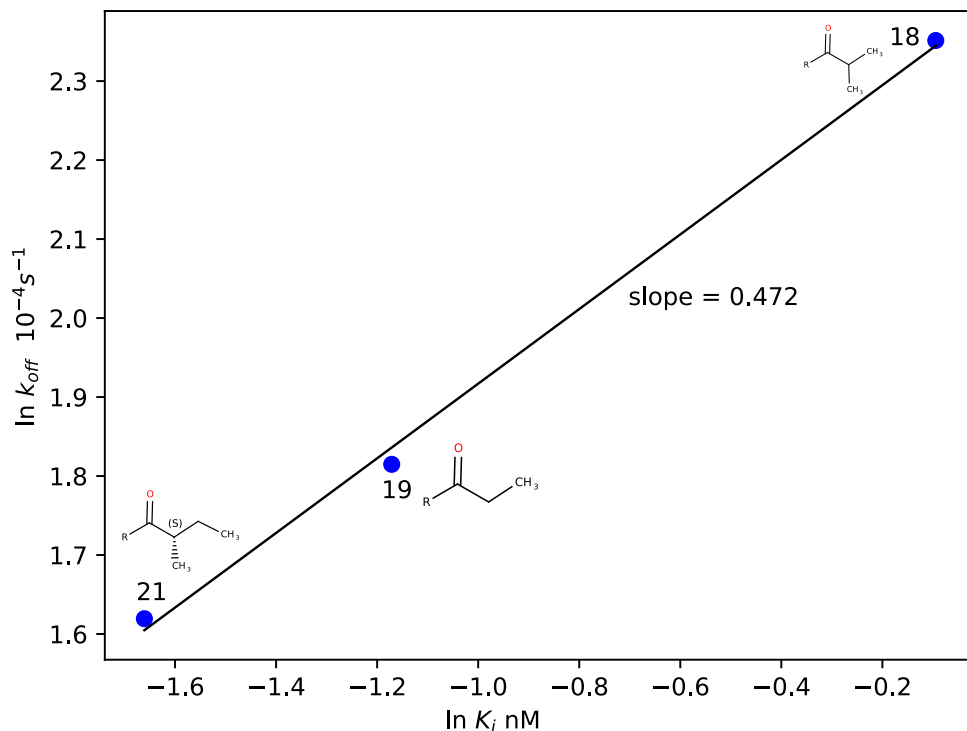
Figure 5.19: Plot of unbinding rates ( \ln k_{\text{off}} ( 10^{-4} \text{ s}^{-1} )) vs. the inhibition constants ( \ln K_i (nM)) of inhibitor ligands from Lee et al. [2] that have the same scaffold (i.e. same non-R2 structure) but different R2 substituents. The structure of the R2 substituents are pictured next to each point. The result of a linear regression is plotted in black and is shown to have a slope of 0.472. For this series the relationship between k_{\text{off}} and K_i is linear ( R^2 = 0.998 ), at least for this small sample size. When considering all inhibitors of sEH measured in [2] this particular series is a much better fit. R^2 = 0.999 for the untransformed data shown in this figure, compared to an R^2 = 0.440 21 when considering all measured inhibitors in the same region of values for k_{\text{off}} and K_i .
