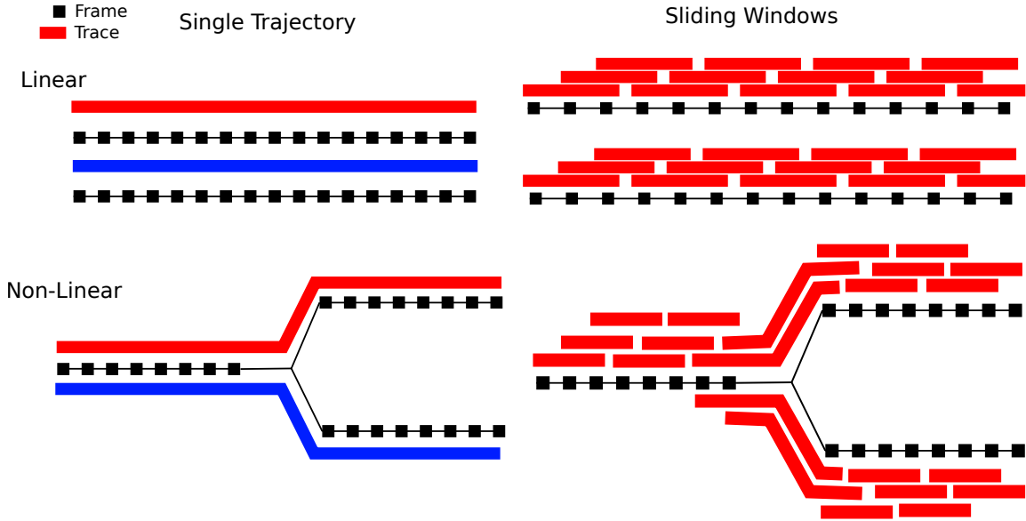
Figure 2.3: Non-linear trajectories comparison. The black squares indicate single frames which are connected in time by the thin black lines. The larger lines indicate a locally linear trajectory, here called a "trace".
