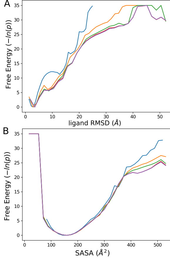
Figure 5.2: Cumulative non-equilibrium free energy profiles of A) ligand RMSD to the initial structure after superimposing the protein binding sites and B) ligand SASA [4]. Each line consists of values taken from the frames of cycles indicated in the legend, i.e. in increments of 300 cycles. Raw weights ( p ) were binned and summed across the progress coordinate values (30 bins) within each set of cycles before computing the free energy, FE_{\text{bin}} = -\ln \sum_i^M p_i , where M is the number of observations in a bin.
