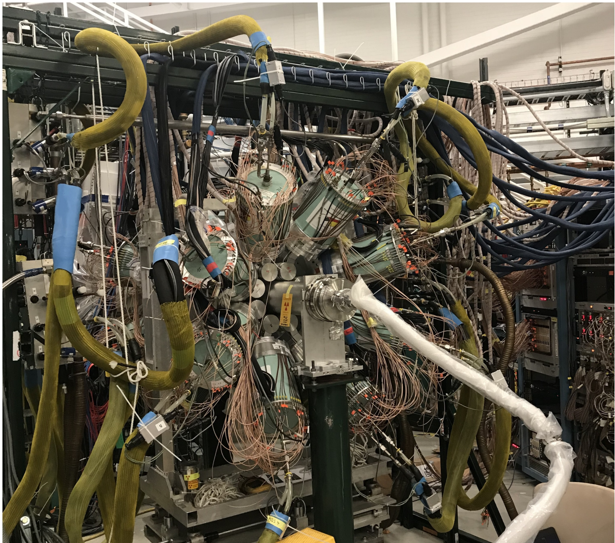
Figure 3.17: SeGA arranged in the barrel configuration at ReA3. Only six detector end-caps are visible arrayed around the beam pipe. The silicon detectors and target are inside the beam pipe.
