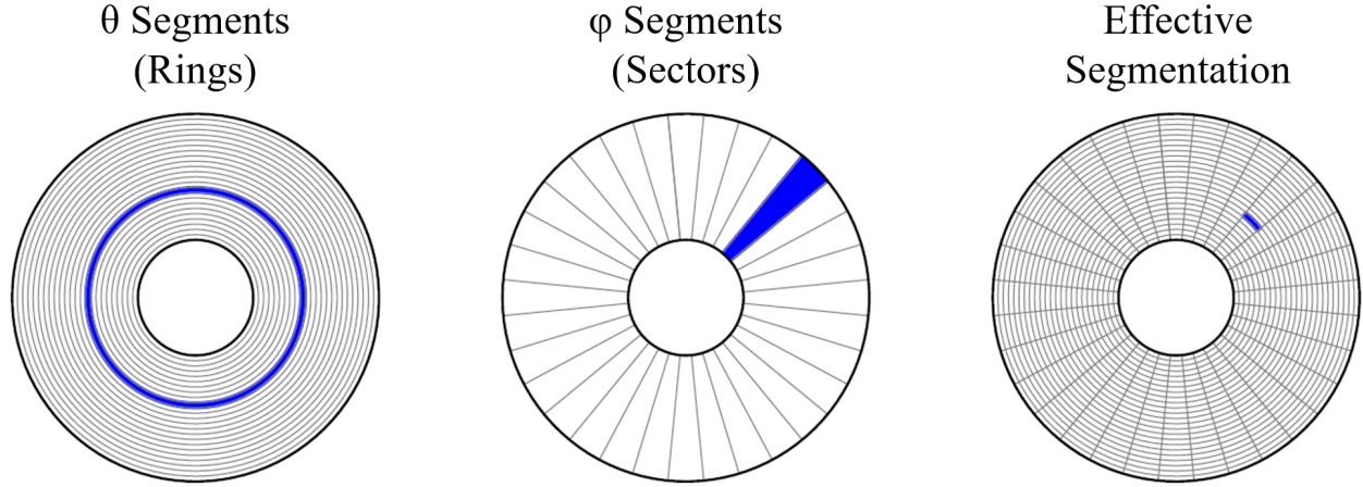
Figure 3.2: Segmentation of the JANUS silicon detectors. Figure adapted from [108].
