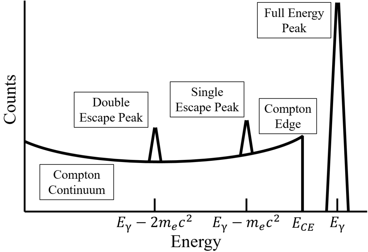
Figure 3.12: An idealized spectrum emphasizing the components which result from the interactions of a mono-energetic \gamma -ray with E_\gamma > 2m_e c^2 . The origins of the individual components are discussed in the text.
