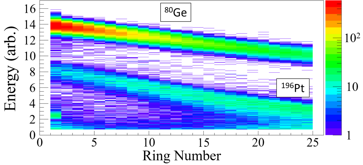
Figure A.1: Kinematic curve observed in the forward silicon detector. The scattered ^{80}\text{Ge} and recoiling ^{196}\text{Pt} are clear. It also clear there is no separation between the ^{80}\text{Ge} and the ^{80}\text{Kr} contamination.
