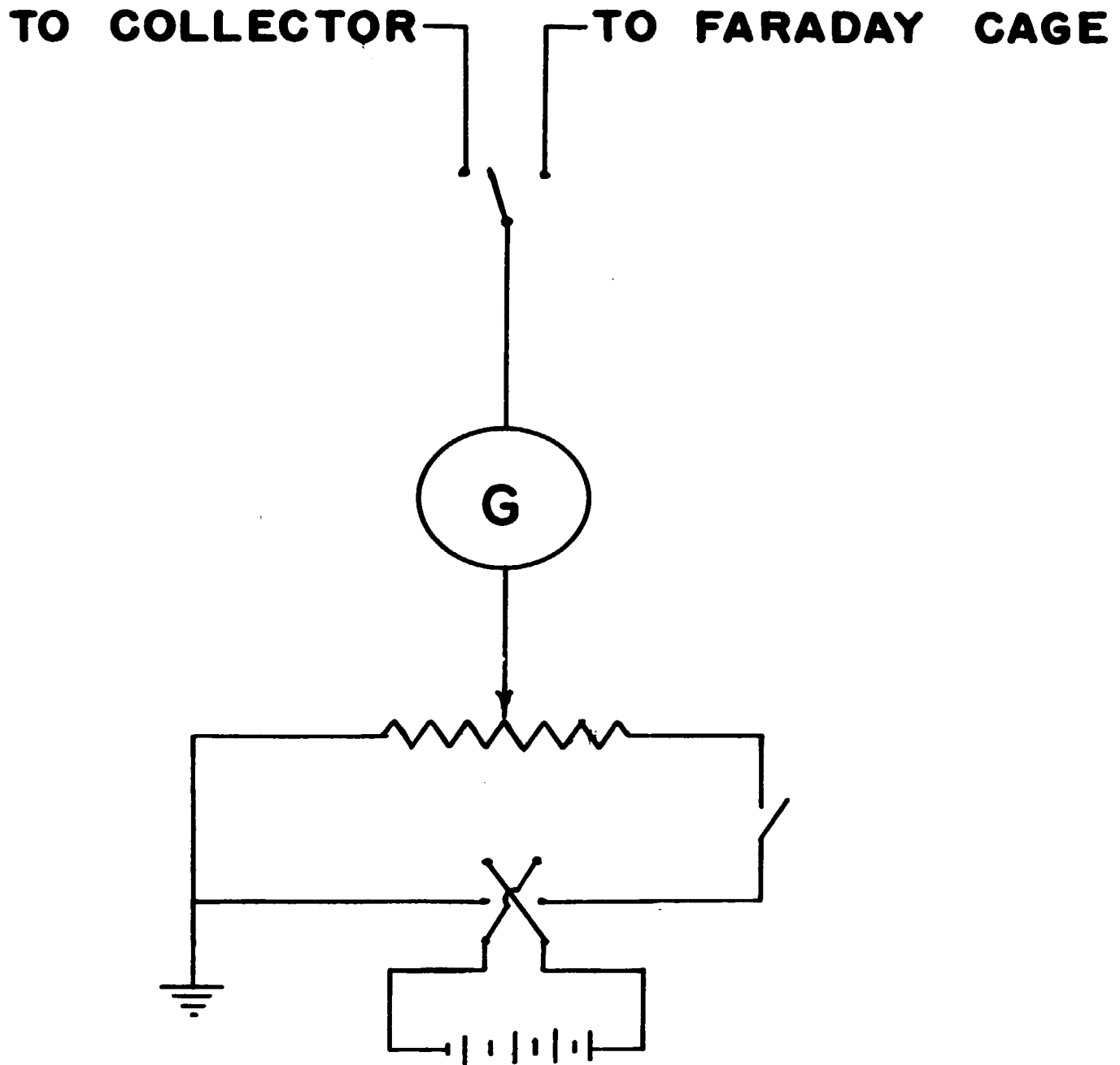
CURRENT MEASURING NETWORK
