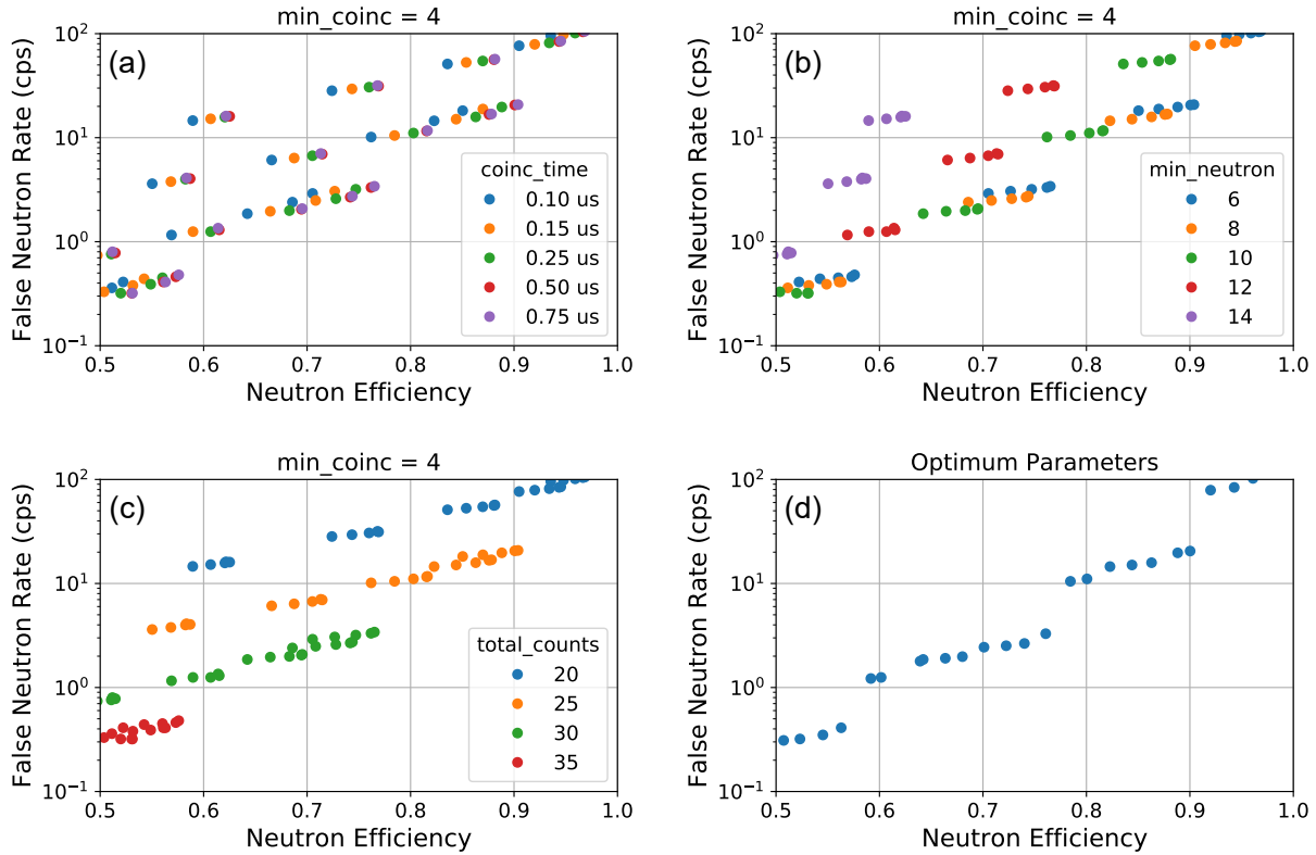
Figure 11.7: (a-c) Performance of filter for parameter sets with min_coinc = 4 only. (d) Performance of the filter algorithm for optimum parameter sets only.
