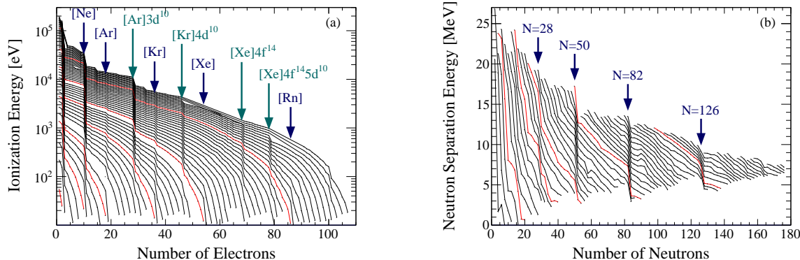
Figure 2.1: (a) Ionization energy vs. electron number [20]. Each line represents an element. Electron configurations are indicated with arrows. (b) Neutron separation energy vs. neutron number [21, 22]. Each line represents an element. The smaller magic numbers 2, 8, and 20 are not shown, but the larger magic numbers are indicated with arrows.
