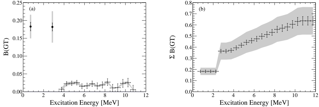
Figure 8.7: (a) Measured B(\text{GT}) distribution. (b) Cumulative B(\text{GT}) distribution. Gray bands indicate systematic error.
