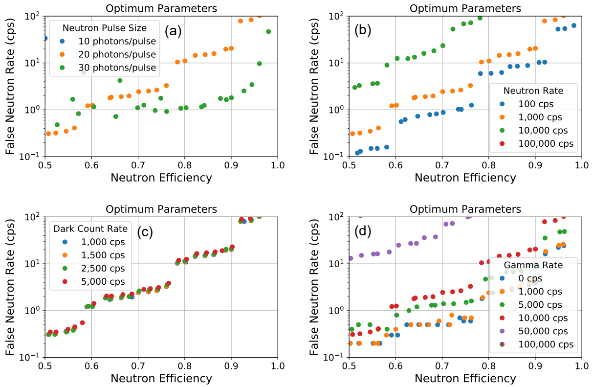
Figure 11.8: Performance of filter for various (a) neutron pulse sizes, (b) neutron rates, (c) dark count background rates, and (d) gamma rates.
