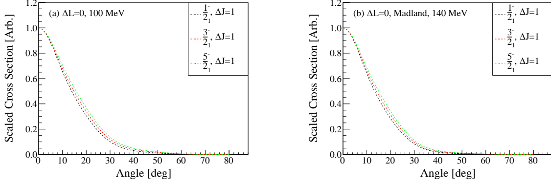
Figure 4.9: (a) Scaled \Delta L = 0 cross sections with the 100 MeV NN interaction [103]. (b) Scaled \Delta L = 0 cross sections with the original NN interaction.
