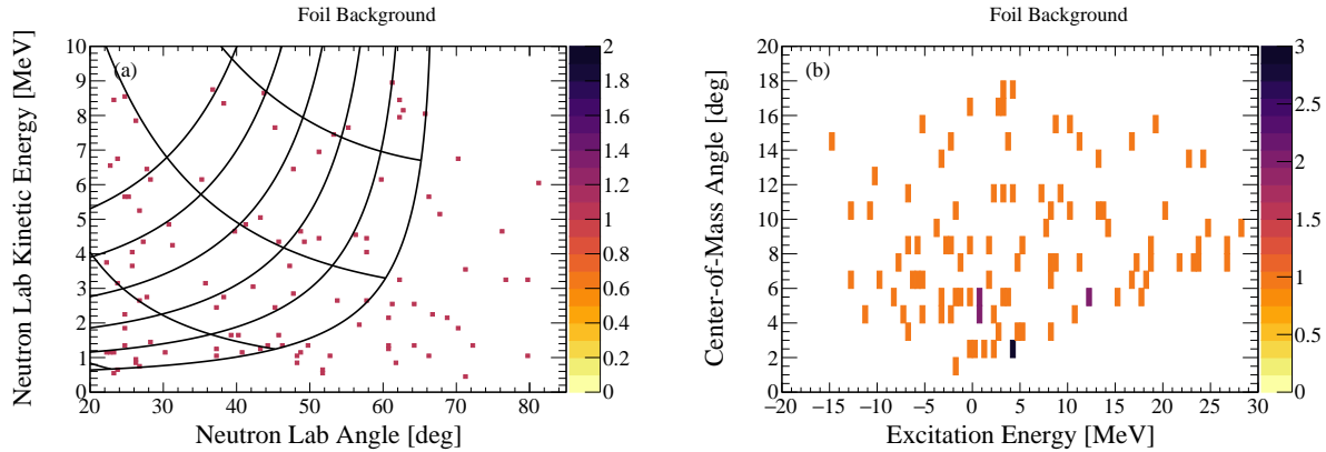
Figure 7.2: Foil background measurement for the 2.4900 Tm rigidity setting in (a) the laboratory frame and (b) the center-of-mass frame.
