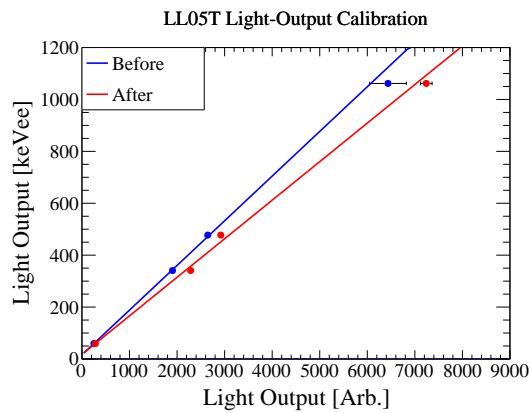
Figure 10.6: Energy calibrations for the LL05T PMT before (blue) and after (red) the experiment.
