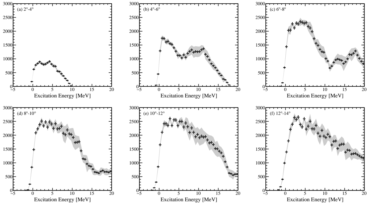
Figure 7.16: First-iteration simulated output, N_{Sim\ out}^{1st} .
