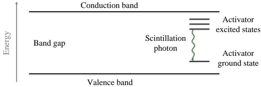
Figure 5.8: Illustration of the energy band structure of an inorganic scintillator with an activator, adapted from Ref. [112]. The scintillation photon comes from the de-excitation of an electron through the activator states.
