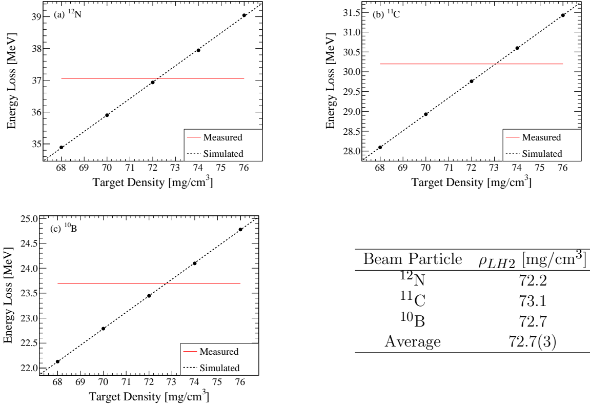
Figure 7.31: Energy loss in the target vs. the target density measured with a (a) 12 N beam, (b) 11 C beam, and (c) 10 B beam. The black points are the simulated energy loss, and the dashed black line is a fit to the black points. The solid red line is the measured energy loss. The point where the red and black lines intersect was used as actual target density.
