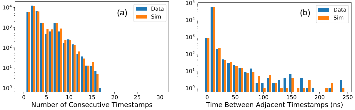
Figure 11.3: (a) The number of consecutive timestamps and (b) the time between adjacent timestamps were used to find the parameters of the dark count background simulation.
