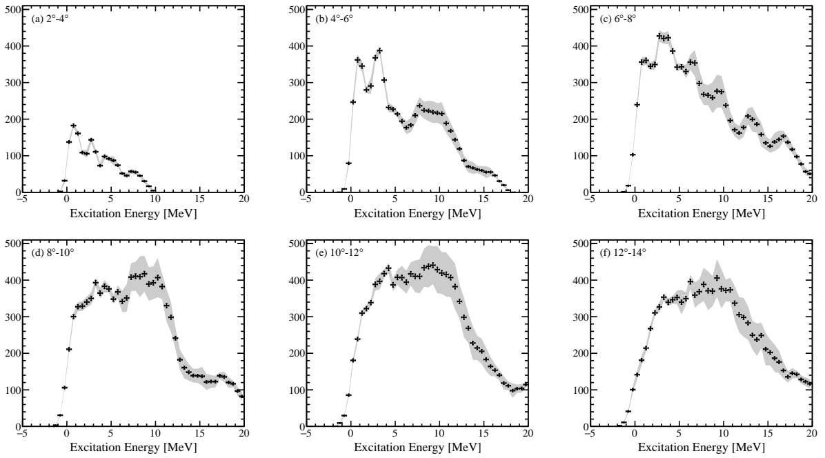
Figure 7.20: Second-iteration simulated output, N_{Sim\ out} .
