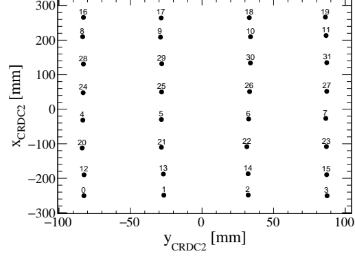
Figure 6.21: Average CRDC positions for each hodoscope crystal. The marker labels indicate the crystal ID number. From this, the crystal ID was assigned to a known crystal location.
