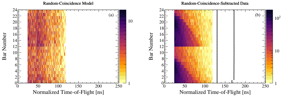
Figure 7.3: Normalized time-of-flight spectrum for each LENDA bar for the 2.3290 Tm setting. The black lines indicate the random coincidence sampling window. The light output maximum cut is not applied so the data at large TOF_{1m} can be seen.
