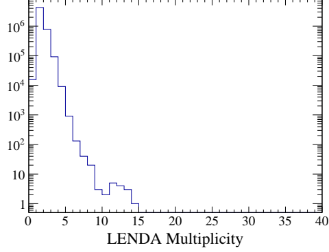
Figure 6.32: LENDA multiplicity for the 2.3290 Tm rigidity setting.
