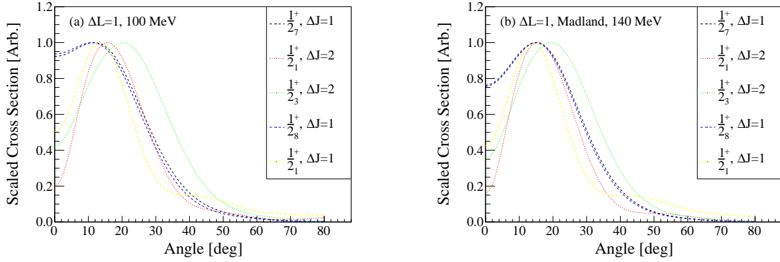
Figure 4.10: (a) Scaled \Delta L = 1 cross sections with the 100 MeV NN interaction [103]. (b) Scaled \Delta L = 1 cross sections with the original NN interaction.
