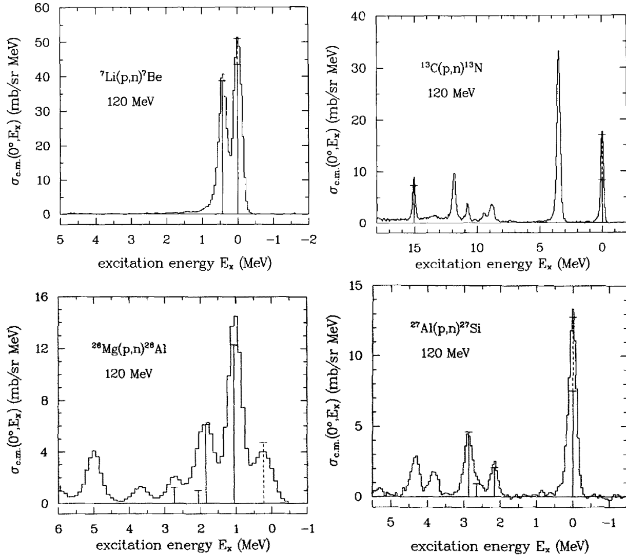
Figure 3.4: Evidence supporting the proportionality relationship [68]. The vertical bars indicate the cross section calculated from the proportionality relationship with B(\text{GT}) from \beta -decay. The dashed portion indicates the Fermi contribution. The bars match the data well, indicating that the proportionality is valid.
