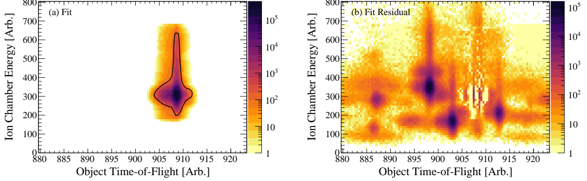
Figure 6.26: (a) Fit used to determine the PID efficiency of the E_{IC} - TOF_{obj} PID for the 2.3290 Tm rigidity setting. (b) The fit residual (the data minus the fit).
