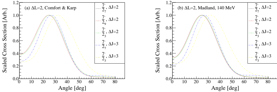
Figure 4.8: (a) Scaled \Delta L = 2 cross sections with optical potential parameters from Ref. [104]. (b) Scaled \Delta L = 2 cross sections with the original optical potential parameters.
