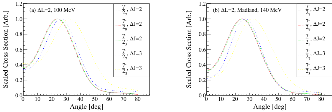
Figure 4.11: (a) Scaled \Delta L = 2 cross sections with the 100 MeV NN interaction [103]. (b) Scaled \Delta L = 2 cross sections with the original NN interaction.
