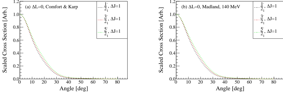
Figure 4.6: (a) Scaled \Delta L = 0 cross sections with optical potential parameters from Ref. [104]. (b) Scaled \Delta L = 0 cross sections with the original optical potential parameters.
