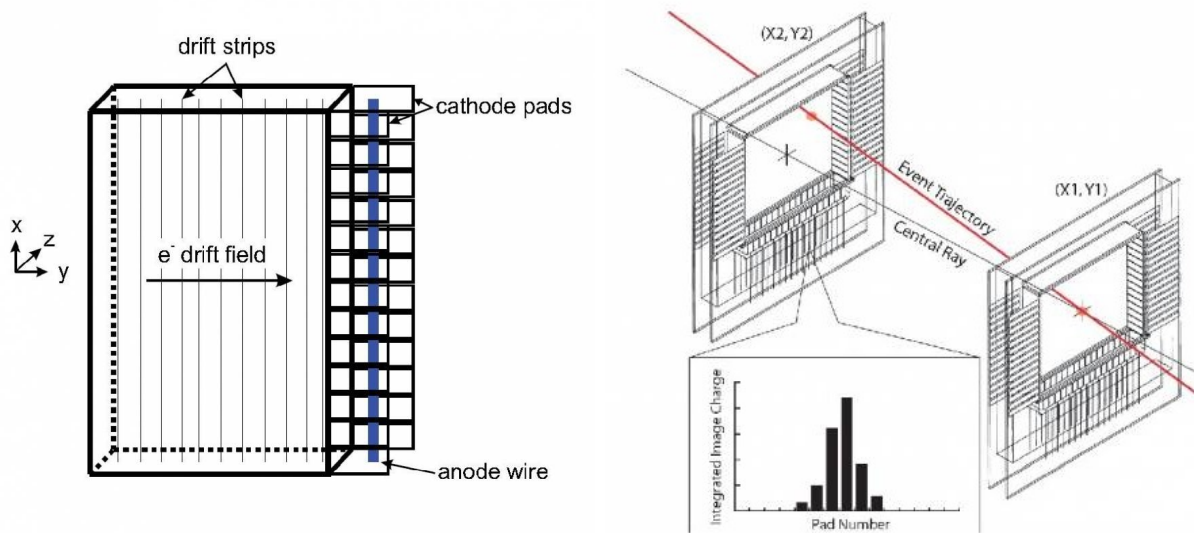
Figure 5.6: Diagram of the S800 focal-plane detectors, taken from Ref. [111]. The cathode readout drift chambers (CRDCs) measured the position and angle, the ionization chamber measured the energy loss, the plastic scintillator measured the time, and the hodoscope measured the remaining energy of each residual nucleus.
