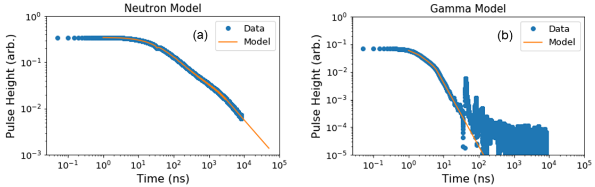
Figure 11.4: Average scintillator response with model for (a) neutrons and (b) gamma rays.
