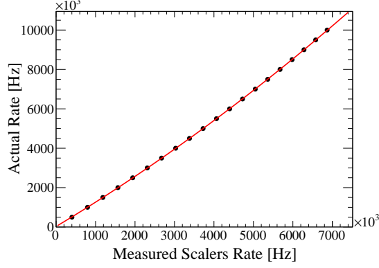
Figure 7.25: The black points are the measured scalers rate R_{scal} calculated from the actual beam rates R_{scal}^{corr} . The red line is a second-degree polynomial fit to the points. The fit was used to calculate R_{scal}^{corr} from R_{scal} .
