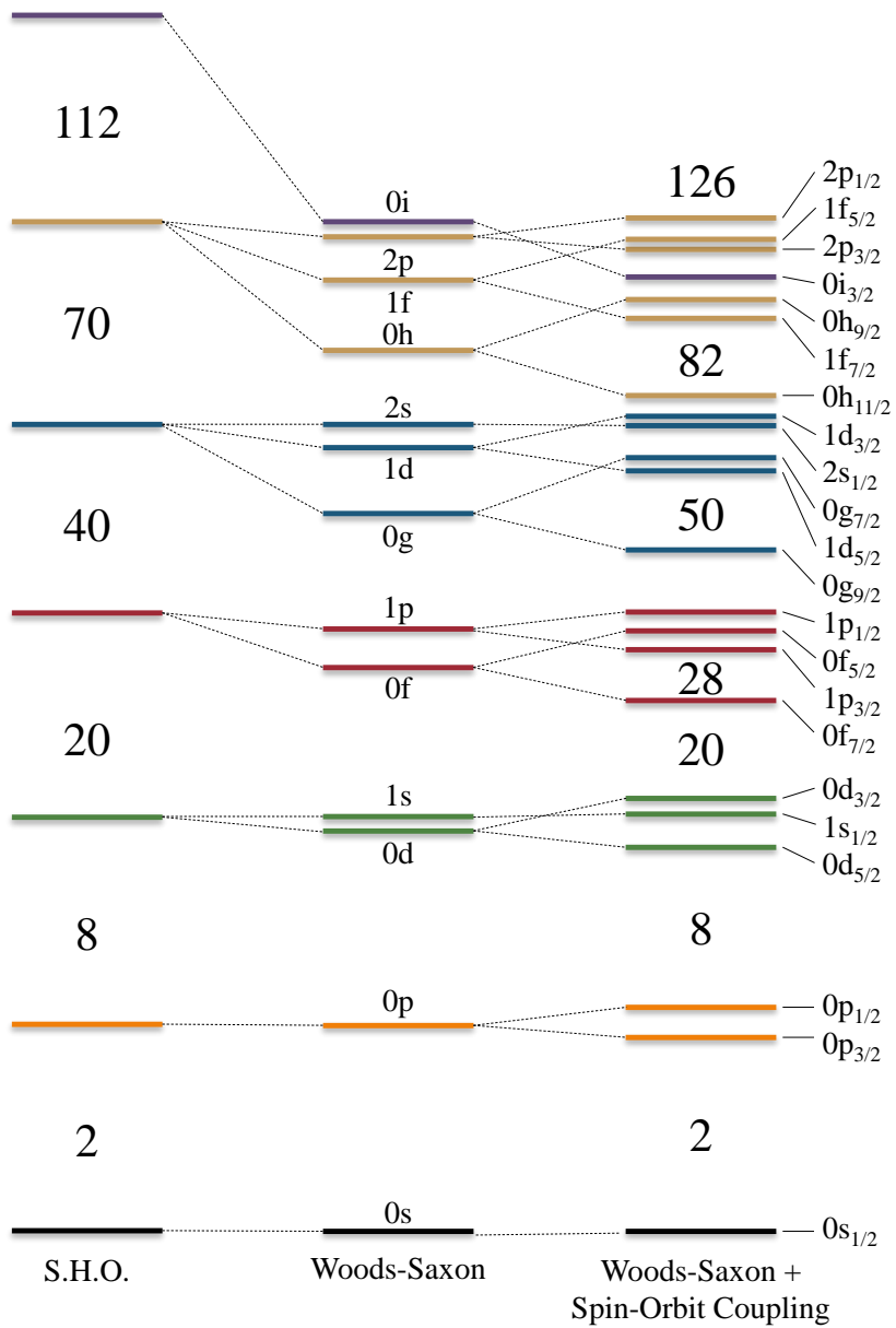
Figure 2.3: Diagram of the nucleon orbitals adapted from Ref. [23].
