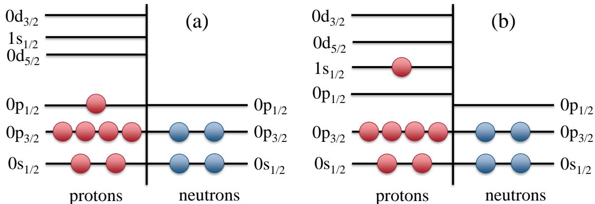
Figure 2.4: (a) Configuration that dominates the ^{11}\text{N} ground state according to the independent particle model. (b) Configuration that actually dominates the ^{11}\text{N} ground state.
