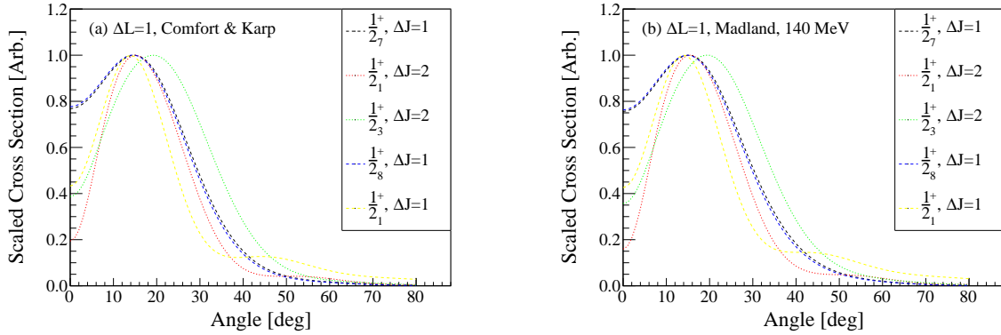
Figure 4.7: (a) Scaled \Delta L = 1 cross sections with optical potential parameters from Ref. [104]. (b) Scaled \Delta L = 1 cross sections with the original optical potential parameters.
