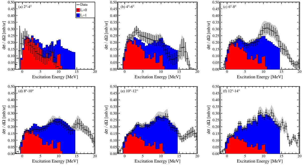
Figure 8.4: Cross sections broken down into their \Delta L components according to the MDA results.
