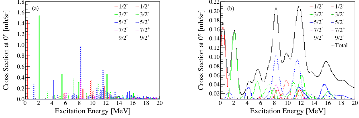
Figure 4.1: (a) Theoretical cross section, including \frac{1}{2}^\pm , \frac{3}{2}^\pm , \frac{5}{2}^\pm , \frac{7}{2}^\pm , \frac{9}{2}^\pm states. (b) Same as (a), smeared with the experimental resolution.
