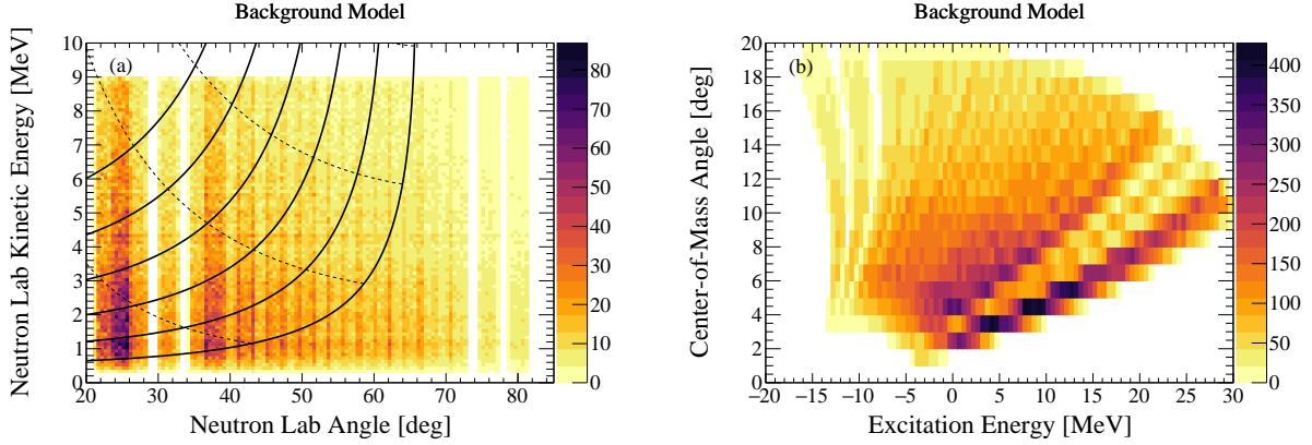
Figure 7.8: Background model, N_{bg} , in (a) the lab frame and (b) the center-of-mass frame for the 2.3290 Tm setting.
