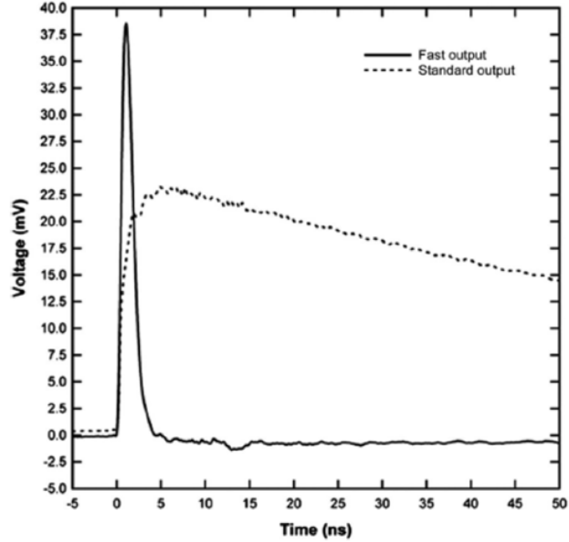
Figure 11.2: Silicon photomultiplier single-photon response [132]. The standard output is used in this case.
