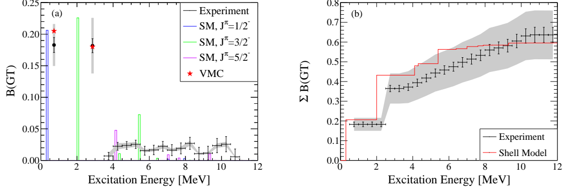
Figure 9.1: (a) Comparison of the data (black, with gray bands indicating systematic error) to the shell-model calculations (blue, green, purple) and VMC calculations (red stars). (b) Measured cumulative B(\text{GT}) distribution (black, with gray bands indicating systematic error) compared to the shell-model calculation (red).
