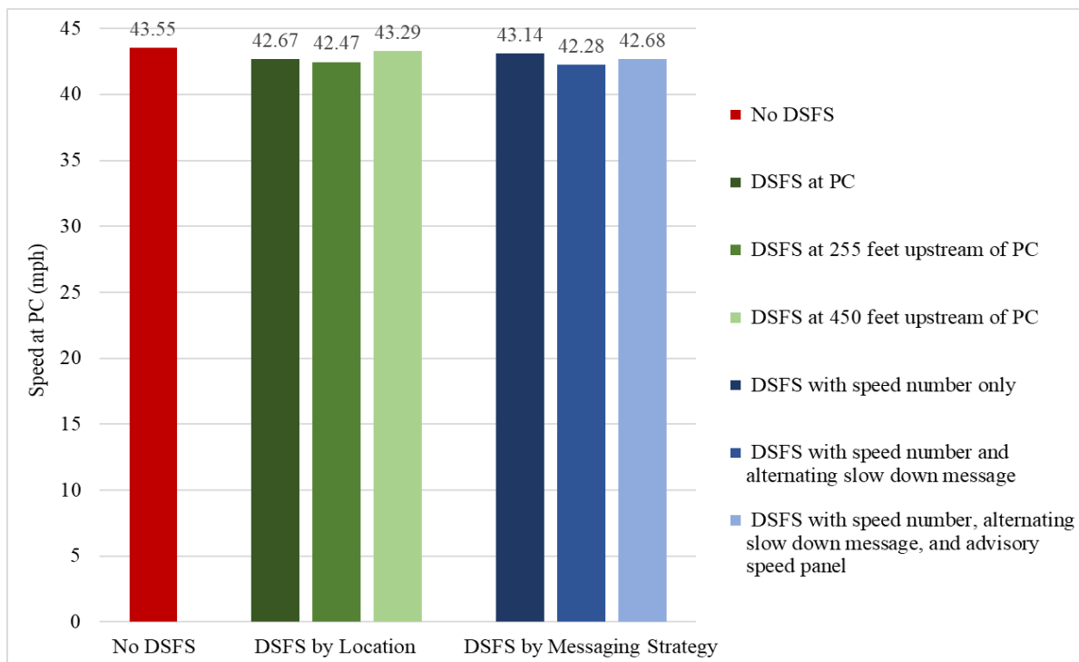
Figure 13 Mean curve entry speeds by DSFS position and messaging strategy (PSGR only)
