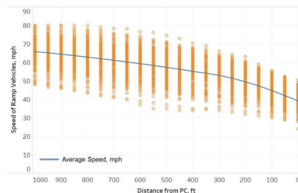
b) LIDAR data interpolated at 50-ft increments
