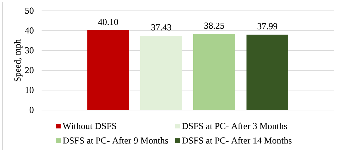
Figure 30 Average curve entry speeds before DSFS installation and during the 14-months after DSFS installation
