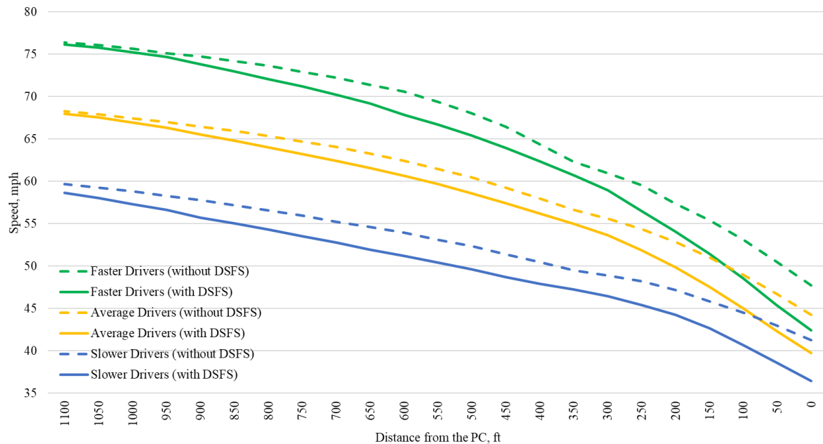
Figure 28 Average vehicle speed profiles for drivers at different speed percentiles
