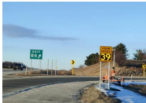
b) Side-mounted DSFS
