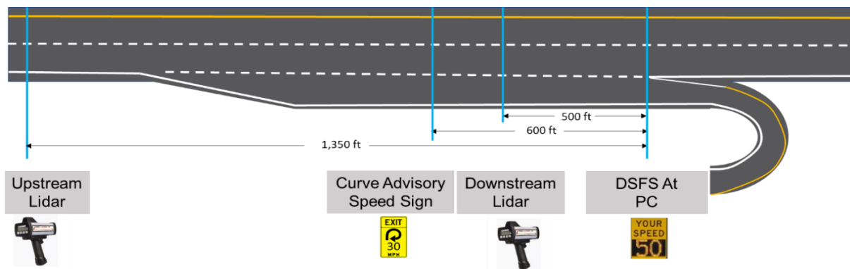
Figure 8 A typical two-person LIDAR data collection setup
