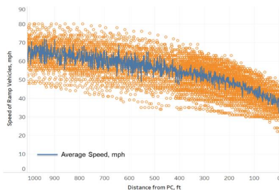
a) Raw LIDAR data (n=203 vehicles)
