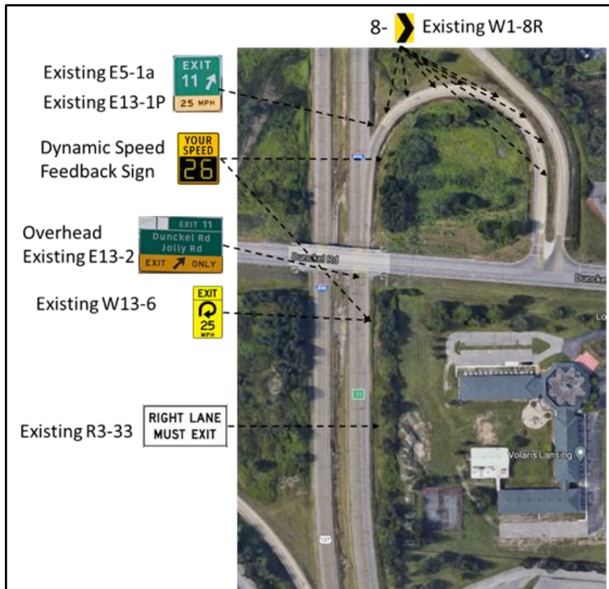
Figure 24 NB US-127 Exit Ramp to Dunckel Rd (Site 5)
