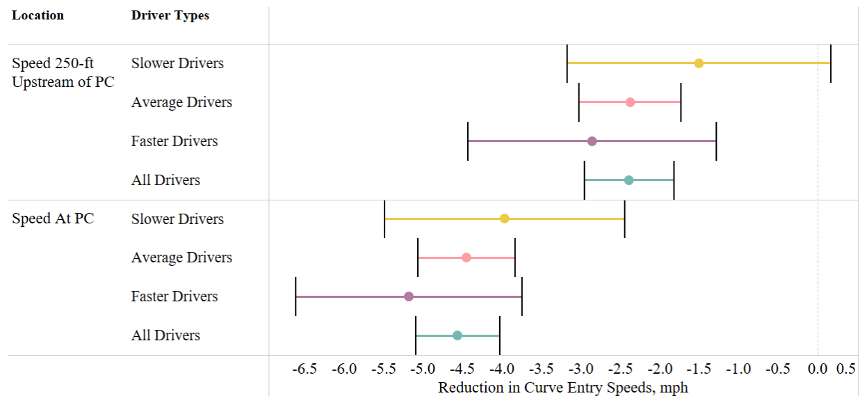
Figure 29 Linear regression parameter estimates for the reduction in speed at freeway exit ramps (with 95% confidence intervals)
