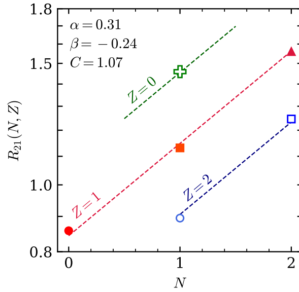
Figure 5.25 The data points are experimental data, and the dashed lines are the isoscaling fits, with fit parameters listed on the top left corner.
