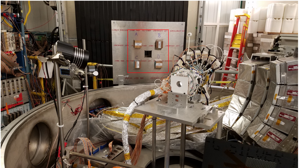
Figure 5.2 A photograph of the experimental setup with the shadow bars inserted. The four shadows are labeled as A, B, C, and D.
