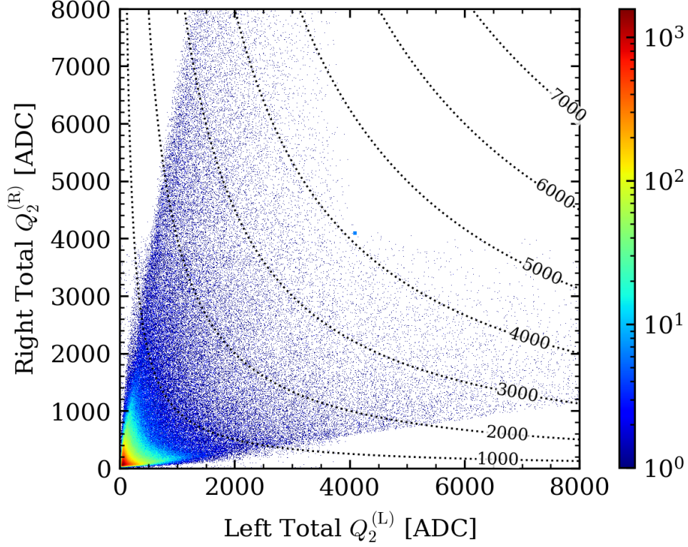
Figure 4.14 The left Total v.s. the right Total for NWB bar 12 from run 4224 to run 4245, inclusively, after non-linearity and saturation corrections.
