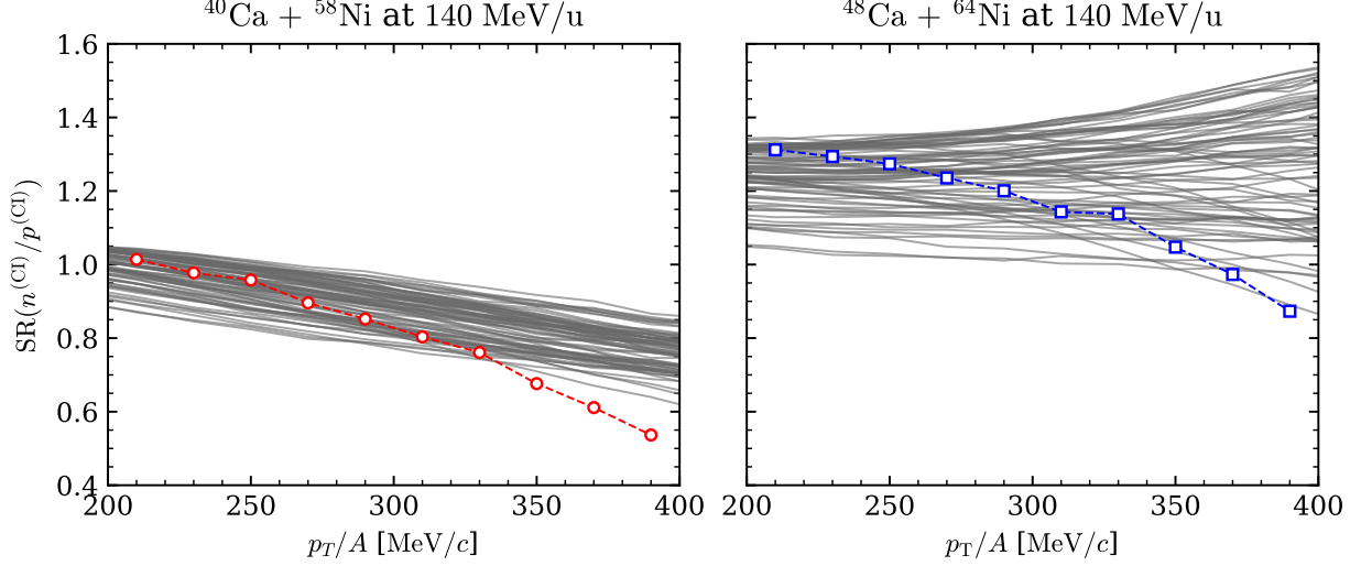
Figure 3.17 Coalescence-invariant (CI) n/p single ratios. The data points are the experimental data, replotted from Figure 3.15. The gray lines behind the data points consist of 75 single ratio spectra from ImQMD used to train the GP emulator.
