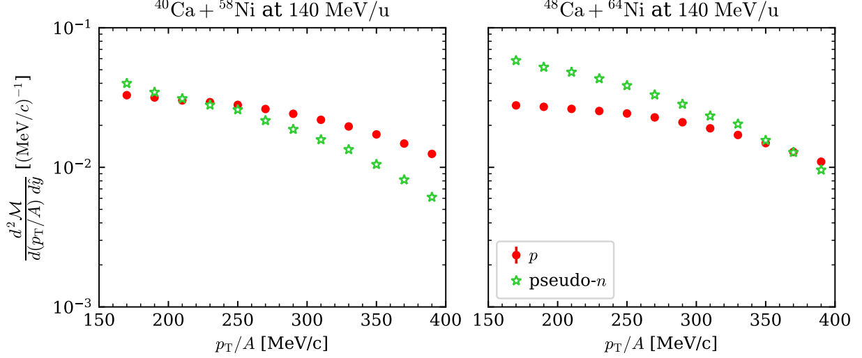
Figure 3.14 The pseudo-neutron spectra from the two Ca + Ni systems at 140 MeV/u.
