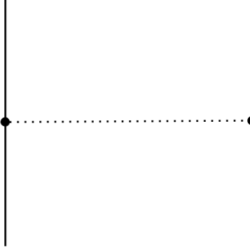
Figure 2.5 The general diagram for a two-body interaction
