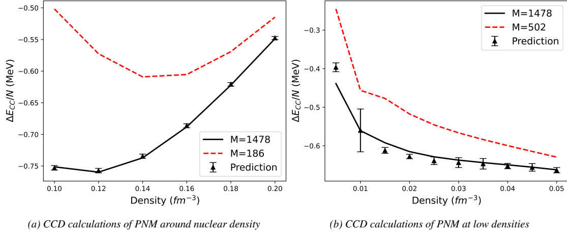
Figure 8.4 The results from predicting the converged \Delta E_{CC}/N for pure neutron matter using the coupled cluster doubles approximation. Figure (a) shows pure neutron matter for a range of densities around nuclear density ( 0.10 \leq d \leq 0.20 ), and figure (b) shows the results for a low-density pure neutron matter ( d \leq 0.05 ). For both graphs, the solid black line plots the fully converged \Delta E_{CCD}/N , calculated at 1,478 single-particle states; the triangular markers represent the SRE predictions at each density of interest. The dashed red lines represent the point used to train the GP algorithms with the highest number of single-particle states ( M=186 for Figure (a) and M=502 for Figure (b)) to show that the training set has not reached convergence
