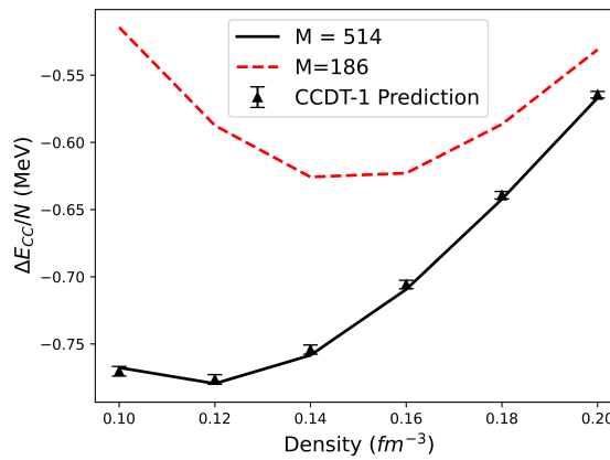
Figure 8.9 The results from predicting the converged \Delta E_{\text{CCDT1}}/N for pure neutron matter at densities around nuclear density. The average percent error across all densities is 0.45%, and the time savings from generating only the training data versus the fully converged \Delta E_{\text{CCDT1}}/N is 917.30 node hours
