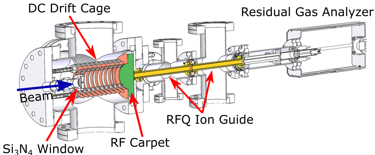
Figure 4.2: A 3D cross-section of the CIDGC prototype developed to perform CID of incoming high-energy molecular ions.
