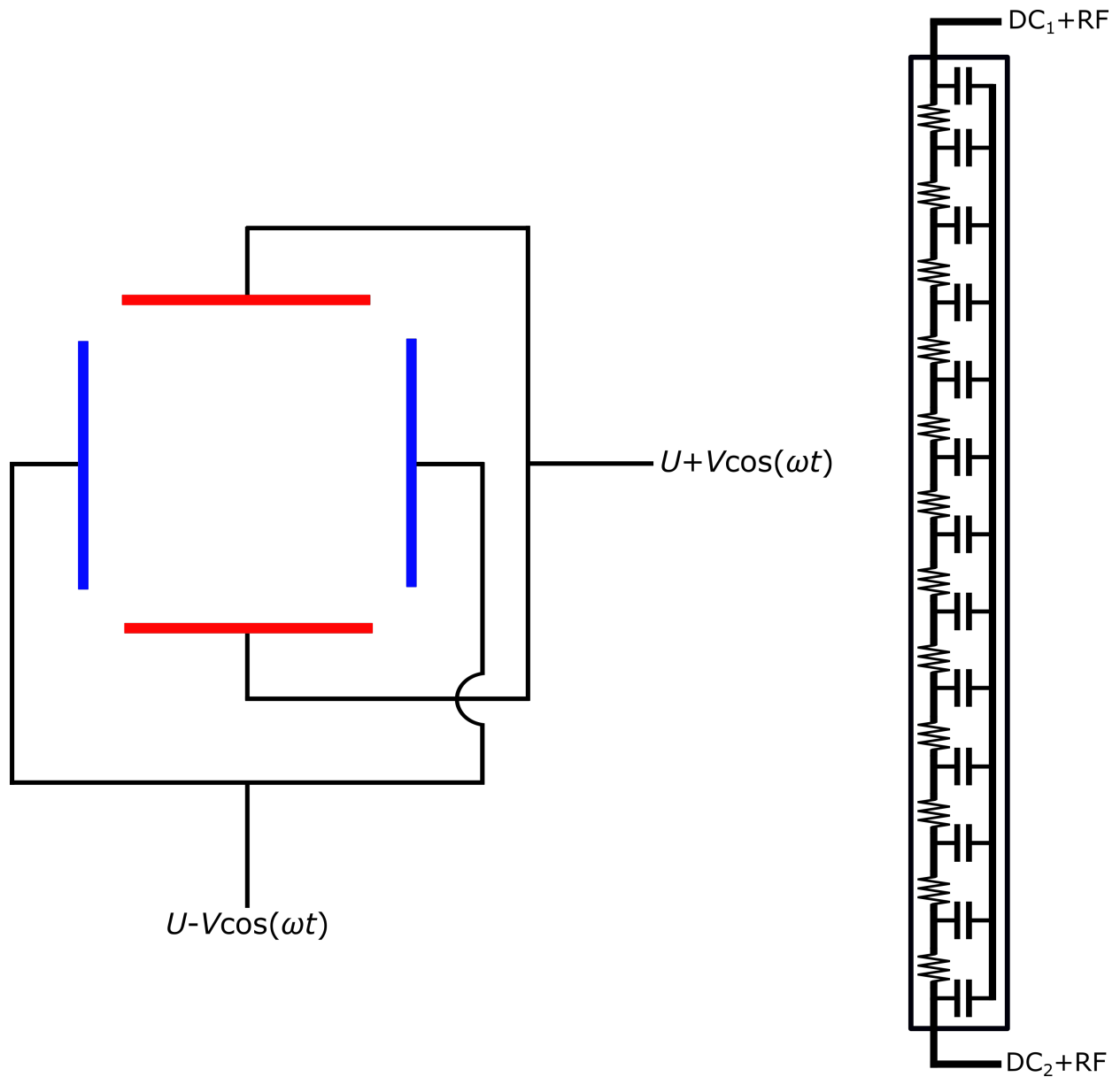
Figure 4.9: A conceptual drawing of the voltages applied to the RFQ and the circuit diagram for the segmented flat RFQ. U is the DC potential applied across the length of the RFQ, V is the RF amplitude and \omega is the angular RF frequency. Your DC_1 + RF and DC_2 + RF connections should connect to the resistors, not to the capacitors.
