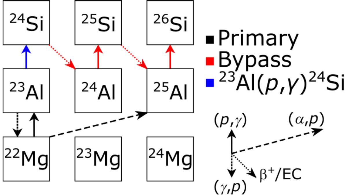
Figure 3.2: The competition between the (\alpha, p) and rp process near the A=22 waiting point. The ^{22}\text{Mg} waiting point forms an equilibrium of proton capture and photodisintegrations due to the low Q value of the reaction.
