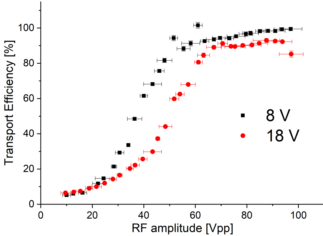
Figure 4.23: The dependence of the push plate voltage on the transport efficiency of the RF carpet. Higher push plate values translate into higher RF amplitudes necessary to transport the ions to the extraction orifice. The measurements were performed at 3 MHz with a current of 1.5 nA at 1 mbar.
