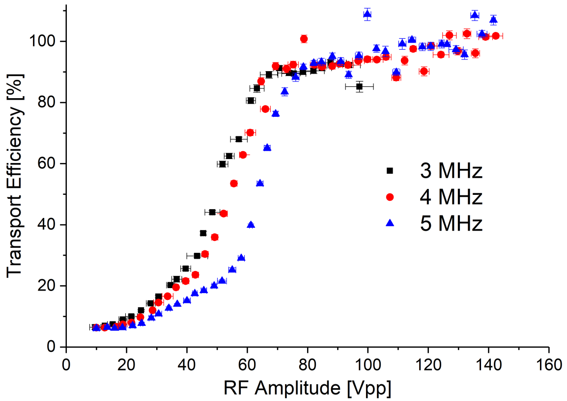
Figure 4.24: Transport efficiency measurements performed with the circular RF carpet at a pressure of 1 mbar and a current of 1.5 nA. The efficiency needed to transport ions shows a frequency dependence, with 3 MHz being more efficient than 5 MHz.
