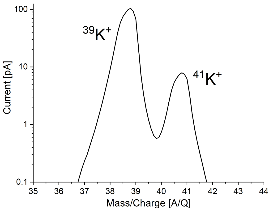
Figure 4.27: The spectrum produced using the RGA in the mass filtering mode. Both peaks for the isotopes of Potassium can be found, and the results match the natural abundance ratio observed in the spectrum. The RGA was operated at 1 \times 10^{-3} mbar with the gas cell at 2.5 mbar.
