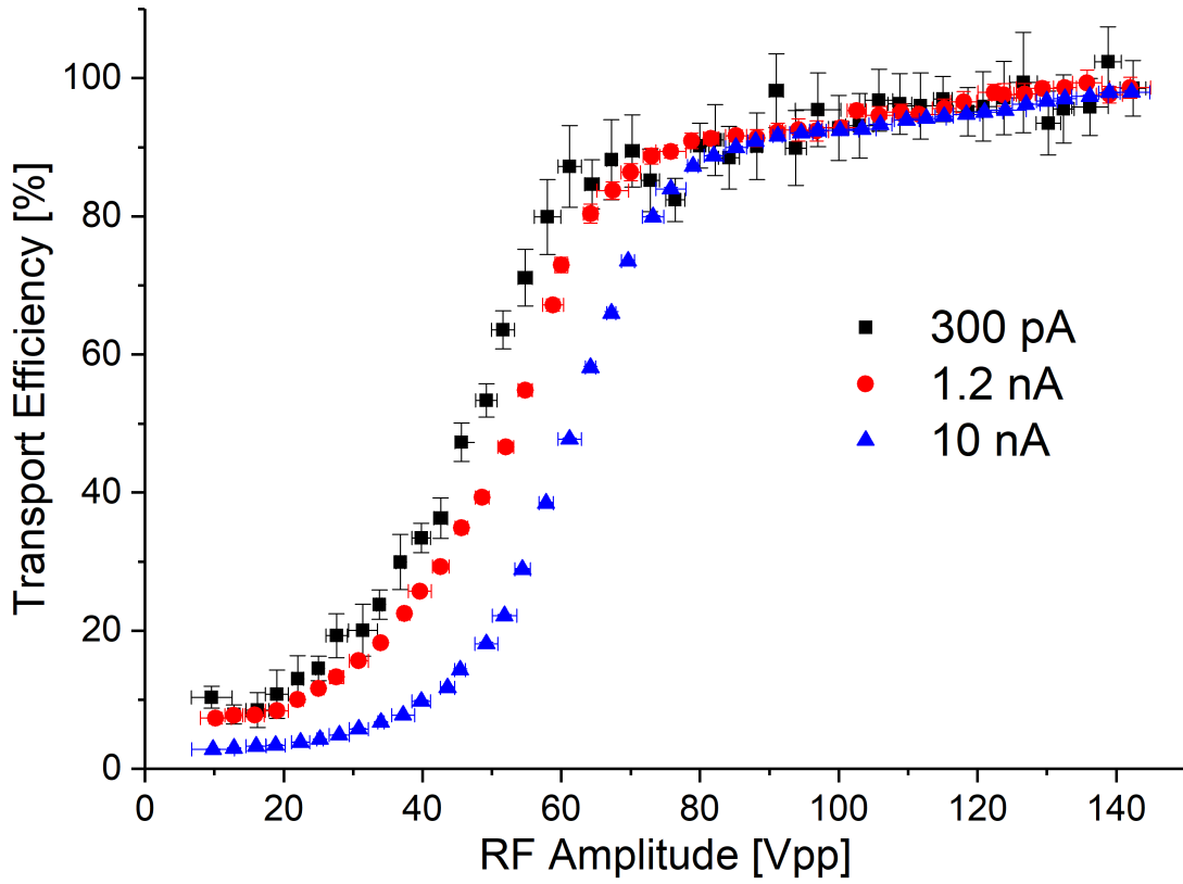
Figure 4.25: The transport efficiency as a function of RF amplitude for different incoming currents to investigate the role of space charge. The carpet was operated at 3 MHz at a pressure of 2.5 mbar. The offset observed at lower currents results from a measured current of ions that pass directly through the orifice without surfing.
