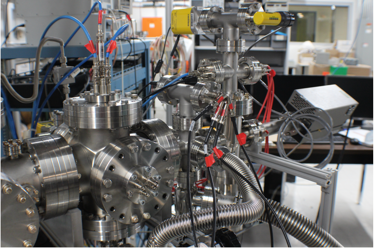
Figure 4.12: The complete CIDGC installed at the end of the first port in the d-line extension. The gas cell, two RFQ sections and the Residual Gas Analyzer. Vacuum gauges are also observable, as well as the wires that connect to DC power supplies and the RF driver circuits.
