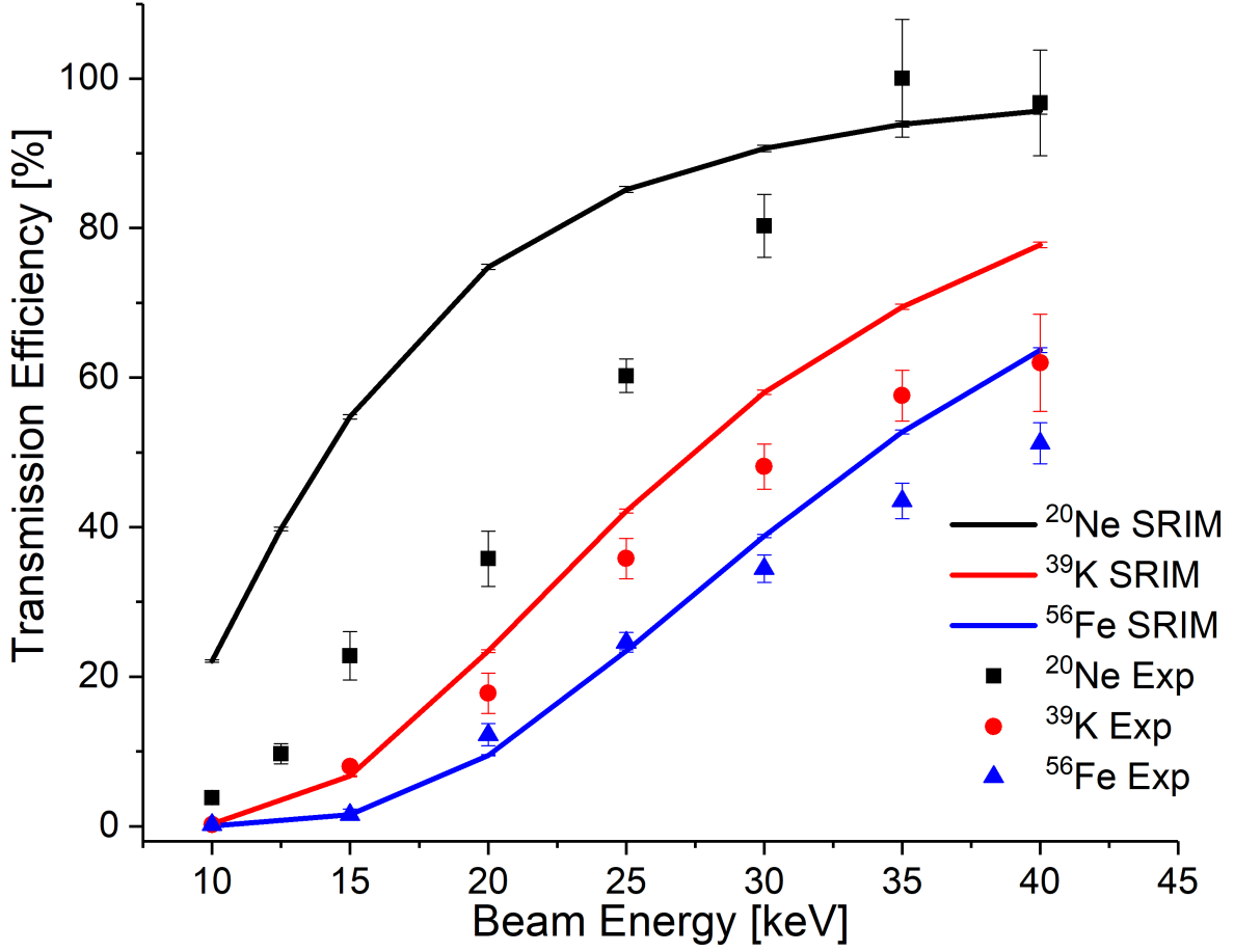
Figure 4.20: Scaled transmission efficiencies for different species delivered from BMIS with the simulated data calculated from SRIM. The ^{20}\text{Ne}^+ data shows a plateau beginning at 35 keV while ^{39}\text{K}^+ and ^{56}\text{Fe}^+ continue to increase. The experimental data follows a similar trend to the output from SRIM but does not agree perfectly.
