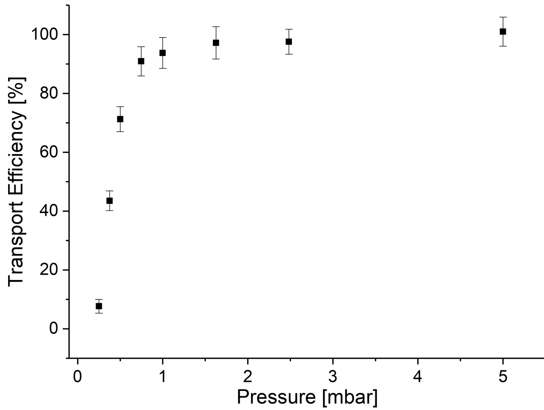
Figure 4.22: The transport efficiency as a function of the pressure for 4-phase ion surfing. The RF carpet was operated at 3 MHz with an amplitude of 90 V pp at a current of 150 pA.
