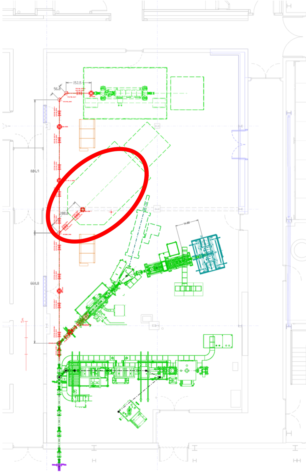
Figure 4.3: An overview of the low-energy area (LEBIT and BECOLA) and the d-line extension. The parts of the beam line colored red represent the d-line extension. The red-bordered ellipse highlights where the location of the CIDGC prototype is installed.
