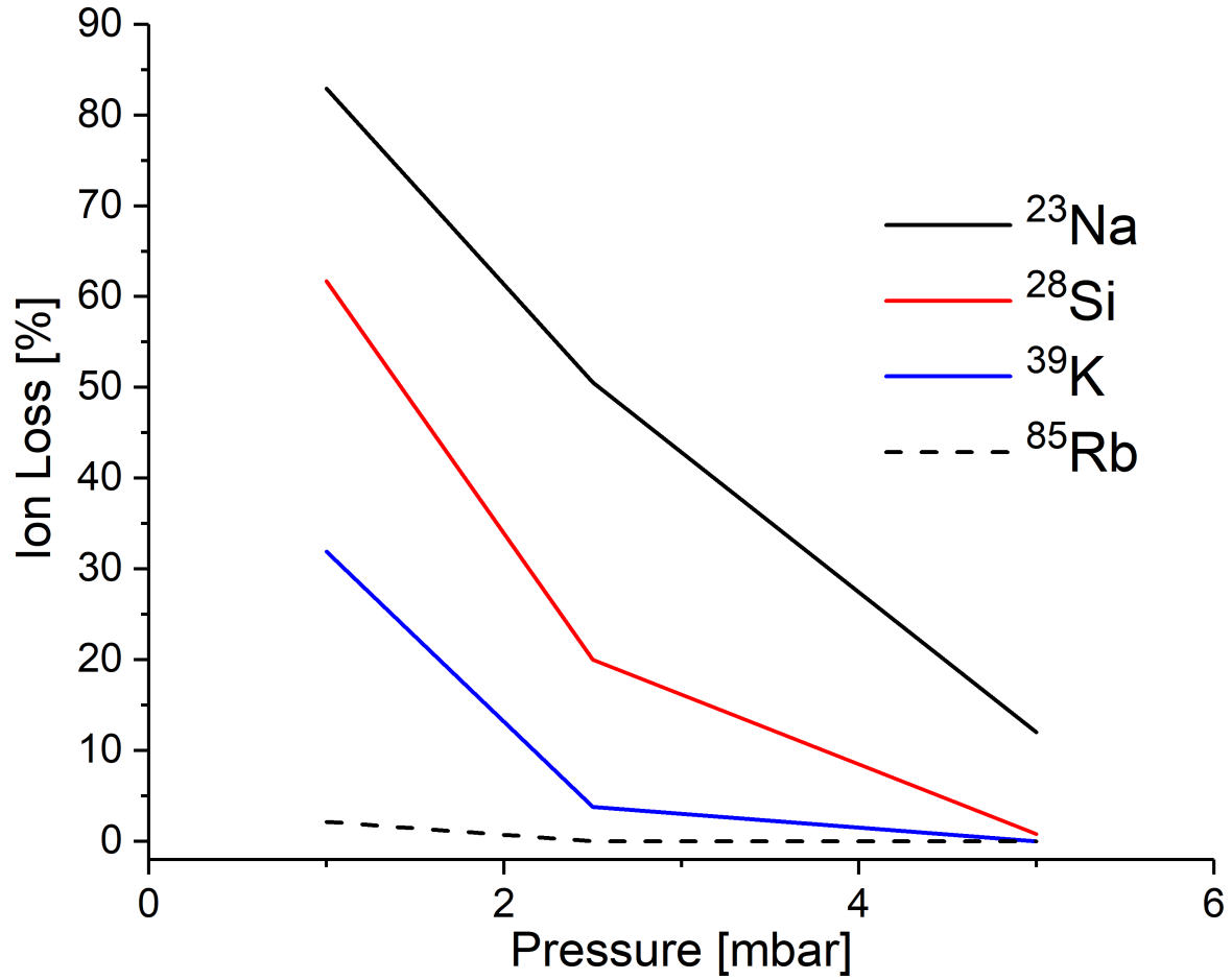
Figure 4.15: The ion losses as a function of pressure from simulated ions after transmitting through 21 nm of \text{Si}_3\text{N}_4 and getting stopped in He gas. The losses were defined as the ratio of ions that are stopped beyond the dimensions of the inner diameter of the ring electrodes and the length of the cell between the \text{Si}_3\text{N}_4 membrane and the RF carpet to the total number of ions generated.
