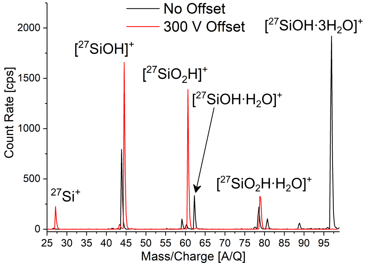
Figure 3.4: A mass scan performed for ^{27}\text{Si} , which saw radioactivity at A = 44, 60, 62, 78, and 98 . After putting a 300\text{ V} offset between the gas cell nozzle and extraction RFQ, the mass scan consolidates the ion of interest to A = 27, 44 and 60 .
