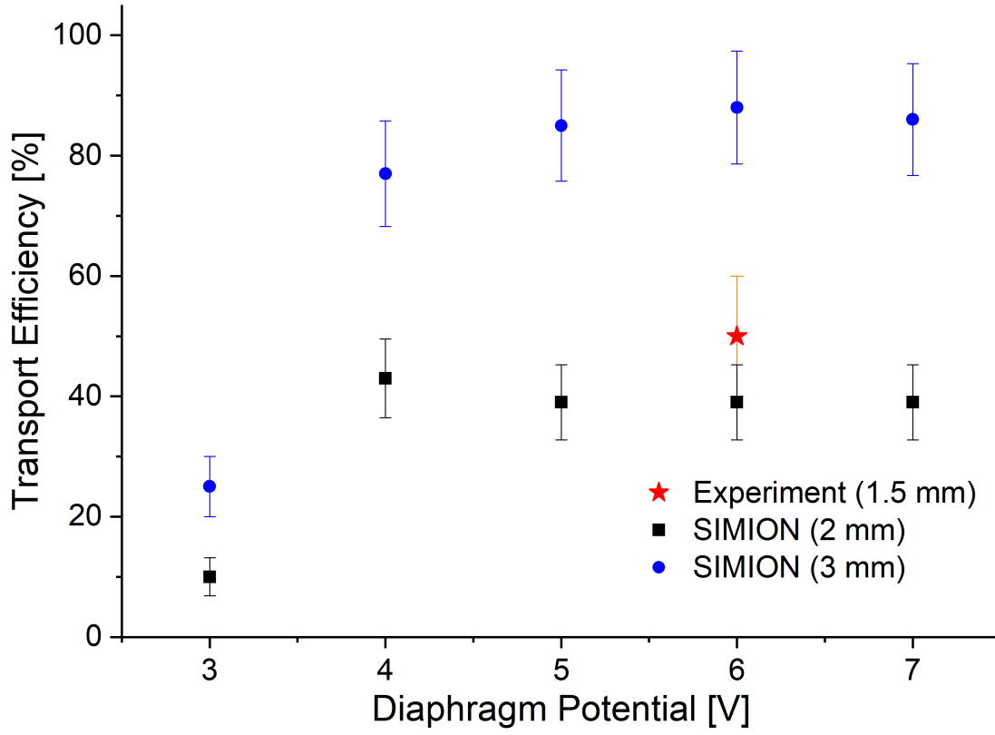
Figure 4.26: Diaphragm potential studies performed using ^{39}\text{K}^+ , with the RFQs operating at 1.2 MHz to understand the impact of the orifice diameter and diaphragm potential on ion transport. Good agreement between experimental data and simulated results was observed.
