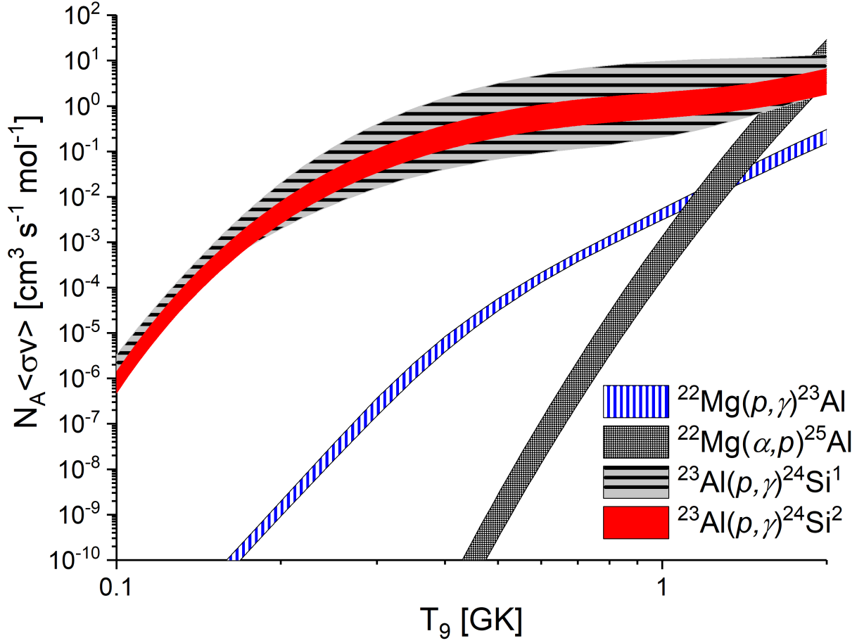
Figure 3.7: The reaction rates for ^{23}\text{Al}(p, \gamma)^{24}\text{Si} (Wolf et al. 2019 [1], denoted by the superscript 1, and this work, denoted by the superscript 2), ^{22}\text{Mg}(p, \gamma)^{23}\text{Al} (Iliadis et al. 2010, [28]) and ^{22}\text{Mg}(\alpha, p)^{25}\text{Al} (Randhawa et al. 2020, [29]) from 0.1 to 2 GK. Our calculations show a dramatic reduction in the 1- \sigma reaction rate uncertainty for ^{23}\text{Al}(p, \gamma)^{24}\text{Si} as a result of our new mass measurement and the corresponding resonance energies.
