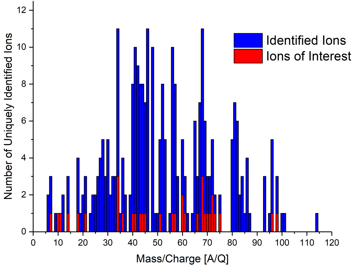
Figure 1.2: A hisotgram of ions that have been identified using PTMS after the LEBIT facility was recommissioned with beam from the beam stop facility in 2013 [9]. The height of each peak represents how many ions were identified at a particular A/Q using PTMS. Ions of interest often came either as a bare isotope or a molecular ion, either singly or doubly charged. The red represents the ions that were measured and published via References [4,10–22]. The histogram illustrates the potentially damaging impact contaminant ions can have during precision measurement campaigns.
