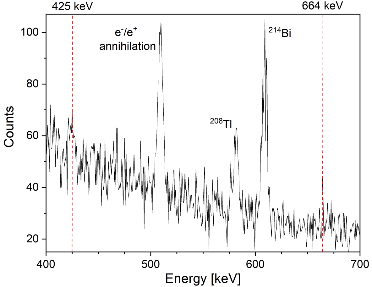
Figure 3.3: The \gamma -rays that were measured using a high-purity germanium detector. Two low energy \beta -delayed \gamma -rays were identified at E = 425 and 664 keV. Since the count rates were so low, seeing their signature was necessary for verifying ^{24}\text{Si} was present in the beam during a mass measurement.
