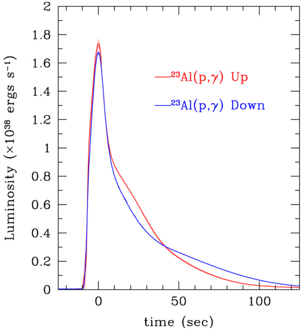
Figure 3.1: A multi-zone X-ray burst model light curve simulation while varying the ^{23}\text{Al}(p, \gamma)^{24}\text{Si} reaction up and down between a factor of 30 to 100. The variation factor depended on temperature and the resonant uncertainty known at the time. The line width of the simulations represents a 1\sigma uncertainty of the light curve. The figure was adapted from [24].
