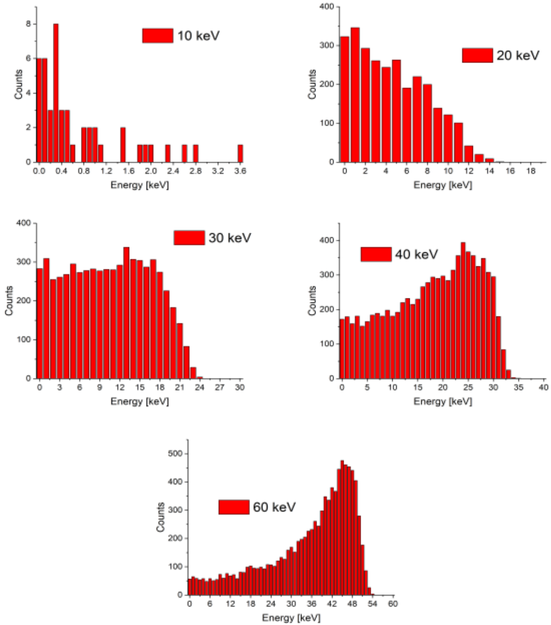
Figure 4.16: The energy distributions of ^{39}\text{K}^+ ions generated and transmitted through a 20 nm thick \text{Si}_3\text{N}_4 membrane. As the energy of the incoming beam increases, the energy distribution of ions changes from a Poisson-like to a skewed Gaussian-like distribution. This data highlights the amount of energy deposited into the \text{Si}_3\text{N}_4 membrane during transmission.
