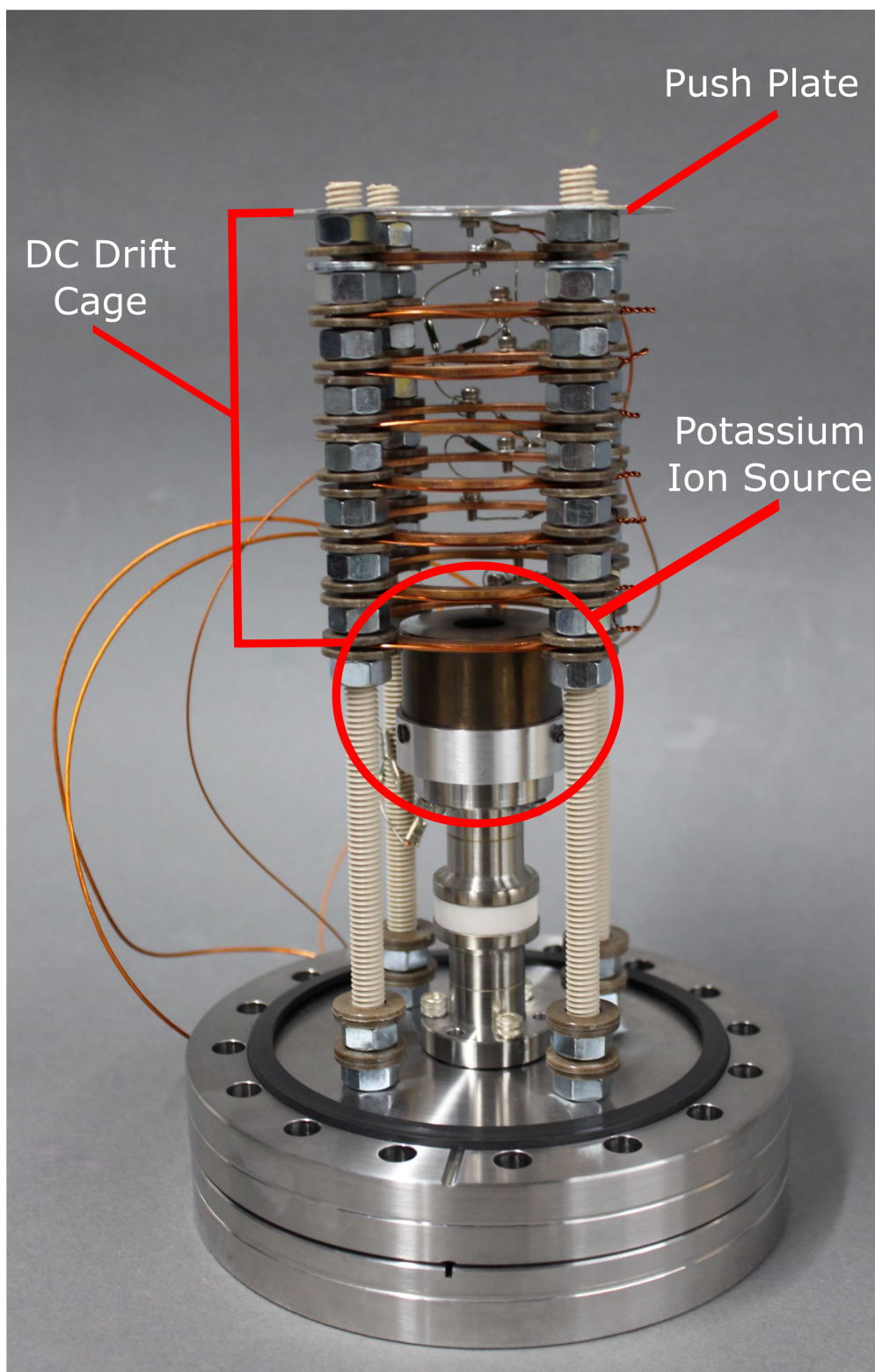
Figure 4.21: The internal structure of the gas cell that was configured for characterizing the CIDGC using a ^{39}\text{K} ion source.
