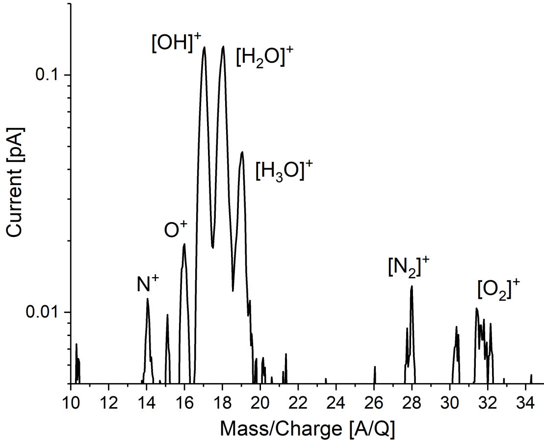
Figure 4.28: Mass spectrum of ions extracted from the stopping cell measured in the RGA with online ^{39}\text{K}^+ beam from BMIS injected into CIDGC. Only major contaminants could be observed, such as water, oxygen and nitrogen.
