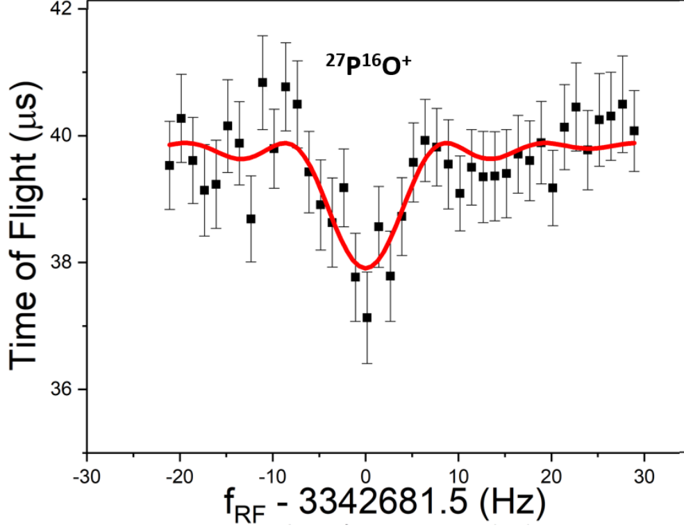
Figure 2.4: Sample 100 ms continuous quadrupolar excitation TOF-ICR resonance of ^{27}\text{PO}^+ obtained by scanning f_{rf} applied to ^{27}\text{PO}^+ ions prepared with pure initial magnetron motion and measuring time of flight between the Penning trap and an MCP detector. The theoretical fit (red) is calculated in [1]. The minimum corresponds to the cyclotron frequency f_c .
