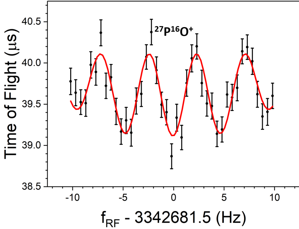
Figure 2.5: Sample 250 ms Ramsey resonance of ^{27}\text{PO}^+ . Instead of a continuous 250 ms excitation, an excitation scheme of 50 ms RF, 150 ms free evolution, 50 ms RF was applied to generate the above interference pattern. The above theoretical fit (red), and fits for other complex schemes are described in [30]. The central ToF minimum corresponds to the cyclotron frequency f_c .
