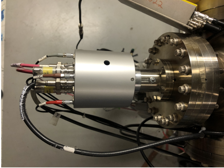
Figure A.4: The FT12TP vacuum feethrough and connector plug. A screw and pair of washers have been mounted on the right, just before the flange to keep the plug more stable. There is an identical screw and washer pair 180^\circ away on the bottom side with the same function.
