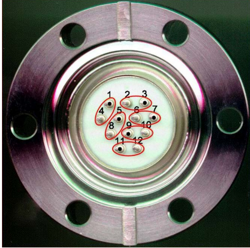
Figure A.3: Pinout for the vacuum side of the FT12TP. On the air side the pin numbers will be mirrored (e.g. top left pin is #3). Red ovals mark the pins for twisted cable pairs
