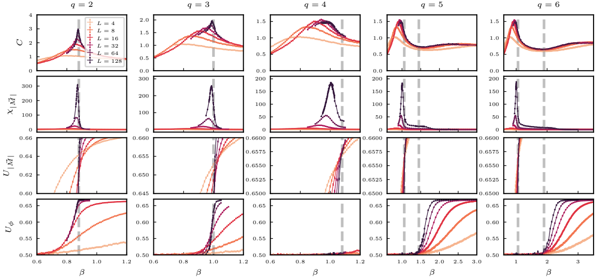
Figure 4.51 As in Fig. 4.50 but with h_q = 0.1 .
