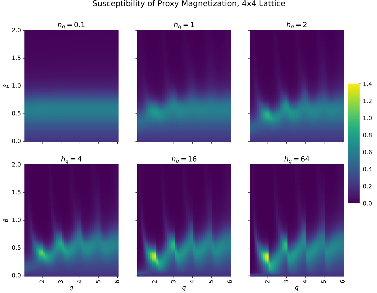
Figure 4.37 Here we show a heatmap of the susceptibility of the proxy magnetization obtained via Monte Carlo on a 4 \times 4 lattice. Each panel shows the result at a different value of the symmetry-breaking parameter h_q . Note that each pixel corresponds to a distinct MCMC simulation.
