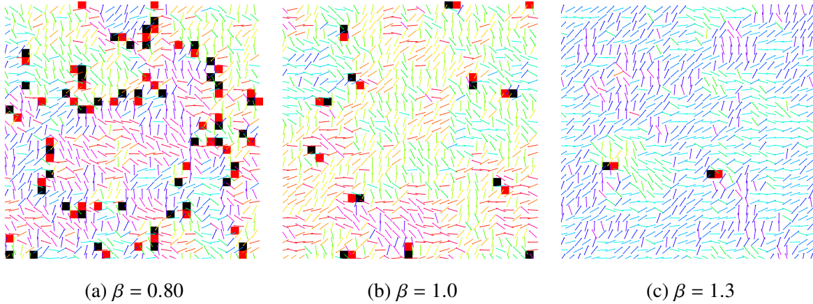
Figure 2.10 A few examples of equilibrium vortices from independent Monte Carlo simulations of the XY model performed on 32 \times 32 lattices with periodic boundary conditions. Vortex positions are identified by computing the winding number Eq. (2.42) of each plaquette. A winding number of +1 corresponds to a vortex, and a winding number of -1 corresponds to an antivortex. In panel (a), an equilibrium configuration is shown for \beta = 0.8 , which is in the disordered phase. The vortex-antivortex pair density is high and many are unbound. Panel (b) comes from a simulation performed at \beta = 1.0 , which is not far from the critical point of the XY model. Panel (c) shows an equilibrium configuration at \beta = 1.3 , which is in the quasi-ordered phase. Here the vortex-antivortex pair density is small, and they are tightly bound.
