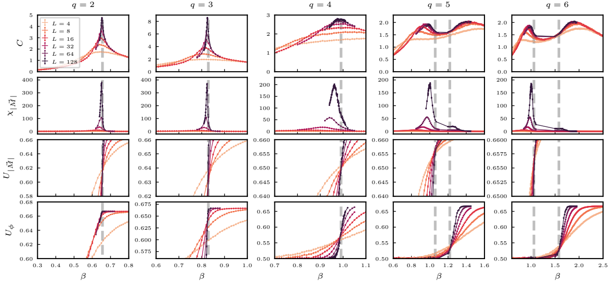
Figure 4.50 Here, we show the specific heat (top row), magnetic susceptibility (second row), Binder cumulant (third row), and the Binder cumulant of the rotated magnetization (bottom row). From left to right, the columns correspond to q = 2, 3, 4, 5, 6 . In all cases, h_q = 1 . The different color shades correspond to different lattice sizes ranging from L = 4 (light) to L = 128 (dark). Connecting lines are added to help guide the eyes. The vertical dashed gray lines show where the Binder cumulants intersect.
