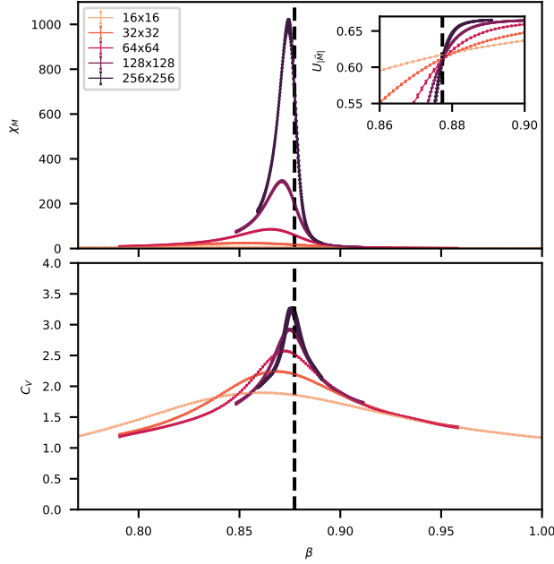
Figure 4.60 Here we look at data for some volumes ( L = 16, \dots, 256 ) for the model with q = 2 and h_q = 0.1 . The top panel shows the magnetic susceptibility, the bottom panel shows the specific heat, and the inset within the top panel shows the Binder cumulant. The data is from reweighted Monte Carlo with error bars included. The vertical dashed line is at \beta_c \approx 0.8773 where the Binder cumulant curves cross. This figure illustrates the behavior typical of a second-order phase transition—the Binder cumulants cross at the transition point, the magnetic susceptibility diverges, and the specific heat diverges logarithmically.
