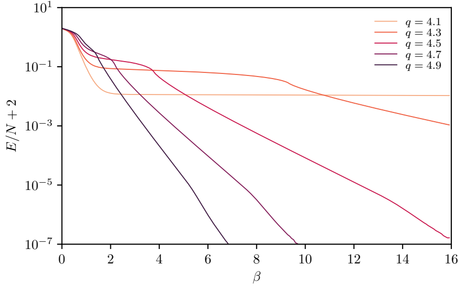
Figure 4.10 The energy density for the fractional- q -state clock model from TRG for q = 4.1, 4.3, 4.5, 4.7 , and 4.9 . These results were obtained with a volume 1024 \times 1024 . The energy is shifted vertically by 2 (to make it positive) and plotted on a log scale to better illustrate the difference between the curves.
