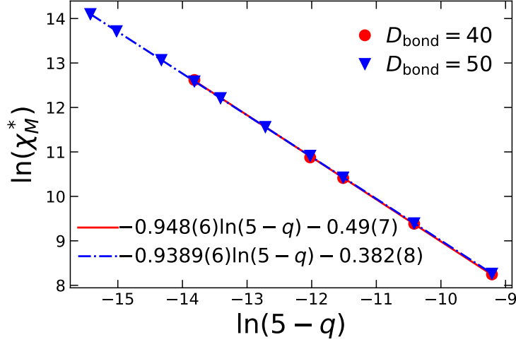
Figure 4.15 The log-log plot of the maximal value of the magnetic susceptibility \chi_M for the small- \beta peak as a function of 5 - q . The peak height diverges with a power law when q \rightarrow 5^- .
