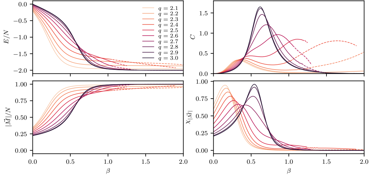
Figure 4.3 Monte Carlo results for the extended q -state clock model on a 4 \times 4 lattice for 2.1 \leq q \leq 3.0 . The top panel shows energy density and specific heat, and the bottom panel shows proxy magnetization and magnetic susceptibility. Statistical error bars are omitted since they are smaller than the line thickness. Dashed lines indicate regions where we have data but we do not have the uncertainty fully under control.
