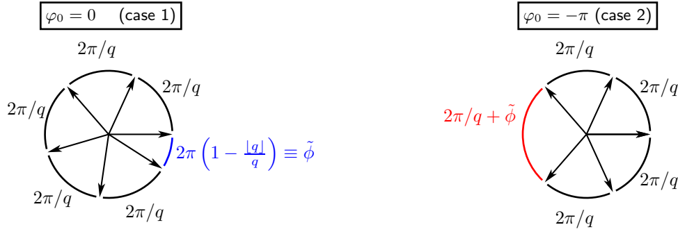
Figure 4.1 Arrows indicate the allowed spin orientations for the extended q -state clock model with the choice \varphi_0 = 0 (left) and \varphi_0 = -\pi (right). In this example, q = 5.5 . Blue and red denote the leftover angles in the two cases. See Eq. (4.8).
