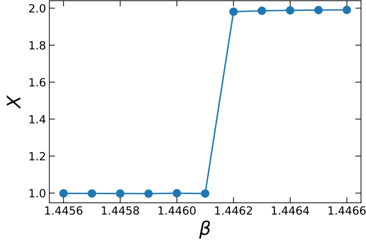
Figure 4.23 The \beta dependence of X , defined in Eq. (4.38), from the fixed point tensor for q = 4.9 . The discontinuity is located between 1.4461 and 1.4462, consistent with the result from the extrapolation of the peak position of \chi_M to zero external field in Fig. 4.22. The tensor bond dimension is 40.
