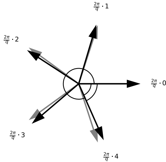
Figure 4.53 The clock angles for q = 5.0 (gray) and q = 4.9 (black). For q = 5 , there are five equidistant angles which divide the unit circle into five equal sectors. For q = 4.9 , there are again five angles, but the \mathbb{Z}_5 symmetry is broken. Now there are four equal sectors and one slightly smaller “leftover” sector.
