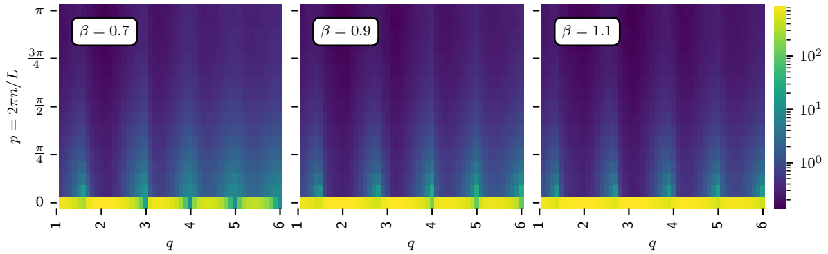
Figure 4.48 Heatmaps of the structure factor F(p) with momenta p on the vertical axis and with q on the horizontal axis. The different panels correspond to different \beta with \beta = 0.7, 0.9, 1.1 from left to right. These results are from 32 \times 32 lattices with h_q = 1 and are from the model where \beta is treated as a coupling. Note that each pixel corresponds to a distinct MCMC simulation.
