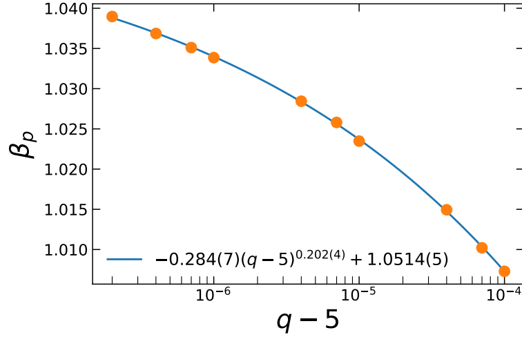
Figure 4.31 Same as Fig. 4.17, but for \varphi_0 = -\pi , q \rightarrow 5^+ . D_{\text{bond}} = 50 .
