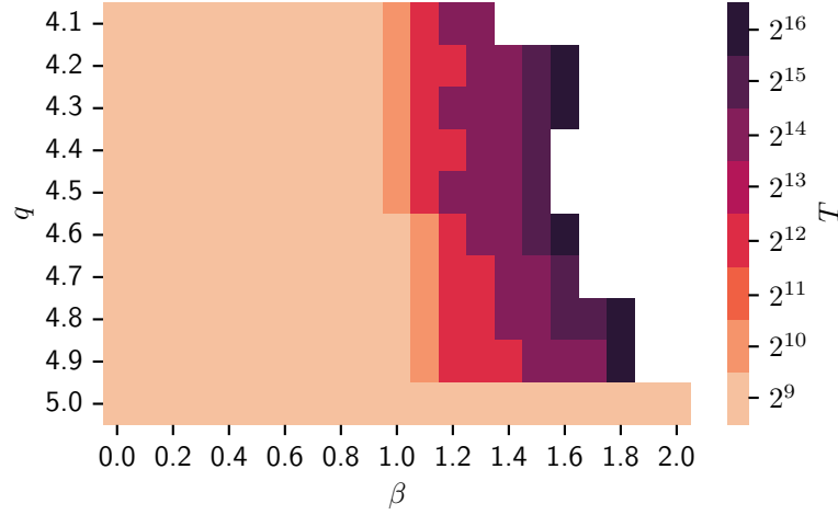
Figure 4.9 The values of T defined in Eq. (4.17) needed to extract the integrated autocorrelation times shown in Fig. 4.8. The vertical axis gives the values of q and the horizontal axis gives the values of \beta . Blank/white regions in this heatmap indicate cases where T > 2^{16} is needed to get a reliable estimate of the integrated autocorrelation time. These were not attempted due to the computational cost.
