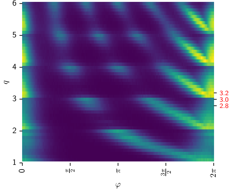
Figure 4.47 Heatmaps of the angle histograms for constant \beta = 1 and varying q \in [1.1, 6.0] . Results are from 4 \times 4 lattices with h_q = 1 . The red labels on the right edge correspond to the q -values shown in Fig. 4.45. Note that each pixel corresponds to a distinct MCMC simulation.
