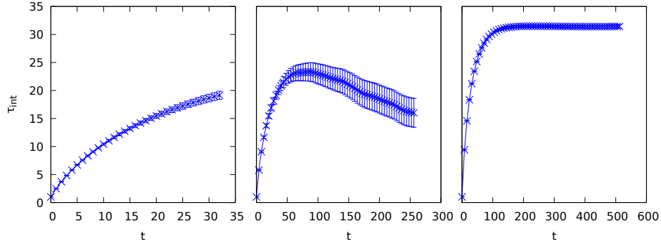
Figure 3.2 Here we show the integrated autocorrelation curve of the energy for the Ising model on a 16 \times 16 lattice near the critical point calculated from a time series of 2^{16} heatbath sweeps with one measurement per sweep. The integrated autocorrelations are estimated using Eq. (3.31), and we are trying to find the maximum/plateau value. In the left panel, the time extent T = 32 is clearly insufficient to resolve the plateau. In the middle panel, we increased T and located a peak which gives an estimate of the integrated autocorrelation time. However, in this case we have large error bars and don't have a nice plateau, which indicates that our data was generated with insufficient statistics to accurately resolve the integrated autocorrelation time. In the final panel, we increased the statistics of the simulation by a factor of 256 to 2^{24} heatbath sweeps, and we increased T to 512. Now we see a nice plateau with small error bars. In many practical examples, it would be difficult to get sufficient statistics to resolve the plateau this well and one might be forced to estimate the integrated autocorrelation time from plots more like the middle one.
