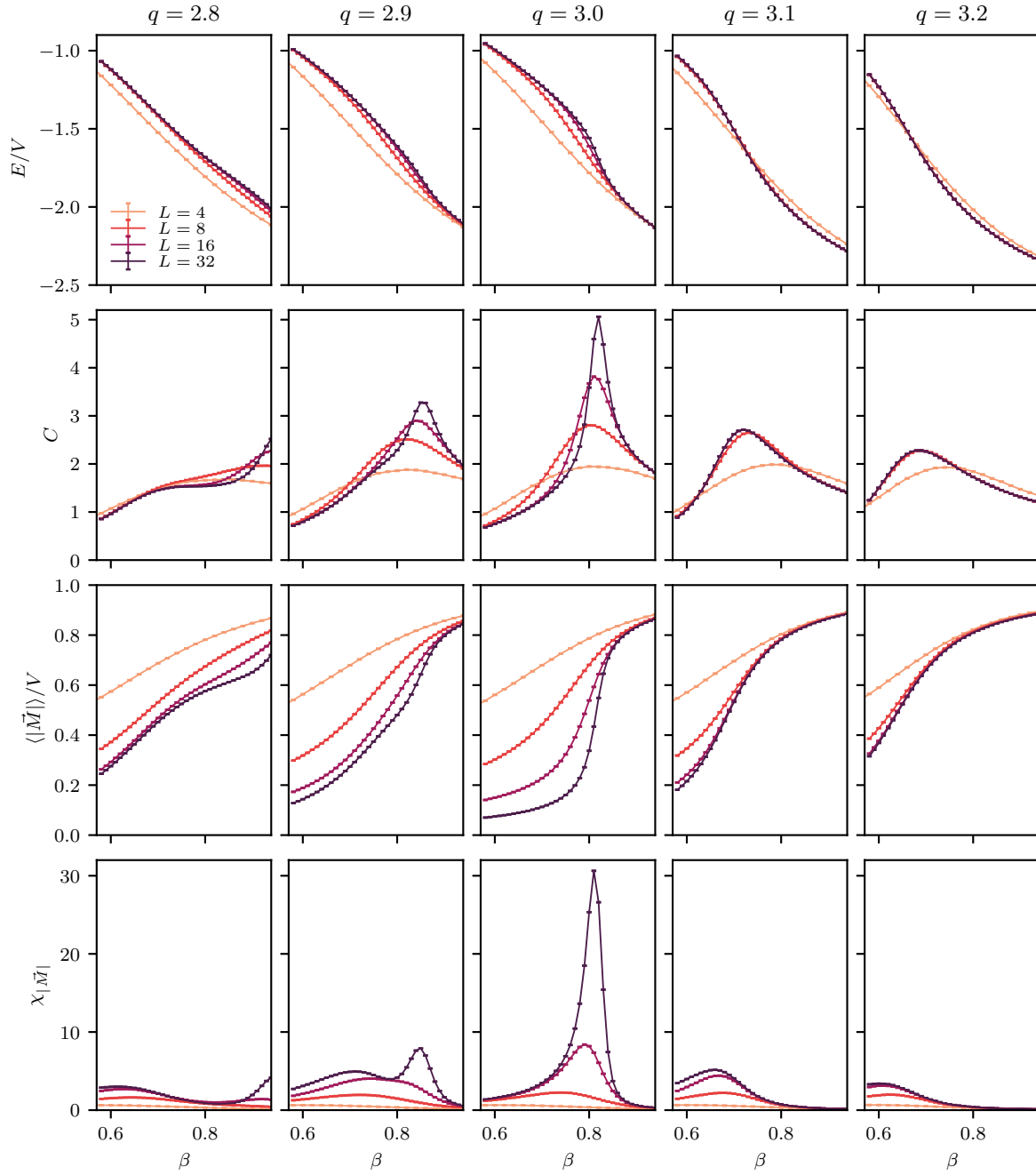
Figure 4.43 From left to right, the columns correspond to q = 2.8, 2.9, 3.0, 3.1, 3.2 . From top to bottom, the rows illustrate the energy density, specific heat, proxy magnetization, and susceptibility of the proxy magnetization. The different colors correspond to the different lattice sizes L = 4, 8, 16, 32 . Connecting lines are drawn to help guide the eyes. For q = 2.8 and 2.9 we see evidence of a crossover at smaller \beta and a phase transition at larger \beta . For q = 3.0 , there is only a phase transition, and for q = 3.1 and 3.2 we see only a crossover for the illustrated \beta range.
