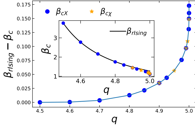
Figure 4.26 The difference between the critical point of the rescaled Ising model \beta_{rIsing} and the true critical point \beta_c for fractional- q -state clock models as a function of q . The circles are from the discontinuity of values of X , \beta_{cX} , the stars are from the extrapolations of the peak position of \chi_M to zero external field, \beta_{c\chi} . The inset shows the values of the true critical point as a function of q and the solid line is Eq. (4.40).
