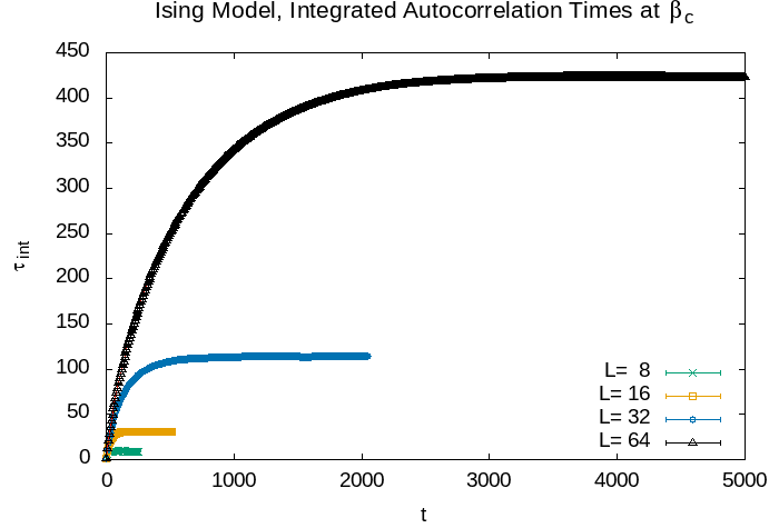
Figure 3.1 Plots of the integrated autocorrelation curve of the energy for the two-dimensional Ising model at four different lattice sizes. Each simulation is performed at the critical point \beta_c using a heatbath algorithm. The curves are computed using Eq. (3.31), and the plateau value gives the estimate of the integrated autocorrelation time \tau_{int} . Notice that \tau_{int} grows with lattice volume, and to obtain the plateau value, one must go to much larger values of t as the lattice size is increased.
