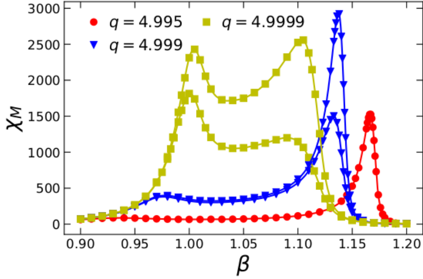
Figure 4.13 The magnetic susceptibility as a function of \beta at N = 2^{24} \times 2^{24} . For q = 4.995 , the external field is h = 4 \times 10^{-5} . For q = 4.999, 4.9999 , the external field is h = 4 \times 10^{-5} for the lower curve and h = 2 \times 10^{-5} for the upper curve.
