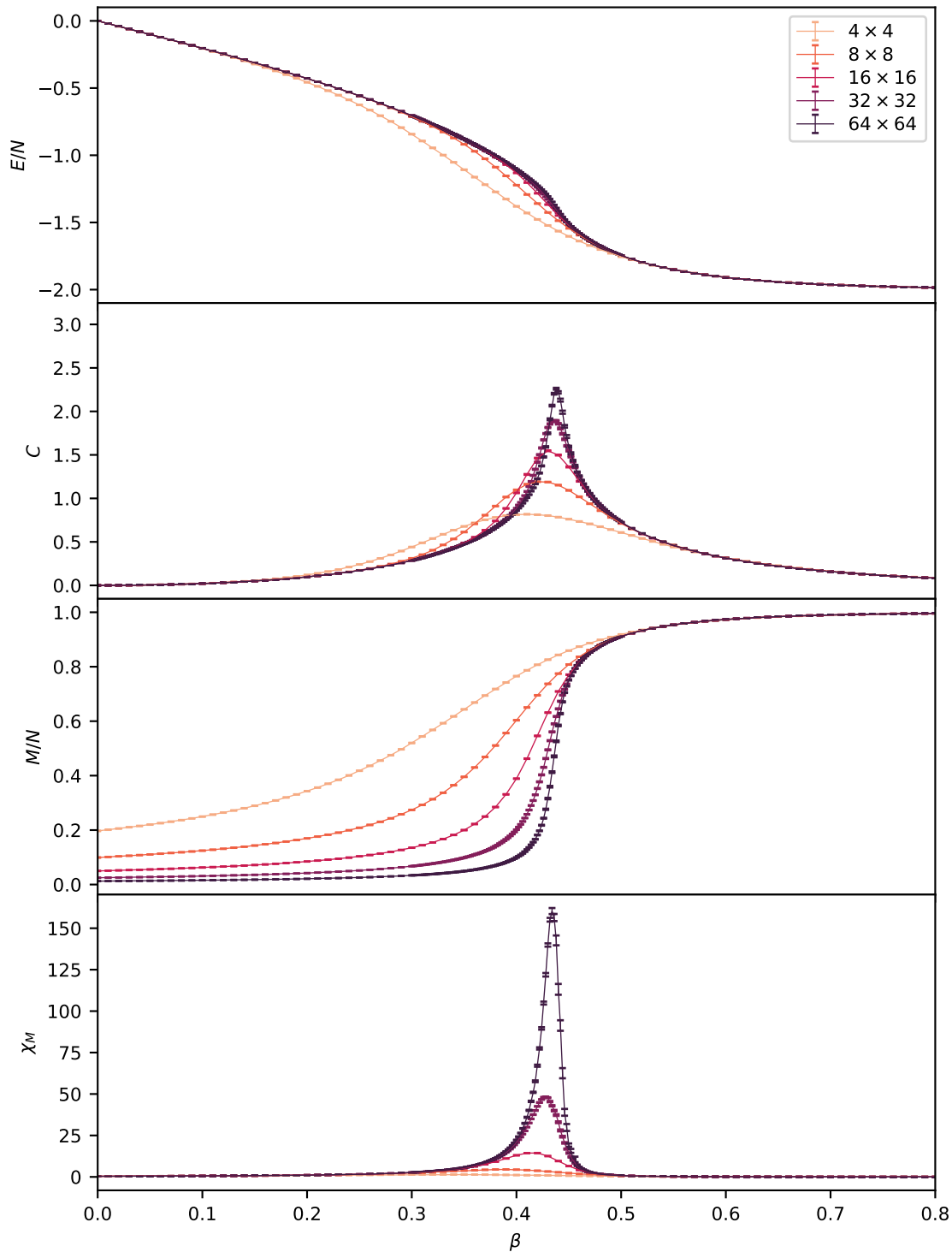
Figure 2.2 Here we show several thermodynamical functions versus \beta for the Ising model on several different lattice sizes. From top to bottom, we have the energy density, specific heat, magnetization per site, and the magnetic susceptibility. Notice how these functions behave near the critical point \beta_c = \ln(1 + \sqrt{2})/2 \approx 0.4407 where there is a second-order phase transition.
