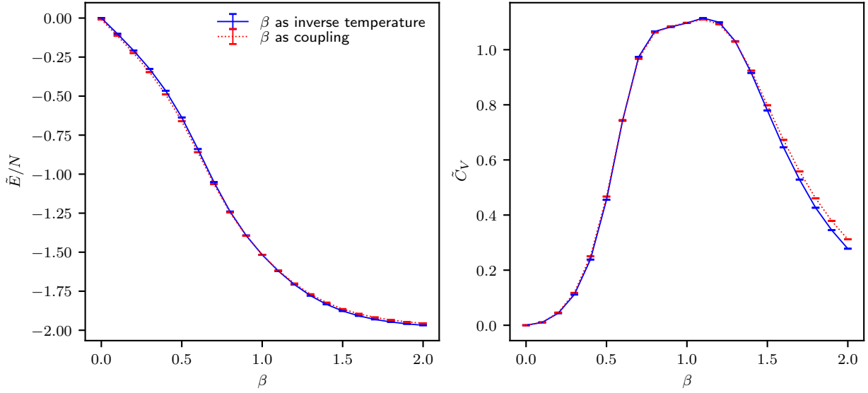
Figure 4.39 (Left) The interaction energy of the Extended-O(2) model with q = 4.9 and h_q = \tilde{h}_q = 5 on a 4 \times 4 lattice. (Right) The corresponding specific heat. The results in blue are from the model with \beta as the inverse temperature, and the results in red are from the model where \beta is treated as a coupling. The results coincide for \beta = 1 but differ slightly elsewhere. The connecting lines are only to guide the eyes.
