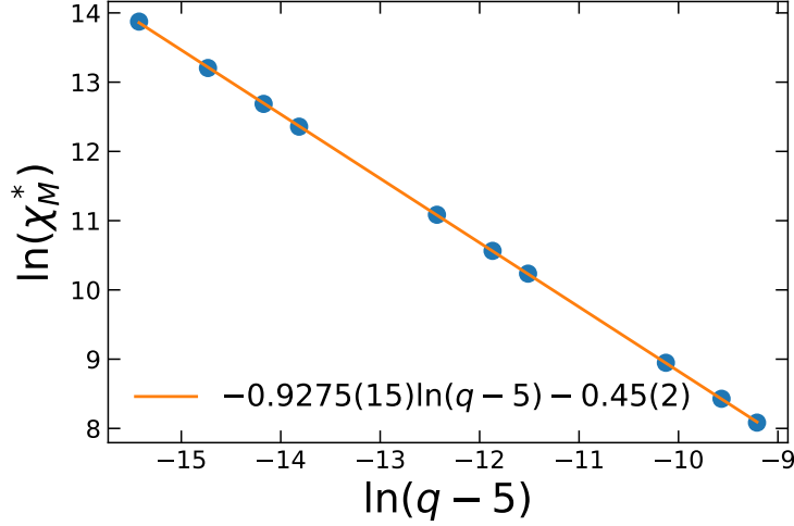
Figure 4.30 Same as Fig. 4.15, but for \varphi_0 = -\pi, q \rightarrow 5^+ . D_{\text{bond}} = 50 .
