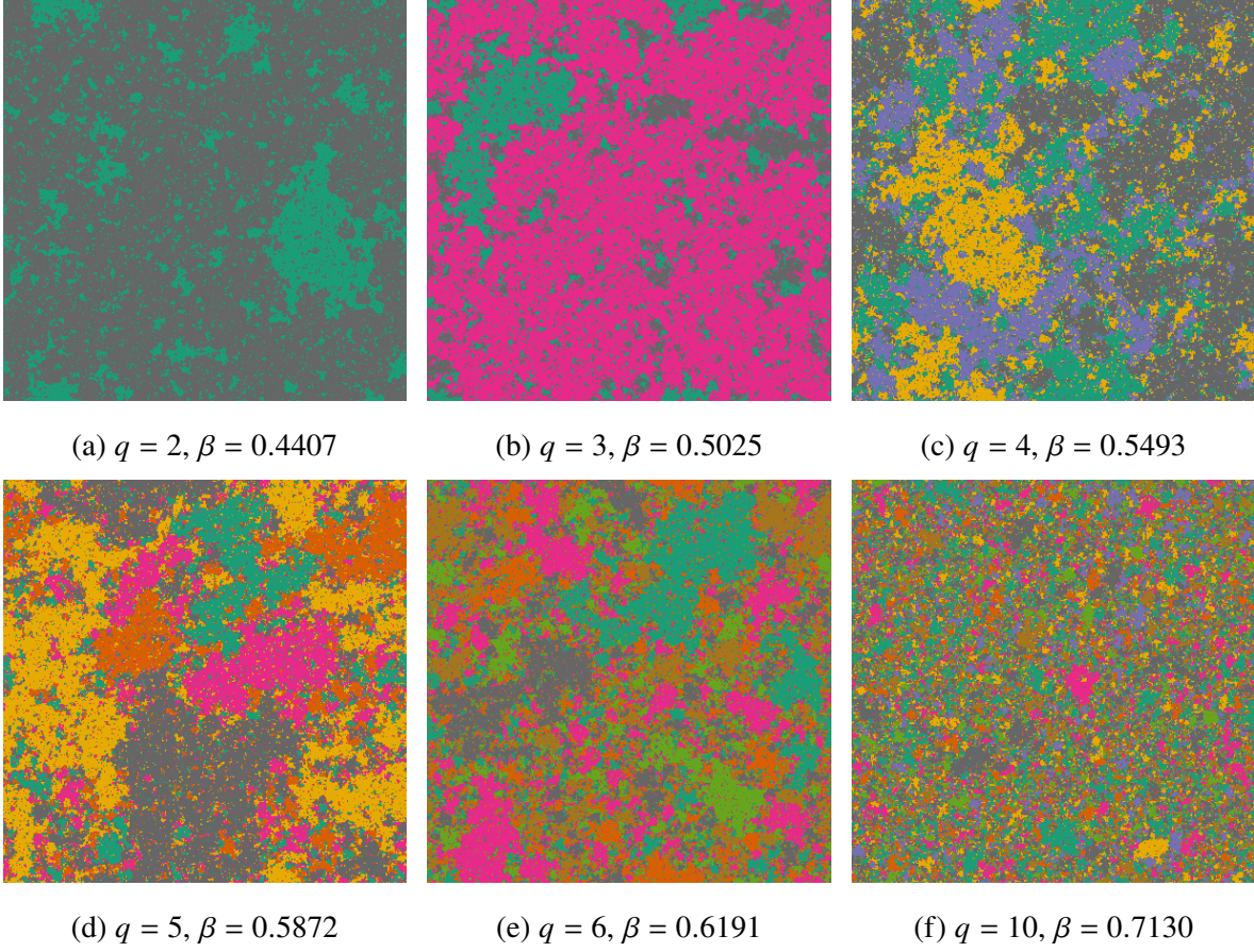
Figure 2.4 Example q -state Potts model configurations at different q from MCMC simulations performed on 400 \times 400 lattices near their critical points.
