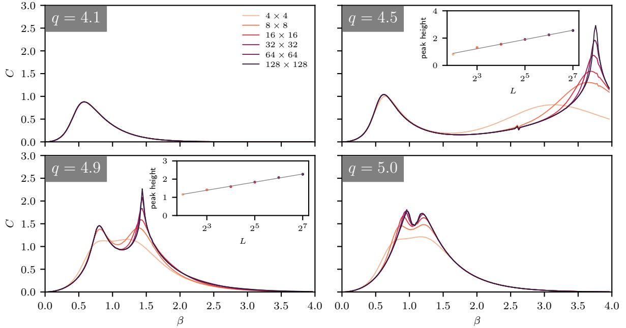
Figure 4.11 Specific heat of the extended q -state clock model from TRG for q = 4.1, 4.5, 4.9 , and 5.0 at volumes from 4 \times 4 up to 128 \times 128 . All vertical axes use a shared scale, and all horizontal axes use a shared scale. In general, there is a double-peak structure in the specific heat (for q = 4.1 , the second peak is at \beta \sim 75 ). Insets show the height of the second peak versus the linear system size L = \sqrt{N} plotted on a log scale, where the solid line is a linear fit.
