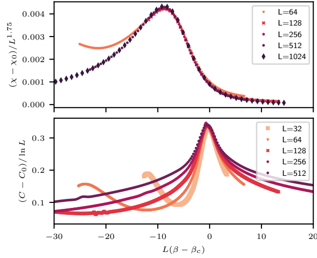
Figure 4.65 In the top panel, data collapse of the magnetic susceptibility from TRG for the large- \beta peak for the model with q = 3.9 and h_q = 1 . The estimate \beta_c = 1.196 was obtained by fitting the peak positions to the finite-size scaling form Eq. (3.78). To extract the magnetic susceptibility, an external field h = 40/L^{15/8} was imposed ( dh = 10^{-5} for the numerical differentiation). In the bottom panel, data collapse of the specific heat from TRG for the same model. These results are consistent with there being a second-order phase transition here of the Ising universality class.
