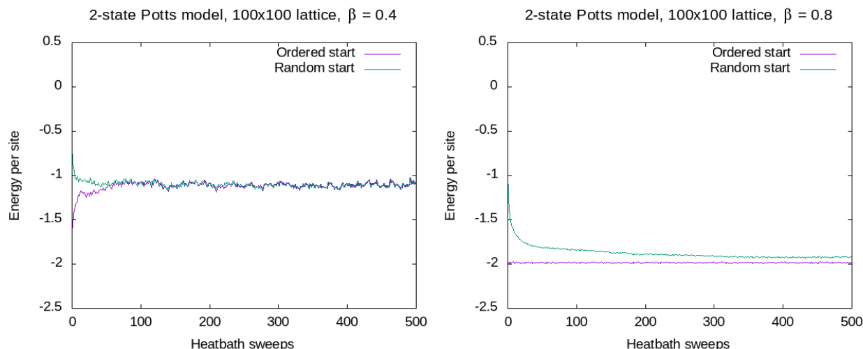
Figure 3.7 In these illustrations, the 2-state Potts model (aka the Ising model) is simulated on a 100x100 lattice using both cold (ordered) and hot (disordered) starts. On the left, the simulation is performed at \beta = 0.4 , and we see that the lattice equilibrates quickly. On the right, the simulation is performed in the ordered phase at \beta = 0.8 , and we see that at least one of the start types is having trouble reaching equilibration. Since we know the exact energy density for the two-dimensional Ising model on a finite lattice, we can tell that the ordered start is at the correct value. The random start has significantly more trouble reaching equilibration. In general, it seems that for a simulation performed in the ordered phase, the random start may take significantly longer to reach equilibration than the ordered start [5].
