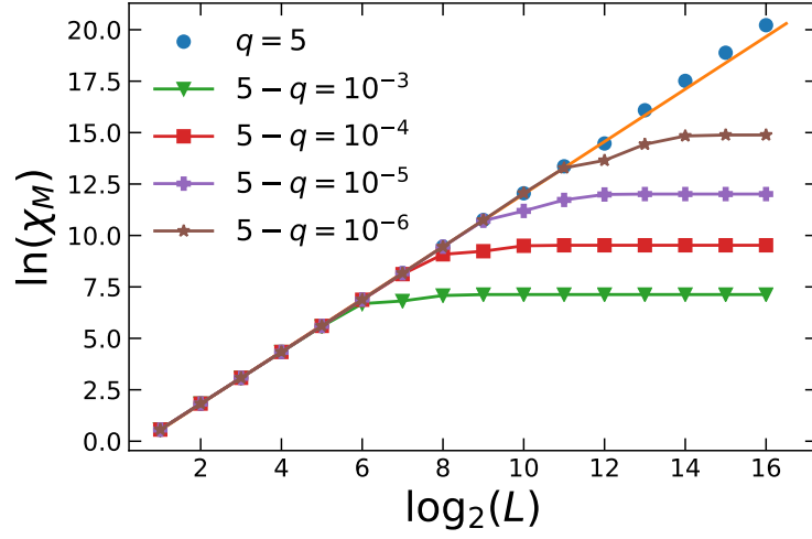
Figure 4.20 The dependence of magnetic susceptibility on the size of the system L for \beta = 1.1 with D_{\text{bond}} = 40 . The line on the circles is a linear fit for the first ten points: 1.275(3) \log_2(L) - 0.74(2) .
