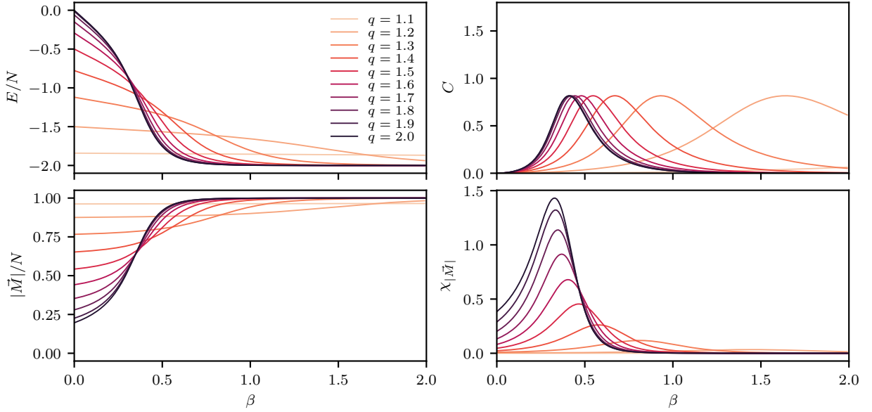
Figure 4.2 Monte Carlo results for the extended q -state clock model on a 4 \times 4 lattice for 1.1 \leq q \leq 2.0 . The top panel shows energy density and specific heat, and the bottom panel shows proxy magnetization and magnetic susceptibility. Statistical error bars are omitted since they are smaller than the line thickness.
