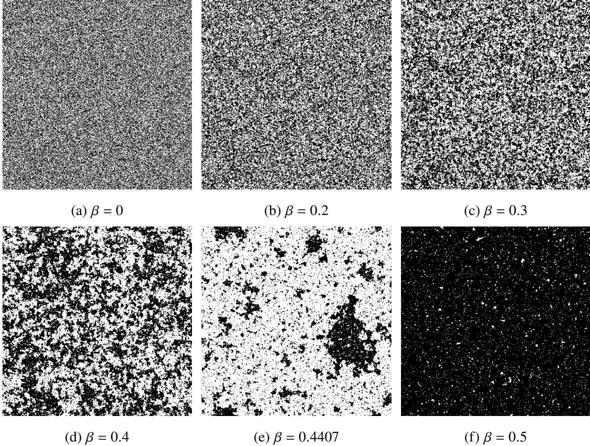
Figure 2.1 Example Ising configurations at different \beta (inverse temperature) from MCMC simulations performed on 400 \times 400 lattices. At \beta = 0 , the system is at infinite temperature and completely disordered/random. As \beta is increased, the system cools and increasingly large domains develop. Near \beta = 0.4407 , the system undergoes a second-order phase transition in the infinite-volume limit. At larger values of \beta , the system is “frozen” with a single domain having taken over the entire lattice. Note that these images are obtained from independent MCMC simulations at fixed \beta .
