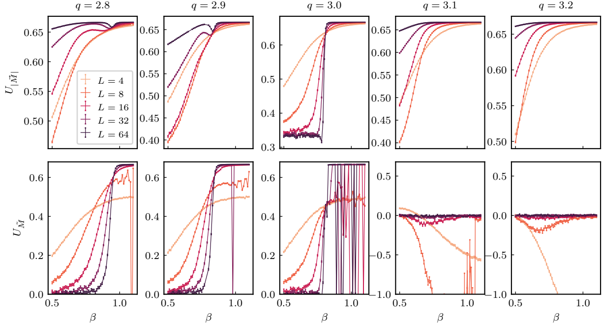
Figure 4.52 Here we look at some Binder cumulants for the model with noninteger q and h_q = 1 near the “hotspot”. From left to right, the columns correspond to q = 2.8, 2.9, 3.0, 3.1, 3.2 . The different shades correspond to different lattice sizes from L = 4 (light) to L = 64 (dark). The top row corresponds to the ordinary Binder cumulant defined in Eq. (4.66). For noninteger q , the Binder cumulants pinch together instead of cross at a second-order phase transition. In the bottom row, we show the Binder cumulant defined in Eq. (4.69) that has been modified to emphasize the Ising-ness of the model. This Binder cumulant shows again the classic crossing phenomenon at the phase transition. This data is from the model where \beta is treated as a coupling, and so the transition points may be slightly shifted from our usual model where \beta is treated as an inverse temperature.
