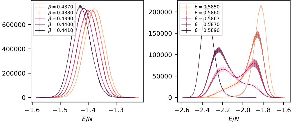
Figure 2.7 Histograms of the energy density at different values of \beta in the vicinity of a phase transition. In the left panel, histograms of the energy density near the second-order phase transition of the 2-state Potts model (i.e. the Ising model). In the right panel, histograms of the energy density near the first-order phase transition of the 5-state Potts model. Notice that the distribution becomes bimodal near a first-order critical point. These results were obtained on 100 \times 100 lattices using an MCMC heatbath algorithm.
