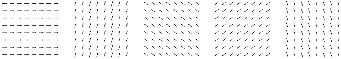
Figure 4.54 At very low temperatures, the spin system tends to be fully or nearly fully magnetized. For the q = 5.0 or q = 4.9 state clock models, there are five possible directions for this magnetization—corresponding to the five “clock angles” (See Fig. 4.53). When q = 5 , there is \mathbb{Z}_5 symmetry, and these directions are equivalent. When q = 4.9 , this is not true.
