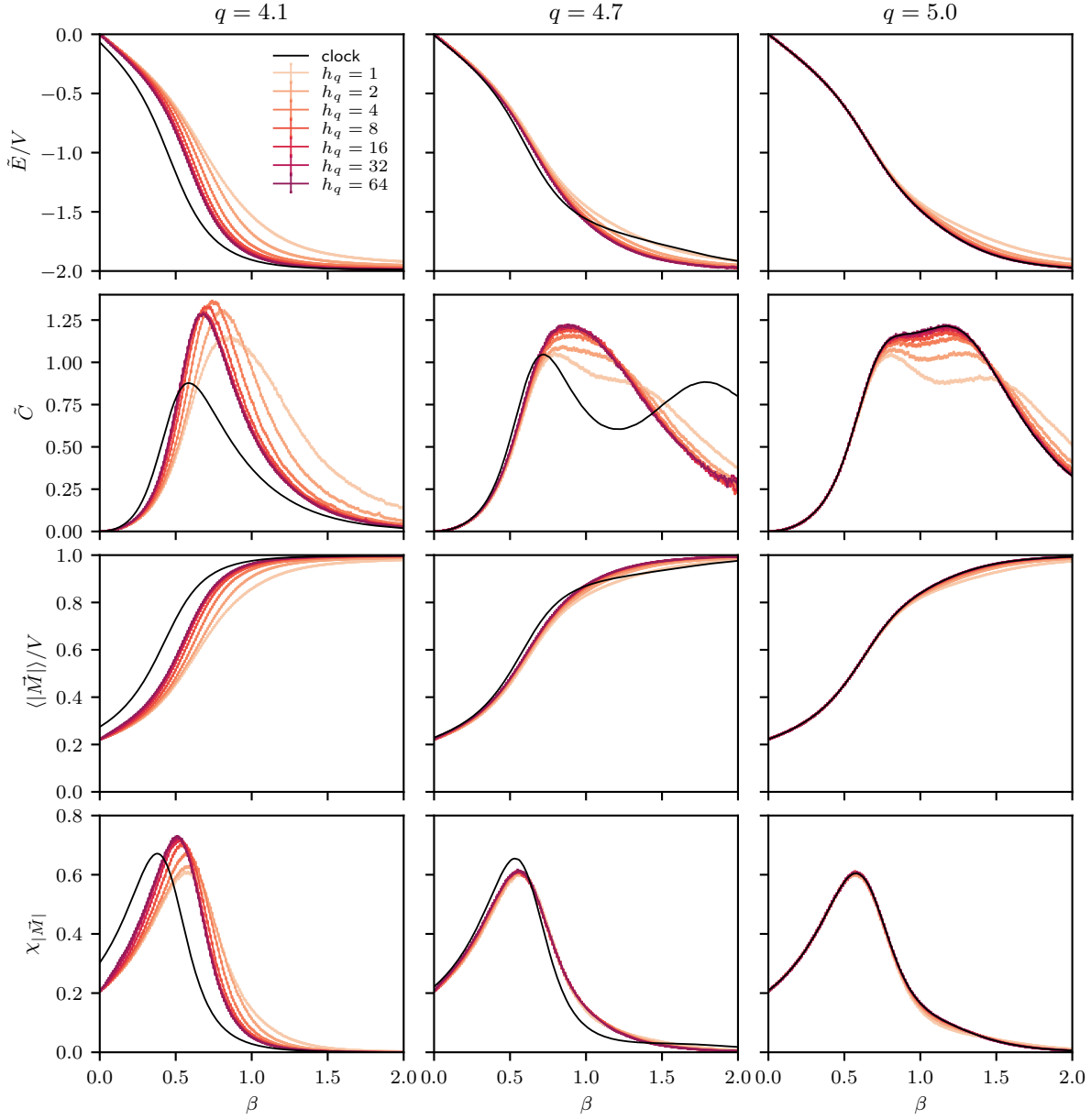
Figure 4.40 Here we compare the q -state clock model, which has been extended to noninteger values of q and has energy function Eq. (4.59) (black curves), with the Extended-O(2) model which has energy function Eq. (4.61) (colored curves) on a 4 \times 4 lattice. For the Extended-O(2) model, we consider increasing values of finite h_q in order to understand the limit h_q \rightarrow \infty . Naively, we expect the Extended-O(2) model to limit to the clock model when h_q is taken large. The Extended-O(2) model results are from lower statistics runs. The top row compares the “interaction” energy, the second row compares the corresponding specific heat, the third row compares the proxy magnetization, and the bottom row compares the susceptibility of the proxy magnetization. The different columns correspond to different values of q with q = 4.1, 4.7, 5.0 from left to right. In the naive approach ( \varphi \in [0, 2\pi) ) illustrated here, the h_q \rightarrow \infty limit of the Extended-O(2) model is the clock model only when q is integer. For noninteger values of q , the h_q \rightarrow \infty limit of the Extended-O(2) model differs from the clock model.
