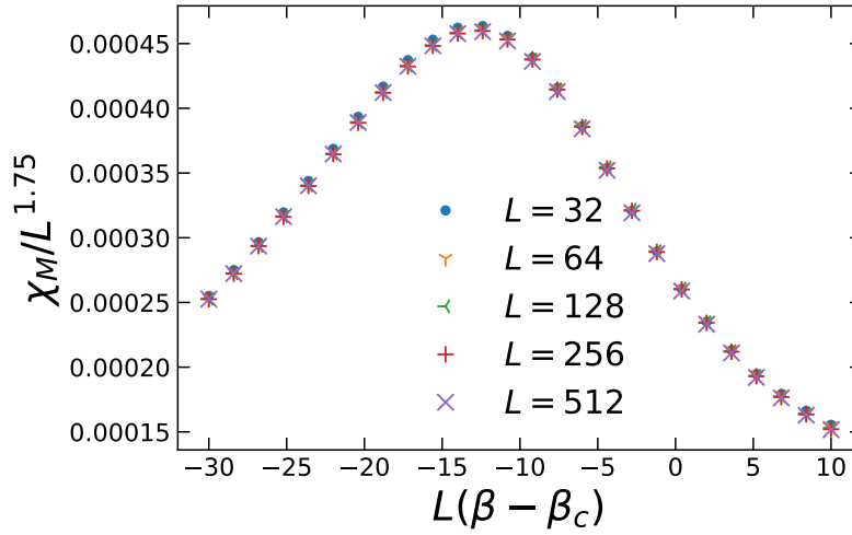
Figure 4.21 Data collapse of the rescaled magnetic susceptibility versus the rescaled inverse temperature for q = 4.3 . The reduced external field is hL^{15/8} = 40 , and \beta_c \approx 9.3216 , which is the approximate critical point of the model with q = 4.3 , is obtained from Eq. (4.40).
