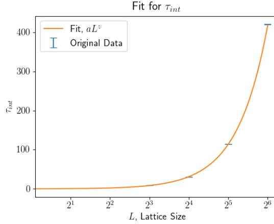
Figure 3.4 The integrated autocorrelation time of the energy is calculated using the heatbath algorithm for the two-dimensional Ising model at the critical point on four different lattice sizes. See Figure 3.1. The results are fitted to Eq. (3.35) to get an estimate of the dynamical critical exponent z .
