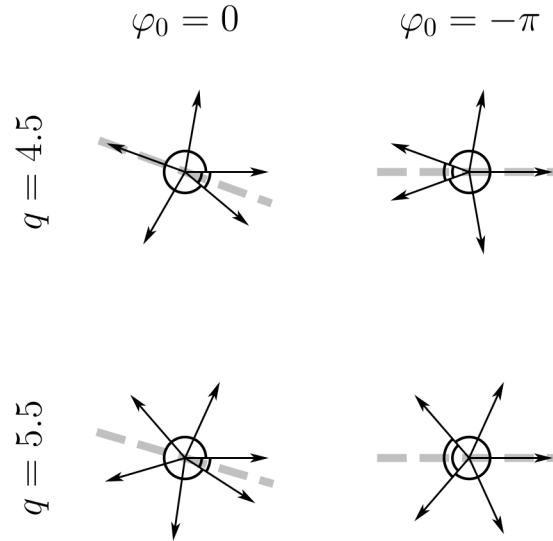
Figure 4.27 The allowed spin orientations for the extended q -state clock model when \varphi_0 = 0 (left column) and \varphi_0 = -\pi (right column) for two different values of q . When q = 4.5 (top row), the number of allowed spin orientations and their relative sizes are the same, and the models are equivalent. When q = 5.5 (bottom row), there are six allowed spin orientations when \varphi_0 = 0 , but only five allowed orientations when \varphi_0 = -\pi , so the two models are different. The dashed gray lines indicate the \mathbb{Z}_2 symmetry axes.
