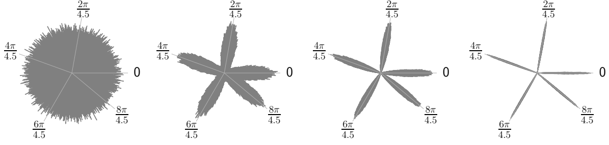
Figure 4.34 Here we illustrate how the spin angle distribution changes with h_q for the example q = 4.5 . From left to right, we have h_q = 0, 1, 4, 64 . For large values of h_q , the spins strongly prefer the “clock” angles defined by \varphi = 2\pi k/q for k = 0, 1, \dots, \lfloor q \rfloor . Note the “leftover” angle, which in this case is \tilde{\phi} = \pi/4.5 . These results are obtained by setting \beta = 0 in the model where \beta is treated as a coupling instead of as an inverse temperature.
