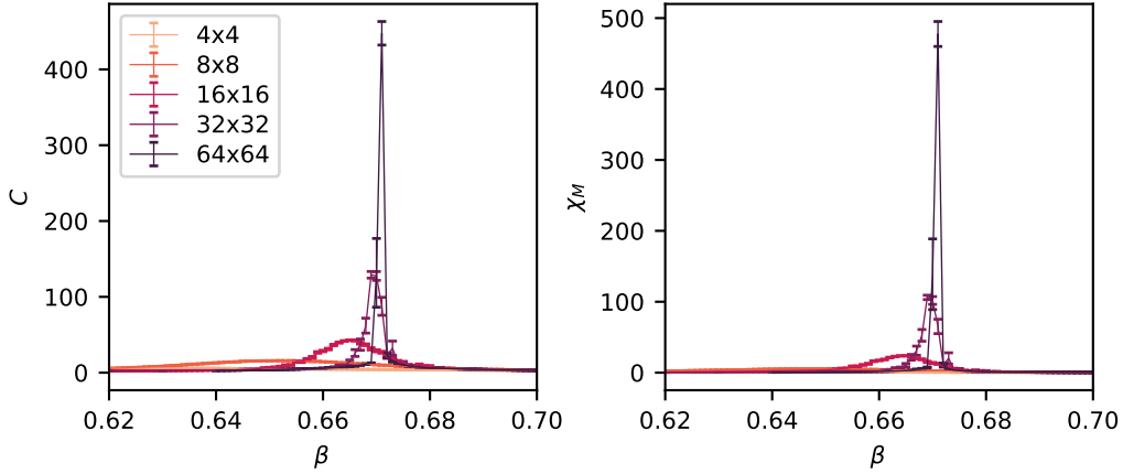
Figure 2.6 The specific heat (left) and magnetic susceptibility (right) of the 8-state Potts model both diverge sharply at the first-order phase transition near \beta \approx 0.671227 . On a finite lattice, these divergences are finite, but indicate the presence of a phase transition in the infinite volume model. These examples were obtained from small-statistics MCMC simulations using a heatbath updating algorithm.
