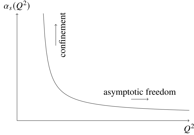
Figure 5.1 In QCD, the coupling constant \alpha_s = g^2/4\pi varies with the energy scale—a phenomenon referred to as the “running of the coupling”. As the energy and momentum transfer Q^2 increases, the coupling decreases logarithmically—a phenomenon known as asymptotic freedom. On the other hand, the coupling increases with decreasing energy, resulting in confinement.
