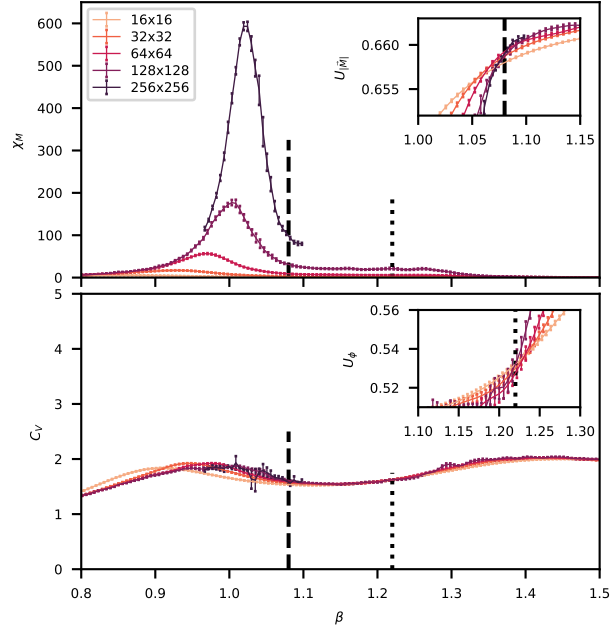
Figure 4.62 Here we look at data for some volumes ( L = 16, \dots, 256 ) for the model with q = 5 and h_q = 1.0 . The top panel shows the magnetic susceptibility, and the bottom panel shows the specific heat. The inset within the top panel shows the Binder cumulant of the proxy magnetization. The vertical dashed line is at \beta_{c1} \approx 1.08 , where the Binder cumulant curves cross. The inset within the bottom panel shows the Binder cumulant of the rotated magnetization defined in Eq. (4.51). The vertical dotted line is at \beta_{c2} \approx 1.22 , where the Binder cumulant curves cross. The data is from reweighted Monte Carlo with error bars included. This figure illustrates the behavior typical of the two BKT transitions that occur in the ordinary clock model for q \geq 5 . The magnetic susceptibility diverges at both transitions, and the specific heat plateaus at both transitions. For L = 256 , we show only results near the first transition point. Already here the error bars are rather large.
