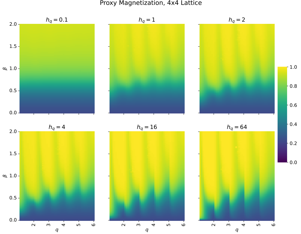
Figure 4.36 Here we show a heatmap of the proxy magnetization obtained via Monte Carlo on a 4 \times 4 lattice. Each panel shows the result at a different value of the symmetry-breaking parameter h_q . Note that each pixel corresponds to a distinct MCMC simulation.
