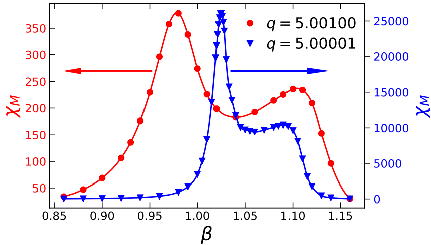
Figure 4.29 Same as Fig. 4.28, but for q = 5.001, 5.00001 . The large- \beta peak fades away and moves across the BKT phase transition point at q = 5 .
