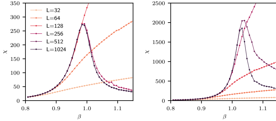
Figure 4.64 Here we look at the behavior of the magnetic susceptibility near the small- \beta peak for noninteger q . In this example, q = 4.1 . We obtain the susceptibility from TRG with bond dimension 32 after applying small external magnetic fields h = 10^{-5} , \delta h = 10^{-5} . In the left panel, h_q = 0.01 and in the right panel, h_q = 0.001 . For sufficiently large volumes, the magnetic susceptibility peaks plateau—implying a crossover. For a true phase transition, the peaks would diverge with increasing volume. As the symmetry-breaking parameter h_q is decreased toward zero, one must go to larger volumes to show that the peaks are not diverging.
