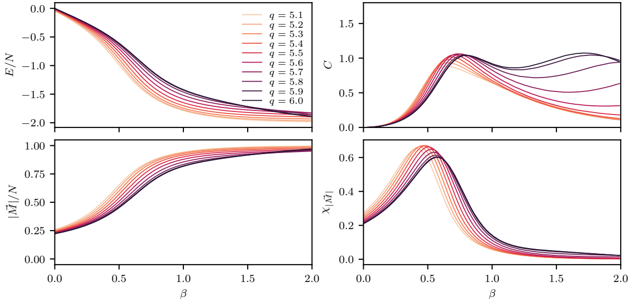
Figure 4.6 Monte Carlo results for the extended q -state clock model on a 4 \times 4 lattice for 5.1 \leq q \leq 6.0 . The top panel shows energy density and specific heat, and the bottom panel shows proxy magnetization and magnetic susceptibility. Statistical error bars are omitted since they are smaller than the line thickness.
