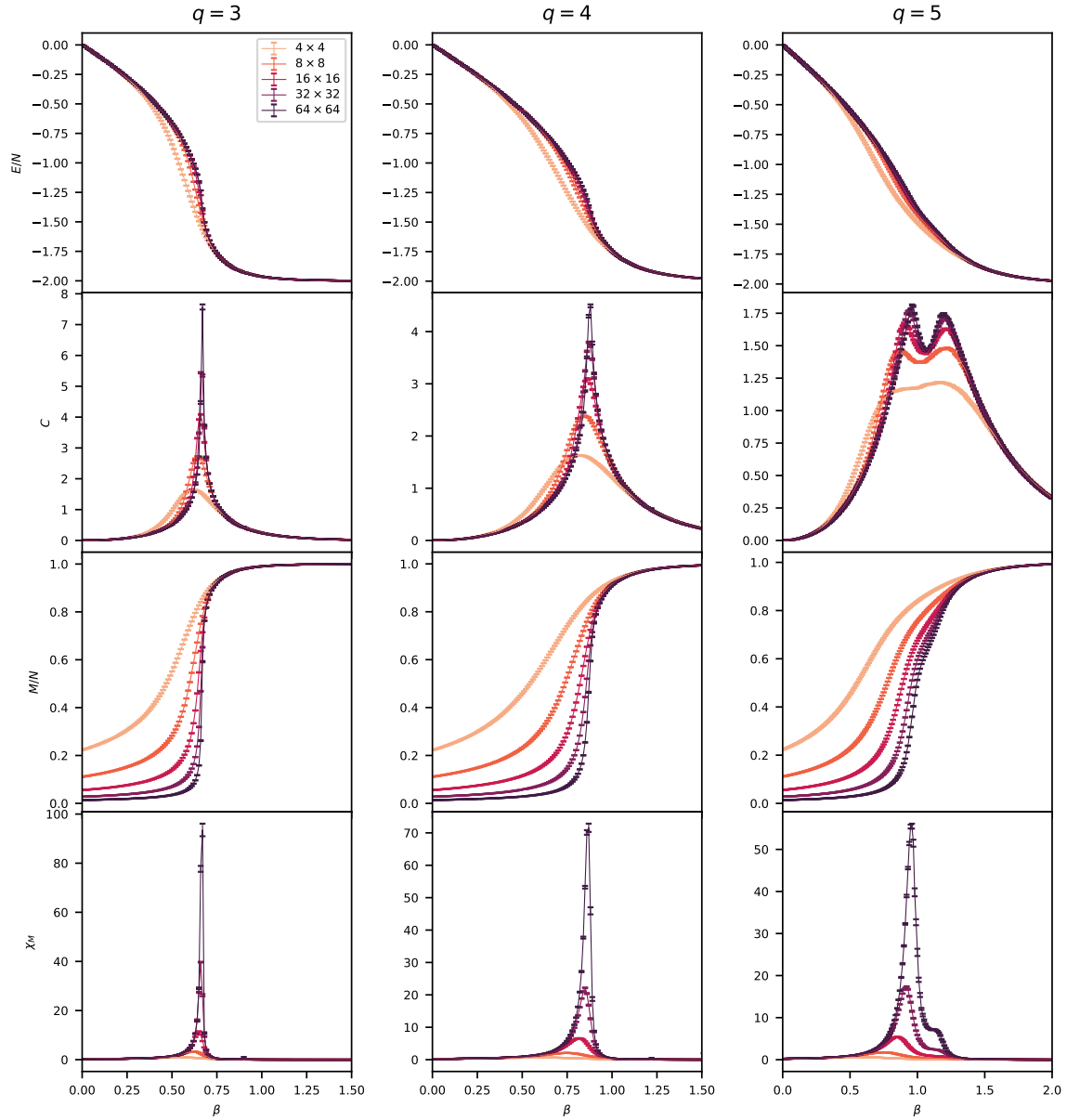
Figure 2.12 Here we show several thermodynamic quantities versus \beta for the q = 3, 4, 5 state clock models at different lattice sizes. In the top row, we show the energy density, and in the second row the specific heat. In the third row, we show the magnetization per lattice site, and in the bottom row, we show the magnetic susceptibility. Note that the 2-state clock model is just the Ising model, with results shown in Figure 2.2.
