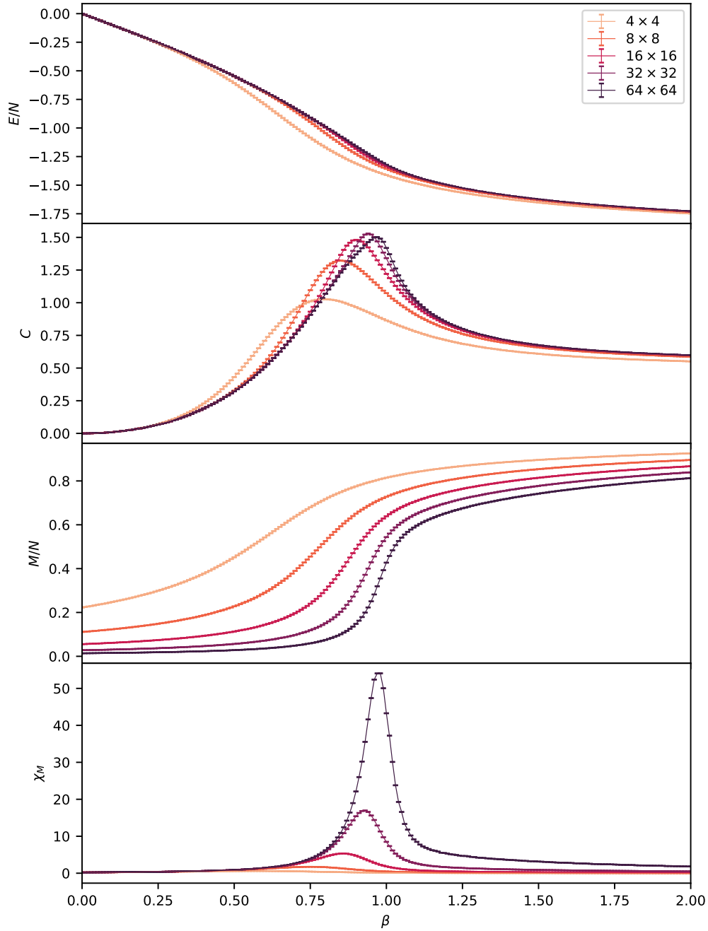
Figure 2.8 Here we show several thermodynamic quantities versus \beta for the XY model at different lattice sizes. In the top panel, we show the energy density, and in the second panel the specific heat. In the third panel, we show the magnetization per lattice site, and in the bottom panel, we show the magnetic susceptibility. Near the critical point, the magnetic susceptibility diverges with volume, but the specific heat does not. This is in contrast to the behavior of the specific heat near a first or second-order transition.
