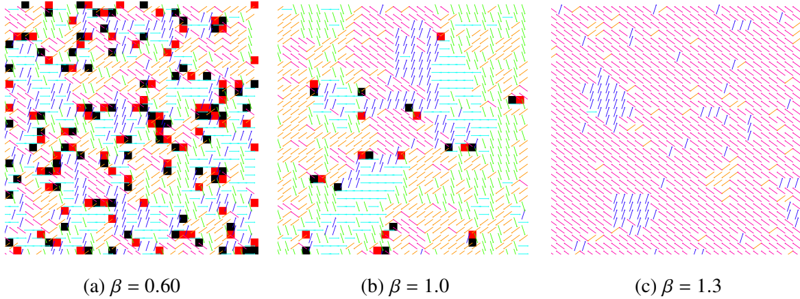
Figure 2.13 A few examples of equilibrium vortices from independent Monte Carlo simulations of the 5-state clock model performed on 32 \times 32 lattices with periodic boundary conditions. Vortex positions are identified by computing the winding number Eq. (2.42) of each plaquette. A winding number of +1 corresponds to a vortex, and a winding number of -1 corresponds to an antivortex. In panel (a), an equilibrium configuration is shown for \beta = 0.6 , which is in the disordered phase. The vortex-antivortex pair density is high and many are unbound. Panel (b) comes from a simulation performed at \beta = 1.0 , which is close to the critical region of the 5-state clock model. Panel (c) shows an equilibrium configuration at \beta = 1.3 , which is in the quasi-ordered phase. Here the vortex pair density is very low. In this example we see no vortices.
