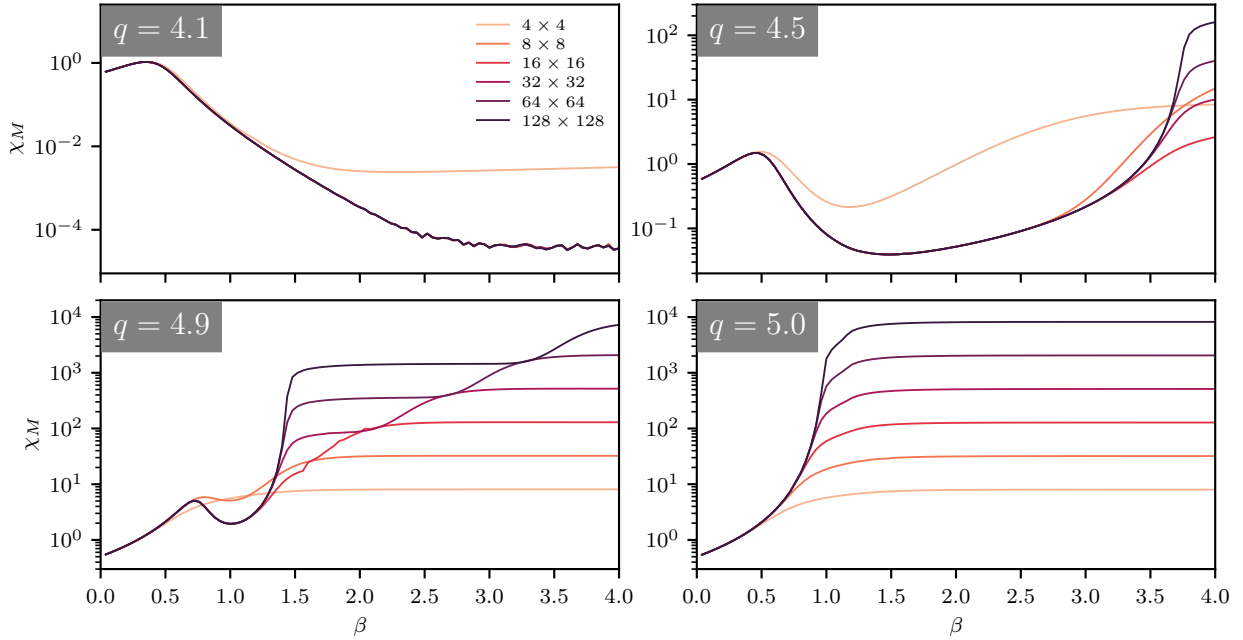
Figure 4.12 The magnetic susceptibility as a function of \beta for finite volumes. D_{\text{bond}} = 40 .
