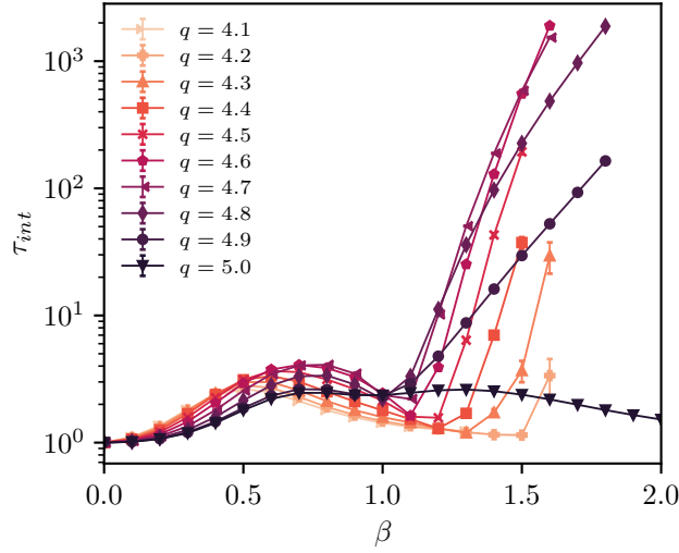
Figure 4.8 The integrated autocorrelation time of the energy density for several q on a 4 \times 4 lattice using a heatbath algorithm. At large \beta , the integrated autocorrelation time \tau_{int} grows abruptly when q \notin \mathbb{Z} . Note the log scale on the vertical axis. Connecting lines are included to guide the eyes. The rapid increase of the integrated autocorrelation time for noninteger q occurs because the MCMC approach is having difficulty sampling the full configuration space. Details are given in the main text.
