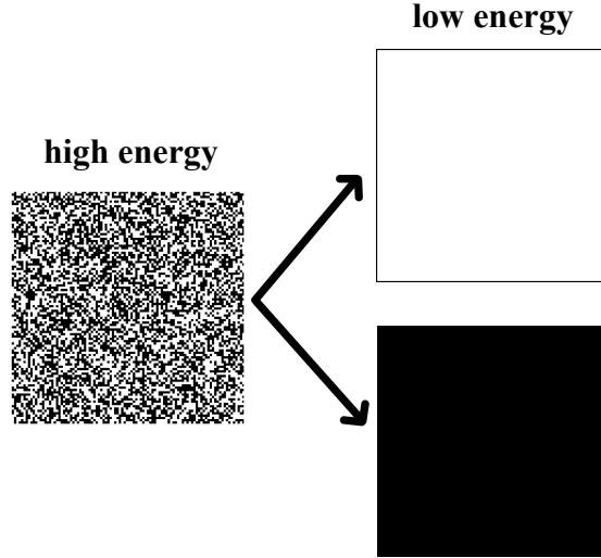
Figure 2.3 In the Ising model with no external field, there is a global \mathbb{Z}_2 symmetry—one can transform the spin variables S \rightarrow -S without changing the energy function Eq. (2.2). This symmetry is spontaneously broken when at low energy, the system chooses either the configuration with most spins oriented up or the configuration with most spins oriented down. These two configurations have the same energy, however, there is a very large energy barrier between them, and it is very unlikely for the overall magnetization to flip orientations in the low energy sector.
