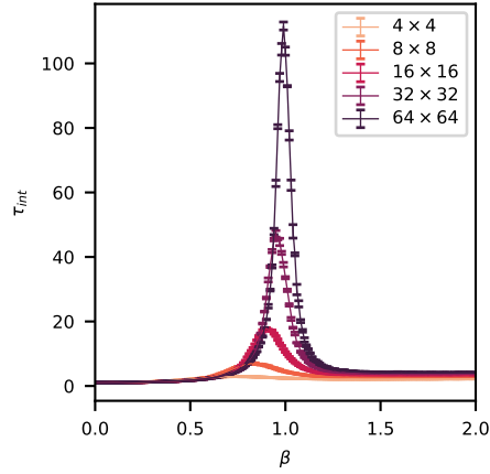
Figure 3.3 The integrated autocorrelation time (of the energy here) blows up at a phase transition as shown here for the XY model using a Biased Metropolis Heatbath Algorithm on lattices of various size. This is the cause of the critical slowing down that plagues MCMC simulations near critical points. The high autocorrelation time means many configurations must be discarded between measurements in order to get an independent sample, and so the overall computational time required gets very large at the critical point.
