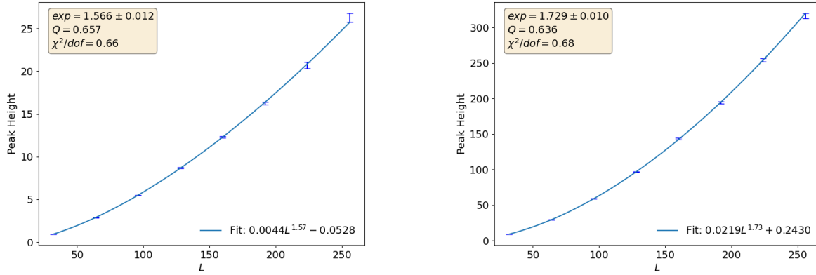
Figure 4.57 Finite size scaling of the magnetic susceptibility (left) and the structure factor (right) for the model with q = 4.9 and h_q = 1 at the large- \beta peak where we expect a phase transition. According to the scaling law Eq. (3.79), these two quantities must scale with the same exponent. That scaling law is clearly violated here since \gamma/\nu = 1.566(12) and 2 - \eta = 1.729(10) . We believe this apparent violation is due to the freezing effect which occurs with MCMC at large lattice sizes. The result is that with MCMC alone, we cannot perform reliable finite size scaling for the Extended- O(2) model with noninteger q .
