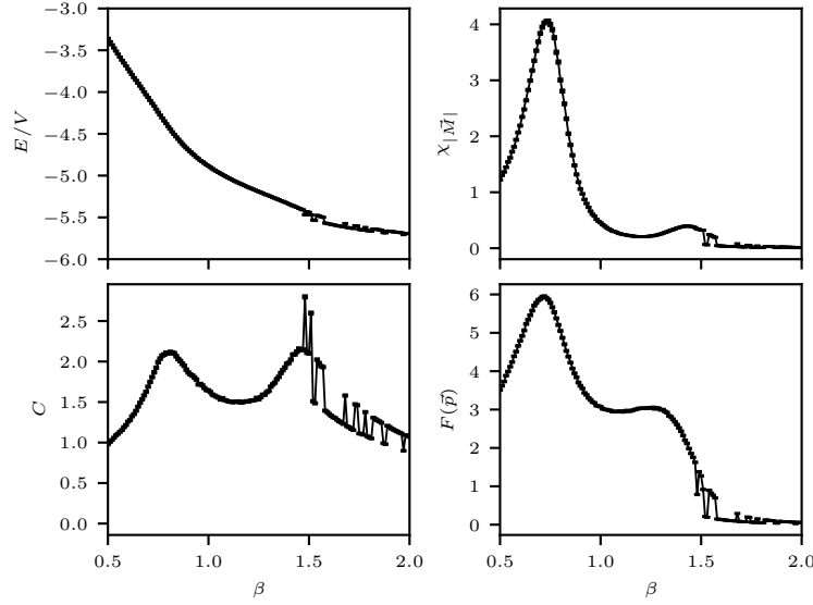
Figure 4.55 Here we show some thermodynamic results for the model with q = 4.9 , h_q = 4 on a 16 \times 16 lattice. Clockwise from the top-left panel we show the energy density, magnetic susceptibility, structure factor, and specific heat. Data points are connected with lines to help guide the eyes. Near \beta = 1.5 we see that all four thermodynamic quantities become unstable in a manner that suggests the Markov chain became stuck in one of two thermodynamically distinct sectors. Clearly, the naive error bars (here the statistical variance only) are not enough to capture the true uncertainty.
