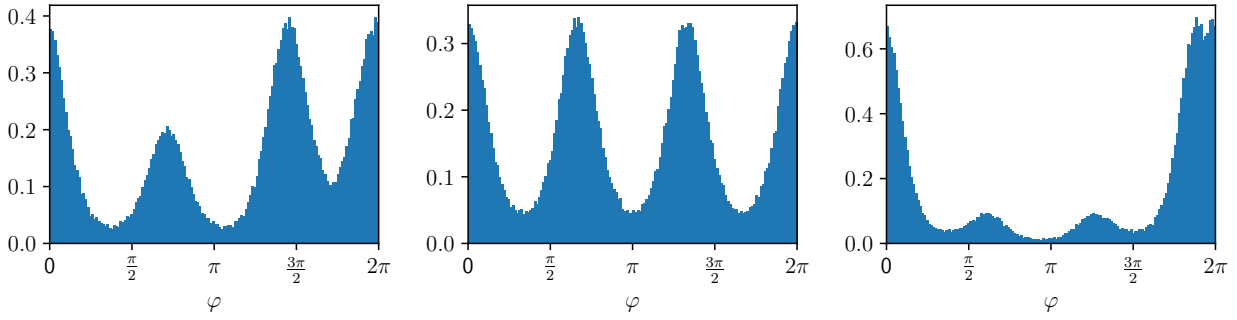
Figure 4.45 Here we show the distribution of spin angles \varphi via histograms. These results were obtained on 4 \times 4 lattices with \beta = h_q = 1 and q = 2.8 (left), q = 3.0 (center), and q = 3.2 (right).
