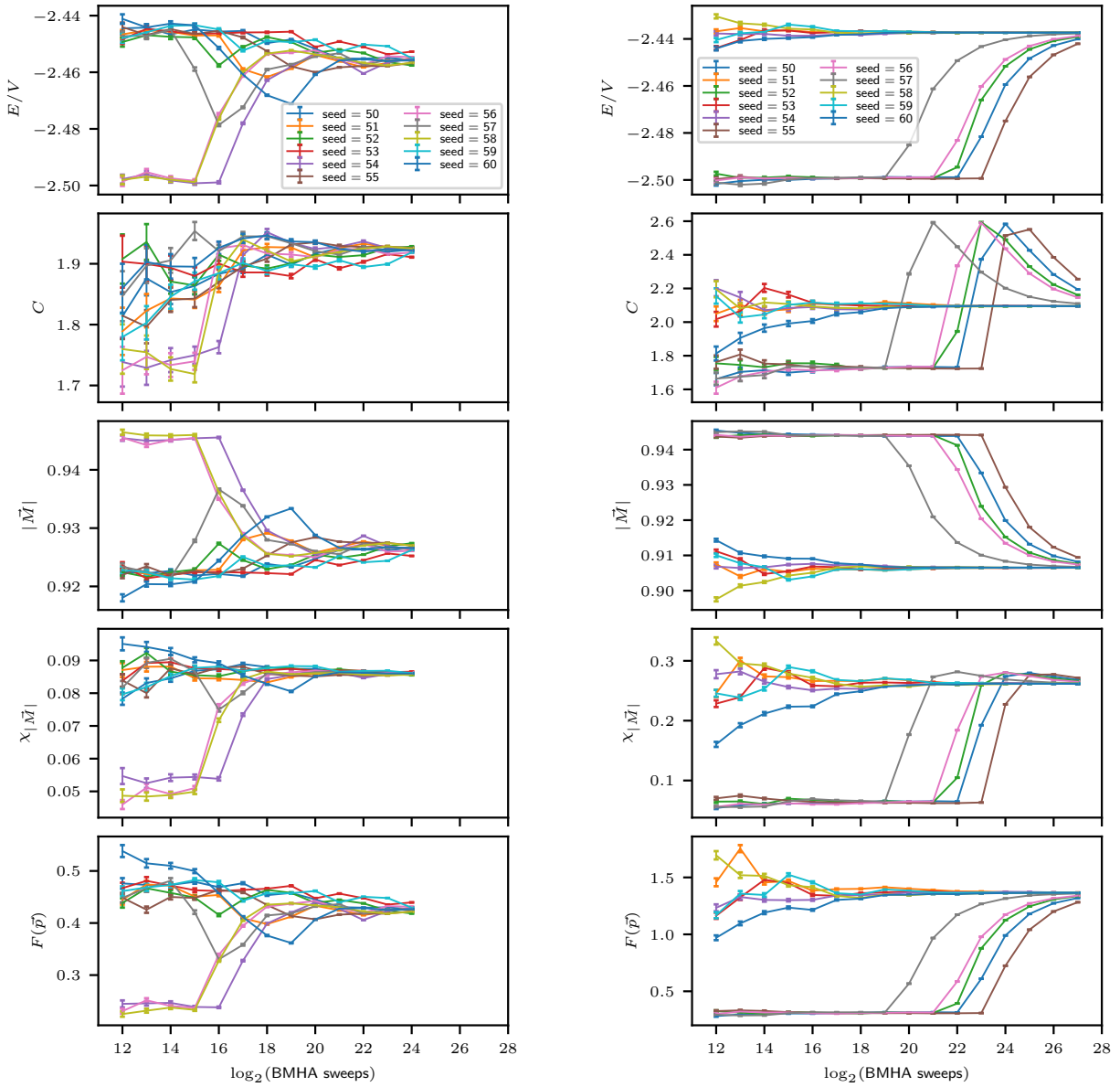
Figure 4.56 Here we show observables estimated on Markov chains of different lengths. The data is from the model with q = 4.9 , h_q = 1 , and \beta = 1.66 . The left column comes from an 8 \times 8 lattice, and the right column comes from a 16 \times 16 lattice. The rows, from top to bottom, are energy density, specific heat, proxy magnetization, susceptibility of the proxy magnetization, and structure factor. The horizontal axis is the log base-2 of the number of updating (BMHA) sweeps performed. That is, ‘12’ on the horizontal axis corresponds to 2^{12} updating sweeps. The different color points (with connecting lines to guide the eyes) correspond to different seeds for the random number generator. These results indicate that the system tends to freeze in one of two thermodynamically distinct sectors, and a reliable estimate of the true value of an observable can only be obtained with very large statistics such that both sectors are sampled. This problem worsens dramatically with increasing lattice size. It is a result of the broken \mathbb{Z}_q symmetry and only occurs when q is not integer.
