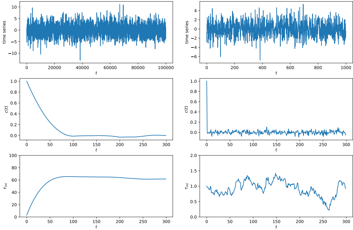
Figure 3.5 Here we illustrate how blocking and preaveraging can be used to mitigate autocorrelations. We construct a stochastic time series containing autocorrelation. This is done by choosing 100K uniformly random numbers \{r\} in [-0.5, 0.5) . The n th element a_n of the autocorrelated time series (plotted in top left) is a_n = r + a_{n-1} where r is a random number, however, if n is a multiple of 100, then a_n = r . The center left panel shows the autocorrelation function c(t) of the series, and the bottom left panel shows that the integrated autocorrelation time is \sim 65 . Next, we do blocking and preaveraging with block size 100. The resulting shorter time series is shown in the top right. The associated correlation function (center right) and \tau_{int} (bottom right), shows that the preaveraged time series is not autocorrelated.
