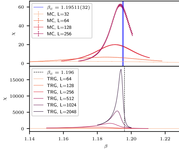
Figure 4.59 We compute the susceptibility for q = 3.9 and h_q = 1 in the vicinity of the second-order transition in two different ways. In the top panel, we see how the susceptibility peaks from Monte Carlo approach the critical point, and in the bottom panel we look at the susceptibility peaks from TRG. From the Monte Carlo peak positions, we estimate \beta_c = 1.19511(32) (vertical blue line) by fitting the peak locations to the finite-size-scaling form Eq. (3.78). From the TRG peak positions, we estimate \beta_c = 1.196 (vertical dashed line) via the same finite-size scaling form. As described in the main text, because of large autocorrelations, the Monte Carlo results at noninteger q are not strictly reliable for L > 32 .
