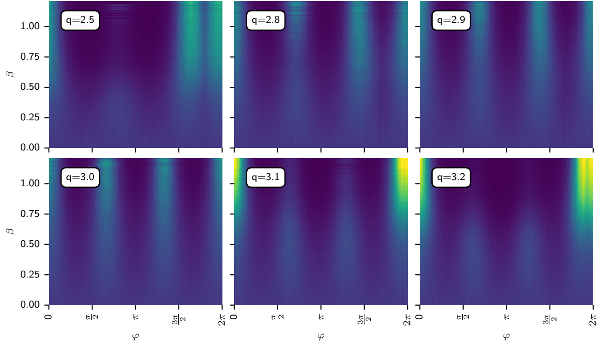
Figure 4.46 Heatmaps of the angle histograms (see Fig. 4.45) for a 4 \times 4 lattice with h_q = 1 , \beta \in [0, 1.2] , and q = 2.5, 2.8, 2.9, 3.0, 3.1, 3.2 . Note that each pixel corresponds to a distinct MCMC simulation.
