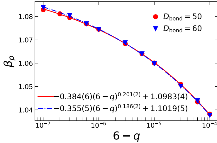
Figure 4.18 Same as Fig. 4.17, but for q \rightarrow 6^- .
