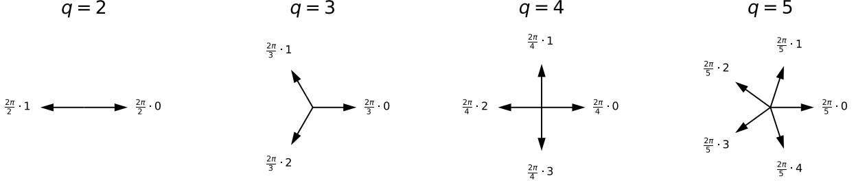
Figure 2.11 Here we show the allowed “clock” angles for several different values of q . In the q -state clock model, the spin-variables sitting at lattice sites can only take the allowed values \theta = \frac{2\pi k}{q} with k = 0, 1, \dots, q - 1 .
