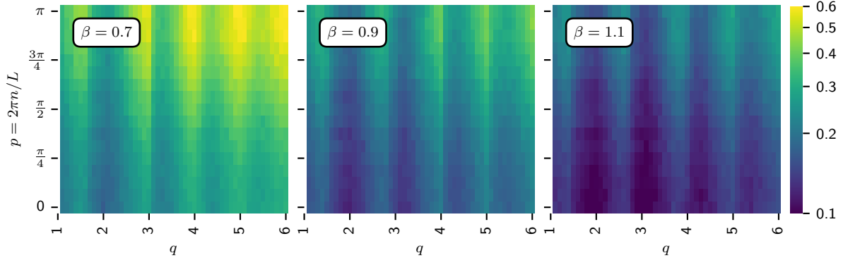
Figure 4.49 Heatmaps of the staggered structure factor F(p) with momenta p on the vertical axis and with q on the horizontal axis. The different panels correspond to different \beta with \beta = 0.7, 0.9, 1.1 from left to right. These results are from 32 \times 32 lattices with h_q = 1 and are from the model where \beta is treated as a coupling. Note that each pixel corresponds to a distinct MCMC simulation.
