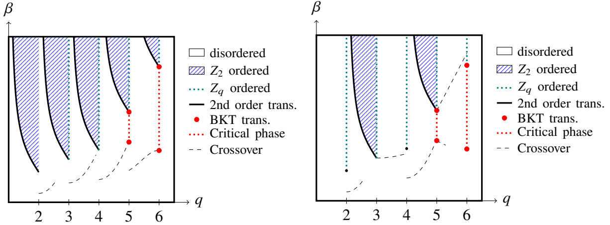
Figure 4.32 The phase diagram of the extended q -state clock model [i.e. the h_q = \infty plane of the extended-O(2) model] for \varphi_0 = 0 (left) and \varphi_0 = -\pi (right). For q = 2, 3, 4 , there is a second-order phase transition with a \mathbb{Z}_q ordered phase at large \beta . For finite integer q \geq 5 , there is a critical phase between a pair of BKT transitions and a \mathbb{Z}_q ordered phase at large \beta . For fractional q > 2 with \varphi_0 = 0 , there is a crossover line, a second-order transition line, and a \mathbb{Z}_2 ordered region between every consecutive pair of integers. For \varphi_0 = -\pi , the same is true for every other consecutive pair of integers.
