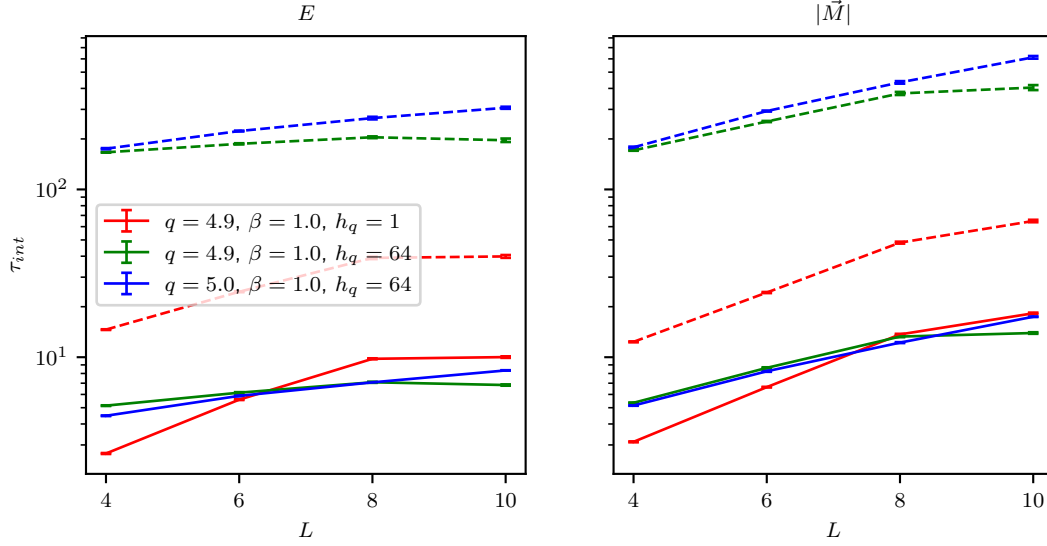
Figure 4.38 The integrated autocorrelation time of the internal energy (left) and the proxy magnetization (right) for several lattice sizes L . The three different colors correspond to three different parameter sets. The solid lines are from the BMHA algorithm, and the dashed lines are from the Metropolis algorithm. We see that the integrated autocorrelation time is one to two orders of magnitude smaller for the BMHA algorithm. All results shown are from simulations performed at \beta = 1 . In practice, we find that the integrated autocorrelation time increases with larger \beta . Note, connecting lines were added only to help guide the eyes.
