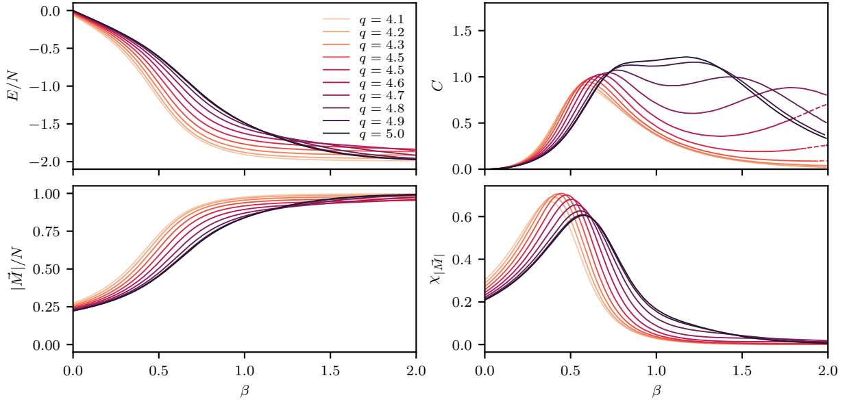
Figure 4.5 Monte Carlo results for the extended q -state clock model on a 4 \times 4 lattice for 4.1 \leq q \leq 5.0 . The top panel shows energy density and specific heat, and the bottom panel shows proxy magnetization and magnetic susceptibility. Statistical error bars are omitted since they are smaller than the line thickness. Dashed lines indicate regions where we have data but we do not have the uncertainty fully under control.
