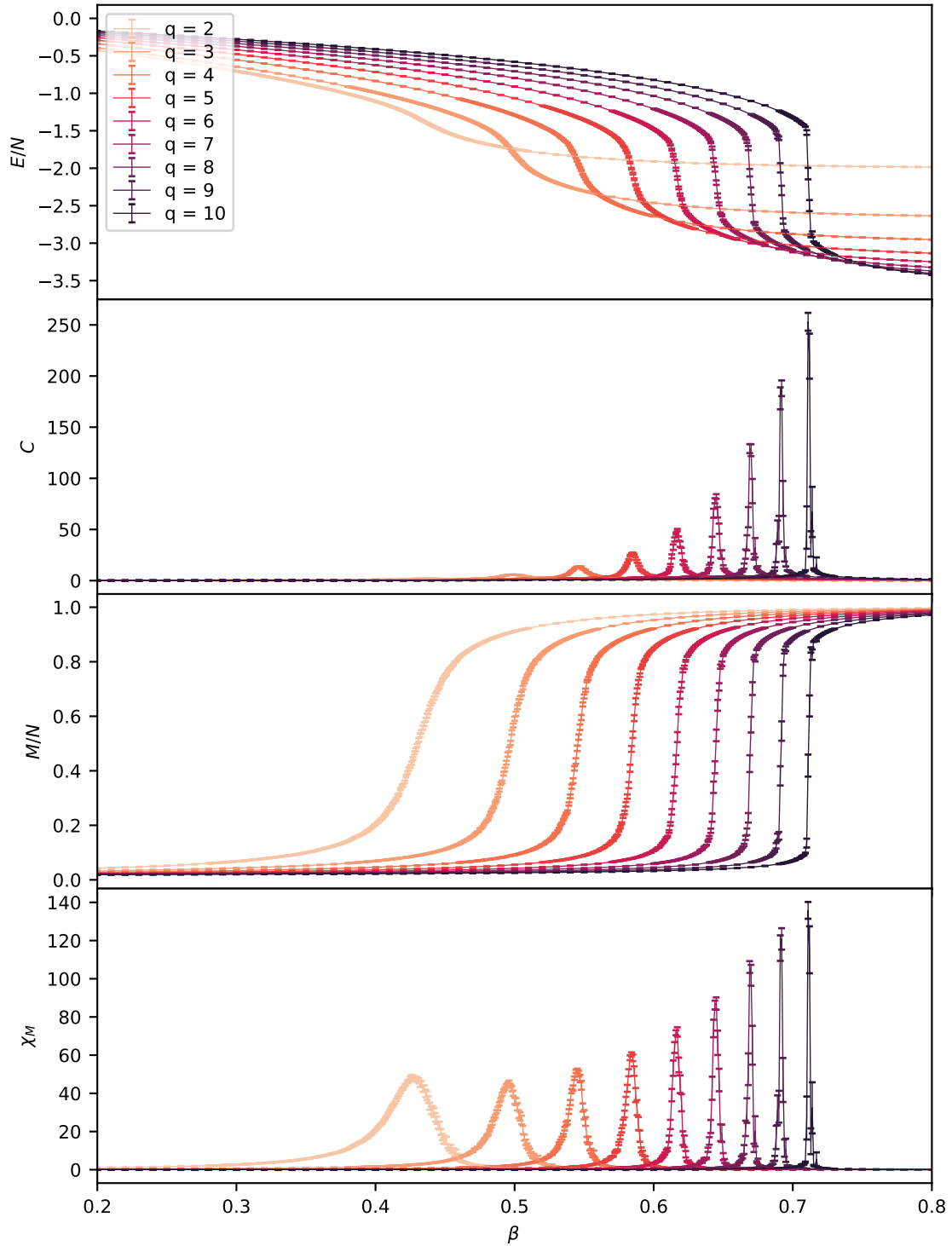
Figure 2.5 The energy density, specific heat, magnetization per site, and magnetic susceptibility of the q -state Potts model on a 32 \times 32 lattice. These were obtained from low statistics MCMC simulations using a heatbath algorithm. Notice how the energy is continuous at q = 2, 3, 4 , but becomes discontinuous at larger q . This is an illustration of the Potts model having a second-order phase transition at small q , but a first-order phase transition at larger q .
