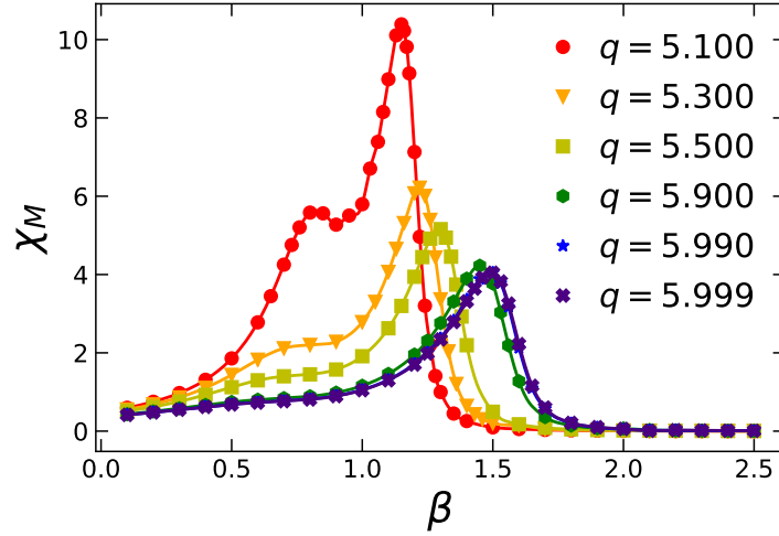
Figure 4.28 The magnetic susceptibility at N = 2^{24} \times 2^{24} , h = 0 , and D_{\text{bond}} = 40 , as a function of \beta for \varphi_0 = -\pi . The susceptibility does not diverge with the volume, which implies there is no phase transition here. This is different from the model with \varphi_0 = 0 , which has a divergent peak in the susceptibility corresponding to a second-order phase transition.
