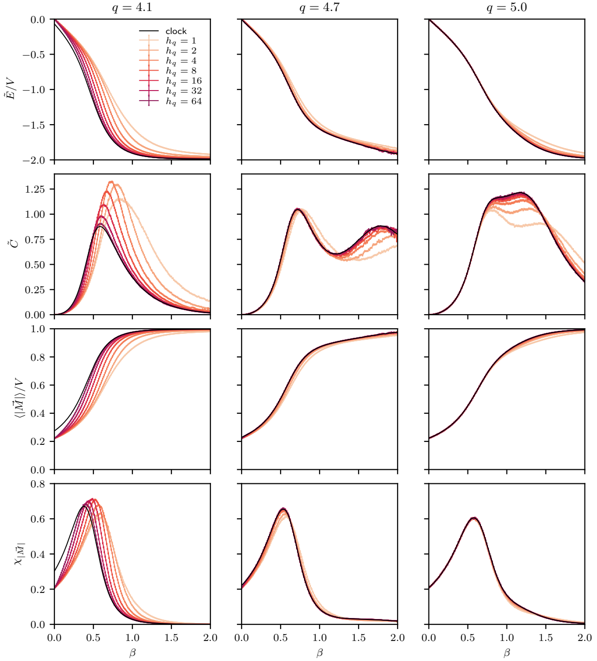
Figure 4.41 Here we compare the q -state clock model (black curves) with the h_q \rightarrow \infty limit of the Extended-O(2) model (colored curves) on a 4 \times 4 lattice. The Extended-O(2) model results are from lower statistics runs. The top row compares the “interaction” energy, the second row compares the corresponding specific heat, the third row compares the proxy magnetization, and the bottom row compares the susceptibility of the proxy magnetization. The different columns correspond to different values of q with q = 4.1, 4.7, 5.0 from left to right. Here, \varphi \in [-\varepsilon, 2\pi - \varepsilon] with \varepsilon given by Eq. (4.63), and now the Extended-O(2) model becomes the clock model in the h_q \rightarrow \infty limit. Notice that the matching breaks down at very small \beta in this illustration when q is noninteger. As explained in the text, the proper matching procedure would be to adjust h_q such that \beta h_q stays large as one approaches \beta = 0 .
