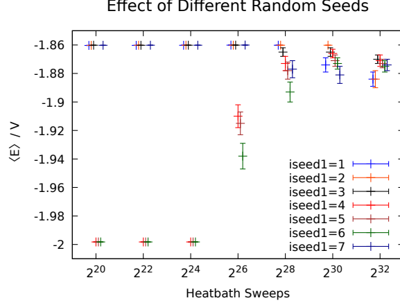
Figure 4.7 The measured energy density for q = 4.5 at different number of heatbath sweeps for different random number generator (RNG) seeds. The vertical axis is the energy density. The horizontal axis gives the number of heatbath sweeps used (not including equilibration sweeps). The different colors indicate runs with different seeds for the RNG. All runs were performed at \beta = 2.5 with hot-started 4 \times 4 lattices. This shows that the configuration space consists of two distinct sectors, and the heatbath algorithm has difficulty appropriately sampling both sectors unless the number of heatbath sweeps is taken very large.
