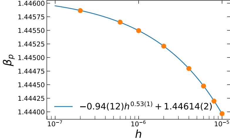
Figure 4.22 The power law extrapolation of the peak position of \chi_M to zero external field for q = 4.9 . Here the extrapolation gives \beta_c = 1.44614(2) . D_{\text{bond}} = 40 .
