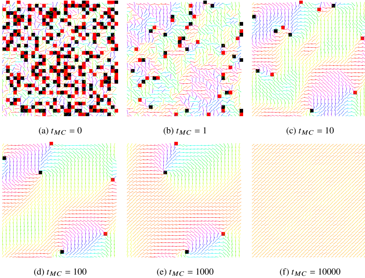
Figure 2.9 Here we show an example of the evolution of a 32 \times 32 lattice in the XY model with periodic boundary conditions when it is started at infinite temperature and immediately quenched to nearly zero temperature. We start in panel (a) with random spins. This corresponds to an infinite temperature lattice. At this temperature, tiny vortices (black squares) and antivortices (red squares) proliferate. Vortex positions are identified by computing the winding number Eq. (2.42) of each plaquette. A winding number of +1 corresponds to a vortex, and a winding number of -1 corresponds to an antivortex. Panel (b) shows the same lattice after one BMHA sweep with the low temperature \beta = 100 . Already many of the vortices and antivortices have annihilated and some order is starting to appear. Panel (c) shows the lattice after 10 BMHA sweeps with \beta = 100 . Panels (d) and (e) show the lattice after 100 and 1000 BMHA sweeps. Now only two or three vortex-antivortex pairs remain. But they are large and annihilate slowly. By the 10000th BMHA sweeps (panel (f)), no vortex-antivortex pairs remain, and the lattice is in a state of quasi-long-range order.
