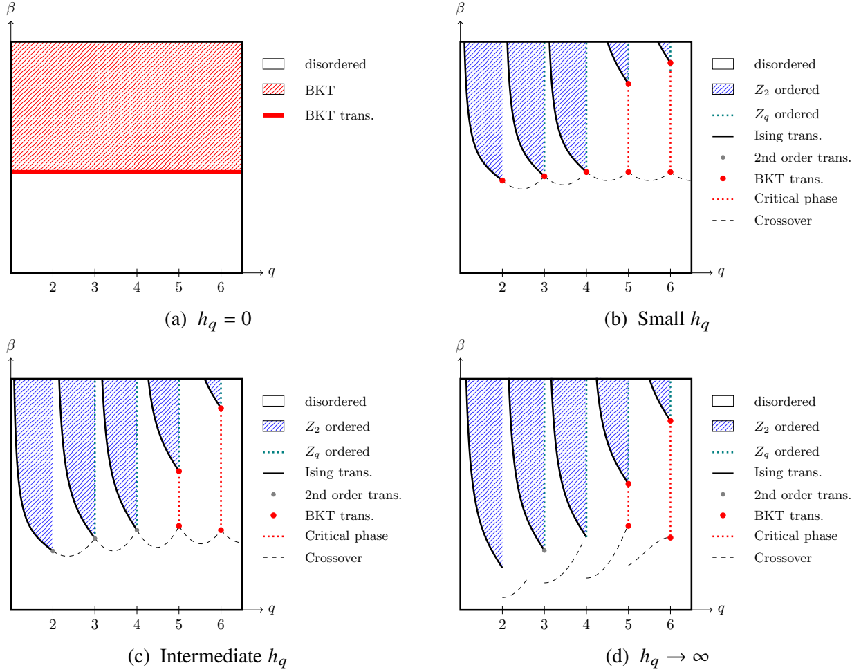
Figure 4.66 Here we present four two-dimensional conjectures for the full three-parameter phase diagram. Each slice is at a different value of the symmetry-breaking parameter h_q . In the top-left panel, the phase diagram at h_q = 0 . This is the well-studied XY model at all values of q . There is a single BKT transition near \beta = 1.12 and a BKT critical phase at larger \beta . The top-right panel gives the conjectured phase diagram at small h_q > 0 . For noninteger q , there is generally a crossover at small \beta and an Ising phase transition at larger \beta with an Ising ordered phase at large \beta . For integer q , our data is consistent with BKT transitions for all integer q given sufficiently small (but positive) h_q . For q = 2, 3, 4 our conjecture that these are BKT transitions is rather tenuous as it is possible that the apparent BKT transition is really the result of studying the model on too small lattices. For integer q \geq 5 , there are two BKT transitions with the second transition appearing at larger \beta . This transition does not seem to connect to the BKT line at h_q = 0 in the limit h_q \rightarrow 0 [122]. In the bottom-left panel, h_q is increased to intermediate values. The most significant change is that for q = 2, 3, 4 the transitions are now second-order, however, they are not in the same universality class as the clock model (i.e. h_q = \infty ) transitions. Finally, in the bottom-right panel, we show the phase diagram for the h_q \rightarrow \infty case. For integer q , this is the ordinary q -state clock model, and for noninteger q , this is what we call the “Extended q -state clock model”.
