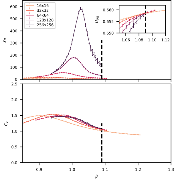
Figure 4.61 Here we look at data for some volumes ( L = 16, \dots, 256 ) for the model with q = 4 and h_q = 0.1 . The top panel shows the magnetic susceptibility, the bottom panel shows the specific heat, and the inset within the top panel shows the Binder cumulant. The data is from reweighted Monte Carlo with error bars included. The vertical dashed line is at \beta_c \approx 1.09 where the Binder cumulant curves merge. This figure illustrates the behavior typical of a BKT phase transition—the Binder cumulants merge at the transition point, the magnetic susceptibility diverges, and the specific heat plateaus.
