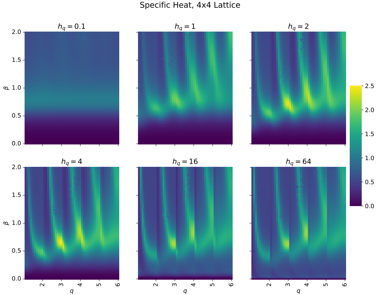
Figure 4.35 Here we show a heatmap of the specific heat obtained via Monte Carlo on a 4 \times 4 lattice. Each panel shows the result at a different value of the symmetry-breaking parameter h_q . For general noninteger q , we see two peaks in the specific heat—one at small- \beta near \beta \in [0.5, 1] and one at large- \beta . Note that each pixel corresponds to a distinct MCMC simulation.
