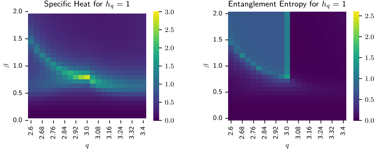
Figure 4.44 The specific heat (left) and the entanglement entropy (right) from TRG for various q near q = 3 with \beta \in [0, 2] and h_q = 1 . These results were obtained from lattices of size L = 1024 . Note that each pixel corresponds to a distinct TRG calculation. The specific heat suggests a smooth curve in the phase diagram, however, the entanglement entropy shows a clear discontinuity across q = 3 .
