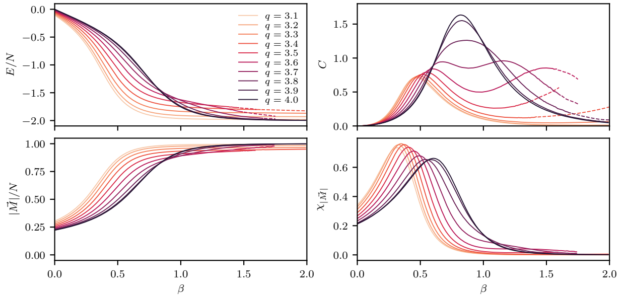
Figure 4.4 Monte Carlo results for the extended q -state clock model on a 4 \times 4 lattice for 3.1 \leq q \leq 4.0 . The top panel shows energy density and specific heat, and the bottom panel shows proxy magnetization and magnetic susceptibility. Statistical error bars are omitted since they are smaller than the line thickness. Dashed lines indicate regions where we have data but we do not have the uncertainty fully under control.
