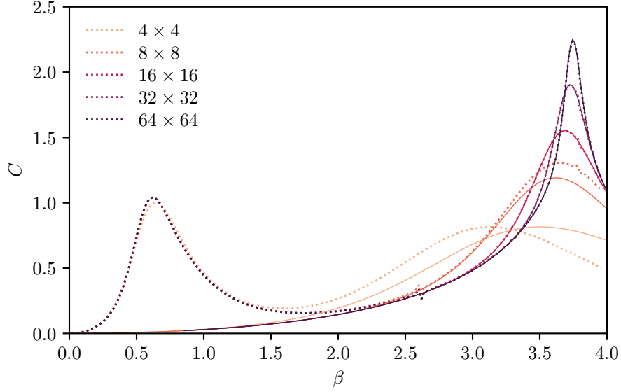
Figure 4.25 The specific heat for q = 4.5 for several different lattice sizes. The dotted curves are from TRG and the solid curves are from the rescaled Ising model. For 16 \times 16 and larger lattices, the rescaled Ising model accurately captures the second peak in the specific heat.
