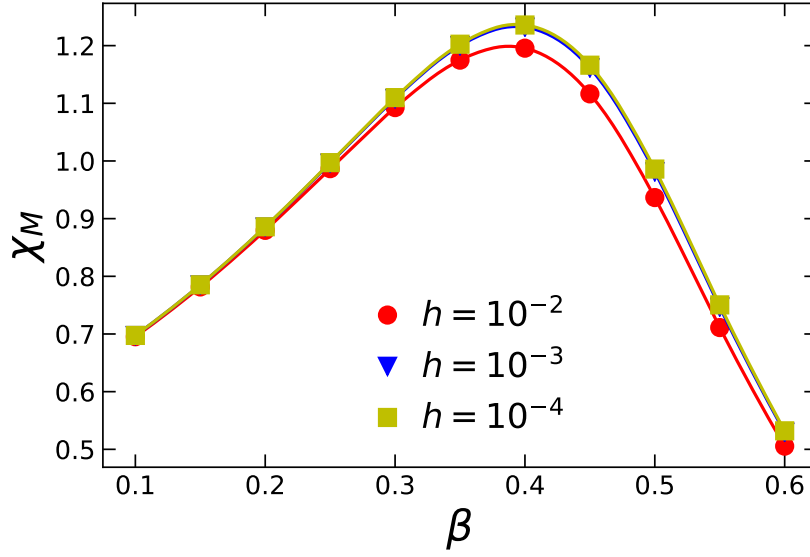
Figure 4.14 The small- \beta peak of magnetic susceptibility as a function of \beta for q = 4.3 . The peak height converges when the external field is taken to zero.
