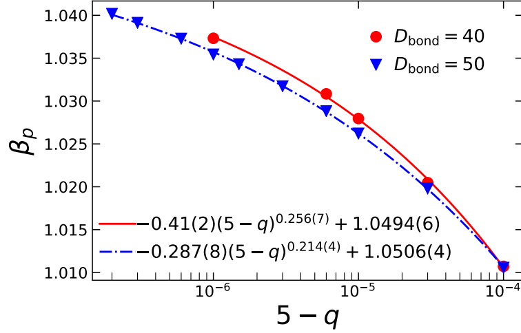
Figure 4.17 The power law extrapolation of the small- \beta peak position to q = 5 from below. Here the extrapolation gives \beta_c = 1.0506(4) .
