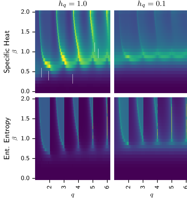
Figure 4.63 Heatmaps from TRG of the specific heat (top row) and entanglement entropy (bottom row) for the Extended-O(2) model with h_q = 1 (left column) and h_q = 0.1 (right column). Each pixel is a distinct TRG calculation performed with L = 1024 and bond dimension 40. There are a few missing points (white) in the top-left panel.
