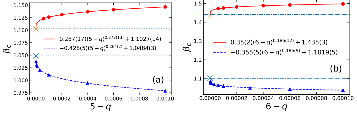
Figure 4.24 Power law extrapolation of the small- \beta peak position (triangles) of \chi_M with zero external field to q = 5 [lower curve in (a)] and to q = 6 [lower curve in (b)]. The same procedure is performed for the Ising critical points (circles) at higher \beta [upper curves in (a) and (b)]. The horizontal dashed lines in (a) are the locations of two BKT transitions for q = 5 obtained from Ref. [51]. The horizontal dash-dotted lines in (b) are the locations of two BKT transitions for q = 6 obtained from Ref. [133]. D_{\text{bond}} = 40 in (a) and D_{\text{bond}} = 60 in (b).
