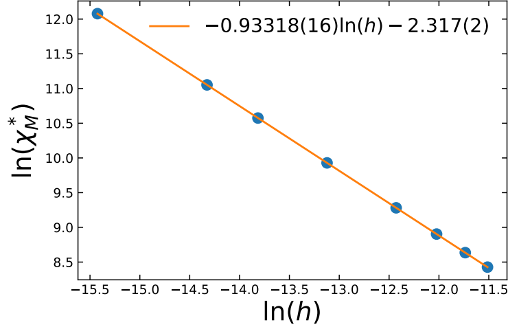
Figure 4.19 The maximal magnetic susceptibility in Fig. 4.22 as a function of the external field for q = 4.9 . A linear fit of the log-log plot gives the exponent \delta = 14.97(4) . This is consistent with the value \delta = 15 of the Ising universality class. D_{\text{bond}} = 40 .
