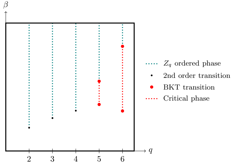
Figure 2.14 The phase diagram of the q -state clock model in two dimensions. The black points indicate critical points associated with second order phase transitions, and red points indicate critical temperatures associated with BKT phase transitions.
