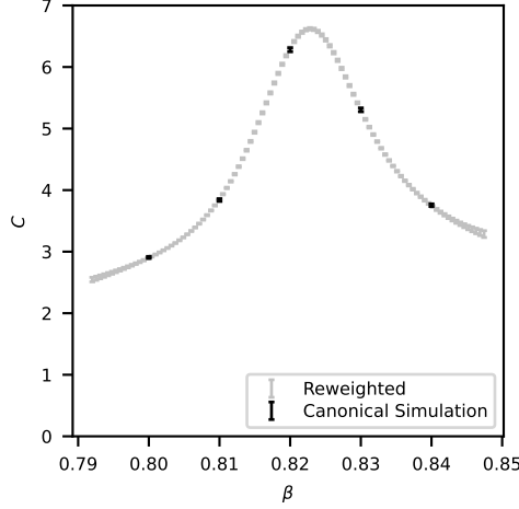
Figure 3.6 Here we show an illustration of how useful multihistogram reweighting can be to precisely locate the peak positions and heights for finite size scaling. The five black points are from canonical MCMC simulations, and the gray points are computed via multihistogram reweighting of the canonical time series. In this example, we are looking at the specific heat from the Extended- O(2) model (discussed in a later chapter) with q = 3 and h_q = 1 simulated on a 64 \times 64 lattice.
