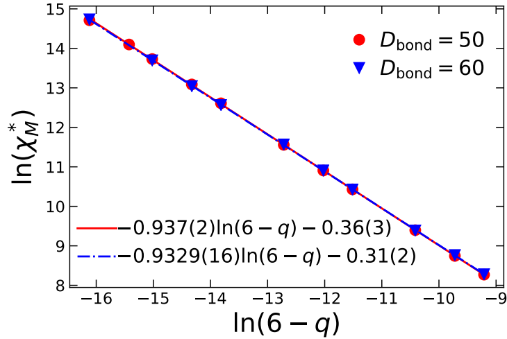
Figure 4.16 Same as Fig. 4.15, but for q \rightarrow 6^- .
