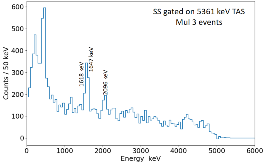
Figure 4.10 Singles Spectrum (SS) gated on the 5361 keV peak in the Total Absorption Spectrum and multiplicity (Mul) 3 events for the ^{33}\text{Mg} \beta -delayed \gamma rays from the SuN-miniDSSD dataset. Decay of the new proposed 5361 keV level via the 3714 keV level and the 1618 keV level in ^{33}\text{Al} can be confirmed.
