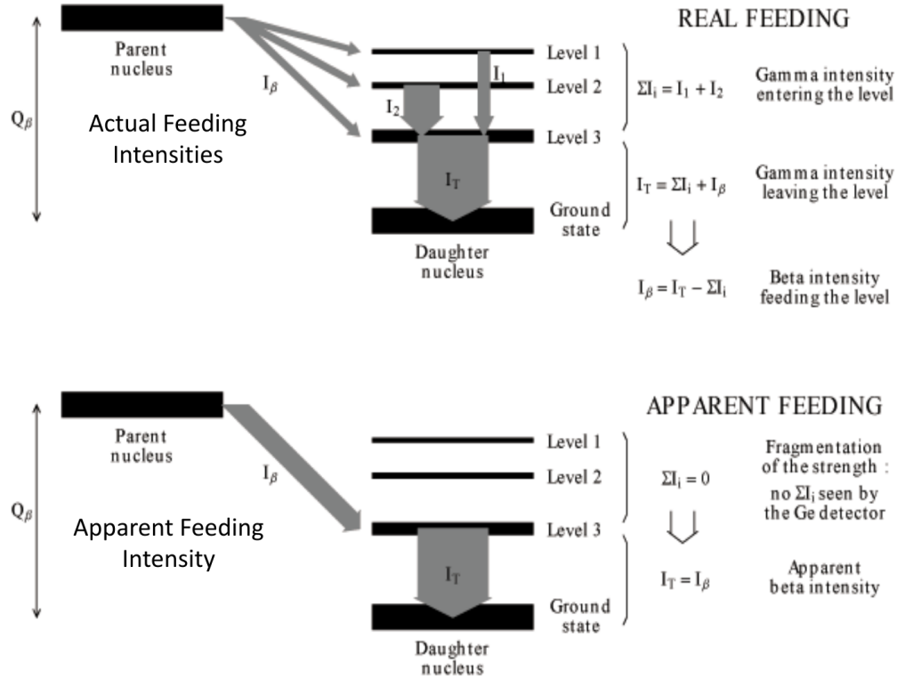
Figure 2.2 Schematic explanation of the Pandemonium effect [74]. Weak \beta -delayed \gamma -transitions from higher excitation energies are hard to detect with high-resolution \gamma -ray detectors. The inferred \beta -feeding intensities are then wrongly attributed to lower excitation energies. This is a known source of systematic error in data analysis. Figure adapted from [78].
