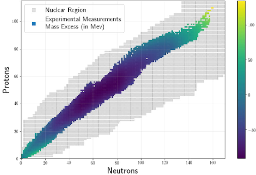
Figure 1.6 The nuclear masses landscape on the chart of nuclides. The colored region is for nuclei whose masses have been experimentally measured as of AME2020 database [62]. The grey region is the extent of nuclear existence, i.e. the region between the proton and the neutron driplines. Points in the grey area that aren't colored are nuclei whose masses remain to be measured experimentally.
