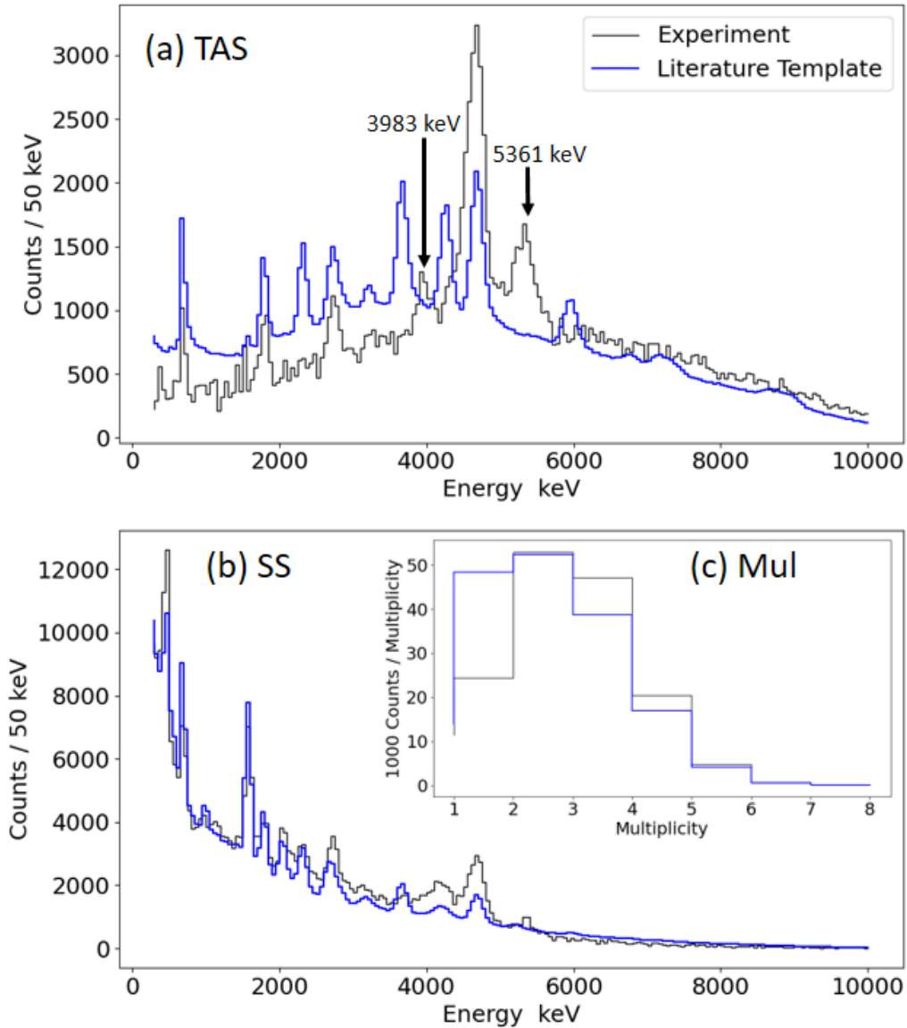
Figure 4.7 Comparison of the \beta -delayed \gamma experimental template from the \beta -decay of ^{33}\text{Mg} consisting of the Total Absorption Spectrum (TAS), Singles Spectrum (SS), and the multiplicity (Mul) from the SuN-miniDSSD dataset with the literature template obtained from GEANT4 simulations of the SuN detector based on \beta -feeding intensities reported by the National Nuclear Data Center (NNDC). Two new levels identified in ^{33}\text{Al} are highlighted in the TAS.
