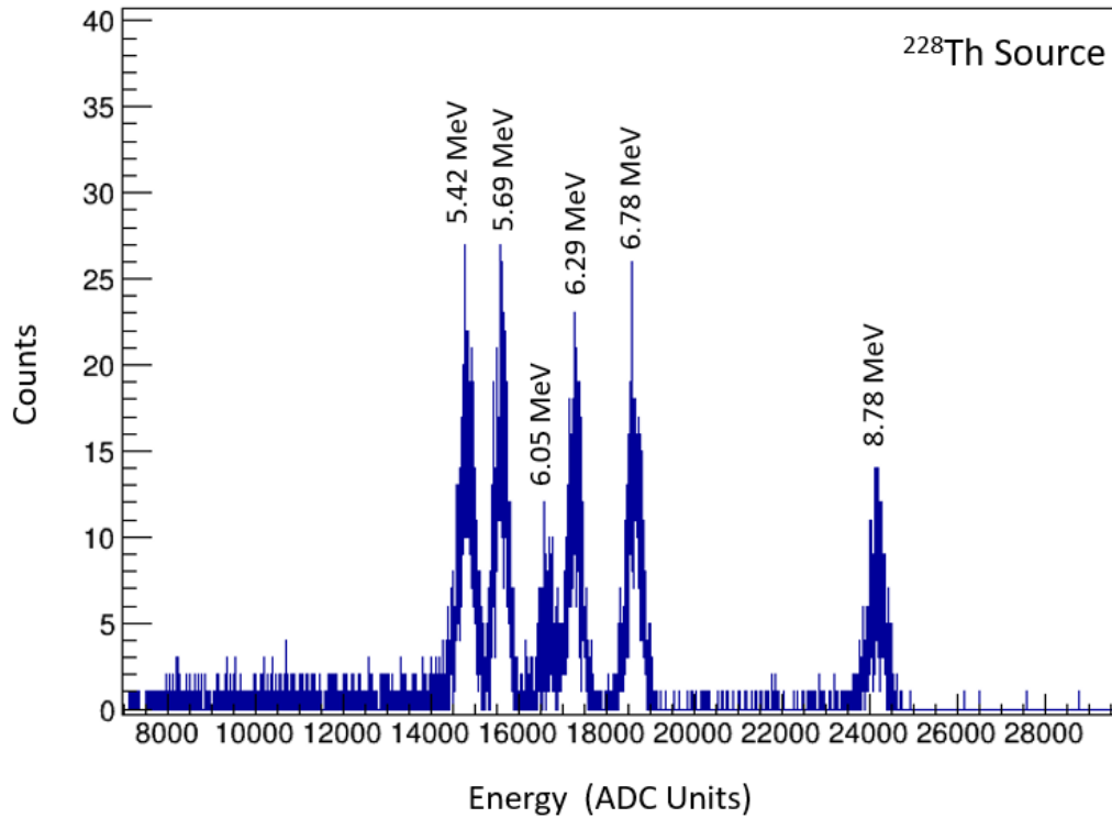
Figure 3.3 Energy spectrum for a sample BCS DSSD strip from a 228 Th energy calibration run. Six characteristic \alpha -peaks from the decay chain of 228 Th are shown in the figure. The centroids for Gaussian fits to the peaks were used for a linear energy calibration.
