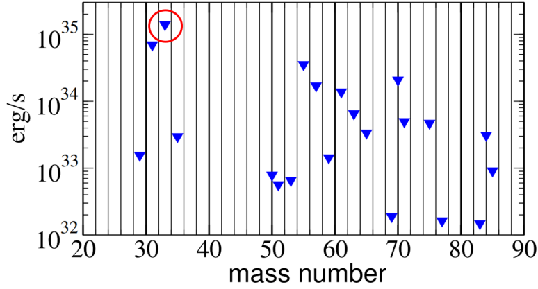
Figure 1.7 Urca cooling luminosity in a particular isobaric mass chain for a neutron star crust composed of typical Type-I X-ray burst ashes powered by rp-process as a function of mass number. These calculations are performed with the Xnet nuclear reaction network for a crust with a constant temperature of 0.5 GK. Mass A = 33 chain, circled in red, has the highest Urca cooling luminosity.
