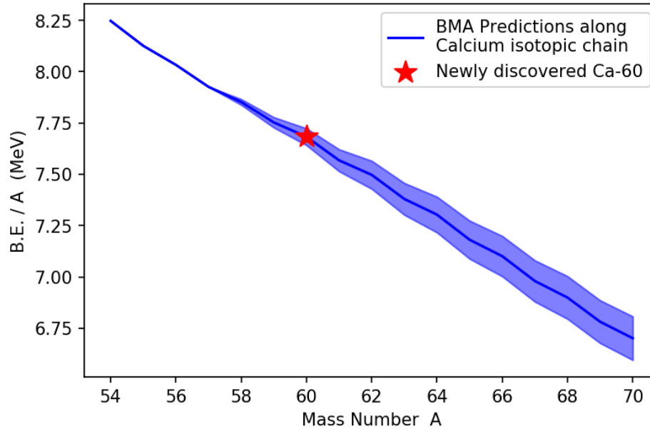
Figure 5.6 The trend in BMA predictions of binding energy per nucleon for the calcium isotopic chain. ^{60}\text{Ca} is the most exotic calcium isotope to be seen in the laboratory so far [146] but its mass hasn't been experimentally measured yet. The red star shows BMA prediction along with uncertainty.
