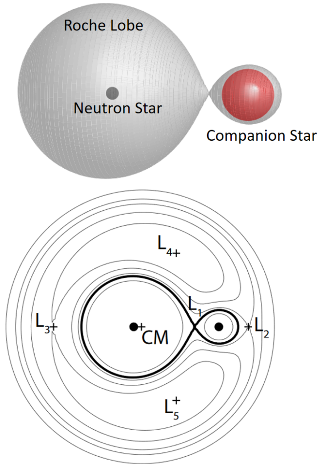
Figure 1.1 Accretion onto a neutron star via the mechanism of Roche lobe overflow. Matter is funneled into an accretion disk around the neutron star through the L1 Lagrange point. Figure modified from Ed Brown (private communication).
