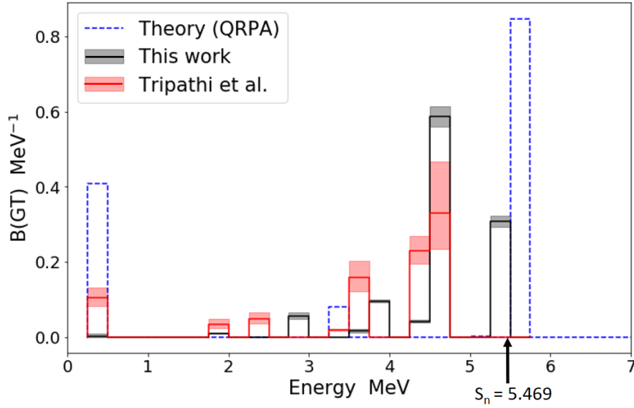
Figure 4.12 Comparison of the experimentally determined Gamow-Teller Transition strengths B(\text{GT}) for the \beta -decay of ^{33}\text{Mg} with Quasi-Random Phase Approximation (QRPA) calculations. Experimental B(\text{GT}) values can only be reliably determined up to the neutron separation energy S_n = 5469 keV.
