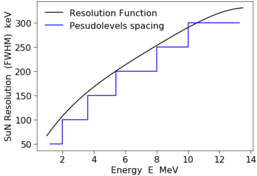
Figure 3.13 SuN photopeak energy resolution in keV calculated as a function of the incident \gamma ray energy. The resolution function used is from [87]. Also shown here is the pseudolevels spacing used for RAINIER and GEANT4 simulations. In these simulations, each pseudolevel represents the contribution from all the energy levels within that energy bin. As long as the spacing is smaller than SuN resolution, the resulting simulated spectra from any level and its corresponding pseudolevel should be nearly identical.
