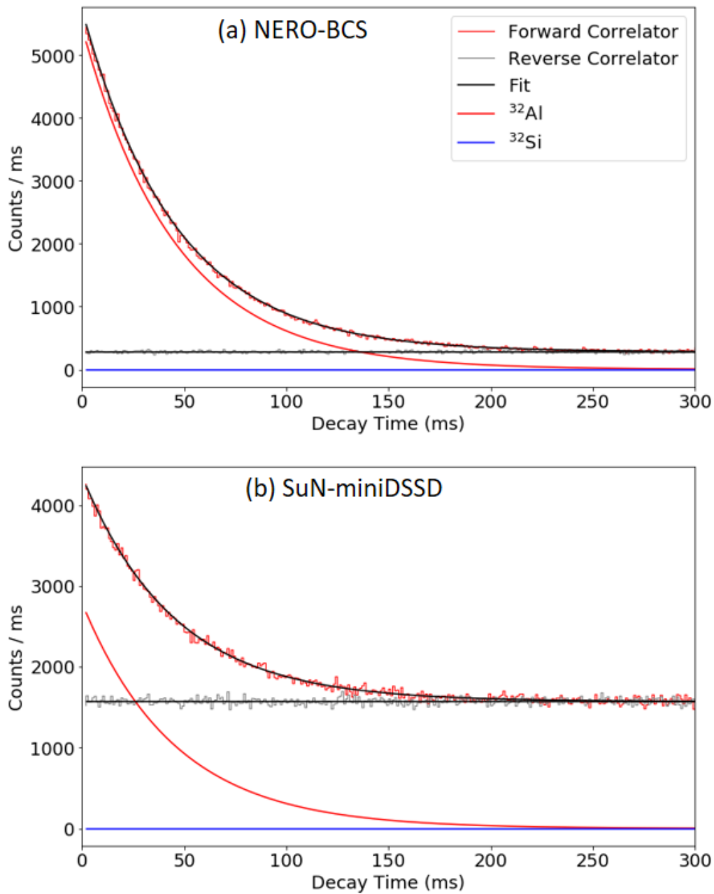
Figure 4.5 ^{32}\text{Al} decay curve fits for the (a)NERO-BCS and the (b)SuN-miniDSSD datasets. Half-lives are reported in Table 4.1.
