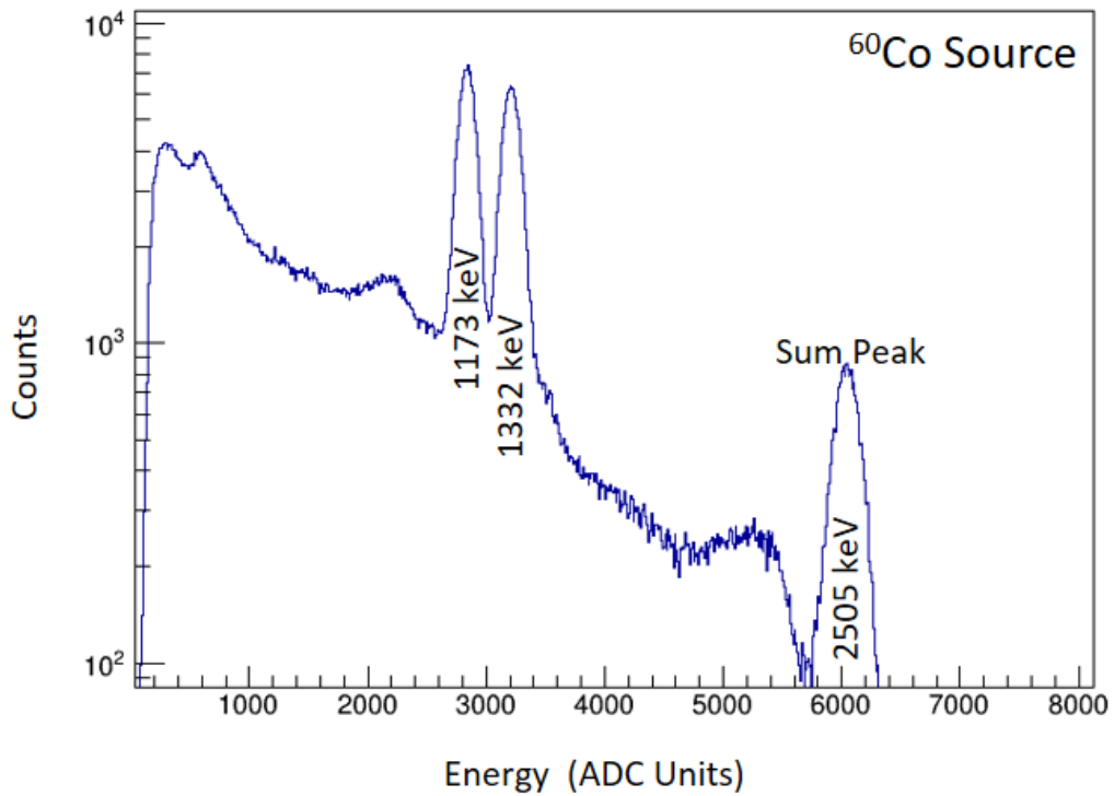
Figure 3.11 Example energy spectrum of a sample SuN Segment (with gain-matched PMTs) from ^{137}\text{Cs} and ^{60}\text{Co} calibration runs. The photopeaks are labeled in the figure corresponding to the \gamma energy. ^{60}\text{Co} calibration run also shows the sum peak.
