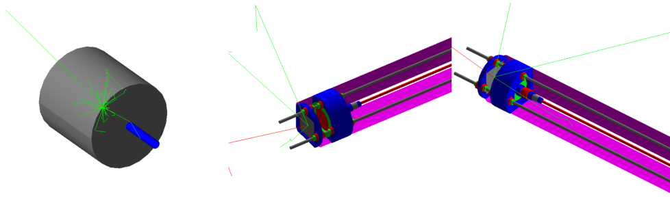
Figure 3.12 GEANT4 visualization of SuN detector in the left panel and the miniDSSD implantation detector in the middle and the right panel. Green lines are for visualizing the \gamma ray tracks whereas the red lines correspond to electron tracks. The green track outside the SuN detector volume represents partial energy deposition in the detector. Figure adapted from [87].
