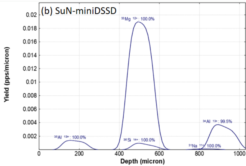
Figure 2.5 LISE++ [79] simulations for the optimized range distribution of ^{33}\text{Mg}^{12+} in the implantation silicon detectors for both parts of the experiment. All the fragments of interest are completely deposited in the center with minimal contaminants. Silicon detectors also have enough thickness to detect the \beta -decay electron.
