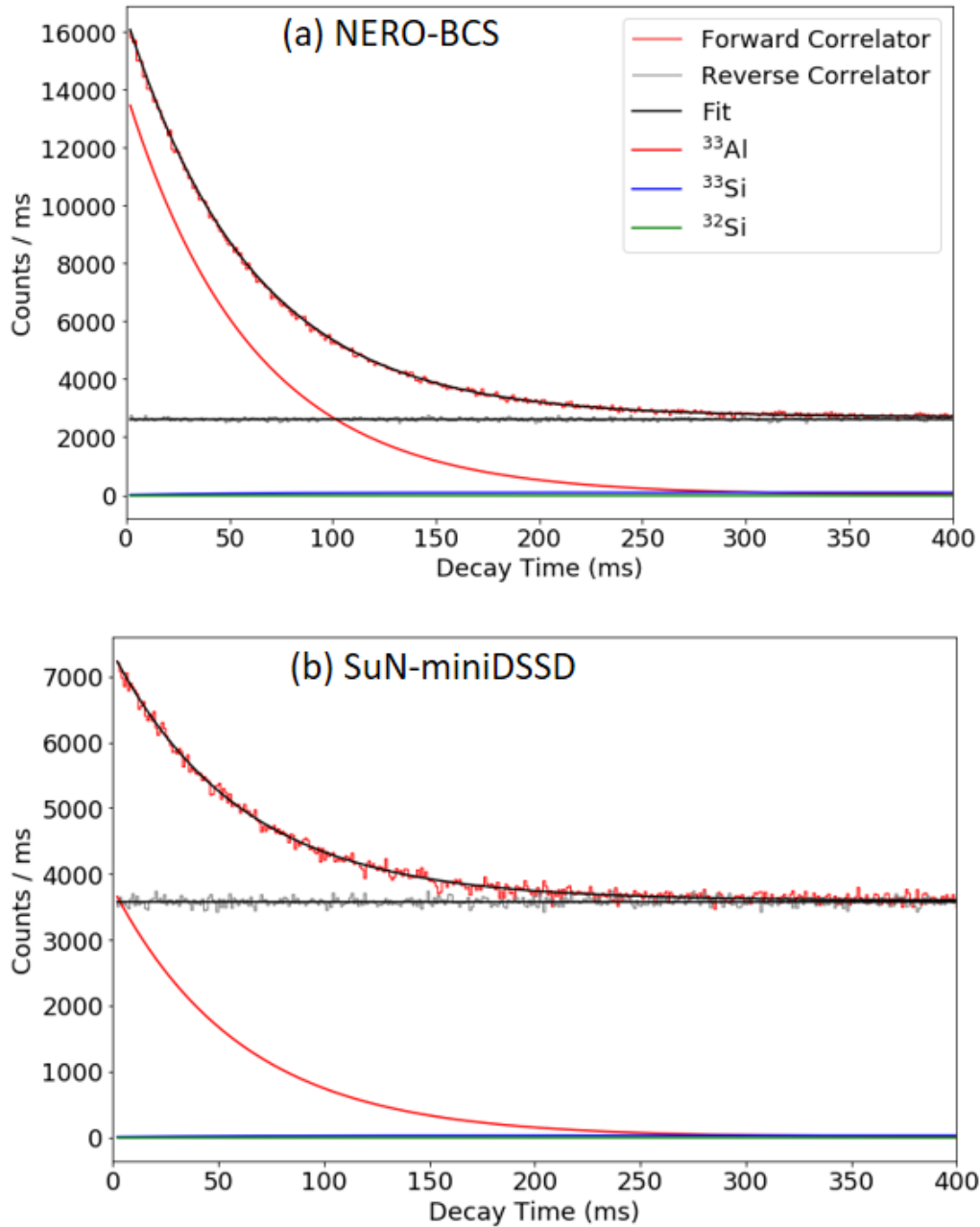
Figure 4.4 ^{33}\text{Al} decay curve fits for the (a)NERO-BCS and the (b)SuN-miniDSSD datasets. Half-lives are reported in Table 4.1.
