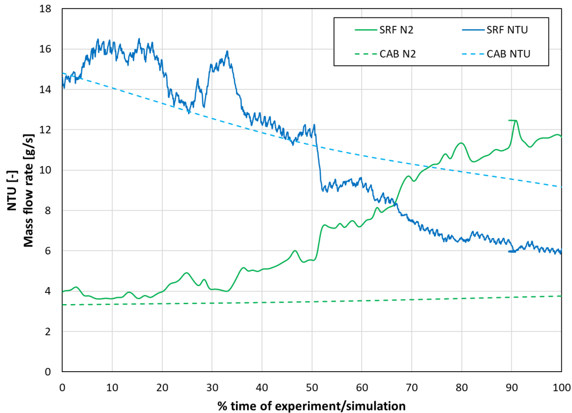
Figure 6-17 Freeze-out heat exchanger NTU and N2 usage compared with commercial purifier test data
