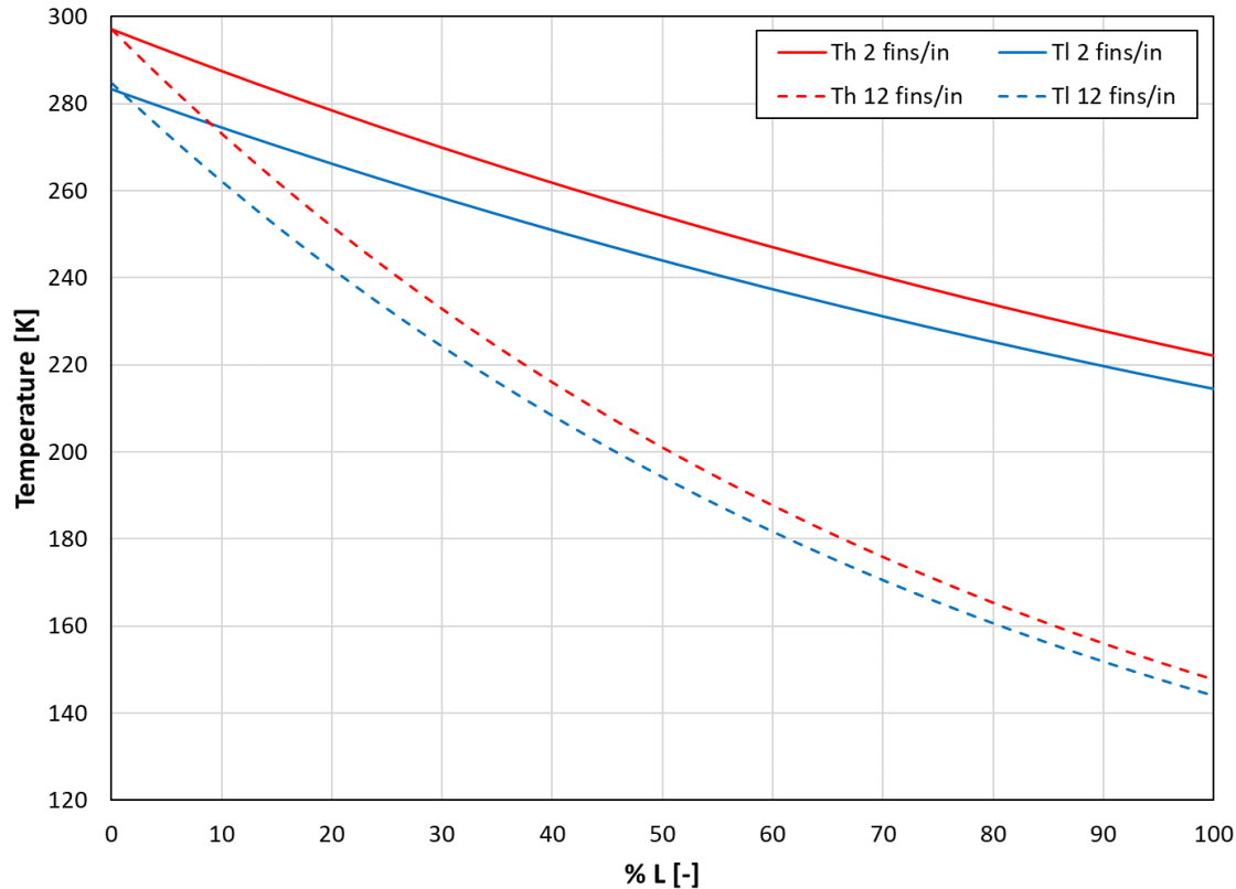
Figure 6-16 Fin density effect on heat exchanger cooling curves
