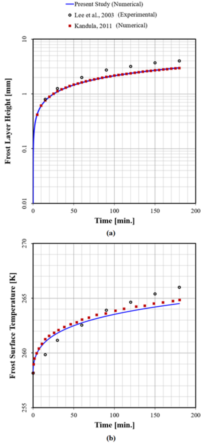
Figure 4-3 Comparison of calculated and measured [9, 11] (a) transient frost layer height and (b) frost surface temperature with humid air stream ( p_i = 1.0 bar, T_i = 288.2 K, T_w = 258.2 K, \omega_i = 0.00633 kg/kg air , and u_i = 2.5 m/s)
