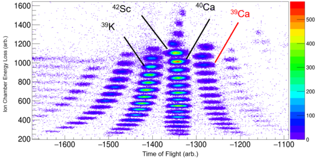
Figure 2.9 Energy loss in the S800 ion chamber as a function of time-of-flight between the E1 and OBJ scintillators. The energy loss vs TOF method is used to distinguish recoil nuclei from reactions between our choice of incoming secondary beam (in this case ^{42}\text{Sc} ) and outgoing reaction products.
