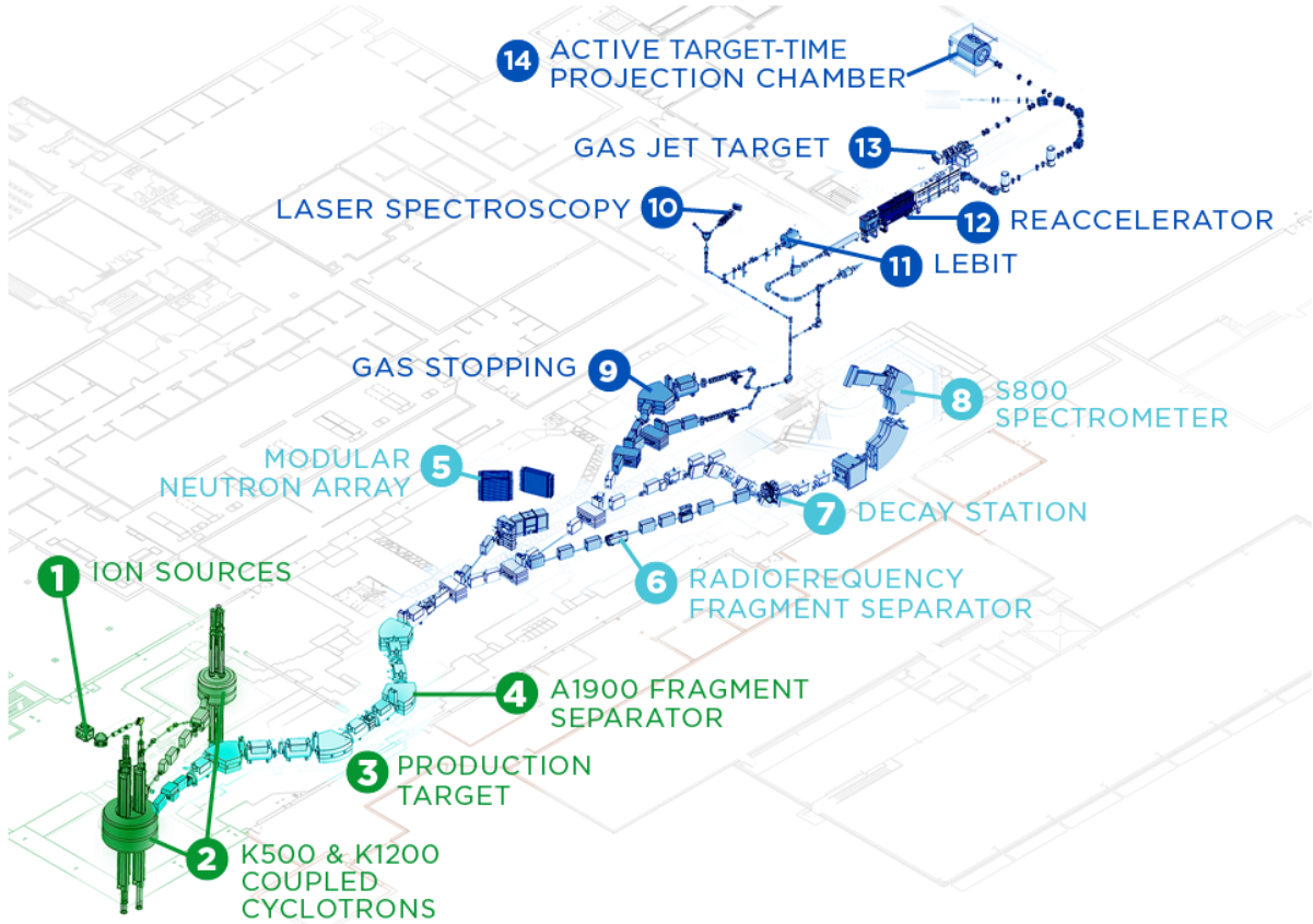
Figure 2.1 Beam line of the National Superconducting Cyclotron Laboratory (NSCL) [61]. The Superconducting Source for Ions (1) feeds ions to the Coupled Cyclotrons (2) which accelerates the primary beam particles to their maximum energy. The primary beam impinges on a production target (3) in which fragmentation reactions create a beam of various species of nuclei. These species are separated by the A1900 Fragment Separator (4) to produce the desired secondary beam(s). The secondary beam is sent to the S3 vault where TRIPLEX and GRETINA (sections 2.5.1 and 2.4.1, respectively) are located at the base of the S800 Spectrometer (8). Nuclei in excited states are produced in reactions on the TRIPLEX target, gamma rays are detected by GRETINA, and the recoil nuclei are identified by the S800. The beam may also be directed to other vaults where detectors such as the MONA (5) and the decay station (7) may be utilized. The beam can also be stopped and reaccelerated by the ReA facility (12) which directs a lower energy beam (single MeV/u) to a variety of other detectors such as the ATTPC (14) and SOLARIS (not depicted). The figure has been adopted from Ref. [61].
