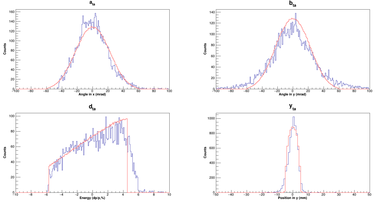
Figure 3.9 Trajectory distributions at the TRIPLEX degrader position for the reaction product ^{39}\text{Ca} taken during a run with target and degrader mounted. Data for the angle in the dispersive plane a_{ta} , angle in the non-dispersive plane b_{ta} , position in the non-dispersive plane y_{ta} , and the energy distribution d_{ta} are displayed in blue while the simulation is displayed in red.
