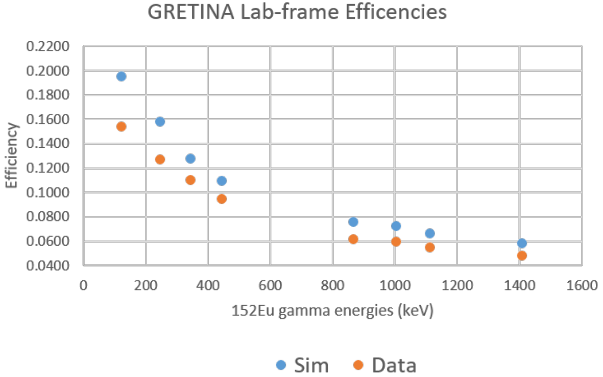
Figure 2.13 The efficiency of GRETINA at the ^{152}\text{Eu} gamma-ray energies observed in the lab-frame. The efficiency of the simulation at a given energy is given in blue while the efficiency of GRETINA is given in orange.
