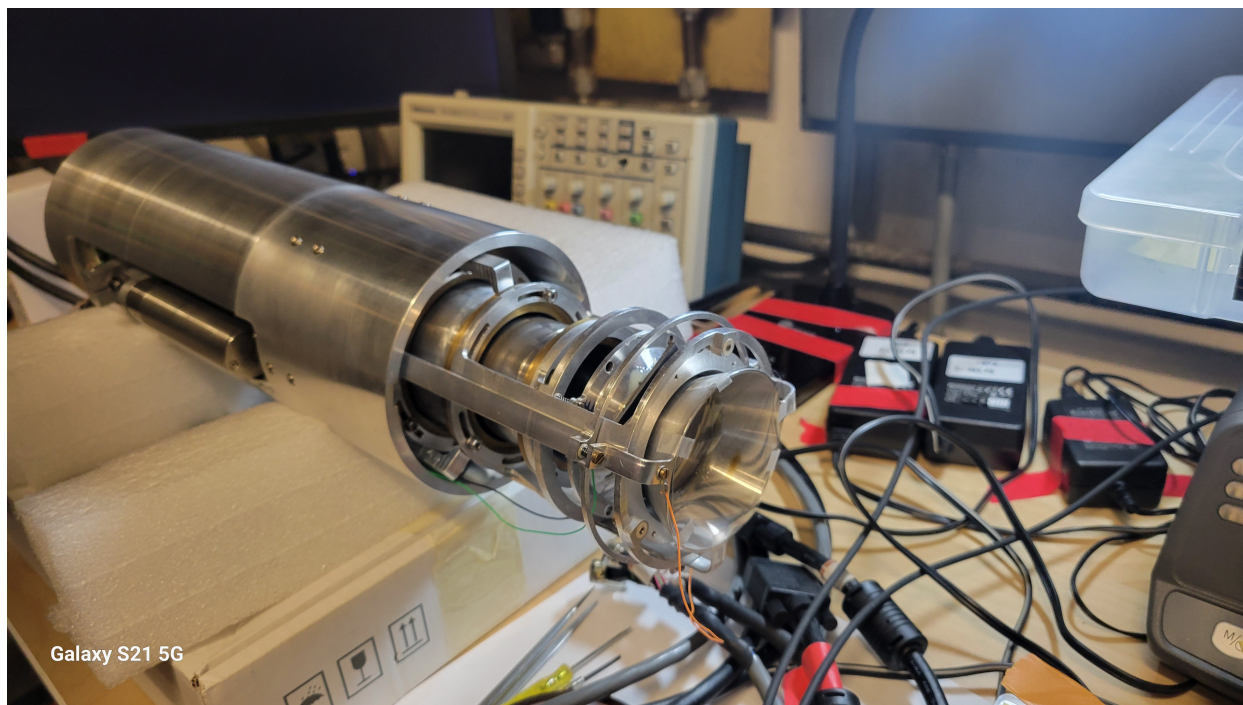
Figure 2.15 Full view of the TRIple PLunger for EXotic beams [57]. The secondary beam enters TRIPLEX from the back (left) and interacts with the target and degraders (right). The outer-most cylindrical housing protects motor control electronics and the TESA precision distance measurement system. A target motor is displayed on the left (small cylinder parallel with housing), this motor moves the inner cylinder which connects to the target ring.
