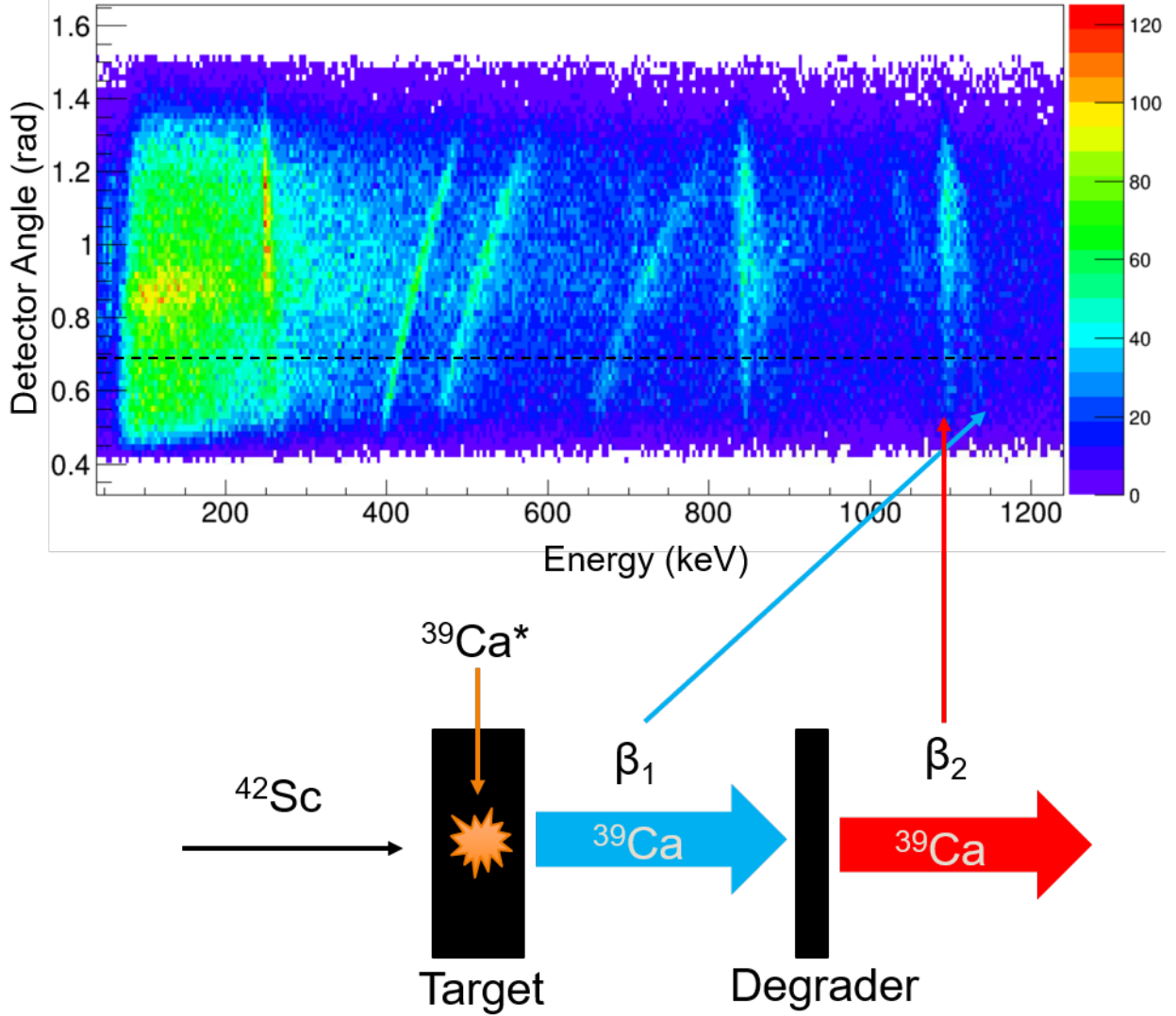
Figure 2.16 The ^9\text{Be}(^{42}\text{Sc}, ^{39}\text{Ca}^*)\text{X} reaction produces nuclei in excited states (denoted by “*”). Gamma rays may be emitted from “fast” nuclei of velocity \beta_1 or “slow” nuclei of \beta_2 , having been slowed by the degrader. The gamma-ray emittance angle (y-axis) is plotted as a function of the Doppler-corrected gamma-ray energy (x-axis) and the number of counts at a particular angle and energy (z-axis).
