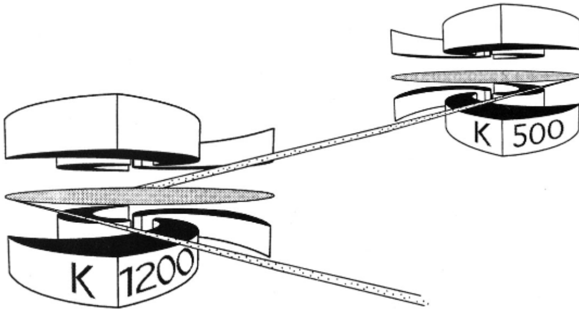
Figure 2.3 Coupled Cyclotron Facility design concept logo. [65]. The figure depicts the K500 and K1200 coupled cyclotrons and particles accelerated by the “dee” electrodes of the K500 which are then injected into the K1200 where they are accelerated to a higher energy, stripped of excess electrons, and then ejected toward the production target. The figure has been adopted from Ref. [65]. Reproduced with permission from Springer Nature.
