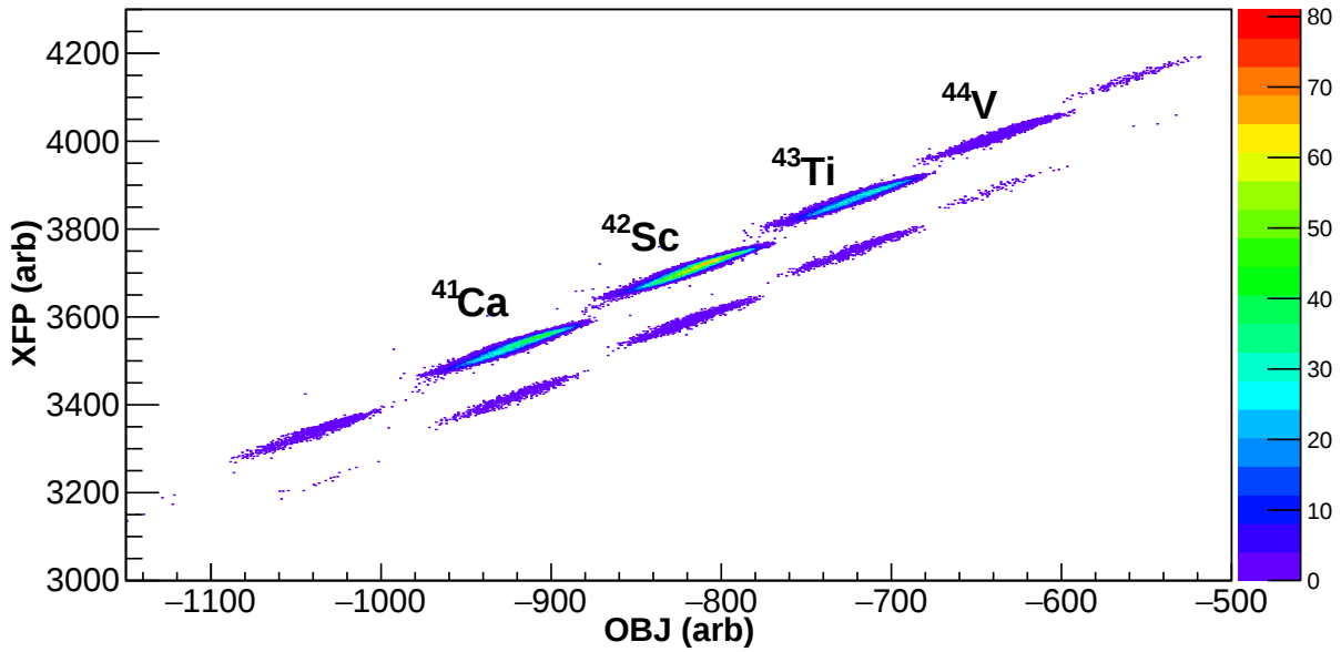
Figure 3.2 Secondary beam components separated by the TOF method where the time differences between the E1 and XFP or OBJ scintillators are plotted on their respective axes. The axes represent arbitrary units of time and the N = 21 isotones have been labeled for the reader. This plot was created from a run without the target installed in TRIPLEX and is used to characterize the secondary beam properties.
