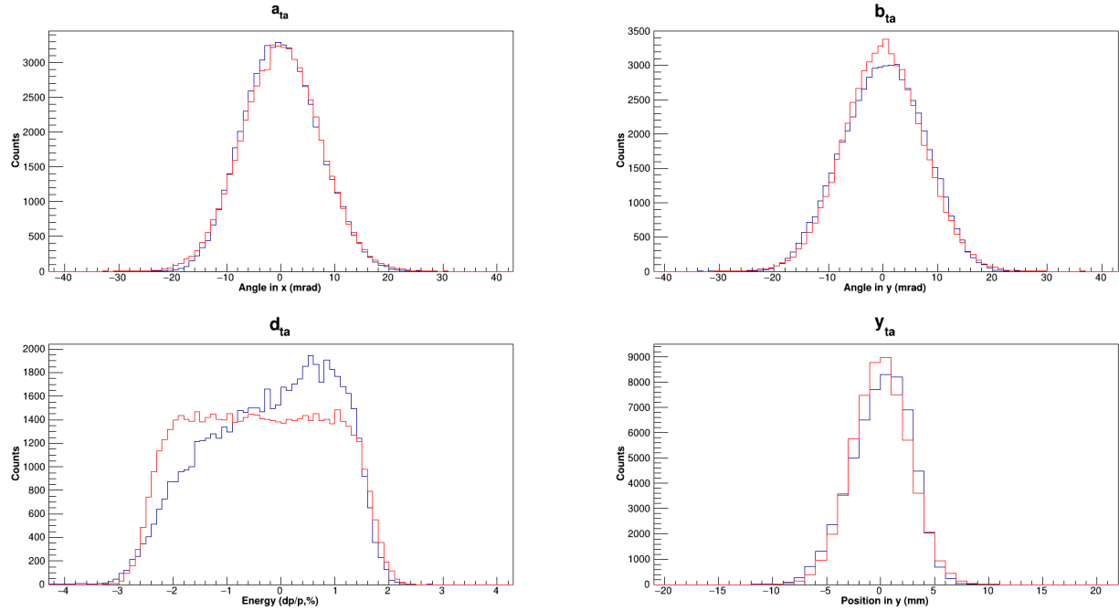
Figure 3.7 Trajectory distributions at the TRIPLEX target position for the unreacted ^{42}\text{Sc} beam. Experimental data for the angle in the dispersive plane a_{ta} , angle in the non-dispersive plane b_{ta} , position in the non-dispersive plane y_{ta} , and the energy distribution d_{ta} are displayed in blue. The simulated secondary beam trajectory information is displayed in red.
