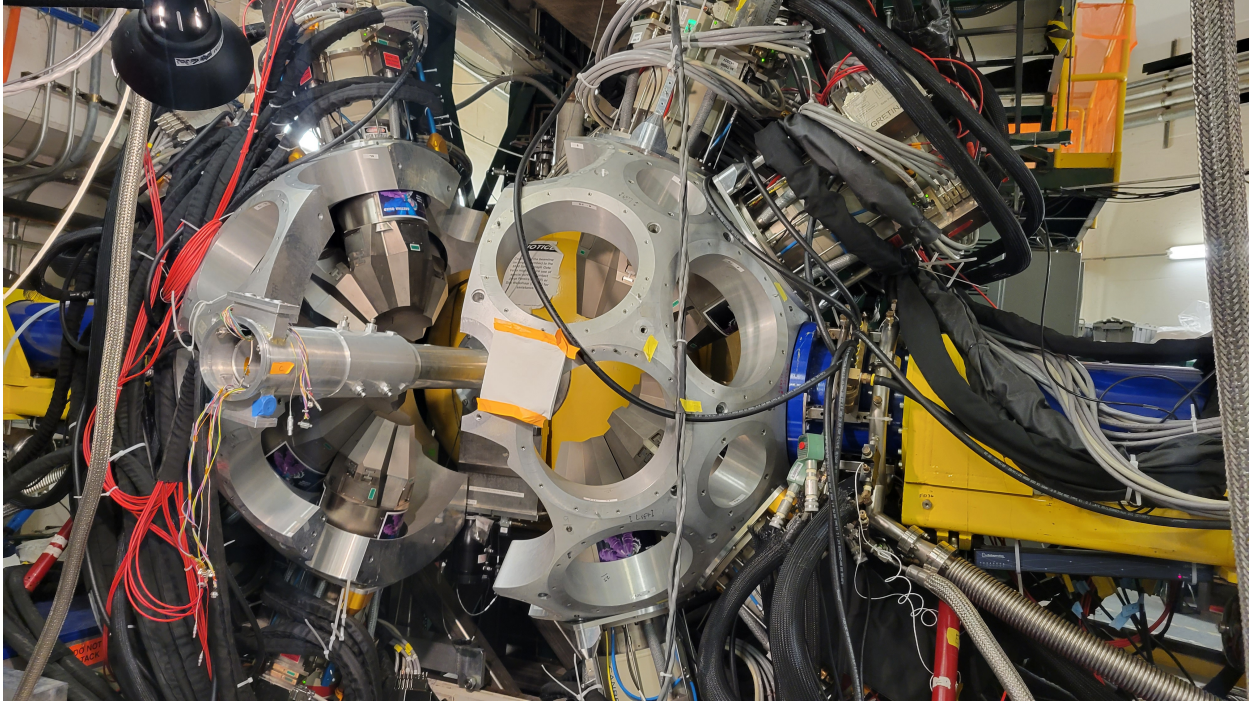
Figure 2.10 The Gamma-Ray Energy Tracking In-beam Nuclear Array with 12 modules positioned for perpendicular and forward focused detection. The module frame has been opened to allow connection of the TRIPLEX beam pipe to the S800 and alignment of the target with the beam spot. The secondary beam moves left to right and interacts with the TRIPLEX target which is located 13 cm upstream from the center of GRETINA. The beam then continues through the S800 for particle identification.
