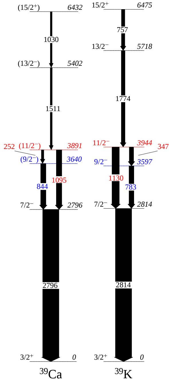
Figure 3.10 Level diagrams for gamma rays observed in the target-only spectra for ^{39}\text{Ca} (left) and ^{39}\text{K} (right). The energy information is from Ref.[45] and rounded to keV. The relative intensities of the observed gamma-ray transitions, indicated by the widths of the arrows, are normalized to the intensity of the 7/2^- \rightarrow 3/2^+_{g.s.} transition for the respective nuclei. The energy information for the (11/2^-) state is highlighted in red, while those for the (9/2^-) state are highlighted in blue [88]. Reprinted figure with permission from A. Sanchez et al. , Phys. Rev. C, vol. 110, p. 024322 (2024). Copyright (2024) by the American Physical Society.
