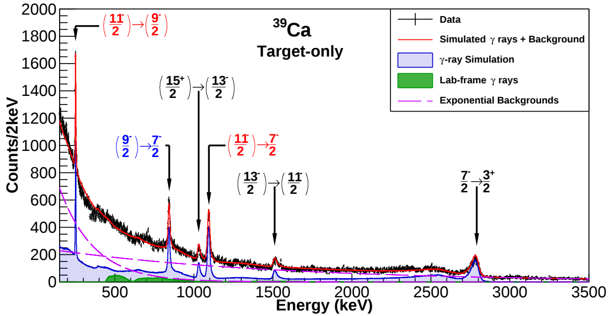
Figure 3.11 Doppler-corrected gamma-ray spectrum for ^{39}\text{Ca} for the target-only run. Transitions from the (11/2^-) state are labeled in red, from which the lifetime is determined in the present work. Gamma rays from the (9/2^-) state are labeled in blue, for which we provide an improved lifetime result [88]. Reprinted figure with permission from A. Sanchez et al. , Phys. Rev. C, vol. 110, p. 024322 (2024). Copyright (2024) by the American Physical Society.
