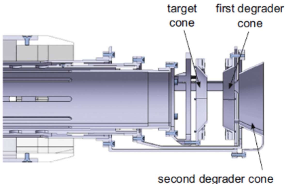
Figure 2.14 Diagram of the TRIPLE PLunger for EXotic beams [57]. TRIPLEX is designed to hold a production target and two degraders. In this diagram, the secondary beam enters from the left then interacts with a ^9\text{Be} target mounted on the target cone which can be moved toward or away from the stationary first degrader cone to allow measurement of lifetimes generally the 10s of picoseconds. Although TRIPLEX can hold a second degrader in the secondary degrader cone, the second degrader was not required for this experiment but the second degrader cone held a stripper foil to increase the number of fully stripped ions. Reprinted from Nuclear Instruments and Methods in Physics Research Section A: Accelerators, Spectrometers, Detectors and Associated Equipment, Vol. 806, H. Iwasaki et al. , The TRIPLE PLunger for EXotic beams TRIPLEX for excited-state lifetime measurement studies on rare isotopes, Pages No.123-131, Copyright (2016), with permission from Elsevier.
