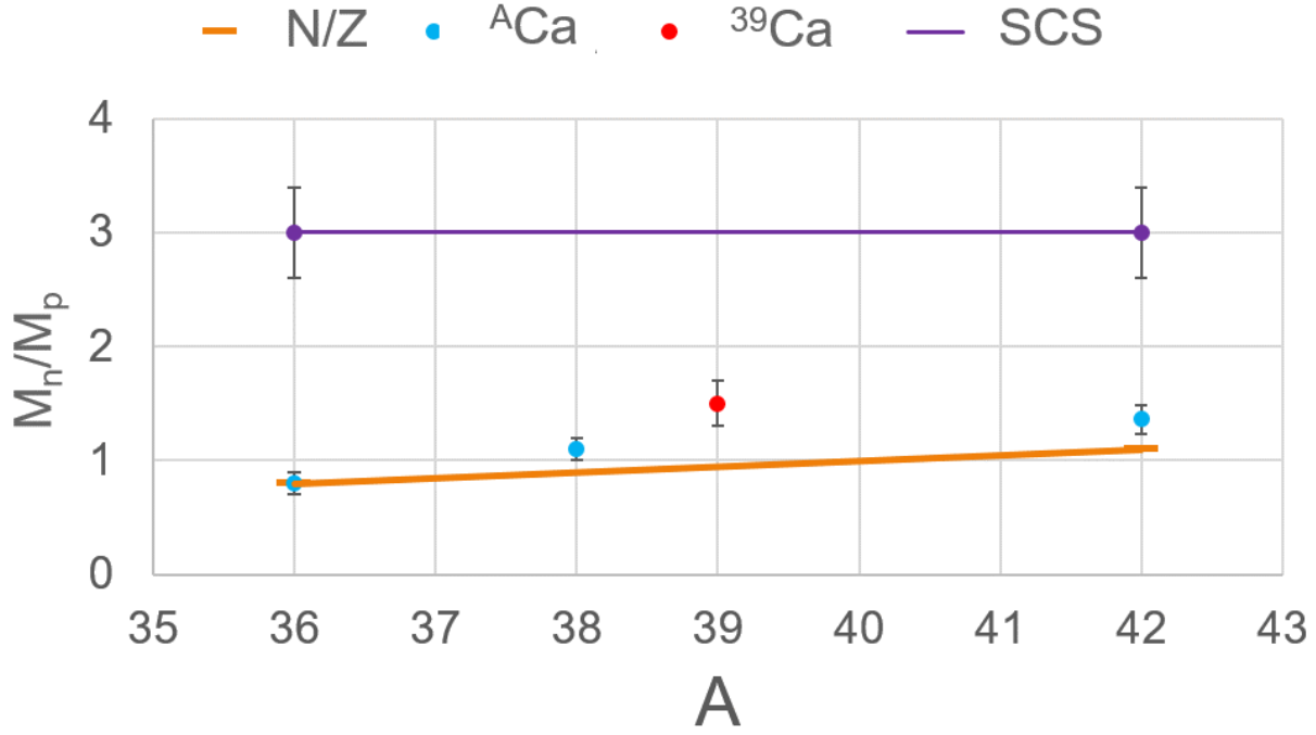
Figure 4.1 Ratios M_n/M_p for calcium isotopes near N = Z compared to the homogeneous collective model ( N/Z ) and the single-closed shell (SCS) estimation e_p/e_n = 3.0(4) . The figure shows an enhanced M_p when compared to the SCS expectation. The A = 36 ratio was obtained from Refs. [49, 48]. The A = 38 ratio is from Refs. [43, 44]. The A = 39 ratio is from this work [88]. And Ref. [40] provides the A = 42 ratio.
