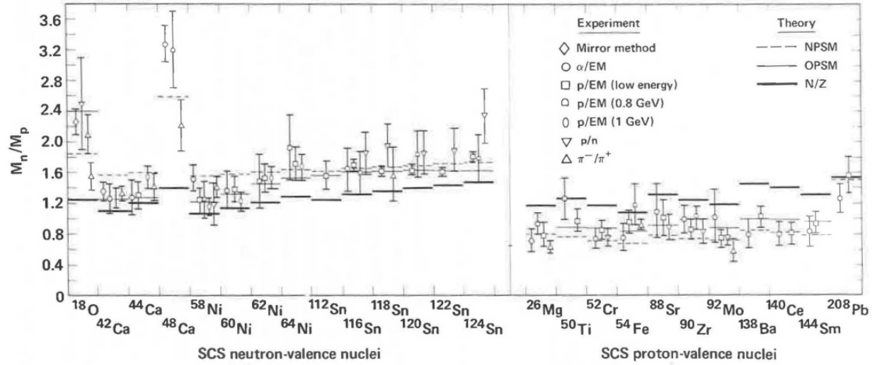
Figure 1.7 The ratios M_n/M_p for the lowest 2^+ \rightarrow 0^+ transitions in various single closed shell (SCS) nuclei and doubly magic ^{48}\text{Ca} and ^{208}\text{Pb} . The data was obtained from hadron scattering experiments and the mirror method described by Eqn. 1.7. Measurements are compared to the homogeneous collective model expectation ( N/Z ), the no-free parameter schematic model (NPSM), and the one-free parameter schematic model (OPSM) [46]. Reprinted from Physics Letters B, Vol. 4, A.M. Bernstein et al. Neutron and proton transition matrix elements and inelastic hadron scattering, Pages No. 255-258, Copyright (1981), with permission from Elsevier.
