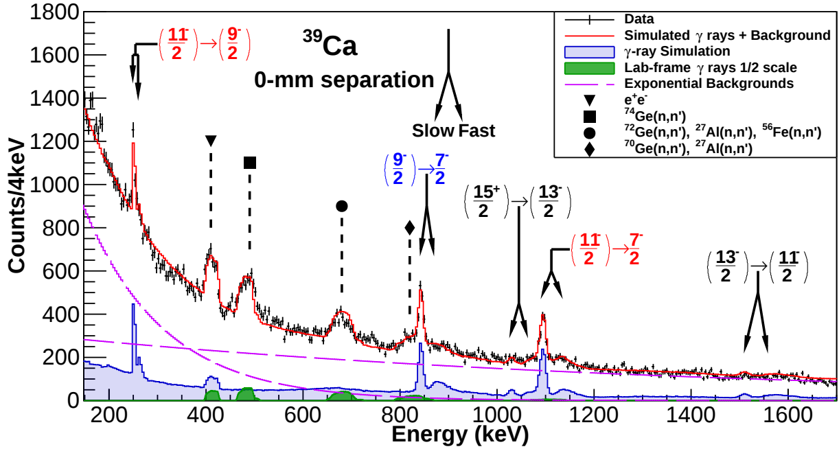
Figure 3.13 Doppler-shift corrected gamma-ray spectrum for ^{39}\text{Ca} taken with the 0-mm target-degrader separation setting. The spectrum has been gated between \theta = 29^\circ and \theta = 46^\circ to improve sensitivity to Doppler shifts. Transitions from the (11/2^-) state are labeled in red, while transitions from the (9/2^-) state are labeled in blue. Laboratory-frame background gamma rays are shown in green and downscaled by a factor of 2 [88]. Reprinted figure with permission from A. Sanchez et al. , Phys. Rev. C, vol. 110, p. 024322 (2024). Copyright (2024) by the American Physical Society.
