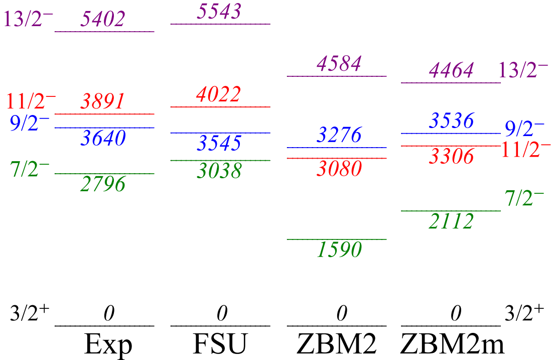
Figure 4.2 Level energies of the lowest 7/2^- , 9/2^- , 11/2^- , and 13/2^- states of ^{39}\text{Ca} from experiment (Exp) compared to shell-model calculations with the FSU [94], ZBM2 [95], and ZBM2m [96] effective interactions [88]. Reprinted figure with permission from A. Sanchez et al. , Phys. Rev. C, vol. 110, p. 024322 (2024). Copyright (2024) by the American Physical Society.
