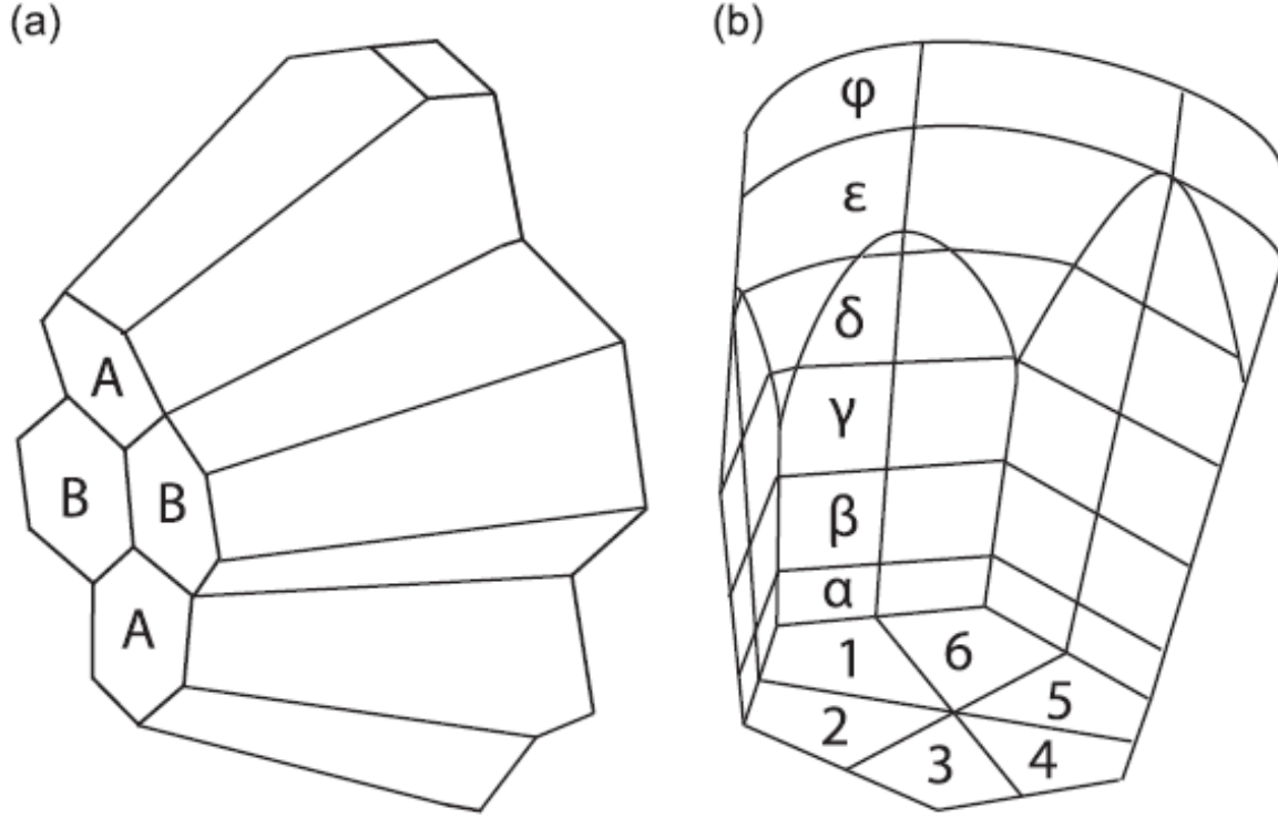
Figure 2.12 Diagram of a GRETINA “quad” (a) and a single crystal segmentation (b) [58]. Each GRETINA module contains a quad of four, closely-packed HPGe crystals (a) with the two pairs of crystals each having unique tapered-hexagonal shapes (A-type and B-type) and length of approximately 9 cm and maximum width of 8 cm. The tapered-hexagonal shapes provide maximum detector volume and solid-angle coverage. Each crystal contains a 36-fold segmentation (b) with a central core contact to collect total energy deposited and each segment with an individual outer-surface contact pad to determine interaction location (36 pads per crystal). The segmentation of each crystal allows for interaction position resolution of approximately 2 mm and tracking of gamma-ray interaction points throughout the detector volume [58]. Reprinted from Nuclear Instruments and Methods in Physics Research Section A: Accelerators, Spectrometers, Detectors and Associated Equipment, Vol. 709, S. Paschalis et al. , The performance of the gamma-ray energy tracking in-beam nuclear array GRETINA, Pages No. 44-55, Copyright (2013), with permission from Elsevier.
