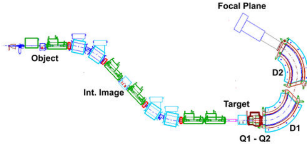
Figure 2.5 The S800 Spectrograph. After exiting A1900 focal plane scintillator XFP (left of diagram), the secondary beam components interact with the S800 object plane scintillator (OBJ). The time-of-flight (TOF) method is used to determine the secondary beam components with the E1 scintillator at the end of the focal plane acting as a reference and trigger. The focal plane and the detector components that comprise it are presented in Fig. 2.6. The figure has been adopted from Ref. [70].
