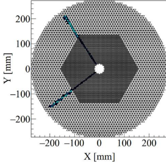
Figure 4.17 Projection of simulated ( d, {}^2\text{He} ) event on the Micromegas plane. Beam-like particles pass through the 3 cm aperture in the central region. Figure obtained from Ref. [107].
