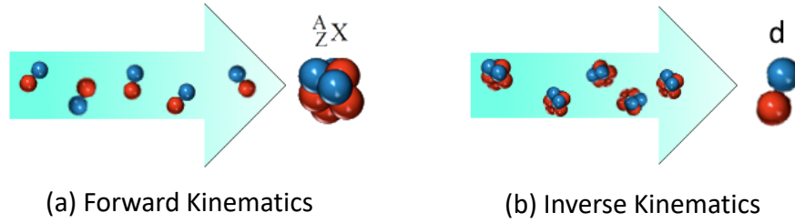
Figure 1.10 (a) In forward kinematics, the heavy isotope is used as the target and the light isotope which in this case is the deuteron is used as the beam. (b) In inverse kinematics, the unstable heavy isotope is used as the beam and impinged on the lighter isotope used as a target.
