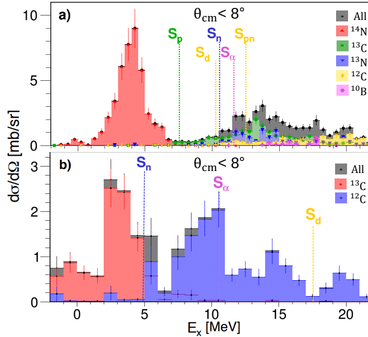
Figure 1.11 Differential cross-sections for the (a) {}^{14}\text{O}(d, {}^2\text{He}) and (b) {}^{13}\text{N}(d, {}^2\text{He}) reactions are depicted for \theta_{\text{c.m.}} \leq 8^\circ . The dashed lines in the figure represent separation energy for different decay channels, while the different colors indicate which residual particle was detected in the S800, as labeled. Figure has been taken from Ref. [68].
