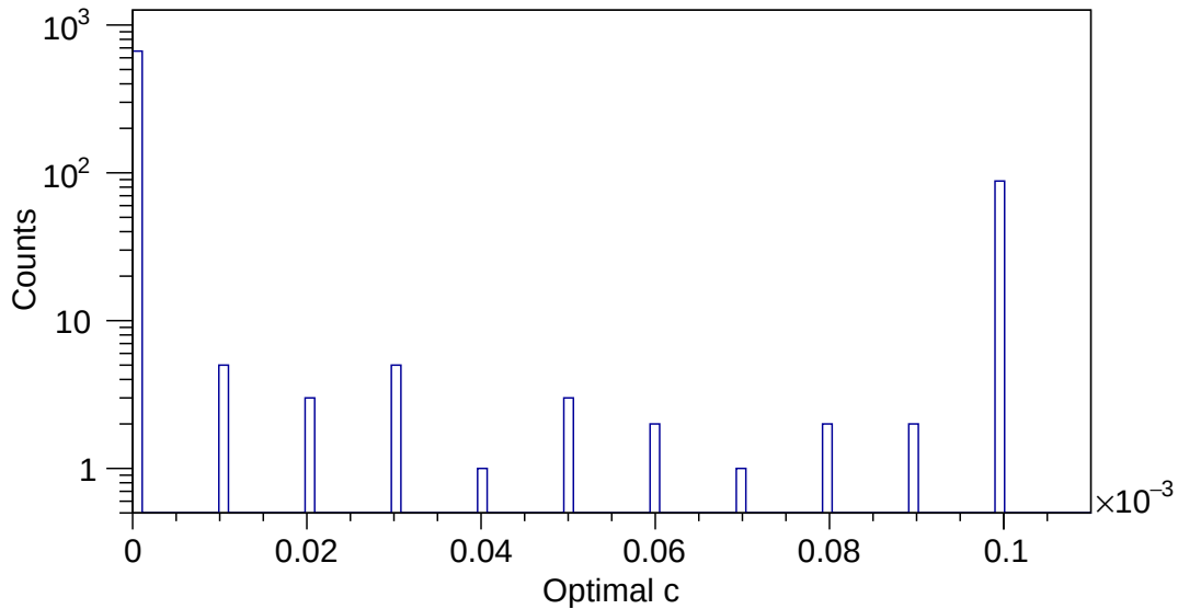
Figure 4.12 Distribution of the optimal curvature parameter c used in the track fitting analysis for the {}^{33}\text{Al}(d, {}^2\text{He}){}^{33}\text{Mg} reaction, plotted on a logarithmic scale. The majority of events exhibit minimal track curvature, as indicated by the peak at c = 0 . The corresponding low \chi^2 values show that space-charge corrections did not significantly improve the fits, leading to the decision not to apply them in the final analysis.
