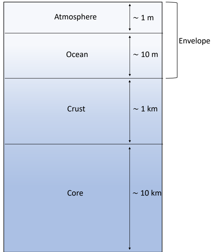
Figure 1.1 Regions of a neutron star with their approximate depths. Note that the depths of different layers are not drawn to scale.
