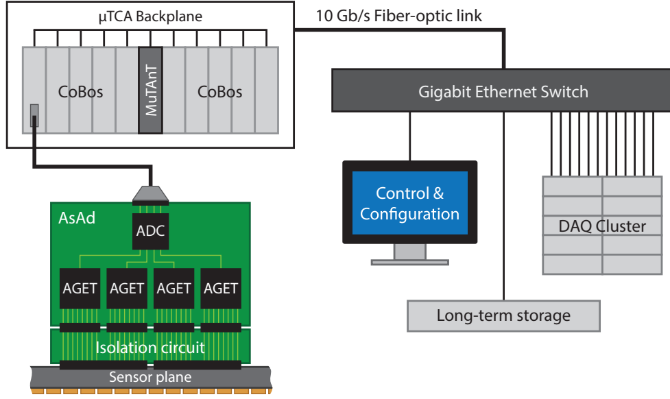
Figure 3.6 Schematic of GET electronics system. Only one out of 40 AsAd boards is shown here for clarity. Figure has been taken from Ref. [105].
