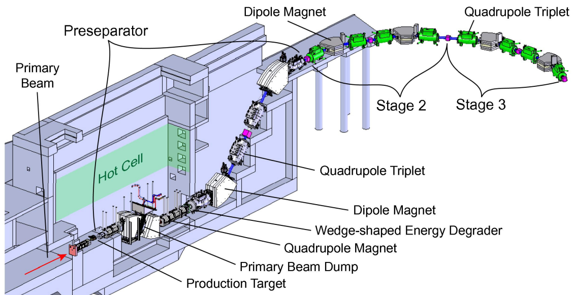
Figure 3.1 Schematic layout of ARIS consisting of three stages. The preseparator stage takes place underground whereas the second and third stage take place at ground. Figure has been taken from Ref. [95].
