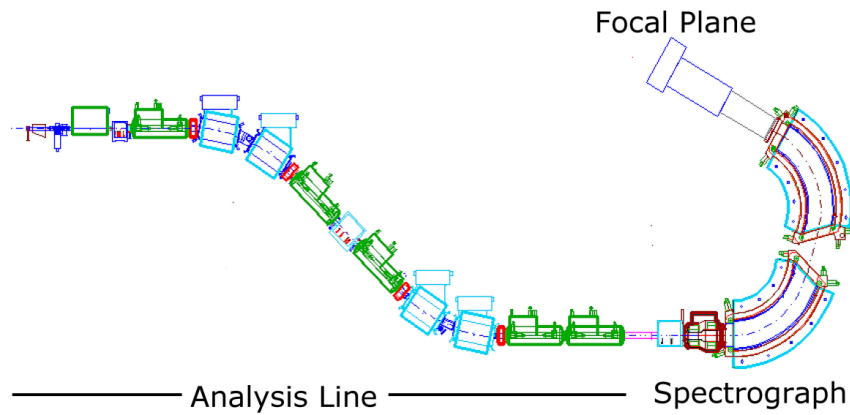
Figure 3.2 Schematic layout of the S800 analysis line and spectrometer in the S3 vault at FRIB. Figure adapted from Ref. [97].
