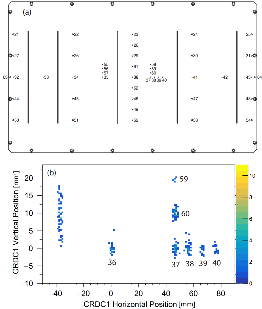
Figure 4.1 (a) Mask used for calibration of the CRDCs. (b) Position measurements for CRDC1 mask calibration. The measurements associated with the known hole positions in the mask are used to measure the offset and slope of the y-position as explained in text.
