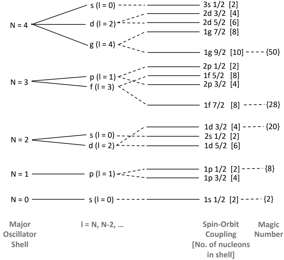
Figure 1.5 Low-lying energy levels shown for a single-particle shell model.
