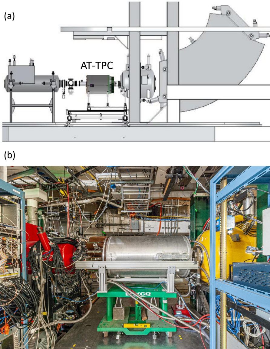
Figure 3.7 (a) Schematic layout of the AT-TPC at the target location of the S800 used for the experiment. Figure has been taken from Ref. [102]. (b) Picture of the AT-TPC at the target location of the S800 after installation of the cabling system prior to the start of the experiment.
