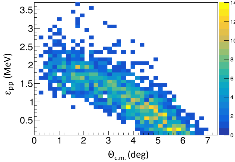
Figure 4.19 Correlation between the relative proton energy \epsilon_{pp} and the center-of-mass scattering angle \theta_{c.m.} for the experimental data from the ^{14}\text{O}(d,^2\text{He})^{14}\text{N} reaction inside the sensitive region of AT-TPC. The figure has been taken from Ref. [68].
