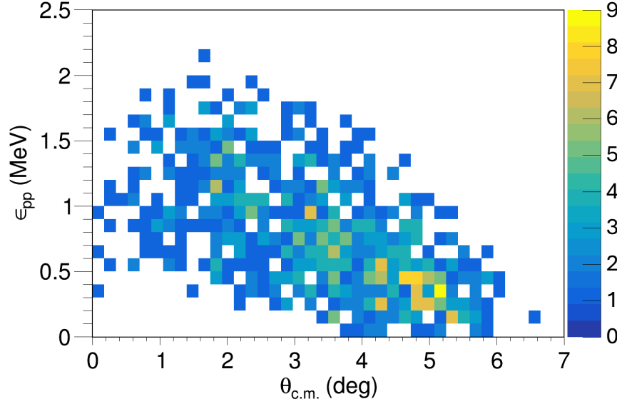
Figure 4.20 Correlation between the relative proton energy \epsilon_{pp} and the center-of-mass scattering angle \theta_{c.m.} for the experimental data from the ^{33}\text{Al}(d, ^2\text{He})^{33}\text{Mg} reaction inside the sensitive region of AT-TPC.
