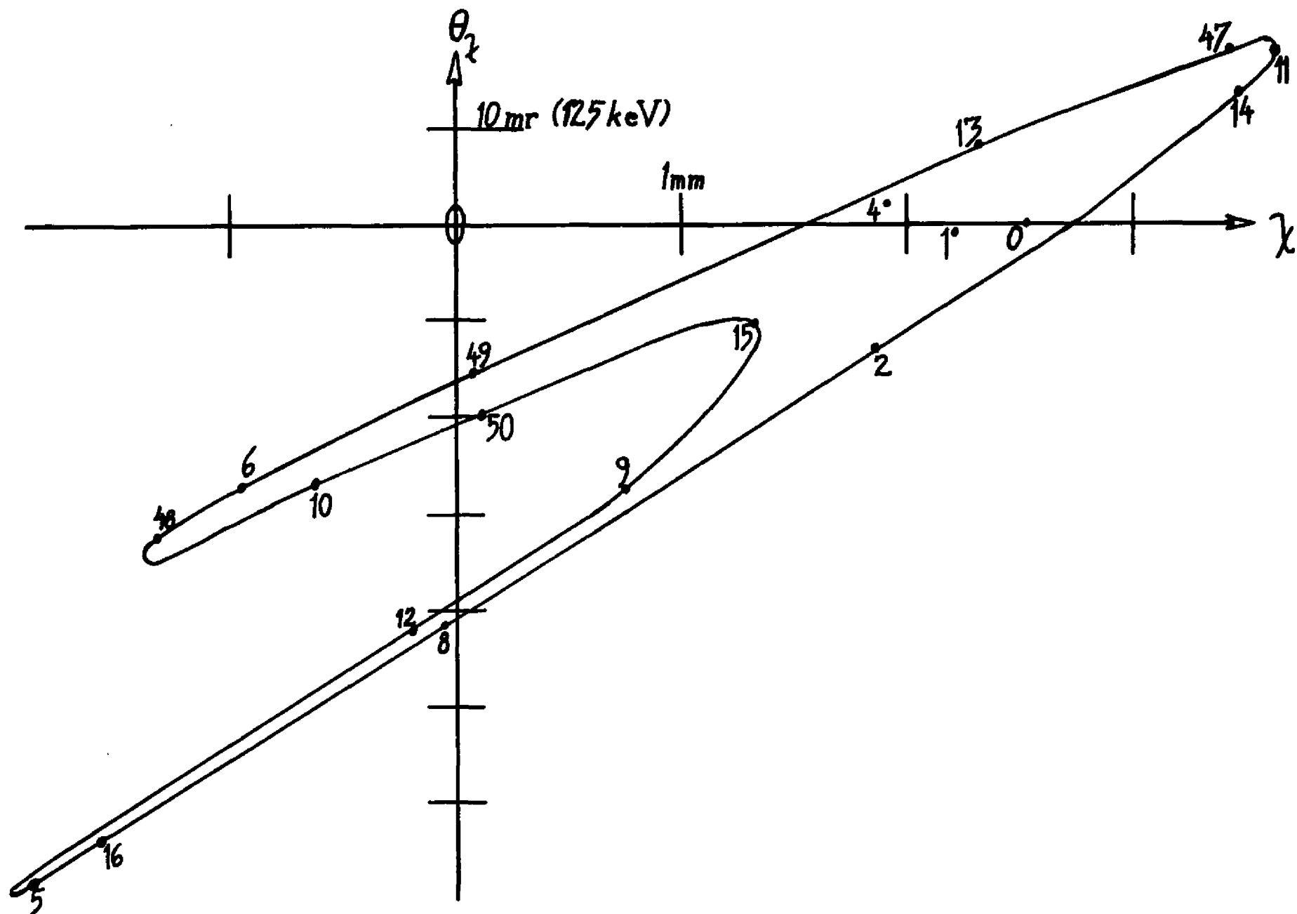
Fig. 4.2.--Median plane emittance at the exit of the outer inflector.
