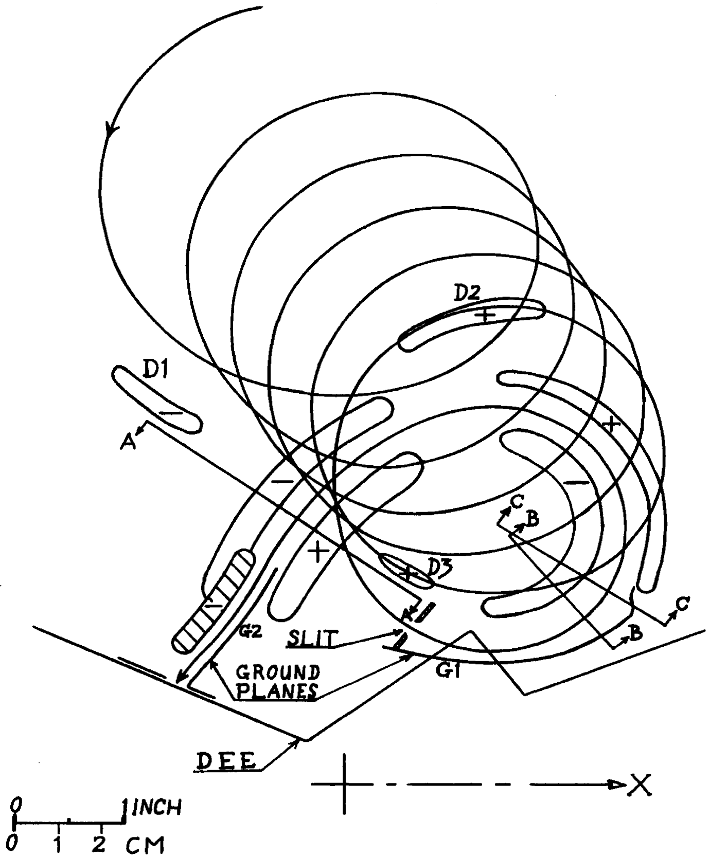
Fig. 3.3.--Inner inflector system --median plane view.
