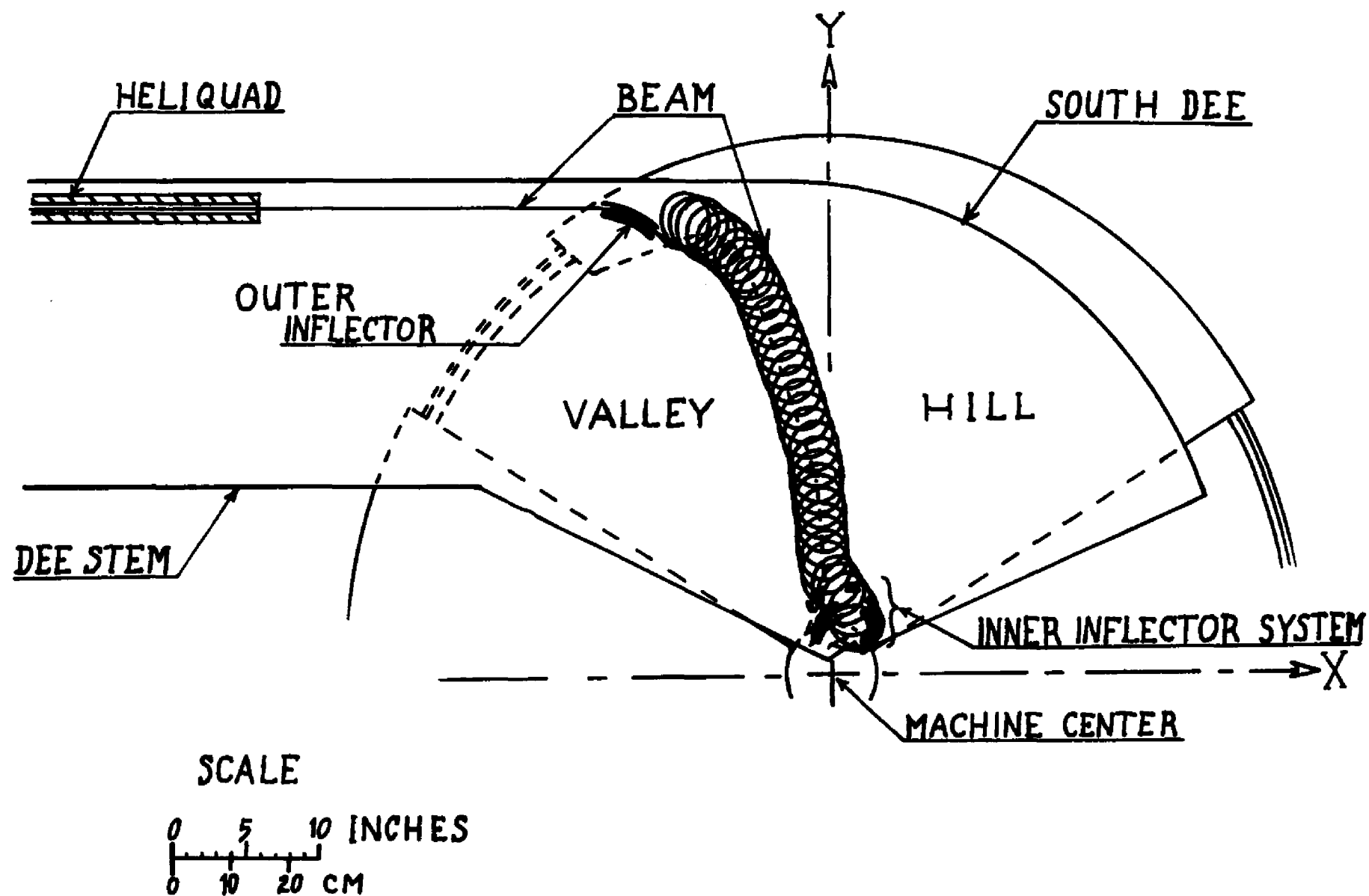
Fig. 2.2.--Cyclotron cross section with injection system.
