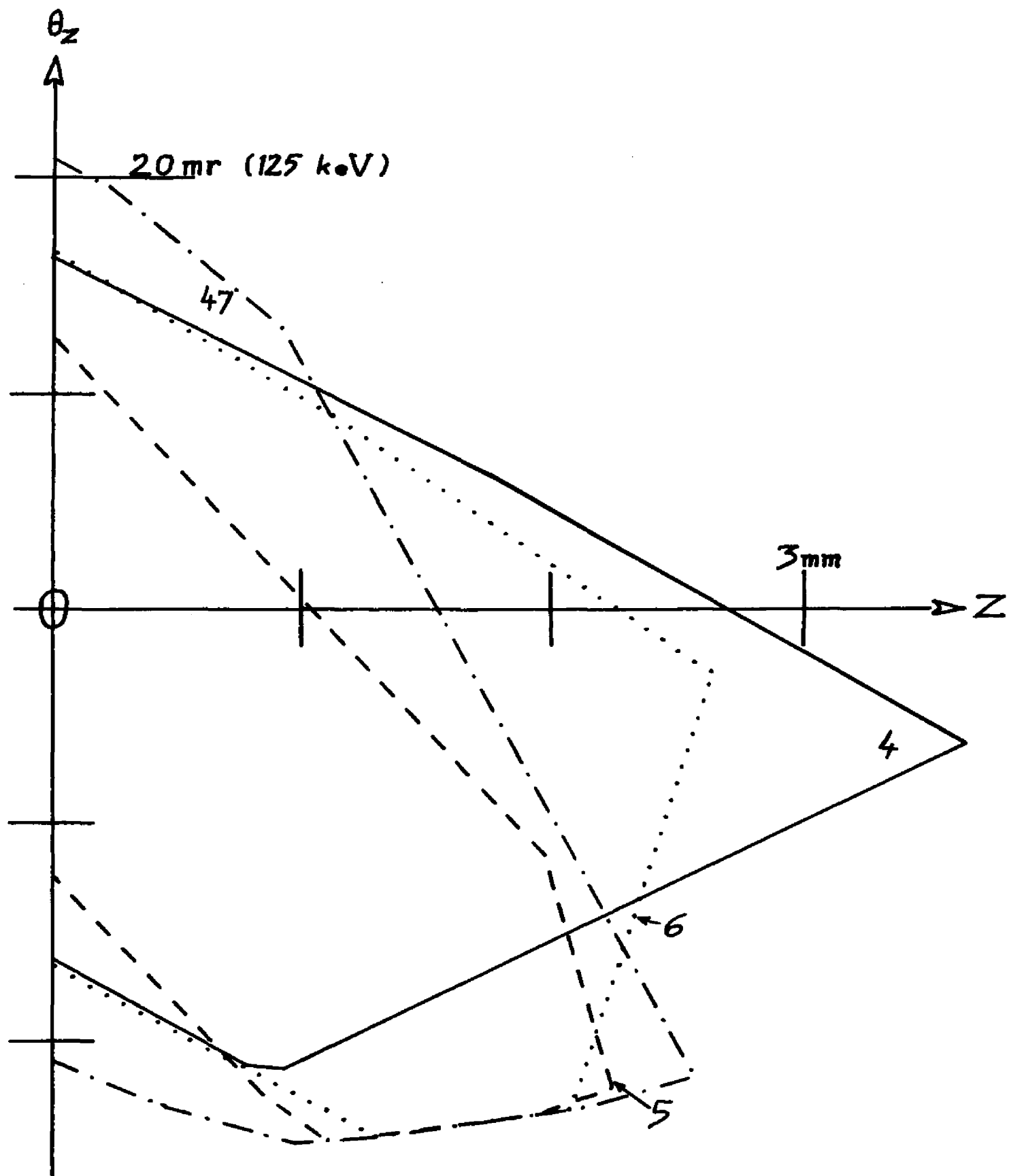
Fig. 4.3.--Vertical acceptances at the final inflector exit.
