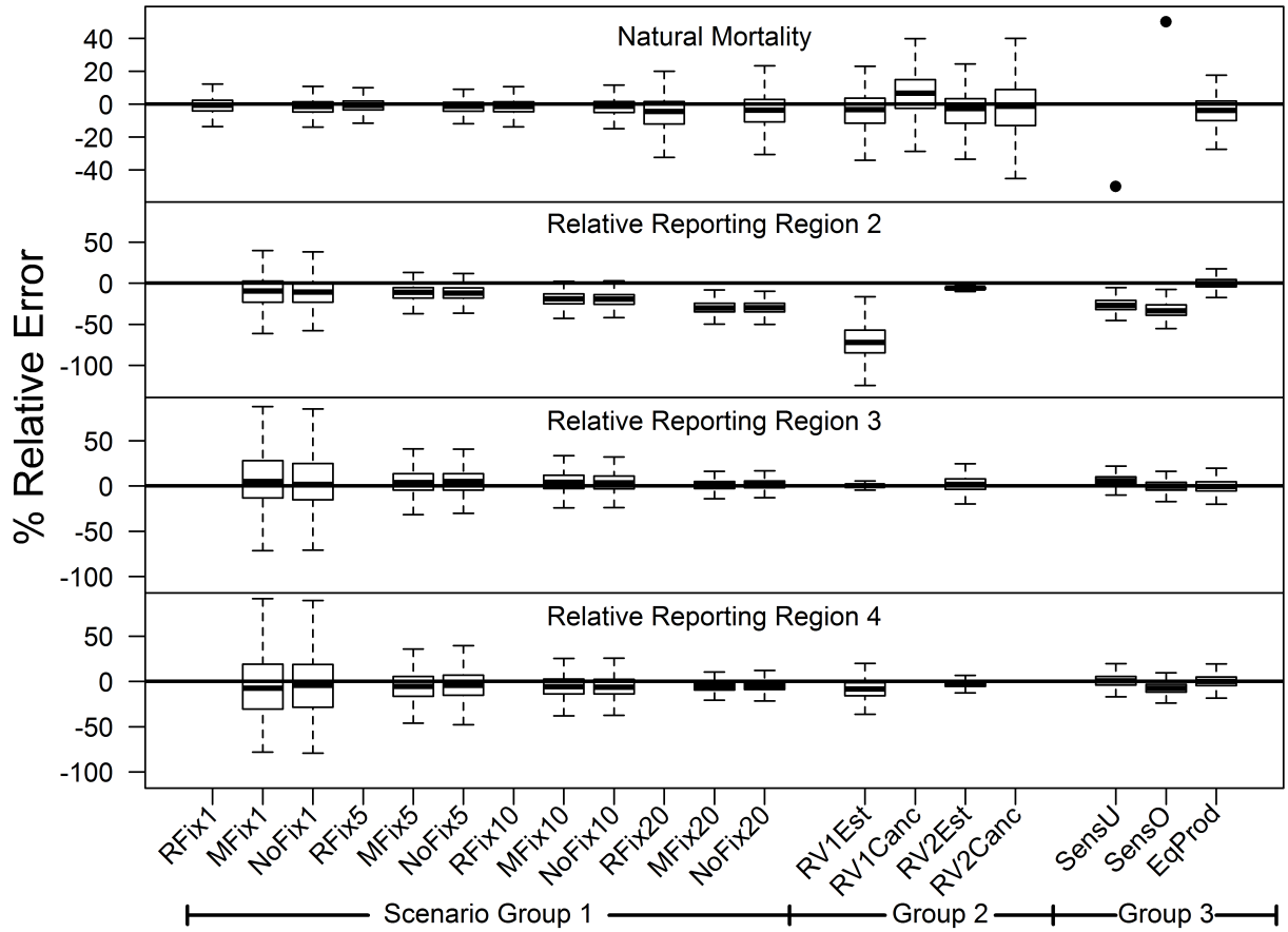
Figure 2.A.4: Relative Error (%) of relative reporting rates and natural mortality for a four region ITCAAN model under different intermixing rates and parameter estimation assumptions (Group 1), spatially varying reporting rates (Group2) and misspecification of natural mortality and equal productivities (Group 3) for 1000 simulation iterations. Table 2.A.2 lists the model abbreviations and corresponding model components. Dots indicate parameters that are fixed within the ITCAAN model at incorrect values. Whiskers on the boxplots extend to 1.5 times the interquartile range or the most extreme relative error, which ever is less extreme. Relative errors outside the whisker range were not plotted.
