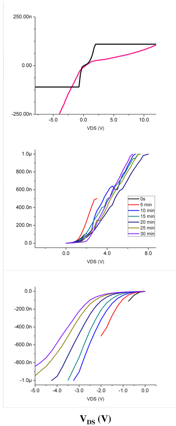
Figure 3.3 Characteristic shifts as a function of time for nanoFET2 under heavy ion radiation (a) Pre-rad to 0 second (b) forward bias and (c) reverse bias.
