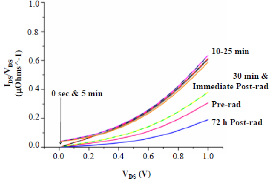
Figure 3.4 Nonlinear relationships between I_{DS}/V_{DS} versus V_{DS} observed for all data sets eliminated space charge limited model.
