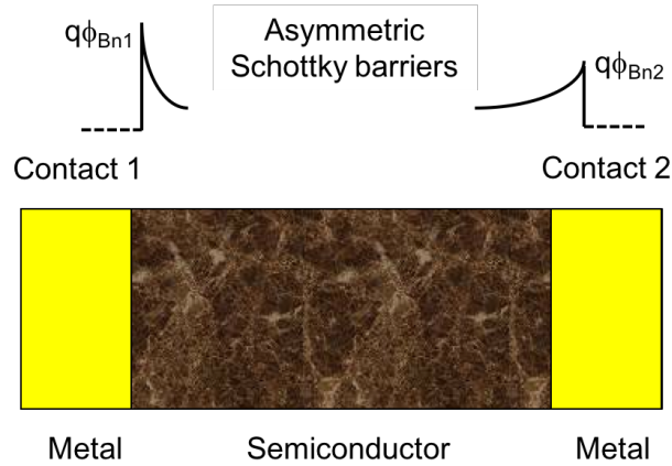
Figure 3.10 Metal-Semiconductor-Metal Structure with Asymmetric Schottky Barriers.
