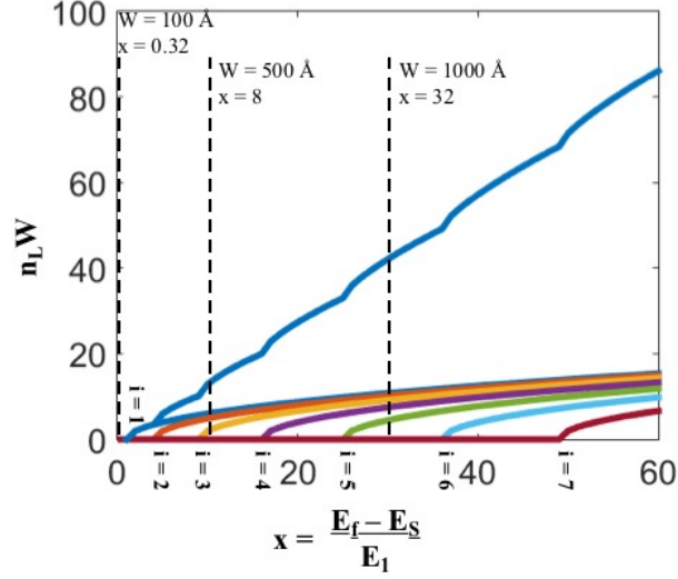
Figure 4.10 Normalized 1D electron number density. The number of channels available for transport has dropped from 5 to 3 to none as a function of the channel width.
