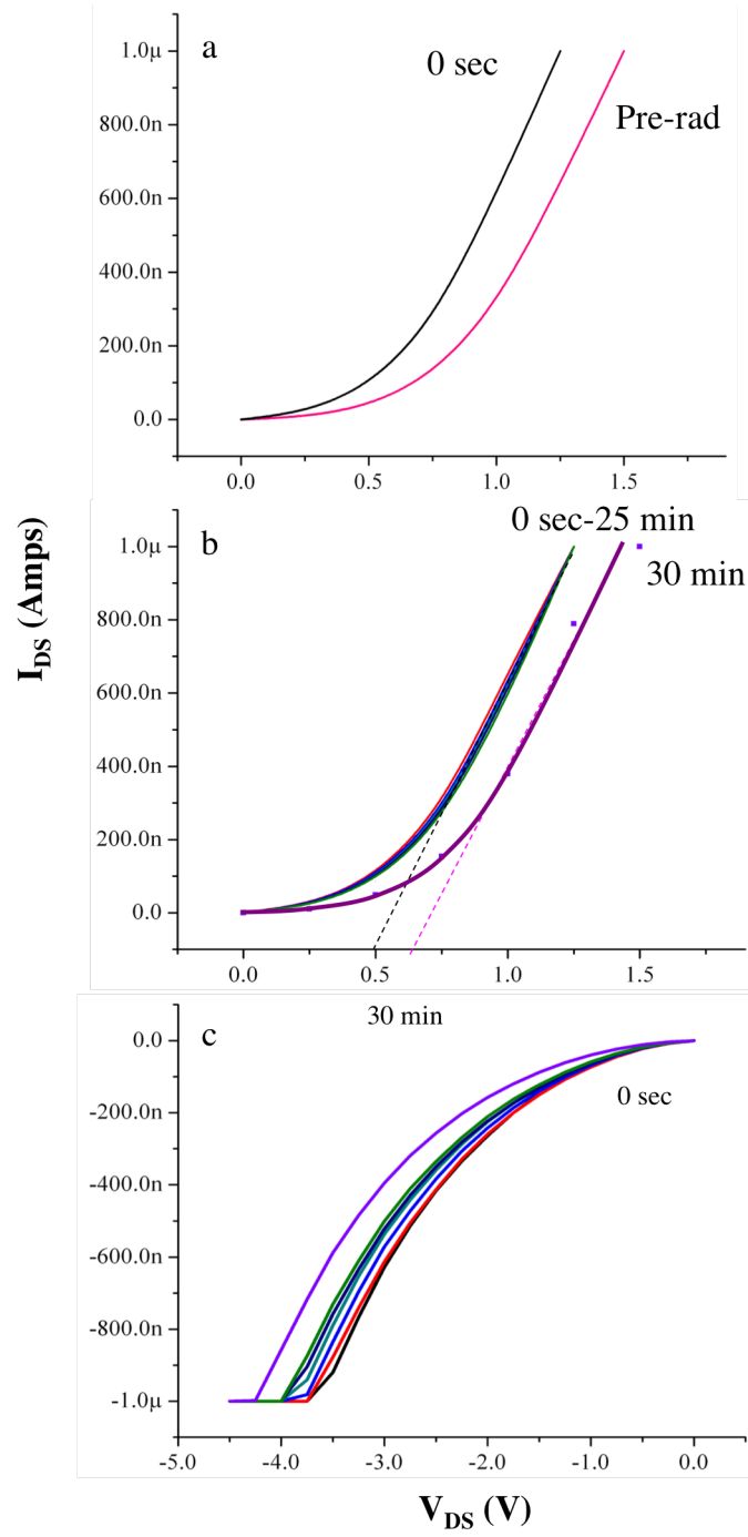
Figure 3.2 Characteristic shifts as a function of time for nanoFET1 under heavy ion radiation (a) Pre-rad to 0 second (b) forward bias and (c) reverse bias.
