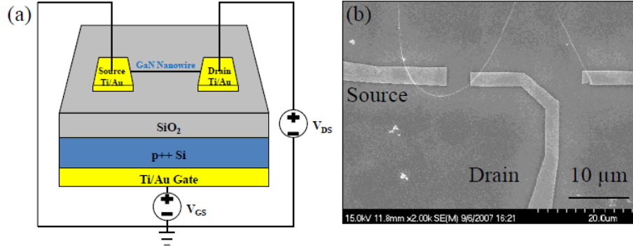
Figure 3.1 (a) NanoFET architecture and (b) top view SEM of EBL contacts and Nanowire taken by BW. Jacobs.
