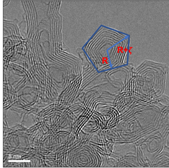
Figure 2.6 Diagram showing the measurement locations for R and \zeta with real HRTRM image example.
