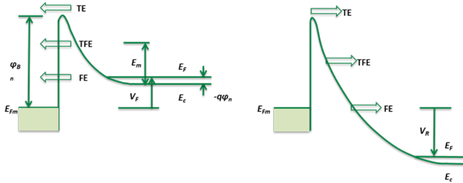
Figure 3.7 Energy-Band Diagram showing transport regimes through the reverse biased Schottky barrier.
