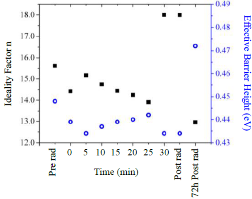
Figure 3.5 Ideality factors and scaled barrier heights from thermionic emission model.
