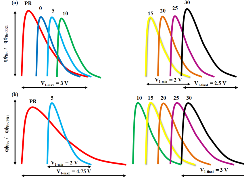
Figure 3.13 Effective barrier height and potential drop V_1 as a function of time in beam for (a) nanoFET1 and (b) nanoFET2. Barrier heights are accurately scaled to the nanoFET1 PR height (Table 1). The maximum (-max), minimum (-min) and final (-final) V_1 values are identified.
