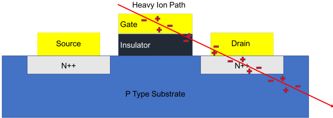
Figure 1.4 Heavy Ion Path in a n-type MOSFET, showing ion track through metal gate layer, insulator and metal drain, as well as the substrate layer.
