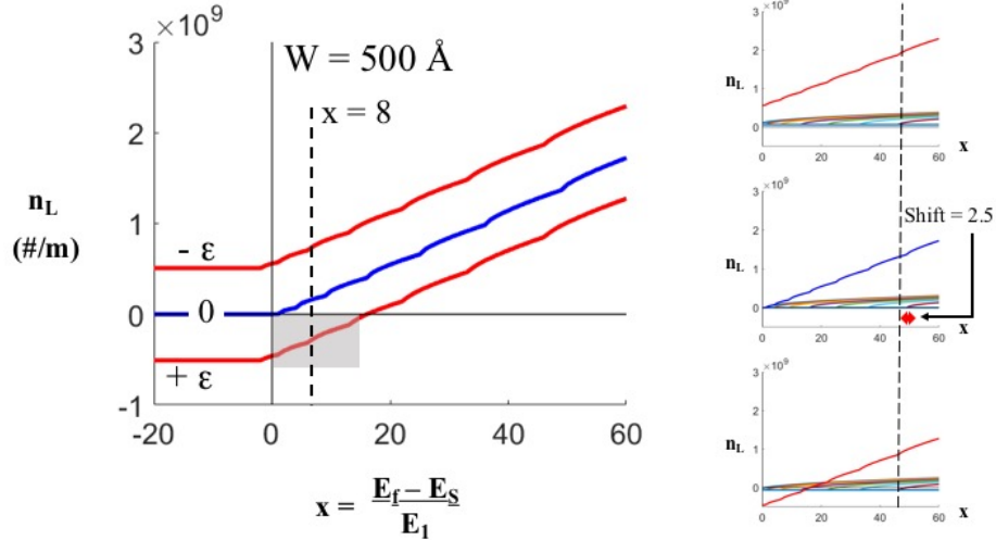
Figure 4.12 For width W = 500\text{\AA} , longitudinal perturbations shift the quantum staircase up or down by approximately by \pm\epsilon and towards lower normalized energy values by an amount 2.5, reducing the quantum channel accessibility, to 0 for the +\epsilon longitudinal perturbation, and changing the number density n_L allowed occupation.
