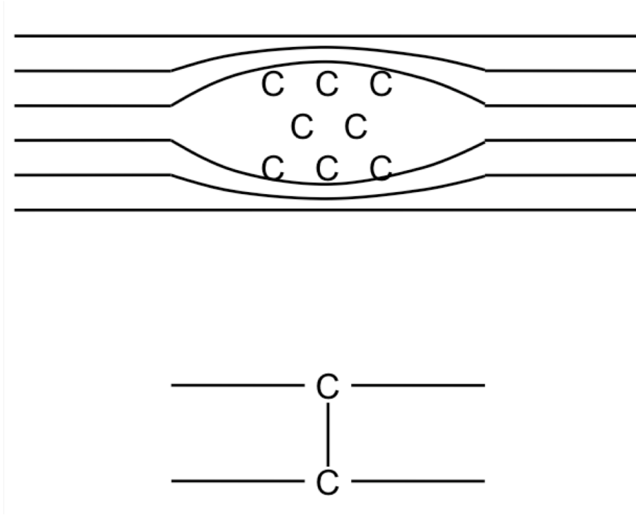
Figure 2.4 Classic knock-on collision creates free carbon atoms and vacancies in graphene layers. These amorphous regions or interstitial aggregates can coalesce to form local spot welds.
