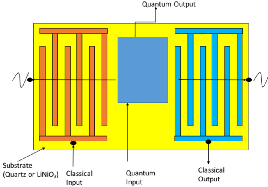
Figure 4.1 Solid State Quantum Relay Device. Qubit generation system is redacted and represented by blue box.
