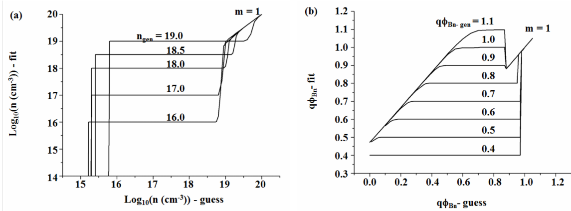
Figure 3.9 Ranges for which fitted results match generation value for (a) carrier concentration and (b) effective barrier height.
