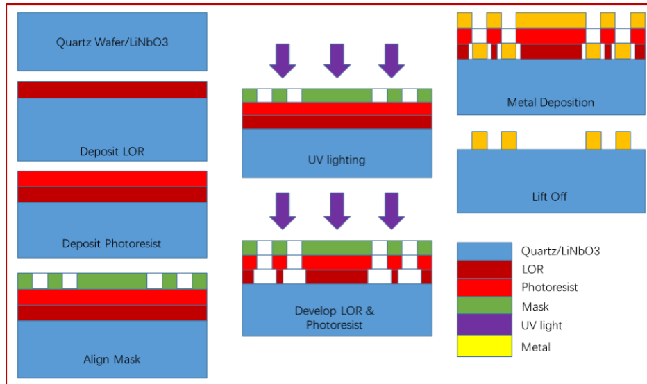
Figure 4.6 Fabrication Recipe for SAW device showing the process lift off using LOR layer.
