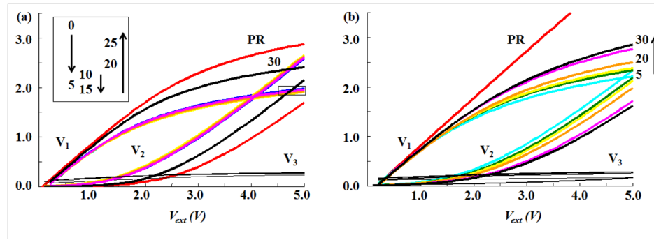
Figure 3.12 (a) Numerically solved potential drops V_1 , V_2 , V_3 as a function of V_{ext} and time in beam for (a) NanoFET1 and (b) NanoFET2. Closely spaced V_1 variation (box) are shown inset.
