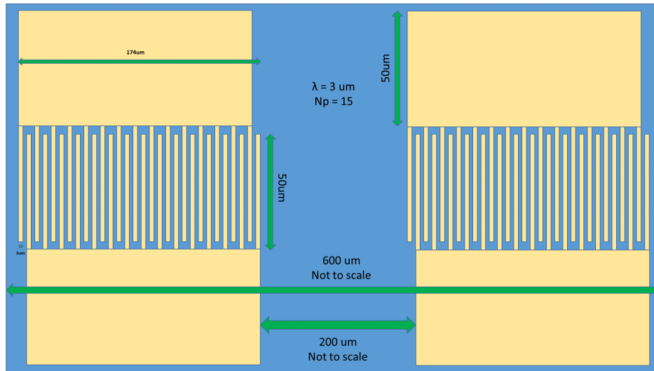
Figure 4.3 Designed SAW device with ( 3\mu\text{m} ) minimum feature and 15 IDT pairs.
