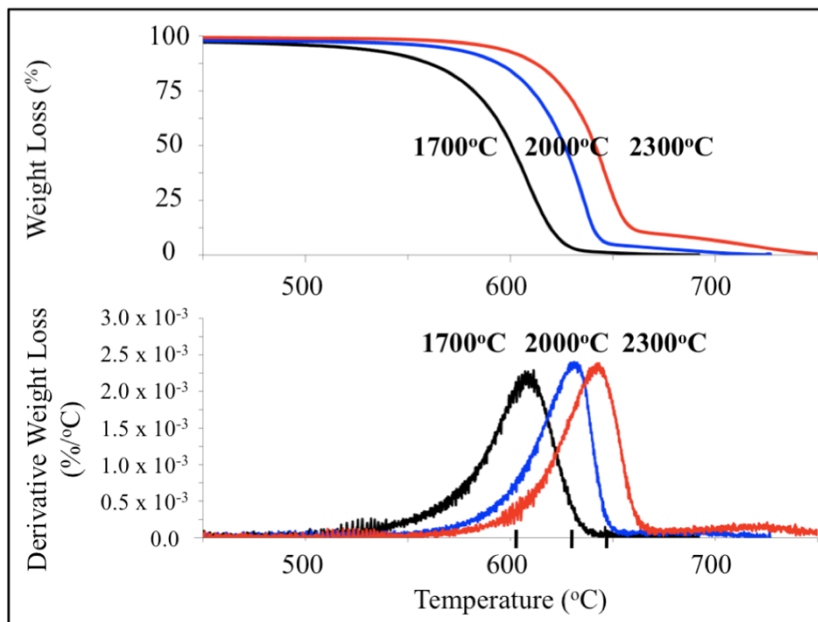
Figure 2.7 Thermogravimetric analysis of pre-irradiation carbon onion samples showed a nonlinear increase in ease of dissociation with increasing polygonal character.
