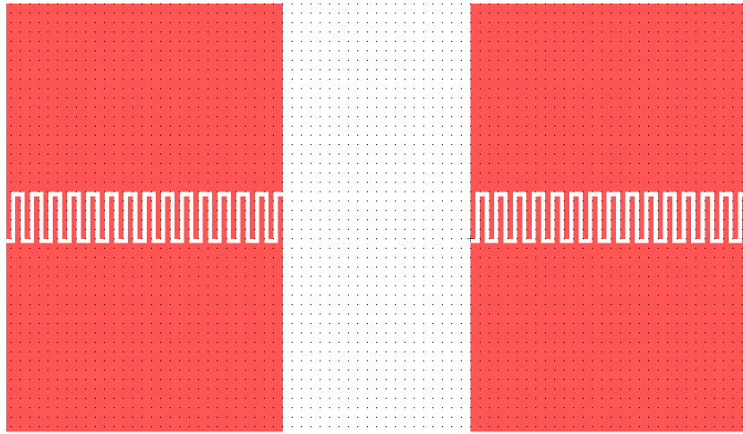
Figure 4.4 Mask design show ( 3\mu\text{m} ) minimum feature and 15 IDT pairs on a single layer.
