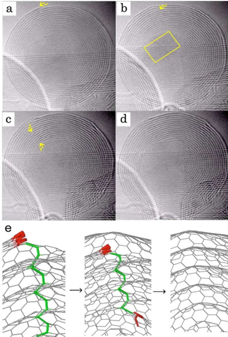
Figure 2.8 (a)-(d) In situ observation of dislocation annihilation. Arrows point out the dislocation edge. In (b), a cubic-diamond region is visible in the highlighted rectangle. (e) An atomic structural model of the annihilation process accompanied by unlinking of the shells. The atoms in dark gray (red) [light gray (green)] belong to the edge [screw] component of the dislocation loop. Image adapted from Ref [69]
