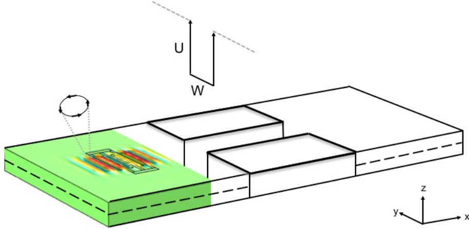
Figure 4.9 2D quantum well in z (dotted line) with additional width W dependent quantum well in y (inset above). GaAs response to propagating SAW wave includes both longitudinal and transverse components (inset above). Modeling is done by Kan Xie using COMSOL.
