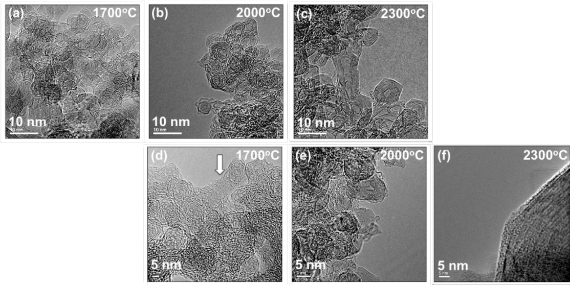
Figure 2.2 HRTEM images of carbon onions synthesized at temperatures 1700 °C, 2000 °C and 2300 °C for (a-c) pre and post (d-f) irradiated by 140 MeV/u argon-40.
