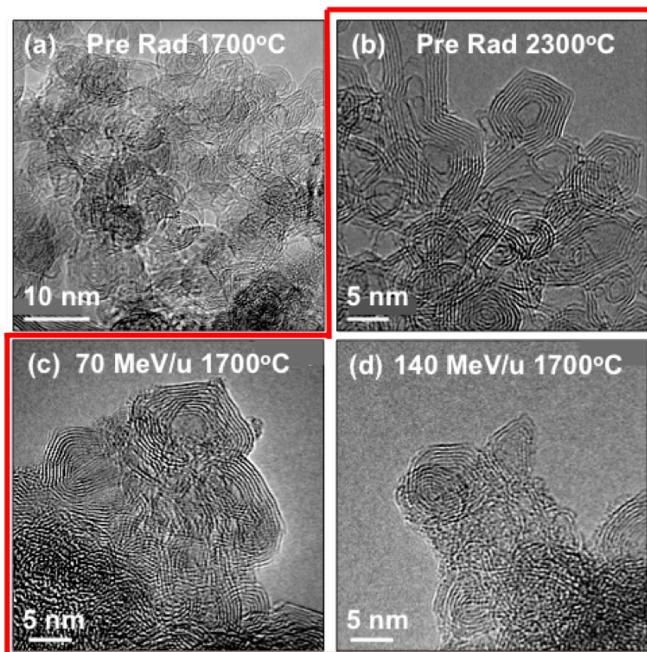
Figure 2.3 Pre-irradiation carbon onions synthesized at (a) 1700 °C and (b) 2300 °C. Post irradiation 1700 °C carbon onions at irradiation energies of (c) 70 MeV/u and (d) 140 MeV/u calcium-48 resemble 2300 °C pre-irradiation carbon onions.
