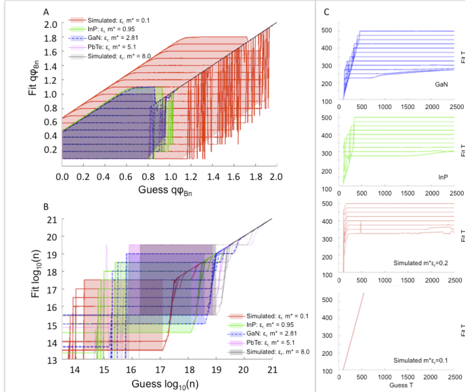
Figure 3.14 Graph show the stable fitting range for A) Barrier height B) Carrier Concentration and C) Temperature with varying material type.
