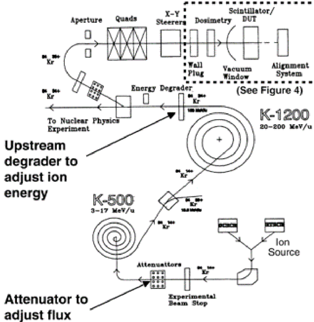
Figure 1.2 Particle acceleration process at NSCL, with smaller K500 accelerator followed by K1200 accelerator, beam path is shown before they are sent to each vault. Image Credit: R Ladbury et al. IEEE T. Nucl.Sci.51,3664 (2004)
