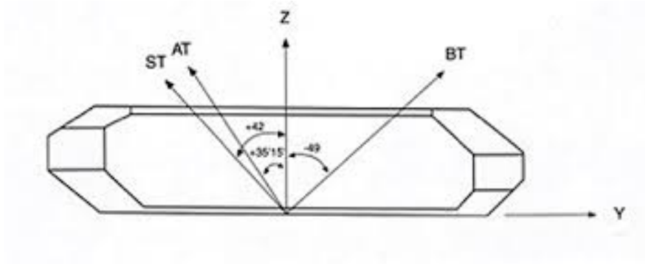
Figure 4.2 Standard crystal cut orientation on a quartz crystal. Image Credit: MEC Quartz Crystal[115].
