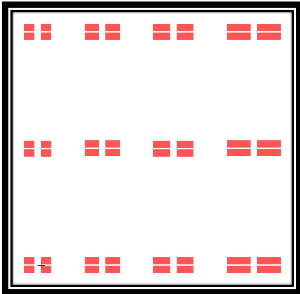
Figure 4.5 Full Mask Design showing all twelve devices on a single wafer surface.
