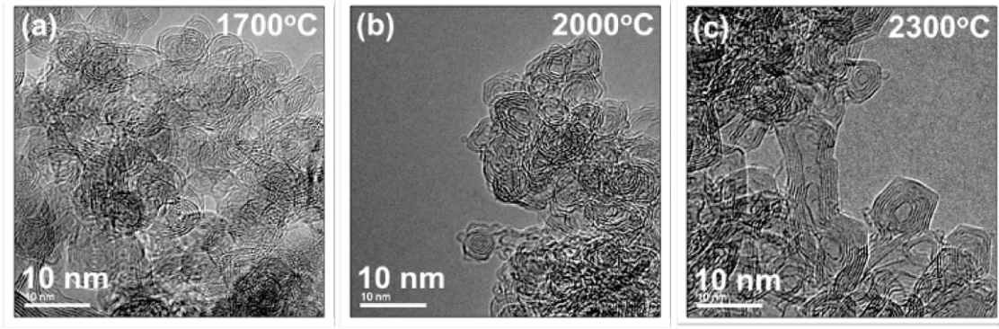
Figure 2.1 HRTEM images of carbon onions synthesized at temperatures 1700 °C, 2000 °C and 2300 °C (a-c).
