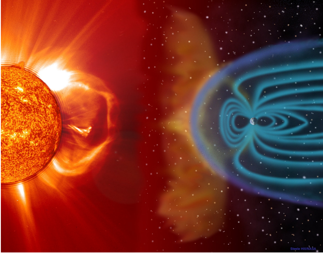
Figure 1.1 Demonstration of the dynamic radiation environment in Low Earth Orbits. Image credit: NASA
