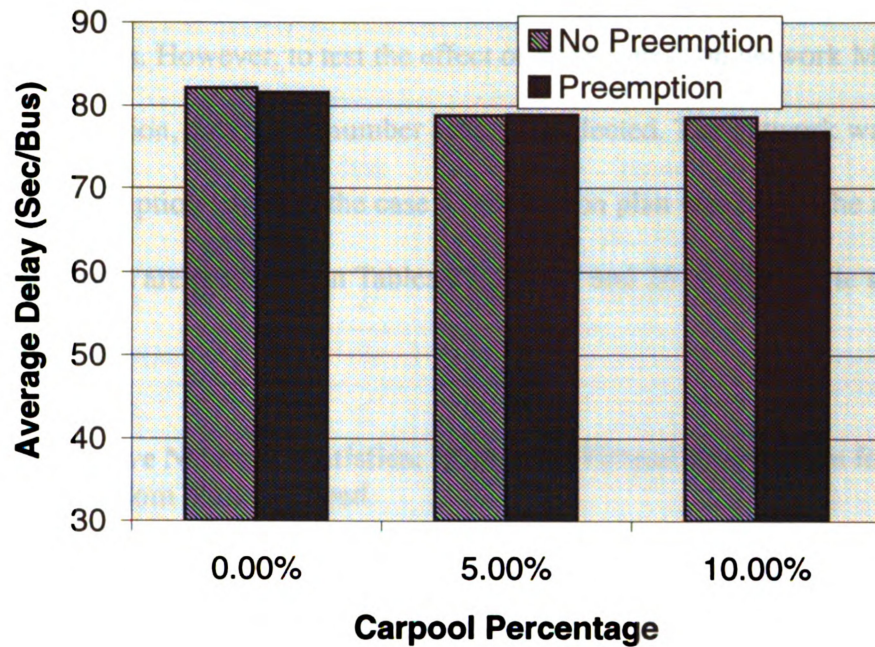
Figure 22: Total Links Bus Delay
