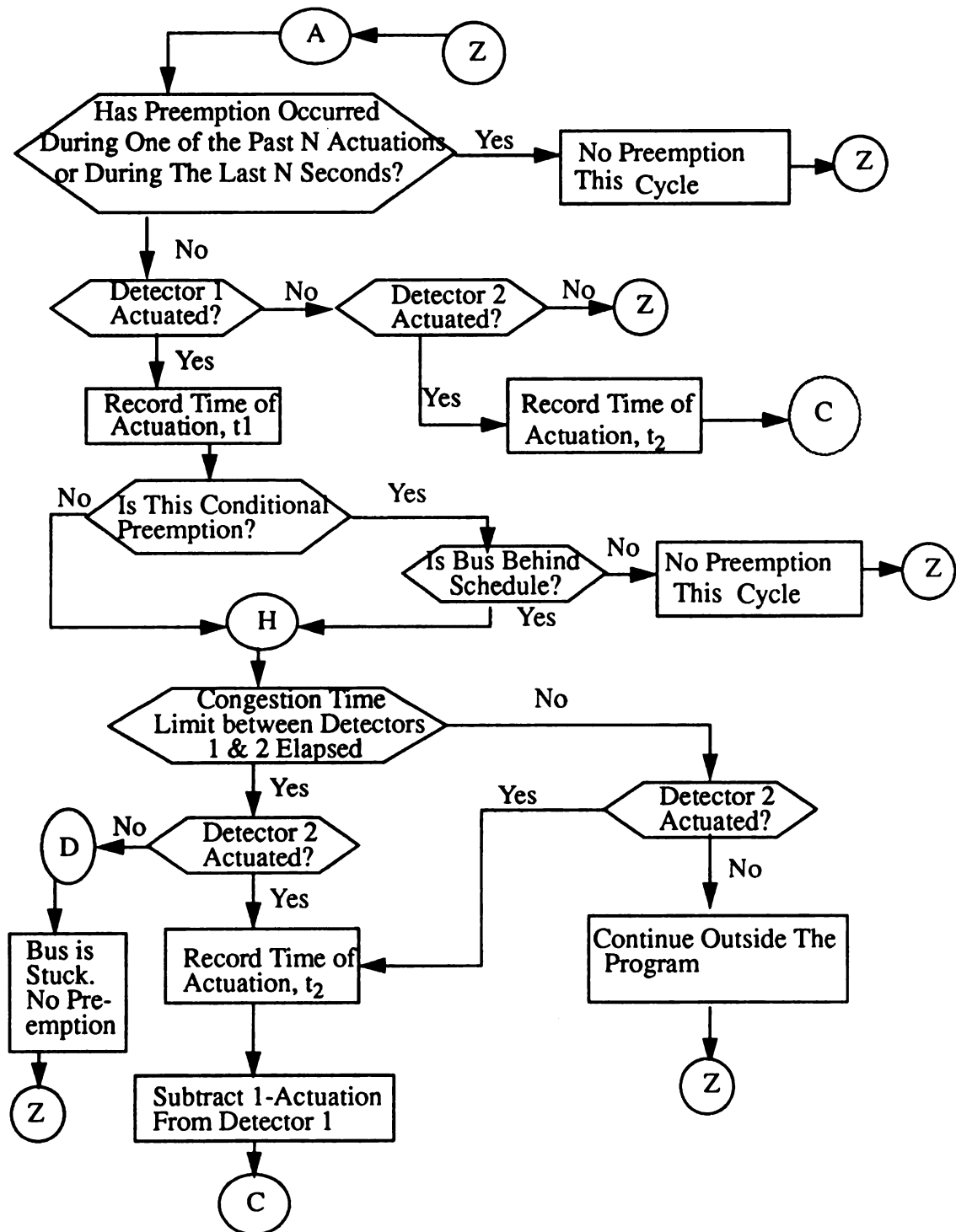
Figure B-1: Far-Side Bus-Stop BPS Algorithm
