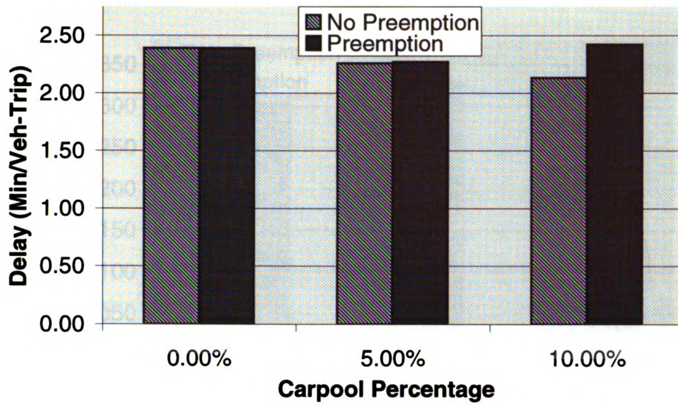
Figure 18: Cumulative Network Delay
