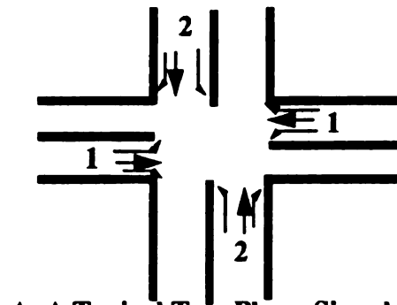
A. A Typical Two-Phase Signal
