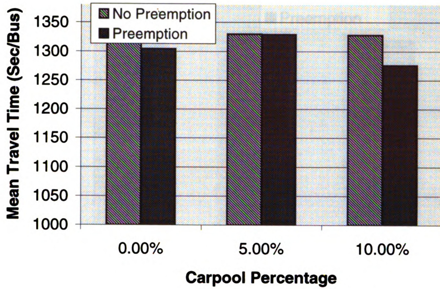
Figure 20: Bus Route 1 Mean Travel Time
