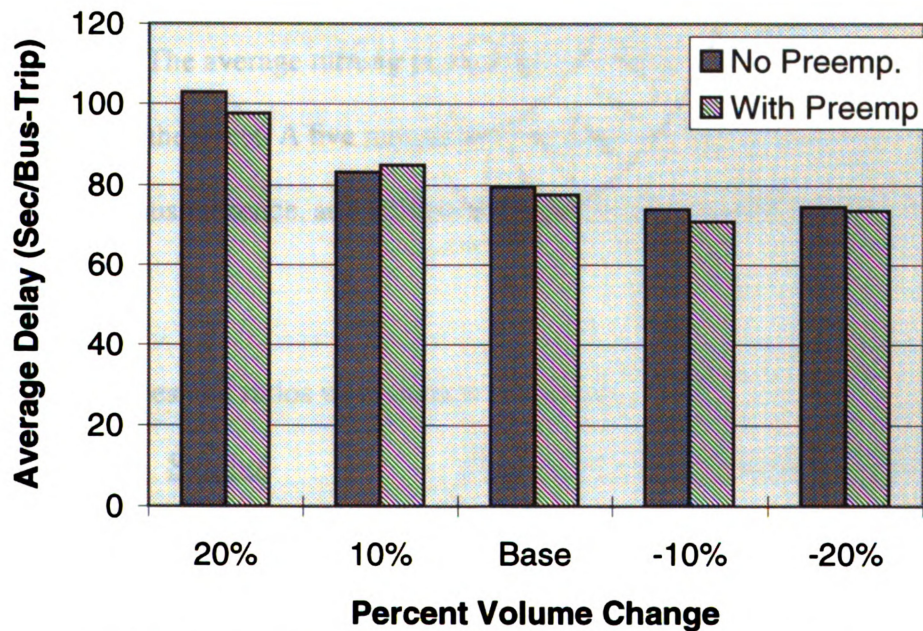
Figure 9: Total Link Bus Delay Due to Volume Change
