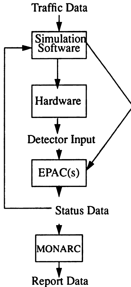
Figure 1: Automatic Signal / Eagle Signal BPS work plan
