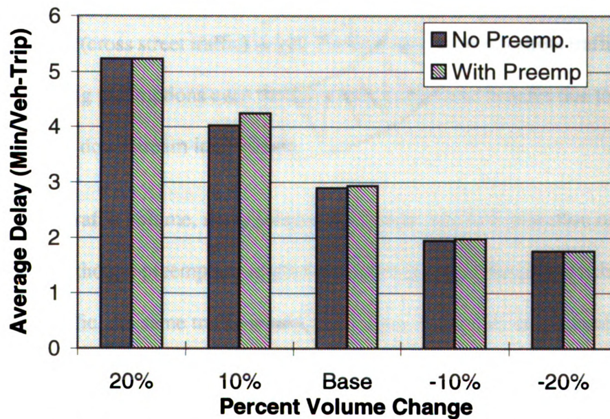
Figure 8: Network Average Delay Due to Volume Change
