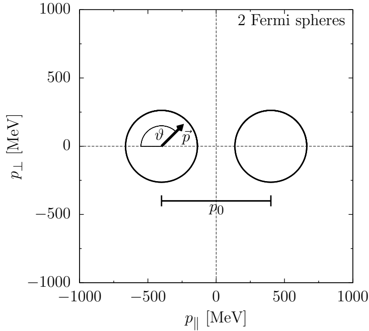
Figure 2.1: Situation within the local rest frame of 2 Fermi spheres separated by p_0 = 800 MeV in p -space.
