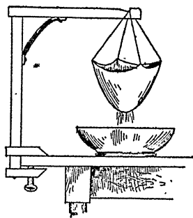
Percolator Holder.
